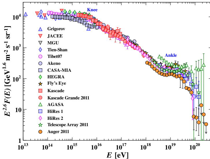
Figure 3.5.: Measured all-particle spectrum of the primary cosmic-rays [42]. The spectrum follows a power law, where dN/dE \propto E^{-2.7} up to energies around 1 PeV, where it becomes steeper dN/dE \propto E^{-3} . This feature is called the "knee". Around 4 \times 10^6 \text{ TeV} the spectrum becomes harder again, so-called "ankle". Finally at the highest energies the spectrum is suppressed due to the interaction with the cosmic microwave photons (GZK cutoff).
