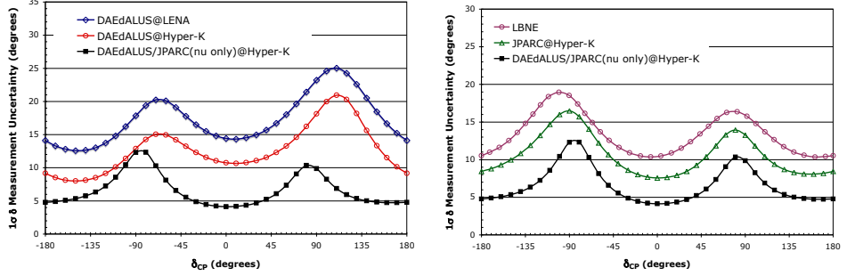
Figure 4.11.: The estimated 1\sigma uncertainties of the Daeδlus approach for the measurement of CP violation phase along with the proposed LENA and Hyper-Kamiokande detectors and impact of combining the result with the long baseline beam from J-Parc to Hyper-Kamiokande. [105]
