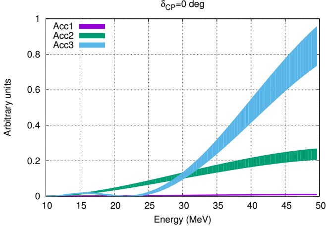
Figure 11.4.: The spread in the energy spectra of the events caused by the uncertainties of other oscillation parameters than the CP violation phase ( \delta_{CP} = 0 ). Different bands show the spread associated to cyclotrons with baselines of 1.5 km (magenta), 8 km (green) and 20 km (cyan), respectively.
