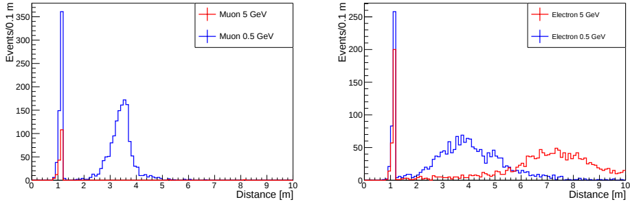
Figure 10.6.: Extracted location of the point with the highest backtracking value with respect to the location of the initial vertex for particles with energy of 0.5 GeV and 5 GeV. The left panel shows the result for muons and the right panel for electrons.
