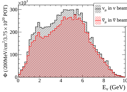
Figure 3.9.: The estimated energy spectrum of muon neutrinos for the proposed CERN to Pyhäsalmi beamline studied in the LAGUNA-LBNO design study. [54]
