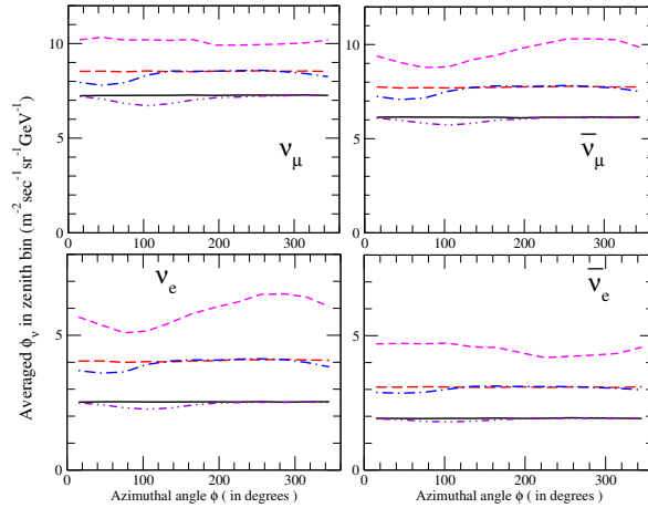
Figure 3.7.: The azimuthal angle dependence of atmospheric neutrino flux, averaged over zenith angle bins of 1 > \cos \theta > 0.6 (solid line), 0.6 > \cos \theta > 0.2 (long dashed), 0.2 > \cos \theta > -0.2 (short dashed), -0.2 > \cos \theta > -0.6 (dashed-dotted), and -0.6 > \cos \theta > -1 (dashed double-dotted), calculated for the Pyhäsalmi site at (anti)neutrino energy E = 3.2 GeV. [44]
