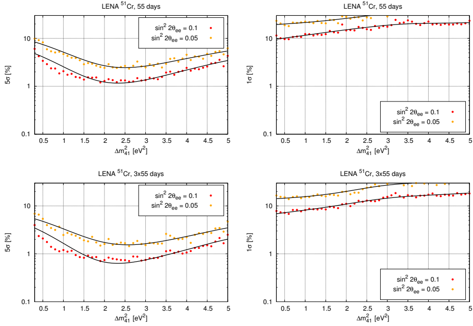
Figure 9.10.: Sensitivity reaches for \Delta m^2_{14} (left) and \sin^2 2\theta_{14} (right) in the case of a ^{51}\text{Cr} source with exposures of 1 \times 55 days (top) and 3 \times 55 days (bottom). The black curves are only to guide the eye.
