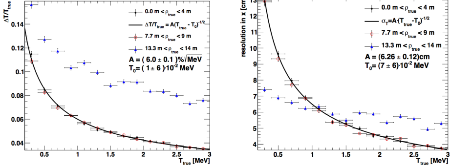
Figure 6.7.: The energy and position resolution as a function of kinetic energy of the electron obtained from the point-fitting algorithm [129].
