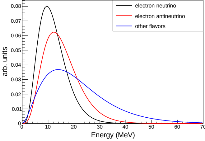
Figure 3.4.: Example of estimated energy spectra for different neutrino flavors in core-collapse supernovae. Parameterisation of Lawrence Livermore group is used. [40]
