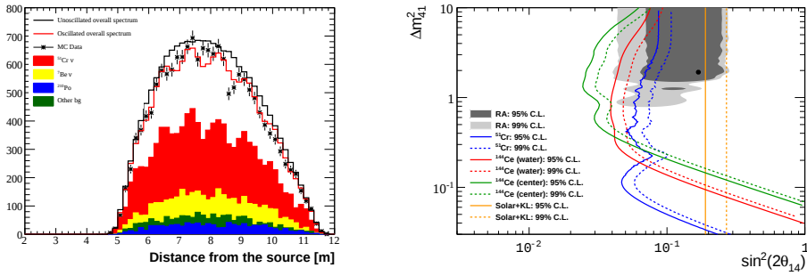
Figure 4.18.: Sterile neutrinos with Borexino-SOX [120]. Left panel: The illustration of spatial event distribution and its components in Borexino-SOX experiment with ^{51}\text{Cr} source ( \sin^2 2\theta_{14}=0.3 , \Delta m_{41}^2=2 \text{ eV}^2 ). Right panel: Estimated sterile neutrinos sensitivity for external ^{51}\text{Cr} and the ^{144}\text{Ce} - ^{144}\text{Pr} source deployed in the volume water buffer (muon veto) or in at the centre of the scintillator vessel in Borexino.
