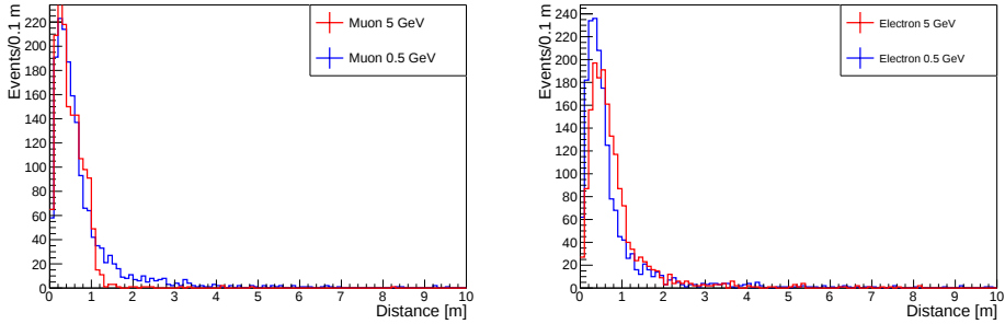
Figure 10.10.: The closest distance from fitted line to the true initial vertex position. The left panel shows the results for muon with energy of 0.5 GeV and 5 GeV. The right panel is for electrons with same energies.
