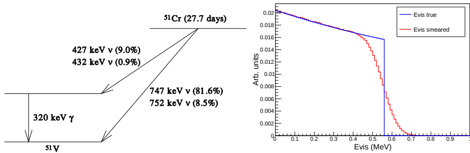
Figure 9.2.: Neutrino production of ^{51}\text{Cr} . Left: Decay scheme of ^{51}\text{Cr} . Right: Visible energy spectrum of recoil electron from 750 \text{ keV } \nu_e - e scattering
