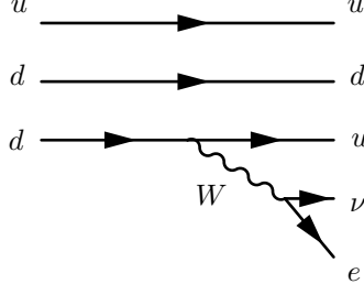
Figure 2.2.: The Feynman diagram of \beta decay.
