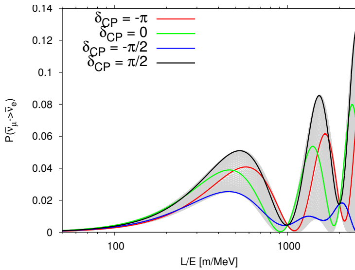
Figure 11.2.: The oscillation probability P(\bar{\nu}_\mu \rightarrow \bar{\nu}_e) as a function of L/E for the CP phase values \delta_{CP} = \pi/2, 0, -\pi/2, -\pi . The shaded area corresponds \delta_{CP} varying in the range from -\pi to +\pi .
