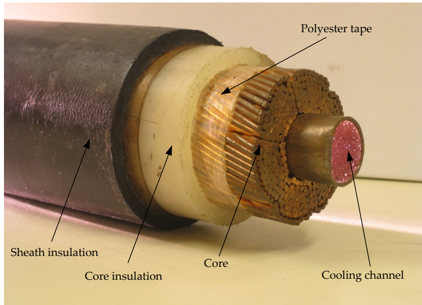
Figure 8.3: Water-cooled conductor with flexible copper core and copper pipe as cooling channel. This layout offers a certain flexibility, but cooling capacity is limited.
