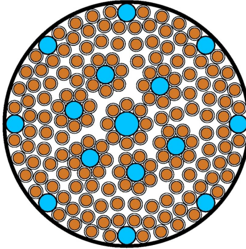
Figure 8.4: Cross-section of the conductor used for magnet coils in the MINOS detector. The larger diameter circles represent the copper cooling channels. The smaller circles are the copper conductor core. The outer circumference is a copper jacket directly cooled by eight cooling tubes (image source: [NK99]).
