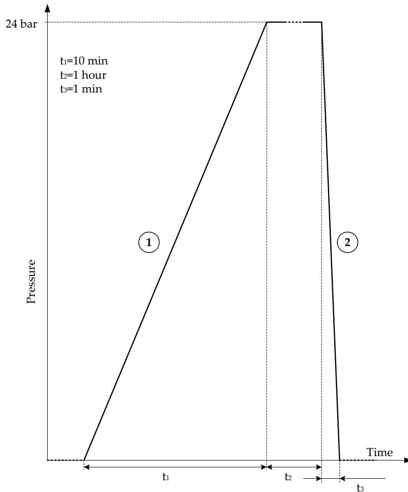
Figure 7.2: Pressure pattern during initial test.
