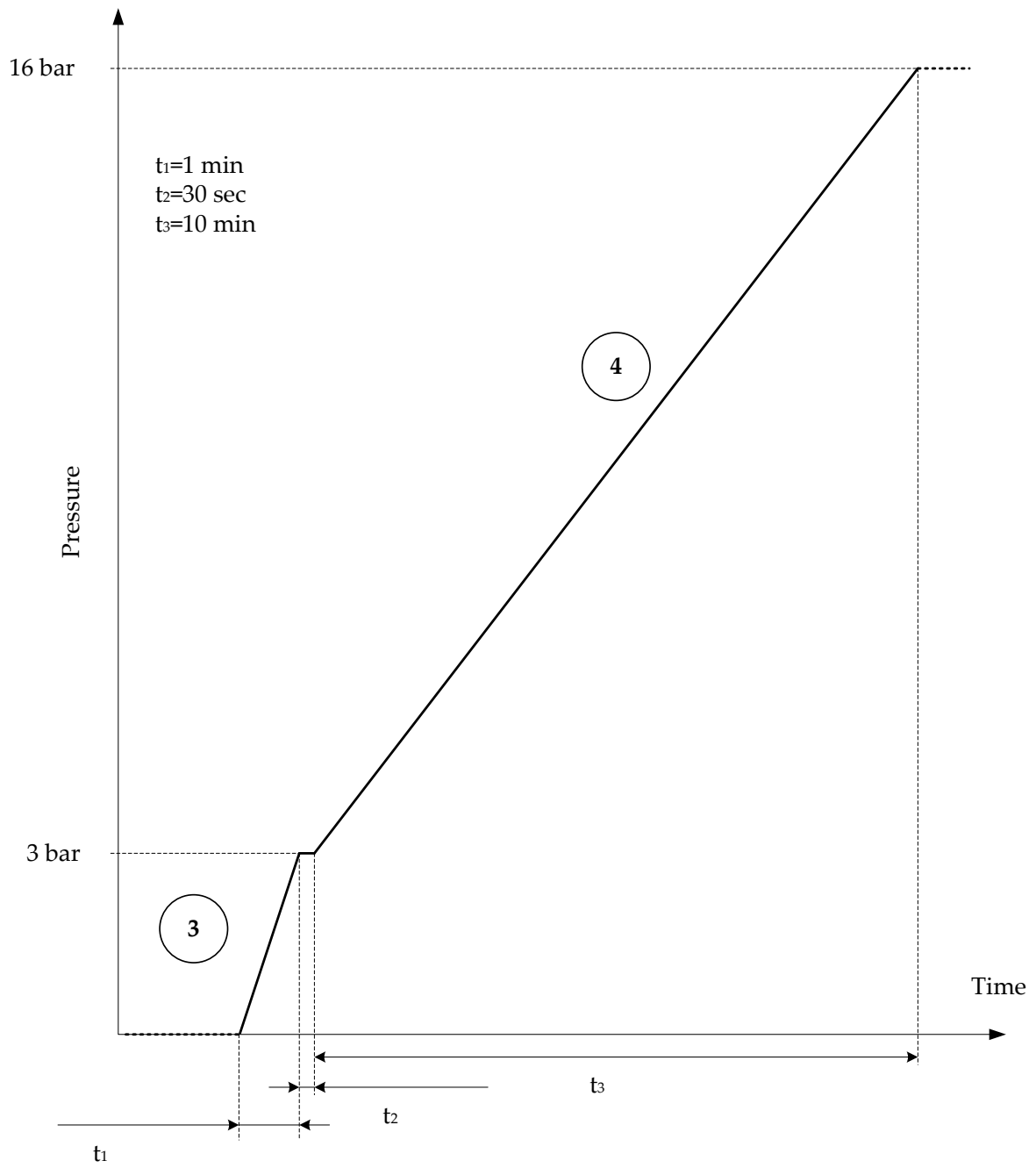
Pressure pattern during commissioning
