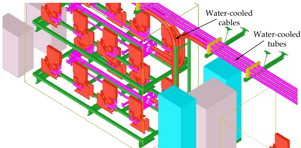
Figure 8.1: CAD-drawing of water-cooled cables and tubes in the LHC. Tubes are used to cover the straight sections, whereas flexible cables are utilized in areas involving bends (image source: CERN internal).
