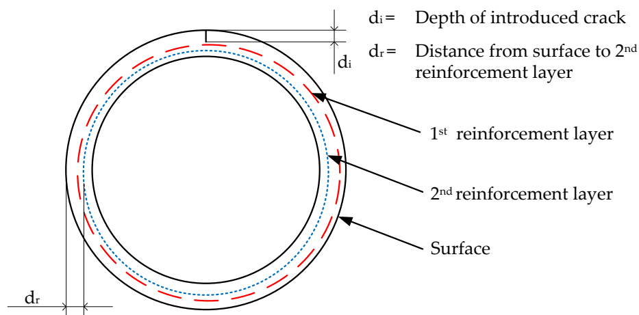
Figure 6.6: Cross-section profile of water-cooled cable hose 2 . Note the excentric alignment of the two reinforcement layers.
