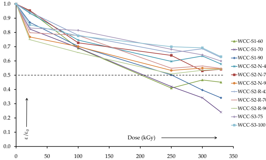
Figure 9.4: Relative elongation \epsilon/\epsilon_0 at F_{max} .
