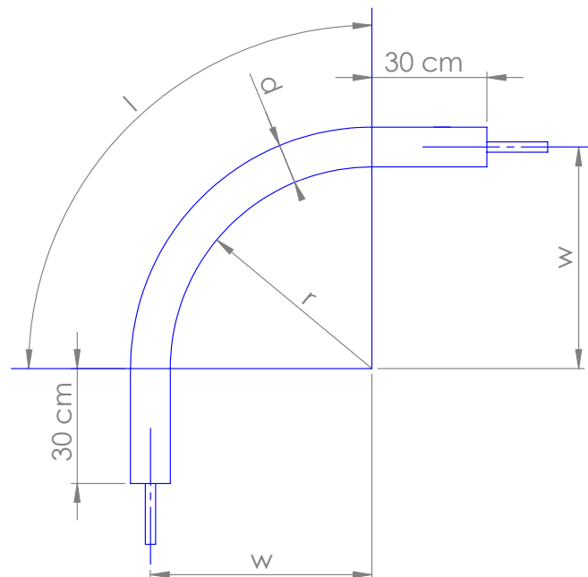
Figure 7.6: Sample bent through 90^\circ .
