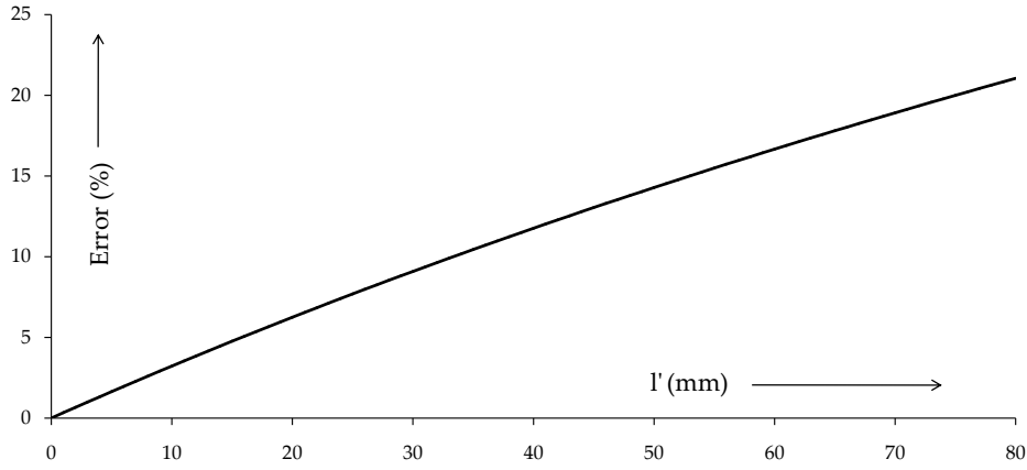
Figure 6.4: Error due to perspective distortion for a camera distance l = 300 mm and an increasing offset distance l' .
