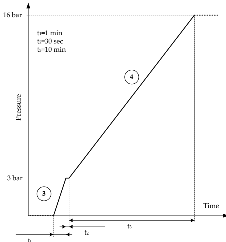
Figure 7.3: Pressure pattern during commissioning.
