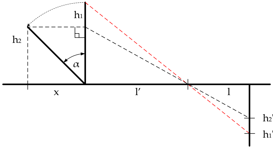
Figure 6.1: Geometric principle of measurement error due to angular misalignment. The object appears reduced in size, depending on the misalignment angle \alpha .
