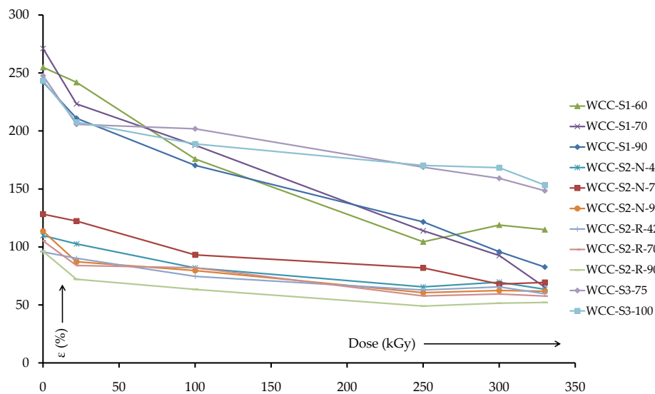
Figure 9.3: Elongation of hose samples at F_{max} . With radiation dose rising, the rubber embrittles and elasticity is decreased. The three “bunches” of curves clearly can be assigned to the three manufacturers.
