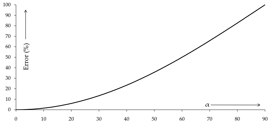
Figure 6.2: Error due to an angular misalignment of the object plane to the image plane. The error increases with the misalignment angle \alpha . At an angle of 90°, the object becomes completely invisible.
