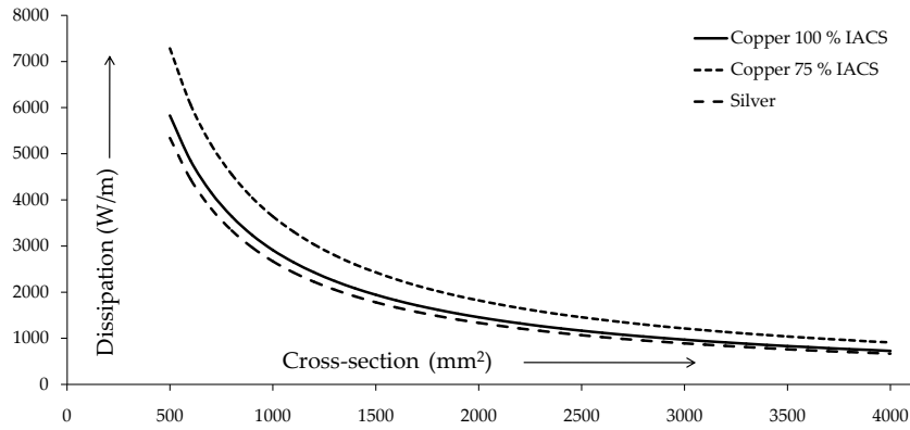
Figure 8.2: Power dissipation per metre for different conductor materials at a current of 13 kA (temperature dependence is ignored).
