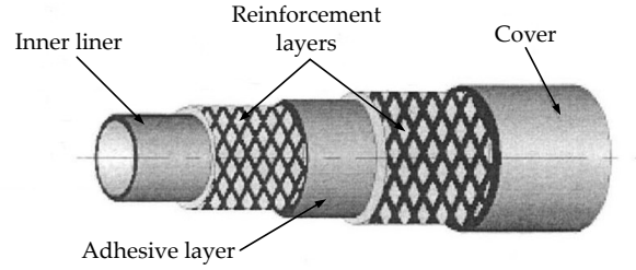
Figure 3.2: Layers of cable hose (image source: [Wyd09]).
