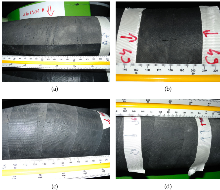
Figure 4.2: Different crack types: transversal cracks (a), longitudinal cracks (b), combination of transversal and longitudinal cracks (c), other (d).
