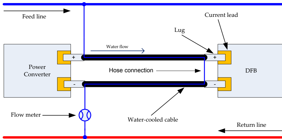
Figure 3.3: Connection pattern between power converter and DFB. Note that both electrical and water connection are established by the lug of the water-cooled cable. Cooling water from the feed line flows through the first cable and is then routed to the second cable by a hose connection. After passing the second cable, it is fed back to the return line. Water flow during operation is monitored with a flow meter (water flow symbolised by the blue line).
