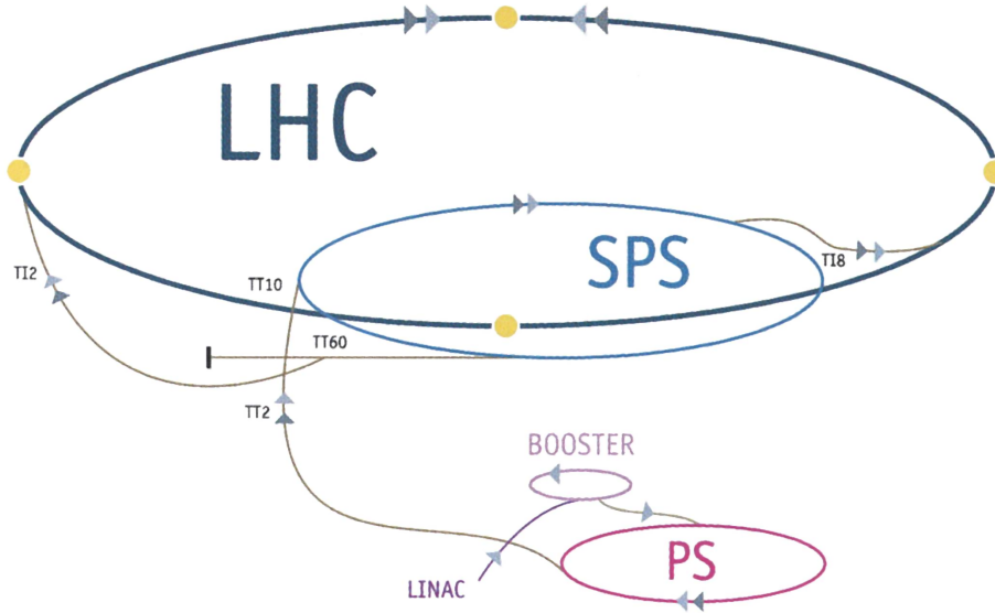
Figure 1.1: Particle accelerator complex at CERN: After initial acceleration in LINAC, particles are further accelerated in the Booster (PSB), passed into the PS and then delivered to the SPS. Finally, they are injected into the LHC. The Figure illustrates the accelerator chain for protons, so LEIR is not shown (image source: [Eva09]).
