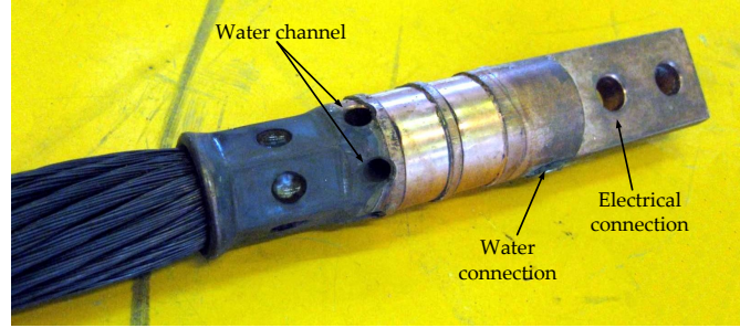
Figure 3.1: Copper core and lug of water-cooled cable. The lug ensures both electrical and water connection. Cooling water is piped to the flexible conductor by water channels.
