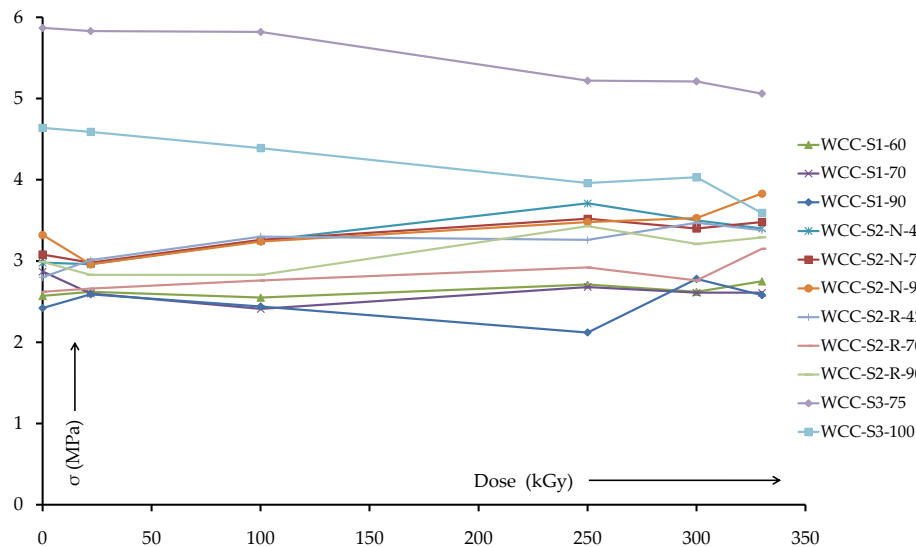
Figure 9.2: Tensile strength of hose samples.
