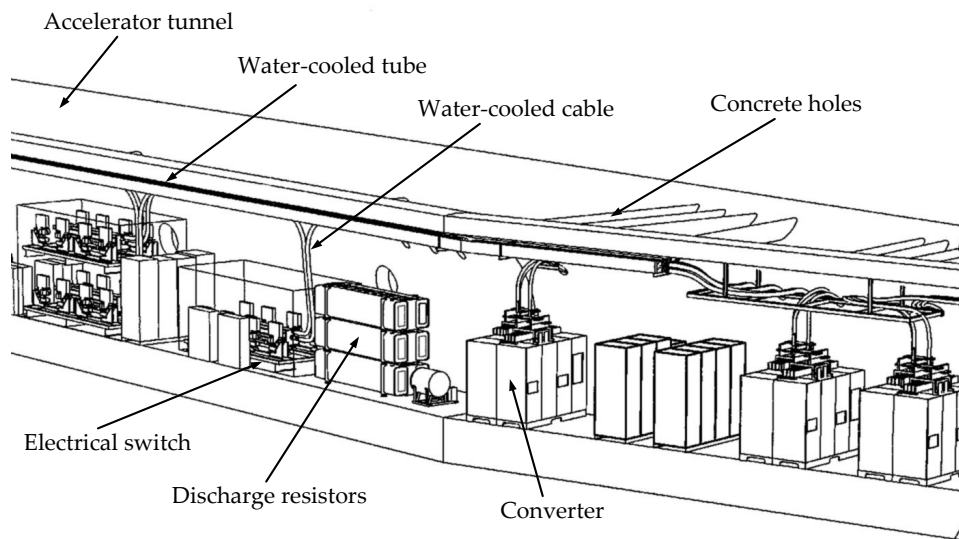
Figure 3.4: Example of water-cooled cable installation. The cables are routed through concrete holes to the DFBs which are located in the accelerator tunnel (image source: [CER03]).
