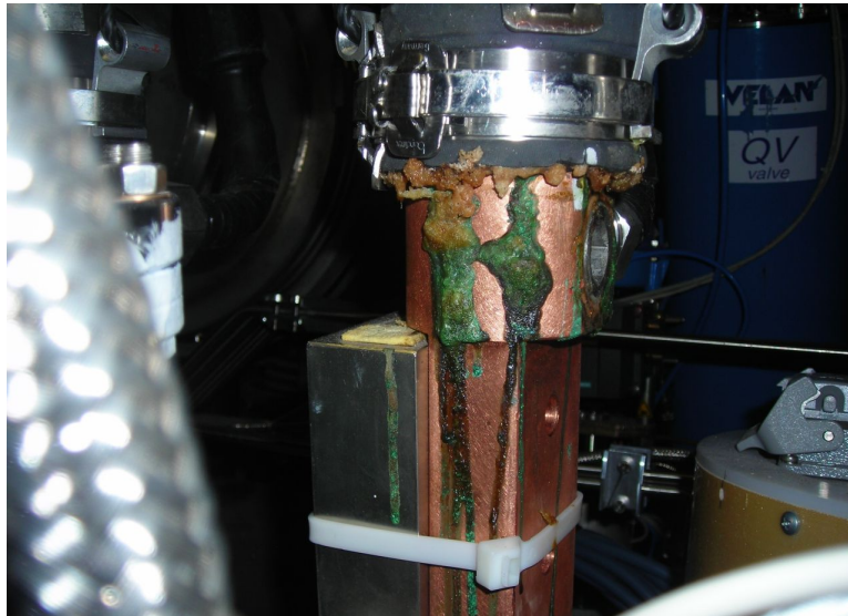
Figure 4.1: Copper oxide on the lug of a water-cooled cable. The connector corroded due to chlorine released from the adhesive layer of the rubber hose.
