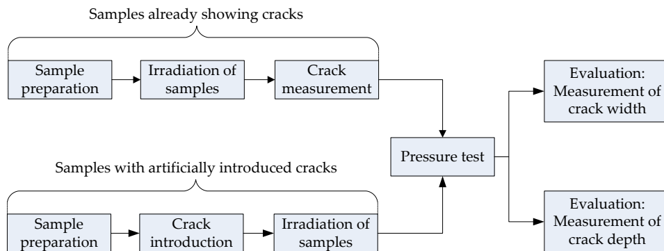
Figure 7.1: Radiation and pressure test procedure.
