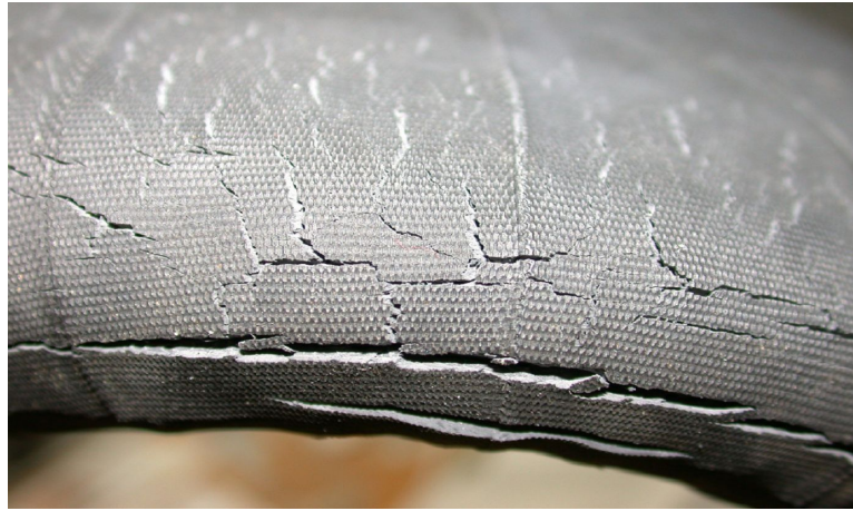
Figure 3.7: Hose sample after 312h exposure to an ozone concentration of 200 pphm O_3 at 40 °C and 55 % relative humidity (image source: [Wyd08a]).
