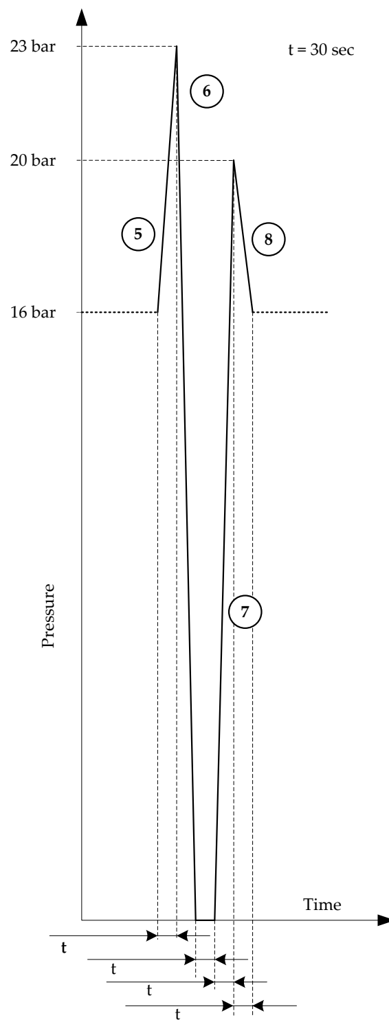
Figure 7.4: Pressure pattern during maintenance of the hydraulic system.
