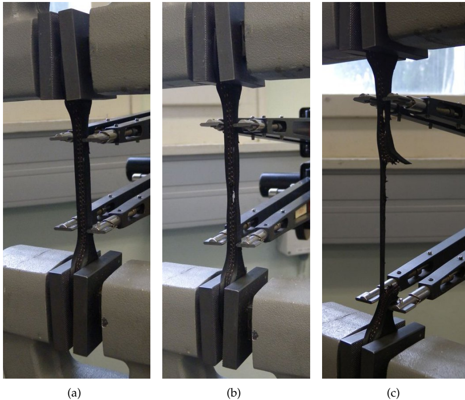
Figure 9.1: Tensile test of water-cooled cable hose: Elastic deformation (a), peak level of tensile force has been achieved and sample starts to break (b), end of the tensile test (c).
