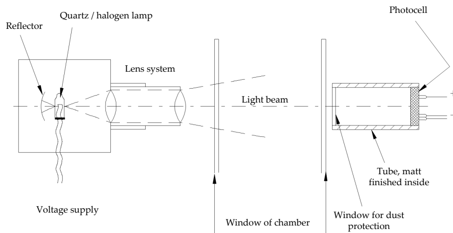
Figure 3.5: Test setup for smoke density test. The sample is combusted inside the test chamber, causing smoke and therefore reduced light transmittance (image source: [IEC 61034-1]).
