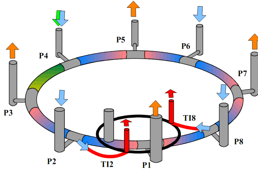
Figure 3.6: Schematic layout of the air flows in the LHC tunnel. Air is provided at each even point and extracted at the odd points of a sector (image source: [Mar03]).
