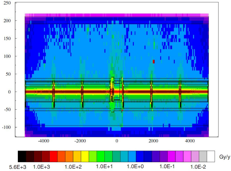
Figure 3.8: Exemplary dose map of annual dose in the LHC arcs. The image shows a longitudinal cut. Dimensions on the x- and y-axis are in cm (image source: [FS01c]).
