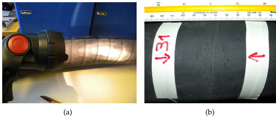
Figure 5.2: Examination of cables: Illumination from a small angle (a), marked crack-area (b).
