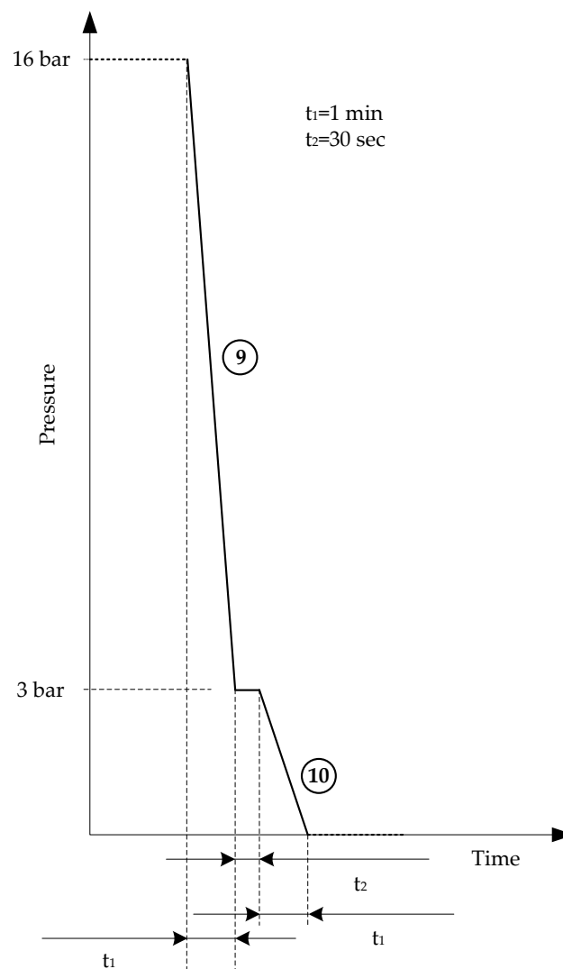
Figure 7.5: Pressure pattern during hydraulic shutdown.
