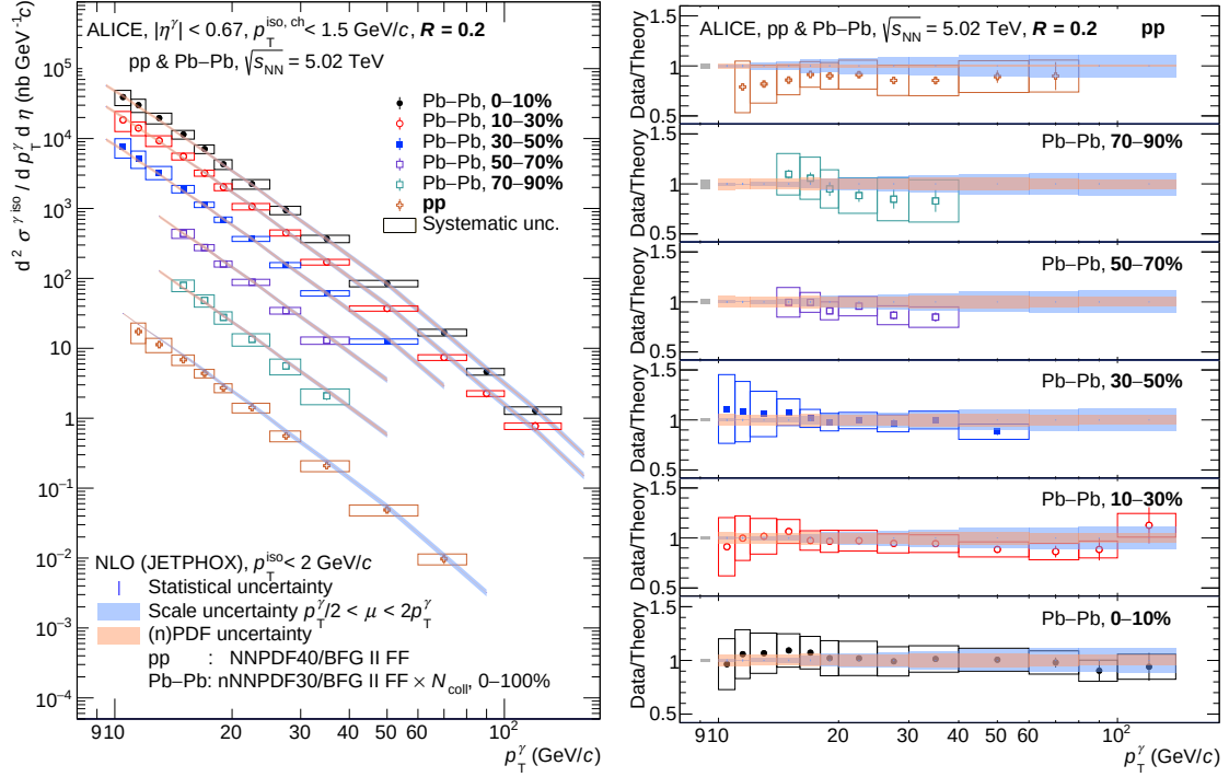
Figure 2.9: Left: isolated-photon differential cross section measured in pp and Pb-Pb collisions at \sqrt{s_{\text{NN}}} = 5.02 TeV for five Pb-Pb centrality classes for R = 0.2 . Right: ratio of data over JETPHOX NLO pQCD calculations. The bands centred at unity correspond to the JETPHOX pQCD calculations, their width represents the scale (blue) uncertainty and PDF (orange) uncertainty, and blue vertical bars indicate the statistical uncertainty of the calculation [93].
