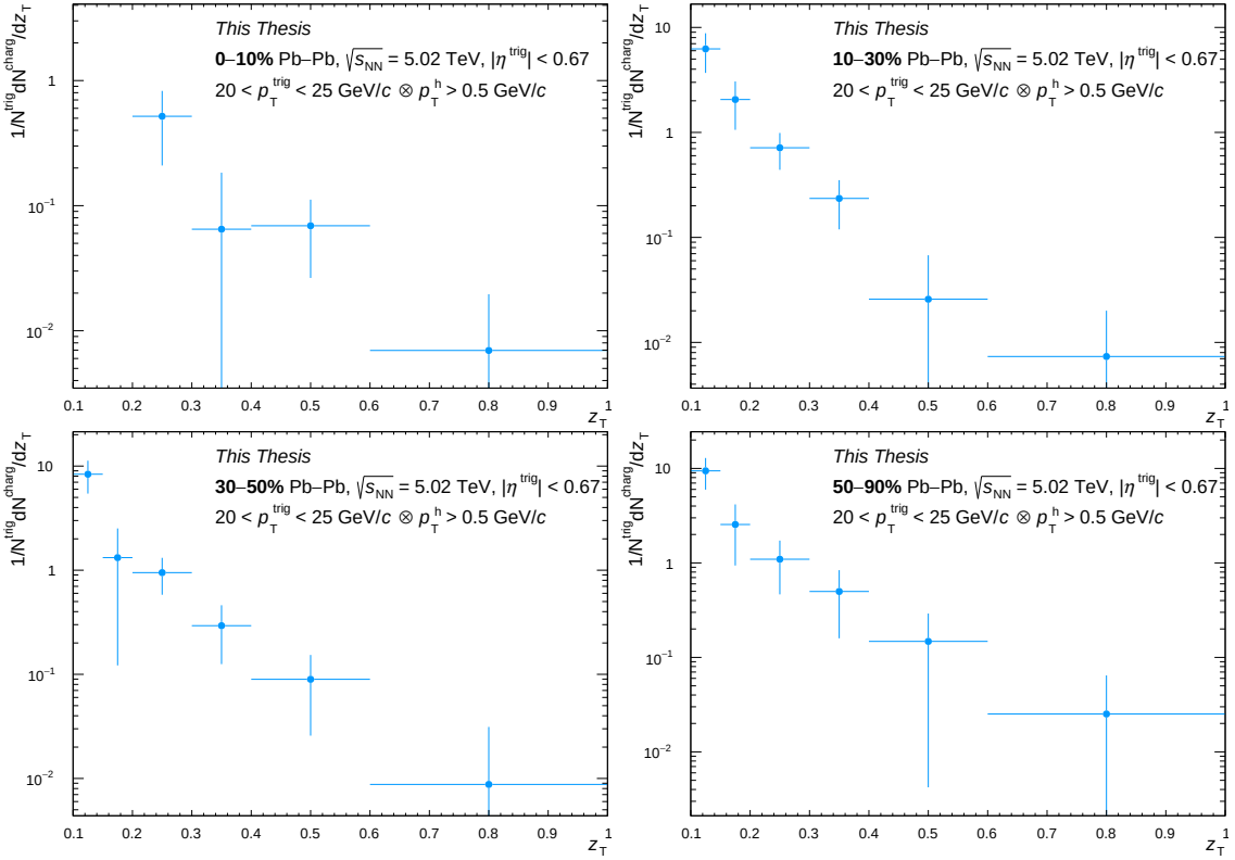
Figure 6.15: D(z_{\text{T}}) distributions as a function of z_{\text{T}} for a p_{\text{T}}^{\text{trig}} between 20 < p_{\text{T}}^{\text{trig}} < 25 GeV/c. From top to bottom, 0-10% Pb-Pb collisions, 10-30% Pb-Pb collisions, 30-50% Pb-Pb collisions and 50-90% Pb-Pb collisions.
