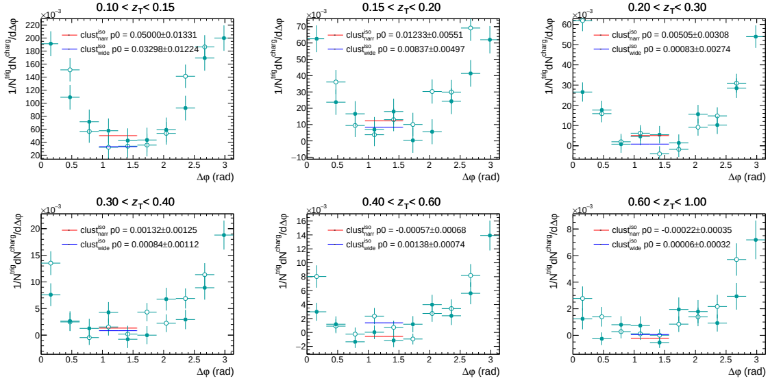
Figure 6.22: Azimuthal correlation distributions as a function of \Delta\varphi for isolated narrow (full green circle) and for isolated wide (empty green circle) clusters after UE subtraction and corresponding constant fits (narrow: red; wide: blue) for different z_T intervals with 20 < p_T^{\text{trig}} < 25 GeV/ c in 30-50% Pb–Pb collisions.
