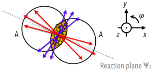
Figure 1.18: Sketch of a collision to highlight the almond shape.
