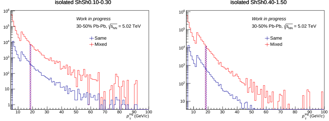
Figure 6.6: p_T^{\text{trig}} distribution for the same event (blue) and mixed event (red) in 30-50% Pb-Pb collisions. Left: distributions for isolated narrow clusters. Right: distributions for isolated wide clusters. As an example one p_T^{\text{trig}} bin has been coloured, corresponding to a certain number of triggers at that transverse momentum.
