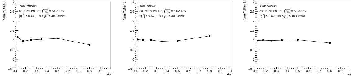
Figure 6.32: Ratio of the z_T distribution obtained with N_{\text{centMix}} = 9 and z_T distribution obtained with N_{\text{centMix}} = 45 in 0-30% (left), 30-50% (middle) and 50-90% (right).
