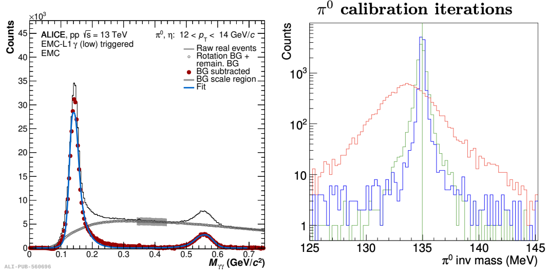
Figure 4.10: Left: Invariant mass distribution for neutral pion and \eta meson candidates at intermediate transverse momenta 12 < p_T < 14 GeV/c reconstructed with both photons in the EMCal in pp collisions at 13 TeV using the L1- \gamma trigger sample. Distribution obtained with a fully calibrated EMCal [135]. Right: Variation of the \pi^0 energy calibration coefficient in all channels of 2012 data from the last iteration (blue) compared to the first iteration (red), and compared to the last iteration of 2011 data (green).
