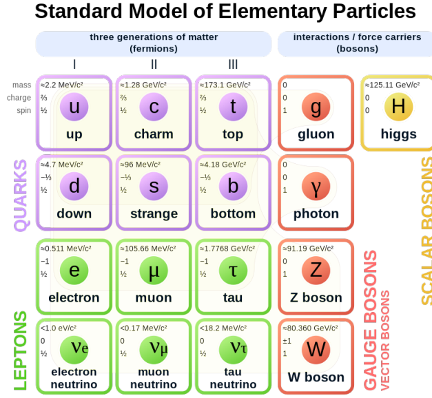
Figure 1.1: The elementary particles of the Standard Model [2].
