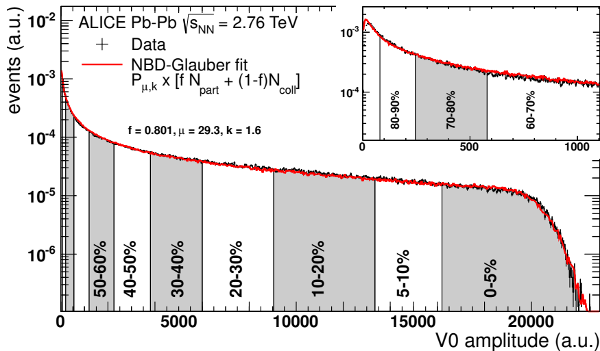
Figure 3.6: Distribution of the V_0 amplitudes measured in Pb–Pb collisions at \sqrt{s_{NN}} = 2.76 TeV. The red line reports the NBD-Glauber fit, while the bands show the different centrality classes [122].
