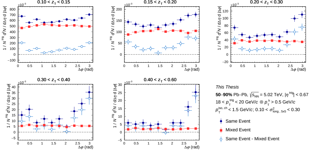
Figure C.16: Azimuthal correlation distribution in 50-90% for isolated narrow clusters for the same event (full blue circle), for mixed event (full red square) and for result of the subtraction (empty light blue circle) as a function of \Delta\phi for different z_T bins with 18 < p_T^{\text{trig}} < 20 GeV/c.
