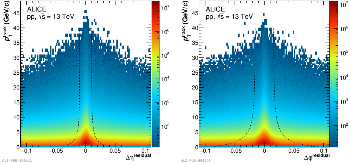
Figure 5.2: Distance between a cluster and the closest projected track in \Delta\eta^{\text{residual}} (left) and \Delta\phi^{\text{residual}} (right) angle versus the track momentum p_T^{\text{track}} in pp collisions at \sqrt{s} = 13 TeV. The black lines indicate the selection reported in Eq. (5.1) and (5.2) [135].
