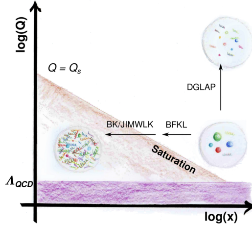
Figure 1.7: Map of QCD as a function of (Q, x) .
