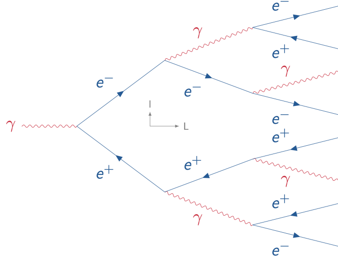
Figure 4.3: Sketch of the development of an electromagnetic shower induced by an incident photon. The axes "L" and "l" represent the longitudinal and radial components of this development respectively. Figure taken from [137]
