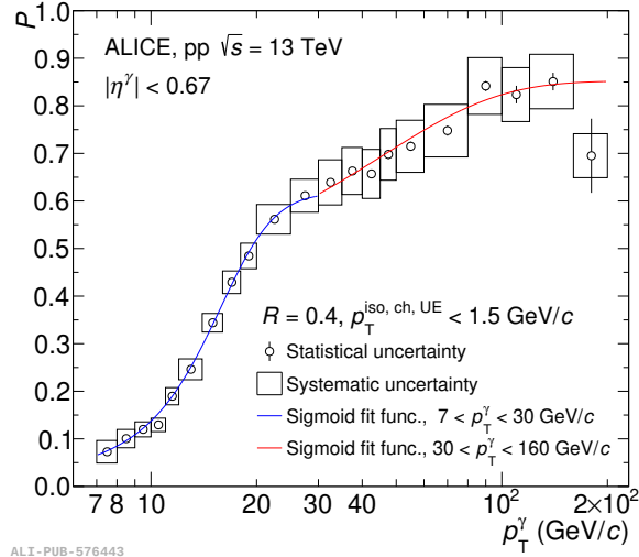
Figure 5.19: Purity of the isolated-photon sample as a function of p_T^\gamma in pp collisions at \sqrt{s} = 13 TeV. The red and blue lines are the results of a fit to the measured purity using a two-sigmoid-function described by Eq. (5.17) for two different transverse momentum intervals [85].
