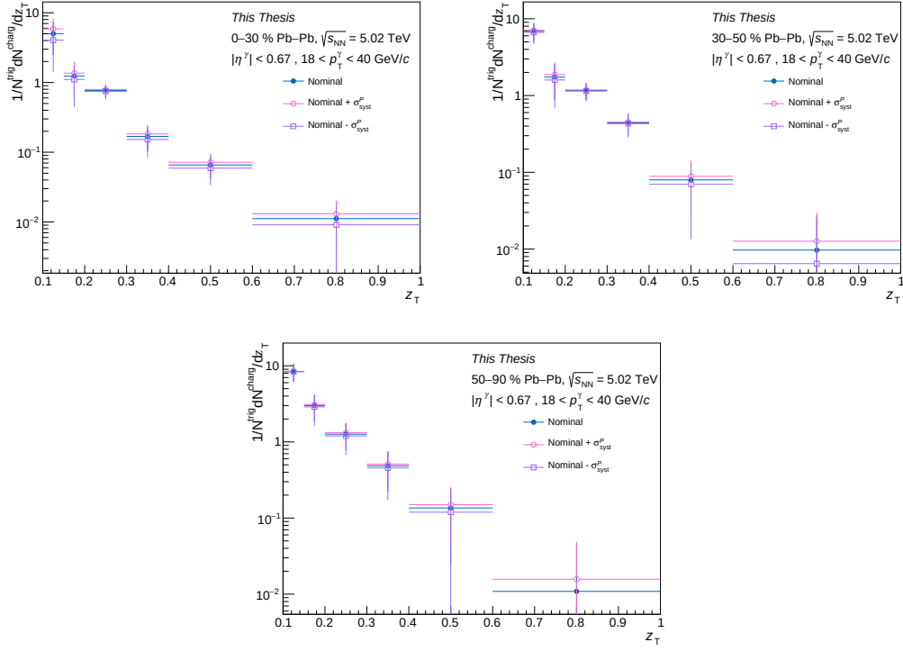
Figure 6.26: The D(z_T) distributions for different purity values: nominal (full blue circle), nominal + \sigma_{\text{syst}}^P (empty pink circle) and nominal - \sigma_{\text{syst}}^P (empty violet square) in 0-30% (top left), in 30-50% (top right) and in 50-90% (bottom) Pb-Pb collisions.
