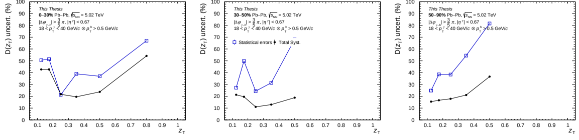
Figure 6.35: Comparison between statistical and systematic uncertainties for the three centrality classes measured.
