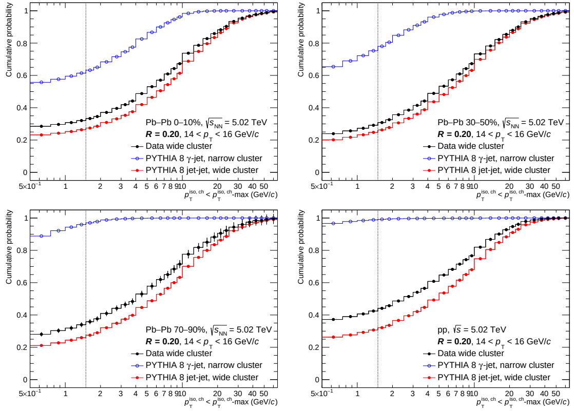
Figure 5.15: p_T^{\text{iso, ch}} cumulative probability distribution (clusters with p_T^{\text{iso, ch}} < p_T^{\text{iso, ch-cut}} overall) for clusters with 14 < p_T < 16 GeV/c for signal narrow clusters in a \gamma -jet simulation (empty blue circle) and background wide clusters in data (full black circle) and background wide clusters in jet-jet simulation (full red circle) with R = 0.2 . From top to bottom, 0-10% Pb-Pb collisions, 30-50% Pb-Pb collisions, 70-90% Pb-Pb collisions and pp collisions. The \eta -band is used to subtract the UE from p_T^{\text{iso, ch}} . Dashed line at selected isolation value of 1.5 GeV/c [148].
