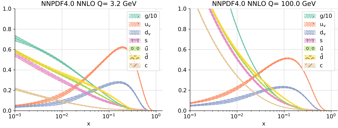
Figure 1.6: NNPDF4.0 NNLO proton PDF as a function of momentum fraction x , evaluated at two different scales Q = 3.2 GeV (left) and Q = 100 GeV (right). Each colour represents the PDF of a different parton species, as indicated in the legend [15].
