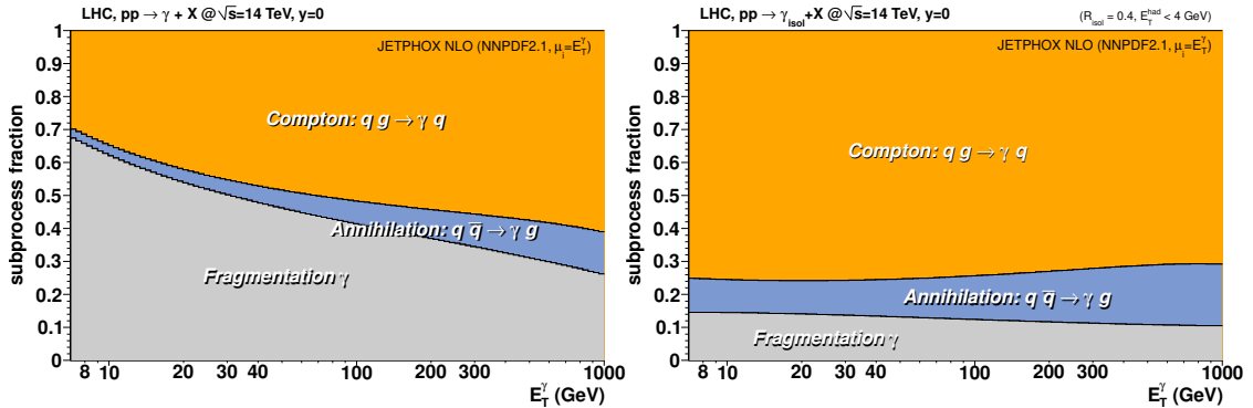
Figure 2.5: Fraction of different processes, Compton (orange), annihilation (blue) and fragmentation (grey), that contributes to the prompt photon production in pp collisions at \sqrt{s} = 14 TeV at LHC from simulation without (left) and with (right) the isolation method [83].
