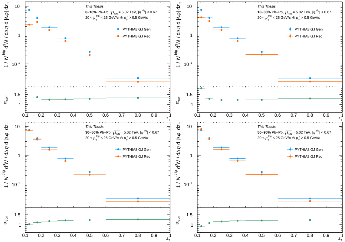
Figure 6.18: Top panels: the D(z_T) distributions as a function of z_T for GJ MC simulation at generated (full light blue square) and reconstructed (full orange square) levels with 20 < p_T^\gamma < 25 \text{ GeV}/c . Bottom panels: the \alpha_{\text{corr}} factor (full green square) as a function of z_T . From top to bottom, 0-10% Pb-Pb collisions, 10-30% Pb-Pb collisions, 30-50% Pb-Pb collisions and 50-90% Pb-Pb collisions.
