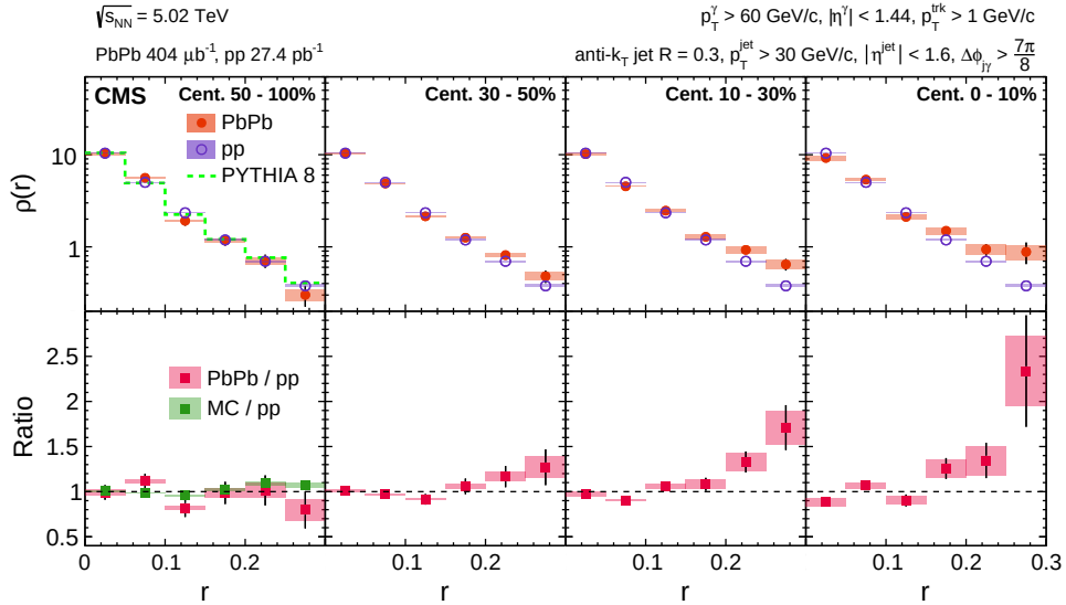
Figure 2.16: Top: Differential jet shape, for jets associated with an isolated-photon from peripheral to central Pb–Pb (full circles), and pp (open circles) collisions at \sqrt{s_{\text{NN}}} = 5.02 TeV. Bottom: Ratios between the Pb–Pb and pp distributions by CMS [107].
