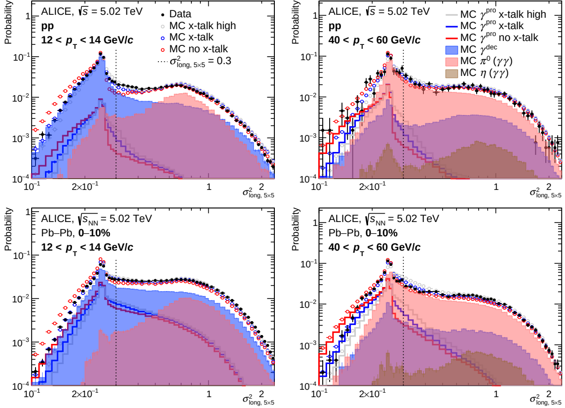
Figure 5.9: Inclusive-cluster \sigma^2_{\text{long}, 5 \times 5} distribution in data (black bullets) and PYTHIA simulations. The simulation is decomposed in its different particle origins: prompt photons (blue line), not merged decay photons (MC \gamma_{\text{decay}} , blue area), merged decays from \pi^0 (MC \pi^0 , red area) or \eta (brown area). Three different treatments of cross-talk (x-talk) were considered in the simulation: “no x-talk” (open red circles); “x-talk high” (open grey circles), stronger cross talk obtained for the previous isolated-photon measurements [76, 85, 135]; and “x-talk” (open blue circles), obtained for this measurement. The four panels display these distributions for two selected cluster p_T ranges, 12 < p_T < 14 GeV/c on the left and 40 < p_T < 60 GeV/c on the right, and two collision systems: pp (top) and Pb–Pb 0–10% central (bottom) at \sqrt{s_{\text{NN}}} = 5.02 TeV [93].
