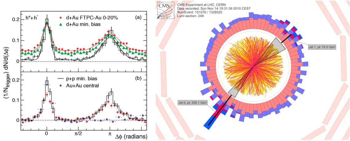
Figure 1.24: Left: azimuthal correlation distributions in pp (black line), in central d-Au (full red circle), in minimum bias d-Au (full green triangle) and central Au-Au (full blue star) collisions measured by the STAR Collaboration. The trigger hadron p_T is 4 < p_T < 6 GeV/ c , while the selected charged particles p_T are between 2 < p_T^{assoc} < p_T^{trig} GeV/ c [66, 67]. Right: CMS event display at LHC for a single Pb-Pb collision, showing a dijet event [68].
