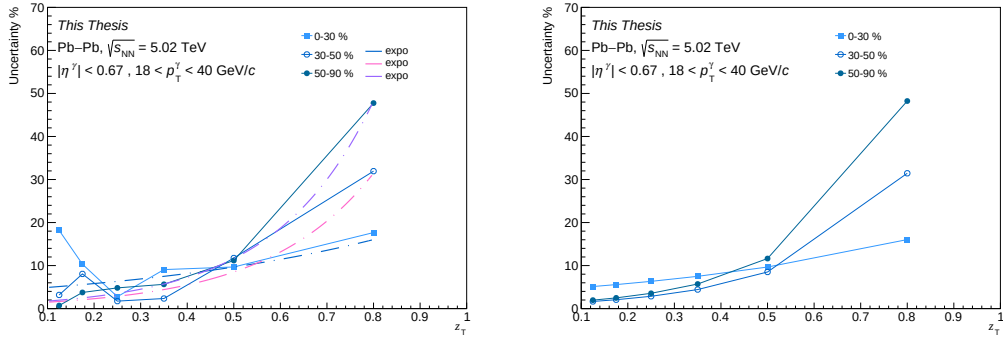
Figure 6.27: Left: Systematic uncertainties of the purity in 0-30% (full light blue square), 30-50% (empty blue circle) and 50-90% (full blue circle) Pb-Pb collisions. smoothing of the systematic uncertainties using an exponential fit in 0-30% (blue dot-dashed line), 30-50% (pink dot-dashed line) and 50-90% (violet dot-dashed line) Pb-Pb collisions. Right: Systematic uncertainties of the purity obtained from the fit.
