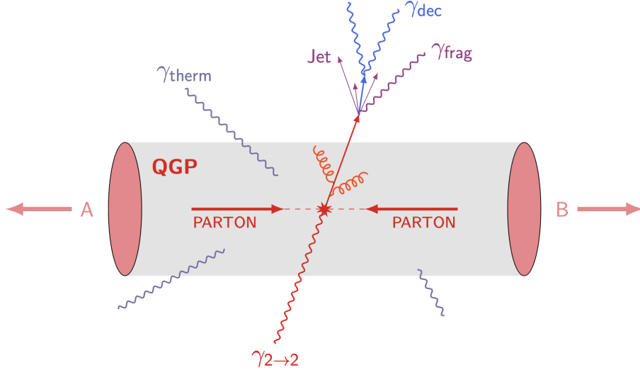
Figure 2.1: Sketch of photon production during a heavy-ion collision between nuclei A and B. They include: \gamma_{2 \rightarrow 2} , \gamma_{\text{decay}} , \gamma_{\text{fragm}} and \gamma_{\text{therm}} .
