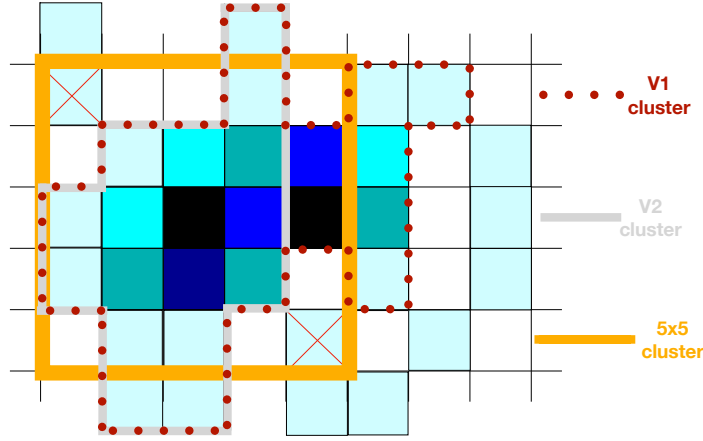
Figure 5.7: Schematic view of the cell energy repartition of two high-energy decay photons from a neutral meson, each centred in the black-filled cells, on top of a high-multiplicity low-energy particle underlying event environment, the lightest blue cells. The grey lines are the contour of cells selected restricting the growth of the cluster (V2) used to calculate the cluster energy and position. The orange square is the 5 \times 5 region around the highest-energy cell used for the shower shape calculation, excluding cells that only have a common corner, red cross. The red dotted lines are the contour of a cluster without growth restriction (V1), as used in previous pp and p-Pb isolated photon analyses [93].
