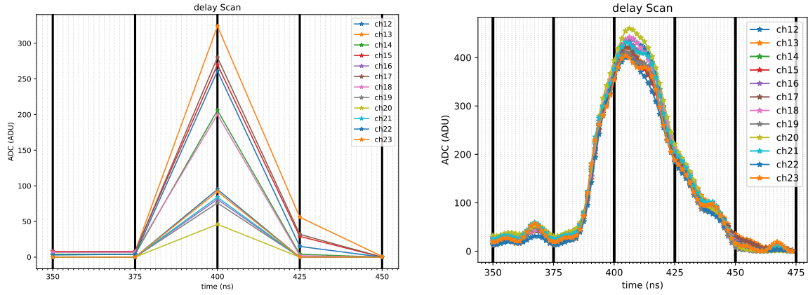
Figure 7.13: ADC mean distribution as a function of the time for channels from 12 to 23. Left: ADC mean distribution for the coarse calibration. Right: ADC mean distribution for the fine calibration.
