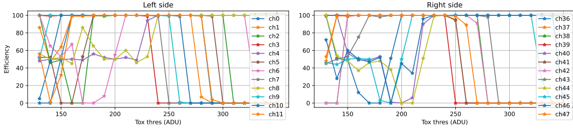
Figure 7.25: Efficiency curves as a function of the global thresholds for different channels and for the two sides of one ASIC of the prototype, after the calibration procedure.
