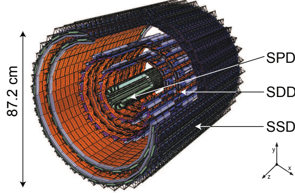
Figure 3.3: Schema of the Inner Tracking System [122].
