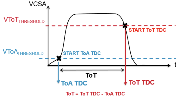
Figure 7.5: Sketch for describing the relationship between the TOA and the TOT. An analog signal as a function of the time is shown.
