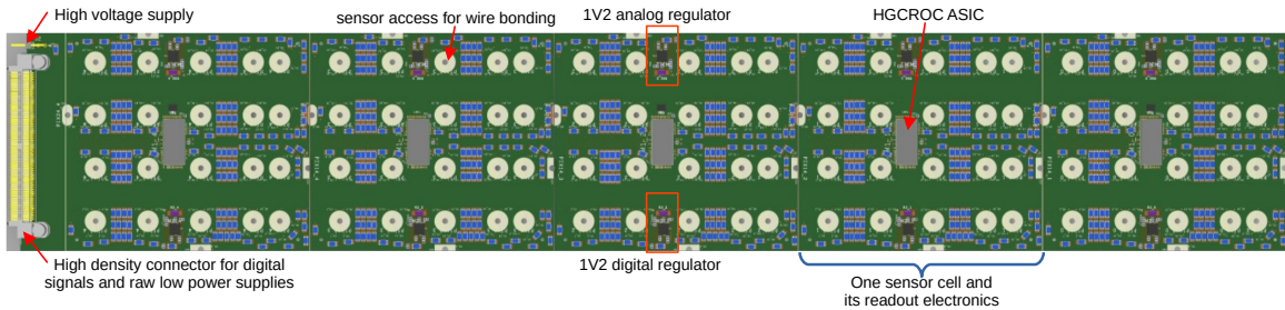
Figure 7.3: The pad-layer board is made out of 5 individual pad sensors each with 72 channels of 1 \times 1 \text{ cm}^2 , which will be readout by one HGCROC chip.
