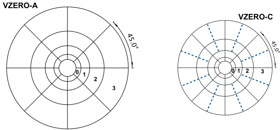
Figure 3.5: Sketches of V0-A and V0-C arrays showing their segmentation. Scintillator thicknesses are 2.5 and 2 cm respectively. The scintillator segments on both sides of the dashed lines are connected to the same PMT [47].
