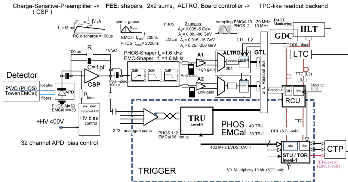
Figure 4.7: Scheme of the EMCal front end electronics [140].
