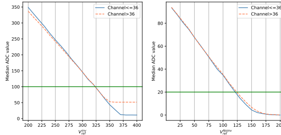
Figure 7.11: Left: median ADC value as a function of inverting voltage. Right: median ADC value as a function of non-inverting one.
