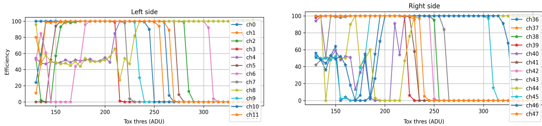
Figure 7.24: Efficiency curves as a function of the global thresholds for different channels and for the two sides of one ASIC of the prototype, before the calibration procedure.
