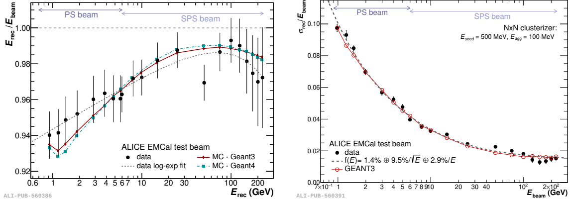
Figure 4.11: Left: Energy nonlinearity correction as a function of reconstructed energy for electrons obtained from test beam data (black points), and from MC simulations with GEANT3 (red points) and GEANT4 (cyan points) transport codes. Right: energy resolution of the EMCal as a function of the incident particle energy [135].
