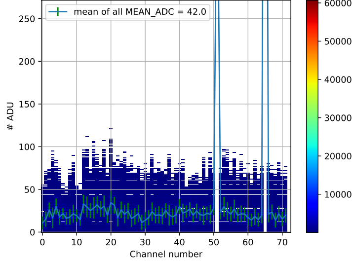
Figure 7.12: Effect of the dynamic range calibration. The mean of the ADC mean distribution for all the channels.
