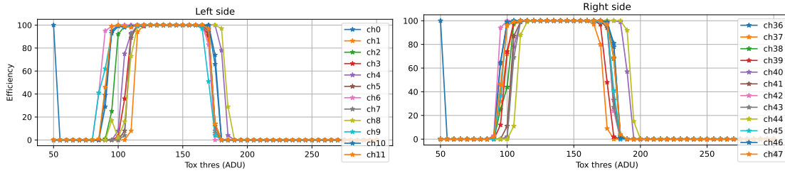
Figure 7.16: Efficiency as a function of global thresholds for different channels and for the two sides of the HGCROC after the calibration.
