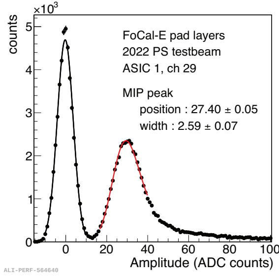
Figure 7.19: MIP peak measured from a single channel of a FoCal-E pad layer in PS 2022 test beam [179].
