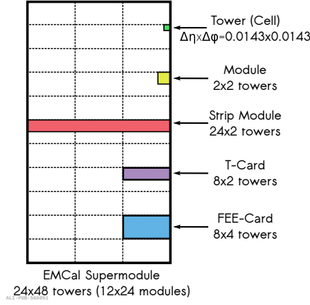
Figure 4.6: Illustration of one EMCal supermodule with the different segmentation levels: tower (green), module (yellow), strip module (pink), T-Card (violet) and FEE-Card (light blue) [132].
