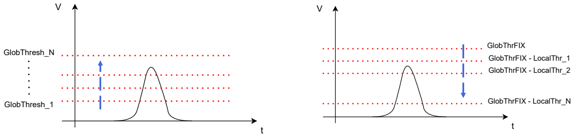
Figure 7.14: Left: Sketch that describes the global thresholds scan. Right: Sketch that describes the local thresholds scan. The blue arrow indicates the direction.
