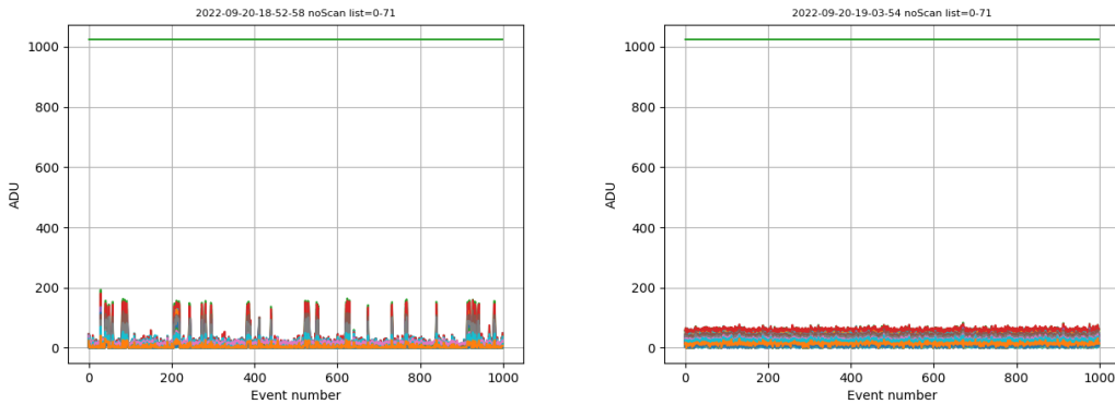
Figure 7.26: Left: ADC pedestals affected by the activation of the TOA . Right: ADC pedestals after the variation of TOA thresholds.
