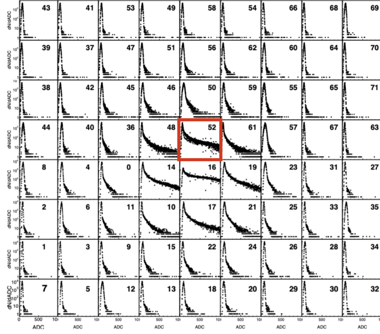
Figure 7.23: ADC response at higher energy. The prototype was irradiated with electrons. The beam spot is in channel 52, indicated by a red square.
