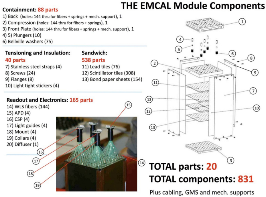
Figure 4.5: Photo and drawing of the EMCal module components [132].
