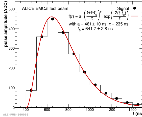
Figure 4.8: Digital signal (full black circle) of a tower obtained at the output of a FEE card as a function of time, fitted by the function \Gamma_n(t) (full red line) defined in Eq. (4.3) [132].
