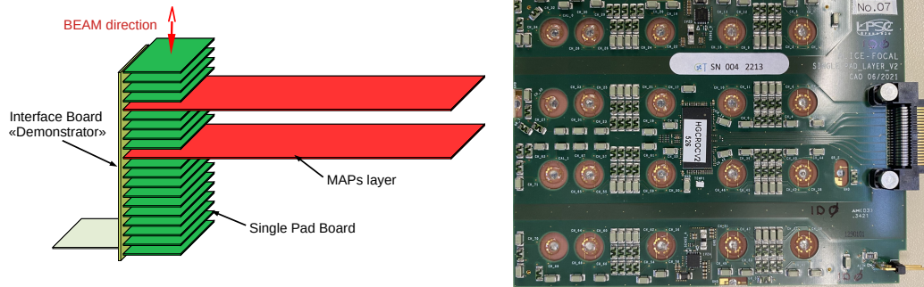
Figure 7.7: Left: Focal prototype tower composed of 18 single-pad boards with a test-beam dedicated interface board. Right: picture of one single-pad used in the FoCal tower prototype [168].
