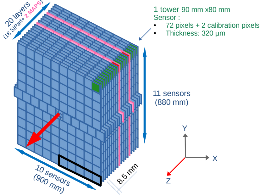
Figure 7.2: The longitudinal structure of the FoCal-E has a total of 20 layers: 18 layers of tungsten and silicon pads (blue) interleaved with two layers of tungsten and silicon pixels MAPS (pink) [168]. z is the beam direction.
