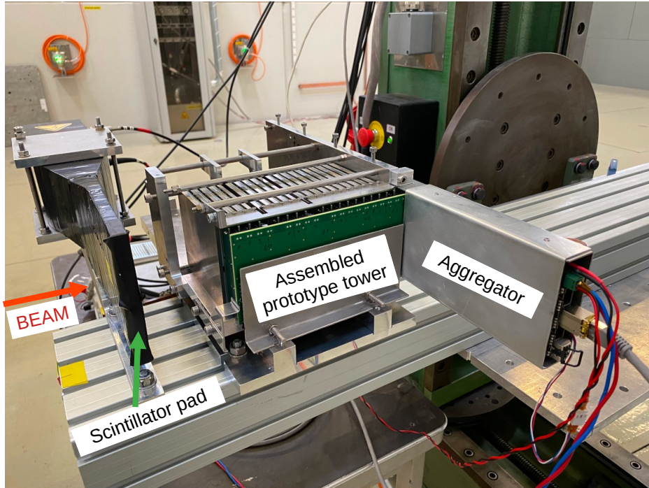
Figure 7.17: Picture of the FoCal tower prototype installed on the T9 beamline at the CERN PS.
