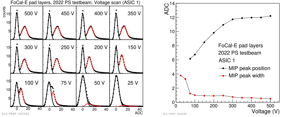
Figure 7.20: Left: ADC distributions as a function of the ADC channel for different voltage values. Right: MIP peak position (full black dot) and MIP peak width (full red dot) as a function of the voltage [179].
