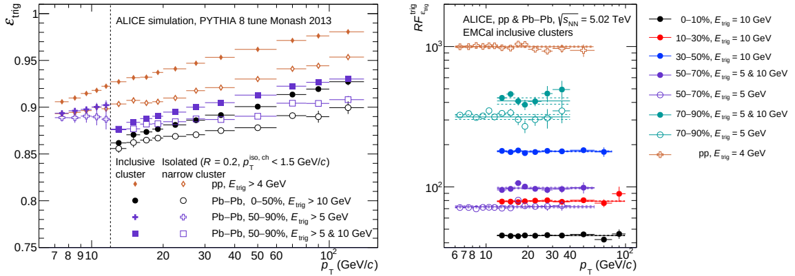
Figure 4.9: Left: L1- \gamma trigger efficiency for inclusive clusters (see Table 5.1) and isolated narrow clusters (see Sect. 5.3), obtained with PYTHIA simulation combining \gamma -jet (empty markers) and jet-jet (full markers) processes for pp and embedded in data for Pb-Pb collisions, considering the corresponding trigger thresholds in each system. Right: L1- \gamma trigger rejection factor calculated by applying the trigger efficiency for each of the pp and Pb-Pb centrality classes considered at \sqrt{s_{NN}} = 5.02 TeV. Solid lines over points result of a constant fit and dashed lines indicate the fit uncertainty [93].
