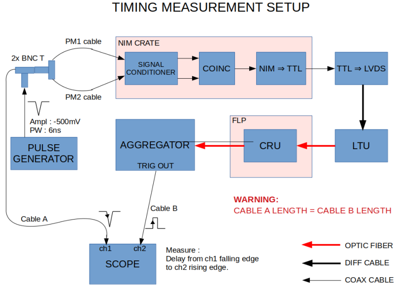
Figure 7.18: Test beam setup used to determine the cables delays to the aggregator. Figure courtesy of D. Tourres.
