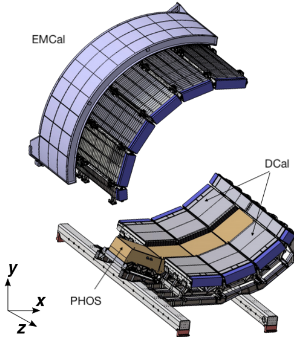
Figure 4.4: Schematic view of the EMCal calorimeter illustrating the module position on two approximately opposite locations in azimuth \varphi . The PHOS calorimeter is inside the DCal and is indicated in brown [135].
