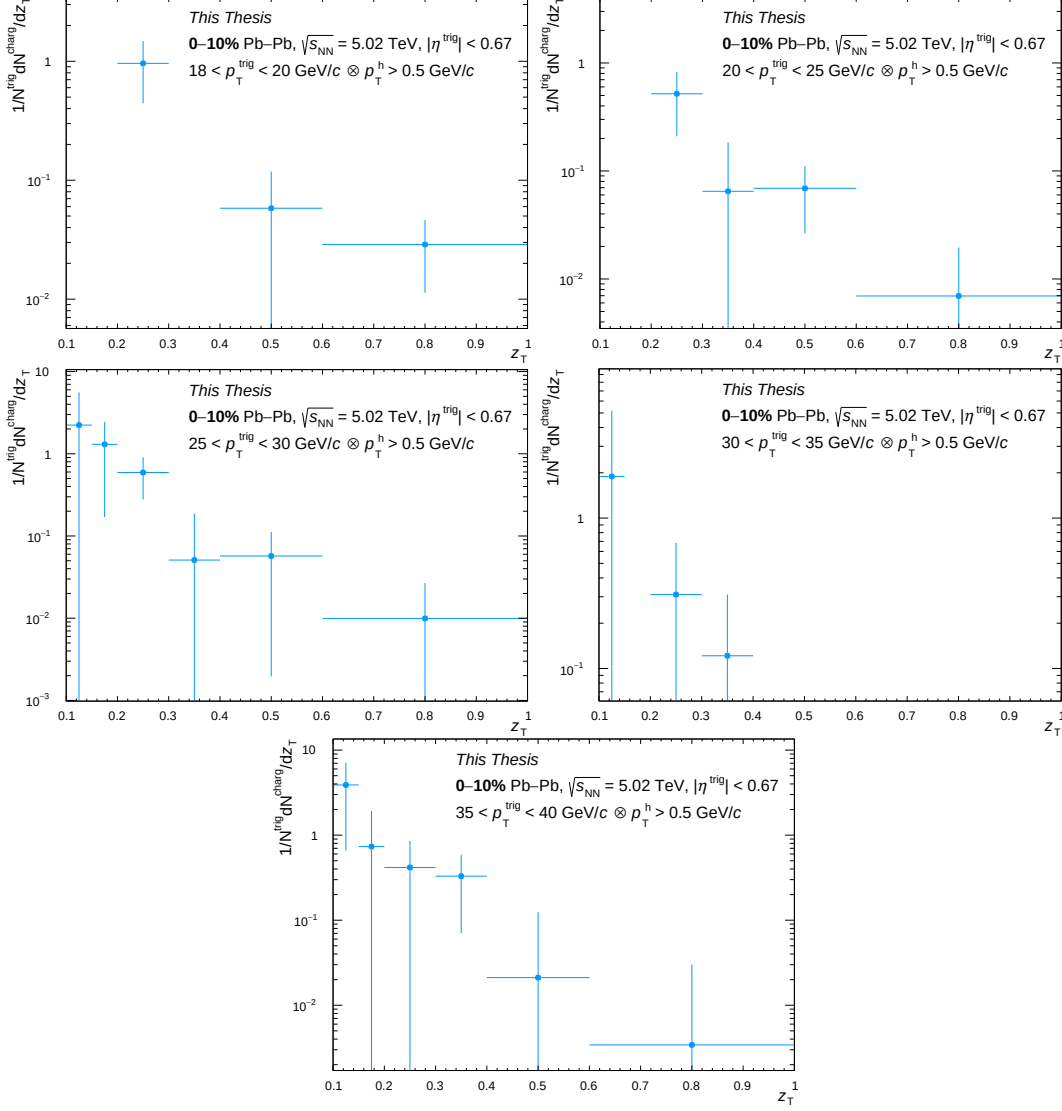
Figure C.61: D(z_T) distribution as a function of z_T in 0-10% Pb-Pb collisions for different p_T^\gamma intervals. From top to bottom: 18 < p_T^\gamma < 20 GeV/c, 20 < p_T^\gamma < 25 GeV/c, 25 < p_T^\gamma < 30 GeV/c, 30 < p_T^\gamma < 35 GeV/c and 35 < p_T^\gamma < 40 GeV/c.
