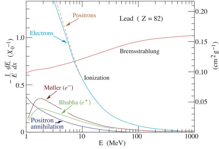
Figure 4.2: Contributions related to the loss of energy per unit radiation length (quantity defined in the text) suffered by an electron or positron in the lead (Pb) as a function of its energy [138].
