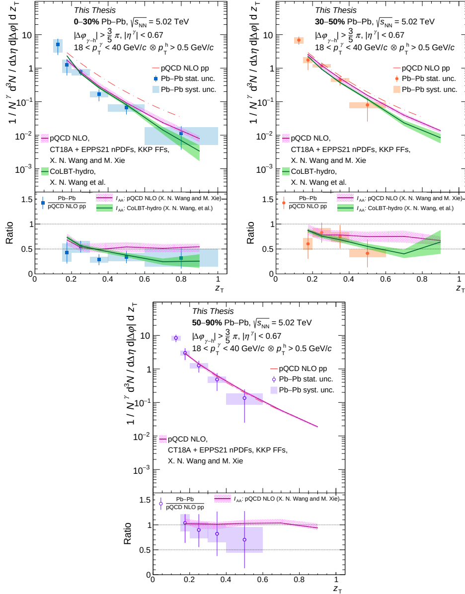
Figure 6.37: Top panels: The D(z_T) distributions as a function of z_T for a p_T^\gamma between 18 < p_T^\gamma < 40 GeV/c in 0-30% (full blue square), 30-50% (full orange circle) and 50-90% (empty violet circle). The statistical uncertainties are indicated by bars, while the systematics uncertainties are shown with coloured boxes. Theoretical calculations are included pQCD NLO (pink) and CoLBT-hydro (green) models. Bottom panels: Ratio of D(z_T) in Pb–Pb collisions to pQCD calculations (bottom panels) as a function of z_T .
