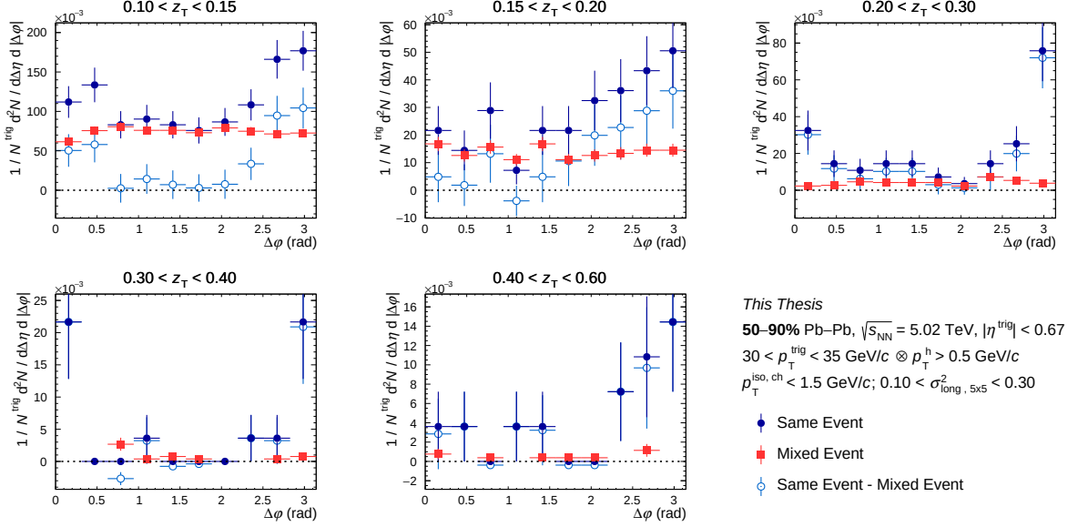
Figure C.19: Azimuthal correlation distribution in 50-90% for isolated narrow clusters for the same event (full blue circle), for mixed event (full red square) and for result of the subtraction (empty light blue circle) as a function of \Delta\phi for different z_T bins with 30 < p_T^{\text{trig}} < 35 GeV/c.
