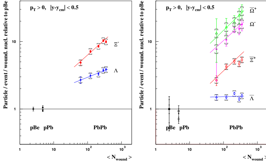
Figure 1.15: Hyperon enhancements as a function of \langle N_{\text{wound}} \rangle in Pb–Pb p–Pb and p–Be collisions at \sqrt{s_{\text{NN}}} = 158 GeV measured by NA57 Collaboration [51].
