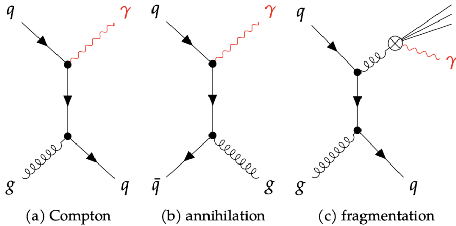
Figure 2.4: Feynman diagrams for prompt photon production.
