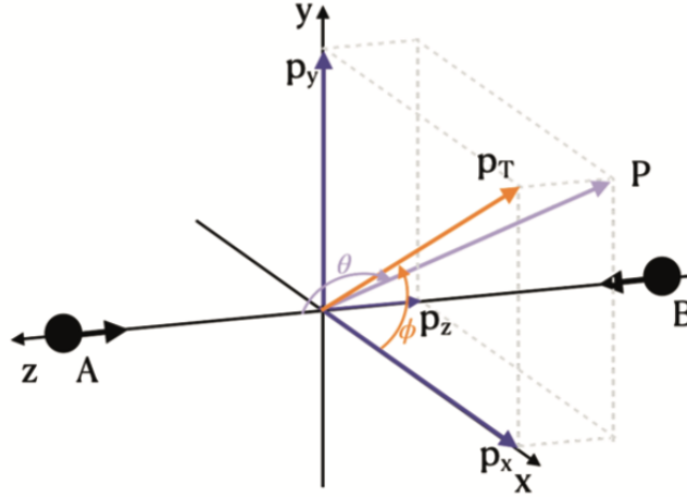
Figure 1.12: Coordinate system describing a collision between A and B nuclei.
