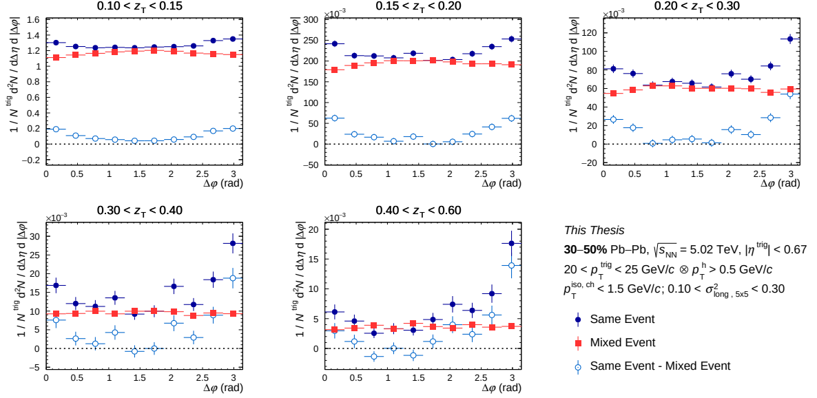
Figure 6.7: Azimuthal correlation distributions in 30–50% for isolated narrow clusters for the same event (full blue circle), for the mixed event (full red square) and the result of the subtraction (empty light blue circle) as a function of \Delta\varphi for different z_T bins with 20 < p_T^{\text{trig}} < 25 GeV/ c .
