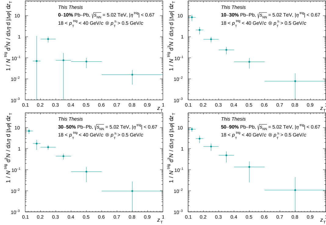
Figure 6.20: The D(z_T) distributions as a function of z_T from \gamma^{iso} -hadron correlations for a p_T^\gamma between 18 < p_T^\gamma < 40 GeV/c. From top to bottom, 0-10% Pb-Pb collisions, 10-30% Pb-Pb collisions, 30-50% Pb-Pb collisions and 50-90% Pb-Pb collisions.
