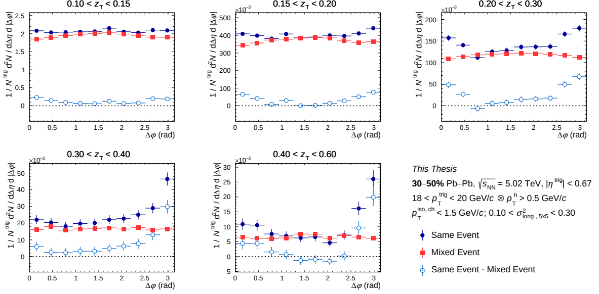
Figure C.11: Azimuthal correlation distribution in 30–50% for isolated narrow clusters for the same event (full blue circle), for mixed event (full red square) and for result of the subtraction (empty light blue circle) as a function of \Delta\phi for different z_T bins with 18 < p_T^{\text{trig}} < 20 GeV/ c .
