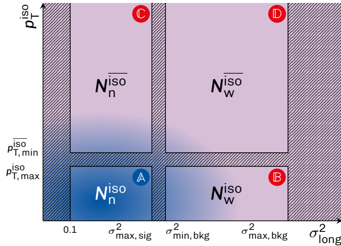
Figure 5.16: Illustration of the parametric-space of the photon p_{\text{T}}^{\text{iso}} (or p_{\text{T}}^{\text{iso, ch}} , etc) and \sigma_{\text{long}}^2 ( \sigma_{\text{long}, 5 \times 5}^2 ), used to estimate the background yield in the signal region ( A ) from the observed yields in the three control regions ( B , C , D ). The red regions indicate areas dominated by background and the blue regions by the photon signal. The color gradient indicates mixture of signal and background [135].
