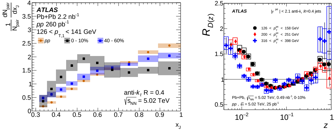
Figure 1.25: Left: measurement of di-jet yield-normalized x_J distributions measured by the ATLAS Collaboration in 0–10% (full black square) and 40–60% (full blue square) Pb–Pb and in pp (full orange circle) collisions at \sqrt{s_{NN}} = 5.02 TeV [69]. Right: ratio R_{D(z)} between fragmentation functions in central Pb–Pb and pp collisions at \sqrt{s_{NN}} = 5.02 TeV measured by ATLAS. Ratios are shown for three different p_T^{\text{jet}} ranges: 126–158 GeV (full black circle), 200–251 GeV (full red diamond) and 316–398 GeV (full blue cross) [70].
