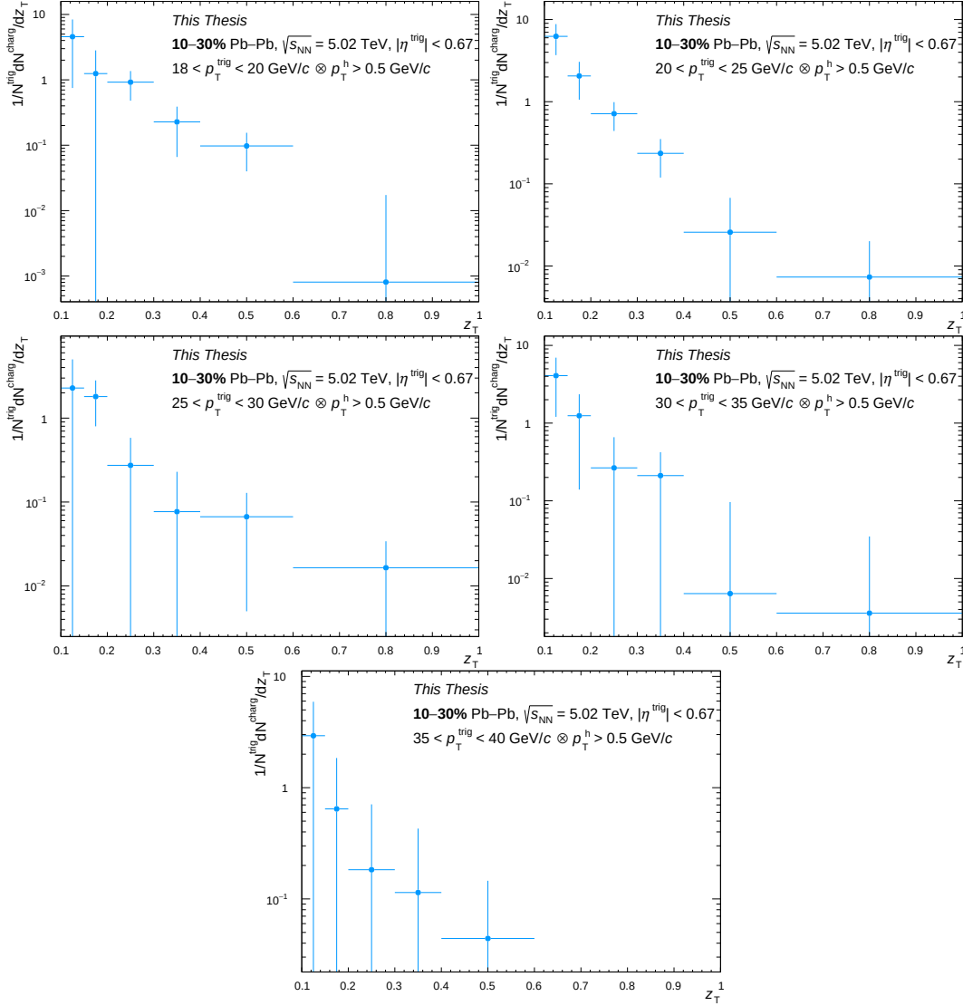
Figure C.62: D(z_T) distribution as a function of z_T in 10-30% Pb-Pb collisions for different p_T^\gamma intervals. From top to bottom: 18 < p_T^\gamma < 20 GeV/c, 20 < p_T^\gamma < 25 GeV/c, 25 < p_T^\gamma < 30 GeV/c, 30 < p_T^\gamma < 35 GeV/c and 35 < p_T^\gamma < 40 GeV/c.
