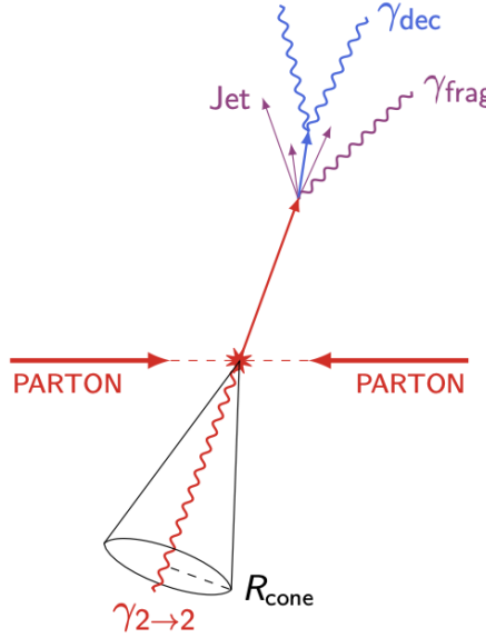
Figure 2.6: Sketch of a collision in which \gamma_{2 \rightarrow 2} , \gamma_{\text{decay}} and \gamma_{\text{fragm}} are produced. The isolation method is applied to select the \gamma_{2 \rightarrow 2} .
