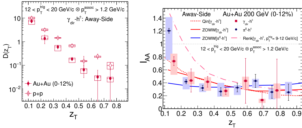
Figure 2.20: Left: D(z_T) distributions for \gamma^{\text{iso}} -hadron correlations as a function of z_T for central Au–Au (full red dot) and for pp (empty red dot) collisions measured by the STAR Collaboration. Right: I_{AA} for \gamma^{\text{iso}} -hadron (red squares) and for \pi^0 -hadron (blue circles) correlations as a function of z_T . The vertical lines represent statistical error and the vertical boxes represent systematic errors. The curves represent theoretical model predictions [111].
