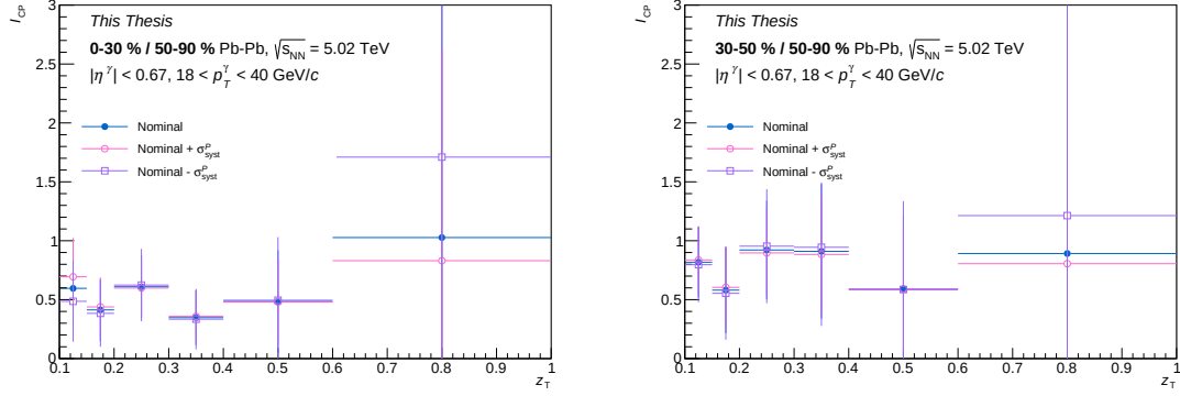
Figure D.1: The I_{CP} ratios for different purity values: nominal (full blue circle), nominal + \sigma_{syst}^P (empty pink circle) and nominal - \sigma_{syst}^P (empty violet square) in 0-30% (left panel) and in 30-50% (right panel) Pb-Pb collisions.
