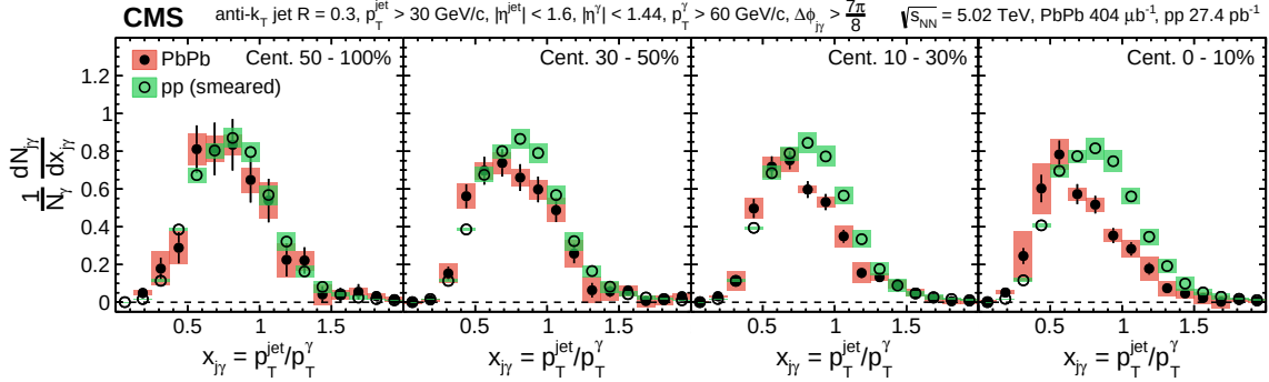
Figure 2.13: The p_T balance observable as a function of x_{j\gamma} for various centralities in Pb-Pb (full markers) and pp (open markers) collisions. Vertical lines display the statistical uncertainties while the coloured boxes (red for PbPb, green for pp) show the systematic uncertainties [101].
