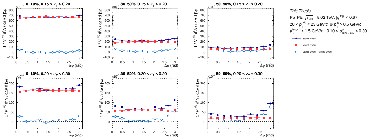
Figure 6.11: Azimuthal correlation distributions for isolated narrow clusters for the same event (full blue circle), for mixed event (full red square) and the result of the subtraction (empty light blue circle) as a function of \Delta\phi for two z_T intervals with 20 < p_T^{\text{trig}} < 25 GeV/c. Comparing three centralities: 0-10% (left), 30-50% (middle) and 50-90% (right) Pb-Pb collisions.
