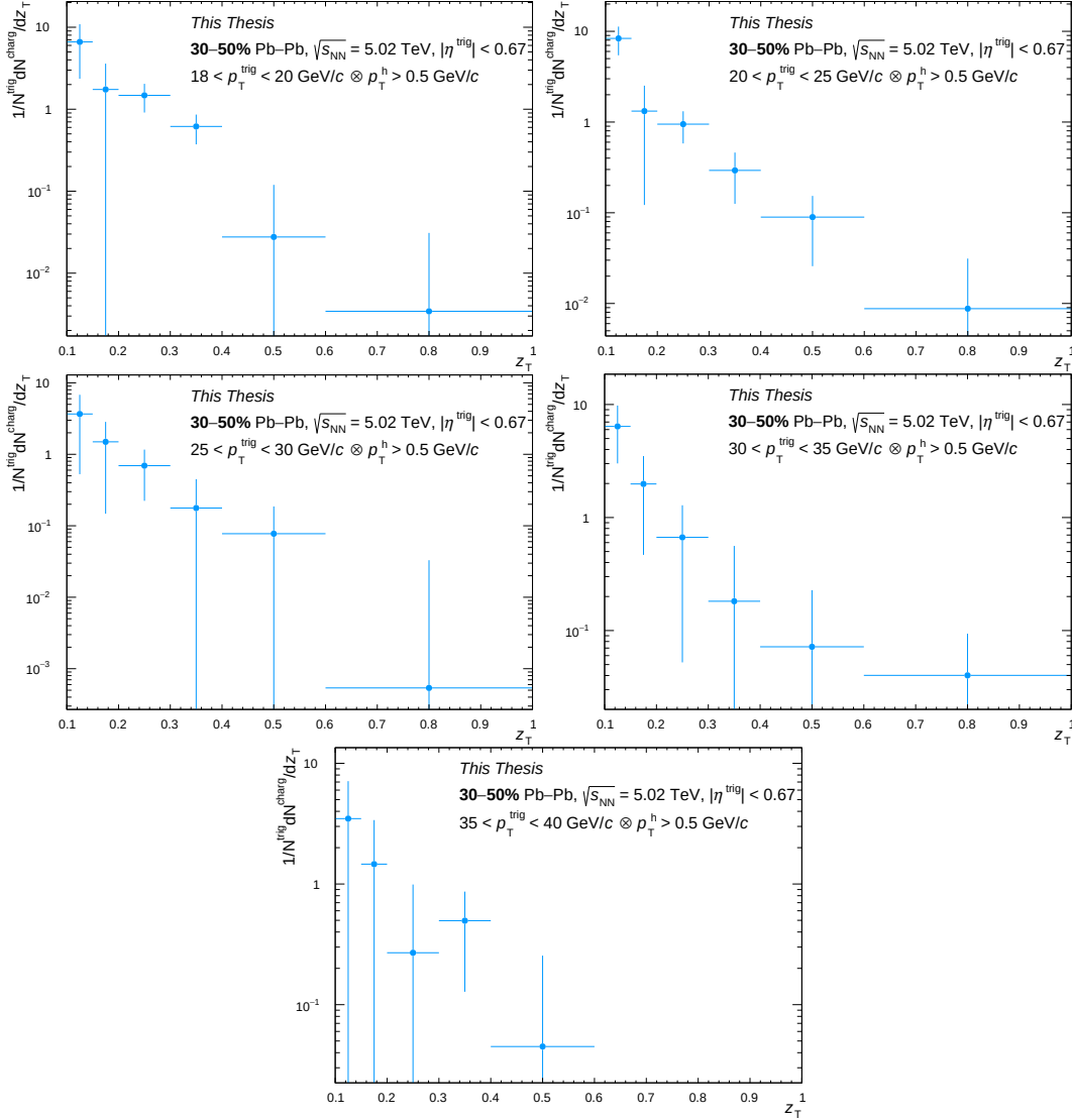
Figure C.63: D(z_T) distribution as a function of z_T in 30-50% Pb-Pb collisions for different p_T^\gamma intervals. From top to bottom: 18 < p_T^\gamma < 20 GeV/c, 20 < p_T^\gamma < 25 GeV/c, 25 < p_T^\gamma < 30 GeV/c, 30 < p_T^\gamma < 35 GeV/c and 35 < p_T^\gamma < 40 GeV/c.
