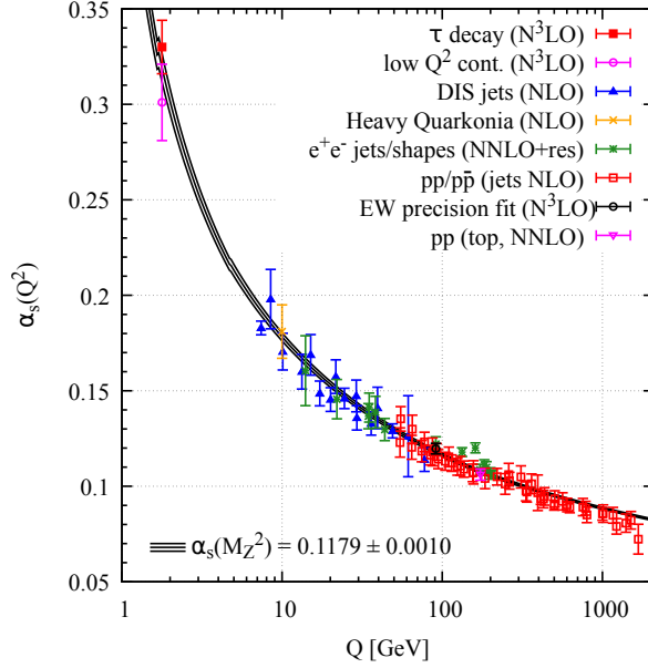
Figure 1.4: Summary of measurements of \alpha_s(Q^2) as a function of the respective energy scale Q . The acronyms in the brackets specify the order used in perturbative QCD calculations that went into the extraction of \alpha_s [10].
