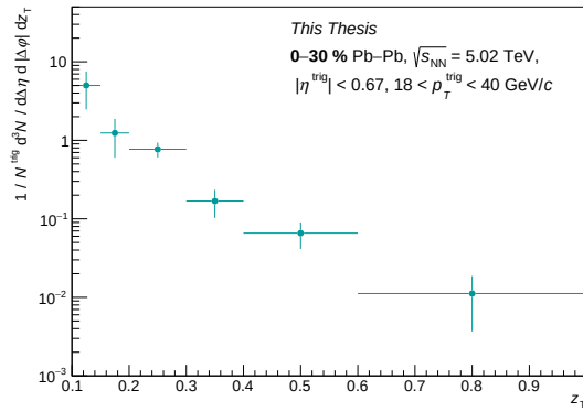
Figure 6.21: z_T distribution in 0-30% for the \gamma^{iso} -hadron correlation after merging the various \Delta\varphi distributions in 0-10% and 10-30% Pb-Pb collisions for a p_T^\gamma in 18 < p_T^\gamma < 40 GeV/c.
