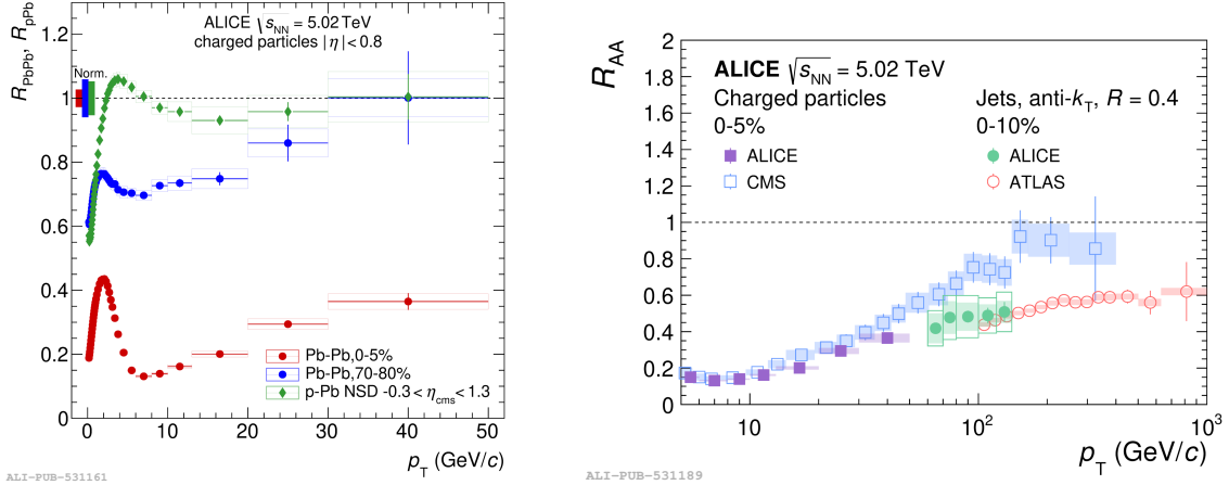
Figure 1.23: Left: R_{AA} for charged particles in central (0-5%) (full red circle) and peripheral (70-80%) (full blue circle) Pb–Pb collisions and R_{pA} for p–Pb collisions (full green diamond) at \sqrt{s_{NN}} = 5.02 TeV by ALICE [65]. Right: nuclear modification factor for charged particles by ALICE (full violet square) and CMS (empty light blue square) and inclusive jets by ALICE (full green circle) and ATLAS (empty red circle) in central Pb–Pb collisions at \sqrt{s_{NN}} = 5.02 TeV [38].
