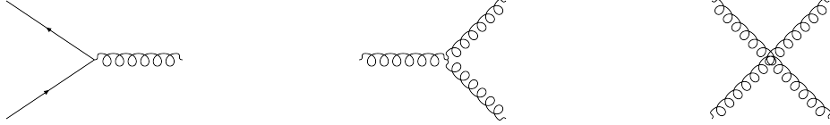
Figure 1.2: QCD vertices [5].
