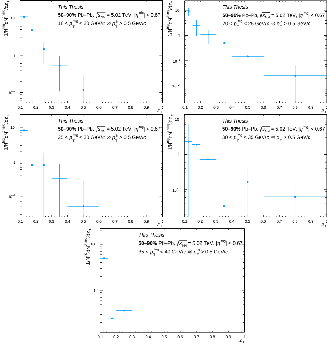
Figure C.64: D(z_T) distribution as a function of z_T in 50-90% Pb-Pb collisions for different p_T^\gamma intervals. From top to bottom: 18 < p_T^\gamma < 20 GeV/c, 20 < p_T^\gamma < 25 GeV/c, 25 < p_T^\gamma < 30 GeV/c, 30 < p_T^\gamma < 35 GeV/c and 35 < p_T^\gamma < 40 GeV/c.
