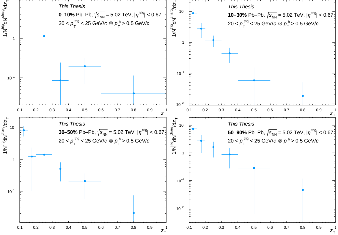
Figure 6.19: The D(z_T) distributions as a function of z_T from \gamma^{\text{iso}} -hadron correlations for a p_T^\gamma between 20 < p_T^\gamma < 25 GeV/c. From top to bottom, 0-10% Pb-Pb collisions, 10-30% Pb-Pb collisions, 30-50% Pb-Pb collisions and 50-90% Pb-Pb collisions.
