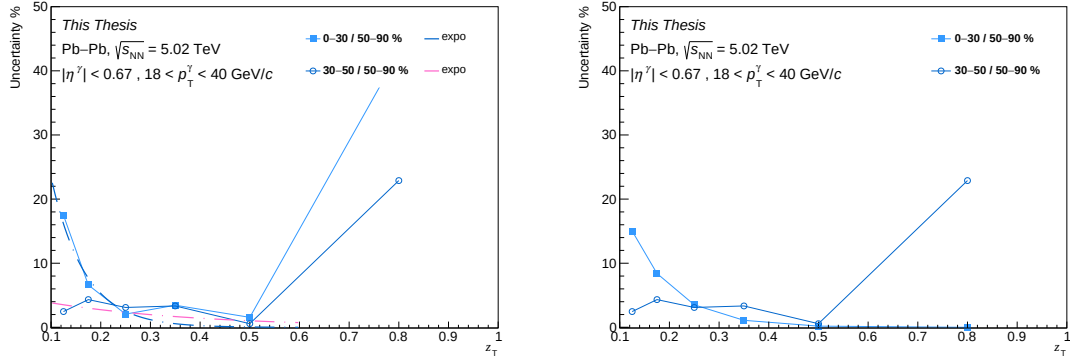
Figure D.2: Left: Systematic uncertainties of the purity on the I_{CP} in 0-30% (full light blue square) and 30-50% (empty blue circle) Pb-Pb collisions. Polishing of the systematic uncertainties using an exponential fit in 0-30% (blue dot-dashed line) and 30-50% (pink dot-dashed line) Pb-Pb collisions. Right: Systematic uncertainties of the purity after the fit.
