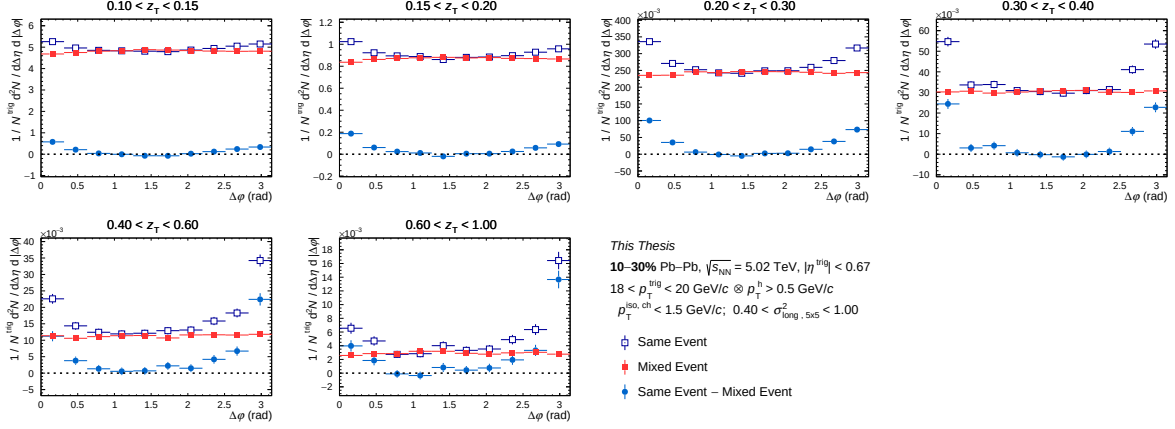
Figure C.26: Azimuthal correlation distribution in 10-30% for isolated wide clusters for the same event (empty blue square), for mixed event (full red square) and for result of the subtraction (full light blue circle) as a function of \Delta\phi for different z_T bins with 18 < p_T^{\text{trig}} < 20 GeV/ c .
