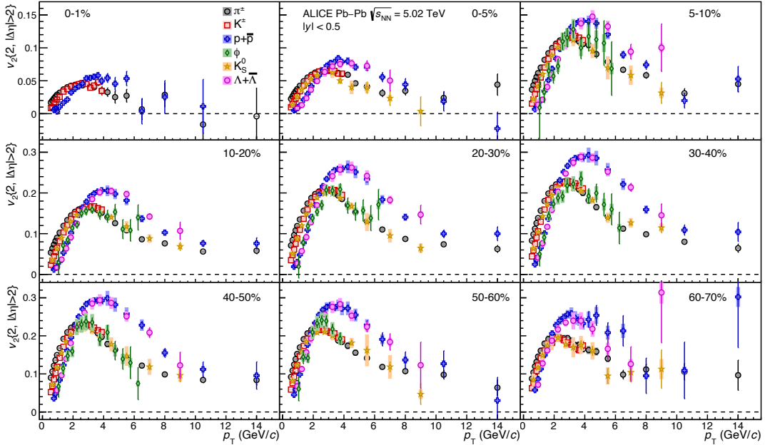
Figure 1.19: Elliptic flow coefficient v_2 of charged pions, charged and neutral kaons, protons, \phi mesons, and hyperons as a function of p_T , measured by the ALICE Collaboration for several centrality classes in Pb–Pb collisions at \sqrt{s_{NN}} = 5.02 TeV [55].
