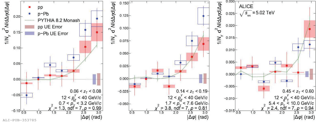
Figure 2.18: Top: \gamma^{\text{iso}} -hadron azimuthal correlation distributions for pp (full red square), p-Pb (full blue circle) data and PYTHIA 8.2 Monash Tune simulation (dashed green line) at \sqrt{s} = 5.02 TeV measured by the ALICE Collaboration. The different panels correspond to different z_T bins [110].
