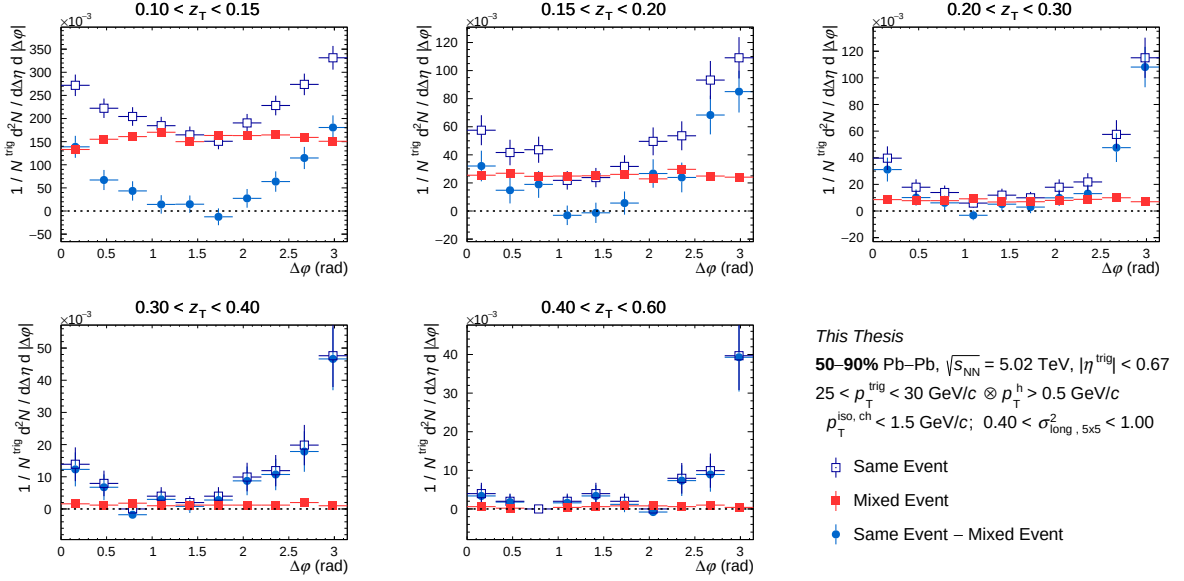
Figure C.38: Azimuthal correlation distribution in 50-90% for isolated wide clusters for the same event (empty blue square), for mixed event (full red square) and for result of the subtraction (full light blue circle) as a function of \Delta\phi for different z_T bins with 25 < p_T^{\text{trig}} < 30 \text{ GeV}/c .
