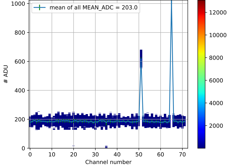
Figure 7.10: Distributions for all the channels, after the pedestal calibration. Average of the ADC distribution as a function of the channel number.
