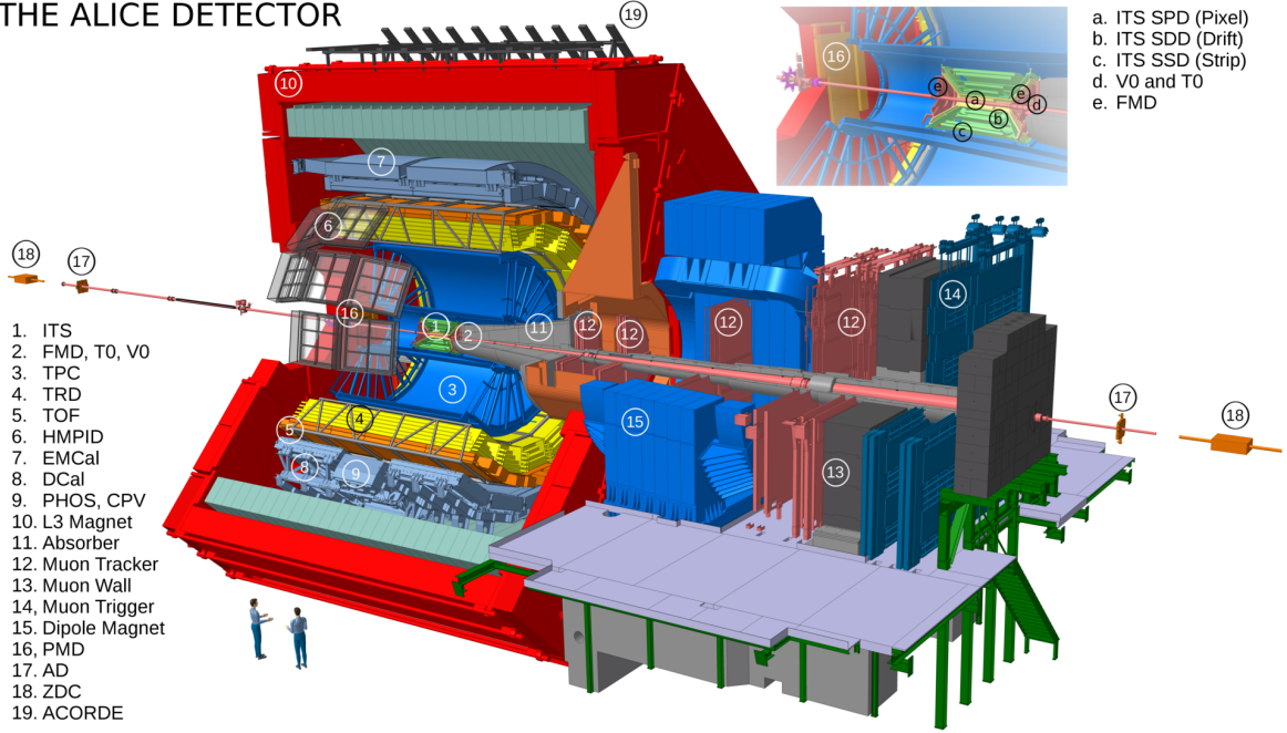
Figure 3.2: The ALICE experimental apparatus with individual sub-detectors labelled during Run 2.
