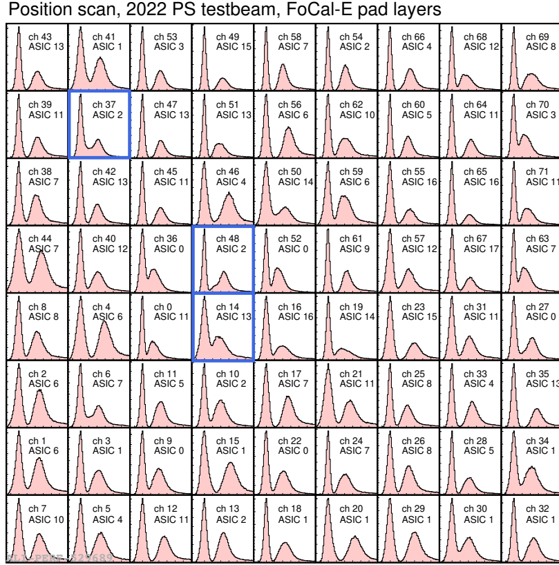
Figure 7.22: Channel scan of MIP’s signal in various ASICs. The squares indicated channels with anomalous MIPs.
