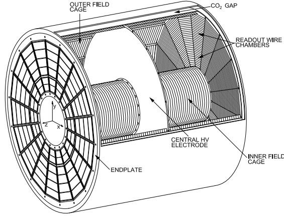
Figure 3.4: Schema of the Time Projection Chamber [122]
