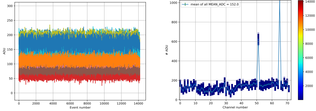
Figure 7.9: ADC distributions before the pedestal calibration. Left: ADC mean distributions for all the channels as a function of the event number. Right: average of the ADC mean distributions as a function of the channel number.
