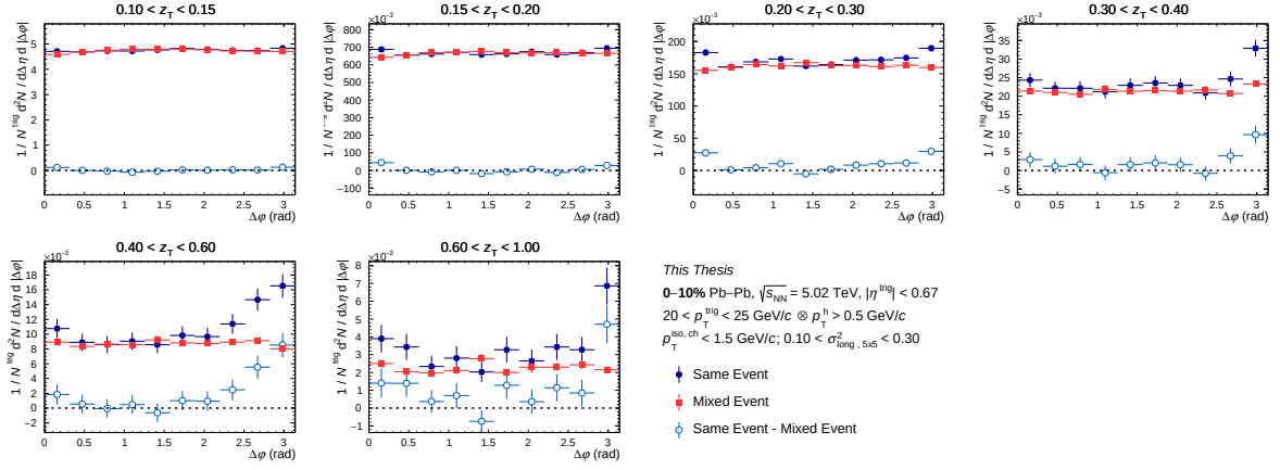
Figure C.2: Azimuthal correlation distribution in 0-10% for isolated narrow clusters for the same event (full blue circle), for mixed event (full red square) and for result of the subtraction (empty light blue circle) as a function of \Delta\varphi for different z_T bins with 20 < p_T^{\text{trig}} < 25 \text{ GeV}/c .
