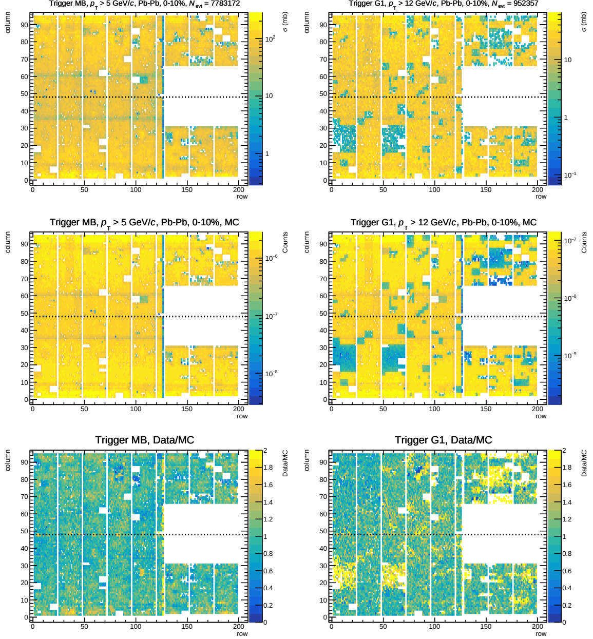
Figure B.1: Calorimeter cell column-row hit map for the period 2015 (LHC15o), Pb-Pb 0-10%, MB (left) and L1- \gamma (right) triggered data, top row for data, second row for the corresponding embedded MC \gamma -jet + jet-jet biased events. The last row for the ratio data over simulation, each one normalized by the histogram integral.
