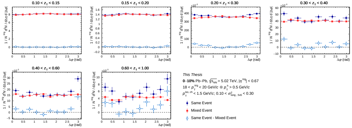
Figure C.1: Azimuthal correlation distribution in 0-10% for isolated narrow clusters for the same event (full blue circle), for mixed event (full red square) and for the result of the subtraction (empty light blue circle) as a function of \Delta\phi for different z_T bins with 18 < p_T^{\text{trig}} < 20 GeV/c.
