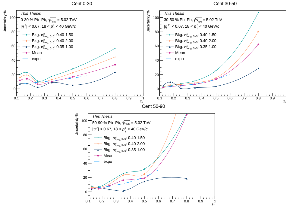
Figure 6.29: Systematic uncertainties due to \sigma_{\text{long}, 5 \times 5}^2 background ranges: 0.40 < \sigma_{\text{long}, 5 \times 5}^2 < 1.50 (full green diamond); 0.40 < \sigma_{\text{long}, 5 \times 5}^2 < 2.00 (full orange cross) and 0.35 < \sigma_{\text{long}, 5 \times 5}^2 < 1.00 (full black triangle) in 0-30% (top left), in 30-50% (top right) and in 50-90% (bottom) Pb-Pb collisions. The average of the systematic uncertainties in the three ranges is pink, while the exponential fit is shown with a dashed light blue line.
