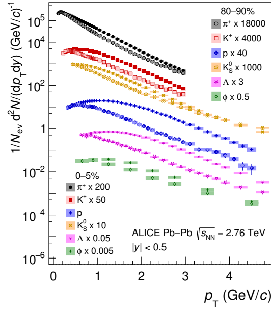
Figure 1.17: Transverse momentum spectra of charged pions, kaons, protons, \Lambda baryons, and \phi mesons for central (0–5%) (full marker) and peripheral (80–90%) (empty marker) Pb–Pb collisions at \sqrt{s_{NN}} = 2.76 TeV measured by ALICE [38].
