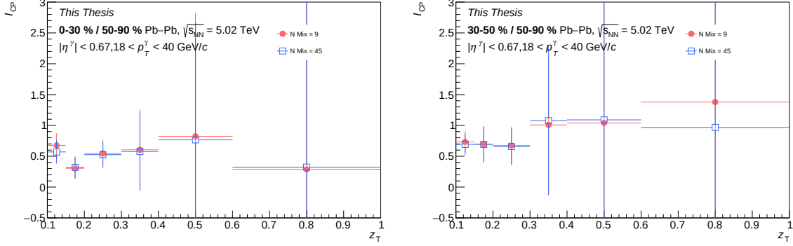
Figure D.5: The I_{CP} distributions obtained using 9 centrality bins (full pink circle) and 45 centrality bins (empty blue square) for filling the mixed event pool in 0-30% (left) and 30-50% (right).
