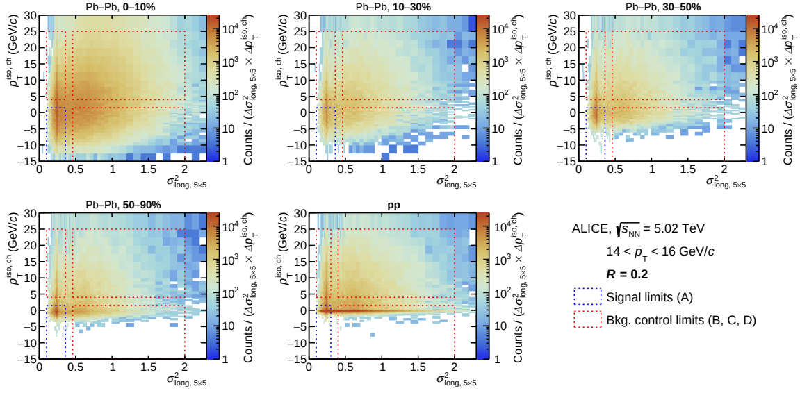
Figure 5.17: Illustration of the parametric-space of the photon p_T^{\text{iso}} and \sigma_{\text{long}}^2 ( \sigma_{\text{long}, 5 \times 5}^2 ) for and 14 < p_T < 16 GeV/c in five centrality classes in Pb–Pb collisions and in pp collisions, used to estimate the background yield in the signal region (A) from the observed yields in the three control regions (B, C and D). The dashed boxes indicate the limits of each class [148].
