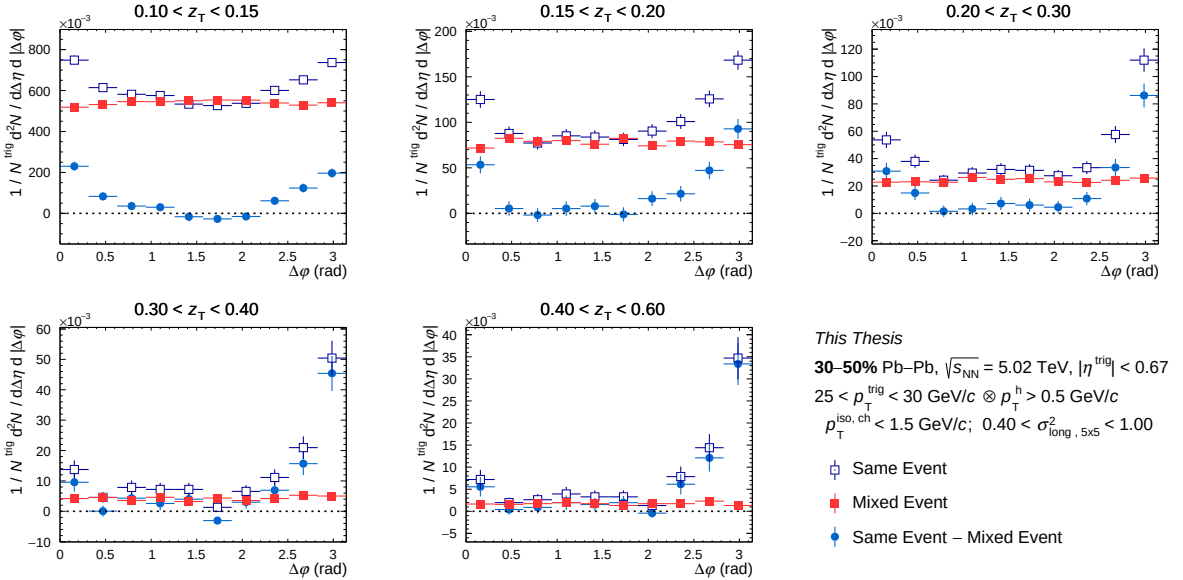
Figure C.33: Azimuthal correlation distribution in 30–50% for isolated wide clusters for the same event (empty blue square), for mixed event (full red square) and for result of the subtraction (full light blue circle) as a function of \Delta\phi for different z_T bins with 25 < p_T^{\text{trig}} < 30 GeV/ c .
