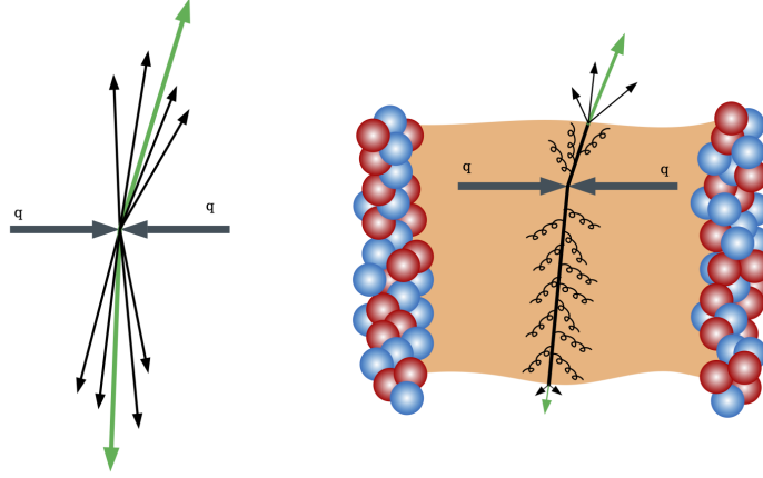
Figure 1.22: Sketch of jet production in pp collisions (left) and in AA collisions (right).
