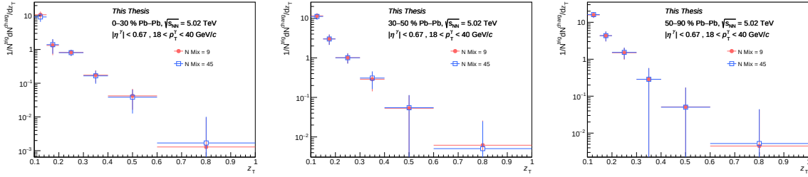
Figure 6.31: The differential z_T distributions obtained using 9 centrality bins (full pink circle) and 45 centrality bins (empty blue square) for filling the mixed event pool in 0-30% (left), 30-50% (middle) and 50-90% (right).
