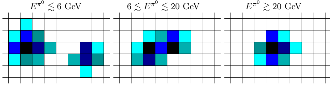
Figure 5.6: Schematic view of cluster energy repartition in cells in low particle multiplicity environment, for two decay photons from a neutral meson ( \pi^0 or \eta for example) at low (left), medium (middle) and high meson energy (right). The opening angle of the decays gets smaller due to the Lorentz boost and thus the two showers tend to merge at high energy. Darker colours indicate higher energy cells [135].
