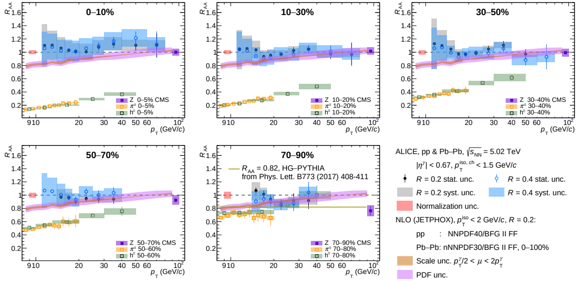
Figure 2.11: Nuclear modification factor for isolated photons at \sqrt{s_{\text{NN}}} = 5.02 TeV for isolation cone radii R = 0.2 (full black circle) and R = 0.4 (empty blue circle). Distribution compared to the R_{\text{AA}} for charged particles [65] (empty green square) and charged pions [97] (empty orange square) from ALICE, and to the ratio of the Z bosons (full violet square) production in each centrality class to the 0–90% class measured by CMS [98]. The bands correspond to pQCD calculations with JETPHOX for Pb–Pb collisions (nPDF) for 0–100% centrality over pp collisions (PDF). The width of each band corresponds to the scale (orange) and PDF (pink) uncertainties [93].
