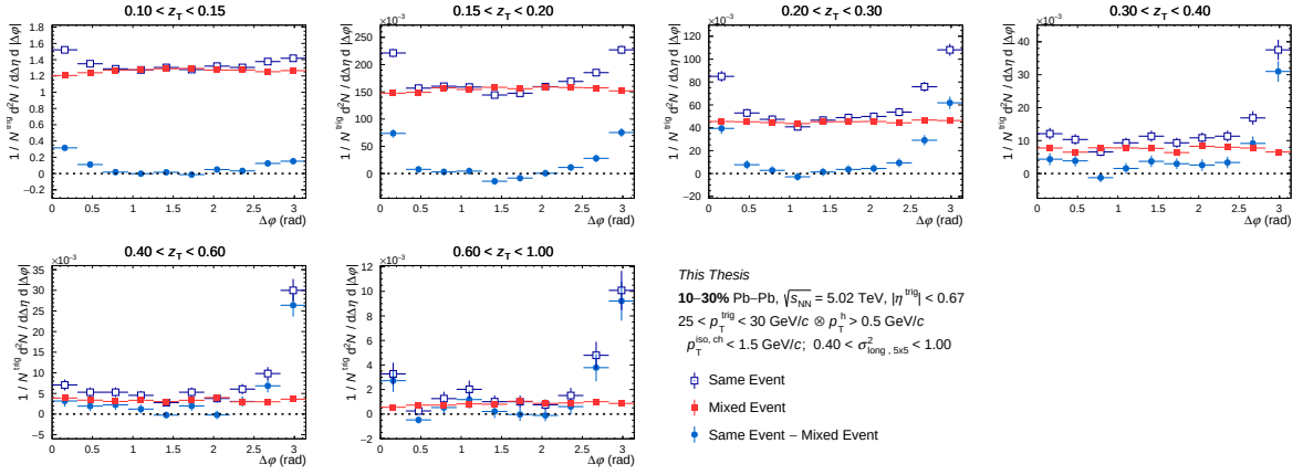
Figure C.28: Azimuthal correlation distribution in 10-30% for isolated wide clusters for the same event (empty blue square), for mixed event (full red square) and for result of the subtraction (full light blue circle) as a function of \Delta\phi for different z_T bins with 25 < p_T^{trig} < 30 GeV/c.
