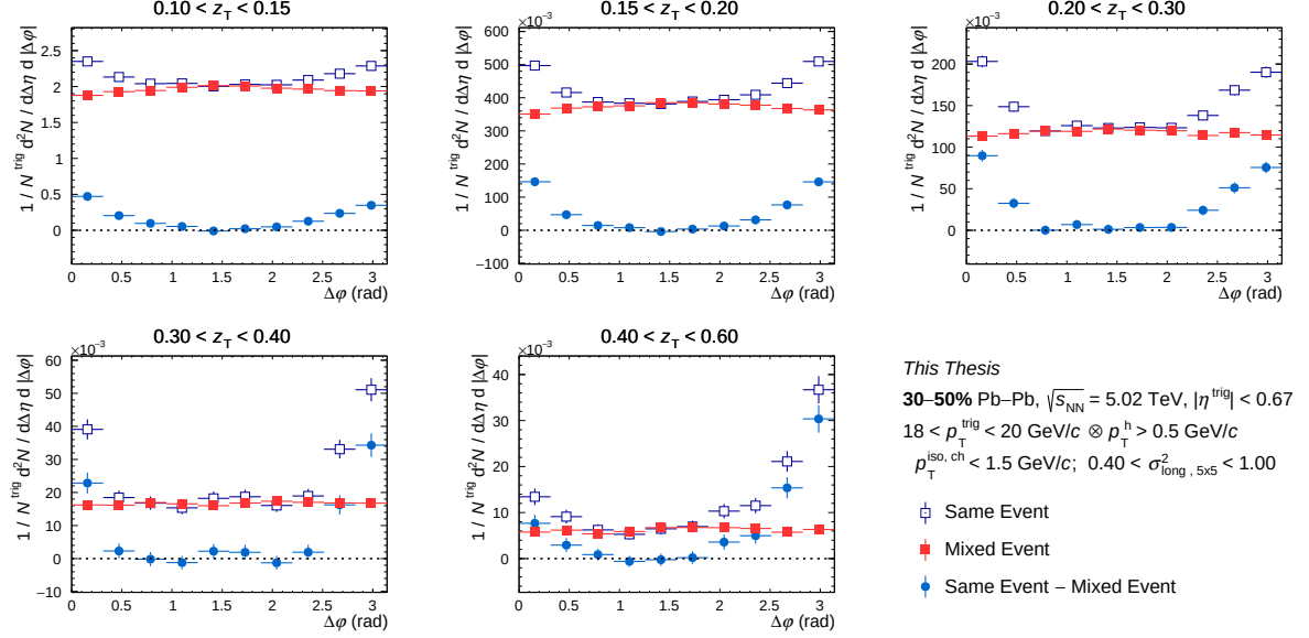
Figure C.31: Azimuthal correlation distribution in 30-50% for isolated wide clusters for the same event (empty blue square), for mixed event (full red square) and for result of the subtraction (full light blue circle) as a function of \Delta\phi for different z_T bins with 18 < p_T^{\text{trig}} < 20 GeV/c.
