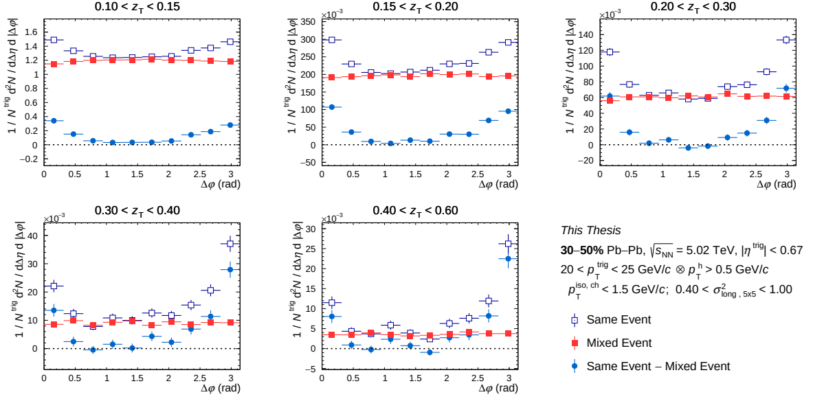
Figure C.32: Azimuthal correlation distribution in 30–50% for isolated wide clusters for the same event (empty blue square), for mixed event (full red square) and for result of the subtraction (full light blue circle) as a function of \Delta\phi for different z_T bins with 20 < p_T^{\text{trig}} < 25 GeV/ c .
