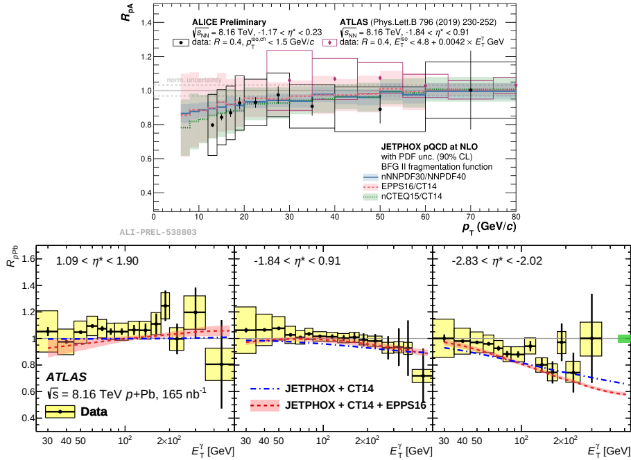
Figure 2.8: Top: R_{pA} of isolated-photon production in p–Pb collisions at \sqrt{s_{NN}} = 8.16 TeV by ALICE (full black circle) and by ATLAS (full pink circle) compared with different JETPHOX calculations using nNNPDF30 (blue line), using CT14 proton PDF + EPPS16 Pb nPDF (red dashed line) and using CT14 proton PDF + nCTEQ15 Pb nPDF (dotted green line) [91]. Bottom: nuclear modification factor R_{pA} at \sqrt{s_{NN}} = 8.16 TeV in p–Pb collisions measured purely by ATLAS (full black circle) at different rapidities confronted with JETPHOX calculations using CT14 proton PDF (blue dot-dashed line) and using CT14 proton PDF + EPPS16 Pb nPDF (red dashed line) [92].
