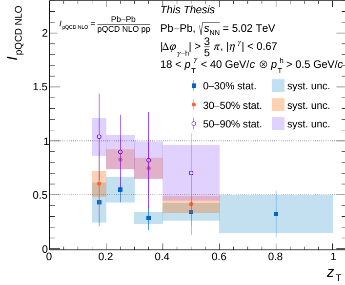
Figure 6.38: The I_{\text{pQCD NLO}} distributions as a function of z_T in 0-30% (full blue square), 30-50% (full orange circle) and 50-90% (empty violet circle) Pb-Pb collisions.
