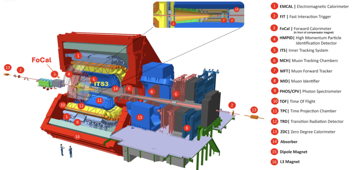
Figure 7.1: ALICE detector configuration for Run 4. FoCal is located in front of the compensator magnet and outside the magnet doors on the A-side, opposite the muon arm. Figure taken from [166].
