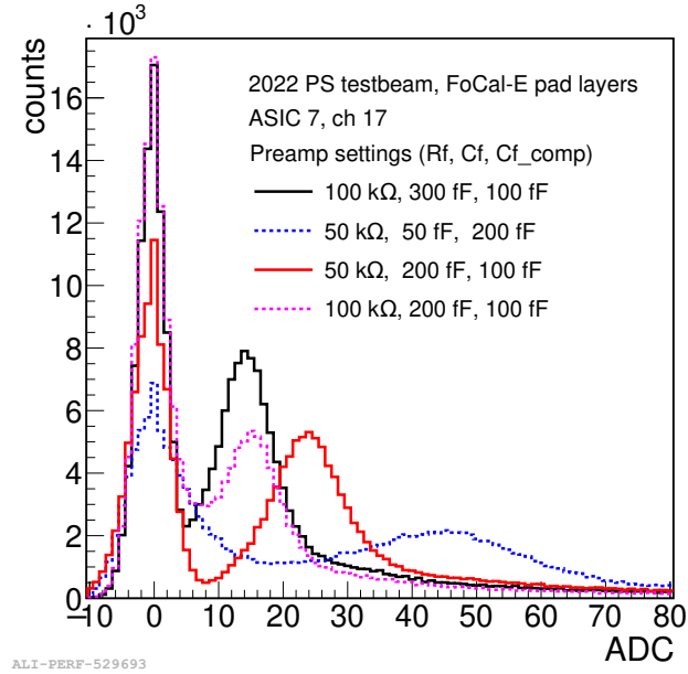
Figure 7.21: ADC response obtained using four different gains for a specific ASIC and channel [179].
