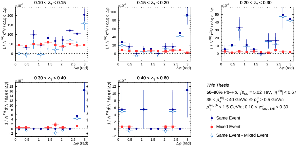
Figure C.20: Azimuthal correlation distribution in 50-90% for isolated narrow clusters for the same event (full blue circle), for mixed event (full red square) and for result of the subtraction (empty light blue circle) as a function of \Delta\phi for different z_T bins with 35 < p_T^{\text{trig}} < 40 GeV/c.
