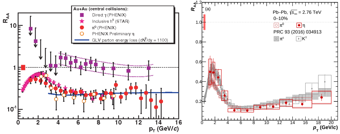
Figure 2.2: Left: nuclear modification factor of direct \gamma (full violet square), inclusive hadrons (full pink star), \pi^0 mesons (full red circle) and \eta mesons (empty yellow circle) as a function of p_T for central Au–Au collisions at RHIC [77, 78]. Right: nuclear modification factor for the \pi^0 (empty red circle), \eta mesons (full red circle), kaons (full grey circle) and charged pions (empty grey circle) in 0–10% Pb–Pb collisions at \sqrt{s_{NN}} = 2.76 TeV measured by ALICE [79].
