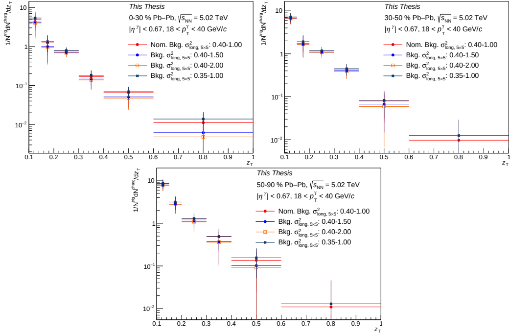
Figure 6.28: The D(z_T) distributions obtained using different \sigma_{\text{long}, 5 \times 5}^2 background ranges: 0.40 < \sigma_{\text{long}, 5 \times 5}^2 < 1.00 (full red circle) 0.40 < \sigma_{\text{long}, 5 \times 5}^2 < 1.50 (full blue circle); 0.40 < \sigma_{\text{long}, 5 \times 5}^2 < 2.00 (empty orange square) and 0.35 < \sigma_{\text{long}, 5 \times 5}^2 < 1.00 (full black cross) in 0-30% (top left), in 30-50% (top right) and in 50-90% (bottom) Pb-Pb collisions.
