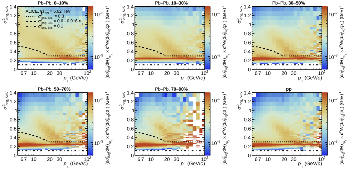
Figure 5.8: Inclusive cluster \sigma^2_{\text{long}, 5 \times 5} distribution as a function of p_T in data for five different centralities in Pb–Pb collisions and for pp collisions. The dotted line corresponds to the tight value of the upper selection limit ( \sigma^2_{\text{long}, 5 \times 5} = 0.3 ) for single photon candidate clusters (narrow clusters), the dashed line corresponds to a looser photon upper selection used in Pb–Pb collisions below 18 GeV/c. The dot-dashed line defines a lower selection limit ( \sigma^2_{\text{long}, 5 \times 5} = 0.1 ) used in Pb–Pb and pp collisions.
