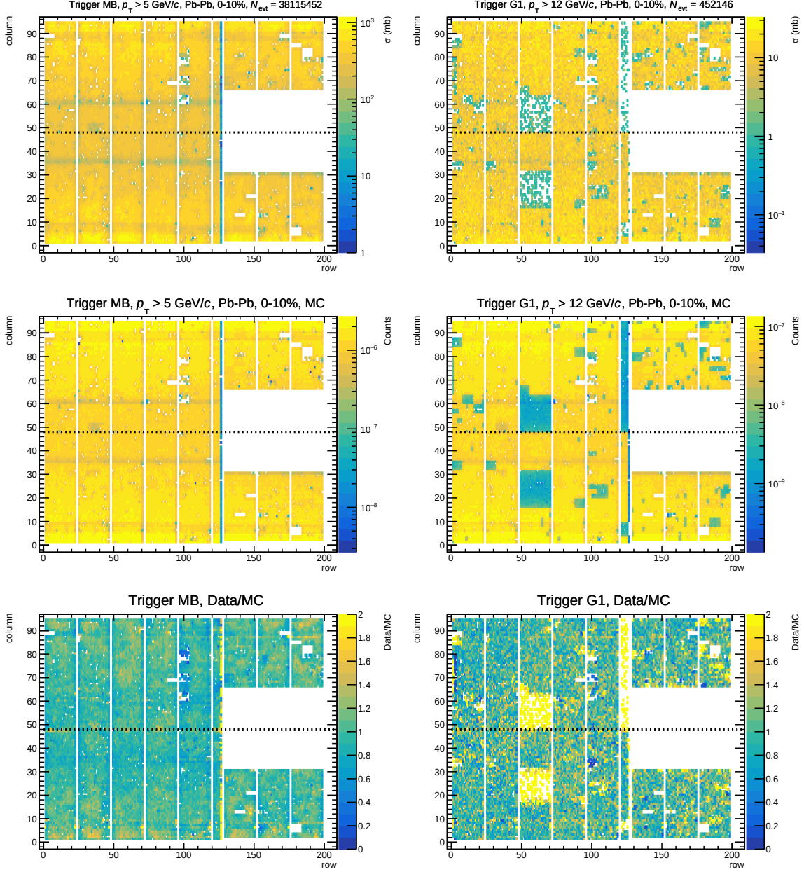
Figure B.2: Calorimeter cell column-row hit map for first period of 2018 (LHC18q), Pb-Pb 0-10%, MB (left) and L1- \gamma (right) triggered data, top row for data, second row for the corresponding embedded MC \gamma -jet + jet-jet biased events. The last row for the ratio data over simulation, each one normalized by the histogram integral.
