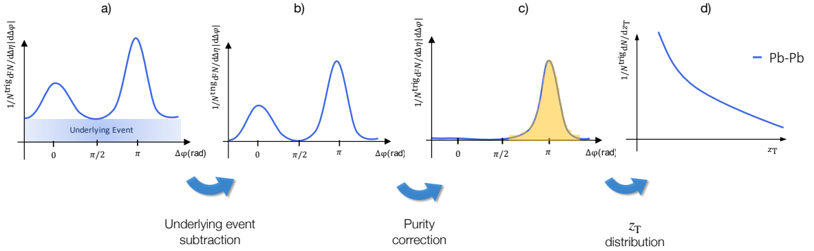
Figure 6.5: Sketch of the three main steps of the analysis.
