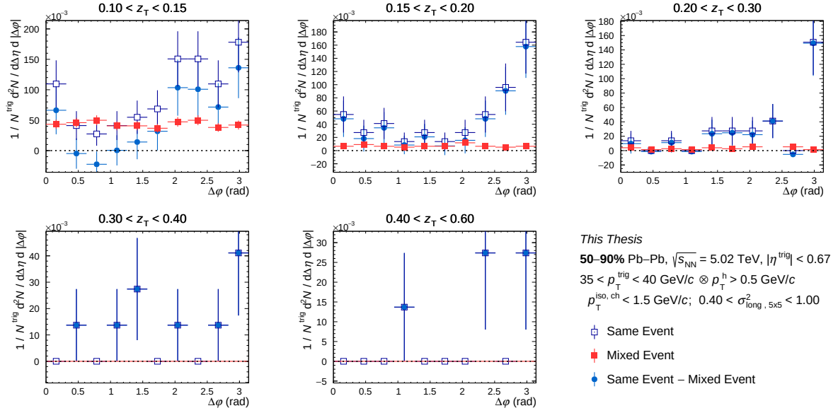
Figure C.40: Azimuthal correlation distribution in 50-90% for isolated wide clusters for the same event (empty blue square), for mixed event (full red square) and for result of the subtraction (full light blue circle) as a function of \Delta\phi for different z_T bins with 35 < p_T^{\text{trig}} < 40 GeV/c.
