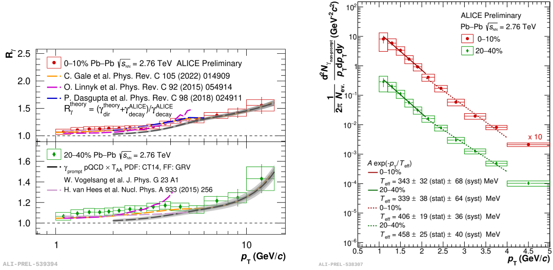
Figure 2.3: Left: R_\gamma as a function of p_T for 0–10% central (top, red full circle) and 20–40% semi-central (bottom, green full diamond) Pb–Pb collisions at \sqrt{s_{NN}} = 2.76 TeV compared with different model calculations by ALICE. Right: thermal photon spectra as a function of p_T for 0–10% central (red full circle) and 20–40% semi-central (green full diamond) in Pb–Pb collisions at \sqrt{s_{NN}} = 2.76 TeV by the ALICE Collaboration [80]
