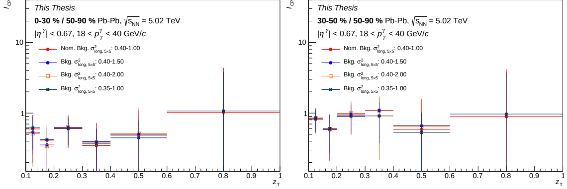
Figure D.3: The I_{CP} distributions obtained using different \sigma_{\text{long}, 5 \times 5}^2 background ranges: 0.40 < \sigma_{\text{long}, 5 \times 5}^2 < 1.00 (full red circle) 0.40 < \sigma_{\text{long}, 5 \times 5}^2 < 1.50 (full blue circle); 0.40 < \sigma_{\text{long}, 5 \times 5}^2 < 2.00 (empty orange square) and 0.35 < \sigma_{\text{long}, 5 \times 5}^2 < 1.00 (full black cross) in 0-30% (top left) and in 30-50% (top right) Pb-Pb collisions.
