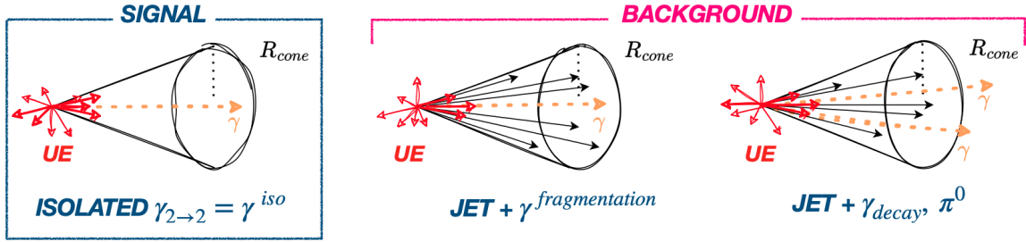
Figure 5.10: Production of different types of photons with the isolation cone sketched. Left: isolated photon produced alone. Middle and right: fragmentation photons and decay photons produced in combination with a jet.
