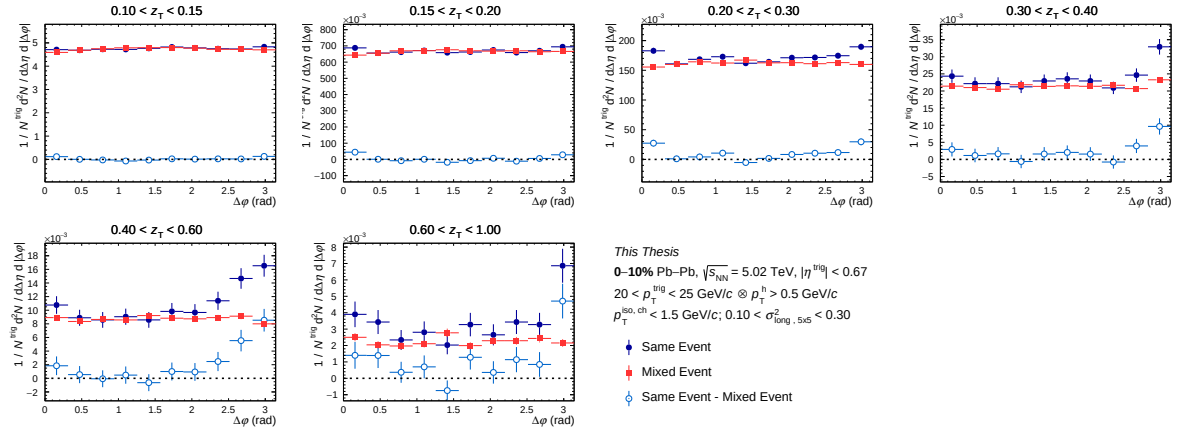
Figure 6.9: Azimuthal correlation distributions in 0-10% for isolated narrow clusters for the same event (full blue circle), for the mixed event (full red square) and the result of the subtraction (empty light blue circle) as a function of \Delta\varphi for different z_T bins with 20 < p_T^{\text{trig}} < 25 \text{ GeV}/c .
