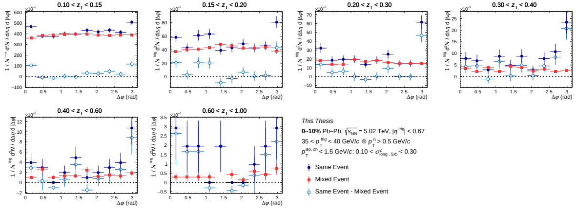
Figure C.5: Azimuthal correlation distribution in 0-10% for isolated narrow clusters for the same event (full blue circle), for mixed event (full red square) and for the result of the subtraction (empty light blue circle) as a function of \Delta\varphi for different z_T bins with 35 < p_T^{\text{trig}} < 40 GeV/c.
