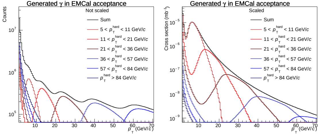
Figure 6.2: Left: Not scaled GJ MC distributions as a function of p_T . Right: Scaled GJ MC distributions as a function of p_T . The distributions are presented for various p_T^{\text{hard}} intervals.
