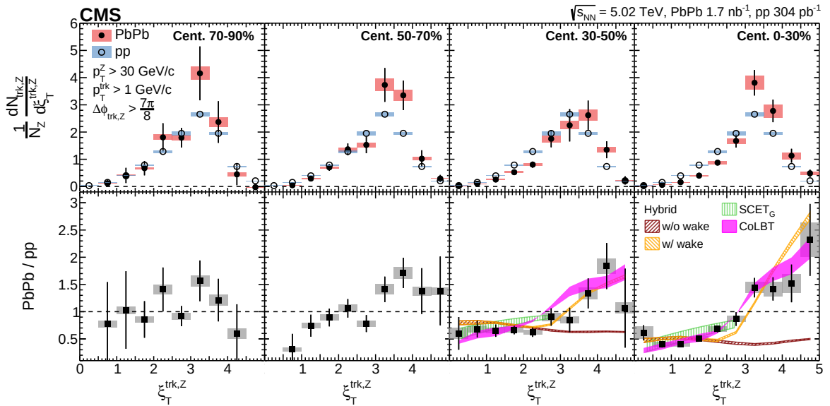
Figure 2.15: Top: distributions of \xi_T^{\text{trk,Z}} in pp collisions compared to Pb–Pb collisions in various centrality bins. Bottom: ratios of the Pb–Pb to pp distributions. The vertical bars and coloured boxes represent the statistical and systematic uncertainties, respectively. The distributions are compared with CoLBT-hydro model (pink line) and HYBRID model with wake (yellow line) and without wake (brown line) [106].
