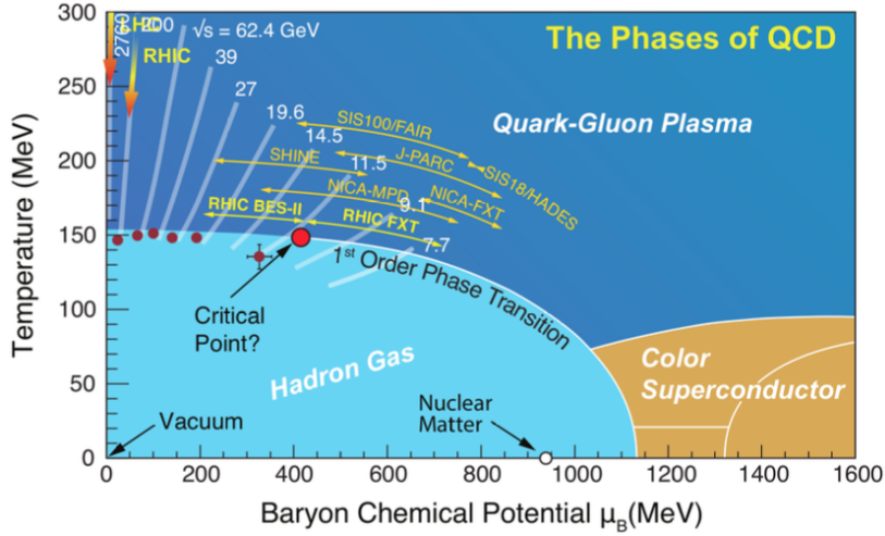
Figure 1.8: The QCD phase diagram as a function of the temperature and the baryon-chemical potential [25].
