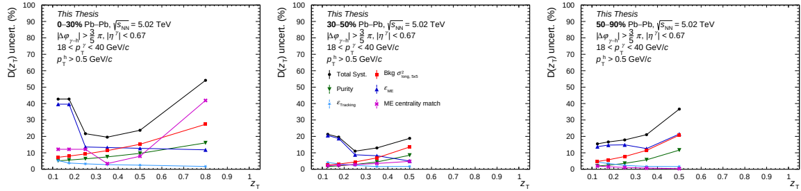
Figure 6.34: Various systematic uncertainty sources for the three centrality classes measured.
