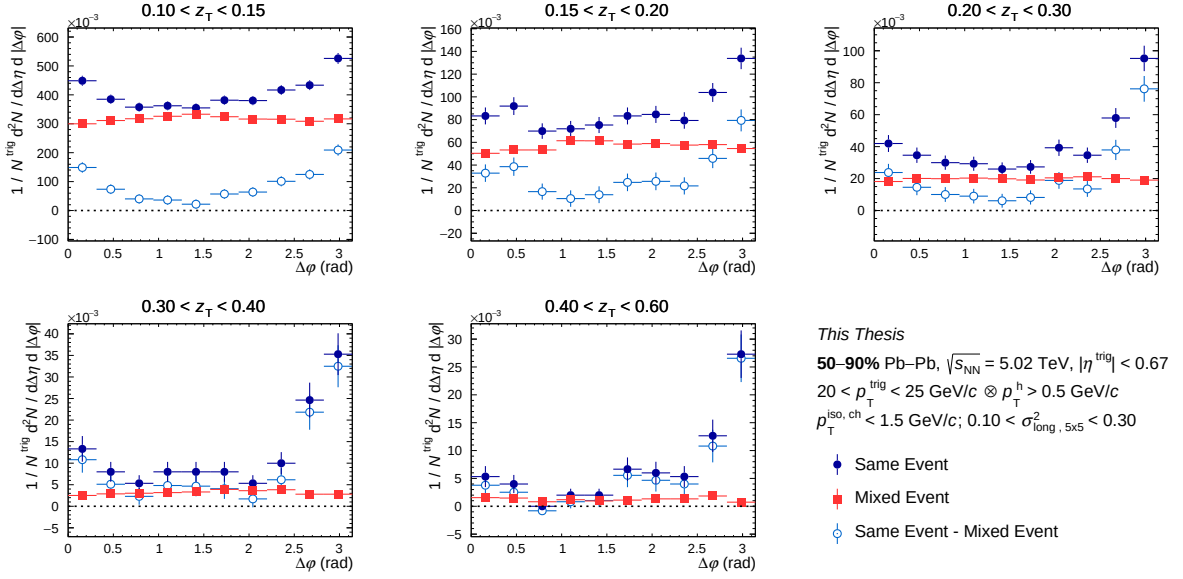
Figure C.17: Azimuthal correlation distribution in 50-90% for isolated narrow clusters for the same event (full blue circle), for mixed event (full red square) and for result of the subtraction (empty light blue circle) as a function of \Delta\phi for different z_T bins with 20 < p_T^{\text{trig}} < 25 GeV/c.
