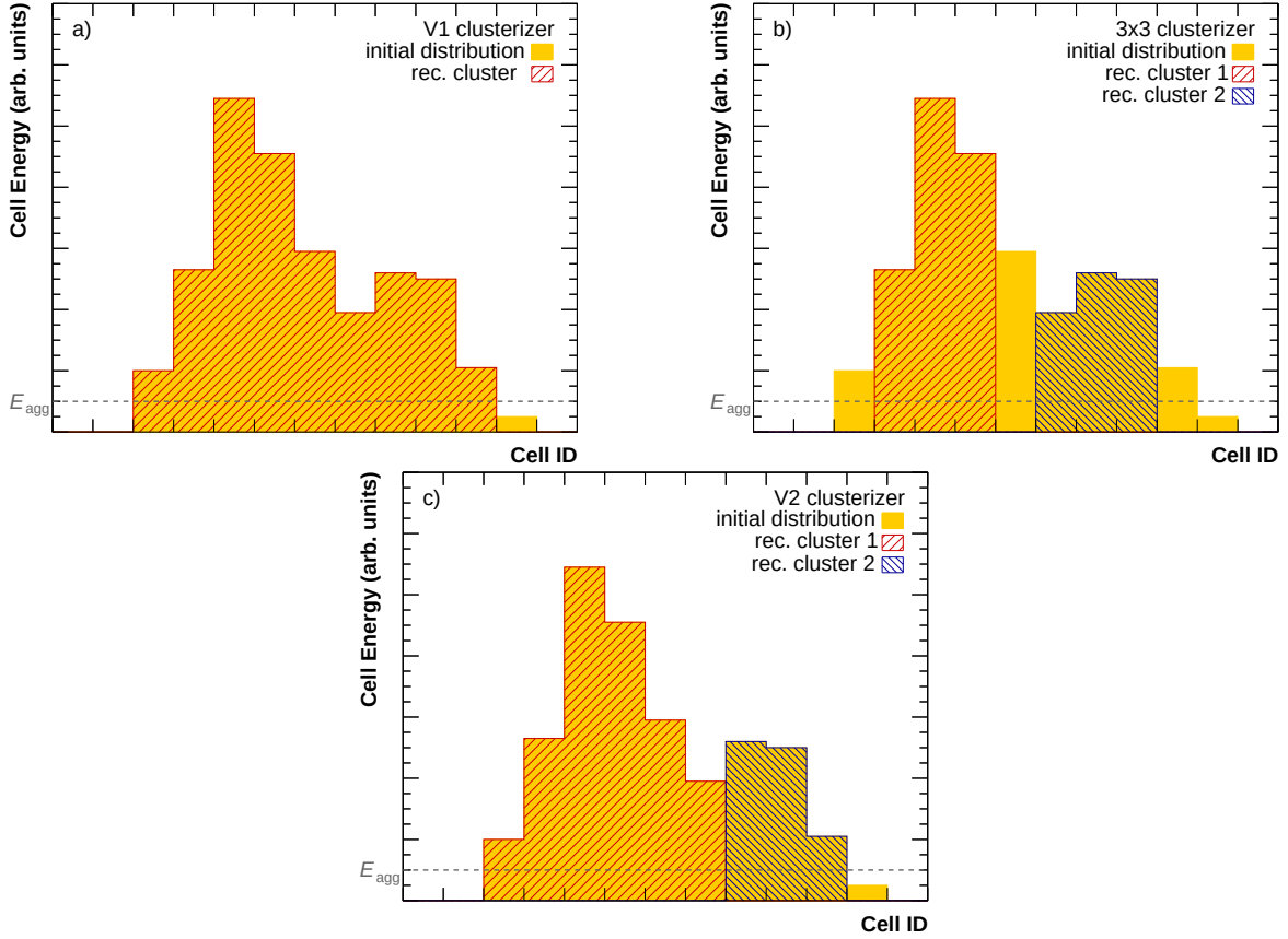
Figure 5.1: Schematic comparison of different clusterization algorithms: a) V1, b) 3 \times 3 , c) V2. Yellow boxes represent the energy in each cell. E_{\text{agg}} is the aggregation energy. Different clusters are indicated by blue and red hatched areas [135].
