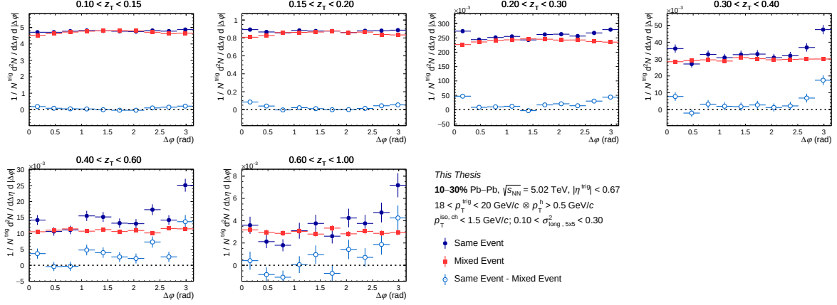
Figure C.6: Azimuthal correlation distribution in 10-30% for isolated narrow clusters for the same event (full blue circle), for mixed event (full red square) and for the result of the subtraction (empty light blue circle) as a function of \Delta\varphi for different z_T bins with 18 < p_T^{trig} < 20 GeV/c.
