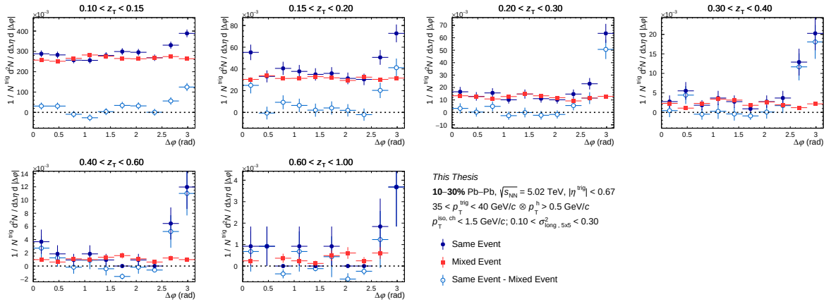
Figure C.10: Azimuthal correlation distribution in 10-30% for isolated narrow clusters for the same event (full blue circle), for mixed event (full red square) and for the result of the subtraction (empty light blue circle) as a function of \Delta\phi for different z_T bins with 35 < p_T^{trig} < 40 GeV/c.
