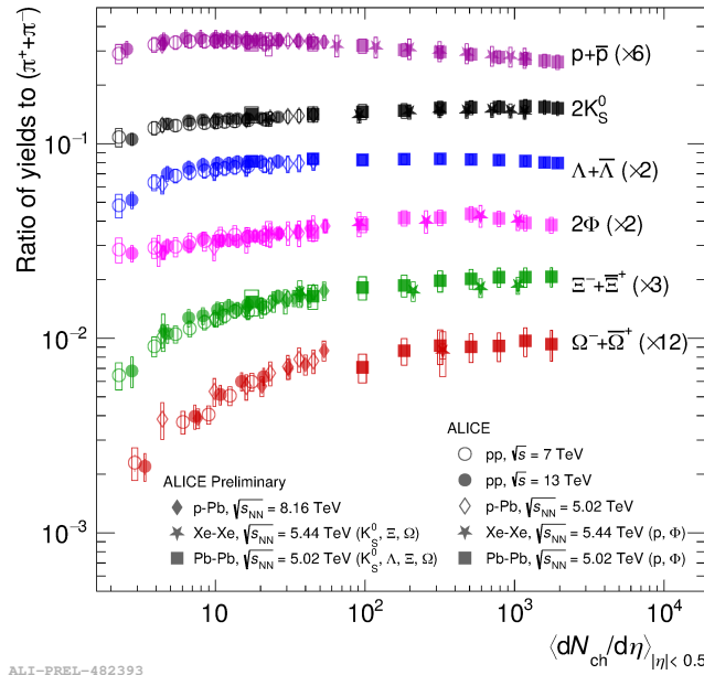
Figure 1.16: Ratios of the p_T -integrated yield of hadrons with strange-quark content and charged pions as a function of the charged-particle multiplicity at midrapidity, measured by the ALICE Collaboration in various collision systems and at different center-of-mass energies [53].
