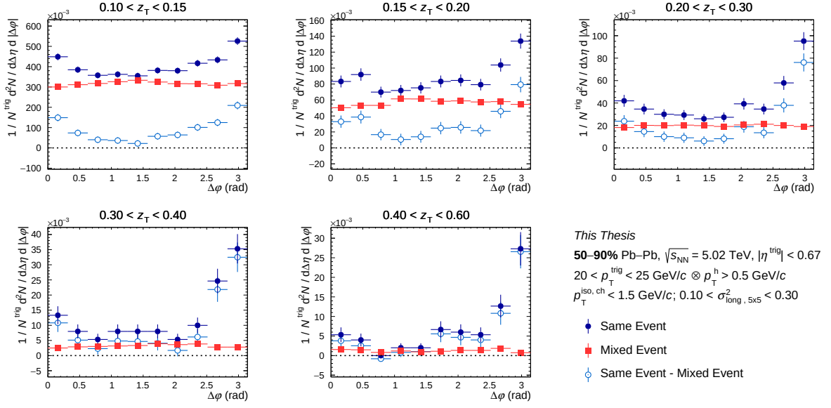
Figure 6.10: Azimuthal correlation distributions in 50-90% for isolated narrow clusters for the same event (full blue circle), for mixed event (full red square) and the result of the subtraction (empty light blue circle) as a function of \Delta\phi for different z_T bins with 20 < p_T^{\text{trig}} < 25 GeV/c.
