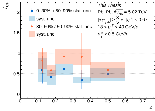
Figure 6.39: I_{\text{CP}} as a function of z_T for central (full blue square) and for semi-central (full orange circle) Pb-Pb collisions.
