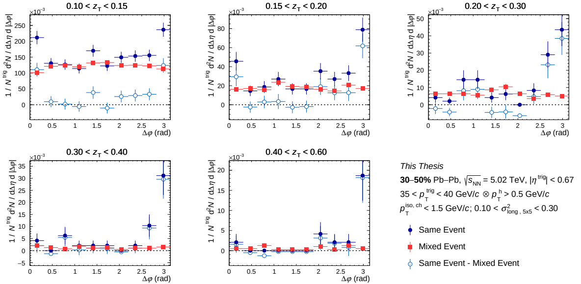
Figure C.15: Azimuthal correlation distribution in 30-50% for isolated narrow clusters for the same event (full blue circle), for mixed event (full red square) and for result of the subtraction (empty light blue circle) as a function of \Delta\varphi for different z_T bins with 35 < p_T^{\text{trig}} < 40 \text{ GeV}/c .
