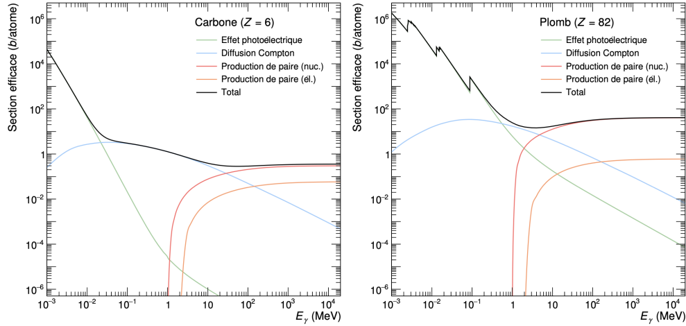
Figure 4.1: Photon-matter interaction cross section and its three main contributions as a function of incident photon energy in carbon (left) and lead (right) [136]. Pair production actually has two components, linked to the nuclear (nuc.) and electronic (el.) electric fields of the atom near which the process takes place [137].
