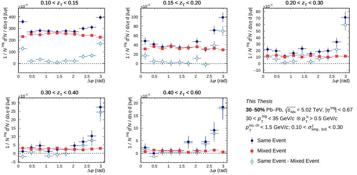
Figure C.14: Azimuthal correlation distribution in 30-50% for isolated narrow clusters for the same event (full blue circle), for mixed event (full red square) and for result of the subtraction (empty light blue circle) as a function of \Delta\varphi for different z_T bins with 30 < p_T^{\text{trig}} < 35 \text{ GeV}/c .
