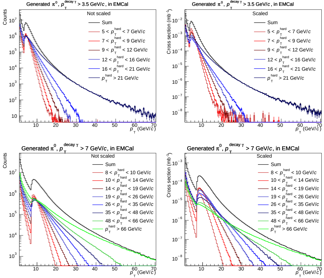
Figure 6.3: Left: Not scaled JJ-low (top) and JJ-high (bottom) MC distributions as a function of p_T . Right: Scaled JJ-low (top) and JJ-high (bottom) distributions as a function of p_T . The distributions are presented for various p_T^{\text{hard}} intervals.
