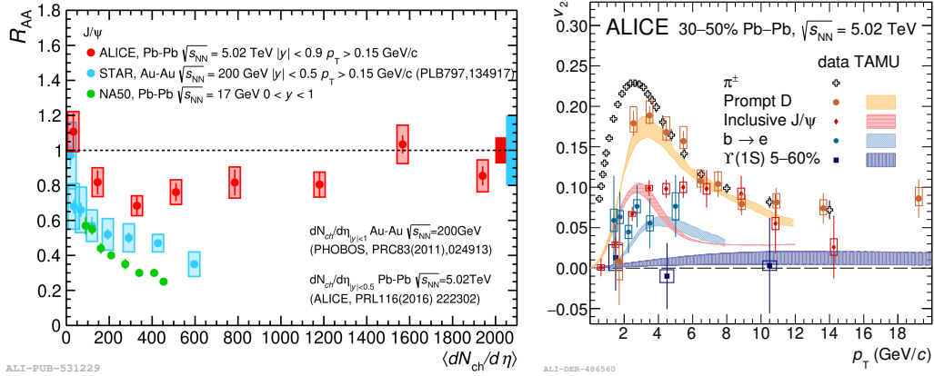
Figure 1.21: Left: R_{AA} of the J/\psi hadron measured in heavy-ion collisions at different center-of-mass energies as a function of the charged multiplicity by ALICE (red full circle), by NA50 (green full circle) and by STAR (light blue full circle) experiments [38]. Right: v_2 coefficient of charged pions, prompt D mesons, electrons from beauty-hadron decays, J/\psi mesons, and \Upsilon mesons as a function of p_T for Pb–Pb collisions at \sqrt{s_{NN}} = 5.02 TeV in the 30–50% centrality class [38].
