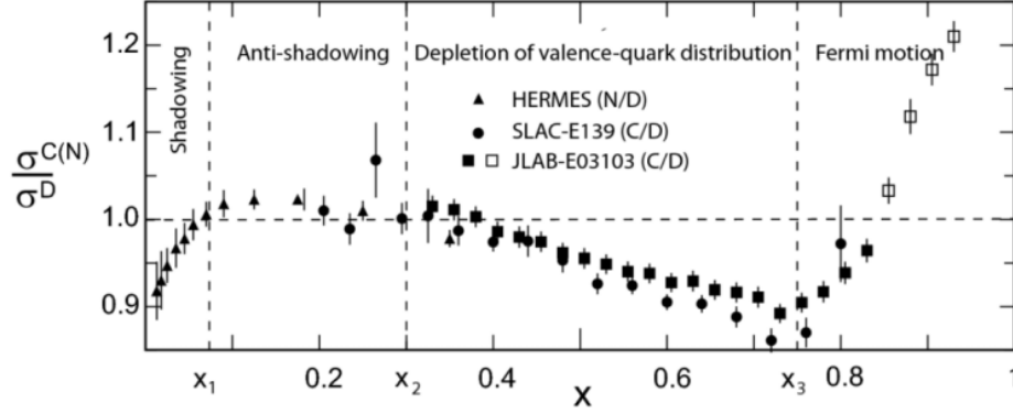
Figure 1.10: Measurements of the nuclear modification of the PDFs performed by several experiments in a wide range of Bjorken x .
