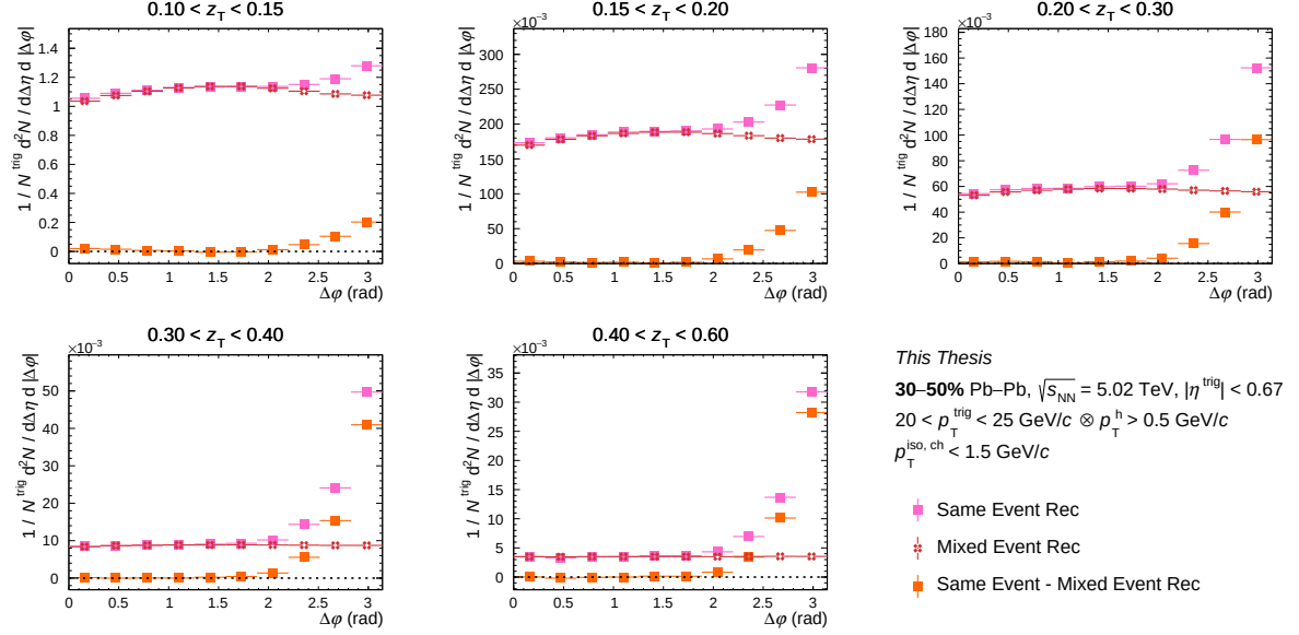
Figure 6.17: Azimuthal correlation distribution 30-50% Pb-Pb collisions for pp PYTHIA 8 \gamma -jet events embedded into MB data of the Same Event (full pink square), of the Mixed Event (red cross) and of the Same Event without UE (full orange square) as a function of \Delta\phi for different z_T bins with 20 < p_T^{\text{trig}} < 25 GeV/c.
