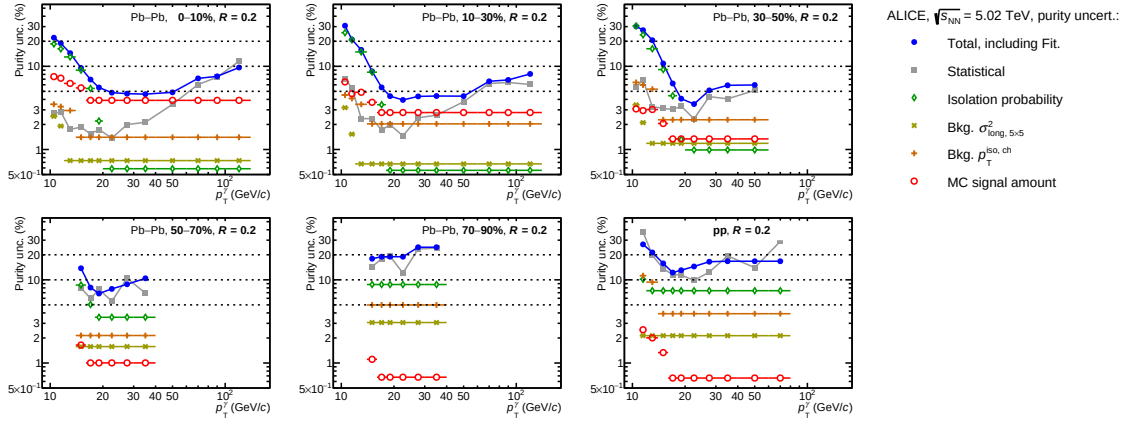
Figure 6.25: Isolated photon purity uncertainty components for R = 0.2 in pp and Pb–Pb collisions. Purity calculated with the ABCD method [93].
