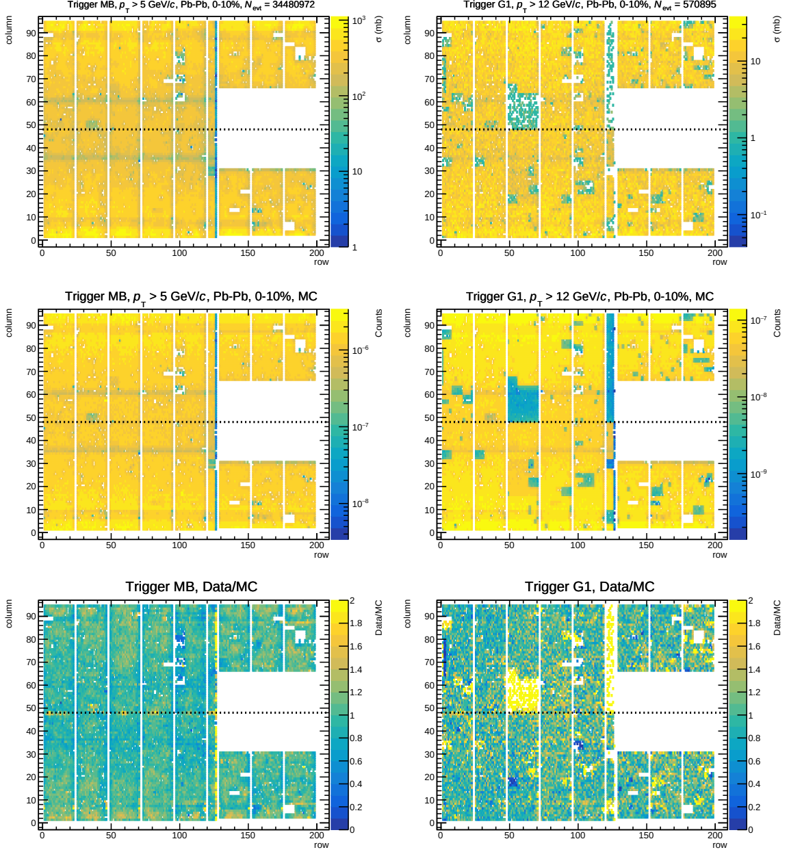
Figure B.3: Calorimeter cell column-row hit map for the second period of 2018 (LHC18r), Pb-Pb 0-10%, MB (left) and L1- \gamma (right) triggered data, top row for data, second row for the corresponding embedded MC \gamma -jet + jet-jet biased events. The last row for the ratio data over simulation, each one normalized by the histogram integral.
