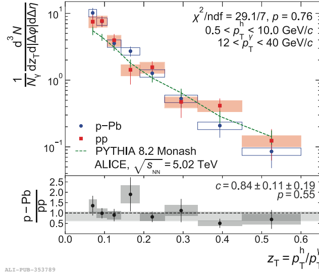
Figure 2.19: \gamma^{\text{iso}} -hadron fragmentation function for pp (full red square), p-Pb data (full blue circle) and PYTHIA 8.2 simulation (dashed green line). The ratio between p-Pb and pp distributions (black marker) is shown in the bottom panel. The boxes represent the systematic uncertainties while the vertical bars indicate the statistical uncertainties [110].
