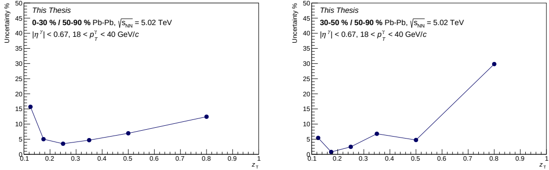
Figure D.6: Systematic uncertainties for different numbers of centrality bins used for filling the mixed event pool in 0-30% (left) and 30-50% (right).
