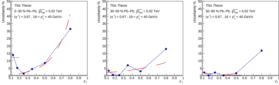
Figure 6.33: Systematic uncertainty for different numbers of centrality bins used for filling the mixed event pool in 0-30% (left), 30-50% (middle) and 50-90% (right).
