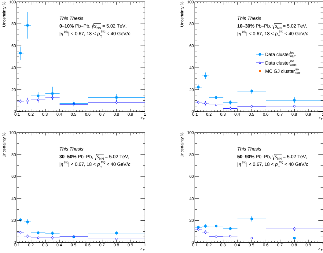
Figure 6.23: Systematic uncertainty of the mixed event for isolated narrow (full light blue circle) and wide (empty blue circle) clusters as a function of z_T . From top to bottom, 0-10% Pb-Pb collisions, 10-30% Pb-Pb collisions, 30-50% Pb-Pb collisions and 50-90% Pb-Pb collisions.
