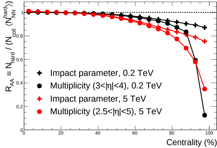
Figure 3.7: R_{AA} versus centrality for Au–Au and Pb–Pb collisions at \sqrt{s_{NN}} = 0.2 TeV (black markers) and \sqrt{s_{NN}} = 5.02 TeV (red markers), respectively, calculated with HG-PYTHIA model [99].
