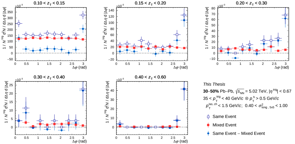
Figure C.35: Azimuthal correlation distribution in 30-50% for isolated wide clusters for the same event (empty blue square), for mixed event (full red square) and for result of the subtraction (full light blue circle) as a function of \Delta\phi for different z_T bins with 35 < p_T^{\text{trig}} < 40 GeV/c.
