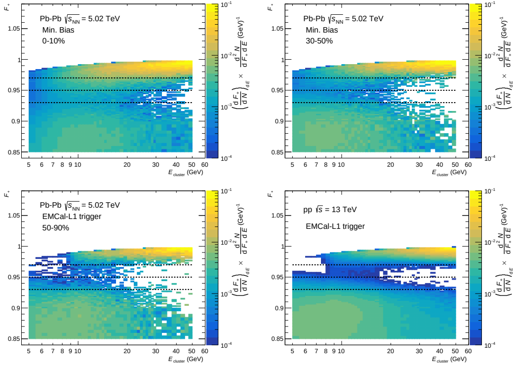
Figure 5.4: The exoticity F_+ versus E_{\text{cluster}} for 0-10% and 30-50% in minimum bias Pb-Pb collisions at \sqrt{s_{\text{NN}}} = 5.02 TeV (top rows) and for 50-90% Pb-Pb collisions at \sqrt{s_{\text{NN}}} = 5.02 TeV and pp collisions at \sqrt{s} = 13 TeV (bottom rows) with n_{\text{cells}} > 1 . Lines at F_+ = 0.97 , 0.95 and 0.93 are added to guide the eye on the exotics upper band limits [93].
