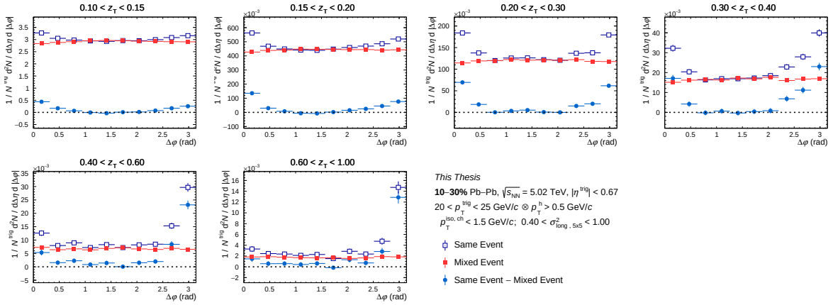
Figure C.27: Azimuthal correlation distribution in 10-30% for isolated wide clusters for the same event (empty blue square), for mixed event (full red square) and for result of the subtraction (full light blue circle) as a function of \Delta\phi for different z_T bins with 20 < p_T^{\text{trig}} < 25 GeV/ c .
