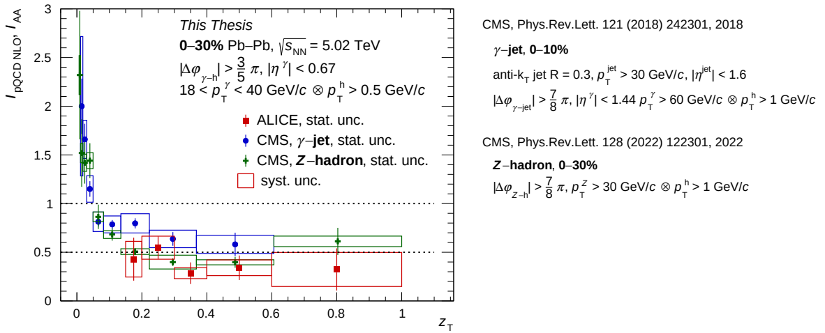
Figure 6.40: Top: The I_{\text{AA}} distributions as a function of z_{\text{T}} in central collisions for \gamma -jet (full blue circle) and Z-hadron (full green cross) correlation from the CMS Collaboration [102, 106] and the I_{\text{pQCD NLO}} from the \gamma^{\text{iso}} -hadron (full red square) correlation by ALICE.
