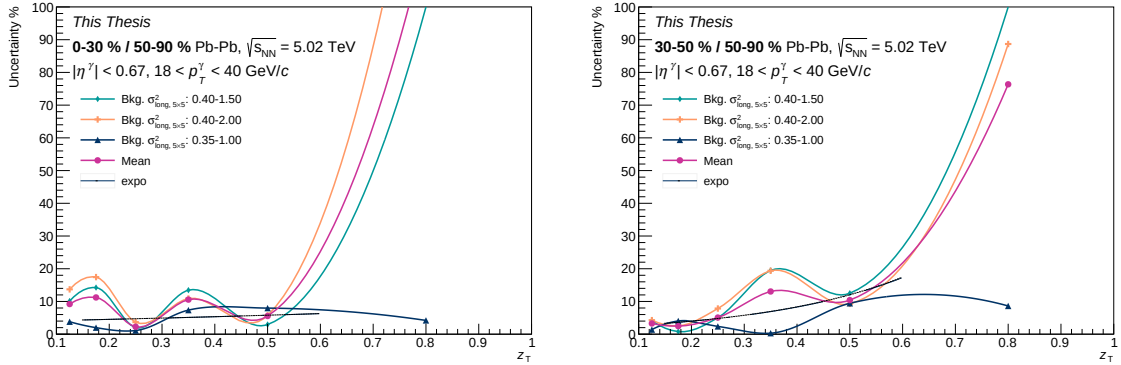
Figure D.4: Systematic uncertainties due to \sigma_{\text{long}, 5 \times 5}^2 background ranges: 0.40 < \sigma_{\text{long}, 5 \times 5}^2 < 1.50 (full green diamond); 0.40 < \sigma_{\text{long}, 5 \times 5}^2 < 2.00 (full orange cross) and 0.35 < \sigma_{\text{long}, 5 \times 5}^2 < 1.00 (full black triangle) in 0-30% (top left) and in 30-50% (top right) Pb-Pb collisions. The average of the systematic uncertainties in the three ranges is pink, while the exponential fit is shown with a dashed light blue line.
