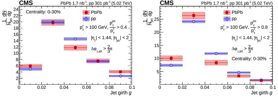
Figure 2.17: Distributions of jet girth g of \gamma^{\text{iso}} -tagged jets in Pb–Pb (full red square) and pp (empty blue circle) collisions for x_{j\gamma} = p_T^{\text{jet}}/p_T^\gamma > 0.4 (left) and for x_{j\gamma} > 0.8 (right) measured by CMS [108].
