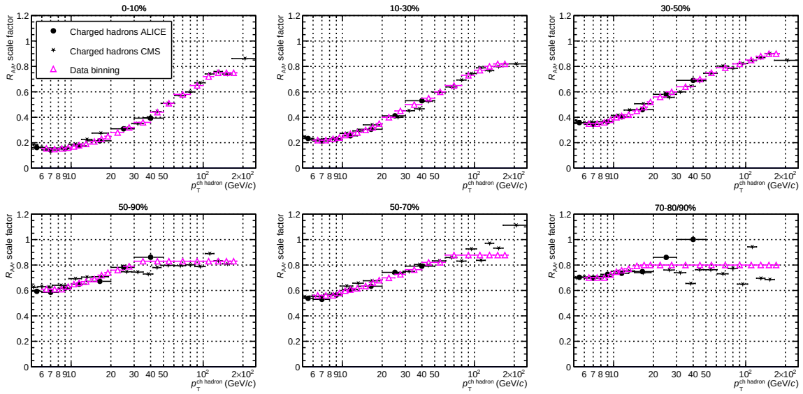
Figure 6.4: The R_{AA} distributions for charge hadrons by ALICE (full black circle), by CMS (full black star) and R_{AA} weights (empty pink triangle) as a function of p_T^{\text{ch, hadron}} from central to peripheral Pb–Pb collisions (clock-wise) by ALICE [65] and CMS [152] at \sqrt{s_{NN}} = 5.02 TeV.
