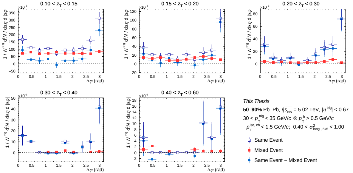
Figure C.39: Azimuthal correlation distribution in 50-90% for isolated wide clusters for the same event (empty blue square), for mixed event (full red square) and for result of the subtraction (full light blue circle) as a function of \Delta\phi for different z_T bins with 30 < p_T^{\text{trig}} < 35 \text{ GeV}/c .
