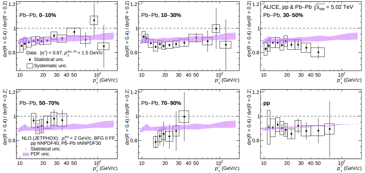
Figure 2.10: Ratio of isolated-photon spectra measured with R = 0.4 over R = 0.2 , for Pb-Pb and pp collisions at \sqrt{s_{\text{NN}}} = 5.02 TeV. Each panel corresponds to a Pb-Pb collisions centrality class or to pp collisions. The pink band corresponds to pQCD calculations with JETPHOX [93].
