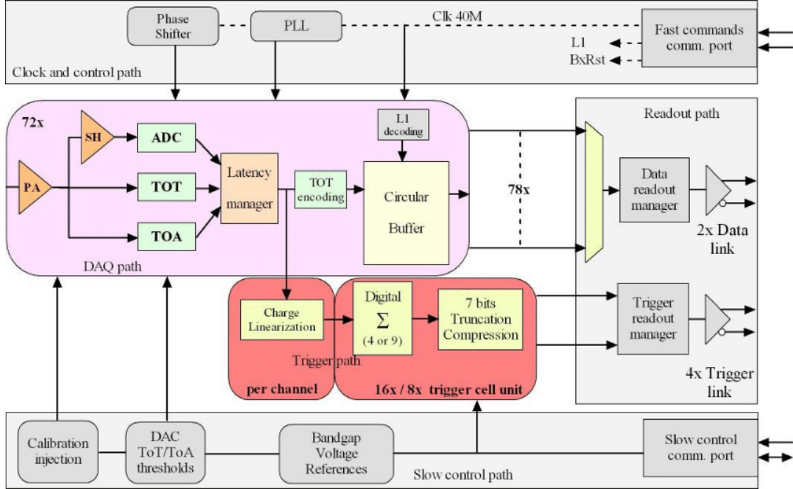
Figure 7.4: Architectural overview of the HGCROC-V2 [172].
