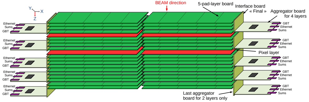
Figure 7.6: Overview of layer stacking in the beam direction. The silicon pad sensor layers and their associated front-end electronics are shown in green, and the MAPS layers (without their readout) are shown in red. The readout partition is shown for a full module: four 5-pad-layer boards per aggregator for the first four groups and two 5-pad-layer boards for the last silicon pad layers. The mechanical adaptation between the 5-pad-layer boards and the aggregator is achieved with a dedicated “final” interface board.
