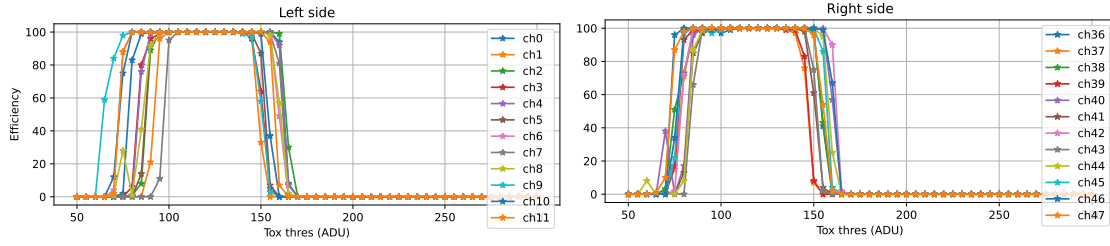
Figure 7.15: Efficiency curves as a function of global thresholds for different channels and for the two sides of the HGCROC, before the calibration procedure.
