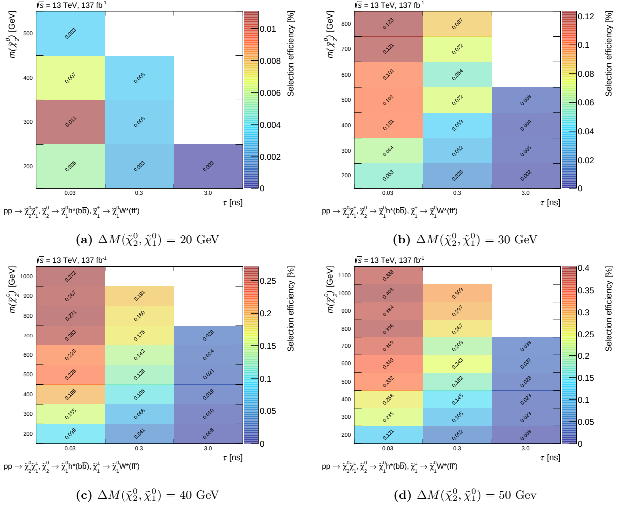
Figure 7.20: Selection efficiency for bino-wino signal models as a function of \tilde{\chi}_2^0 mass and lifetime with (a) \Delta M(\tilde{\chi}_2^0, \tilde{\chi}_1^0) = 20 GeV, (b) \Delta M(\tilde{\chi}_2^0, \tilde{\chi}_1^0) = 30 GeV, (c) \Delta M(\tilde{\chi}_2^0, \tilde{\chi}_1^0) = 40 GeV, and (d) \Delta M(\tilde{\chi}_2^0, \tilde{\chi}_1^0) = 50 GeV. Bins with no MC samples are shown as blank.
