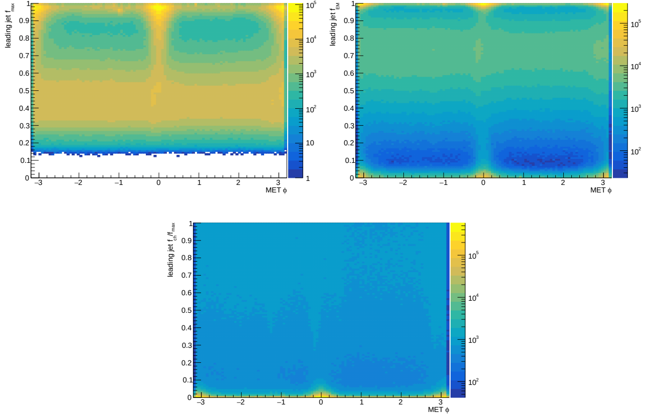
Figure 7.5: Correlation between the E_{\text{T}}^{\text{miss}} \phi and the leading jet f_{\max} (top left), f_{\text{EM}} (top right), and f_{\text{ch}}/f_{\max} (bottom). The events are required to pass the trigger, E_{\text{T}}^{\text{miss}} filter, event cleaning, PV conditions, and offline E_{\text{T}}^{\text{miss}} selection.
