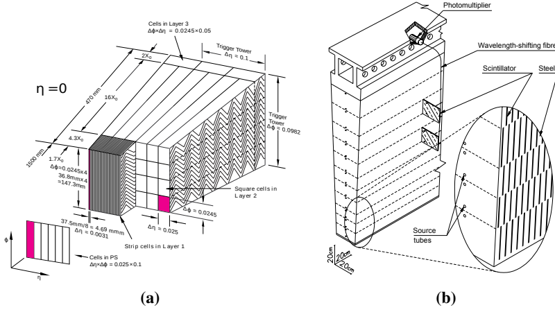
Figure 2.9: Sketch of (a) an ECAL barrel module, where the different longitudinal layers are depicted with the characteristic accordion shape and (b) a Tile calorimeter module, also showing the layers of steel absorber and active scintillator material, as well as the optical read-out.
