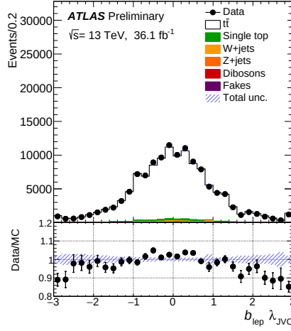
Figure 4.13: Comparison between data and MC for the \lambda_{\text{JVC}} distribution of the b_{\text{lep}} -jet after the reweighting is applied. The uncertainty band consists of both the statistical and systematic uncertainties, with the systematic component computed with the method described in Section 4.2.4.
