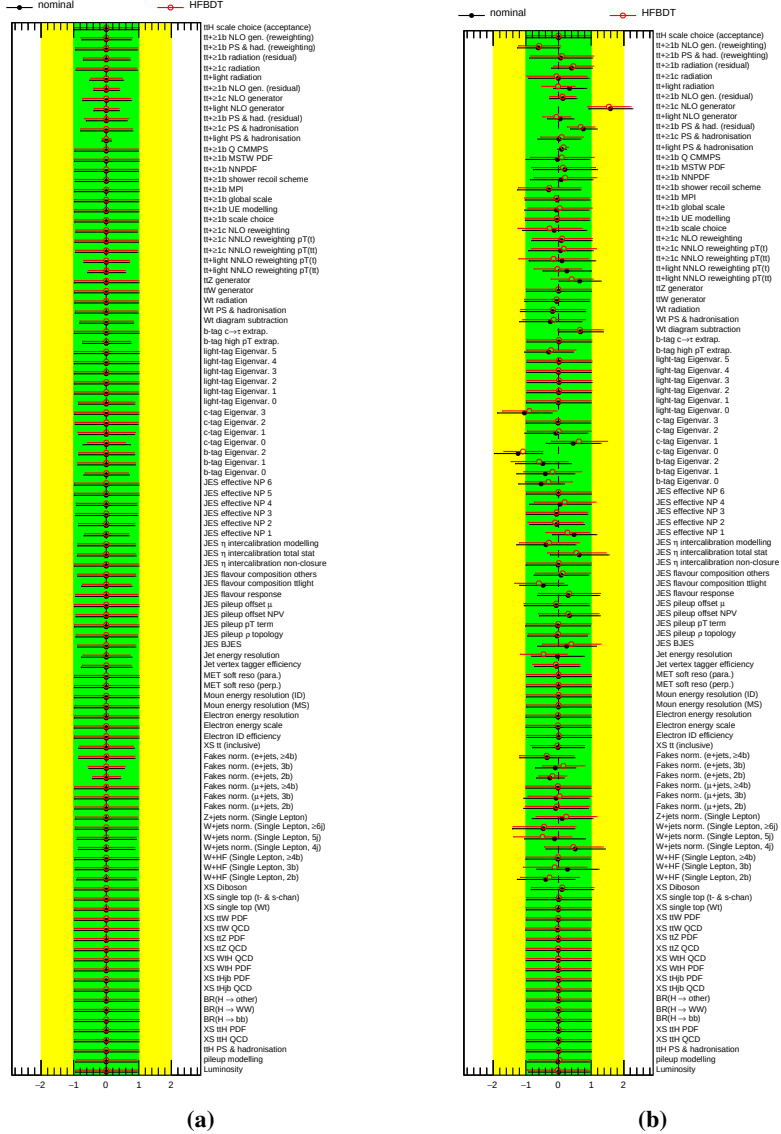
Figure 5.14: Comparisons of the fitted nuisance parameters obtained with the nominal fit (black full circles) and a fit with the HFBDT in the (5j, 3b) CR (red open circles). The fit on the Asimov dataset under the signal-plus-background hypothesis is shown on the left and the fit on real data under the background-only hypothesis is on the right. In all the CR the H_T variable is used and the classBDT discriminants are employed in the SR only for the Asimov fit.
