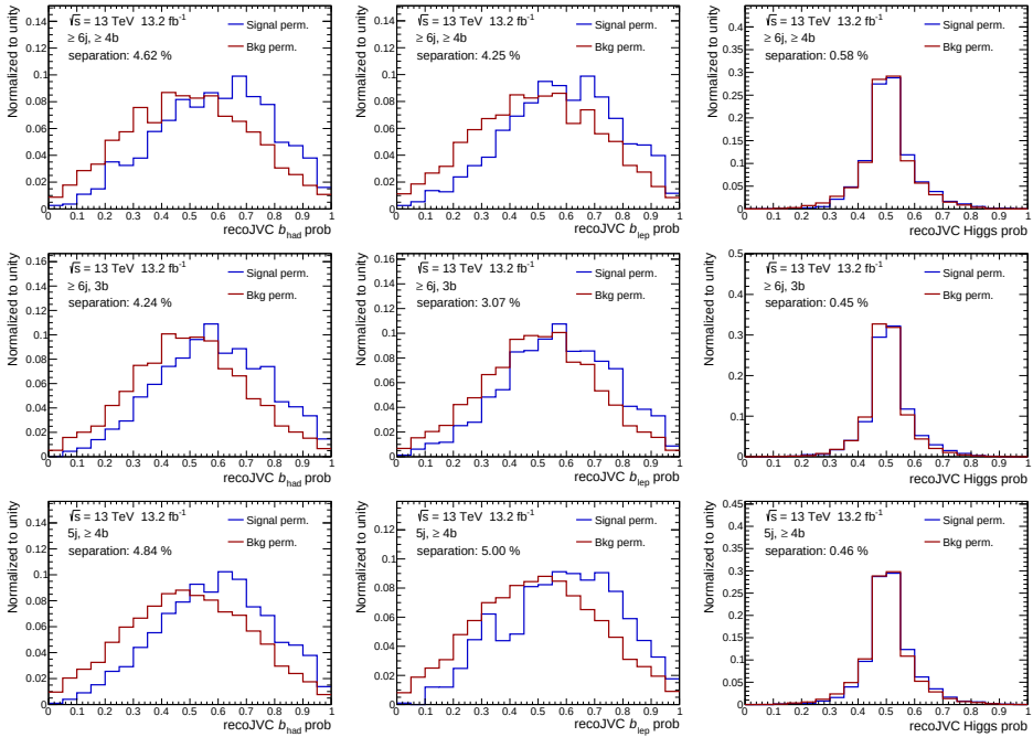
Figure B.1: Distribution for the b_{had} (left), b_{lep} (centre) and Higgs (right) probability as defined by Equations 5.1 and 5.2 for the signal and background permutation for the three signal regions of the ICHEP analysis. The values of the separation for each variable in each region is reported.
