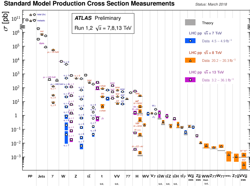
Figure 1.11: Summary of several Standard Model total and fiducial production cross section measurements, corrected for leptonic branching fractions, compared to the corresponding theoretical expectations. All theoretical expectations were calculated at NLO or higher. Not all measurements are statistically significant yet. Taken from Ref. [45].
