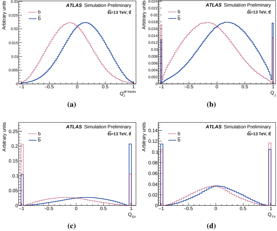
Figure 4.1: Distributions of the basic charge variables for positive (blue) and negative (red) truth b -jets: (a) jet charge computed from all available tracks ( Q_J^{\text{all tracks}} ), (b) jet charge ( Q_J ), (c) secondary vertex charge ( Q_{SV} ) and (d) tertiary vertex charge ( Q_{TV} ).
