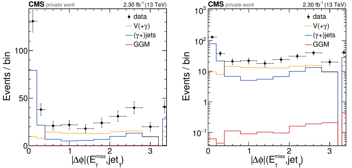
Figure 4.4: The pre-fit distributions of both templates shown with data and the GGM signal point using linear (left) and logarithmic (right) scales. A possible presence of signal is not expected to influence the fit result.
