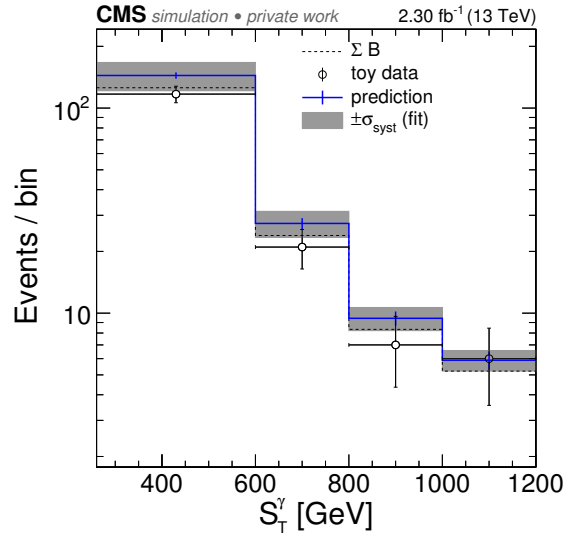
Figure 4.5: Closure test of the extrapolation of the fitted scale factors to the signal region for f_{V(+\gamma)} = 0.5 , f_{(\gamma+)}\text{jets} = 1.5 . The dashed line is the sum of all background processes scaled with the f_i , the open circles are the toy data generated from this true distribution. The prediction obtained from the fitted SF_i is shown in blue and the systematic error is originating from the fit errors.
