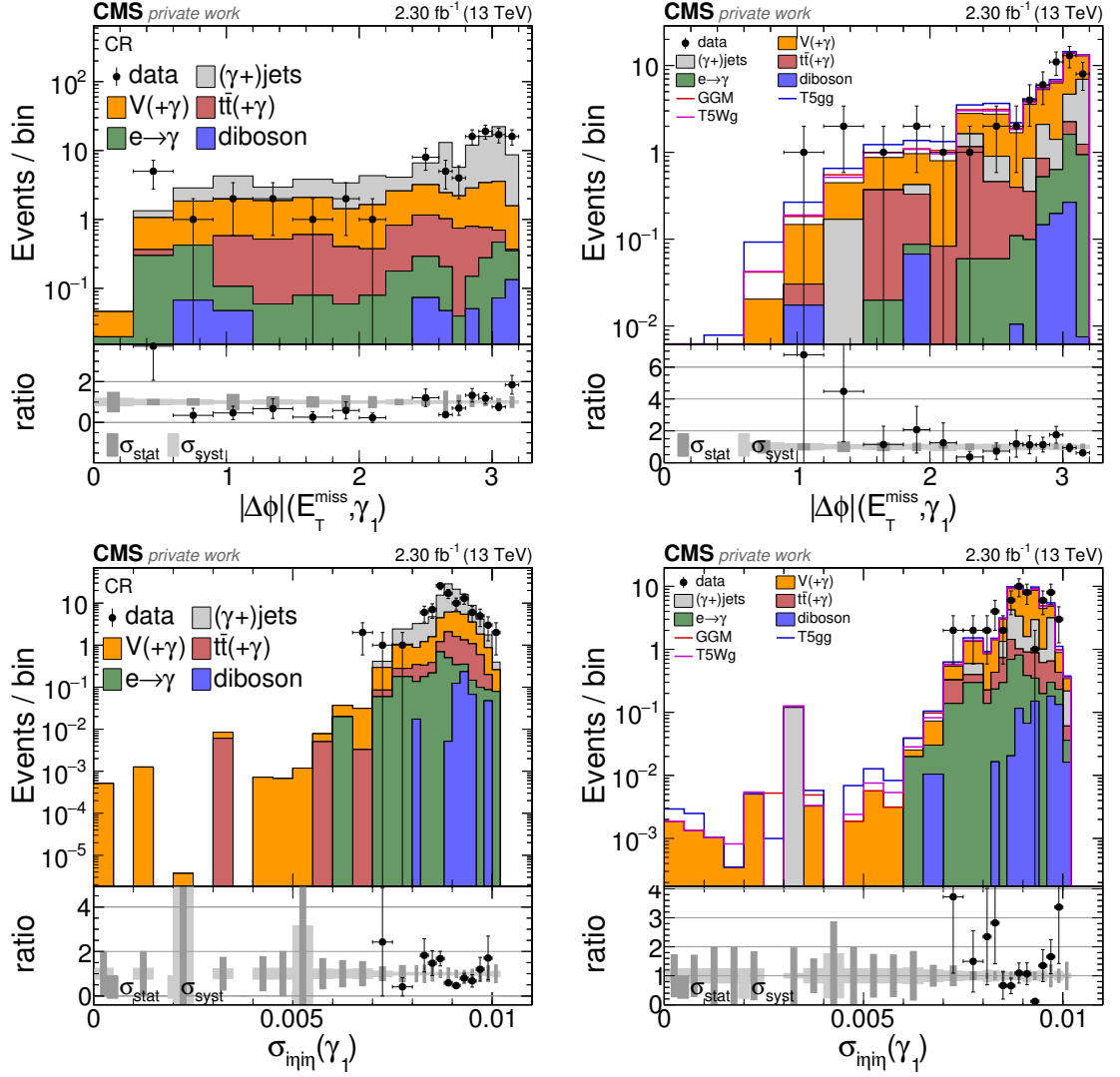
Figure 4.17: Non-collision background check using the |\Delta\phi|(E_T^{\text{miss}}, \gamma) and \sigma_{\text{in}\eta}(\gamma) distributions for |\eta|(\gamma) > 1.0 in the CR (left) and SR (right).
