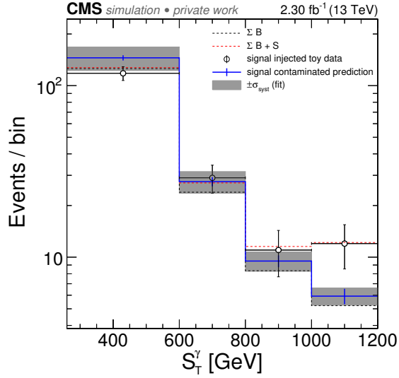
Figure 4.8: Closure test of the extrapolation of the fitted scale factors to the signal region for f_{V(+\gamma)} = 0.5 , f_{(\gamma+)\text{jets}} = 1.5 in the presence of signal in both the SR and CR. The black dashed line is the sum of all background processes scaled with the f_i and the red dashed line also includes the signal. The open circles are the toy data generated from the true distribution containing the signal. The prediction obtained from the SF_i is shown in blue and the systematic error is originating from the fit errors.
