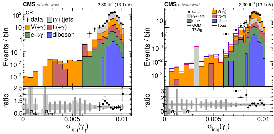
Figure 4.18: Check for ECAL-spike events using the \sigma_{inj\bar{inj}} distribution without the |\eta|(\gamma) > 1.0 requirement in the CR (left) and SR (right).
