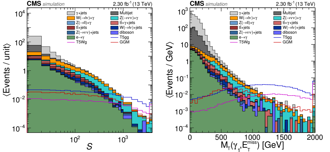
Figure 3.9: The S and M_T distributions after the preselection. All used samples are taken from MC simulation, except the e \rightarrow \gamma component, which is determined using the method described in Section 4.2. The overflow is contained in the last bin shown and the bin contents are divided by the bin widths [1].
