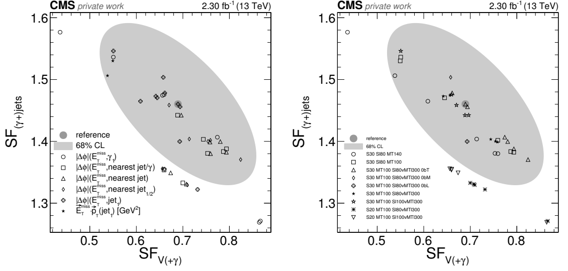
Figure 4.3: The same fit results as shown in Fig. 4.2 (bottom) in two dimensions. The nominal value is shown with its 1\sigma uncertainty ellipse. The same points are shown on both sides. Left: The same marker indicates one template variable. Right: The same marker indicates one selection used for the fits.
