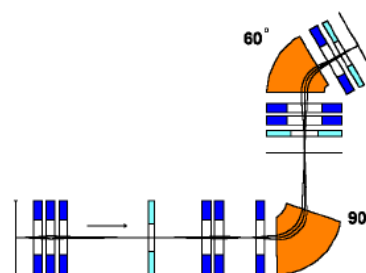
Fig. 5.3 b) High Resolvent Separator , HRS [69].
