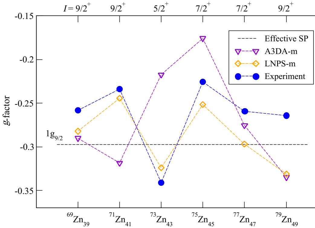
Figure 6.9: Comparison of measured high-spin state g -factors for isotopes from N = 39 - 49 and the predictions from the LNPS-m and A3DA-m shell-model interactions.
