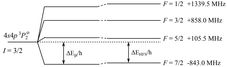
Figure 2.4: Final splitting of the 3d^{10}4s4p\ ^3P_2^\circ level in the I = 3/2 ground state of ^{63}\text{Zn} after the perturbations due to the electric quadrupole component of the hyperfine interaction are considered in addition to contributions from the magnetic dipole component.
