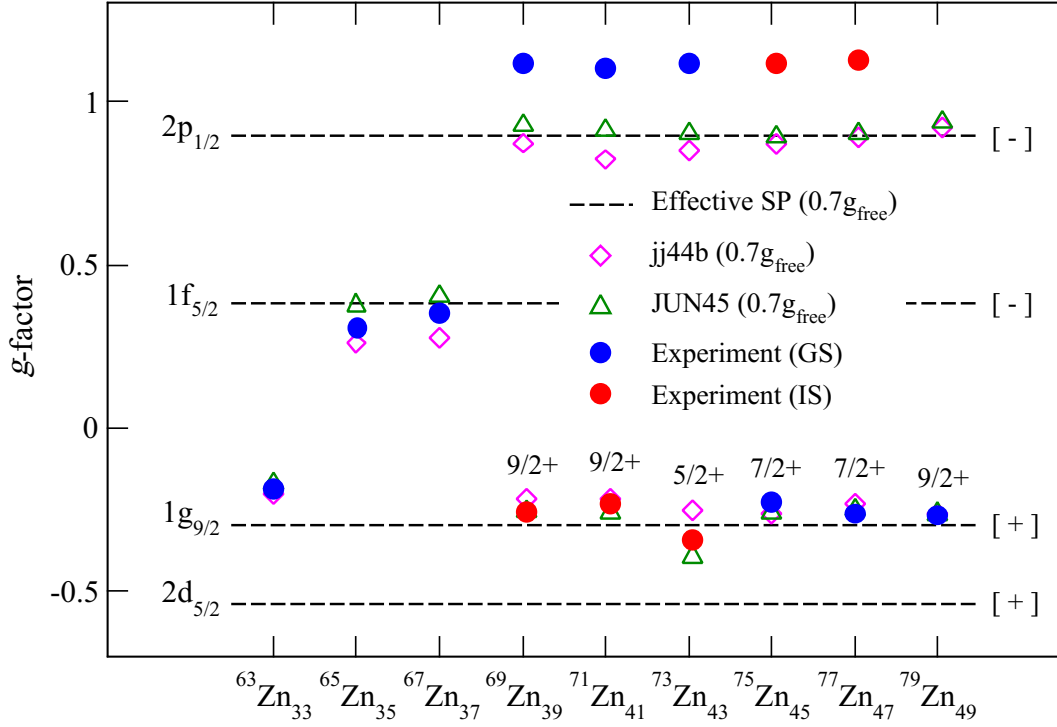
Figure 6.2: Experimental g -factors across the isotope chain in comparison to single-particle estimates and predictions from the JUN45 and jj44b interactions. The measured g -factor of ^{79m}\text{Zn} is not shown here due to scaling, as g_{\text{expt}} = -2.036 . Errors on measured g -factors are smaller than the size of the symbols.
