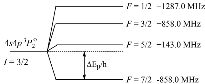
Figure 2.2: Scale representation of the observed hyperfine level splitting of the 3d^{10}4s4p\ ^3P_2^\circ level in the I = 3/2 ground state of ^{63}\text{Zn} due to the magnetic dipole component of the hyperfine interaction.
