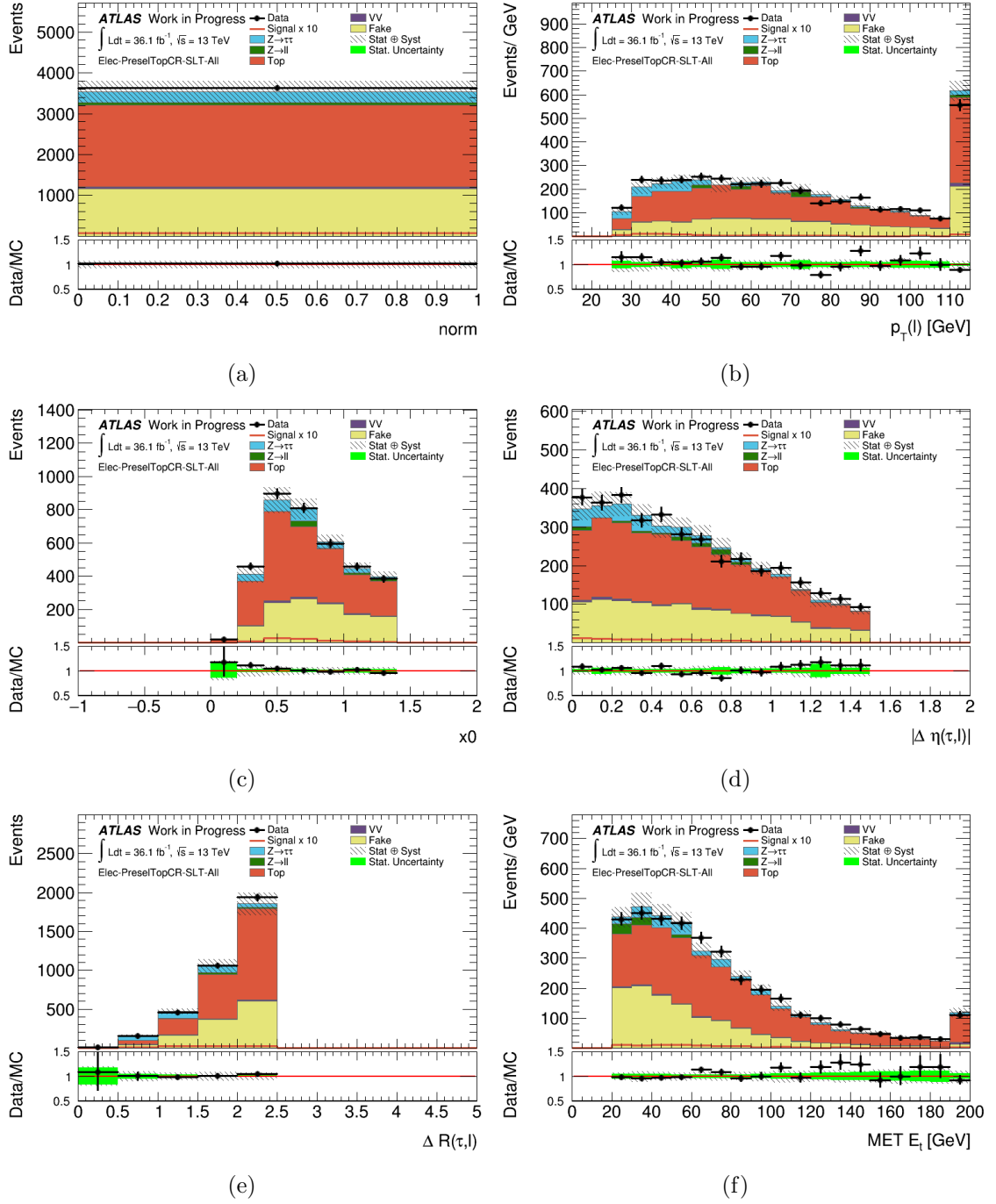
Figure 6.7.: Distributions in Top CR at Preselection level for \tau_e\tau_{had} channel : a) norm , b) elec. p_T , c) coll. approx. x_0 , d) \Delta\eta(lep, \tau) , e) \Delta R(lep, \tau) , f) E_T^{miss} .
