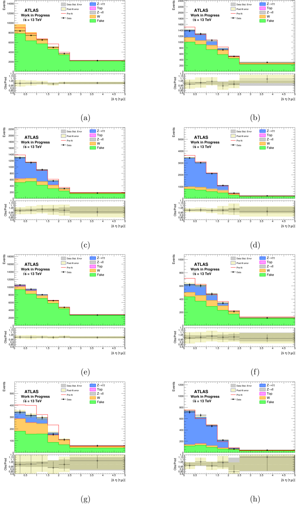
Figure 4.13.: \Delta\eta(\mu, \tau) postfit distribution for 20 GeV < p_T < 25 GeV, 1 prong : a) not loose, b) loose not medium, c) medium not tight, d) tight cat. ; 3 prong : e) not loose, f) loose not medium, g) medium not tight, h) tight categories .
