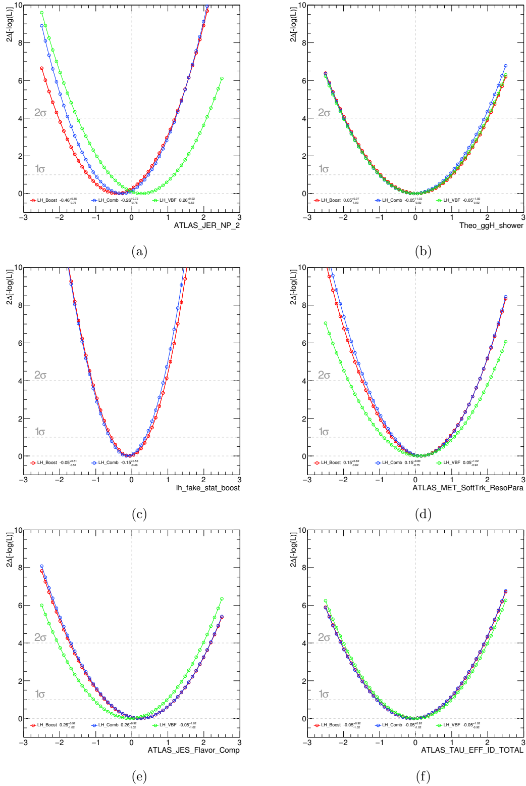
Figure 6.34.: NLL profiles scans for the highly ranked NPs in Fig. 6.31 (a).
