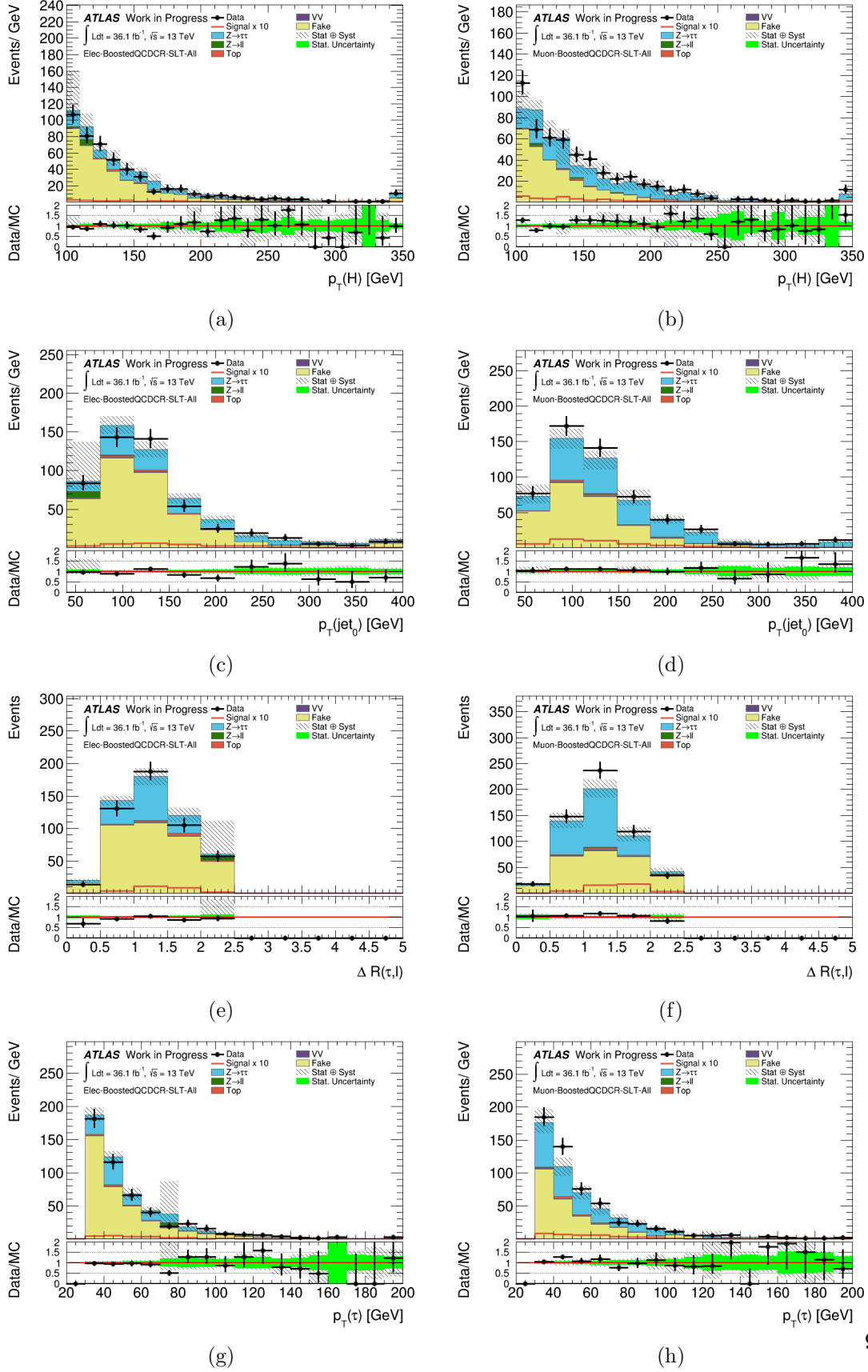
Figure 6.22.: Distributions in QCD CR in Boosted region for \tau_e \tau_{had} ( \tau_\mu \tau_{had} ) channel : a) (b) p_T^H , c) (d) lead jet p_T , e) (f) \Delta R(\ell ep, \tau) , g) (h) \tau p_T . The large uncertainty observed in some bins in the \tau_e \tau_{had} channel are due to large weights coming from Sherpa MC generator for the Z \rightarrow ll process.
