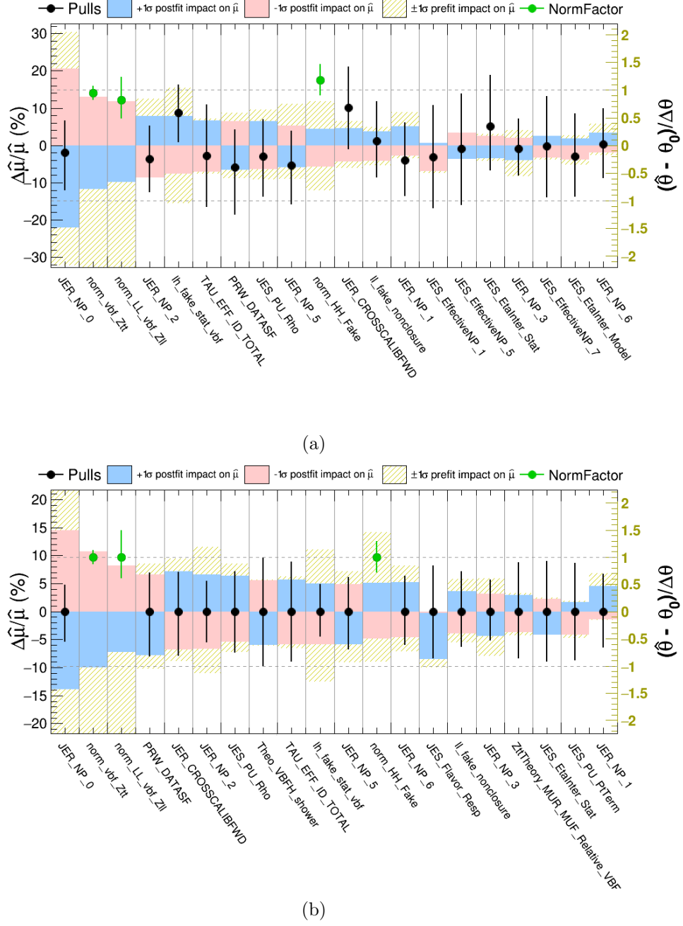
Figure 6.38.: Comparison of nuisance parameter ranking for Combined VBF category fit: a) Unblinded Fit, b) Asimov Fit.
