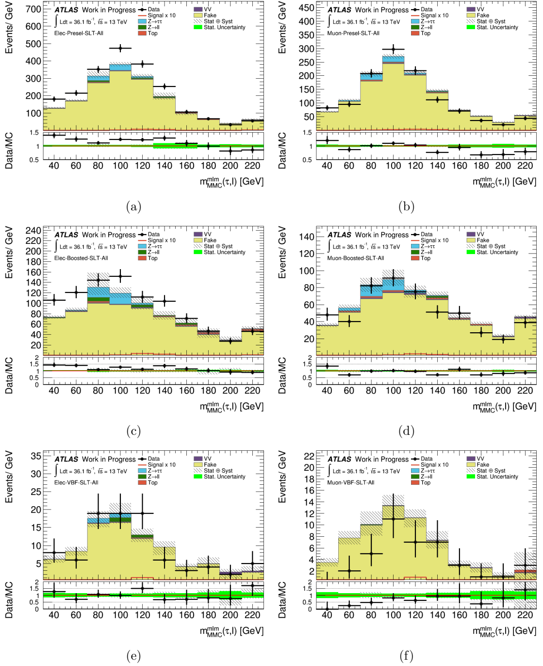
Figure 6.15.: MMC distributions in the same sign closure region: a) b) \tau_e\tau_{had} ( \tau_\mu\tau_{had} ) Preselection, c) d) \tau_e\tau_{had} ( \tau_\mu\tau_{had} ) Boosted region, e) \tau_e\tau_{had} ( f) ( \tau_\mu\tau_{had} ) VBF region. Figures do not show Fake-Factor systematic uncertainties discussed in Section 6.4.1. For the signal, m_H = 125 GeV is chosen.
