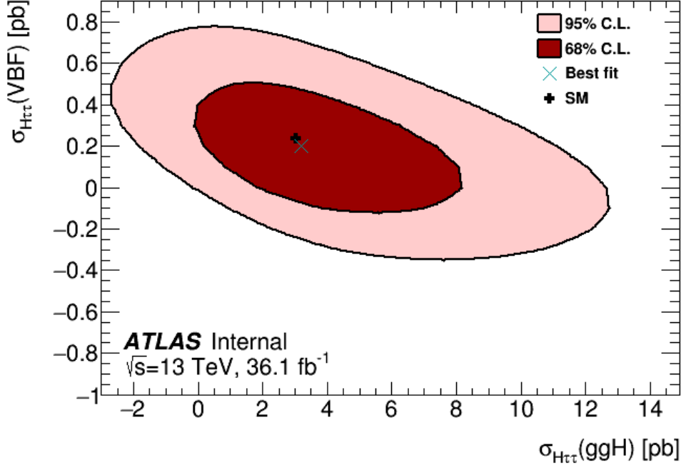
Figure 6.35.: Two dimensional 68 % and 95 % confidence level contours in the plane ( \sigma_{H\tau\tau}(\text{ggH}) , \sigma_{H\tau\tau}(\text{VBF}) ). Results from standalone \tau_{\text{lep}}\tau_{\text{had}} fit.
