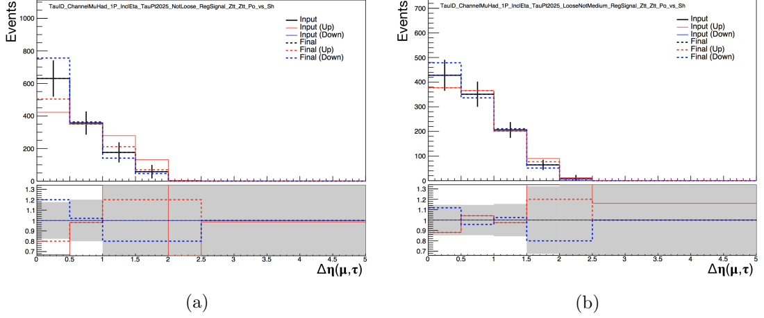
Figure 4.8.: Envelope plots for \Delta\eta(\mu, \tau) Z \rightarrow \tau\tau MC generator uncertainty for 20 \text{ GeV} < p_T < 25 \text{ GeV} , 1 prong : a) not loose, b) loose not medium ID categories.
