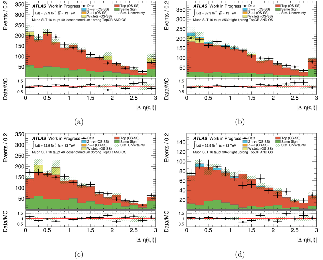
Figure 4.3.: Examples of modelling in Top CR for: a) p_T > 40 GeV, 1 prong, loose not medium ID category, b) 25 < p_T < 30 GeV, 1 prong, tight ID category, c) p_T > 40 GeV, 3 prong, loose not medium ID category, d) 30 < p_T < 40 GeV, 3 prong, tight ID category.
