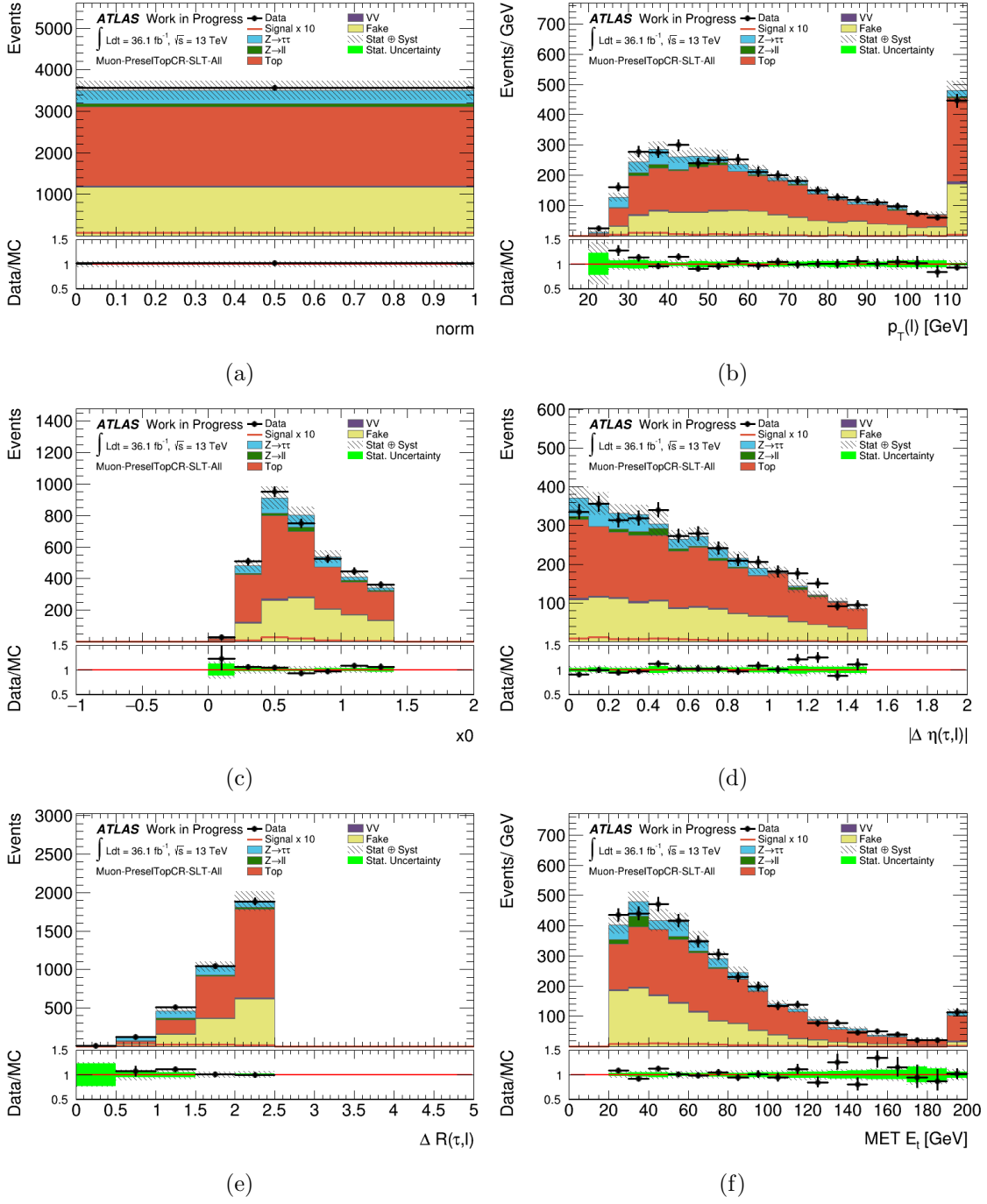
Figure 6.8.: Distributions in Top CR at Preselection level for \tau_\mu \tau_{had} channel : a) norm, b) muon p_T , c) coll. approx. x_0 , d) \Delta\eta(lep, \tau) , e) \Delta R(lep, \tau) , f) E_T^{miss} .
