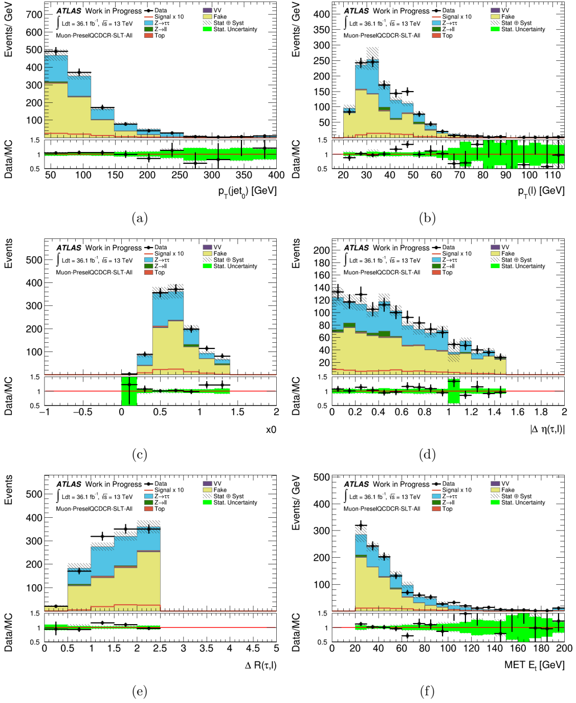
Figure 6.6.: Distributions in QCD CR at Preselection level for \tau_\mu \tau_{had} channel : a) lead jet p_T , b) muon p_T , c) coll. approx. x_0 , d) \Delta\eta(lep, \tau) , e) \Delta R(lep, \tau) , f) E_T^{miss} .
