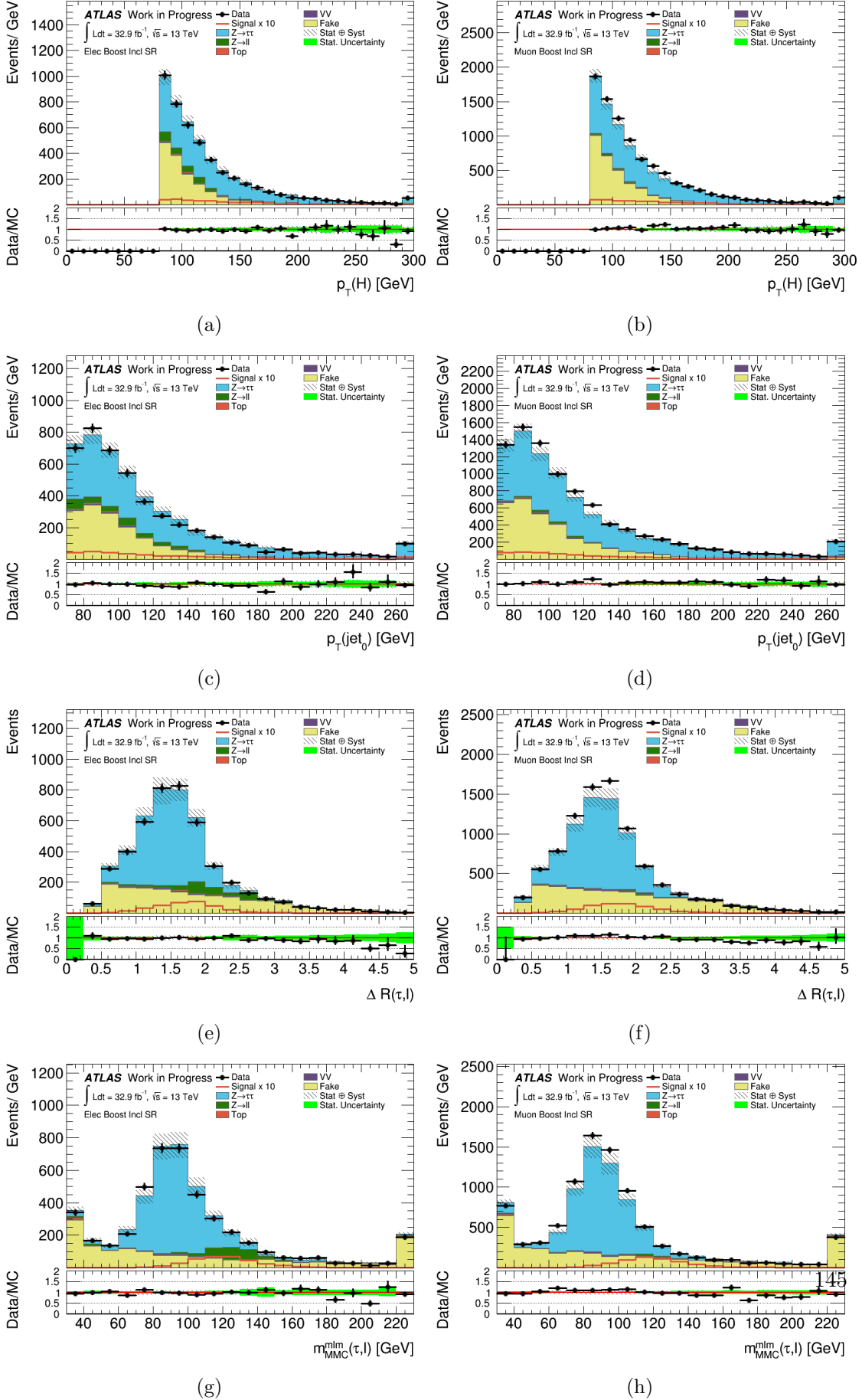
Figure 7.7.: Distributions in Boosted signal region for \tau_e\tau_{had} ( \tau_\mu\tau_{had} ) channel : a) (b) Higgs p_T , c) (d) lead jet p_T , e) (f) \Delta R(l\tau, \tau) , g) (h) MMC.
