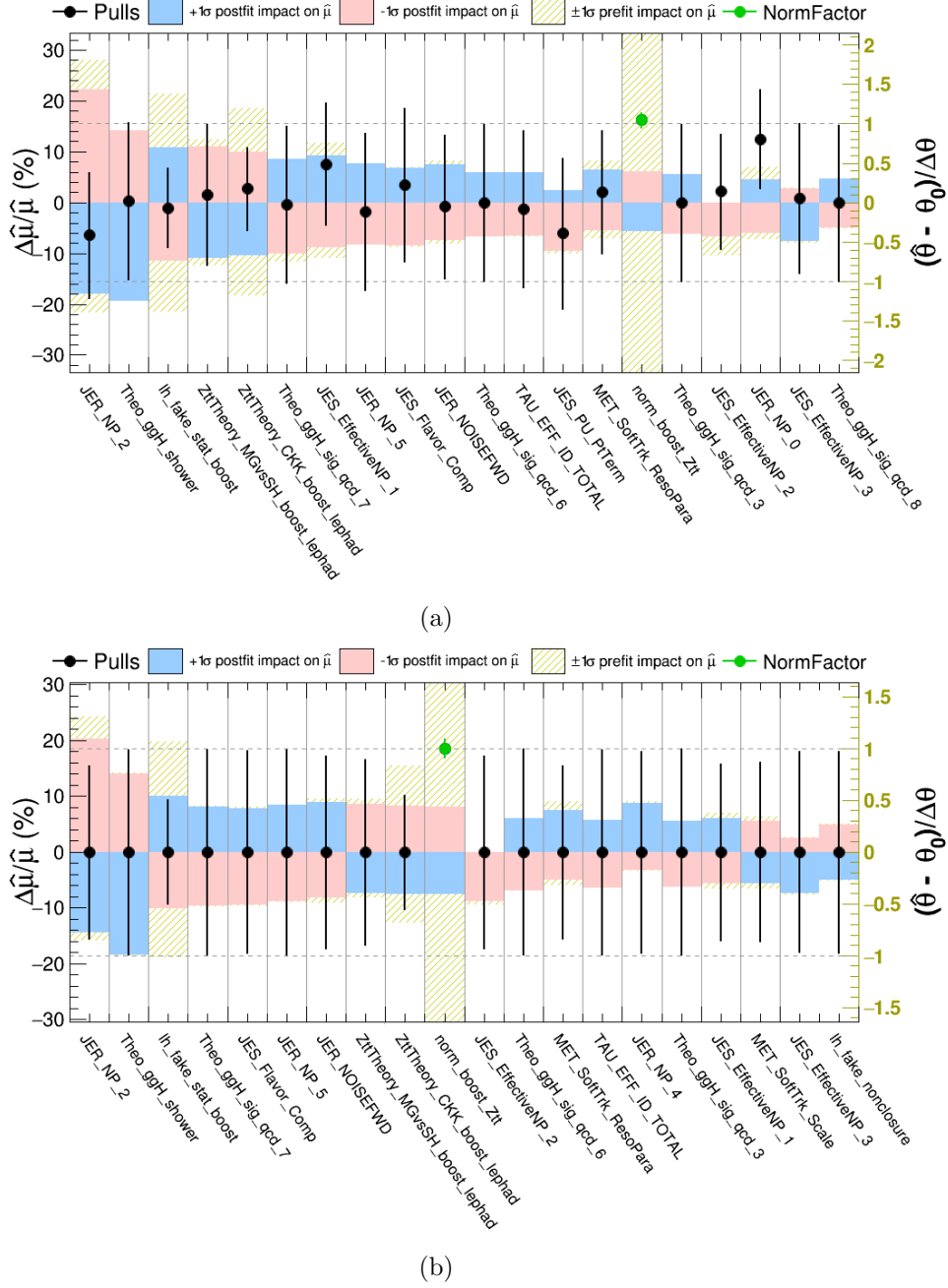
Figure 6.32.: Comparison of nuisance parameter ranking for Standalone \tau_{lep}\tau_{had} Boost category fit: a) Unblinded Fit, b) Asimov Fit.
