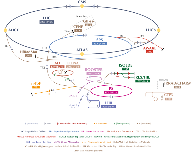
Figure 2.1: The CERN accelerator complex [77].
