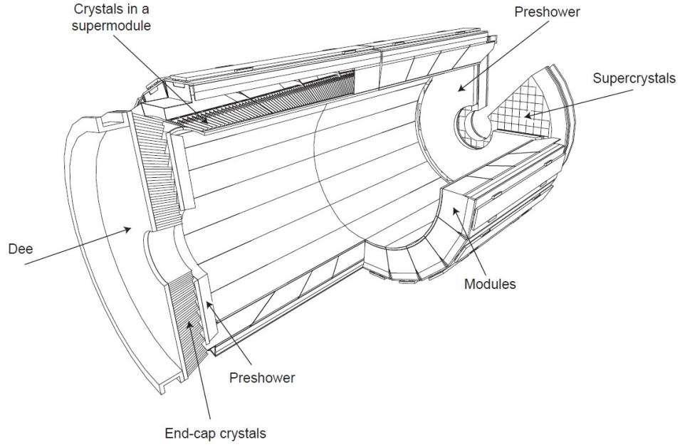
Figure 2.4: Layout of the CMS ECAL [19].
