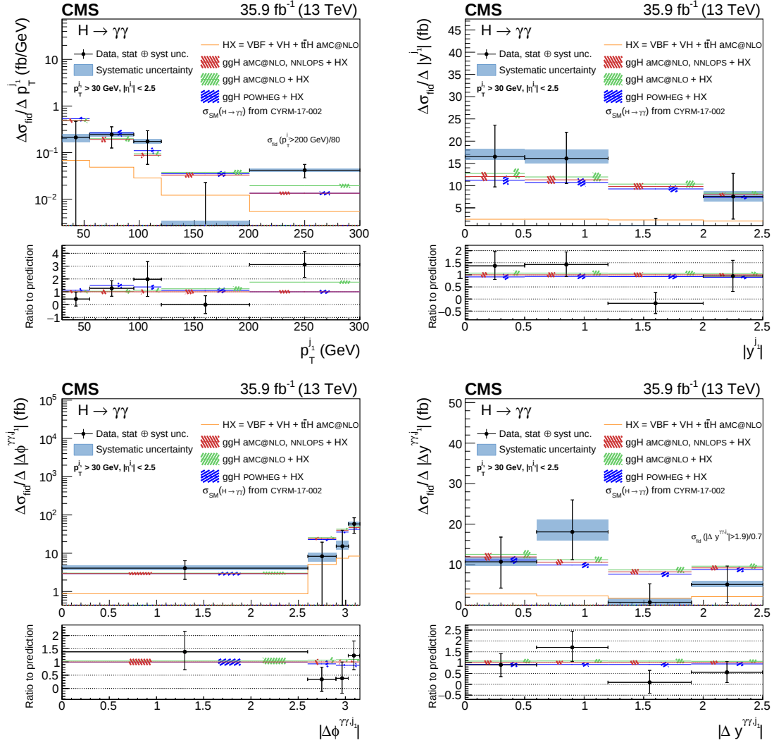
Figure 6.9: The measurement of the differential cross section for p_T^{j1} , |y^{j1}| , |\Delta\phi^{\gamma\gamma j1}| , and |\Delta y^{\gamma\gamma j1}| . The black points indicate the data, with the error bars showing 1 standard deviation total uncertainty. The blue band indicates the systematic component of the total uncertainty. The measurements are compared to the theoretical predictions, normalized to the predictions from Ref. [35] and obtained with different Monte Carlo programs. The normalization of the cross section in the last bin of the distribution, when this is an overflow bin, is indicated in the figure.
