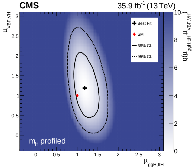
Figure 5.23: The best fit value (black cross) of the two-dimensional likelihood scan for \mu_{\text{ggH, ttH}} versus \mu_{\text{VBF, VH}} is compared to the SM expectation (red diamond). The solid (dashed) contour shows the 68% (95%) confidence region.
