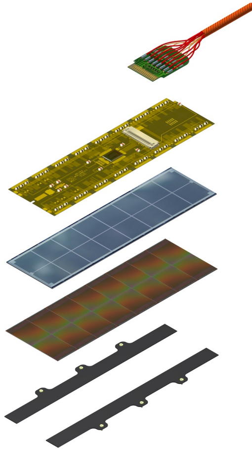
Figure 8.6: Drawing showing separately the components of the modules installed in L2-4 and in the Fpix, from top to bottom: the module cable, the HDI with the TBM, the silicon sensor, the ROCs array, and the mounting strips. The FPix modules use a modified mounting system, while L1 modules employ two TBMs and the mounting strips are omitted to reduce the material budget.
