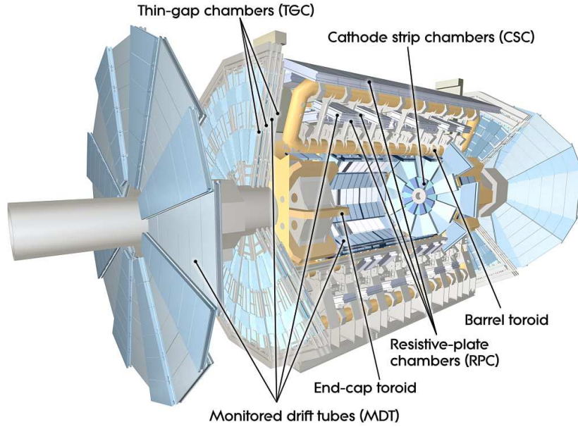
Figure 3.5: Cut-away view of the ATLAS muon spectrometer.
