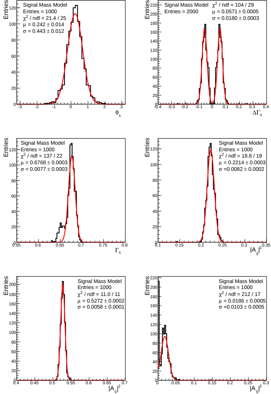
Figure 7.9: Distributions of fit values from fits to 1000 pseudo-experiments generated with an alternative signal mass model including a Gaussian fit (red).
