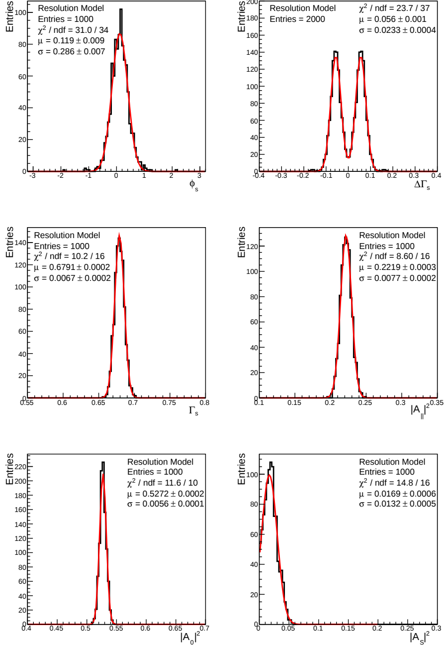
Figure B.9: Distributions of fit values from fits to 1000 pseudo-experiments generated with an alternative signal decay time model. The red curve is a Gaussian fit to the distribution.
