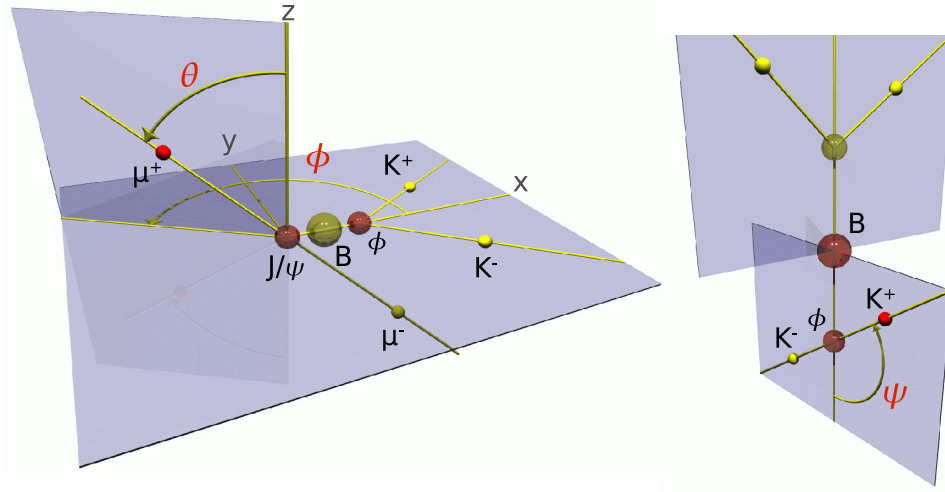
Figure 2.8: Transversity basis defined in terms of three angles between the final state particles. The angles \theta and \phi are defined in the J/\psi meson rest frame and the angle \psi is defined in the \phi rest frame.
