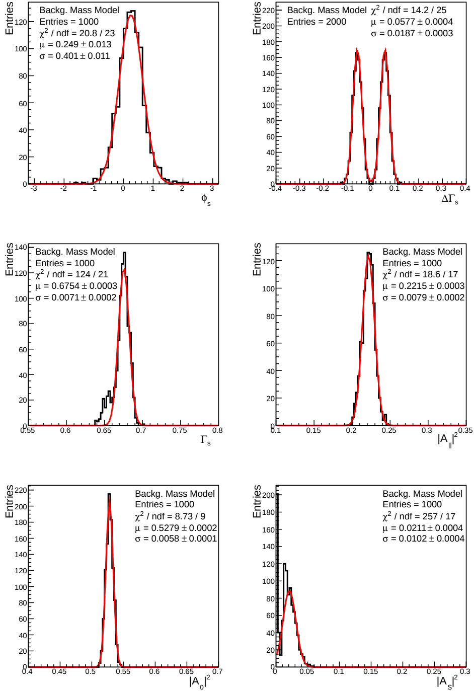
Figure 7.10: Distributions of fit values from fits to 1000 pseudo-experiments generated with an alternative background mass model, fitted with a Gaussian function (red).
