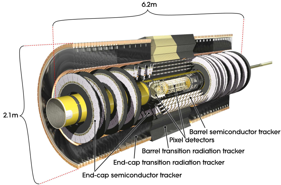
Figure 3.4: The inner detector tracking systems of ATLAS.
