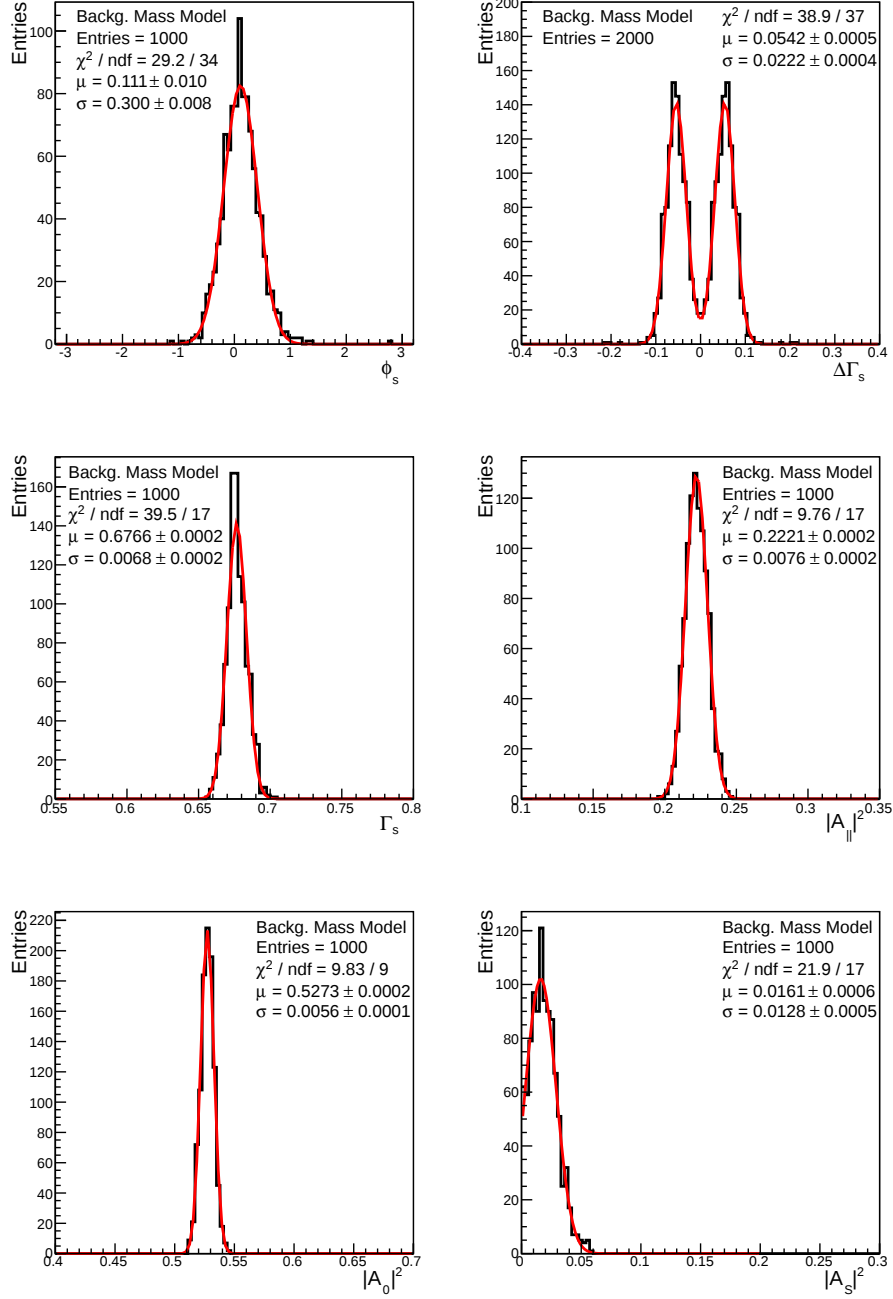
Figure B.7: Distributions of fit values from fits to 1000 pseudo-experiments generated with an alternative background mass model. The red curve is a Gaussian fit to the distribution.
