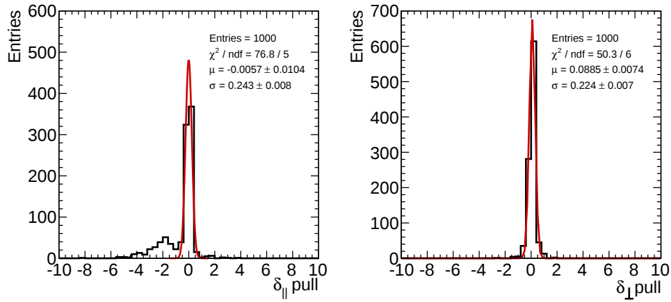
Figure 7.7: Pull distributions of 1000 pseudo-experiments generated with the untagged fit model for the strong phases \delta_\parallel (left) and \delta_\perp (right). Gaussian fits to the distributions are shown in red.
