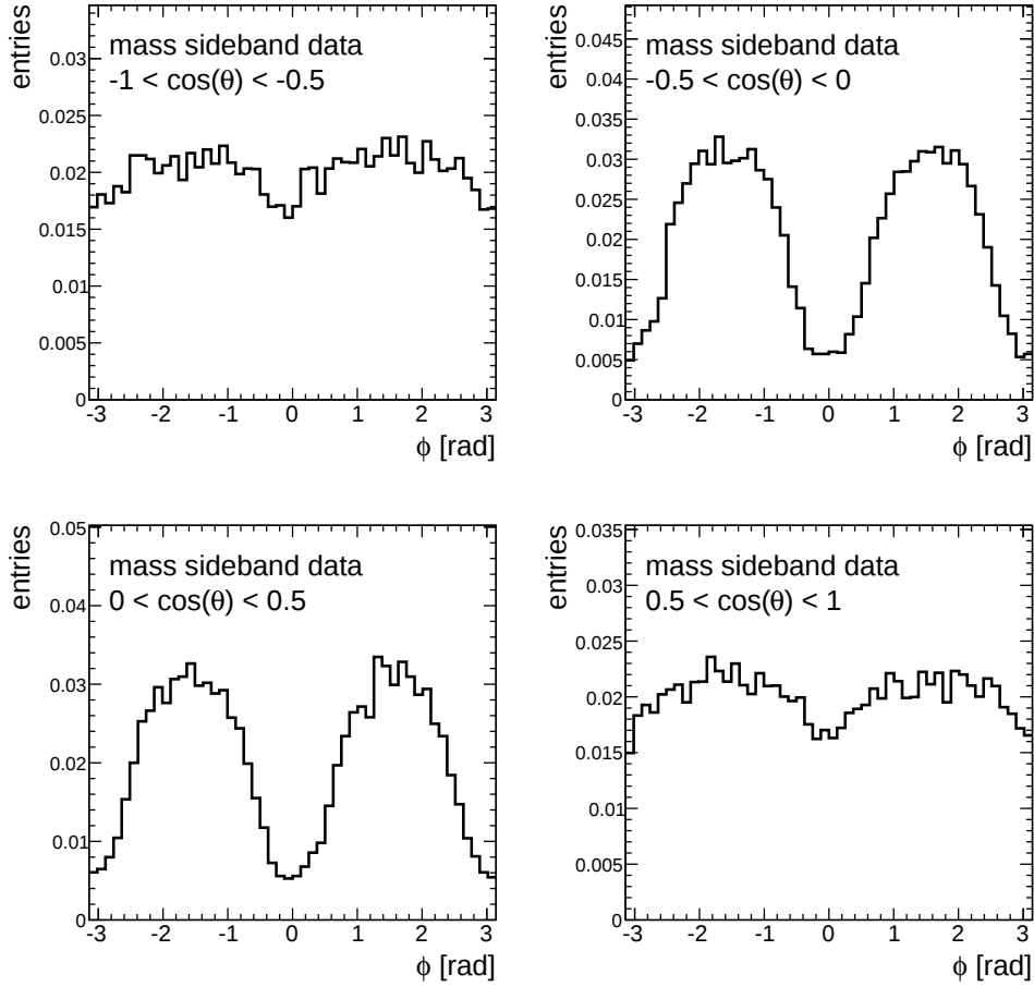
Figure 7.14: Normalized distribution of the transversity angle \phi from mass sideband data for different intervals of \cos \theta . To estimate the systematic effect of not treating the correlation between \cos \theta and \phi of the background angles, pseudo-experiments are produced using these four histograms for the generation of \phi for the background events. The mass regions 5.150 GeV – 5.317 GeV and 5.417 GeV – 5.650 GeV are used as sidebands.
