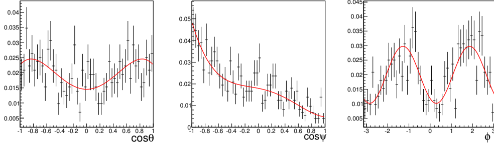
Figure 6.4: Normalized distributions of the transversity angles \cos \theta , \cos \psi and \phi of the B_s^0 candidates reconstructed in the B_d^0 \rightarrow J/\psi K^* MC sample. The red curves represent the fits to the distributions using the functions defined in equation 6.15. The parameters of the functions are kept fix in the full likelihood fit.
