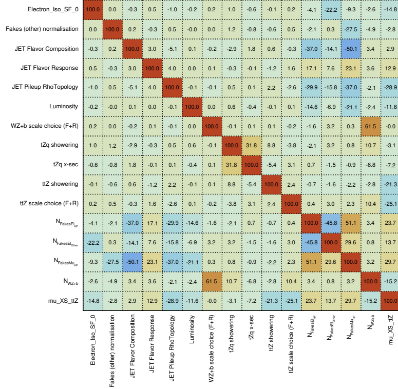
Figure 9.4: Correlation matrix for all NPs with an absolute correlation of \geq 20\% with other NPs or with the signal strength, \mu_{t\bar{t}Z} .
