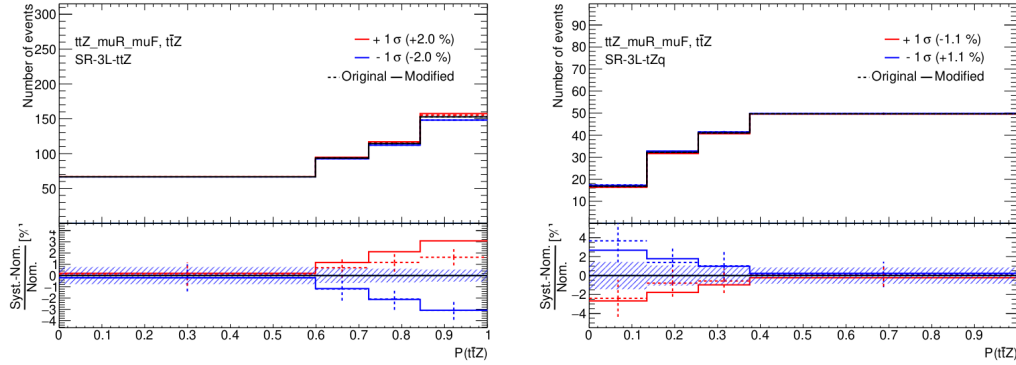
Figure 8.3: effect of the joint variation of the factorisation and renormalisation scale for the t\bar{t}Z process in the SR\text{-}3\ell\text{-}t\bar{t}Z region (left) and the SR\text{-}3\ell\text{-}tZq (right).
