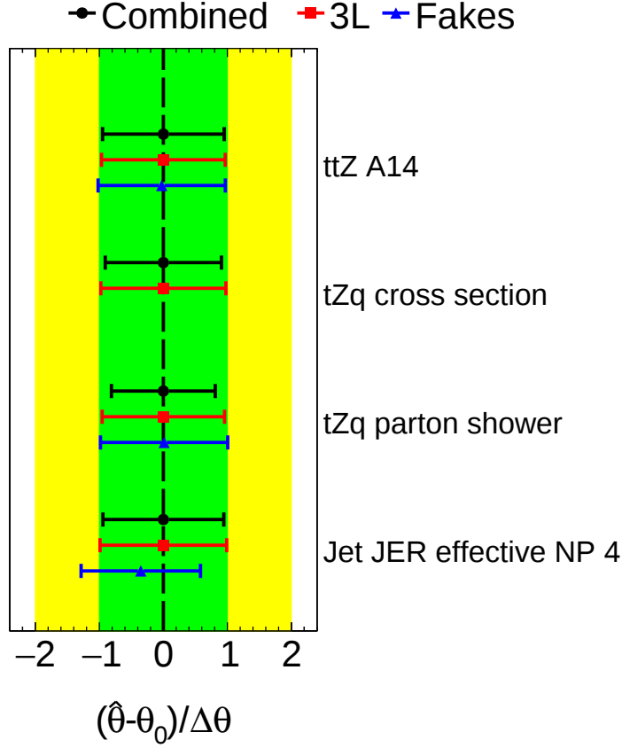
Figure 9.2: NPs that are pulled (constrained) in the Asimov fit by (\hat{\theta} - \theta_0)/\Delta\theta > 0.10 (0.025). The different markers denote the three fits. The coloured bands indicate the 1\sigma and 2\sigma uncertainty bands.
