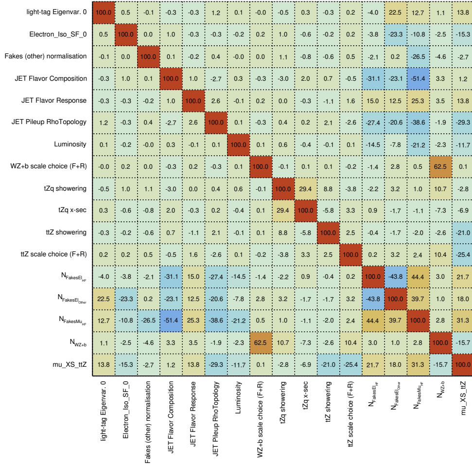
Figure 9.6: Correlation matrix for all NPs with an absolute correlation of \geq 20\% with other NPs or the signal strength, \mu_{t\bar{t}Z} , in the fit to ATLAS data.
