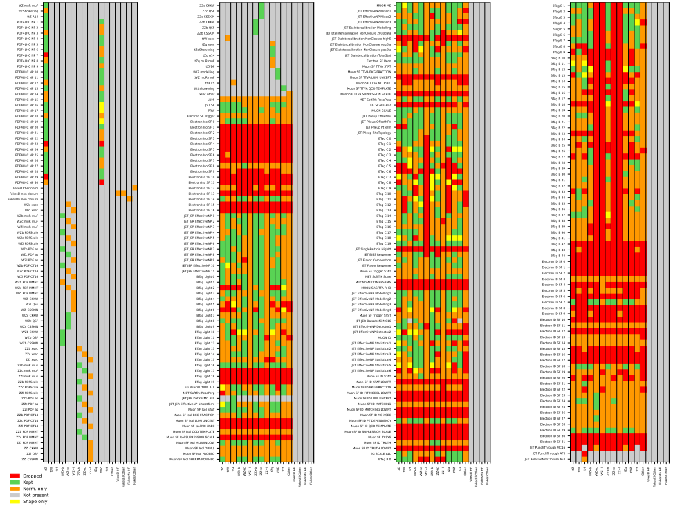
Figure B.1: Summary of pruned NPs in the SR-3l-ttZ region.
