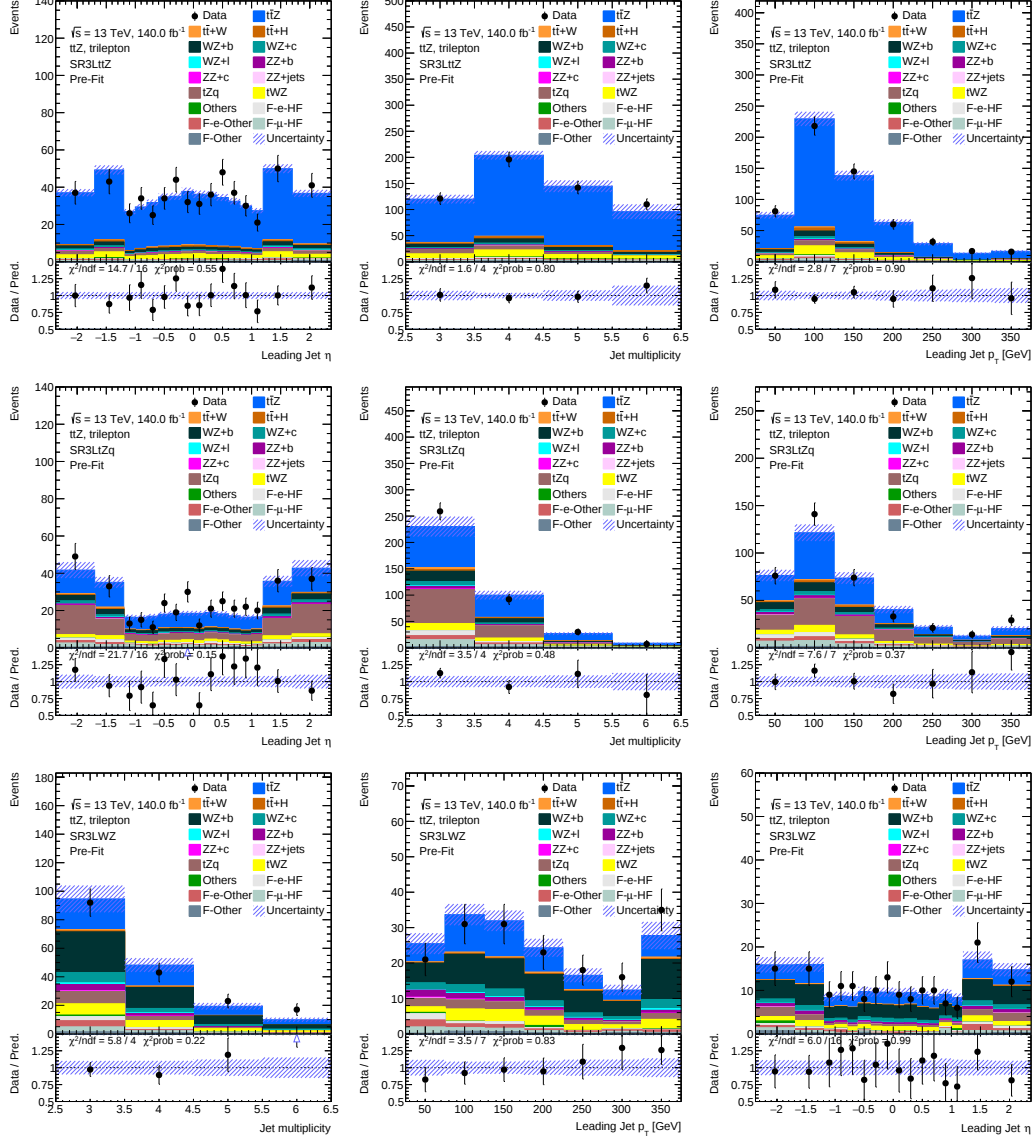
Figure 5.9: Data/MC comparison for basic kinematic variables in the SR\text{-}3\ell\text{-}t\bar{t}Z and SR\text{-}3\ell\text{-}tZq signal regions with events passing the event selection criteria. The blue uncertainty band includes statistical and systematic uncertainties. Events outside the histogram range are merged into the corresponding first or last bin.
