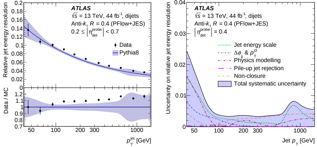
Figure 8.2: The relative JER as a function of p_T (left) and the overview of major JER uncertainty components for anti- k_t particle-flow jets (right). The black dots represent the resolution in data, and the solid blue line is the resolution in MC. The uncertainty is split into the major components, represented by a set of dotted lines, with the full uncertainty shown as a blue area. Figure is taken from Ref. [255].
