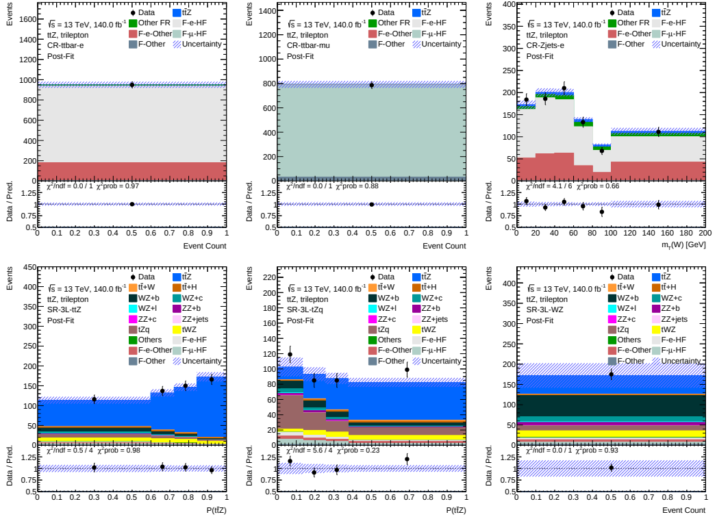
Figure 9.1: Distributions used in the fit to extract the inclusive cross-section. A fit is performed using the three signal regions ( SR\text{-}3\ell\text{-}t\bar{t}Z , SR\text{-}3\ell\text{-}tZq , SR\text{-}3\ell\text{-}WZ ) and the three fake-enriched control regions ( CR\text{-}t\bar{t}\text{-}e , CR\text{-}t\bar{t}\text{-}\mu , CR\text{-}Z\text{-}e ). The shaded error bands represent the combined statistical and systematic uncertainties. The shown observables, starting from the top left, are the event yield for CR\text{-}t\bar{t}\text{-}e and CR\text{-}t\bar{t}\text{-}\mu , the reconstructed transverse mass of the W ( m_T(W) ) for CR\text{-}Z\text{-}e , t\bar{t}Z probability ( P(t\bar{t}Z) ) for SR\text{-}3\ell\text{-}t\bar{t}Z and SR\text{-}3\ell\text{-}tZq , and the Event Count for SR\text{-}3\ell\text{-}WZ .
