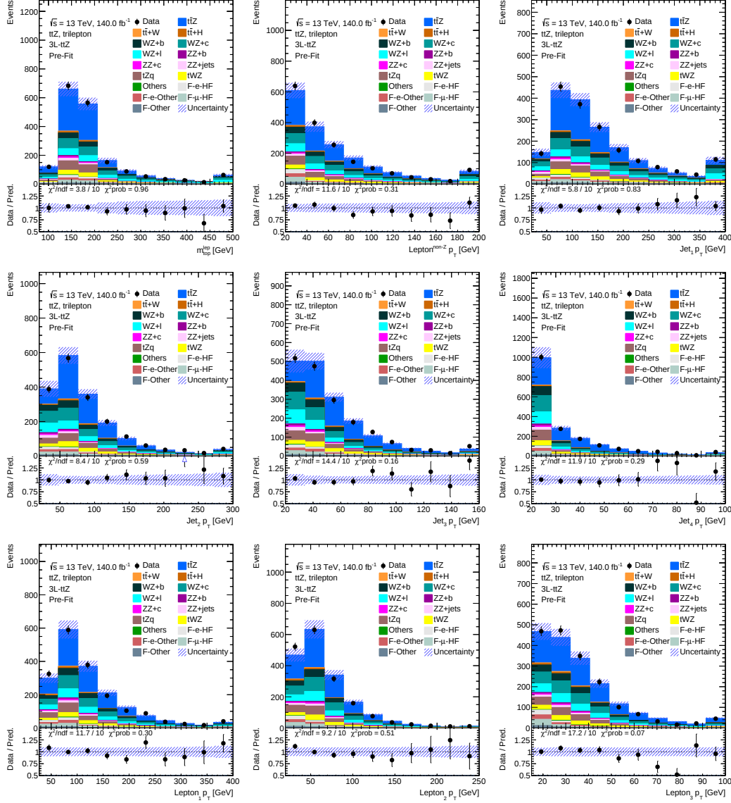
Figure 4.2: Distributions of the reconstructed mass of the leptonically decaying top quark, the p_T of the lepton not originating from the reconstructed Z boson, second-highest b -tagging working point in the event, the highest jet p_T , the 2 nd -highest jet p_T , the 3 rd -highest jet p_T , the 4 th -highest jet p_T , the highest lepton p_T , the 2 nd -highest lepton p_T , and the 3 rd -highest lepton p_T . The data is shown using black dots. The blue uncertainty band includes statistical and systematic uncertainties. Events outside the histogram range are merged into the corresponding first or last bin. A \chi^2 test evaluates the agreement between data and the MC simulation. The corresponding p -values are drawn in the lower pads of the distributions.
