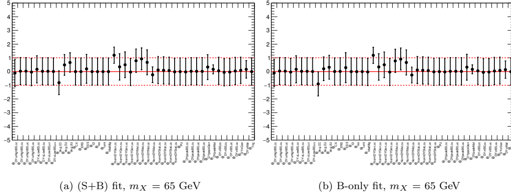
Figure 5.81: Pulls of the constrained nuisance parameters obtained for a signal mass hypothesis of 65 GeV, for the (a) S+B fit and (b) the background-only fit.
