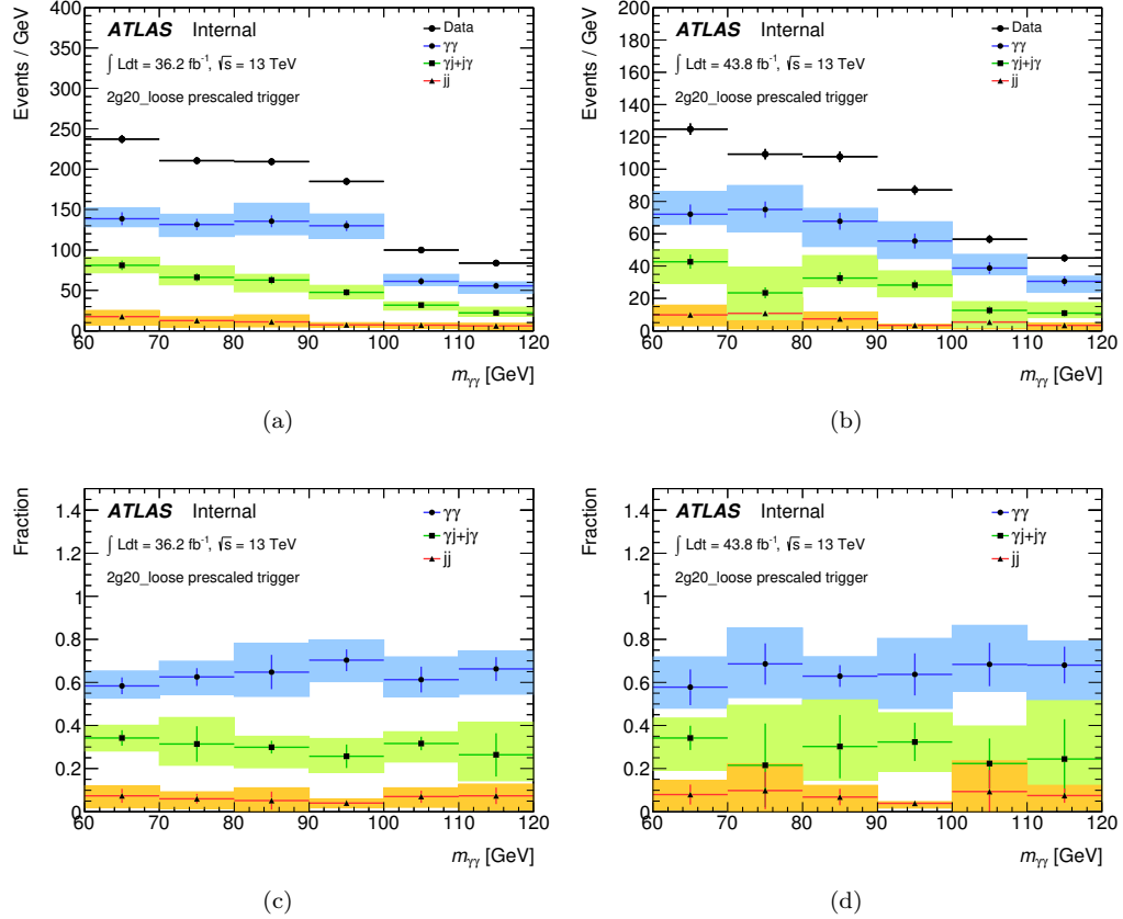
Figure 5.24: Data and \gamma\gamma , \gamma j and j j yields for the CC category, determined by the 2x2D sideband method as a function of the diphoton mass, for the years 2015+2016 (a) and 2017 (b). The resulting fractions are shown below and for 2015+2016 (c) and 2017 (d).
