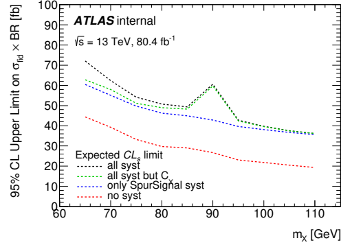
Figure 5.74: Expected limits on the fiducial production cross-section \sigma_{fid}.BR(X \rightarrow \gamma\gamma) of a narrow resonance as a function of the resonance mass m_X in the 65-110 GeV mass range, for different hypotheses: in red no systematic uncertainties are considered, in blue only the Spurious Signal uncertainties are considered, in green all uncertainties are considered except for the one on the C_X factor, in black all uncertainties (including the ones on the signal yield and the DY background) are considered.
