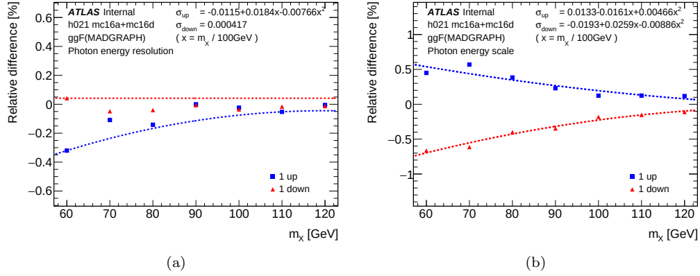
Figure 5.67: Systematic uncertainties associated with the photon energy resolution (a) and photon energy scale (b) as a function of m_X , computed with the Madgraph ggF sample.
