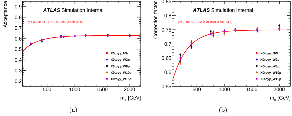
Figure 1.2: The acceptance factor (a) and the correction factor (b) for several resonance widths and at several masses of a scalar particle. The first part of the label Xtoyy refers to MC produced from a new particle X decaying to two photons. The last part of the labels are used to designate the decay width of the particles used in the MC samples, NW being the nominal narrow width sample.
