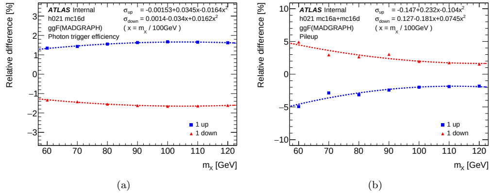
Figure 5.65: Systematic uncertainties associated with to the trigger efficiency (a) and pile-up (b) as a function of m_X , computed with the Madgraph ggF sample.
