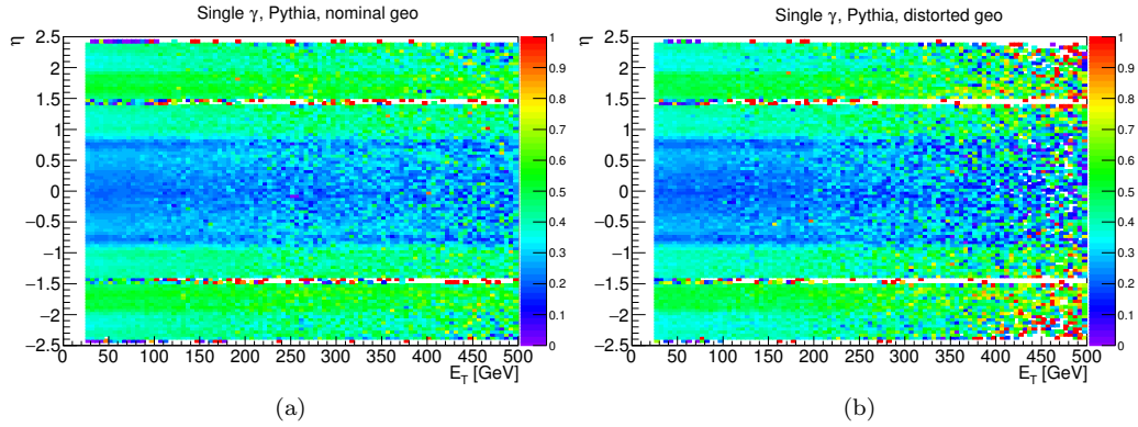
Figure 5.69: fraction of converted photons in bins of E_T and \eta for the (a) nominal and (b) distorted geometries.
