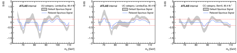
Figure 5.39: The spurious signal S divided by the background uncertainty in gray, and the relaxed spurious signal \zeta divided by the background uncertainty in blue as a function of M_X for the UU (a), UC (b) and CC (c) categories [43].
