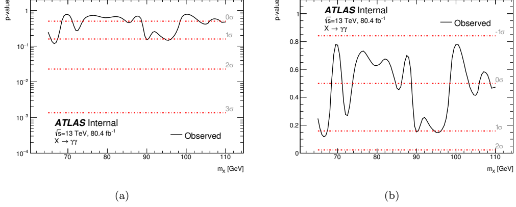
Figure 5.80: Observed p-value for the background-only hypothesis, p_0 , in (a) logarithmic and (b) linear scale, as a function of the resonance mass m_X .
