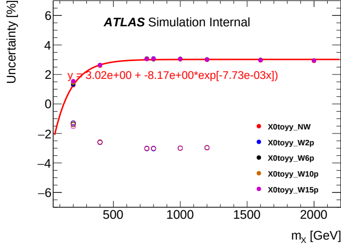
Figure 1.3: The uncertainty and fit function used for the photon ID efficiency. The closed circles represent variation of the nominal value up by 1\sigma . The open circles represent the variations down by 1\sigma .
