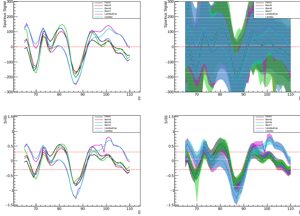
Figure 5.34: The spurious signal and the spurious signal divided by the background uncertainty with dashed lines representing 30% background uncertainty. Figures on the right include uncertainty in the CC category. The figures on the left are the same as those on the right but with no error bars shown.
