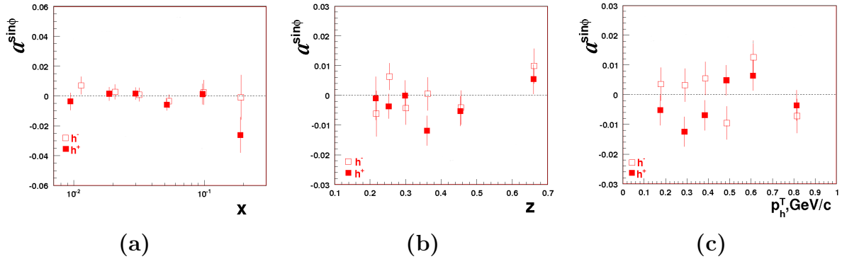
Figure 7.2: Amplitudes of \sin \phi_h as function of x , (a), z , (b), and P_T^h , (c). Results from positive (full squares) and negative (open squares) are superimposed.
