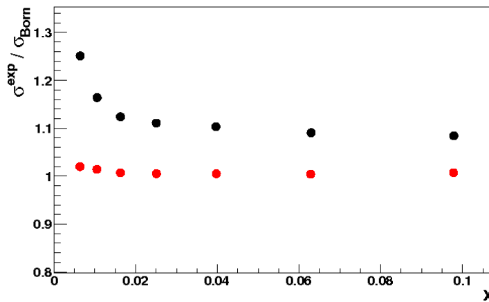
Figure 5.22: Weights ( \sigma^{\text{exp}}/\sigma^{\text{Born}} ) as function of x defined as the ratio between the DIS cross sections: calculated including the radiative effects and the Born one. The black points are the weights calculated using Lepto+Radgen and the red points are the calculations from [65], made for COMPASS and in the same kinematics.
