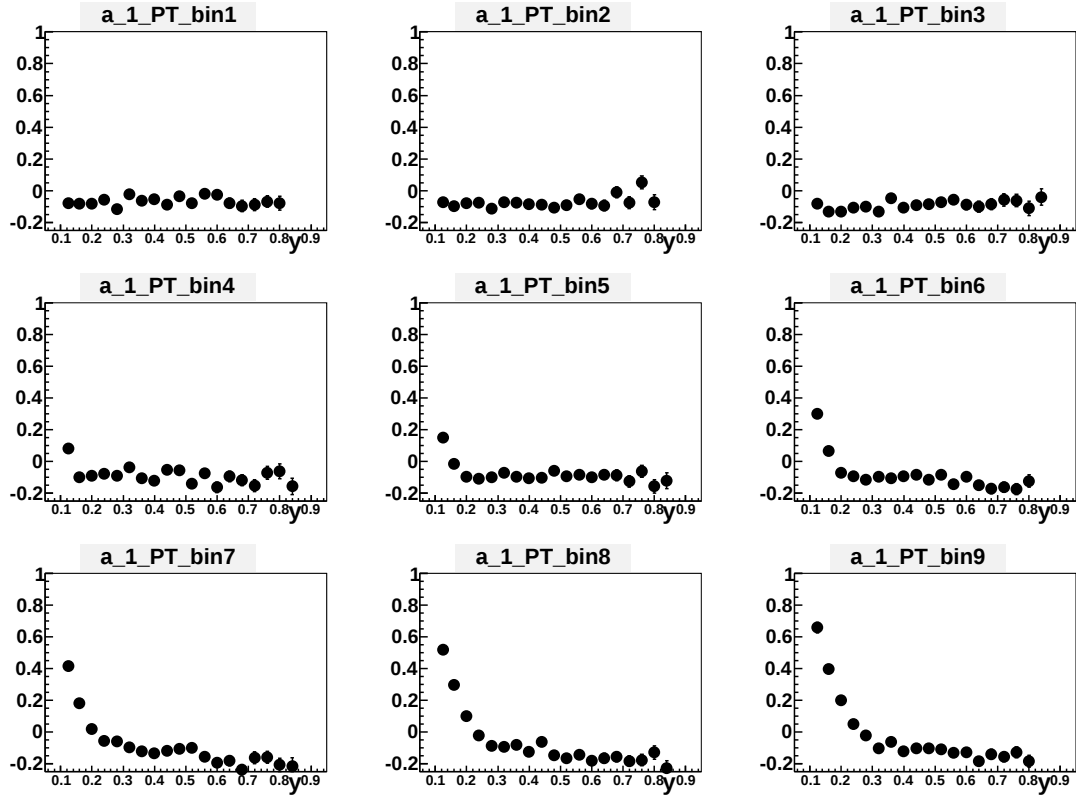
Figure 5.10: amplitudes a_1(y) of the \cos \phi_h modulation as a function of y (only the cuts P_T^h < 1 \text{ GeV}/c and \theta_{\gamma^*} < 0.06 \text{ rad} have been applied in addition to the “old cuts” described in section 5.1). Different plots correspond to different P_T^h bins (ranging from 0.1 to 1.0 \text{GeV}/c ).
