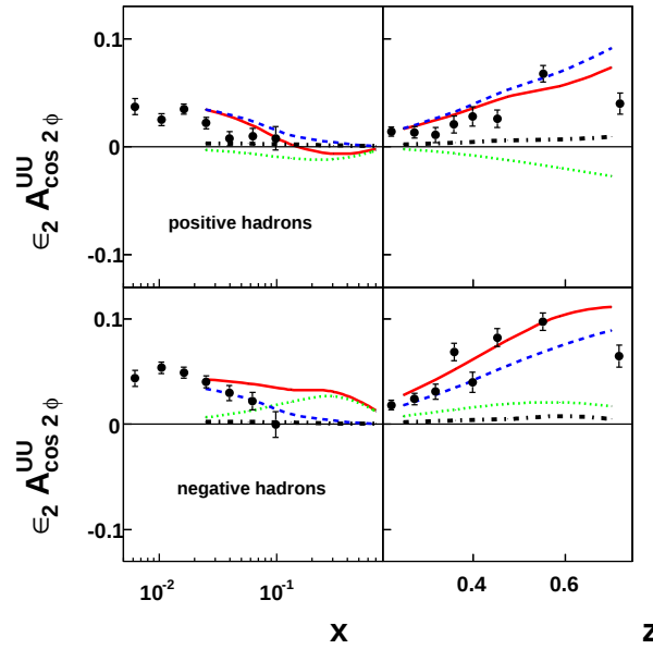
Figure 6.14: Theoretical calculations for the \epsilon_2 A_{\cos 2\phi_h} amplitude as functions of x (left) and z (right) for positive (top) and negative (bottom) pions ( \gtrsim 90\% of the analysed hadrons): predictions from [41]. The red solid line is the sum of three different contributions: Boer-Mulder function (green, dotted), Cahn effect (blue, dotted) and pQCD (black-dotted).
