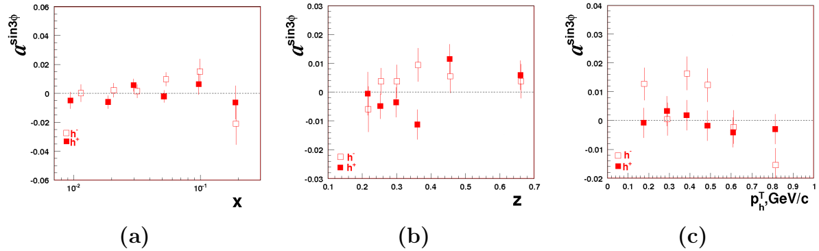
Figure 7.4: Amplitudes of \sin 3\phi_h as function of x , (a), z , (b), and P_T^h , (c). Results from positive (full squares) and negative (open squares) are superimposed.
