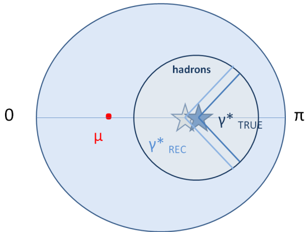
Figure 5.23: Illustration of the effect on the azimuthal distribution of the hadrons of a mis-reconstructed virtual photon. The beam impinges on the picture, perpendicularly to the sheet, and, for simplicity, let assume that the big circle is the acceptance of the COMPASS apparatus projected on the XY plane perpendicular to the beam line. From the momentum conservation the scattered muon (the red point) and the virtual photon (the blue star) go at opposite sides of the incoming muon. The SIDIS hadrons are produced mostly inside a cone, having the virtual photon at the centre and represented by the smaller circle in the picture. The \phi_h distribution is essentially given by the counts of the hadrons which go into one sector of the small circle (drawn at \pi in the picture). If the reconstructed virtual photon direction is systematically shifted towards smaller values of the polar angle, with respect to the real one, a greater number of hadrons is counted in the bin at \pi while a lesser number is counted at zero, with respect to the situation of an exactly reconstructed virtual photon direction. This systematic effect is given, for example, if the momentum of the scattered muon is always underestimated and gives an additional \cos \phi_h modulation in the hadron distribution.
