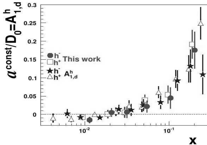
Figure 7.6: Comparison between a_{const}(x)/D_0 and A^h_{1,d}(x) from [86] for positive hadrons (open squares and open triangles) and negative hadrons (full circles and full stars).
