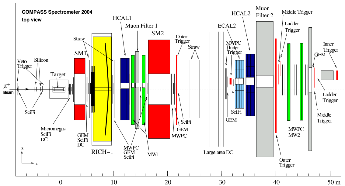
Figure 3.1: Compass 2004 muon setup (top) artistic view, (bottom) top view.
