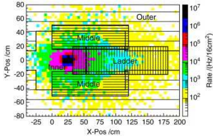
Figure 3.12: Schematic view of the hodoscope stations of the different subsystems projected on the vertical YX plane. The size of the different hodoscopes are also indicated. The simulated beam rate is also shown (the beam comes perpendicular to the sheet).
