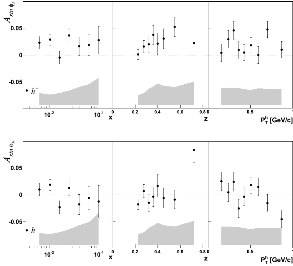
Figure 6.5: The A_{\sin \phi_h} azimuthal asymmetries as functions of x , z and P_T^h , obtained for positive hadrons (upper plot) and negative hadrons (lower plot). Grey bands are the systematic error ( \sigma_{sys} = 2 \cdot \sigma_{stat} ).
