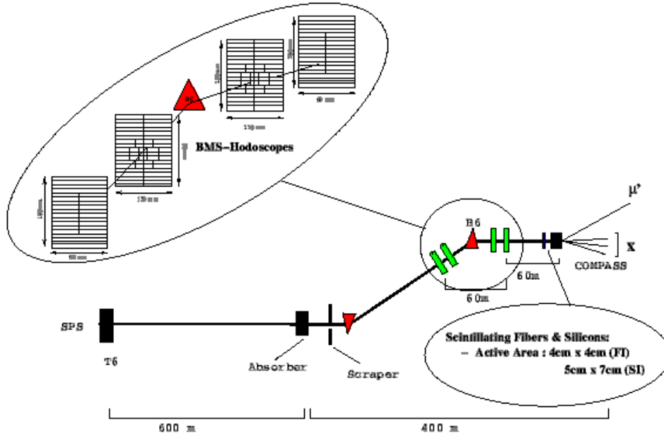
Figure 3.2: The M2 beam line.
