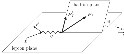
Figure 2.1: Definition of the Gamma Nucleon System (GNS).
