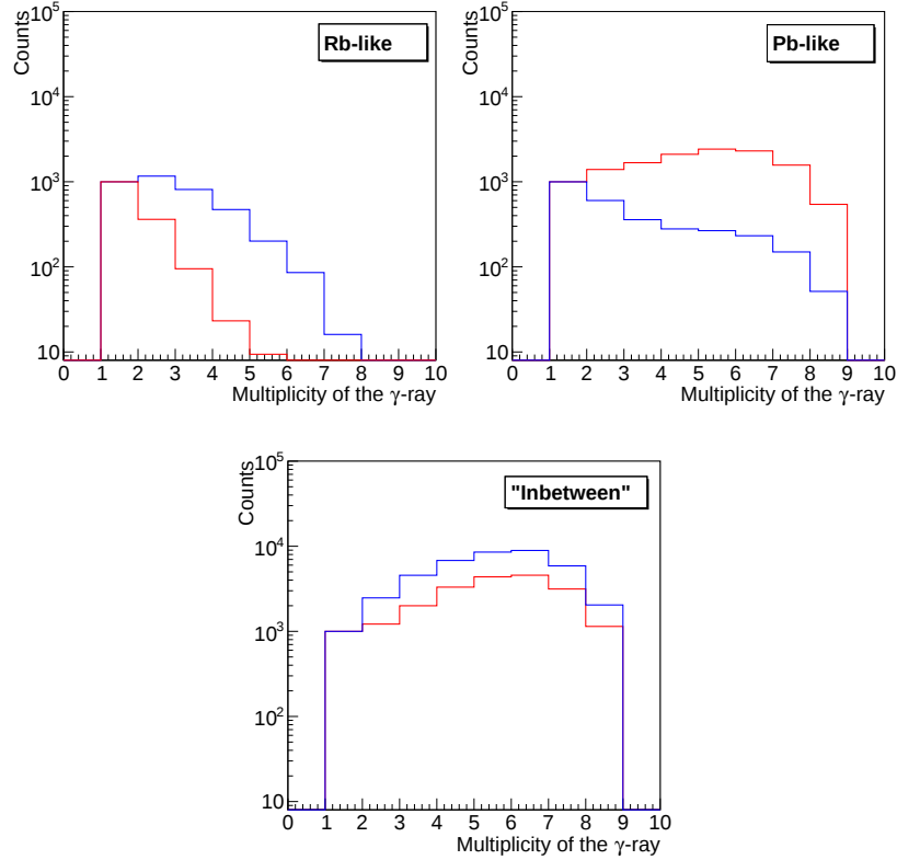
Figure 4.2: Gamma-ray multiplicity distribution in coincidence with the fragment which is given in the inset. The different \theta_{\text{LAB}} regions are labeled with different colors, red corresponding to the \theta_{\text{LAB}} = [41, 54]^\circ , and blue to the \theta_{\text{LAB}} = [54, 63]^\circ .
