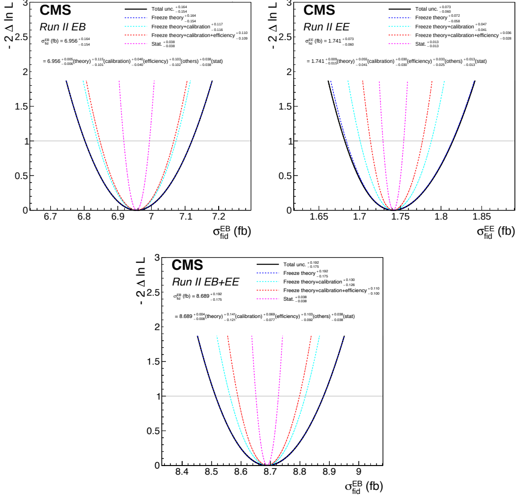
Figure 6.3: Likelihood scans of the fiducial cross section for EB (top left), EE (top right), and combining EB+EE (bottom). The solid black line takes into account all the uncertainties (statistical and systematic), while the dashed lines refer to likelihood scan in which one or more sources of uncertainties are not considered ( frozen ).
