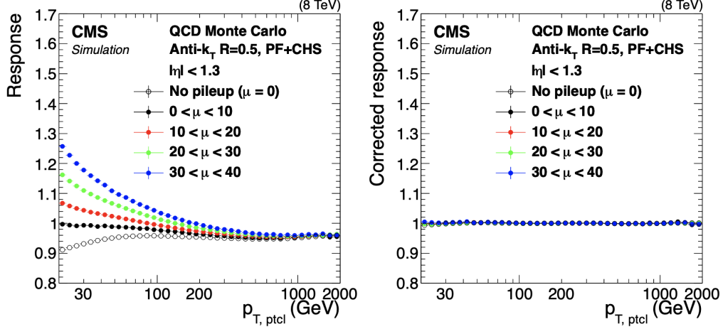
Figure 3.17: Average ratio of the reconstructed jet p_T over the particle-level jet p_T in QCD simulation, as a function of the particle-level jet p_T . The jets are reconstructed with the anti- k_T clustering algorithm (with R=0.5 ) and the CHS method for pileup mitigation. The ratio is shown before any corrections (left) and after (right) all the stages of the JEC, while \mu denotes the average number of pileup interactions per bunch crossing [148].
