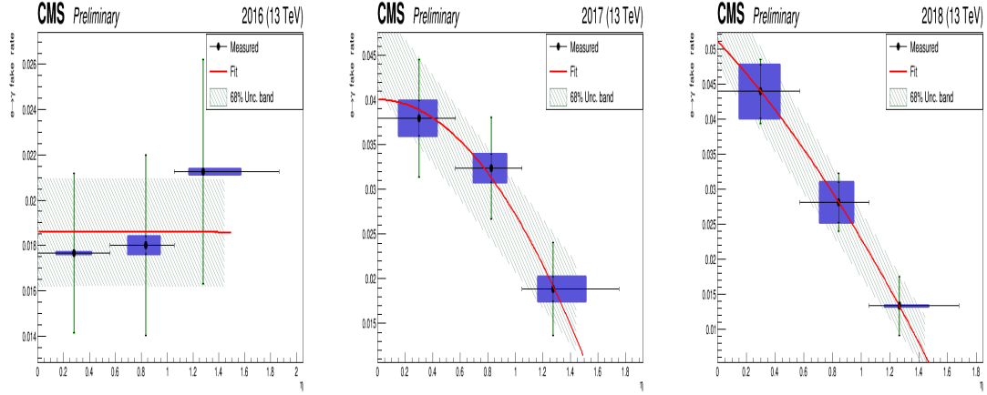
Figure 5.9: Electron to photon fake ratio as a function of the absolute value of pseudo-rapidity \eta for 2016 (left), 2017 (center) and 2018 (right). Green error bars are statistical error and blue rectangles are the systematic errors. The error band corresponds to the 68% coverage of the fake ratio distribution as a result of the uncertainty on the fitted parameters of a 2 nd order polynomial.
