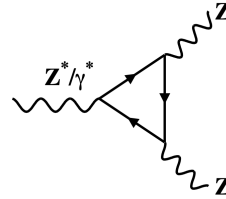
Figure 2.2: Fermionic triangle contributing to the \gamma ZZ and \gamma ZZ couplings at 1-loop level.
