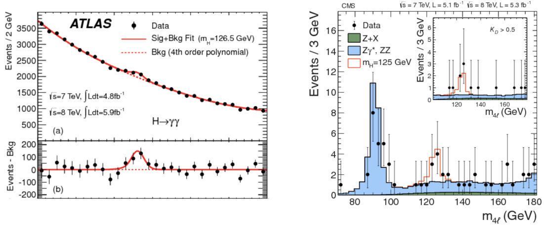
Figure 1.8: (Left) The reconstructed invariant mass distribution of the diphotons candidates in the ATLAS experiment [35]. The points represent the data, the dotted line represents the background, and the solid line the fit to the data of the sum of a signal component fixed to m_H = 126.5 GeV and of a background component. (Right) The distribution of the reconstructed invariant masses of the four leptons candidates in the CMS experiment [34]. The points represent the data, the filled histograms represent the background, and the open histogram shows the signal expectation for a Higgs boson of mass 125 GeV.
