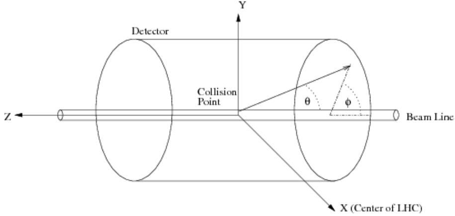
Figure 3.3: Schematic illustration of the coordinate system used by the LHC experiments.
