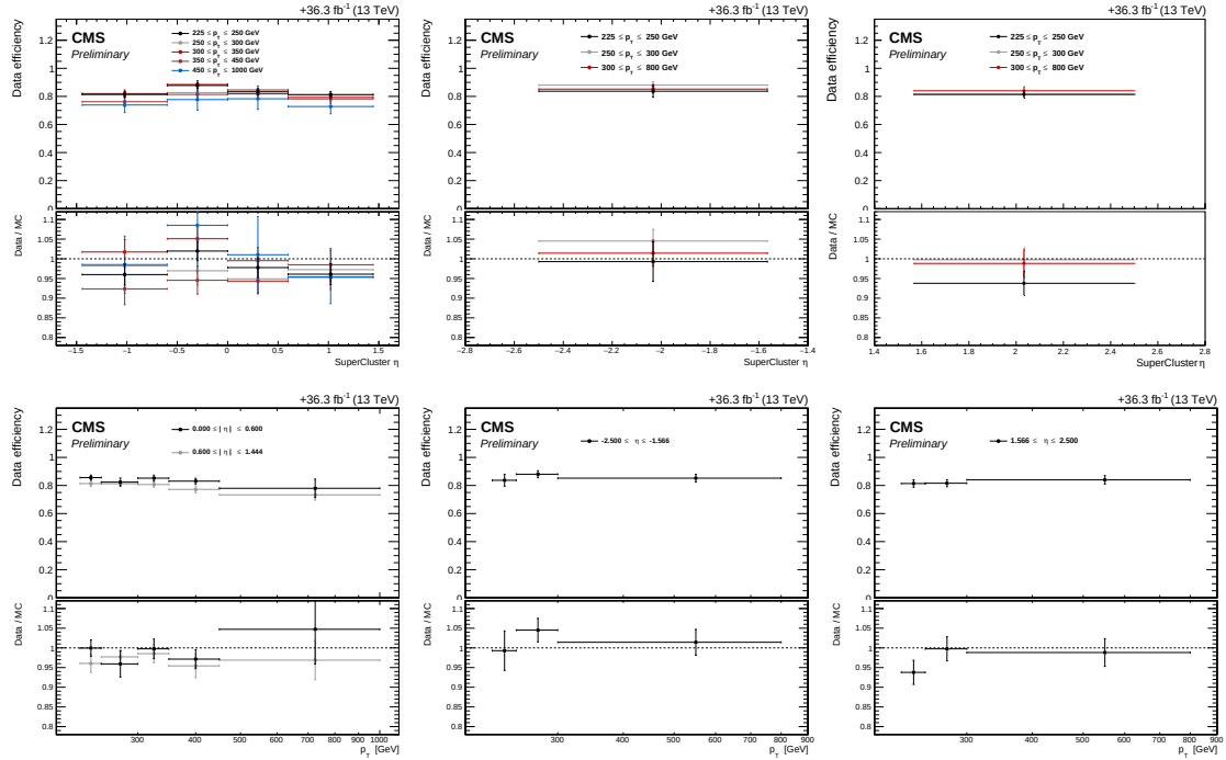
Figure B.6: Photon ID efficiencies in data as a function of \eta (top) and p_T (bottom), for the 2016 year, in EB (left) and EE (center and right). The ratio between the data and the MC efficiencies is also shown in the bottom panel of each plot.
