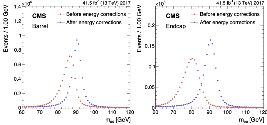
Figure 3.14: Dielectron invariant mass distribution before and after the application of the energy and scale corrections for barrel (left) and endcap (right) electrons for Z \rightarrow e^-e^+ events [142].
