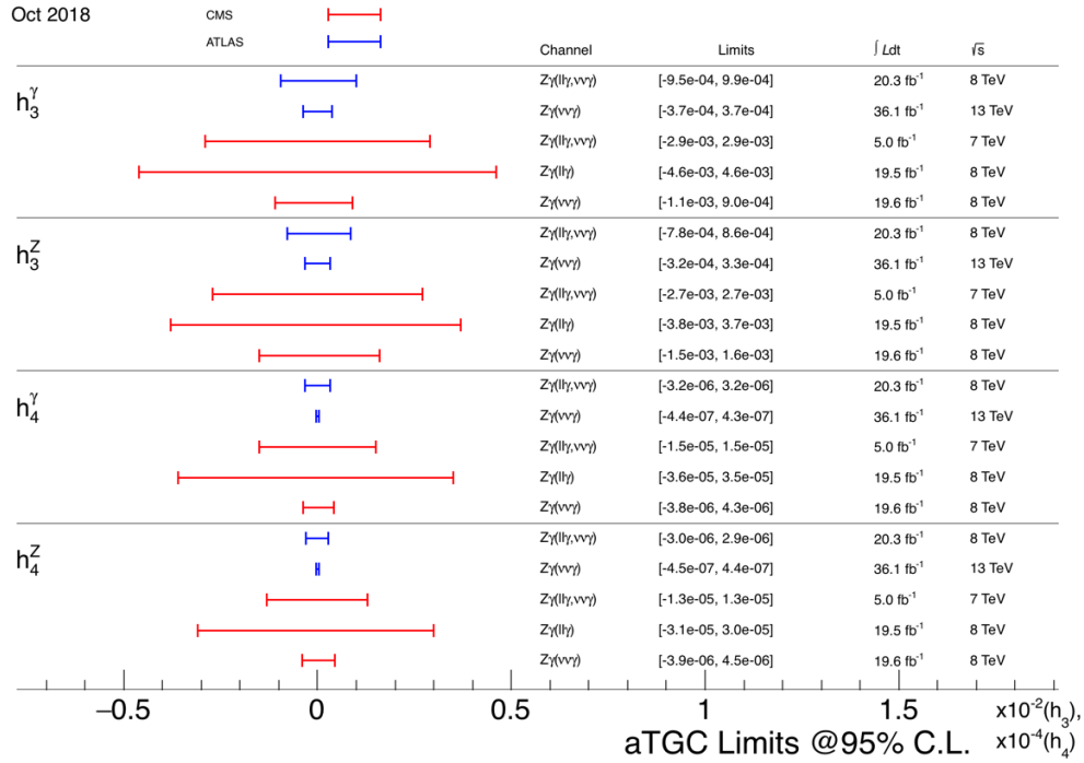
Figure 2.3: Limits on neutral Z\gamma\gamma and ZZ\gamma aTGC couplings. The limits have been placed on the anomalous parameters h_3 and h_4 [99].
