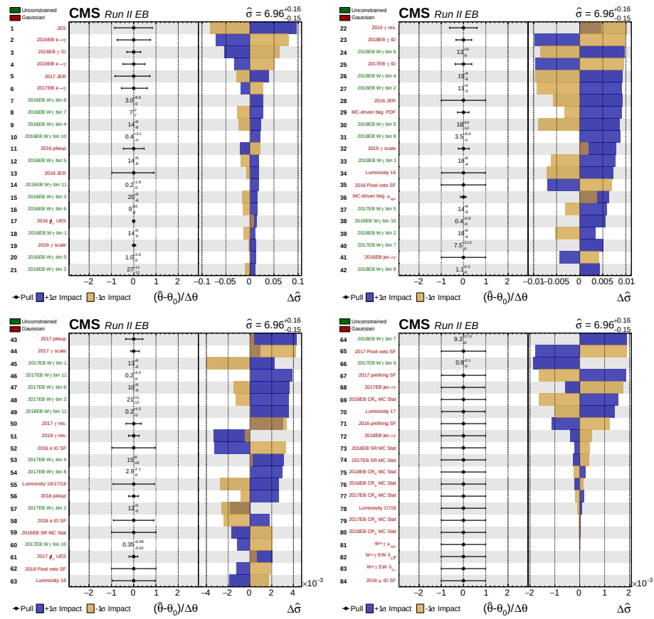
Figure A.1: Impacts and pulls of the systematics on the expected cross section measured in EB.
