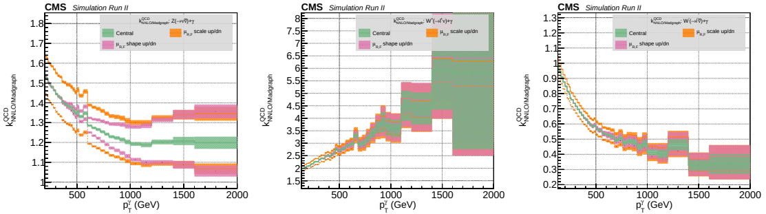
Figure 6.2: QCD NLO/LO k-factors as a function of the photon transverse momentum, as they are applied to Z\gamma (left), W^-\gamma (center) and W^+\gamma (right) simulated events.
