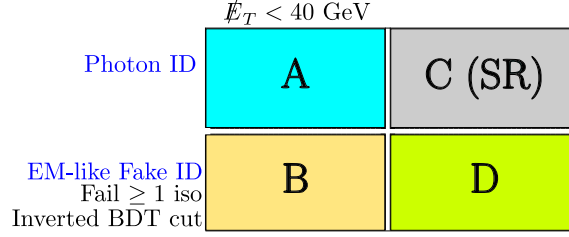
Figure 5.10: The four disjoint regions used to estimate the \text{jet} \rightarrow \gamma fake ratios.
