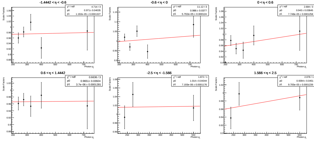
Figure B.9: Fit of the scale factors distribution as a function of p_T for 2016.
