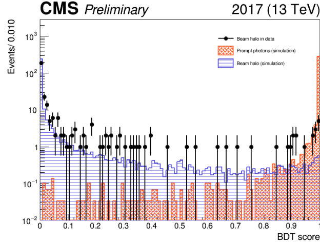
Figure 5.19: Distribution of the BDT score of simulated prompt photons originating from collisions (red) and beam halo (blue). The BDT score of beam halo photons in data is also shown, where the beam halo dataset is built using events that fail the central beam halo filter.
