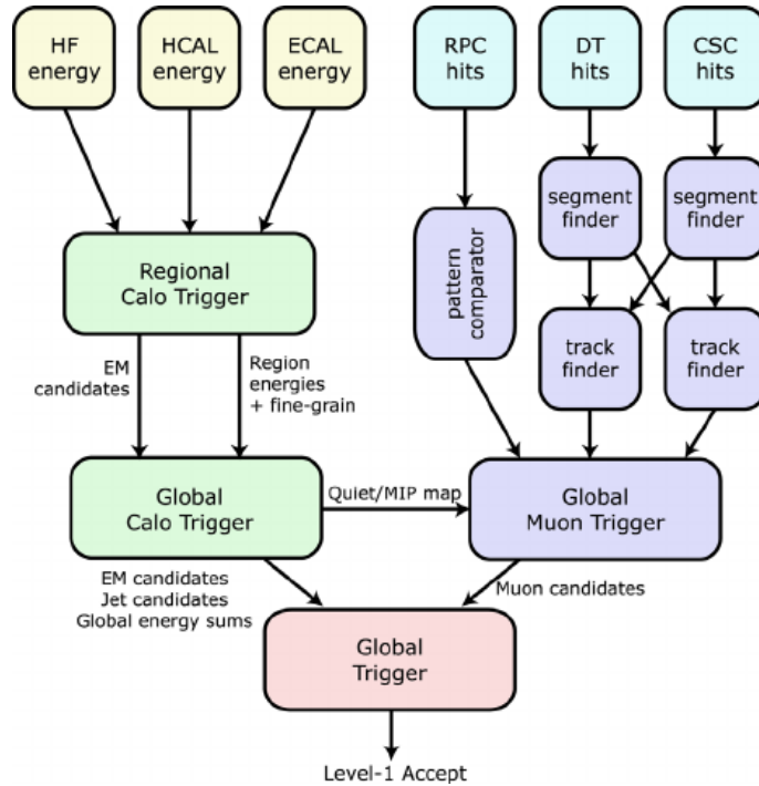
Figure 3.8: Overview of the CMS L1 trigger system. Data from the hadronic and from the electromagnetic calorimeter are processed first regionally (RCT) and then globally (GCT). The hits collected in the muon system are processed and sent onwards to a global muon trigger (GMT). The information from the GCT and GMT is combined in a global trigger (GT), which makes the final trigger decision [131].
