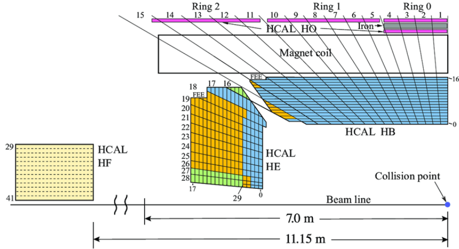
Figure 3.6: A schematic view of one quarter of the CMS HCAL during 2016 LHC operation, showing the positions of its four major components: the hadron barrel (HB), the hadron endcap (HE), the hadron outer (HO), and the hadron forward (HF) calorimeters [126].
