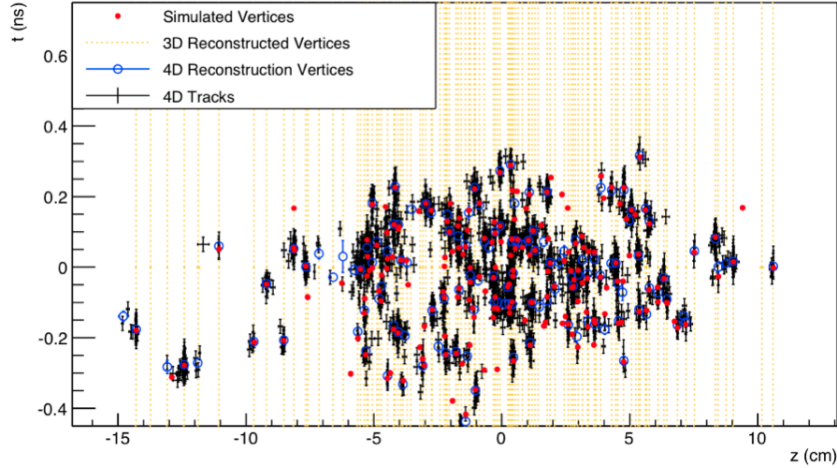
Figure 4.3: Simulated and reconstructed vertices in a bunch crossing with 200 PU interactions assuming a MIP timing detector with 30 ps time resolution covering the barrel and endcap regions. The simulated vertices are the red dots. The vertical yellow lines represent the vertices reconstructed without the timing information (3D vertices), while the black crosses and the blue open circles represent tracks and vertices reconstructed including the time information, and hence they are labeled as 4D. The horizontal axis refers to the z position along the beam line, while the vertical axis to the vertex time. As can be seen, many of the 3D vertices that would not be resolved solely on the basis of the spatial coordinates are clearly separated when using the time information [169].
