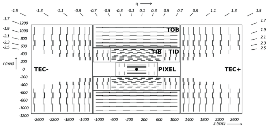
Figure 3.4: Projected view of the CMS tracker layout in the r - z plane [117].
