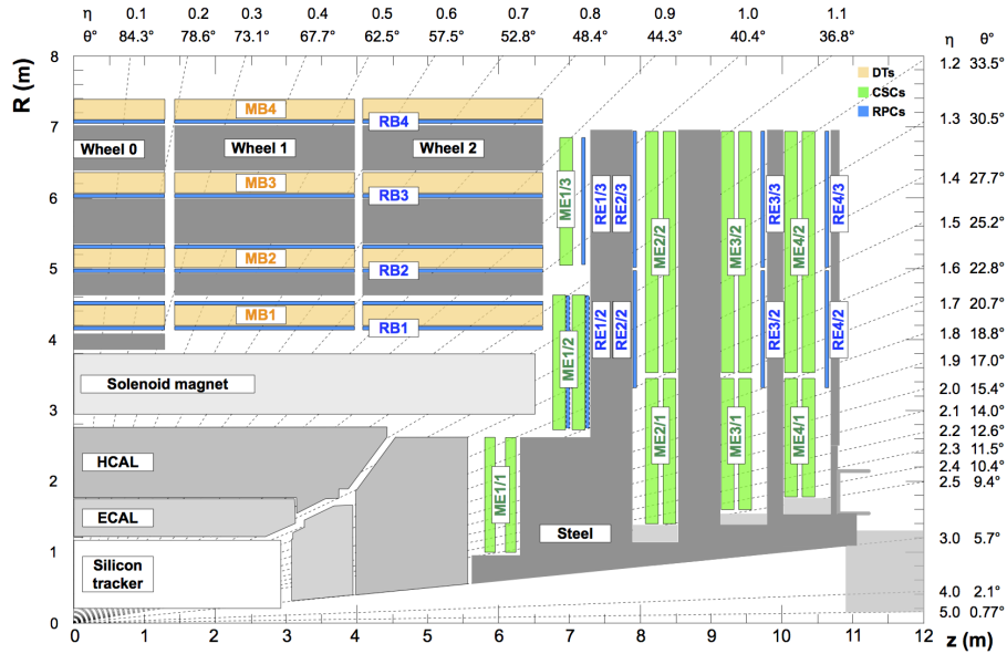
Figure 3.7: An R - z cross section of a quadrant of the CMS detector with the axis parallel to the beam ( z ) running horizontally and the detector's radius ( R ) increasing upward. The drift tube stations (DTs) are labeled MB (“Muon Barrel”) and the cathode strip chambers (CSCs) are labeled ME (“Muon Endcap”). Resistive plate chambers (RPCs) are mounted in both the barrel and endcaps of CMS, where they are labeled RB and RE, respectively [128].
