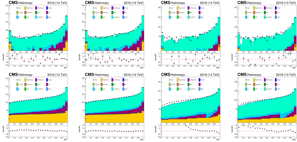
Figure C.4: Data-MC comparison of the BDT score and CDF in Z \rightarrow e^- e^+ + \text{jets} events for 2016, before (left) and after (right) the application of quantile-quantile corrections.
