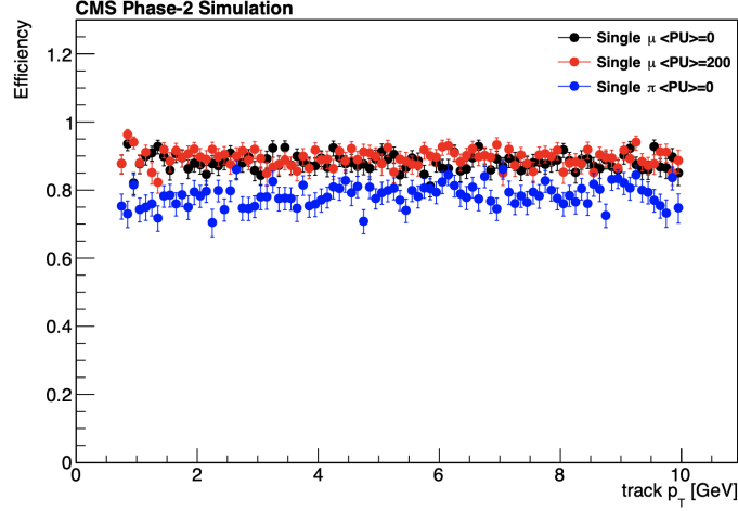
Figure 4.6: Efficiency to find an MTD cluster associated with a reconstructed track as a function of transverse momentum. The efficiency obtained using a sample of simulated muons without pileup is shown in black. The results are compared to those obtained with a simulated sample of muons with an average of 200 pileup events (red) and a simulated sample of pions without pileup (blue). The efficiency is about 90% for muons, and about 80% for pions, lowered by the effects of nuclear interactions in the tracker volume [169].
