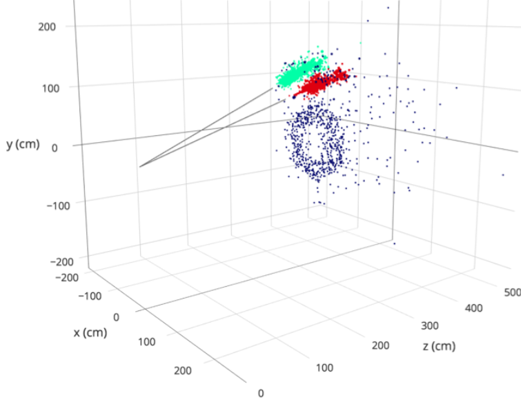
Figure 4.2: Two pions, separated by 30 cm, clustered by the (first exploratory version of) direct 3D clustering algorithm in HGCal [165].
