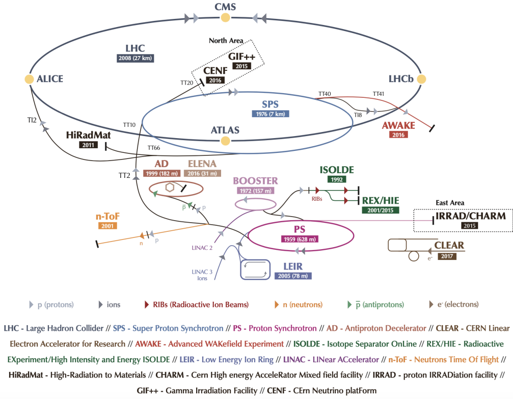
Figure 3.1: The injection chain for the Large Hadron Collider [103].
