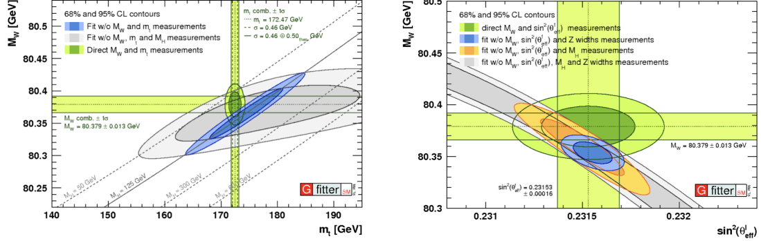
Figure 1.5: (Left) Contours of 68% and 95% confidence level obtained from scans of fits with fixed variable pairs of W mass M_W and top mass m_t . The narrower blue and larger grey allowed regions are the results of the fit including and excluding the M_H measurement, respectively. The horizontal bands indicate the 1\sigma regions of the M_W and m_t measurements. (Right) Contours of 68% and 95% confidence level obtained from scans of fits with fixed variable pairs of M_W and the effective weak mixing angle \sin^2 \theta_{eff} . The narrower blue and larger grey allowed regions are the results of the fit including and excluding the M_H measurements, respectively. The horizontal bands indicate the 1\sigma regions of the M_W and \sin^2 \theta_{eff} measurements (world averages) [50].
