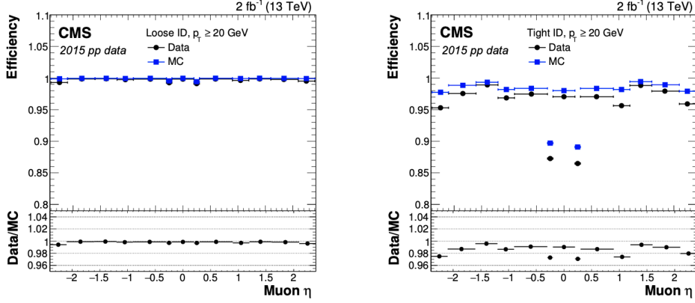
Figure 3.19: Efficiency for muon reconstruction and identification in 2015 data (circles) and simulation (squares), evaluated by applying the Tag and Probe method to muons coming from J/\psi and Z decays. The efficiencies for probe muons with p_T > 20 GeV passing the Loose ID (left) and the Tight ID (right) are shown in the upper panels, while the ratio between efficiencies in data and simulation is shown in the bottom panels. The statistical uncertainties are smaller than the symbols used to display the measurements [150].
