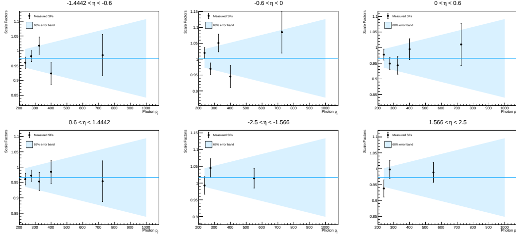
Figure B.12: Additional p_T -systematics estimated for 2016. The error band is obtained from the 68% limit on the gradient of the SFs linear fit.
