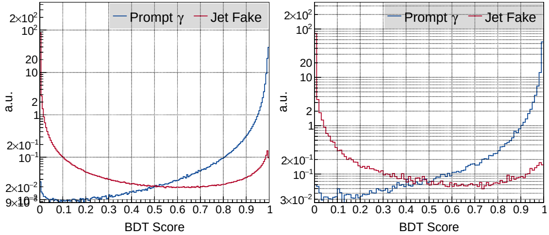
Figure 5.2: BDT distributions for simulated prompt (blue) and fake (red) photons for 2017 EB (left) and EE (right). The overlap between signal and background distributions is lower here than in any single shower shape variable, hence providing a better discrimination power.
