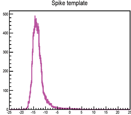
Figure 5.16: Timing distribution of the spike template as observed in [195]. On the x -axis the time associated to spikes is shown, considering as t=0 the seedtime of the supercluster. As it can be seen, spike events are mostly distributed at negative time, outside the prompt ( seedtime \pm 3 ns) window.
