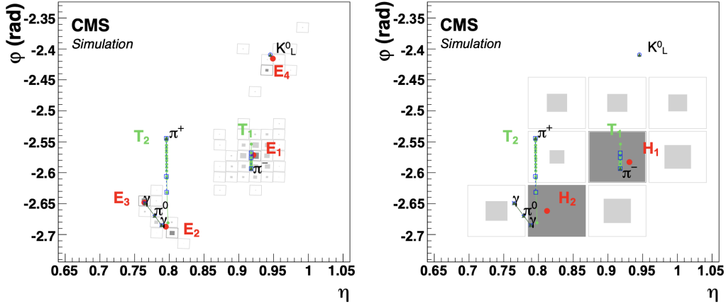
Figure 3.12: ECAL and HCAL clusters originated by a jet made of five particles ( K_L^0 , \pi^+ , \pi^- , \pi^0(\rightarrow \gamma\gamma) ). The ECAL and HCAL cells are represented as squares, with an inner area proportional to the logarithm of the cell energy. Cells with an energy larger than those of the neighboring cells are shown in dark grey, the cluster positions are represented by red dots, the simulated particles by dashed lines, and the positions of their impacts on the calorimeter surfaces by open markers. (Left) Four separated ECAL clusters originated by the K_L^0 , the \mu , and the two photons from the \pi^0 , denoted as E_1 , E_2 , E_3 , E_4 . The \pi^+ does not create a cluster in the ECAL. The two charged \pi are also reconstructed as charged-particle tracks T_1 and T_2 . (Right) Two HCAL clusters, originated by the two charged \pi and denoted as H_1 and H_2 [133].
