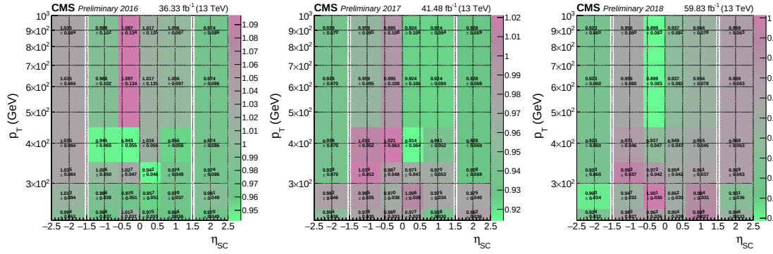
Figure B.5: Photon ID scale factors to correct for differences between data and MC in the estimation of the ID efficiency in 2016 (left), 2017 (center) and 2018 (right).
