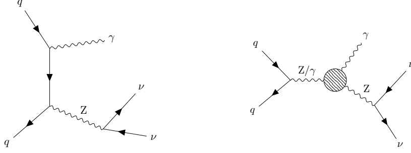
Figure 2.1: Production channels for the Z\gamma process: SM t-channel (left) and s-channel including the presence of the aNTGC (right).
