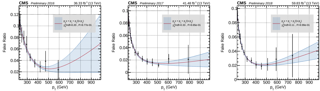
Figure 5.13: Distribution of the \text{jet} \rightarrow \gamma fake ratios as a function of the photon p_T in EB for 2016 (left), 2017 (center) and 2018 (right).
