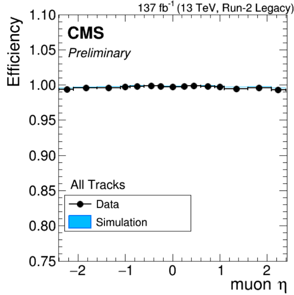
Figure 3.11: The tracking efficiency as a function of the muon pseudorapidity. The efficiency in data (black dots) is compared to that obtained using a simulated Z \rightarrow \mu^- \mu^+ sample (blue boxes) [141].
