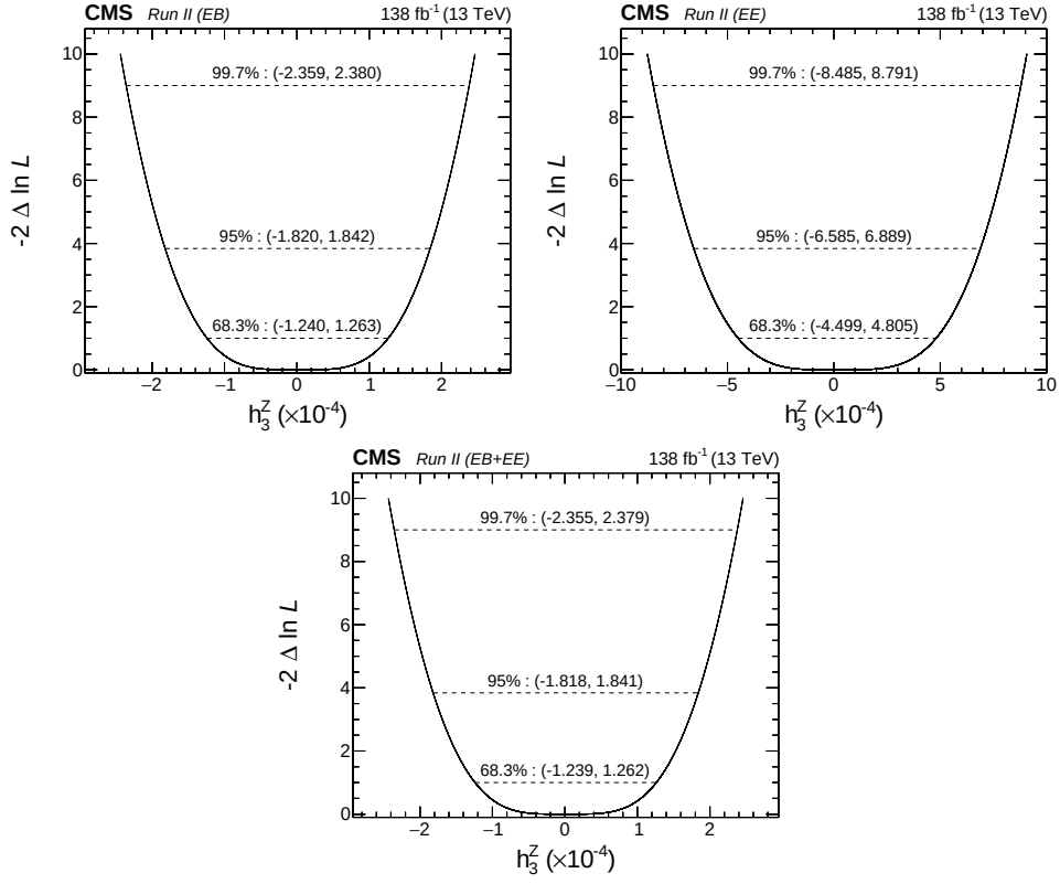
Figure 6.6: Likelihood scans for the estimation of the limits on h_3^Z in EB (top left), EE (top right) and for the EB+EE combination (bottom), with h_4^Z set to zero.
