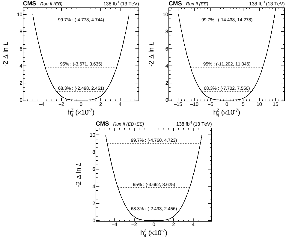
Figure 6.7: Likelihood scans for the estimation of the limits on h_4^Z in EB (top left), EE (top right) and for the EB+EE combination (bottom), with h_3^Z set to zero.
