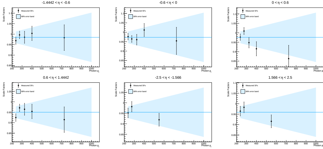
Figure B.13: Additional p_T -systematics estimated for 2017. The error band is obtained from the 68% limit on the gradient of the SFs linear fit.
