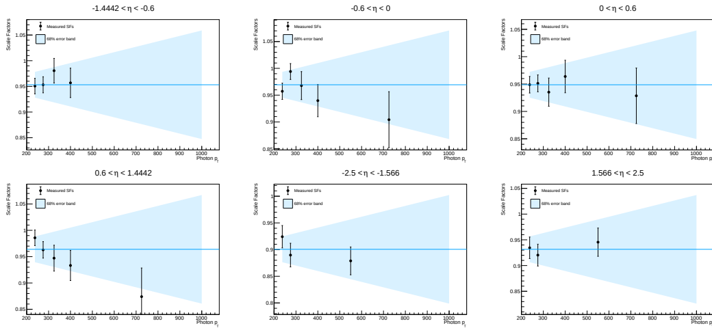
Figure B.14: Additional p_T -systematics estimated for 2018. The error band is obtained from the 68% limit on the gradient of the SFs linear fit.
