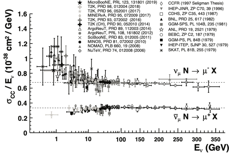
Figure 3.20: Total inclusive charged current cross section for a neutrino ( \nu_\mu N \rightarrow \mu^- X ) scattering off nucleons, as a function of its energy. Neutrino cross sections are typically twice as large as their corresponding antineutrino counterparts. Neutral current cross sections (not shown here) are generally smaller compared to the charged current case [45].
