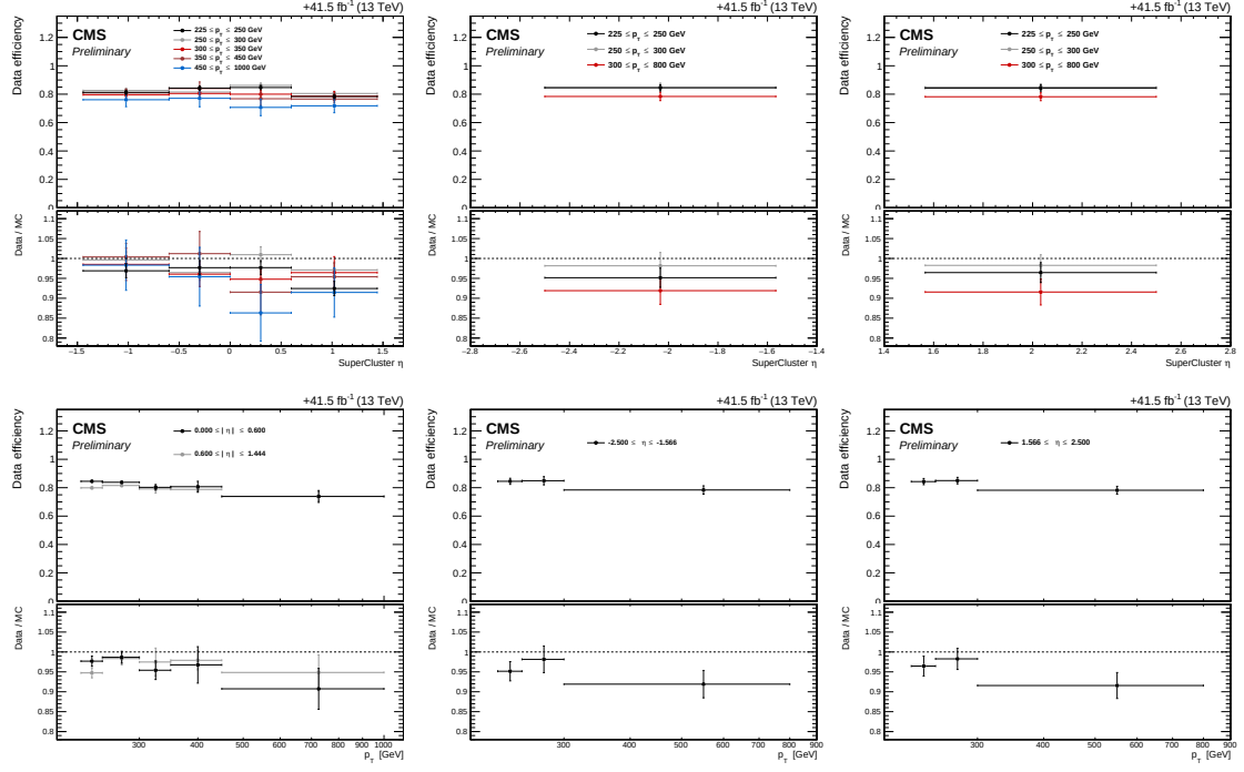
Figure B.7: Photon ID efficiencies in data as a function of \eta (top) and p_T (bottom), for the 2017 year, in EB (left) and EE (center and right). The ratio between the data and the MC efficiencies is also shown in the bottom panel of each plot.
