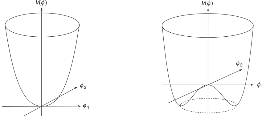
Figure 1.7: The V(\phi) potential for (left) \mu^2 > 0 and (right) \mu^2 < 0 .
