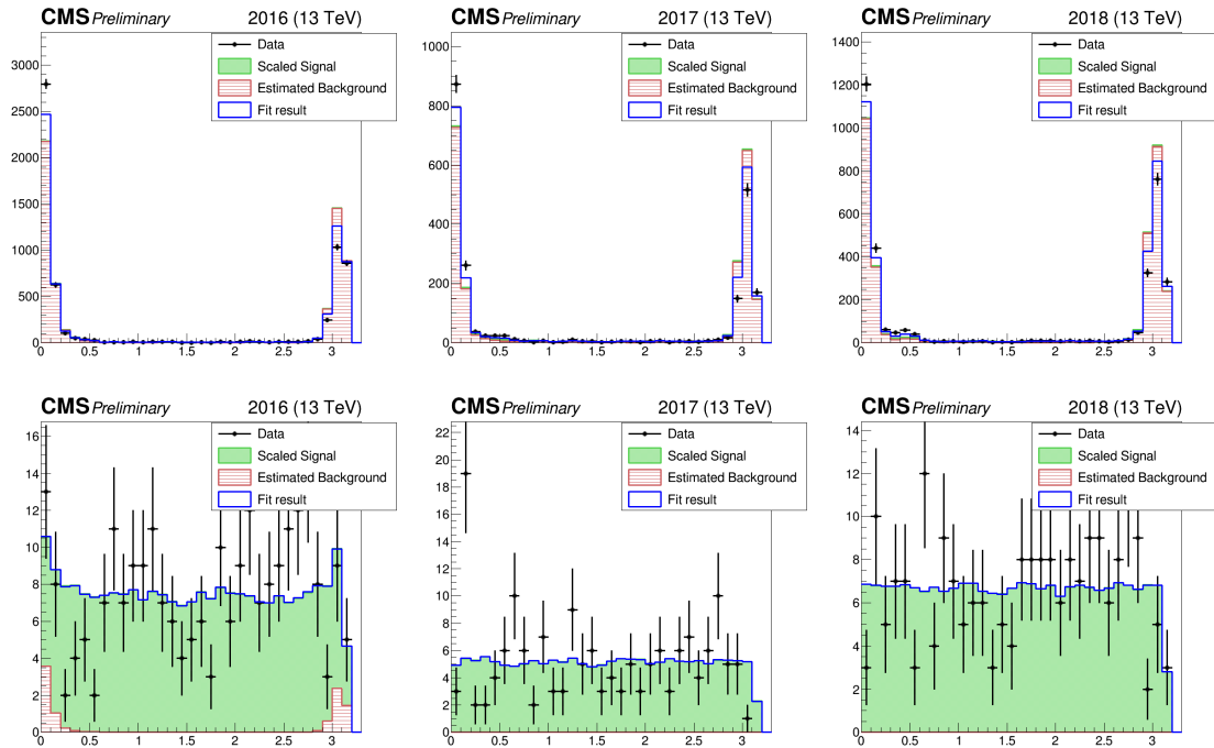
Figure 5.20: Template fits of the \phi distribution of the signal photon in the EE region, for 2016 (left), 2017 (center) and 2018 (right). The distributions are obtained, respectively, using the CMS central tagger (top) and the new BDT BH tagger (bottom).
