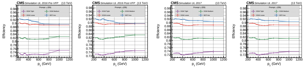
Figure B.1: From left to right: signal efficiency evaluated in EB from MC \gamma + jets samples as a function of p_T for years 2016-preVFP, 2016-postVFP, 2017 and 2018.
