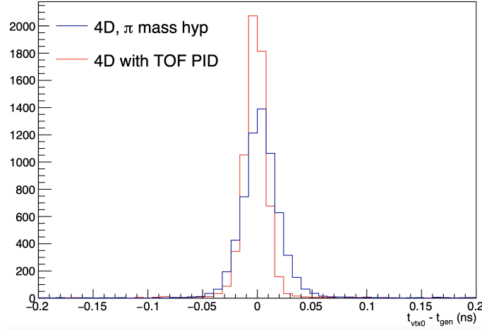
Figure 4.8: Distribution of the difference of the reconstructed ( t_{vtx0} ) and simulated ( t_{gen} ) time of the primary vertex in simulated t\bar{t} events with 200 PU as reported in the MTD Technical Design Report [169]. The resolution resulting after the first step of the 4D vertex reconstruction (using the \pi mass hypothesis) is shown in blue, while the ultimate resolution (after the particle identification step) is shown in red. The root mean square of the distribution obtained after the second step is about 10 ps.
