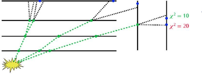
Figure 3.10: The scheme of the Cellular Automaton track seed algorithm when propagating a triplet to the fourth pixel layer [136].
