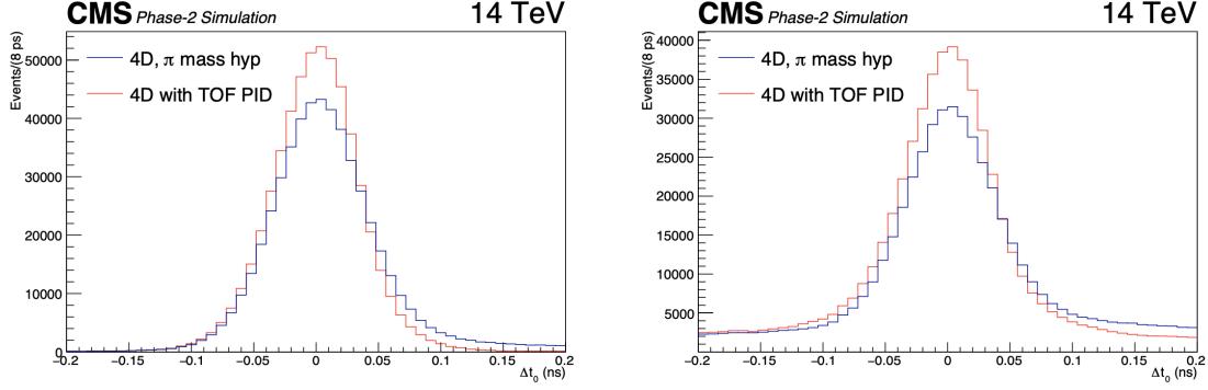
Figure 4.7: Difference between the reconstructed and the simulated track time at the vertex in t\bar{t} events, for particles reconstructed within |\Delta z| < 1 mm of the generated hard interaction. Events with no pileup (left) and 200 PU (right) are shown.
