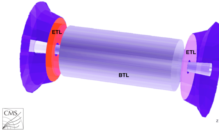
Figure 4.5: A schematic view of the MTD geometry, as it is used by CMS for simulation studies. The grey cylinder represents the BTL, while the red and light violet discs represent the ETL, closing the barrel region at both sides [169].
