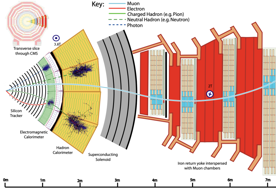
Figure 3.9: A sketch of the specific particle interactions in a transverse slice of the CMS detector. The muon and the charged pion are positively charged while the electron is negatively charged [133].
