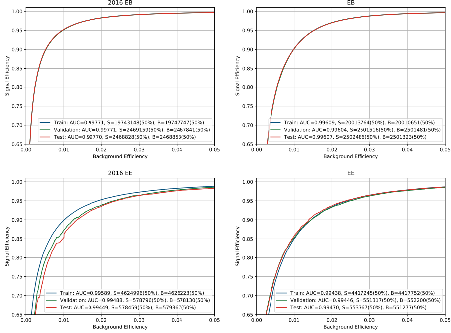
Figure 5.3: Photon BDT ROC curves for 2016 EB (top left) and EE (bottom left), and for 2017/18 EB (top right) and EE (bottom right). The test samples are independent of the training samples, and they show similar performance.
