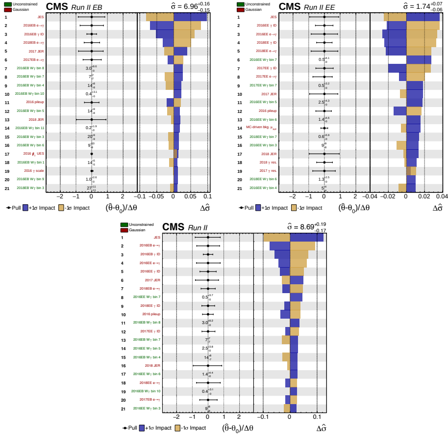
Figure 6.4: Impacts and pulls of the 21 main sources of systematics on the expected cross section measured in EB (top left), EE (top right) and EB+EE (bottom).
