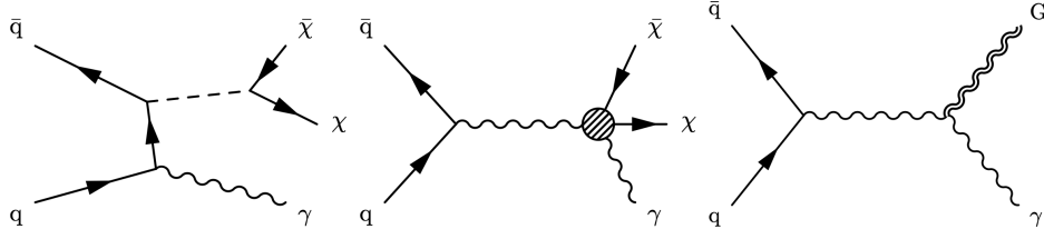
Figure 1.9: Leading-order diagrams of the simplified DM model (left), electroweak-DM effective interaction (center), and graviton (G) production in the ADD model (right), with a monophoton final state [81].
