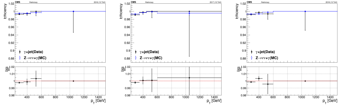
Figure 5.21: Efficiency comparison on \gamma + jets events in data and Z(\rightarrow \nu\bar{\nu})\gamma events in the simulation for 2016 (left) 2017 (center) and 2018 (right).
