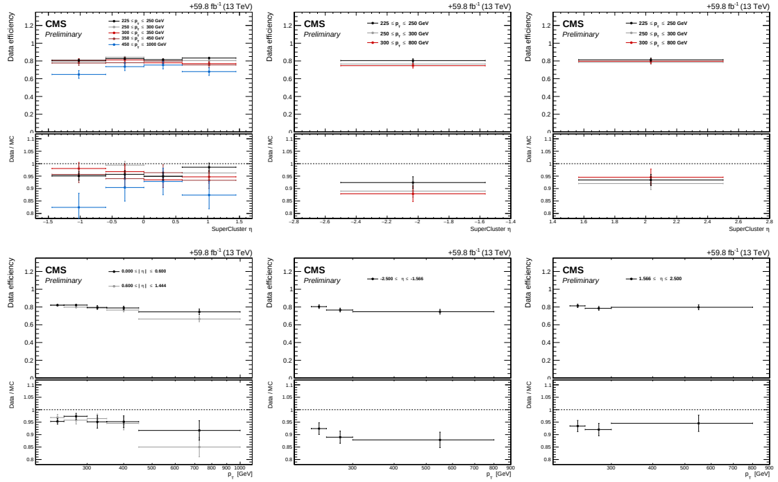
Figure B.8: Photon ID efficiencies in data as a function of \eta (top) and p_T (bottom), for the 2018 year, in EB (left) and EE (center and right). The ratio between the data and the MC efficiencies is also shown in the bottom panel of each plot.
