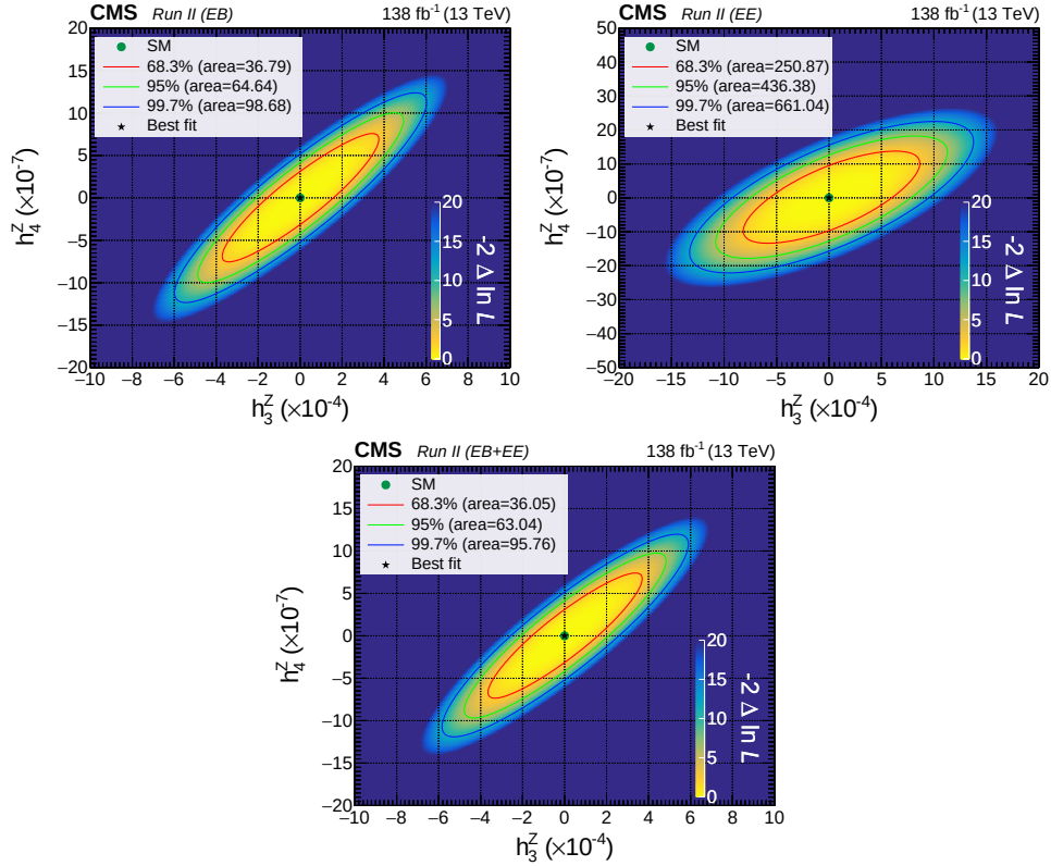
Figure 6.5: 2D likelihood contours in the (h_3^Z, h_4^Z) plane performed for signal events in EB (top left), EE (top right) and for the EB+EE combination (bottom).
