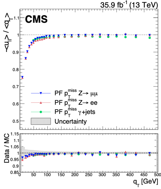
Figure 3.24: The MET response in data, in Z \rightarrow \mu^- \mu^+ (blue), Z \rightarrow e^- e^+ (red), and \gamma + \text{jets} (green) events is shown in the upper panel, while the ratio of the MET response in data and simulation is shown in the lower one. The grey band corresponds to the systematic uncertainties due to the energy scale and resolution of all reconstructed objects entering the MET computations, and it is estimated from the Z \rightarrow e^- e^+ sample [153].
