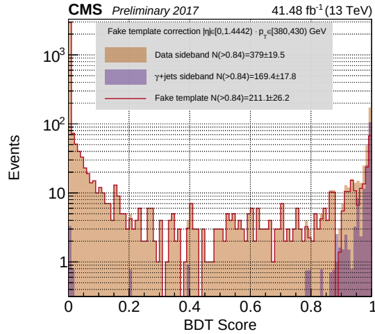
Figure 5.11: The spectrum obtained from the fake sideband A_S (orange) is corrected by subtracting the prompt photon contamination estimated by \gamma + jets MC (violet).
