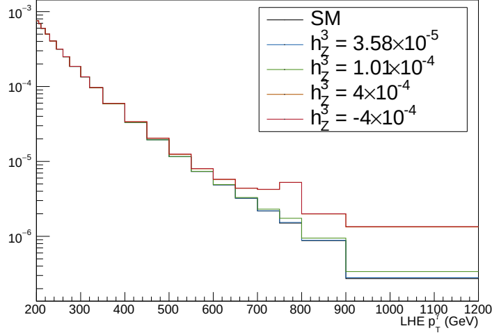
Figure 5.1: Examples of aNTGC excesses over the SM predictions in the photon p_T spectrum.
