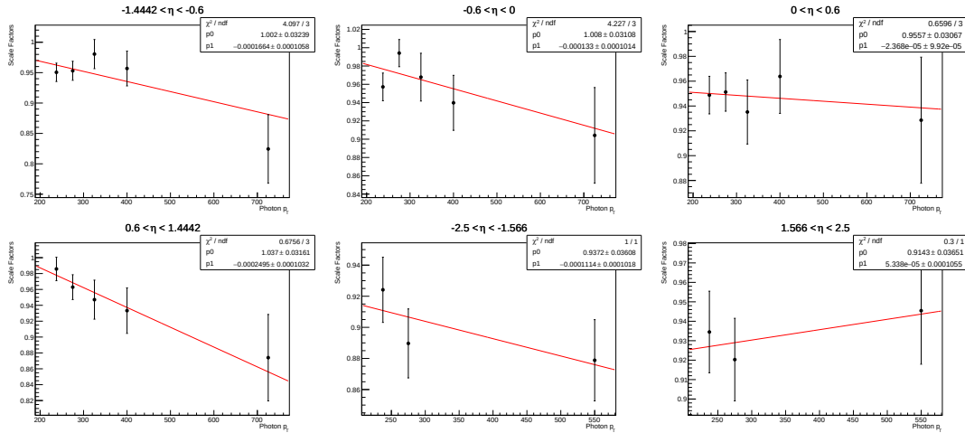
Figure B.11: Fit of the scale factors distribution as a function of p_T for 2018.
