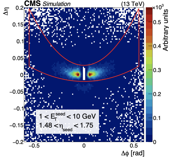
Figure 3.13: Distribution of \Delta\eta = \eta_{seed\ cluster} - \eta_{cluster} versus \Delta\phi = \phi_{seed\ cluster} - \phi_{cluster} for simulated electrons. The energy of the seed cluster is between 1 and 10 GeV and 1.48 < \eta_{seed\ cluster} < 1.75 . The red line contains the clusters selected by the mustache algorithm to form the SC and the white region at the center of the plot represents the seed cluster [142].
