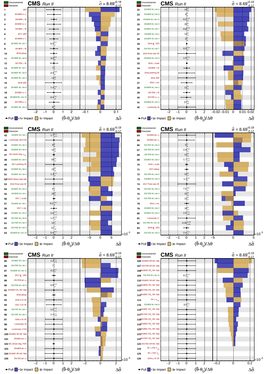
Figure A.3: Impacts and pulls of the systematics on the expected cross section measured combining events in EB and EE.
