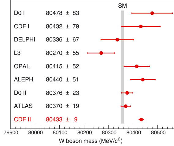
Figure 1.6: Comparison of the CDF II measurement and past m_W measurements with the SM expectation [51].
