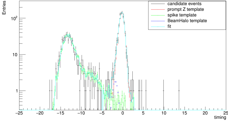
Figure 5.17: Timing fit to candidate events using prompt, spike and beam halo templates for 2017.
