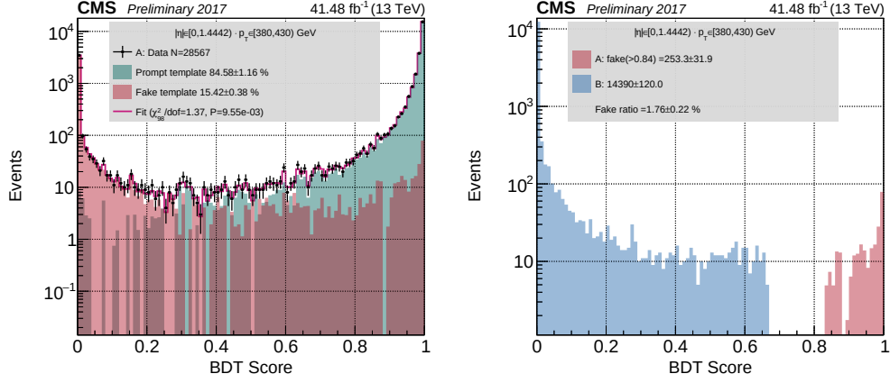
Figure 5.12: (Left) Template to the photon BDT distribution in data for 2017. The prompt template is shown in green, while the fake template in shown in red. (Right) Fake ratio extraction for 2017 EB. The number of events in the region A (red) are estimated selecting those that have the same BDTscore requirement as defined for the photon ID ( BDTscore > 0.8361). The BDTscore selection for the events falling in region B (blue) is instead defined in Tab. 5.13 ( BDTscore < 0.6671).
