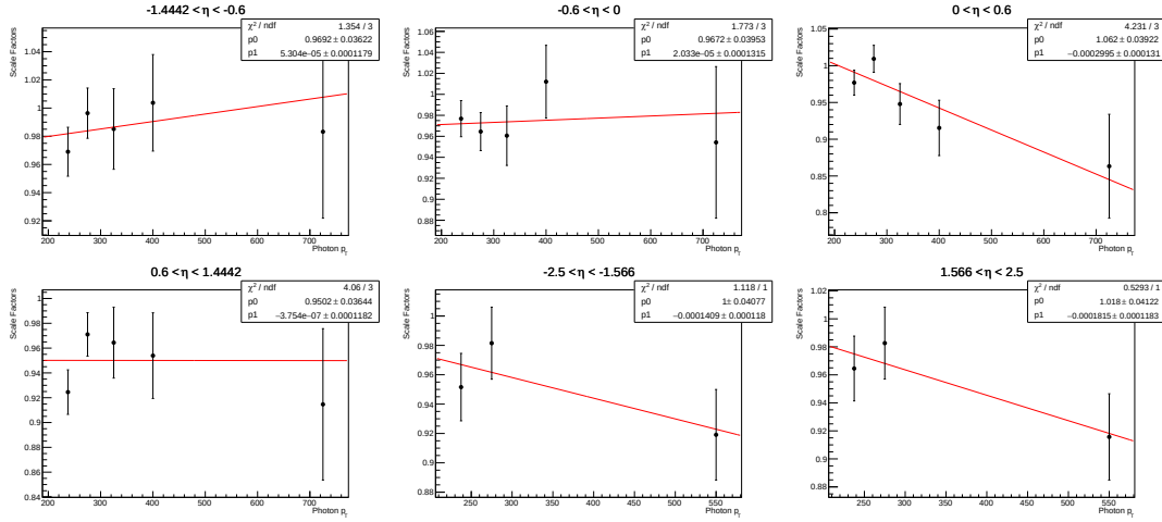
Figure B.10: Fit of the scale factors distribution as a function of p_T for 2017.
