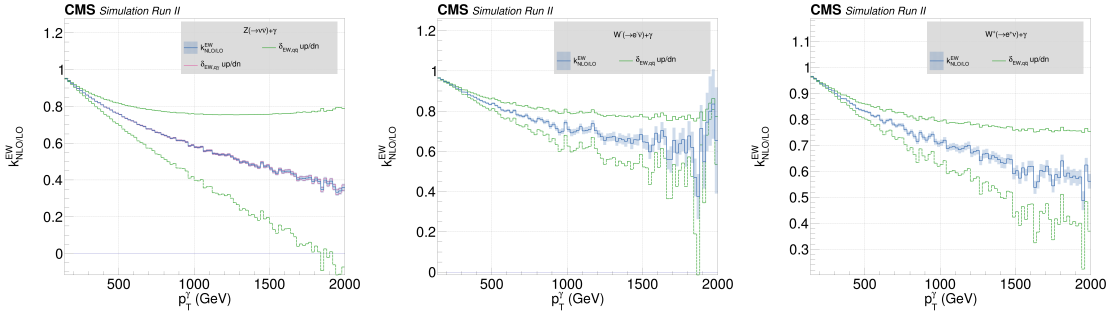
Figure 6.1: Electroweak NLO/LO k-factors as a function of the photon transverse momentum, as they are applied to Z\gamma (left), W^-\gamma (center) and W^+\gamma (right) simulated events.
