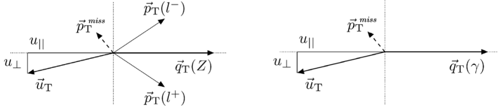
Figure 3.23: Scheme of the Z boson (left) and photon (right) event kinematics in the transverse plane. u_{||} and u_{\perp} are the magnitude of the parallel and perpendicular components of the hadronic recoil \vec{u}_T , respectively. The vectorial missing transverse energy is labeled here as \vec{p}_T^{miss} [154].
