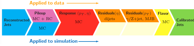
Figure 3.16: Levels of JEC for data and MC simulation, to be applied to jets as reconstructed by the anti- k_T algorithm in order to obtain the final calibrated jets. The corrections marked with MC are derived from simulation studies, RC stands for random cone, and MJB refers to the analysis of multijet events [148].
