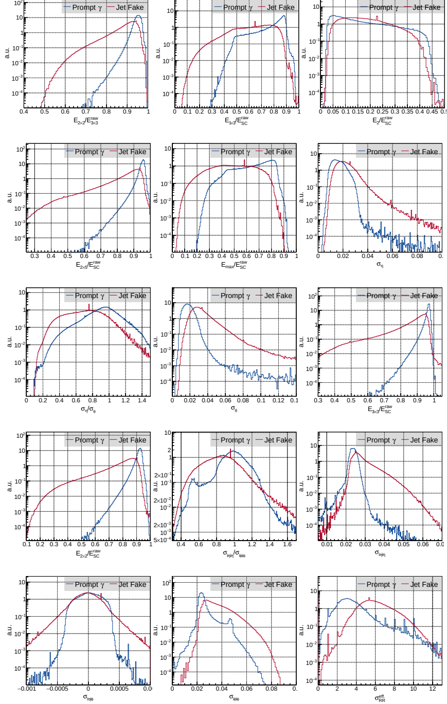
Figure 5.5: The 15 shower shape variables used as input features to the photon BDT in EE. The distributions are obtained using simulated samples.
