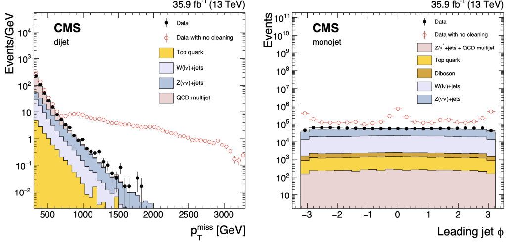
Figure 3.21: The E_T^{miss} (left) and \phi (right) distributions obtained in data for events passing the dijet (left) and monojet (right) selection with (filled dots) and without (open dots) the event filtering algorithms applied, compared with simulation (solid histograms) [153].
