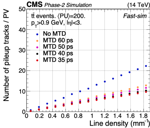
Figure 4.4: Number of pileup tracks incorrectly associated to the primary vertex as a function of the line density, for different time resolutions [169].
