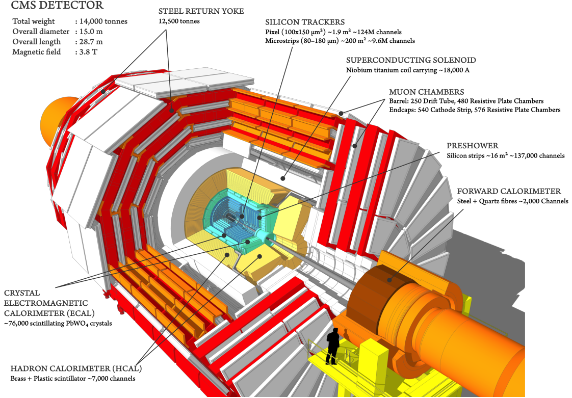
Figure 3.2: The CMS detector and its subsystems. From the innermost to the outermost layer: the silicon tracker, the preshower, the electromagnetic calorimeter, the hadronic calorimeter, the superconducting solenoid and the muon chambers, placed inside the magnet return yoke [108].
