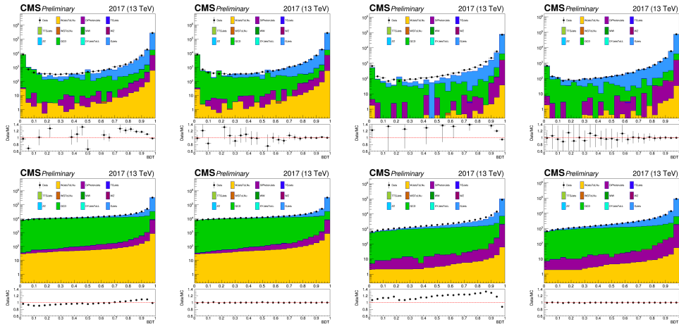
Figure C.2: Data-MC comparison of the BDT score and CDF in \gamma + jets events for 2017, before (left) and after (right) the application of quantile-quantile corrections.
