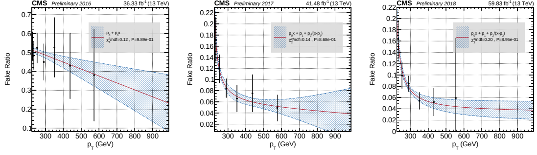
Figure 5.14: Distribution of the \text{jet} \rightarrow \gamma fake ratios as a function of the photon p_T in EE for 2016 (left), 2017 (center) and 2018 (right).
