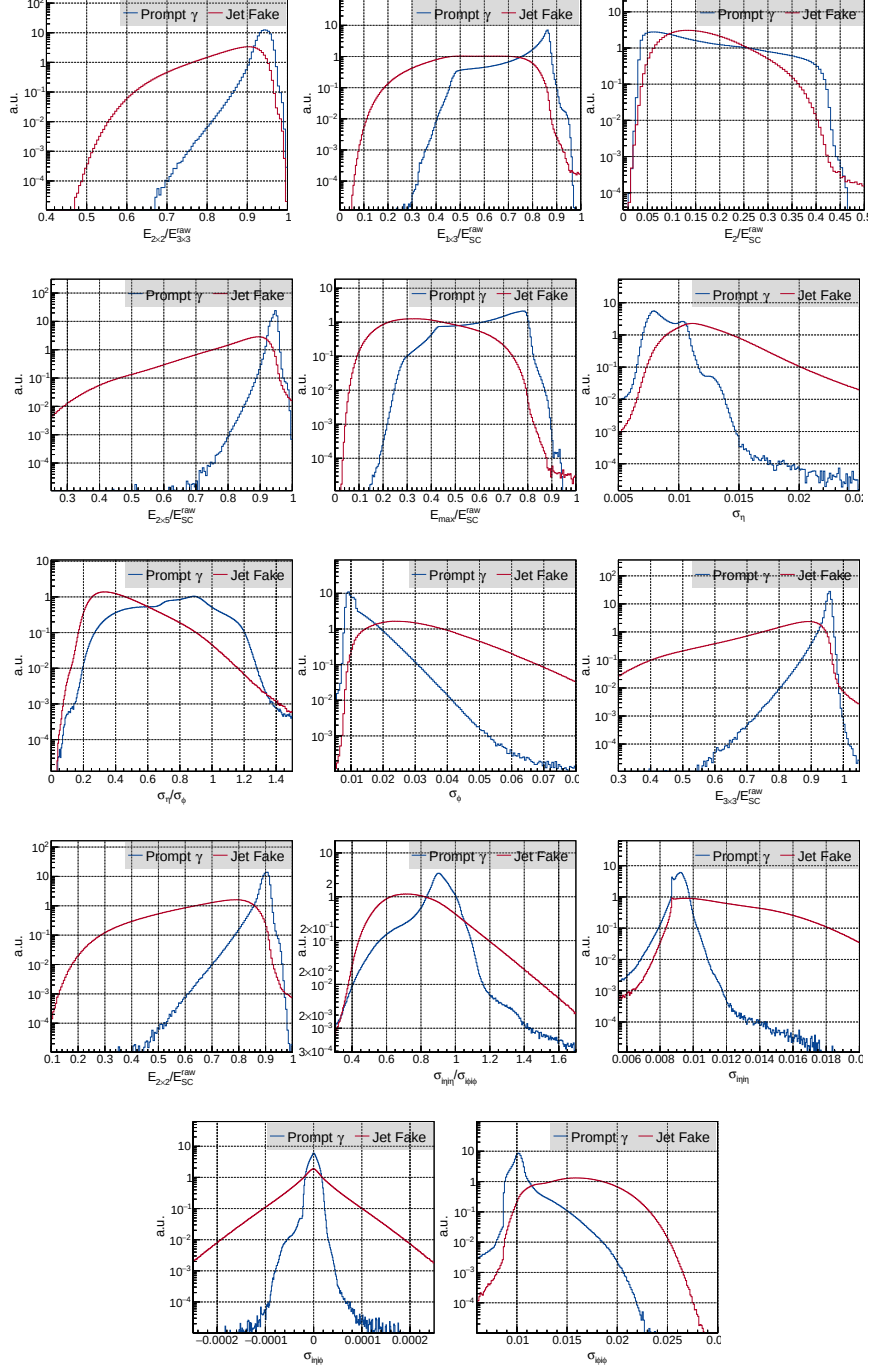
Figure 5.4: The 14 shower shape variables used as input features to the photon BDT in EB. The distributions are obtained using simulated samples.
