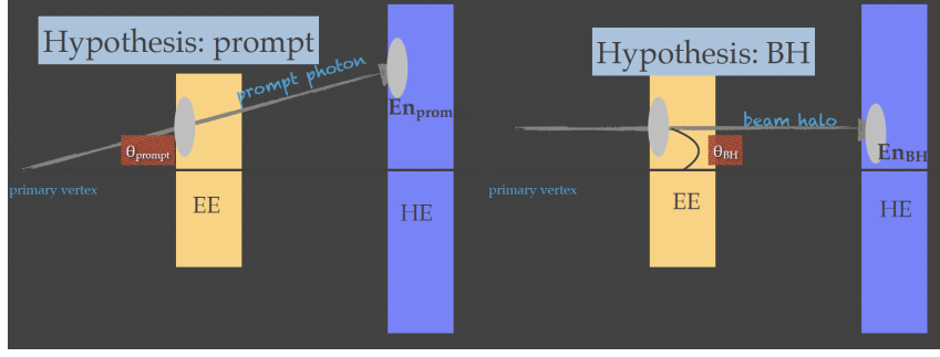
Figure 5.18: PP and BH hypothesis for a photon super-cluster reconstructed in EE.
