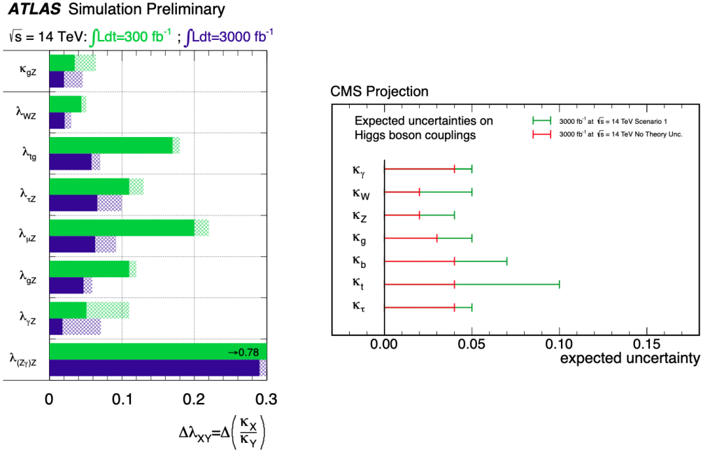
Figure 4.1: Estimated precision of the Higgs boson coupling modifiers with an integrated dataset of 3000 \text{ fb}^{-1} and assuming a center of mass energy of 14 TeV. (Left) ATLAS relative uncertainty on the expected precision for the determination of coupling scale factor ratios \lambda_{XY} . The hashed areas represent the increase of the estimated error due to current theory systematic uncertainties. (Right) CMS projection for the expected uncertainties in the couplings. Scenario 1 assumes the current systematic uncertainties while Scenario 2 considers the experimental uncertainties scaling as 1/\sqrt{L} and reduces the theoretical uncertainties by half [155].
