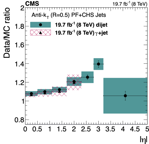
Figure 3.18: Distribution of the scaling factors for the jet p_T resolution as a function of the absolute jet pseudorapidity. The jets are reconstructed with the anti- k_T clustering algorithm (with R=0.5 ) and the CHS method for pileup mitigation. Results determined from \gamma + \text{jets} (hatched boxes) and dijet data (solid boxes) are shown [148].
