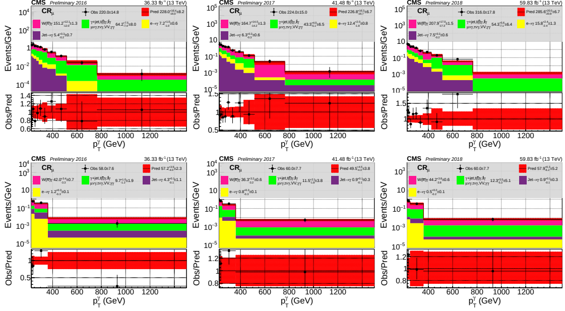
Figure 5.8: Distribution of the photon p_T in the W(\rightarrow \mu\nu)\gamma control region for 2016 (left), 2017 (center) and 2018 (right) for events in EB (top) and EE (bottom).
