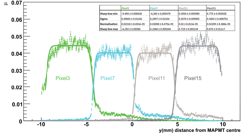
Figure 5.13: Spatial scan of 0.05 mm step of the MAPMT column made by pixel 3,7,11,15. Different colours correspond to the response of different channels: green:pixel 3, cyan:pixel 7, light gray: pixel 11, dark gray: pixel 15.
