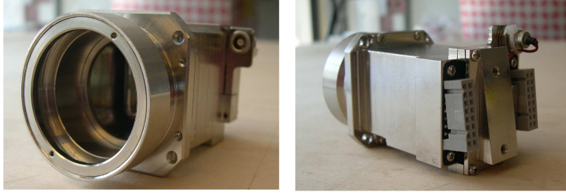
Figure 5.5: Left: frontal view of the magnetic shield, the cylindrical end-cap, working as a lens holder, used to complete the closing of the field line is clearly visible. Right: side back view of the shield case, the bleeder circuit and the analog output connection are housed on the same circuit fixed on the Armco case. The resulting structure is compact and robust.
