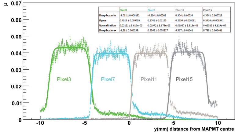
Figure 5.14: Spatial scan of 0.05 mm step of the MAPMT column made by pixel 3,7,11,15 with a magnetic field of 1 mT. Different colours correspond to the response of different channels: green:pixel 3, cyan:pixel 7, light gray: pixel 11, dark gray: pixel 15.
