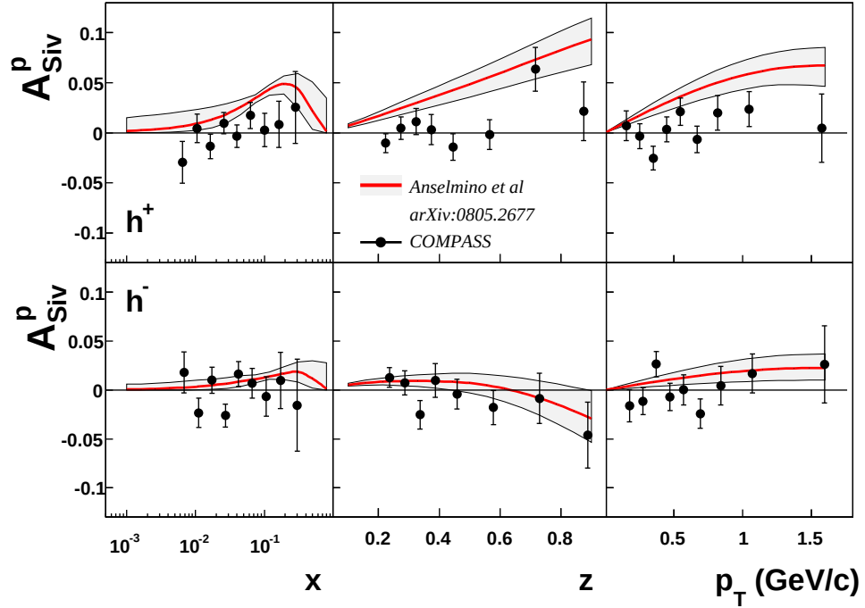
Figure 7.8: COMPASS Siverts asymmetry on proton for positive and negative hadrons, with the latest prediction of Anselmino et al.
