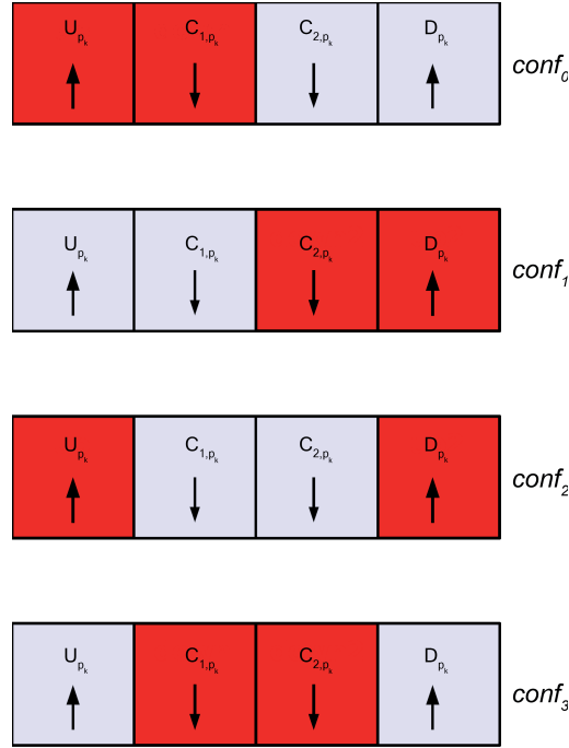
Figure 6.25: Target configurations: the red marked cells are used for the analysis. The configuration names are on the right side, the corresponding cells for the period p_{k+1} have been omitted.
