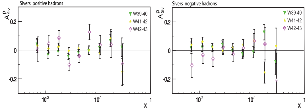
Figure 6.27: False Siverson asymmetries for positive unidentified hadrons (left) and for negative unidentified hadrons (right) as function of x for all the 2007 data taking periods with target \text{conf}_3 .
