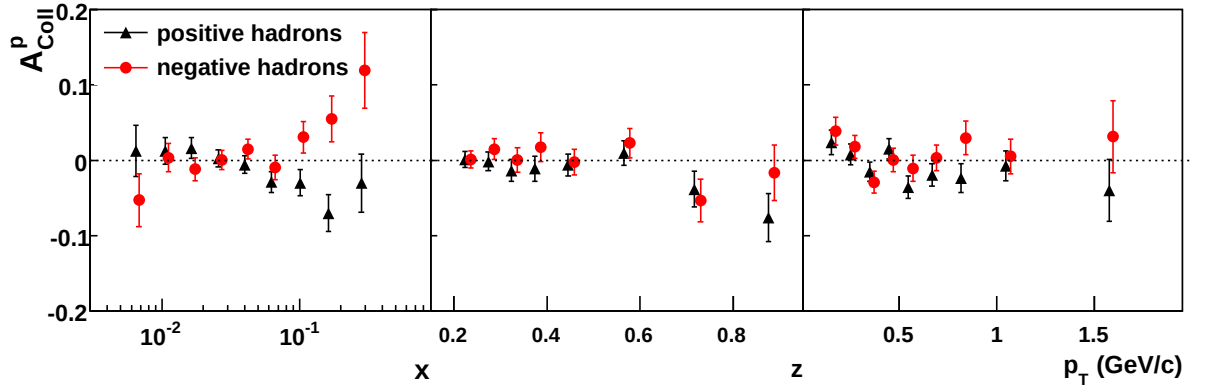
Figure 6.20: Collins asymmetries for positive unidentified hadrons (triangles) and for negative unidentified hadrons (circles) as function of x , P_T^h , and z .
