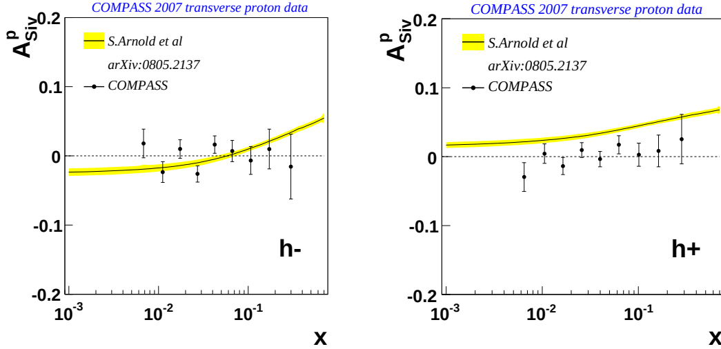
Figure 7.9: COMPASS Sivers asymmetry on proton for positive and negative hadrons, with the prediction of Arnold et al.
