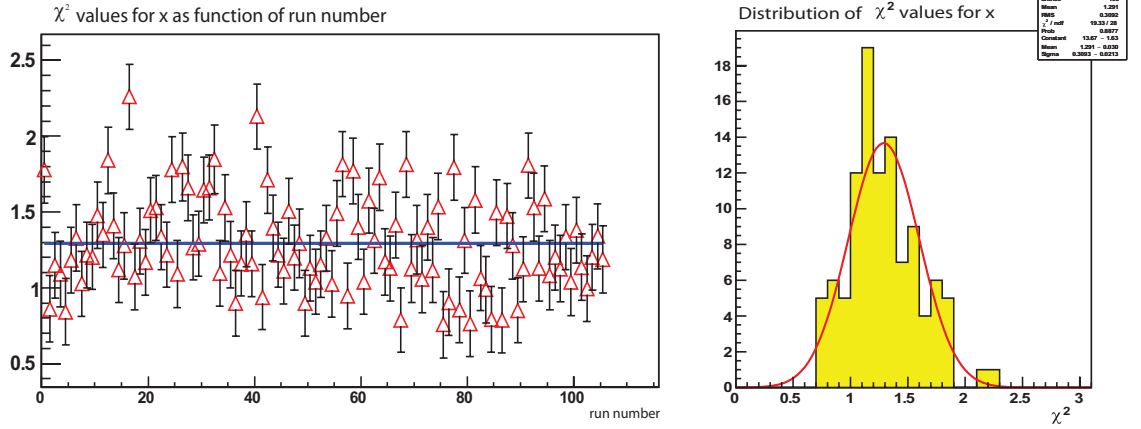
Figure 6.17: Left side: the \chi^2_{Ndf} values from the fit with a constant as a function of the run number for the variable x . Right side: the corresponding \chi^2_{Ndf} distribution with the Gaussian fit superimposed.
