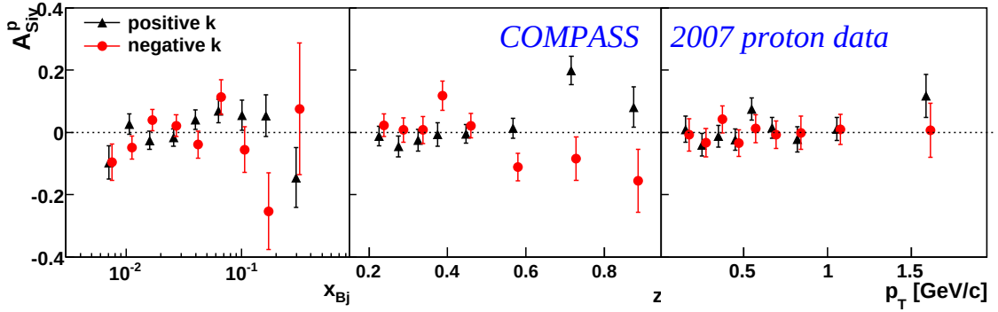
Figure 6.24: Sivers asymmetries for positive kaons (triangles) and for negative kaons (circles) as function of x , P_T^h , and z .
