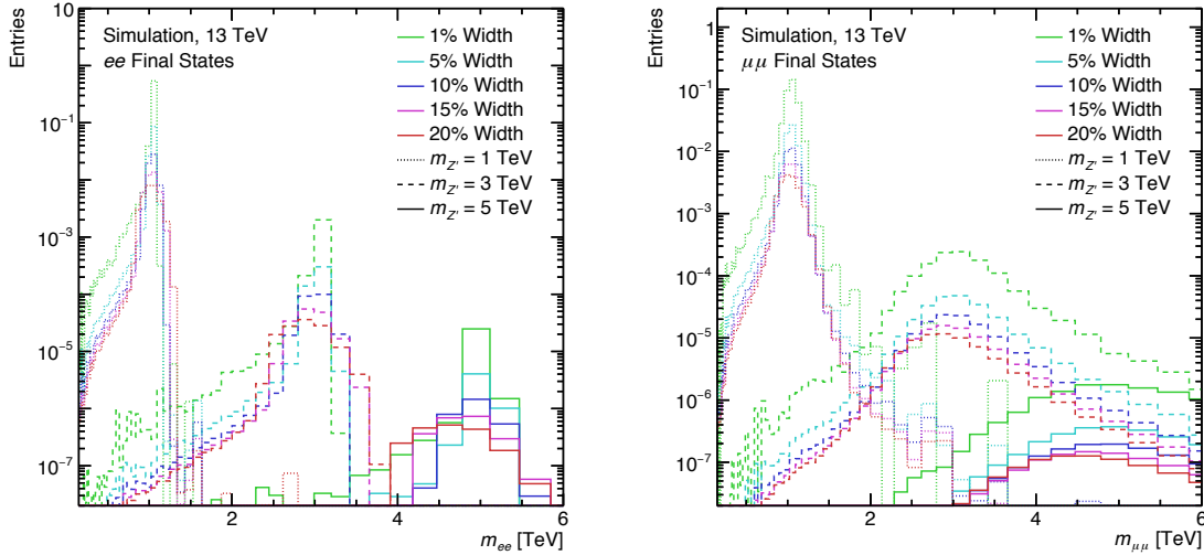
Figure 5.8: Signal templates for Breit-Wigner resonances with different widths at pole masses of 1 TeV, 3 TeV and 5 TeV for dielectron final states (left) and dimuon final states (right).
