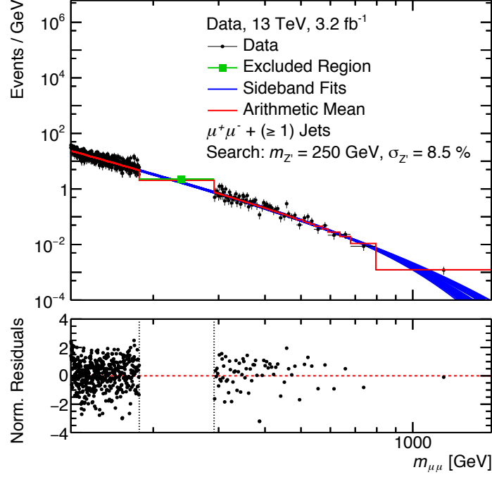
Figure 6.8: Background determination scenario for the spectrum pp \rightarrow \mu^+\mu^- + (\geq 1) \text{ jets} + X at a pole mass m_{Z'} = 250 \text{ GeV} and widths \sigma_{Z'} = 8.5 \% .
