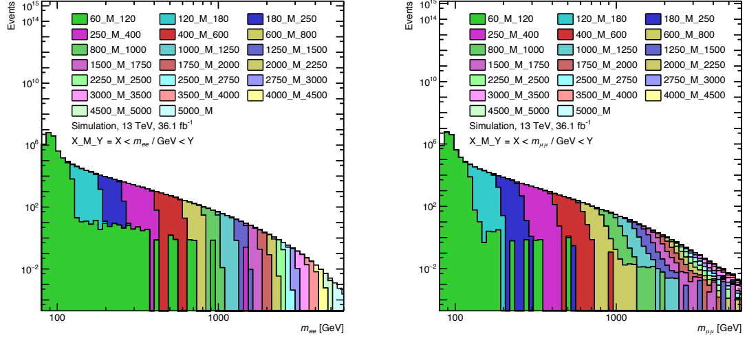
Figure 4.13: Drell-Yan background as a function of the invariant mass of the dielectron final states (left) and the dimuon final states (right).
