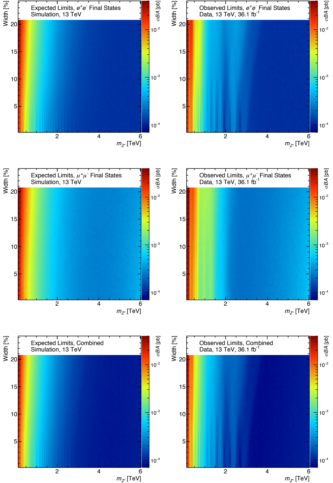
Figure 5.9: Expected and observed model-independent limits on \sigma B\mathcal{A} as a function of the signal pole mass and the signal width for the dielectron case (top), the dimuon case (middle) and the combined case (bottom).
