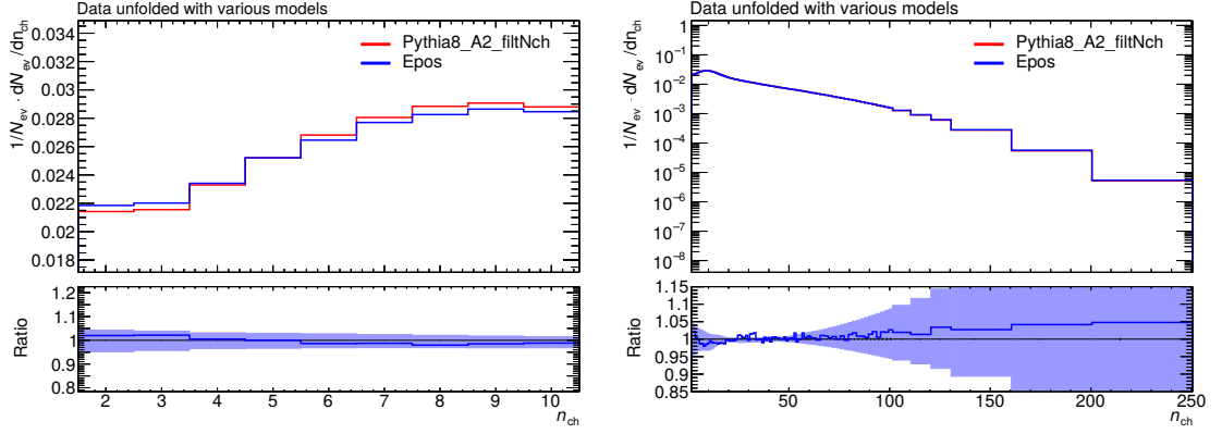
Figure 10.1: Comparison of the unfolded data using the PYTHIA 8 A2 and EPOS generator as input for the matrix calculation. This is shown for the n_{ch} distribution with a zoom in the low region (left) and over the full range (right). The lower panel shows the ratio between the two unfolded distributions with the statistical uncertainty shown in the error band.
