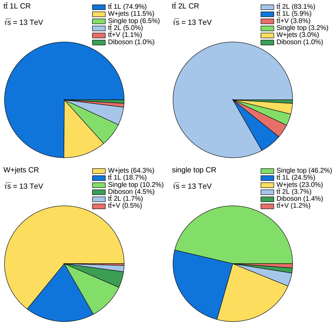
Figure 14.11: Breakdown of the individual SM contributions in the semi-leptonic t\bar{t} (top left), dileptonic t\bar{t} (top right), W+jets (bottom left) and single top (bottom right) control regions.
