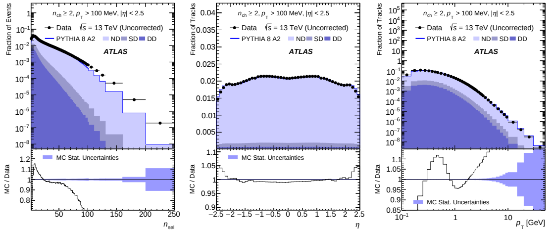
Figure 9.2: Raw distributions of the fraction of events versus the number of selected tracks n_{sel} (left) and of the fraction of tracks versus \eta (middle) and p_T (right). The MC distributions are split into single diffractive (SD), non-diffractive (ND) and double diffractive (DD) events. The lower panel shows the ratio of the MC prediction to data.
