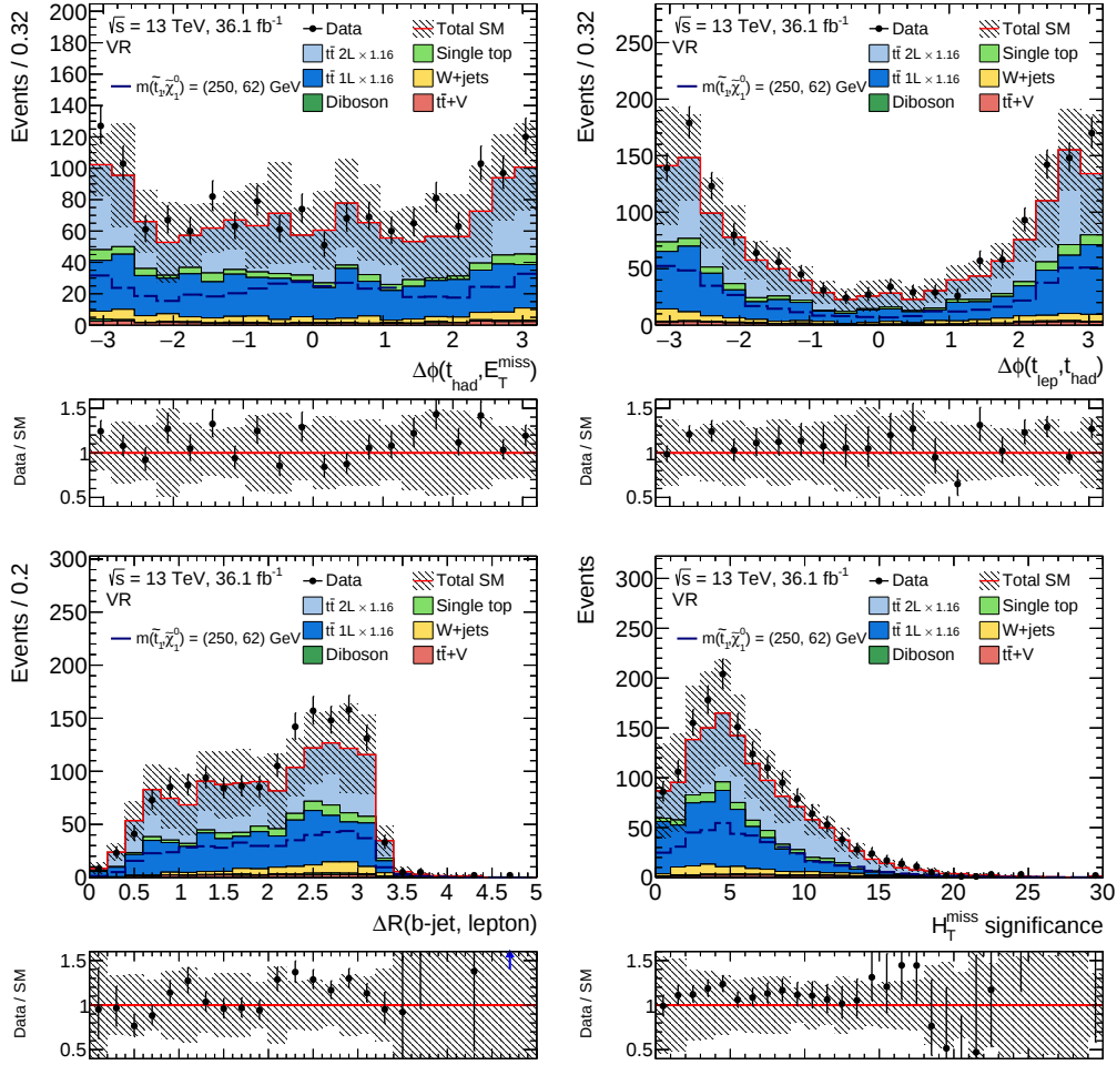
Figure C.25: The \Delta\phi(E_T^{\text{miss}}, t_{\text{had}}) (top left) and \Delta\phi(t_{\text{lep}}, t_{\text{had}}) (top right), \Delta R(b, \ell) (bottom left) and H_{T,\text{sig}}^{\text{miss}} (bottom right) distribution in the BDT VR in the discovery fit setup. Normalisation factors for semi- and dileptonic t\bar{t} are applied. The statistical uncertainty is shown as well as the uncertainties from JES/JER and b -tagging.
