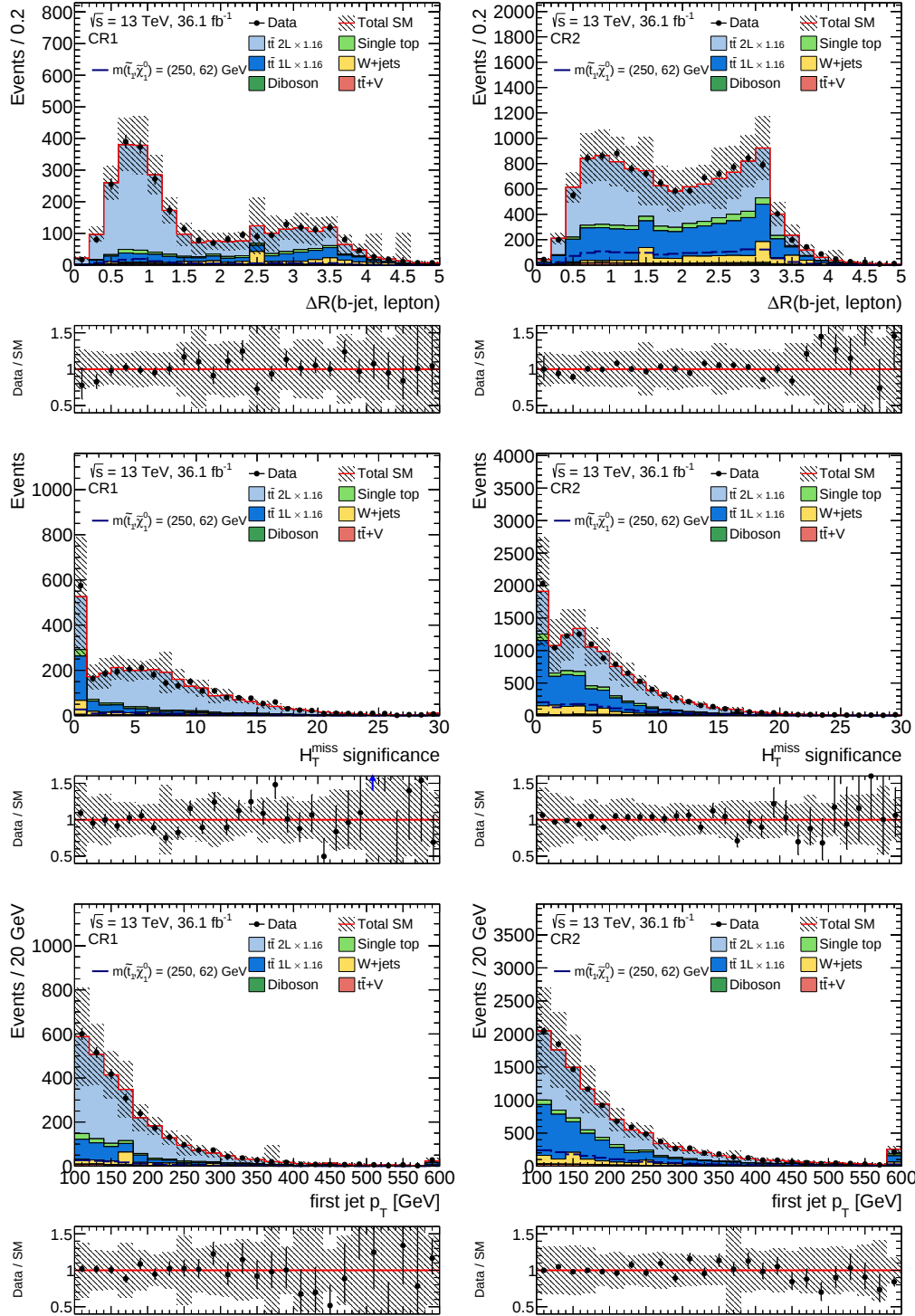
Figure C.33: The \Delta R(b, \ell) (top), H_T^{\text{miss}} (middle) and first jet p_T (bottom) distribution in the CR1 and CR2 region. Normalisation factors for semi- and dileptonic t\bar{t} are applied. The statistical uncertainty is shown as well as the uncertainties from JES/JER and b -tagging.
