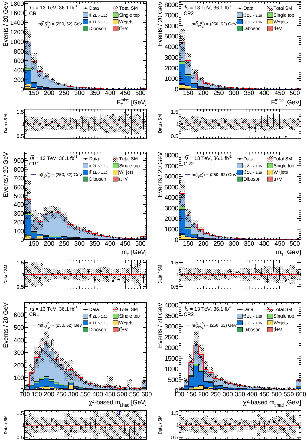
Figure C.31: The E_T^{\text{miss}} (top), m_T (middle) and \chi^2 -based m_{t,\text{had}} (bottom) distribution in the CR1 and CR2 region. Normalisation factors for semi- and dileptonic t\bar{t} are applied. The statistical uncertainty is shown as well as the uncertainties from JES/JER and b -tagging.
