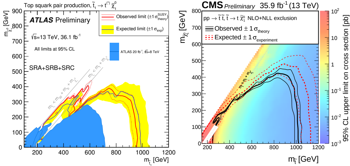
Figure 16.2: Expected and observed 95% excluded regions in the plane of m_{\tilde{t}_1} versus m_{\tilde{\chi}_1^0} for the direct top squark pair production assuming either \tilde{t}_1 \rightarrow t\tilde{\chi}_1^0 or \tilde{t}_1 \rightarrow bW\tilde{\chi}_1^0 decay with a branching ratio of 100%. The excluded area is shown for the full hadronic search from ATLAS [172] (left). Expected (observed) exclusion limits are shown as blue (red) line. Observed limits from previous searches [171] are overlaid for comparison in blue. The excluded area is shown for the one lepton search from CMS [173] (right). Expected (observed) exclusion limits are shown as red (black) lines. For both plots, the uncertainty bands corresponding to the \pm 1 \sigma variation on the expected limit and the sensitivity of the observed limit to \pm 1 \sigma variations of the signal theoretical uncertainties are shown.
