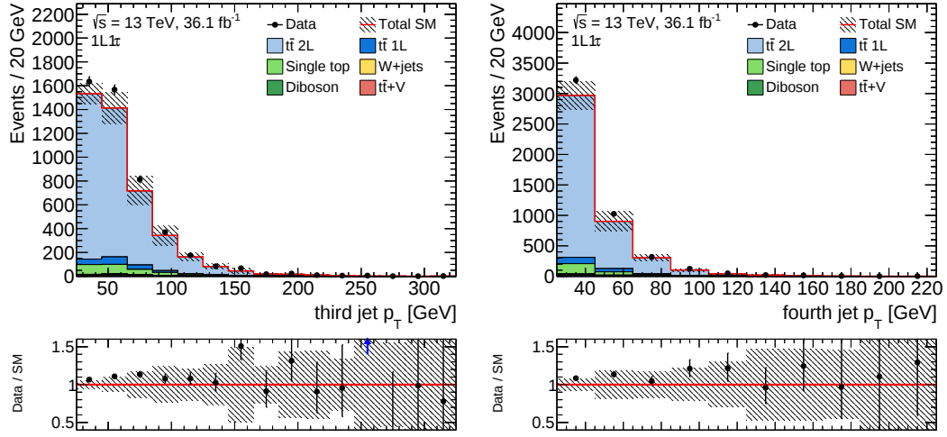
Figure 15.20: Distribution of the p_T of the third and fourth leading jet in the 1L1 \tau selection. The uncertainty band includes only the t\bar{t} theory uncertainties.
