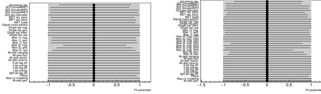
Figure 15.22: Fit parameter for the exclusion fit of the BDT for the benchmark signal using pseudo-data. The nominal setup (left) and a setup using one uncorrelated uncertainty per bin for the fragmentation uncertainty for semi-leptonic t\bar{t} (right). The black dots show the best fit value and uncertainty of the nuisance parameters, encoding the various experimental and theoretical modelling uncertainties.
