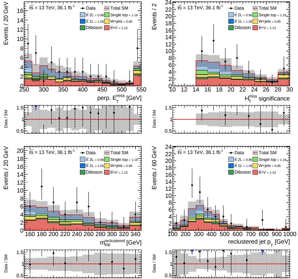
Figure C.16: Comparison of data and simulation for the signal region after applying the normalisation of the simultaneous fit. Statistical uncertainties as well as the systematic uncertainties from JES, JER and b -tagging are displayed. The last bin includes the overflow.
