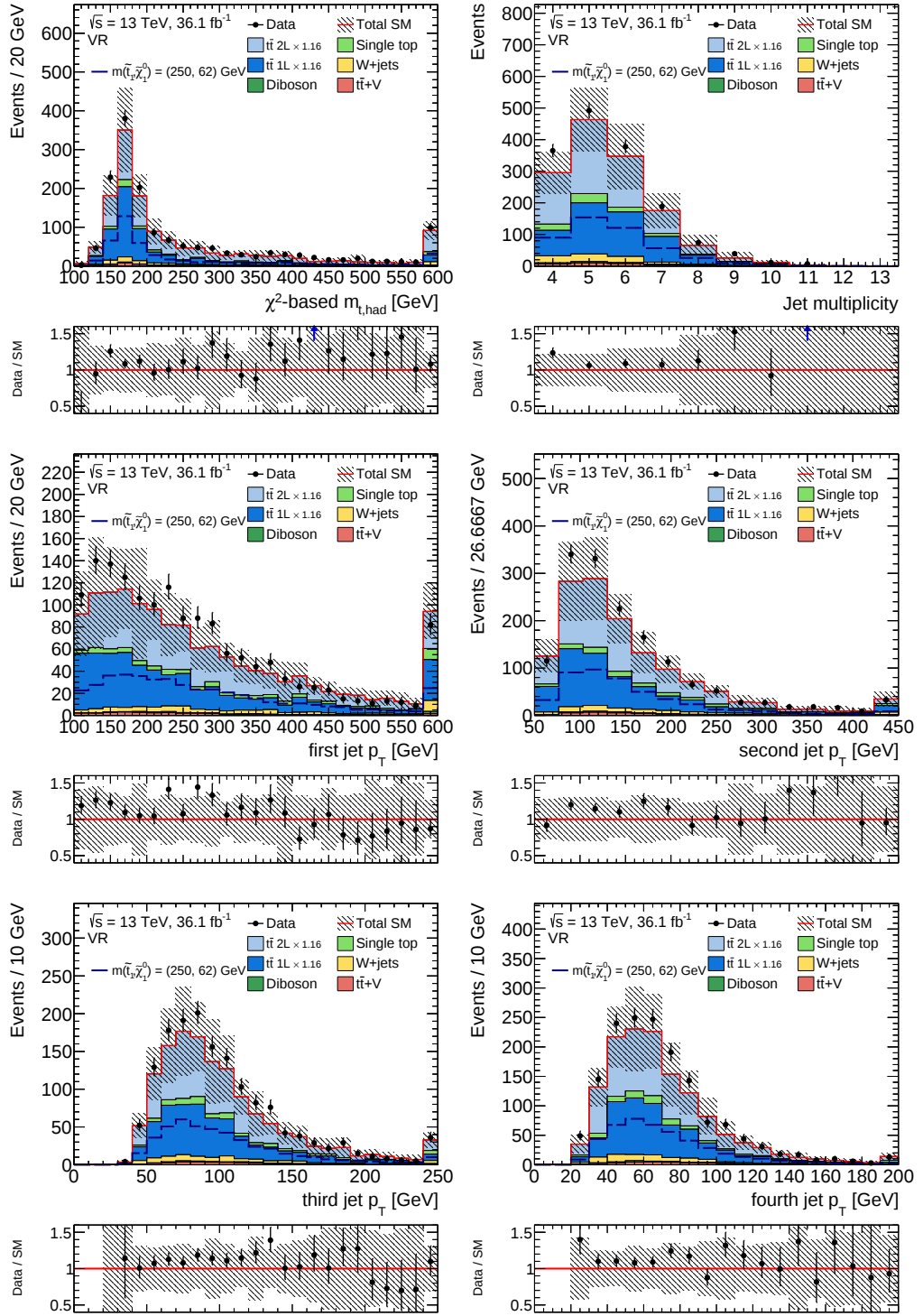
Figure C.26: The \chi^2 -based m_{t, \text{had}} (top left) and number of jet (top right), and the first (middle left), second (middle right), third (bottom left) and fourth (bottom right) jet p_T distribution in the BDT VR in the discovery fit setup. Normalisation factors for semi- and dileptonic t\bar{t} are applied. The statistical uncertainty is shown as well as the uncertainties from JES/JER and b -tagging.
