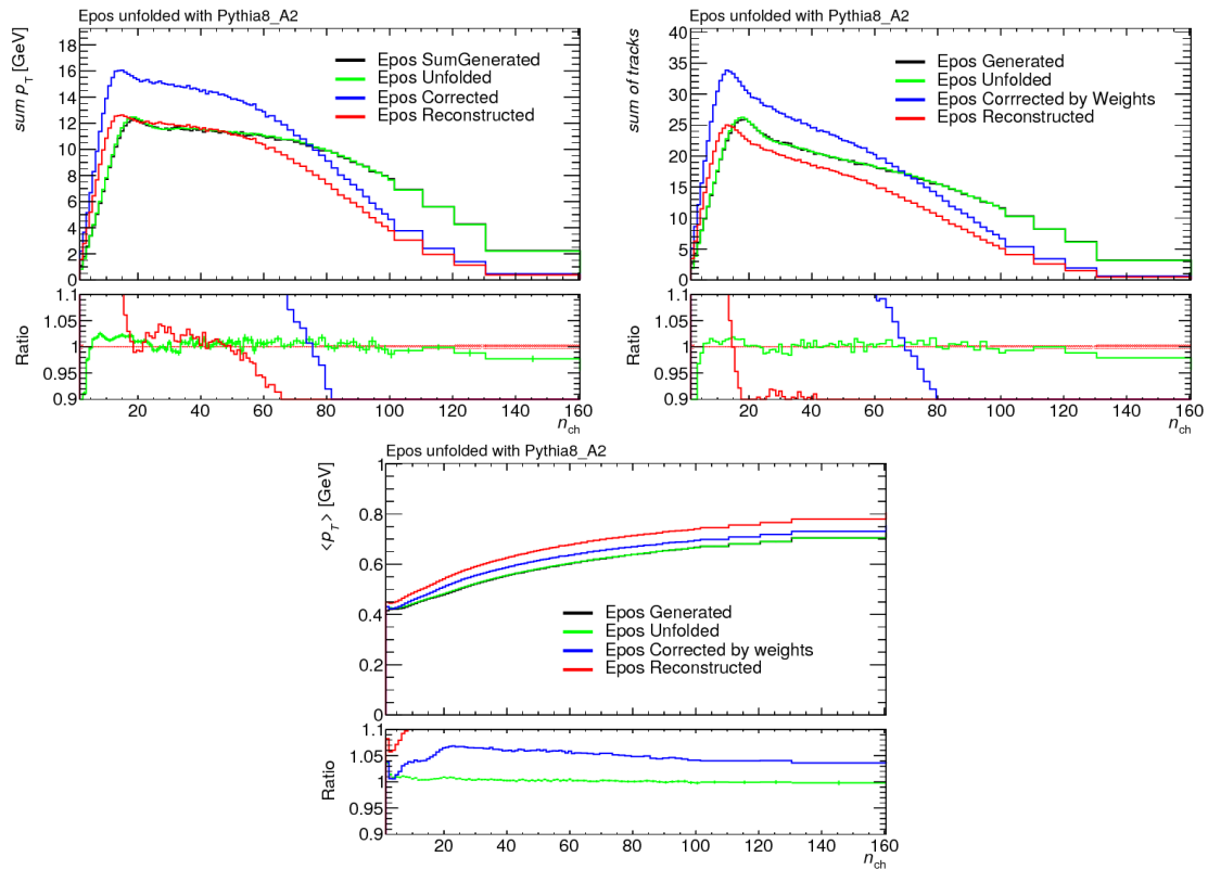
Figure B.5: Closure test for \sum_{\text{tracks}} p_T versus n_{ch} and \sum_{\text{tracks}} 1 versus n_{ch} as well as for \langle p_T \rangle(n_{ch}) using EPOS as input distribution and PYTHIA 8 A2 for constructing the unfolding matrix.
