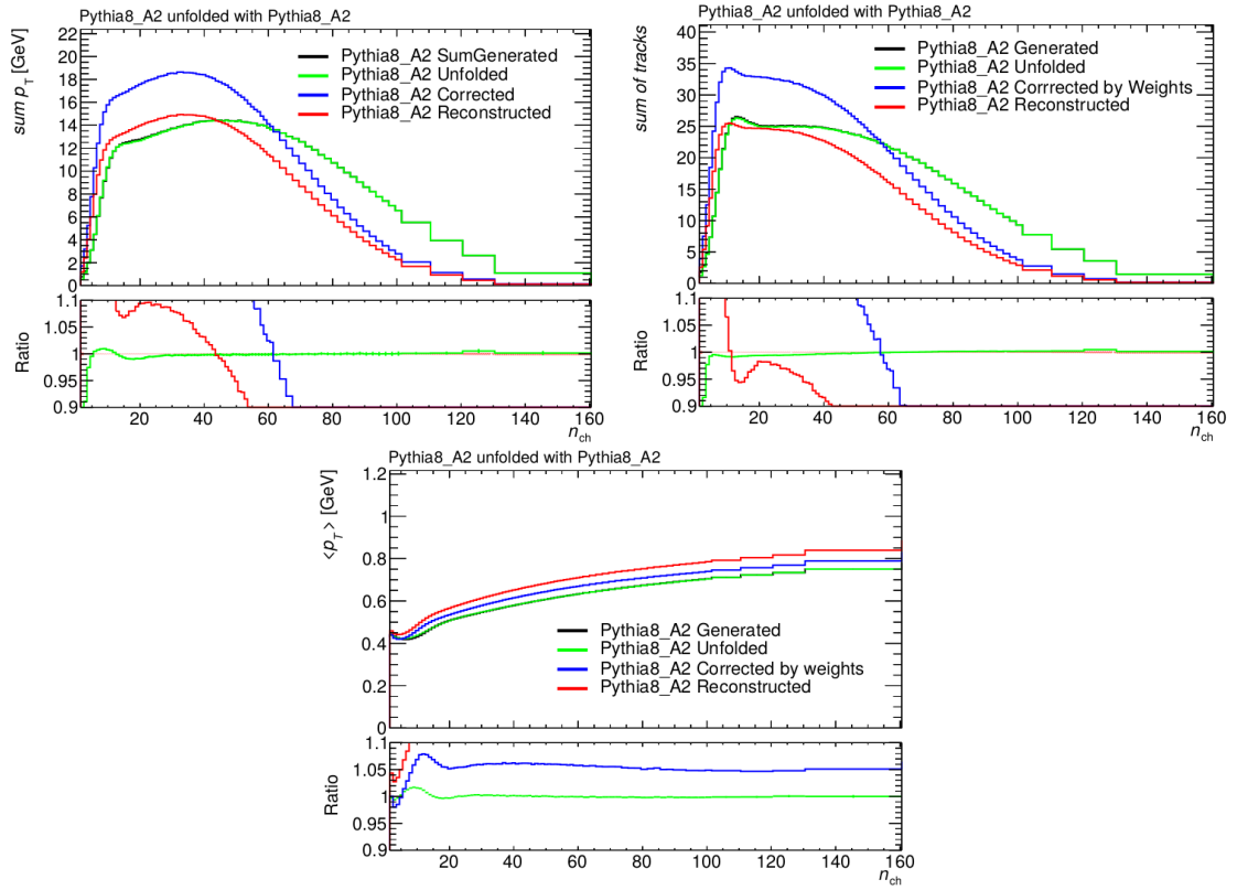
Figure 10.6: Closure test for \sum_{\text{tracks}} p_T versus n_{ch} (left top) and \sum_{\text{tracks}} 1 versus n_{ch} (right top) as well as for \langle p_T \rangle versus n_{ch} (bottom) using the PYTHIA 8 A2 generator for the input distribution and the resolution matrix. The bottom panel shows the ratio to the generated level.
