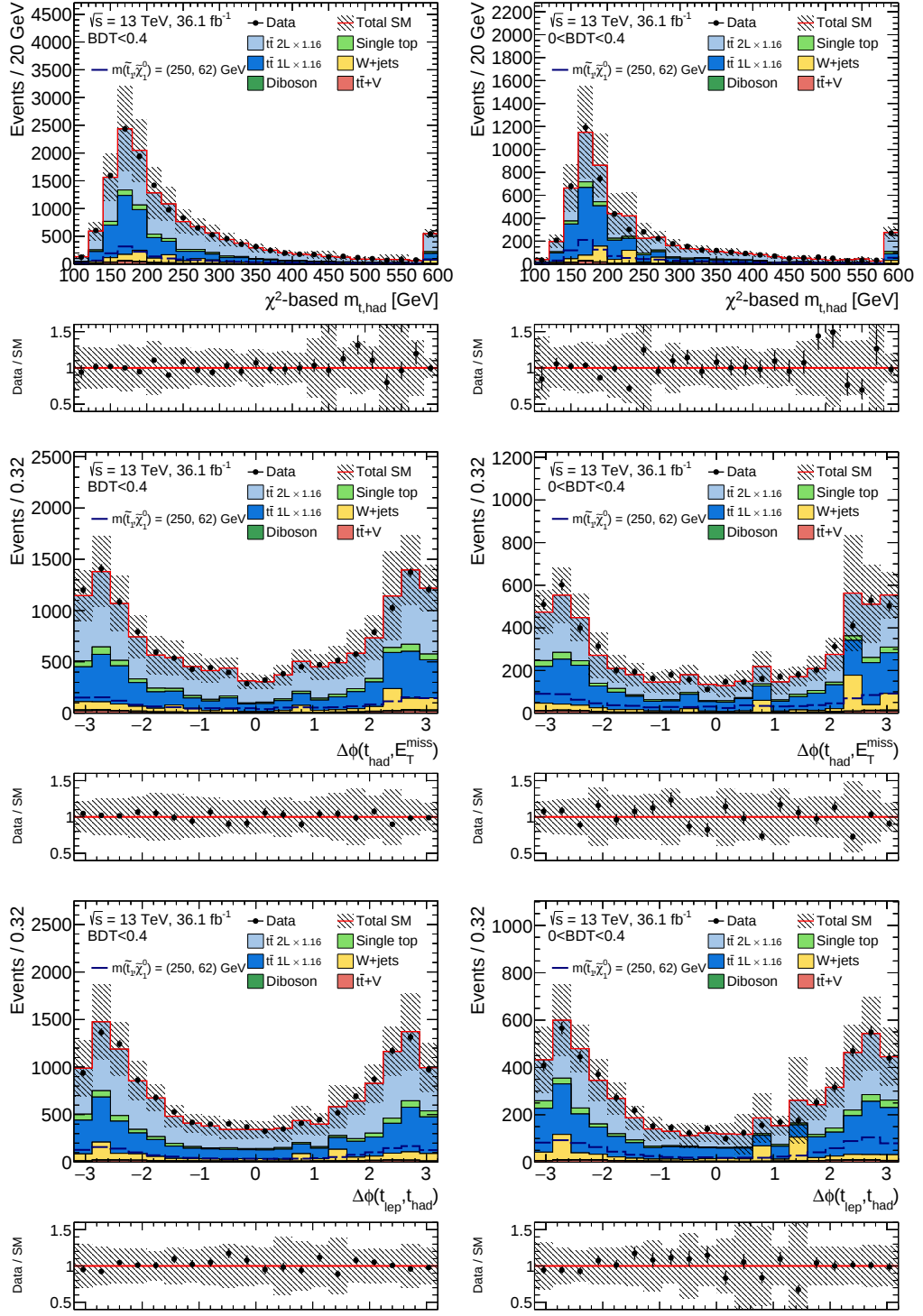
Figure C.28: The \chi^2 -based m_{t, \text{had}} (top), \Delta\phi(E_T^{\text{miss}}, t_{\text{had}}) (middle), and \Delta\phi(t_{\text{lep}}, t_{\text{had}}) (bottom) distribution in a BDT range of -1 to 0.4 (left) and 0 to 0.4 (right). Normalisation factors for semi- and dileptonic t\bar{t} are applied. The statistical uncertainty is shown as well as the uncertainties from JES/JER and b -tagging.
