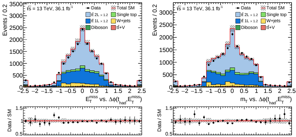
Figure C.46: The correlation of E_T^{\text{miss}} (left) and m_T (right) versus the \Delta\phi(E_T^{\text{miss}}, t_{\text{had}}) . The normalisation factors for t\bar{t} is applied, only statistical uncertainties are shown
