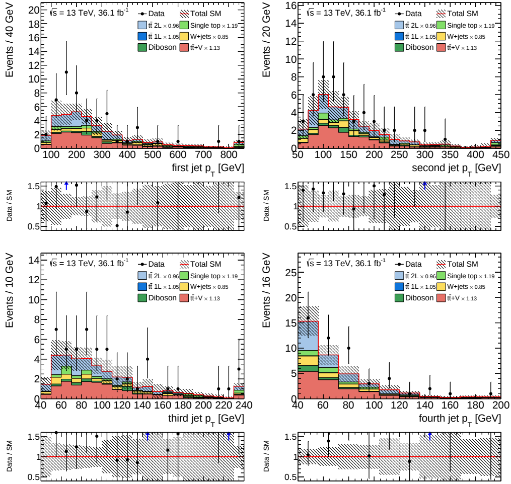
Figure C.17: Comparison of data and simulation for the signal region after applying the normalisation of the simultaneous fit. Statistical uncertainties as well as the systematic uncertainties from JES, JER and b -tagging are displayed. The last bin includes the overflow.
