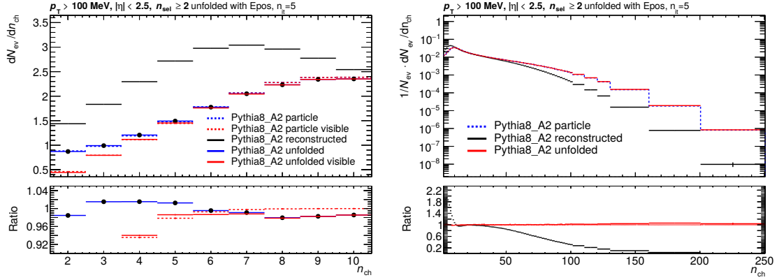
Figure B.1: Closure test using PYTHIA 8 A2 as the input distribution and EPOS generator to construct the unfolding matrix. The label "visible" is used for the subset of events with n_{\text{sel}} \geq 2 that do not migrate outside of the detector phase-space.
