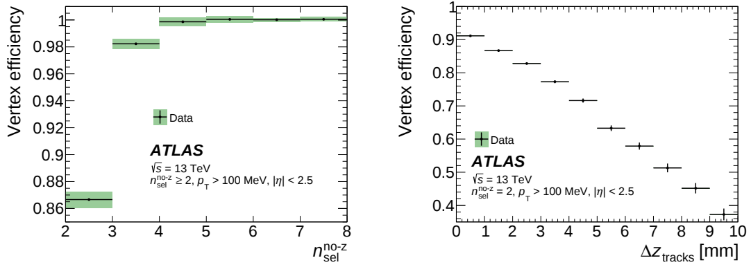
Figure 9.5: The vertex reconstruction efficiency \epsilon_{\text{vtx}} as a function of the number of selected tracks with p_T > 100 MeV and |\eta| < 2.5 without the cut on the longitudinal parameter applied, n_{\text{sel}}^{\text{no-z}} (left). For events with exactly two tracks, the vertex efficiency is considered as a function of the difference in longitudinal impact parameters between these two tracks \Delta z_{\text{tracks}} (right). The statistical uncertainties are shown as black vertical bars, the quadratic sum of statistical and systematic uncertainties as green shaded areas [4].
