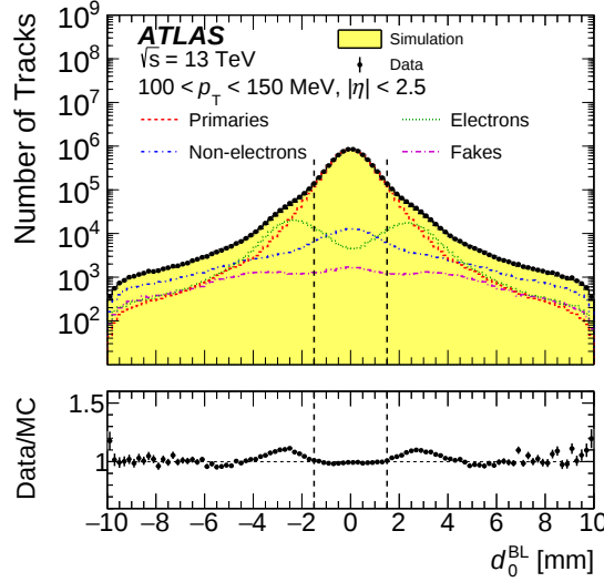
Figure 9.3: Comparison between data and PYTHIA 8 A2 simulation for the transverse impact parameter d_0^{\text{BL}} distribution. The d_0^{\text{BL}} distribution is shown for 100 < p_T < 150 MeV without applying the cut on the transverse impact parameter. The position where the cut is applied is shown as dashed black lines at \pm 1.5 mm. The simulated d_0^{\text{BL}} distribution is normalised to the number of tracks in data and the separate contributions from primary, fake, electron and non-electron tracks are shown as lines using various combinations of dots and dashes. The secondary particles are scaled by the fitted fractions as described in the text. The error bars on the points are the statistical uncertainties of the data. The lower panel shows the ratio of data to the MC prediction [4].
