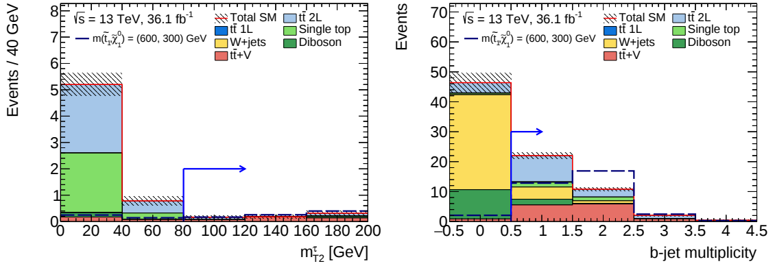
Figure 14.8: Distribution of the m_{T2}^\tau and the b -jet multiplicity after applying all tN_{med} cuts, except the one on the displayed distribution. The background processes are added together and the signal benchmark is overlaid. The cut position and direction is shown as blue line.
