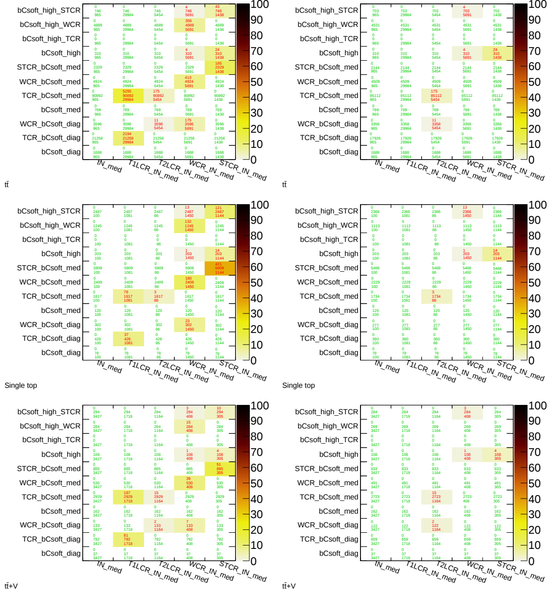
Figure C.18: Number of simulated events selected by any region of the three soft lepton selection and the t\bar{N}_{med} selection for t\bar{t} (top), single top (middle) and t\bar{t} + V (bottom). The left-hand side shows the overlap using the standard selection, the right-hand side shows the remaining overlap after the t\bar{N}_{med} control region veto applied for the soft lepton control regions. The numbers in each bin give the number of overlapping events and the number of events selected by the region indicated on the vertical axis and the horizontal axis from top to bottom. The colour scale indicates the fraction of overlapping events in a bin.
