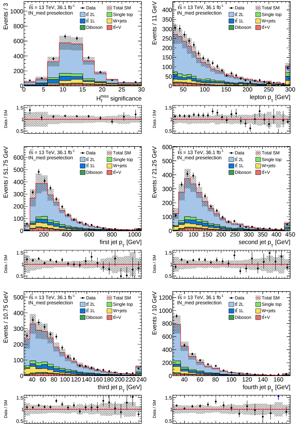
Figure C.2: Comparison of data and simulation applying only the preselection used for the tN_{\text{med}} signal region optimisation. Statistical uncertainties as well as the systematic uncertainties from JES, JER and b -tagging are displayed. The last bin includes the overflow.
