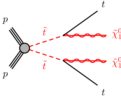
Figure 12.1: The diagram illustrates the top squark decay into a top quark and the lightest neutralino. The sparticles are shown as red lines. The direct top squark production begins with a squark-anti-squark pair, but for simplicity, no charge-conjugate symbols are shown [5].
