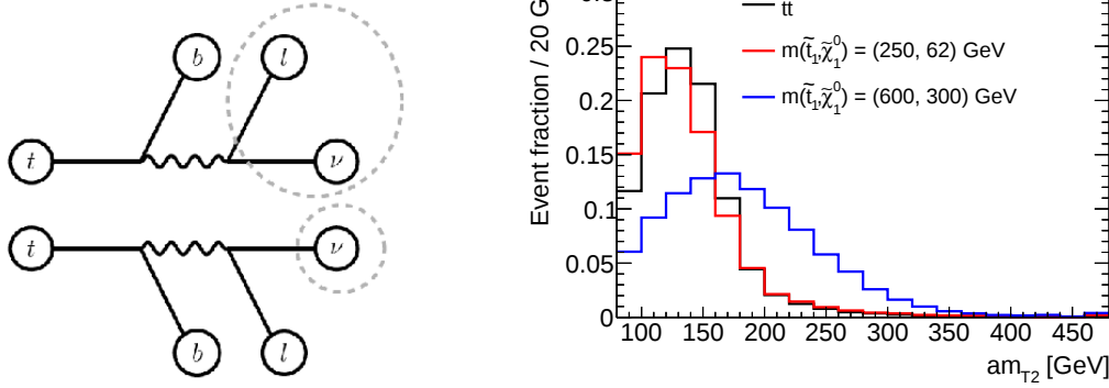
Figure 13.6: Illustration of the am_{T2} reconstruction (left) and the resulting distribution (right) for the leading background process t\bar{t} and a benchmark signal for the diagonal and the tN_med signal region after applying all preselection requirements. The distribution is normalised to unit area in order to show the shape differences.
