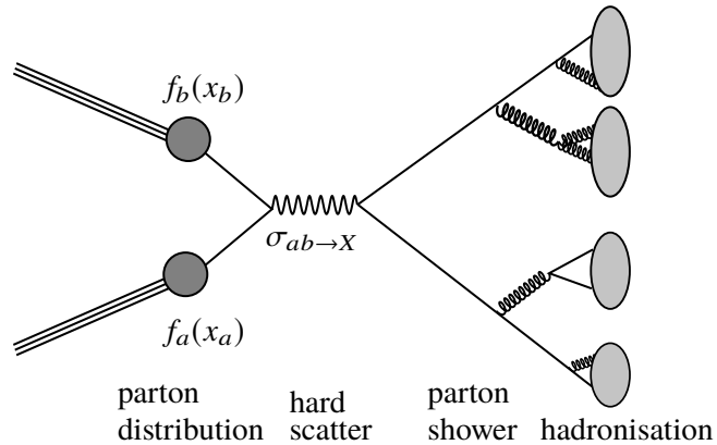
Figure 3.1: Sketch of a pp collision illustrating the different steps of the event simulation.
