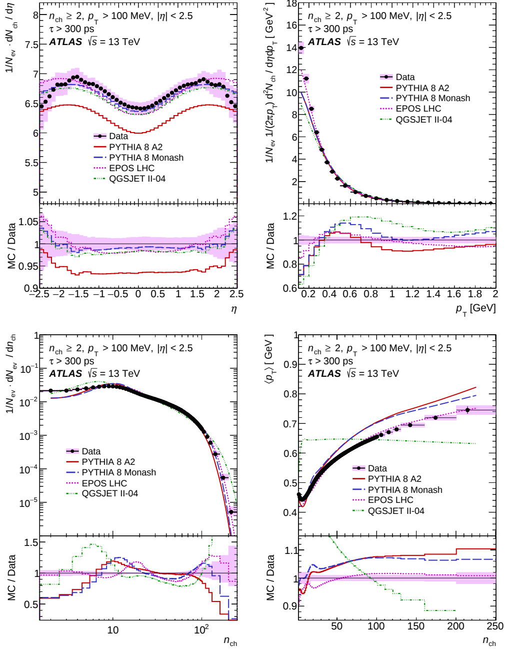
Figure 11.1: Primary charged-particle multiplicities as a function of pseudorapidity \eta (top left) and transverse momentum p_T (top right), the primary charged-particle multiplicity n_{ch} (bottom left) and the mean transverse momentum \langle p_T \rangle (bottom right). The black dots represent the data and the coloured curves the different MC predictions. The vertical bars represent the statistical uncertainty, while the shaded areas show statistical and systematic uncertainties added in quadrature. The lower panel in each figure shows the ratio of the MC prediction to data.
