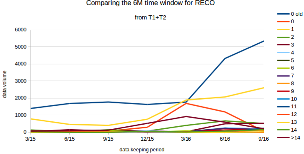
Figure 3.10: Comparison through data keeping periods between bins with different number of accesses.
