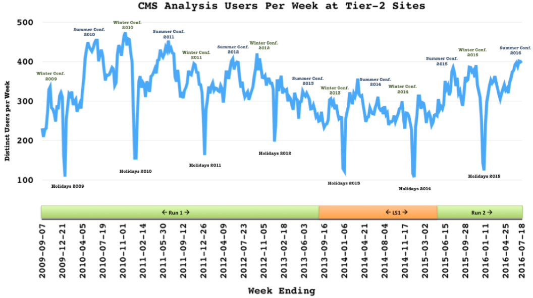
Figure 3.15: Individual CMS analysis submitters per week to the Grid from September 2009 to July 2016. [source: CMS Dashboard] [48]
