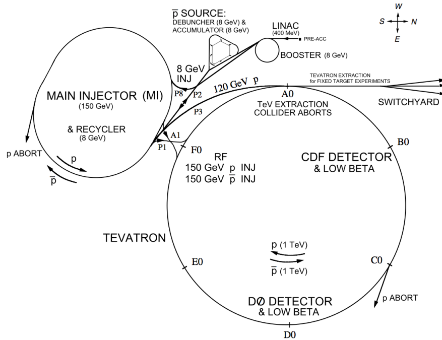
Figure 6.1: The Tevatron Collider chain at FERMILAB.
