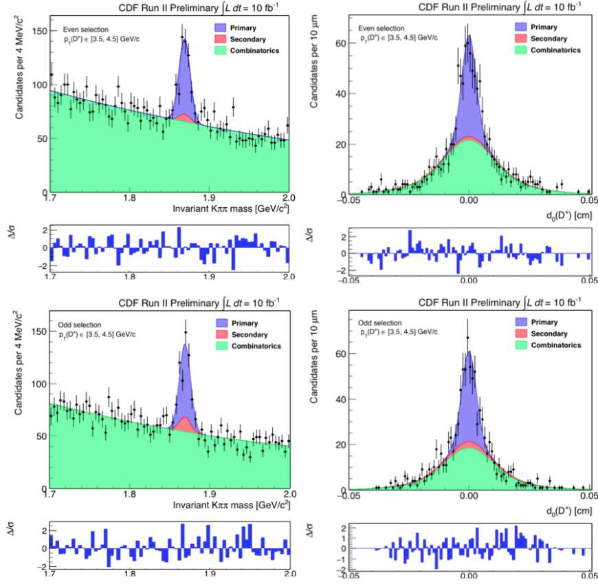
Figure 6.23: Distributions of the K^-\pi^+\pi^+ -invariant mass (left) and impact parameter (right) with fit projections overlaid for the even subsample (top) and odd subsamples (bottom) of events restricted to the p_T(D^+) range 3.5 – 4.5 GeV.
