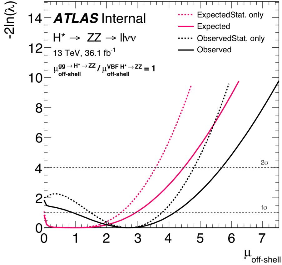
Figure 5.3: Scan of the negative log-likelihood, -2\ln(\lambda) , as function of \mu_{\text{off-shell}} for the \ell\ell\nu\nu channel in both data (black) and simulation (red) with NLO QCD m^{ZZ} dependent K -factors applied to each individual gg \rightarrow ZZ process and an additional NNLO/NLO QCD K -factor of 1.2, as described in Sec. 4.3.1. The cross point of the 2\sigma line with the likelihood scan curve gives the 95% CL upper limit on \mu_{\text{off-shell}} . The dotted line shows the scan when only the statistical uncertainty is considered, while the solid line shows the impact of the systematic uncertainties on the result. The ratio of the ggF and VBF processes is assumed to have the SM value.
