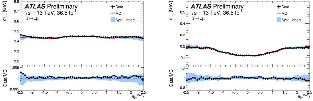
Figure 3.5: Fitted Y(1S) mean mass (left) and dimuon invariant mass resolution (right) of the dimuon system for CB muons from Y \rightarrow \mu\mu decays collected in 2015-2016 and for the corrected simulation as a function of the pseudorapidity of the highest- p_T muon. The upper panel shows the fitted mean mass value (left) and the fitted dimuon invariant mass resolution (right) for data (black) and corrected simulation (red). The lower panel shows the data/MC ratio. The error bars represent the statistical uncertainty; the blue shaded bands represent the systematic uncertainty in the correction and the systematic uncertainty in the extraction method added in quadrature.
