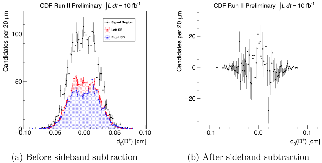
Figure 6.13: Impact-parameter distribution of candidates in the signal region before (a) and after (b) sideband subtraction for p_T(D^+) in 1.5 – 2.5 GeV.
