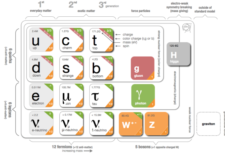
Figure 1.1: Elementary particles in the SM. Figure from [12].
