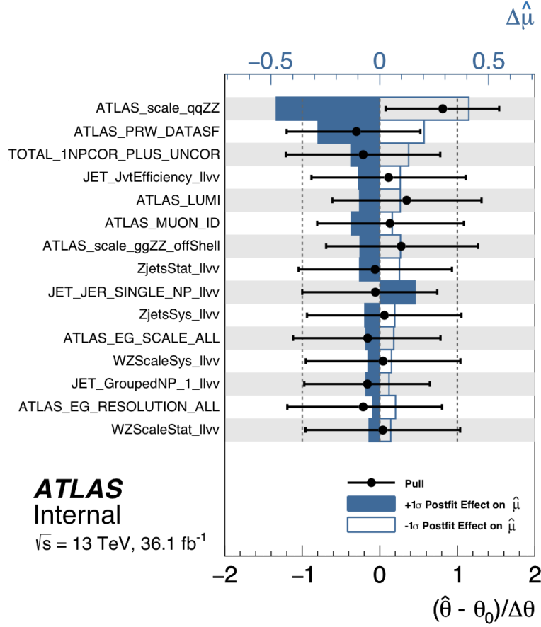
Figure 5.8: Impact of systematic uncertainties on the fitted signal-strength parameter \hat{\mu} in the combined 4\ell+\ell\ell\nu\nu channel. The systematic uncertainties are ranked in descending order of their impact on \hat{\mu} on the y -axis. The boxes show the variations of \hat{\mu} - they refer to the upper x -axis - when fixing the corresponding individual nuisance parameter \theta to its post-fit value \hat{\theta} modified upwards or downwards by its post-fit uncertainty, and repeating the fit. The blue and uncoloured boxes correspond to the upwards and downwards variations, respectively. Dots with error bars refer to the lower x -axis and show the deviations of the fitted nuisance parameters \hat{\theta} from their nominal values \theta_0 , expressed in terms of standard deviations with respect to their nominal uncertainties \Delta\theta . The associated error bars show the post-fit uncertainties of the nuisance parameters, relative to their nominal uncertainties. Systematics are neglected if their effect is smaller than 1%.
