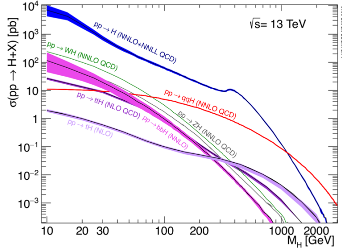
Figure 1.7: Higgs production cross section for the various production modes as a function of the Higgs boson mass, M_H , at \sqrt{s} = 13 \text{ TeV} [42].
