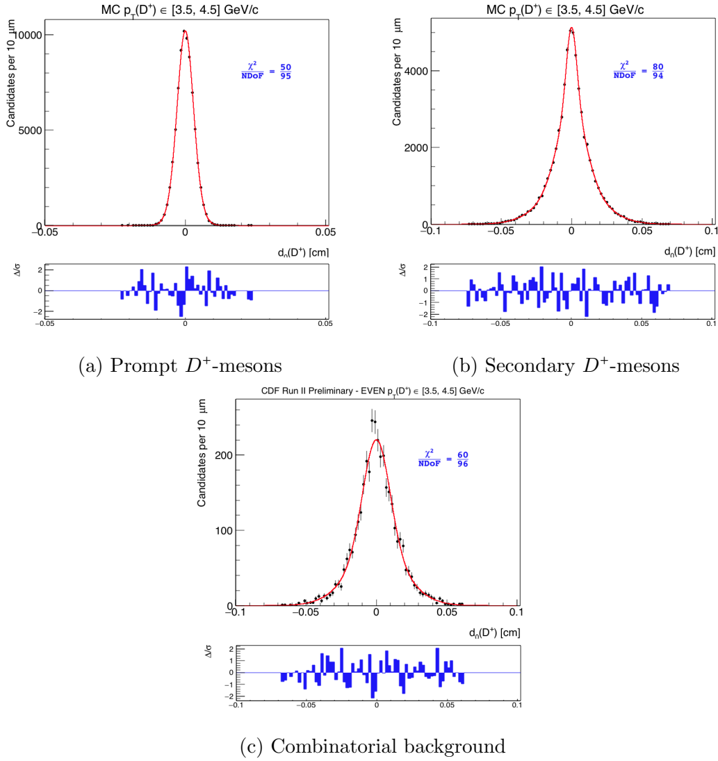
Figure 6.15: Shape parametrization of the impact-parameter distribution for the D^+ prompt (a), secondary (b) and combinatorial component (c) for p_T(D^+) in the range 3.5 – 4.5 GeV for the even-numbered events.
