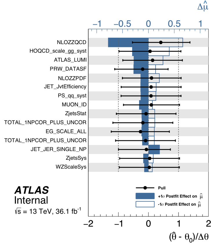
Figure 5.4: Impact of systematic uncertainties on the fitted signal-strength parameter \hat{\mu} in the \ell\ell\nu\nu channel. The systematic uncertainties are ranked in descending order of their impact on \hat{\mu} on the y -axis. The boxes show the variations of \hat{\mu} - they refer to the upper x -axis - when fixing the corresponding individual nuisance parameter \theta to its post-fit value \hat{\theta} modified upwards or downwards by its post-fit uncertainty, and repeating the fit. The blue and uncoloured boxes correspond to the upwards and downwards variations, respectively. Dots with error bars refer to the lower x -axis and show the deviations of the fitted nuisance parameters \hat{\theta} from their nominal values \theta_0 , expressed in terms of standard deviations with respect to their nominal uncertainties \Delta\theta . The associated error bars show the post-fit uncertainties of the nuisance parameters, relative to their nominal uncertainties. Systematics are neglected if their effect is smaller than 1%.
