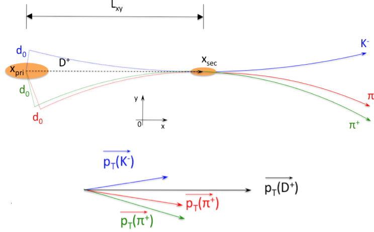
Figure 6.6: Graphical representation in the transverse plane of the decay channel D^+ \rightarrow K^-\pi^+\pi^+ with some kinematics variables indicated.
