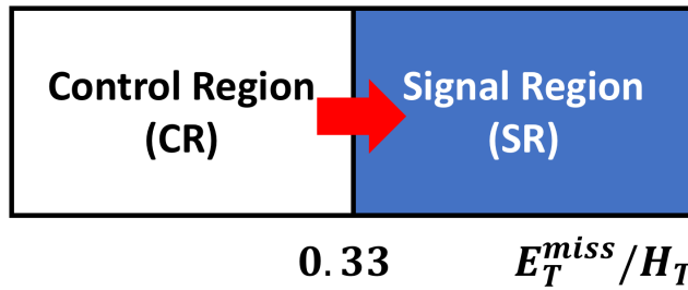
Figure 4.15: Pictorial representation of the Z + jets Control Region. The E_T^{miss}/H_T cut is reversed to construct the Control Region.
