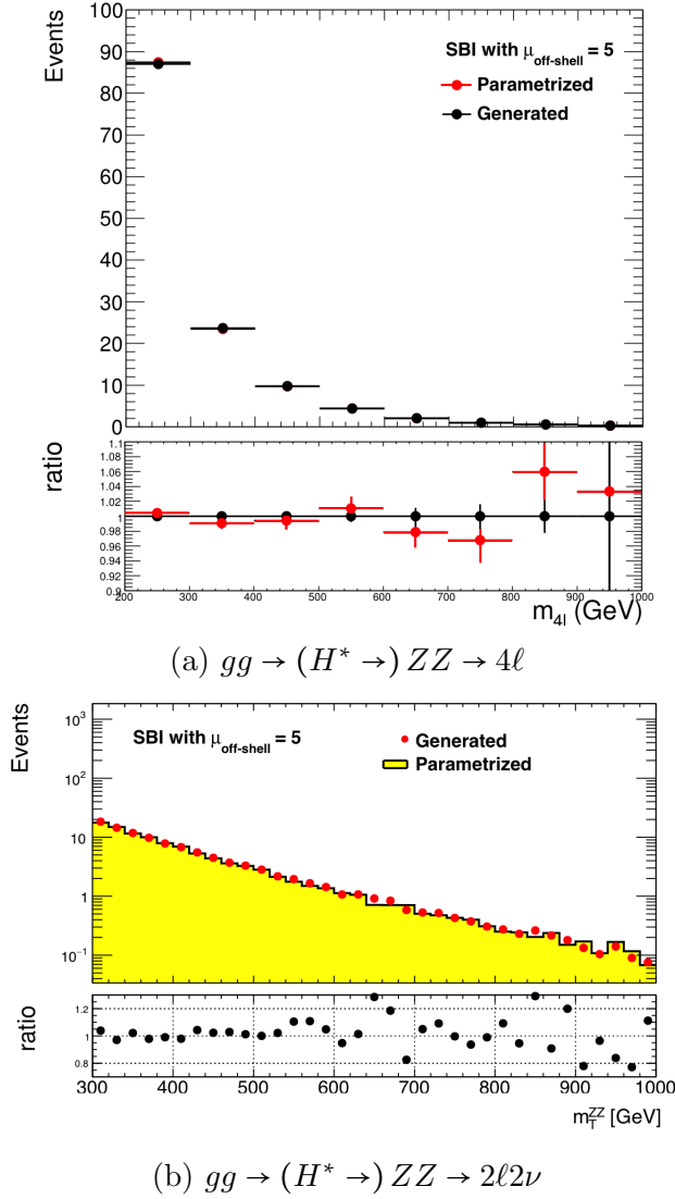
Figure 4.8: Comparison of the distribution of the m_{4\ell} (a) and of the transverse mass m_T^{ZZ} (b) with \mu_{off-shell} = 5 for the generated gg \rightarrow (H^* \rightarrow) ZZ sample [black for (a) and red for (b)] and the gg \rightarrow (H^* \rightarrow) ZZ sample assembled using the parametrization discussed in the text based on the three generated samples: gg \rightarrow H^* \rightarrow ZZ , gg \rightarrow ZZ and gg \rightarrow (H^* \rightarrow) ZZ samples [red markers for (a) and yellow histogram for (b)]. The various distribution are normalized to the same luminosity. Figure (a) produced by an ATLAS collaborator.
