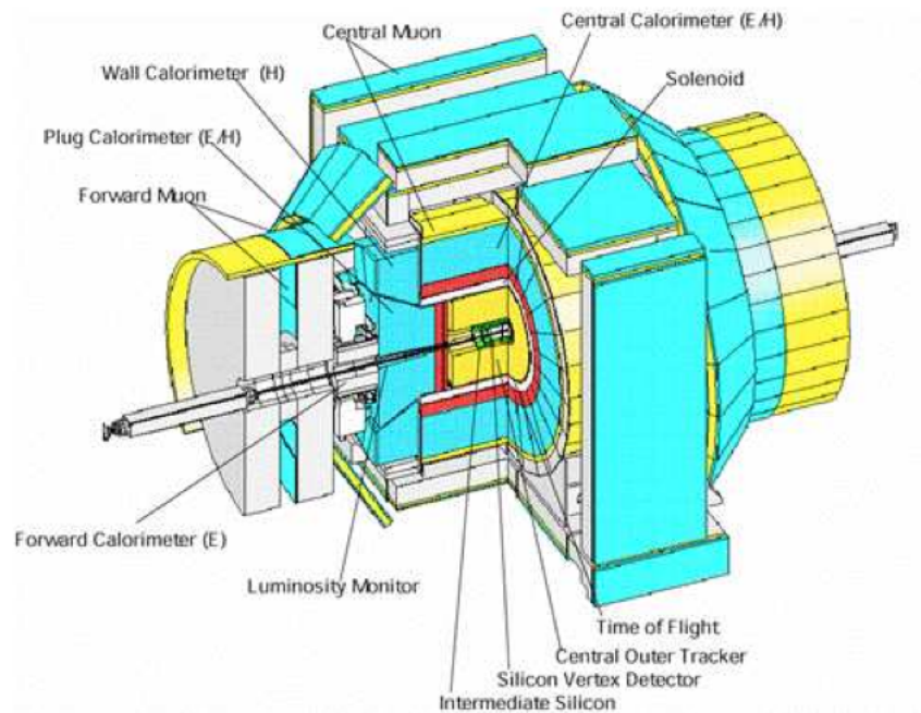
Figure 6.2: Isometric view of the CDF II detector.
