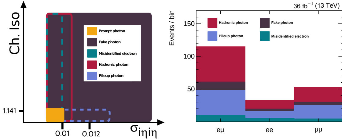
FIGURE 5.15: Left: Illustration showing where the (fake) photons from each category are distributed in the \sigma_{in\eta} / charged isolation grid. The boxes show only where the bulk of the events fall, while in reality plenty of events fall outside them. Most notably the hadronic photon category has non-negligible numbers of events with large \sigma_{in\eta} values, but is at the same time much less spread out than the fake photon category. Different drawing styles are merely used to make it clear where the boxes overlap, and the values indicated on the axes correspond to selection criteria which will become relevant in the next section. Right: Yields of the various nonprompt photon categories in the signal region, with both the \sigma_{in\eta} and charged isolation requirements applied.
