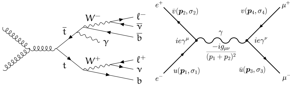
FIGURE 2.2: A Feynman diagram in which a top and antitop quark are produced, one of which radiates a photon, after which both decay decay into a charged lepton, a neutrino, and a bottom quark (left), and a simple lepton pair production diagram (right) [16].
