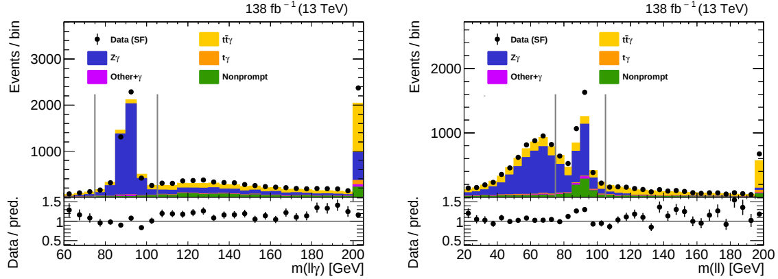
FIGURE 5.8: The m(l\bar{l}\gamma) and m(l\bar{l}) distributions in the SF channels of the signal region, with the requirements on these variables removed. Grey lines indicate range requirements applied to these variables in the signal region event selection. The Z\gamma process peaks in both distributions around the Z boson mass (approximately 91 GeV). Most of the events falling outside of these peaks in either distribution correspond to the bulk of the peak in the other distribution, so that applying range requirements on both variables effectively removes Z\gamma contributions.
