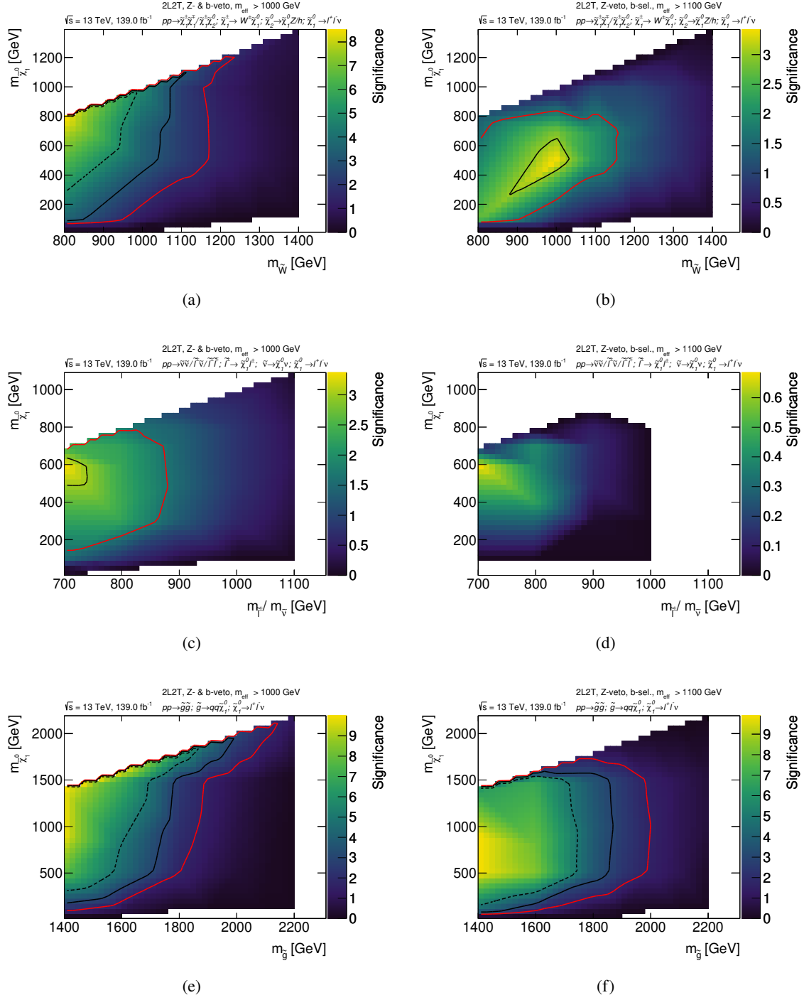
Figure B.4: Expected significance for the RPV models with \lambda_{i33} \neq assuming wino (top), slepton (middle) and gluino (bottom) pair production in SR2 tight b-veto (left) and SR2 b-req (right) events for 139 fb -1 of data assuming a 30% uncertainty on the background. The red, solid black and dashed black lines indicate the 1.68σ, 3σ and 5σ contours, respectively.
