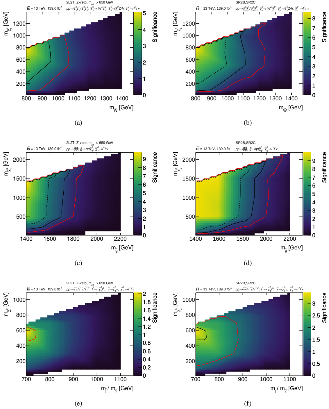
Figure 7.14: Comparison of the sensitivity obtained by the SR2 selection (left) and by the combination of the reoptimized SR2 _{b\text{-veto}}^{\text{tight}} and SR2 _{b\text{-req}} selections to RPV models with active \lambda_{i33} coupling and a wino (top), gluino (middle) and slepton (bottom) as NLSP in 139 fb ^{-1} of \sqrt{s} = 13 TeV pp collision data. The SR are combined by adding the significances in each SR in quadrature. The red, solid black and dashed black lines indicate the 1.68 \sigma , 3 \sigma and 5 \sigma contours, respectively.
