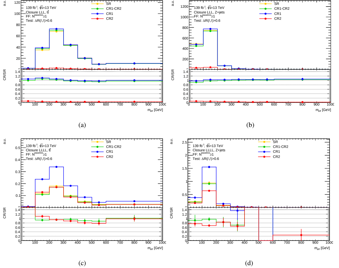
Figure 7.20: Closure test of the reducible estimate on the t\bar{t} (left) and Z + jets (right) sample shown as a function of the effective mass in three-lepton (top) and four-lepton (bottom) events. The yellow line shows the prediction for the signal region-like event selection, the blue and red lines demonstrate the estimate for the associated CR1 and CR2 regions weighted by the appropriate fake factors, respectively and the green line indicates the full reducible estimate which is the difference between the two. The bottom panel shows the ratio of the CRs to the signal region-like event selection.
