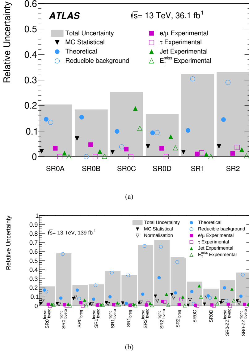
Figure 7.30: Breakdown of the dominant systematic uncertainties in the background estimates for the signal regions in the 36.1 \text{ fb}^{-1} iteration (a) and the full Run 2 iteration (b). The individual uncertainties can be correlated, and do not necessarily sum in quadrature to the total background uncertainty [327, 328].
