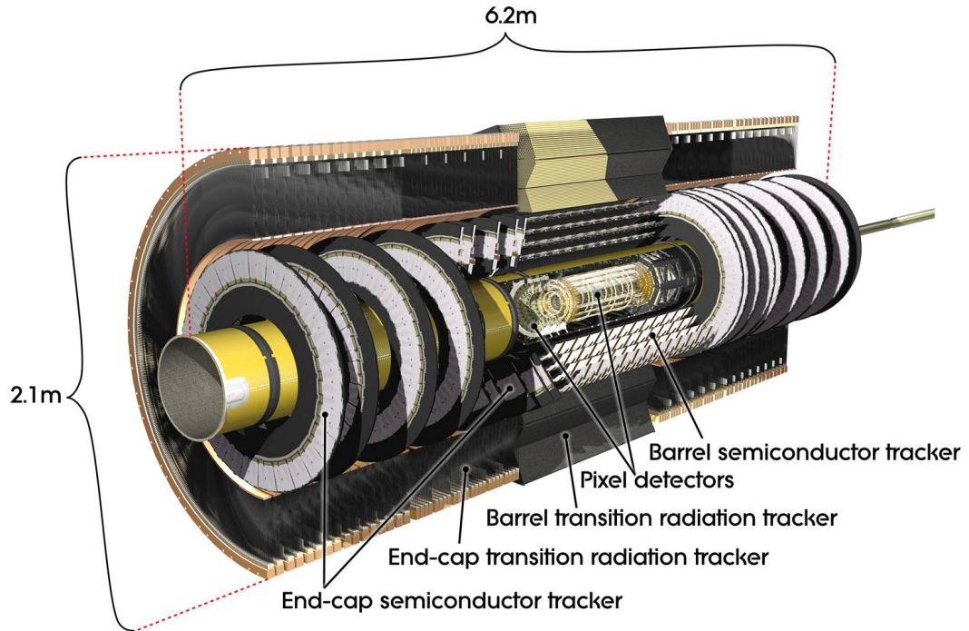
Figure 3.2: Cut-away view of the Inner Detector of ATLAS [133].
