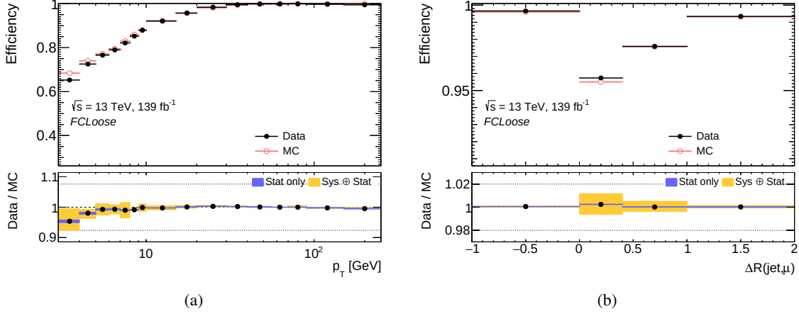
Figure 5.36: FCLoose isolation efficiency for muons shown as a function of the muon p_T (a) and the proximity to reconstructed jets (b) in Z \rightarrow \mu\mu events measured in the full run II dataset. The interval \Delta R < 0 in (b) corresponds to no jet events. The bottom panel shows the efficiency scale factor. The yellow error bands indicate the quadratic sum of statistical and systematic uncertainties.
