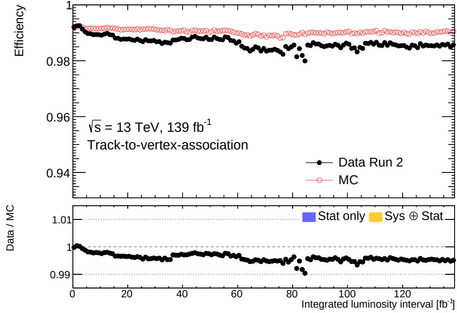
Figure 5.32: TTVA selection efficiency of Loose muons in Z \rightarrow \mu\mu events shown as a function the integrated luminosity interval in the full Run 2 dataset. Each data point corresponds to 1 fb -1 of collected data. The bottom panel shows the efficiency scale factor. The yellow error bands indicate the quadratic sum of statistical and systematic uncertainties.
