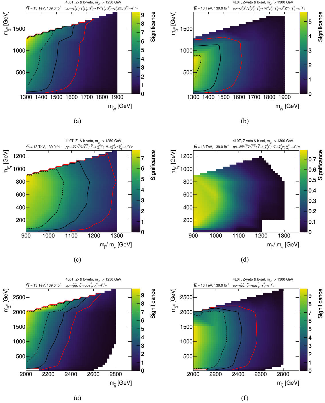
Figure B.2: Expected significance for the RPV models with \lambda_{12k} \neq assuming wino (top), slepton (middle) and gluino (bottom) pair production in \text{SR0}^{\text{tight}}_{b\text{-veto}} (left) and \text{SR0}_{b\text{-req}} (right) events for 139 \text{ fb}^{-1} of data assuming a 30% uncertainty on the background. The red, solid black and dashed black lines indicate the 1.68\sigma , 3\sigma and 5\sigma contours, respectively.
