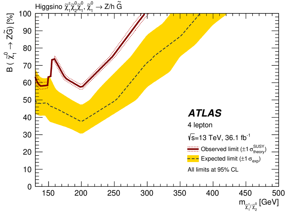
Figure 7.39: Expected (dashed) and observed (solid) 95% CL exclusion limits on the exclusion limits on the higgsino GGM model for the initial analysis of 36.1 \text{ fb}^{-1} of \sqrt{s} = 13 \text{ TeV} data. The limits are set using the statistical combination of disjoint signal regions. Where the signal regions are not mutually exclusive, the observed CLs value is taken from the signal region with the better expected CLs value [327].
