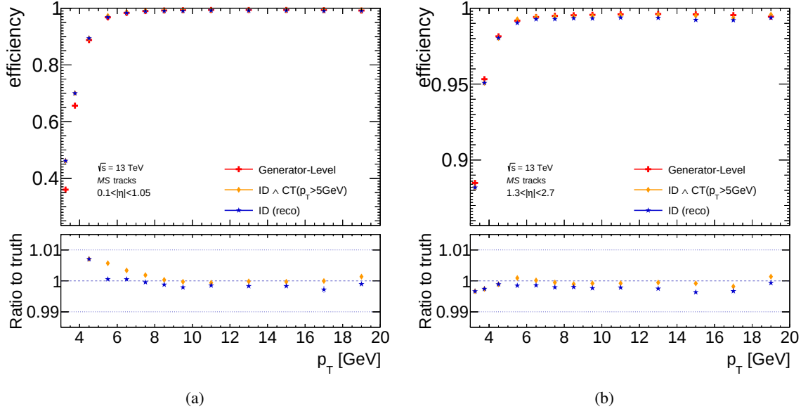
Figure 5.7: MS reconstruction efficiency as a function of the probe transverse momentum in the barrel (a) and in the endcaps (b) of the ATLAS MS in simulated J/\psi \rightarrow \mu\mu events. The red markers indicate the truth efficiency. The orange markers show the efficiency obtained by the T&P method using CT muons as probes for p_T > 5 GeV and ID tracks otherwise. The blue markers show the efficiency using ID tracks as probes. The bottom panel shows the ratio of the respective efficiencies to the truth efficiency.
