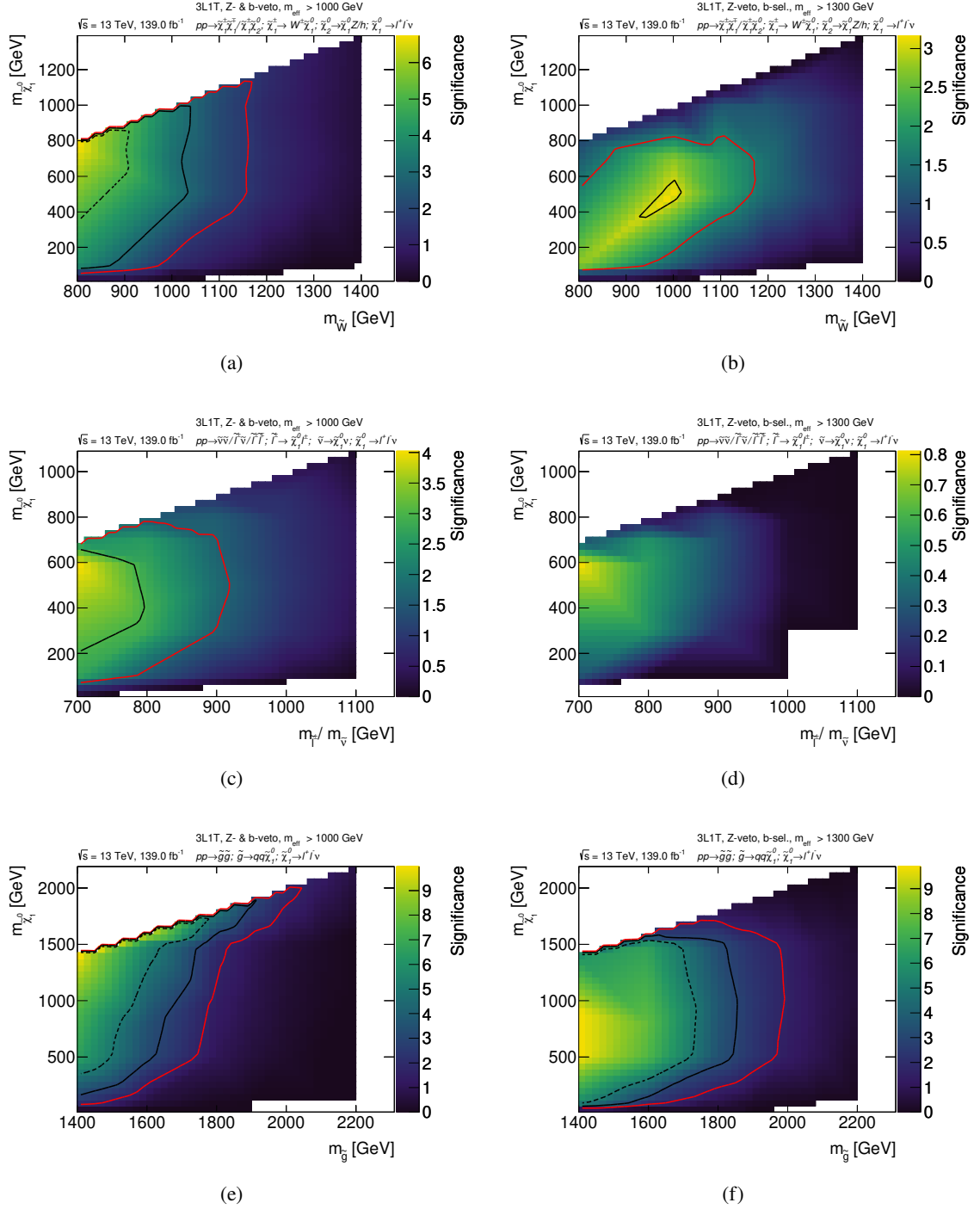
Figure B.3: Expected significance for the RPV models with \lambda_{i33} \neq 0 assuming wino (top), slepton (middle) and gluino (bottom) pair production in SR1 tight b-veto (left) and SR1 b-req (right) events for 139 fb -1 of data assuming a 30% uncertainty on the background. The red, solid black and dashed black lines indicate the 1.68 \sigma , 3 \sigma and 5 \sigma contours, respectively.
