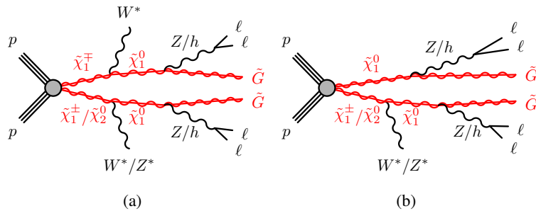
Figure 6.7: Diagrams of the processes in the SUSY RPC GGM higgsino models. The W^*/Z^* from \tilde{\chi}_1^\pm/\tilde{\chi}_2^0 decays are off-shell ( m_{V^*} \sim 1 GeV) and their decay products are usually not reconstructed.
