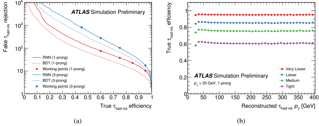
Figure 3.9: Selection efficiency of reconstructed hadronic \tau against the rejection power against particles falsely reconstructed as \tau candidates scanning the requirement on the multivariate classification scores using the RNN classifier (solid lines) and the BDT classifier (dashed lines) and the signal \tau selection efficiency of the RNN-identification working points against p_T [205].
