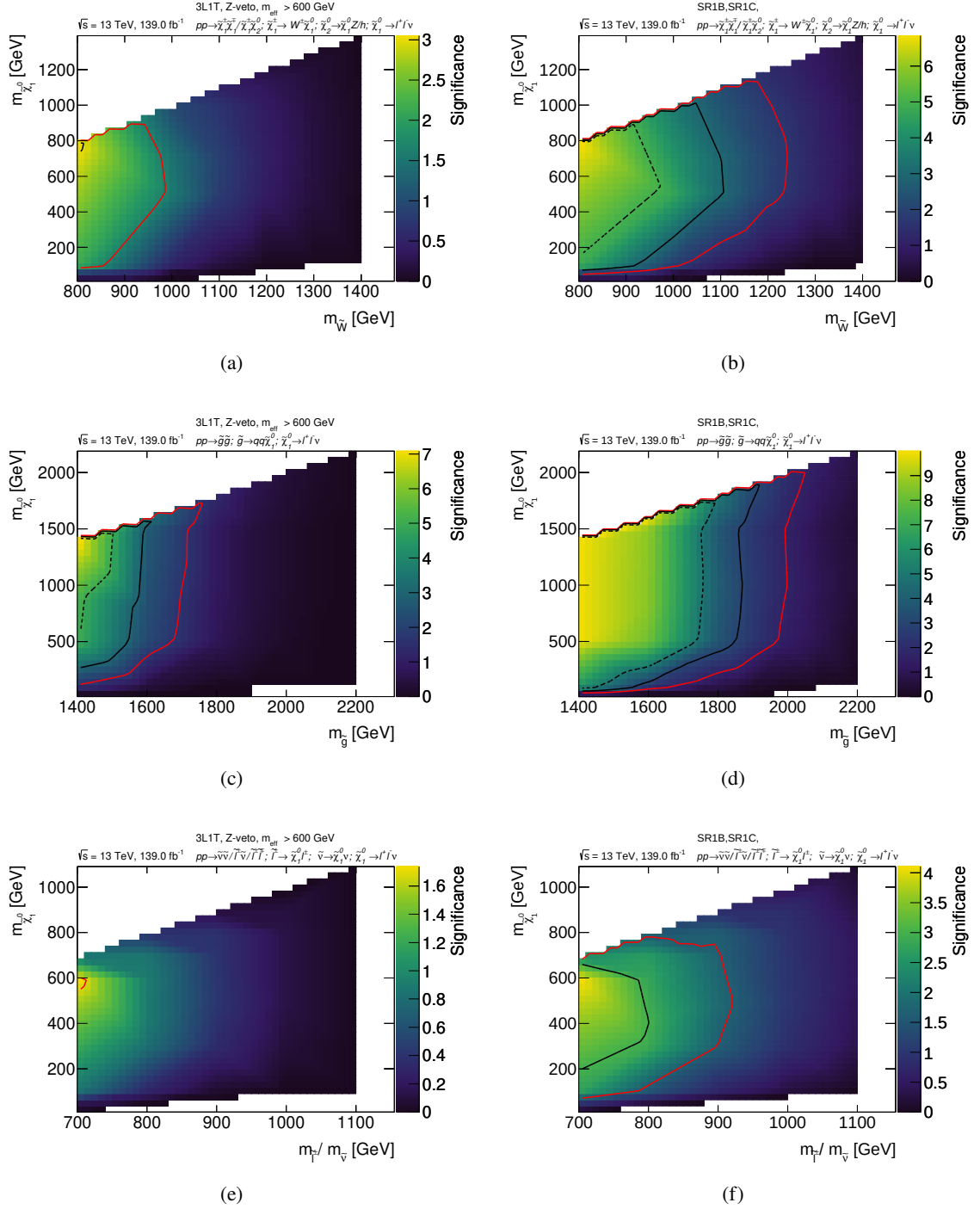
Figure 7.13: Comparison of the sensitivity obtained by the SR1 selection (left) and by the combination of the reoptimized SR1 tight b-veto and SR1 b-req selections to RPV models with active \lambda_{i33} coupling and a wino (top), gluino (middle) and slepton (bottom) as NLSP in 139 fb -1 of \sqrt{s} = 13 TeV pp collision data. The SR are combined by adding the expected significances in each SR in quadrature. The red, solid black and dashed black lines indicate the 1.68σ, 3σ and 5σ contours, respectively.
