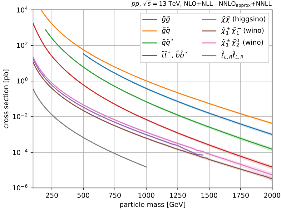
Figure 6.1: Cross sections for various supersymmetric particle production modes as a function of the particle mass at \sqrt{s} = 13 \text{ TeV} [279].
