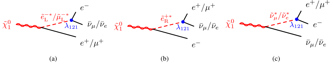
Figure 6.2: Examples of \tilde{\chi}_1^0 \rightarrow \ell\ell\nu decays caused by a non-zero lepton number violating \lambda_{121} interaction term in the superpotential.
