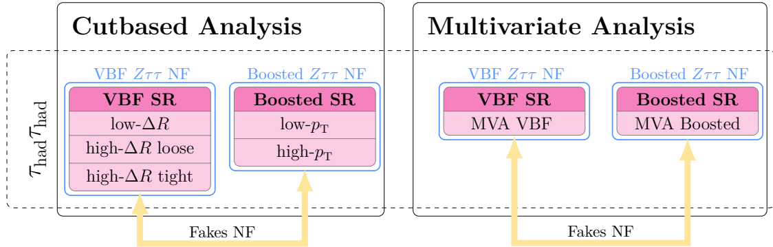
Figure 8.15: Pictogram of the \tau_{\text{had}} \tau_{\text{had}} standalone fit-model. Individual signal regions are combined to inclusive CBA VBF and Boosted regions respectively, each using an independent normalisation nuisance parameter for the Z/\gamma^* \rightarrow \tau\tau process. The Fake background normalisation is treated fully correlated between the regions.
