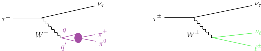
Figure 5.1: Sketches of \tau lepton decays, hadronically on the left, leptonically on the right.
