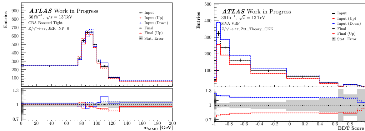
Figure 8.16: The presented distributions reflect the effects of the simplification procedures on a NP describing the jet energy resolution (left) and the CKKW-matching Z/\gamma^* \rightarrow \tau\tau theory uncertainty (right) on the discriminants in CBA and MVA, respectively.
