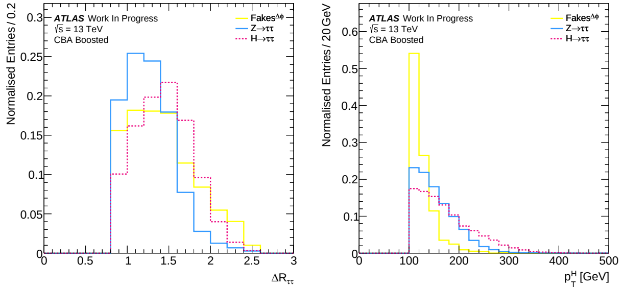
Figure 6.8: The \Delta R_{\tau\tau} (left) and p_T^H (right) distributions for the signal, Z/\gamma^* \rightarrow \tau\tau and the multijet background in the CBA Boosted inclusive region. The event model is introduced in Chapter (7).
