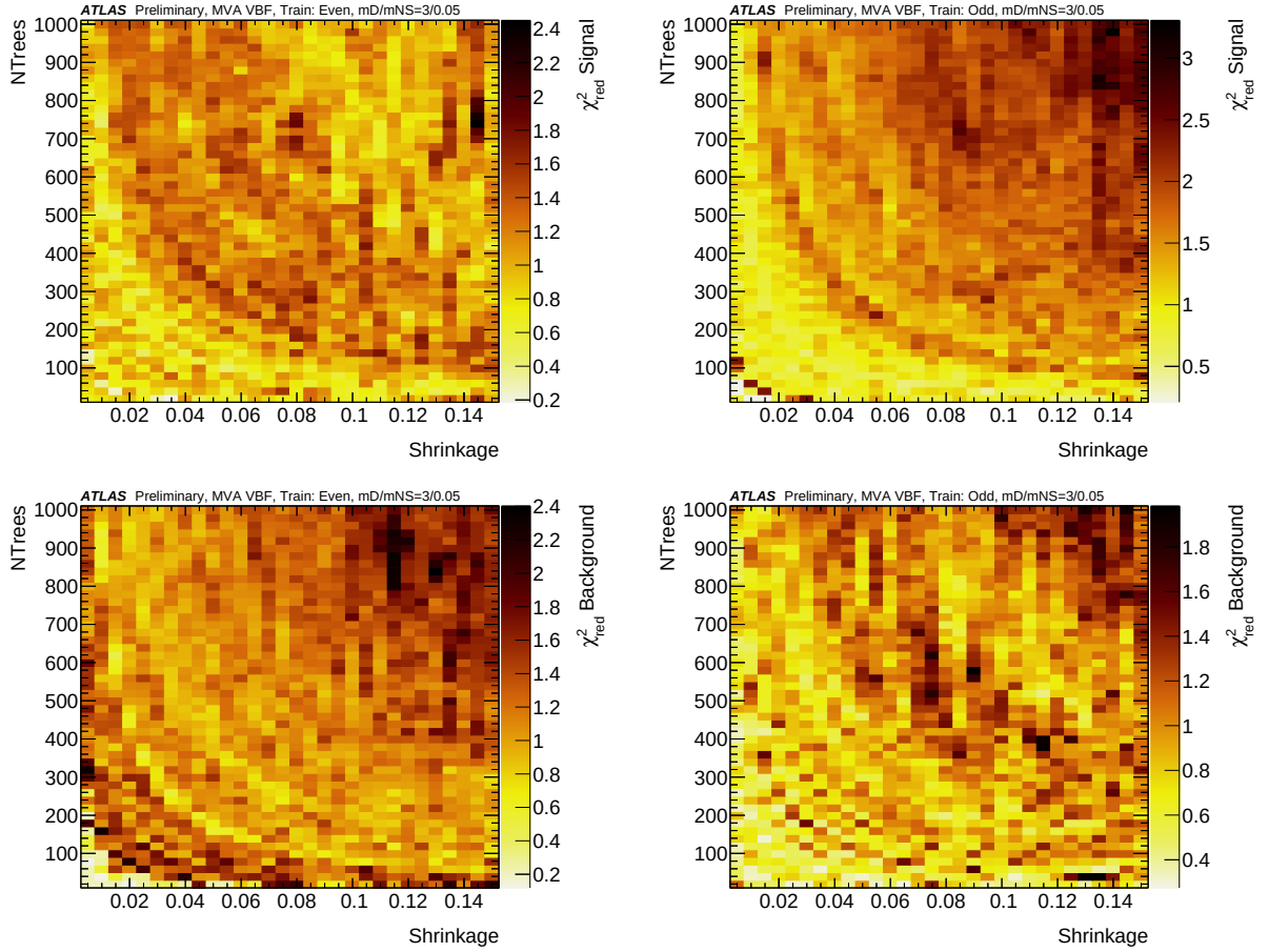
Figure B.11: Detailed parameter scan for optimal BDT Regularisation in MVA VBF. Shown is the \chi^2_{\text{red}} between signal distribution of training and testing events in dependence on number of trees. For the figures on the left (right), the BDTs were trained on the even (odd) set.
