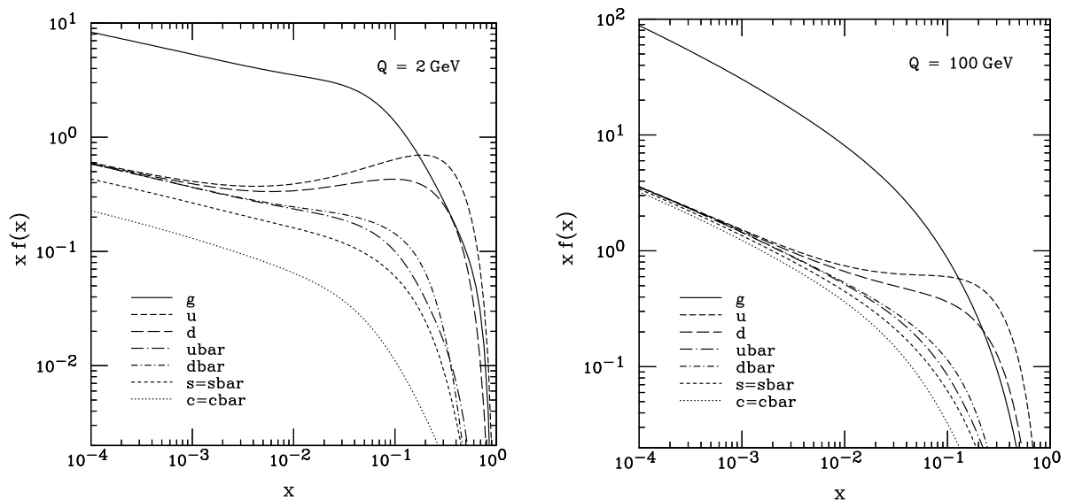
Figure 4.2: As an example, the standard set of CTEQ6M parton distribution functions are shown [78]. Two different energy scales \mu_F^2 = Q = 2 \text{ GeV} and Q = 100 \text{ GeV} were used to probe the proton structure. The solid and hatched lines indicate the probability to find a respective parton at a fraction x of the proton's momentum Q .
