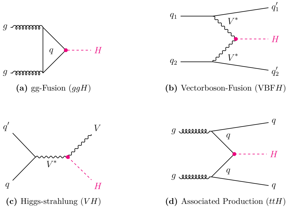
Figure 3.2: Feynman Diagrams of the dominant Higgs boson production channels at pp -colliders like the LHC.
