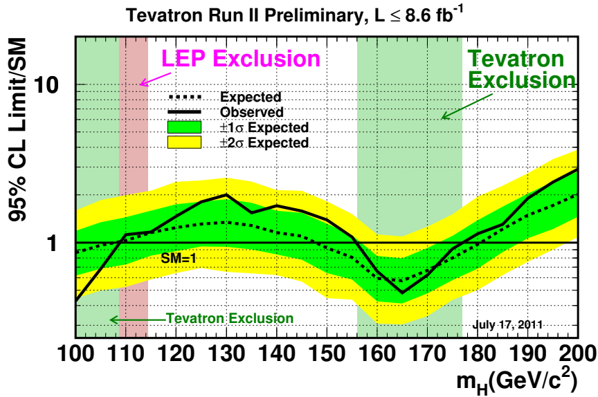
Figure 3.4: Shown are the observed and expected upper limits on the cross section ratio to the SM prediction at a 95% confidence level for the combination of CDF and DØ analyses. Additionally, the combined LEP exclusion range is indicated [4].
