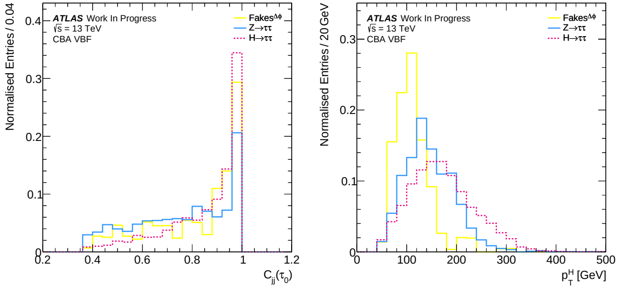
Figure 6.7: The C_{jj}(\tau_0) (left) and p_T^H (right) distributions for the signal, Z/\gamma^* \rightarrow \tau\tau and the multijet background in the CBA VBF inclusive region. The event model is introduced in Chapter (7).
