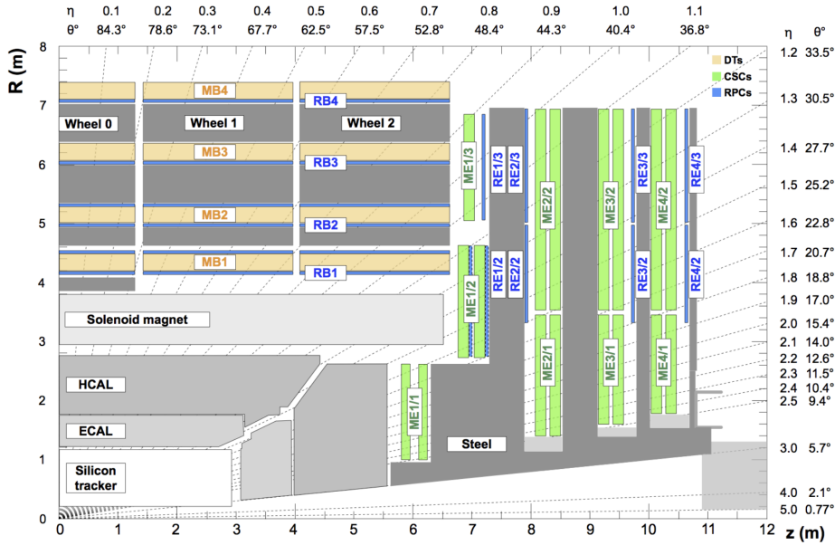
Figure 3.7: Cross section of the CMS detector in the r - z plane illustrating the subdetectors of the muon system [51]. The drift tube stations are shown in yellow (labelled as MB), the cathode strip chambers are shown in green (labelled as ME), the resistive plate chambers are shown in blue (labelled as RB and RE).
