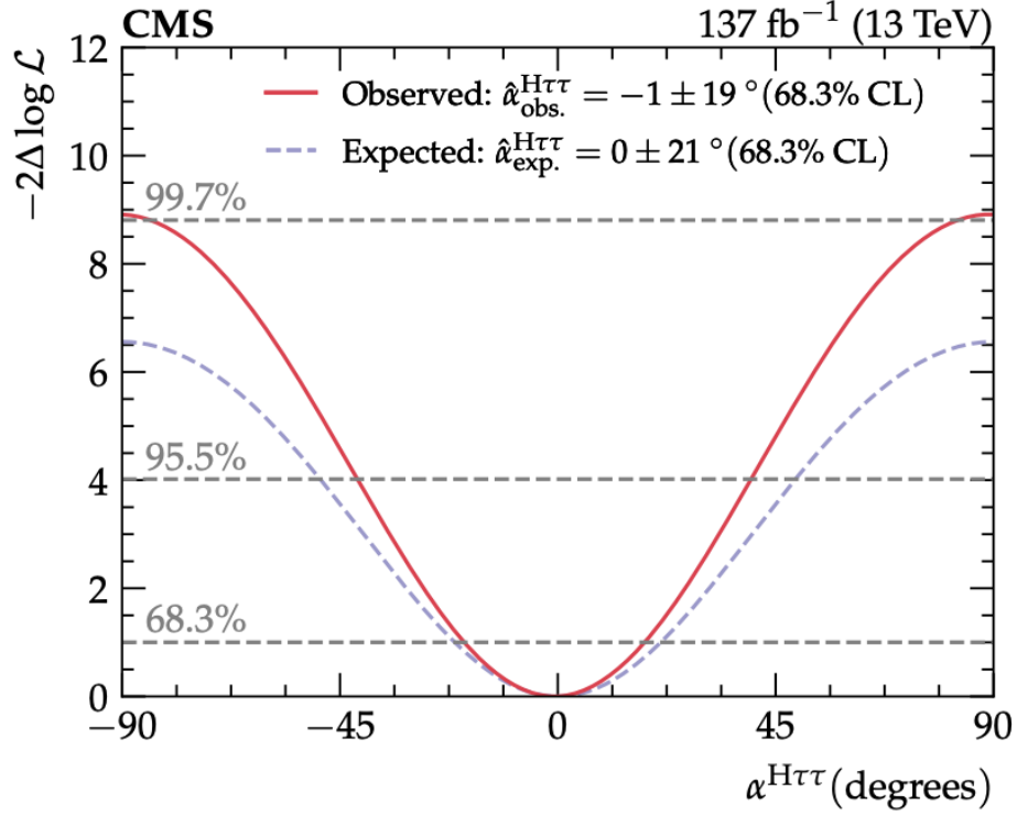
Figure 6.4: Negative log-likelihood scan of the CP mixing angle \alpha^{H\tau\tau} for the combination of \tau_\mu\tau_h , \tau_e\tau_h , and \tau_h\tau_h channels for all the data-taking years on the Azimov (dashed blue line) and collected (red solid line) data sets. Horizontal dashed grey lines indicate the thresholds for the 68.3%, 95.5%, and 99.7% CLs.
