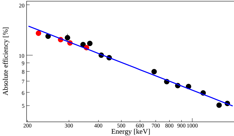
Figure 5.5: Linear fit for the intermediate energy part of the two sources with logarithmic scale for both axes. The ^{152}\text{Eu} data points are shown in black, those of ^{133}\text{Ba} in red.
