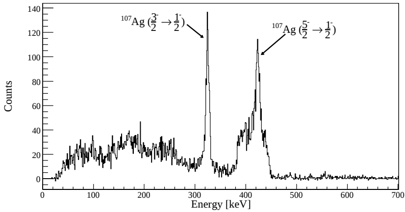
Figure 6.39: Random-subtracted \gamma -ray spectrum, coincident with two identified particles, Doppler corrected for the mercury projectile (a) and for the silver target (b). The same transitions are present here as in figure 6.38.
