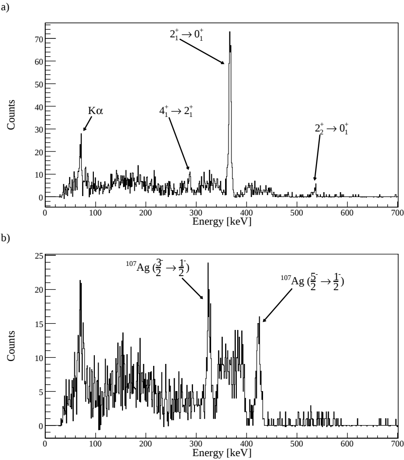
Figure 6.21: Random-subtracted \gamma -ray spectrum, coincident with two identified particles, Doppler corrected for the mercury projectile (a) and for the silver target (b). The same transitions are present here as in figure 6.20.
