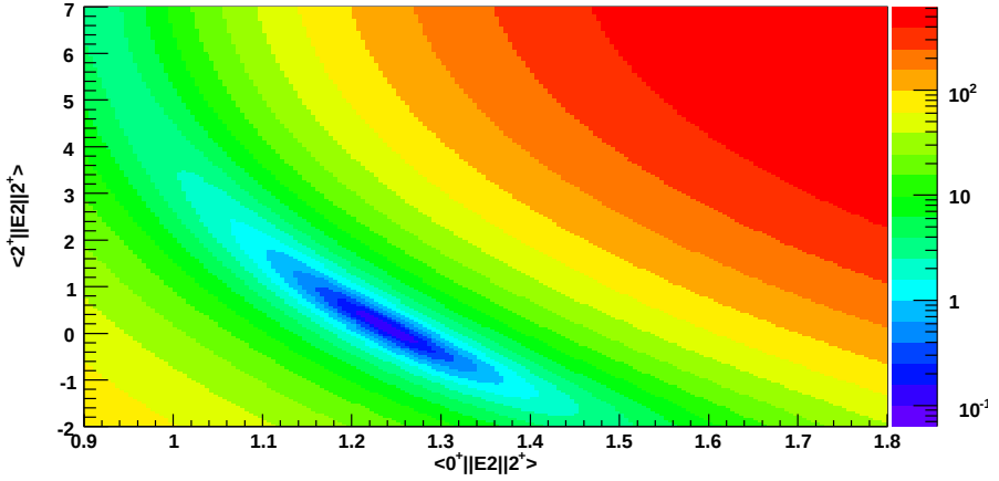
Figure 6.5: Reduced \chi^2_\nu surface assuming different values of the \langle 0^+_{g.s.} \| E2 \| 2^+_1 \rangle and \langle 2^+_1 \| E2 \| 2^+_1 \rangle in ^{182}\text{Hg} .
