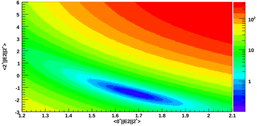
Figure 6.25: Reduced \chi^2_\nu surface assuming different values of the \langle 0^+_{g.s.} \| E2 \| 2^+_1 \rangle and the \langle 2^+_1 \| E2 \| 2^+_1 \rangle matrix elements in ^{184}\text{Hg} .
