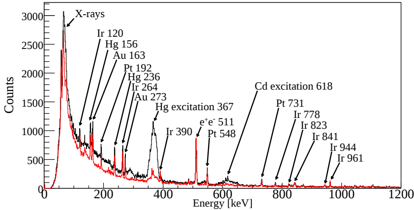
Figure 4.2: \gamma -ray spectra within prompt (black) and random (red) coincidence, the latter having been rescaled. These data were obtained from the ^{184}\text{Hg} -on- ^{112}\text{Cd} experiment. \beta decay and electron capture of ^{184}\text{Hg} and isobaric daughter nuclei result in the presence of \gamma transitions at specific energies. These are presented with the chemical element of the mother nucleus, and the energy in keV. The decay chain also leads to the observation of X-rays. However, X-rays can also be produced by the accelerator cavities, or can originate from the deexcitation of ^{184}\text{Hg} after Coulomb excitation. The photo peak at 511 keV is caused by positron-electron pair annihilation. Coulomb excitation of the ^{184}\text{Hg} projectile and the ^{112}\text{Cd} target leads to the observation of the peaks at 367 keV and 618 keV.
