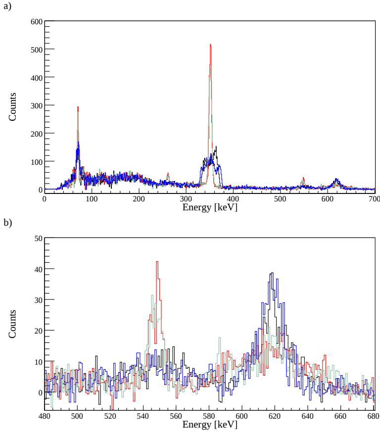
Figure 6.14: a) The four spectra are plotted in a colour referring to their number in the list in the text: black (1), red (2), green (3) and blue (4). b) A focus around the energy region of the 2_1^+ \rightarrow 0_{g.s.}^+ \gamma transition in ^{112}\text{Cd} .
