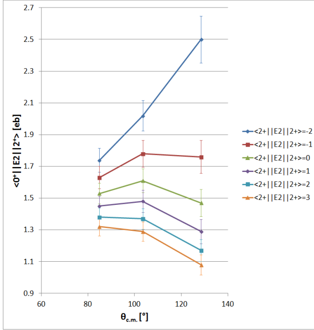
Figure 6.24: The \langle 0^+_{g.s.} || E2 || 2^+ \rangle matrix element in ^{184}\text{Hg} for the three angular ranges, assuming different integer values of the \langle 2^+_1 || E2 || 2^+_1 \rangle matrix element in this nucleus.
