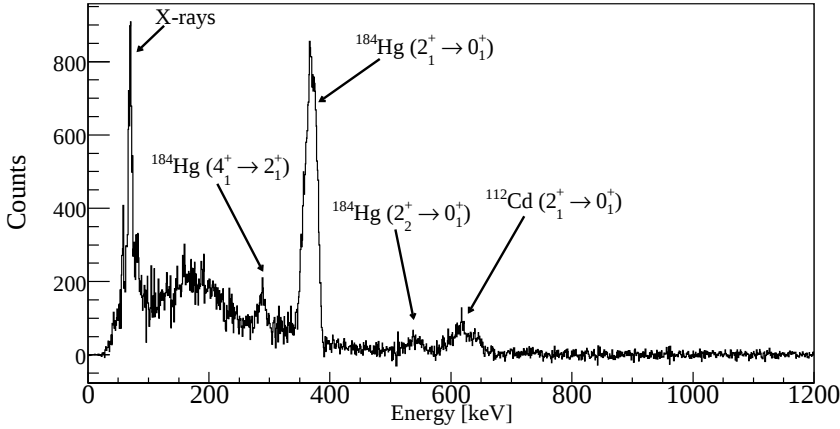
Figure 4.3: Prompt minus rescaled random \gamma -ray spectrum of the ^{184}\text{Hg} experiment on the ^{112}\text{Cd} target.
