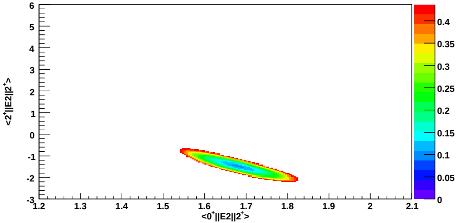
Figure 6.26: Reduced \chi^2_\nu surface with the condition \chi^2 < \chi^2_{\min} + 1 , enabling 1\sigma uncertainties for \langle 0^+_{g.s.} \| E2 \| 2^+_1 \rangle and \langle 2^+_1 \| E2 \| 2^+_1 \rangle to be estimated.
