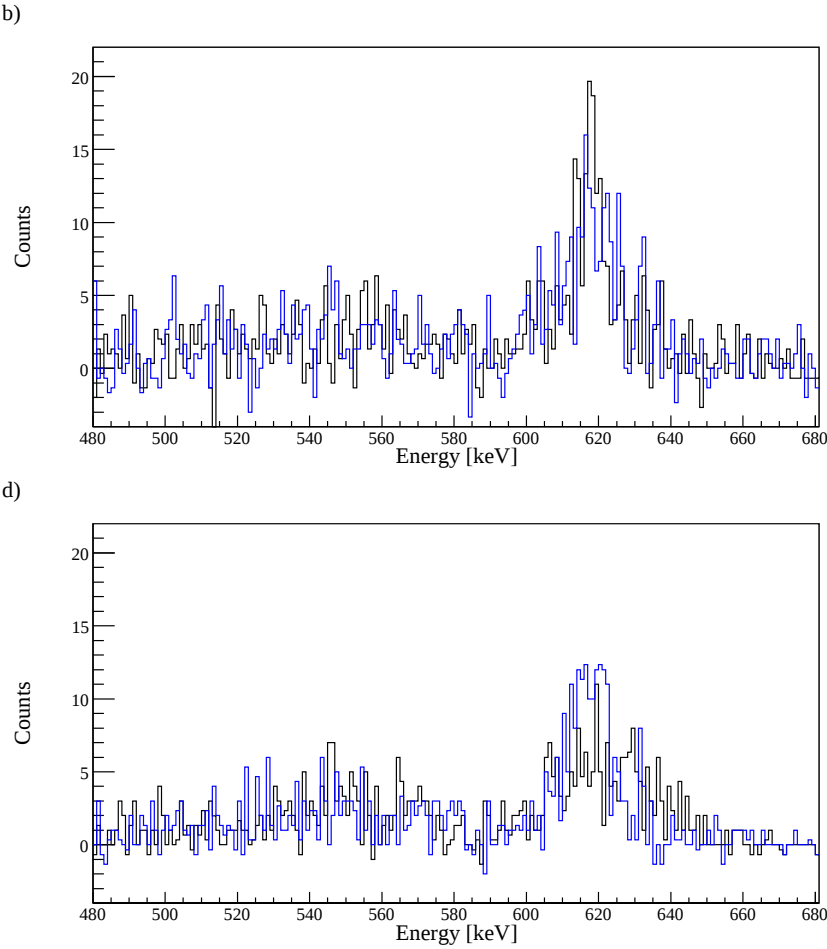
Figure 6.15: \gamma -ray spectra used for the integration of the photo peak originating from cadmium for strips 15 (a), 14 (b), 13 (c) and 12 (d). The black spectra are non-Doppler corrected, the blue spectra are Doppler corrected for cadmium, assuming cadmium falls out of the particle detector.
