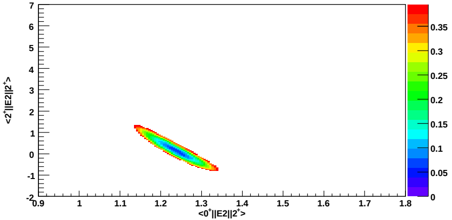
Figure 6.6: Reduced \chi^2_\nu surface with the condition \chi^2 < \chi^2_{\min} + 1 , enabling error bars for \langle 0^+_{g.s.} \| E2 \| 2^+_1 \rangle and \langle 2^+_1 \| E2 \| 2^+_1 \rangle to be estimated.
