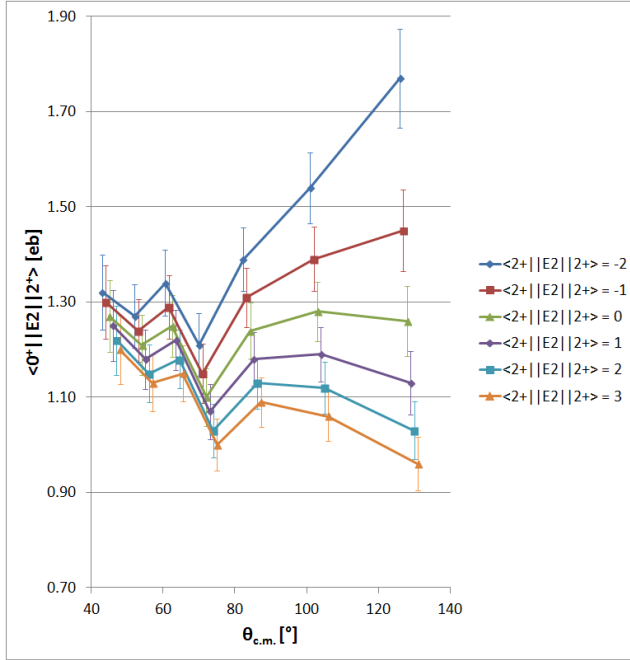
Figure 6.18: \langle 0^+_{g.s.} || E2 || 2^+_1 \rangle for the seven angular ranges, assuming different integer values of \langle 2^+_1 || E2 || 2^+_1 \rangle . Only the photo peak originating from mercury is supposed to be overestimated.
