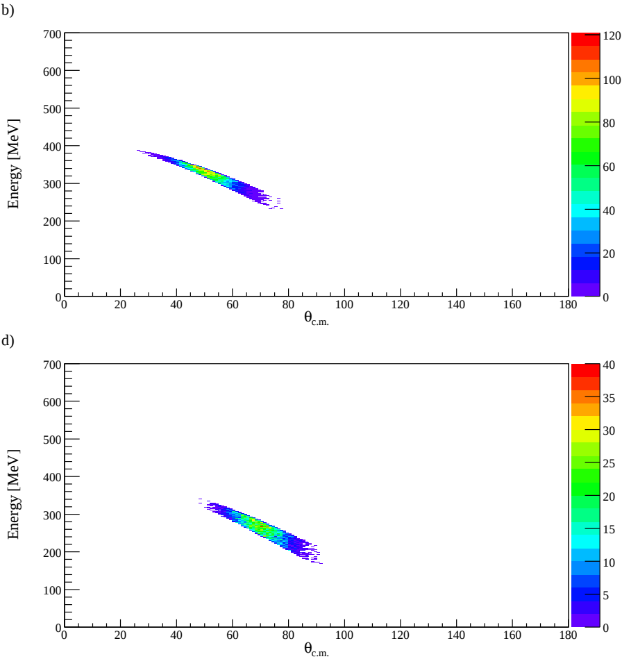
Figure 6.11: Energy of the mercury projectile versus c.m. angle gating on strips 15 (a), 14 (b), 13 (c) and 12 (d).
