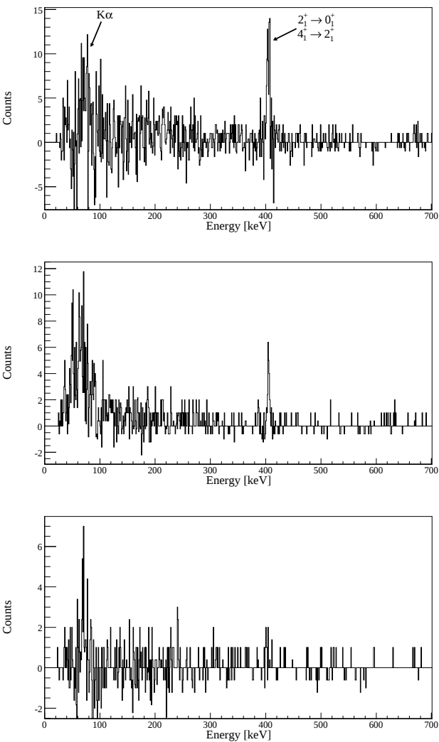
Figure 6.33: Same as figure 6.31, but obtained with the ^{120}\text{Sn} target.
