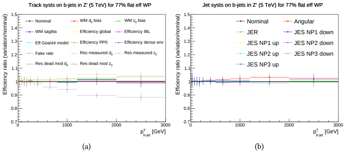
Figure C.1: Ratio of modified and nominal b -tagging efficiencies vs b -jet p_T in a 5 TeV Z' sample for the 77% fixed efficiency WP, showing track (a) and jet (b) systematics defined in Section 4.1.3.
