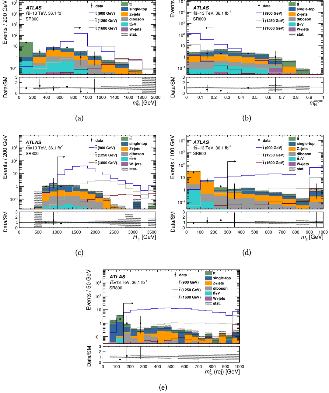
Figure 7.8: Kinematical distributions of m_{bl}^0 (a), m_{bl}^{asym} (b), H_T^{bl} (c), m_{\ell\ell} (d), and m_{bl}^1(rej) (e) in SR800 after the background only fit, where all selections are applied except the one on the displayed variable [19]. For comparison, the signal models generated with \tilde{t} masses of 900, 1250, and 1600 GeV and with 50% BR into b - e and b - \mu are included.
