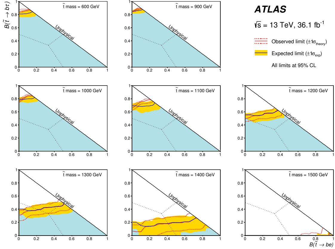
Figure 7.9: Expected and observed limits at 95% CL on the \tilde{t} signal in Figure 7.1 in the \text{BR}(e) - \text{BR}(\tau) plane with \text{BR}(e) + \text{BR}(\mu) + \text{BR}(\tau) = 1 , for \tilde{t} masses between 600 GeV and 1.5 TeV [19]. For each combination of \text{BR}(e) , \text{BR}(\mu) and \text{BR}(\tau) under exam, the limits are based on the best expected \text{CL}_s among the different flavour channels of the SRs.
