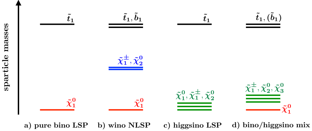
Figure 5.3: Schematic view of four possible mass spectra involving third generation squarks and light neutralinos and charginos [184]. The individual cases are discussed in the text.
