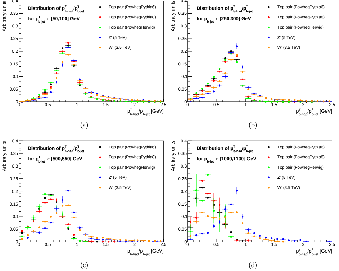
Figure 4.3: Distribution of the ratio of b -hadron and b -jet p_T in t\bar{t} (with Pythia 6, Pythia 8 and Herwig as PS generators), Z' and W' samples in the b -jet p_T ranges 50-100 GeV (a), 250-300 GeV (b), 500-550 GeV (c) and 1000-1100 GeV (d). The histograms are obtained using the MC truth information and are normalised to unit area.
