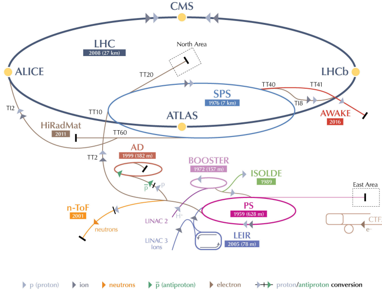
Figure 2.2: Scheme of the experimental facilities of CERN, showing the accelerator complex and the associated experiments.
