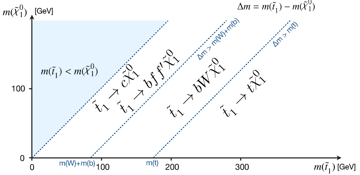
Figure 5.4: Decay modes of the \tilde{t} in the m_{\tilde{t}}-m_{\tilde{\chi}_1^0} plane [183].
