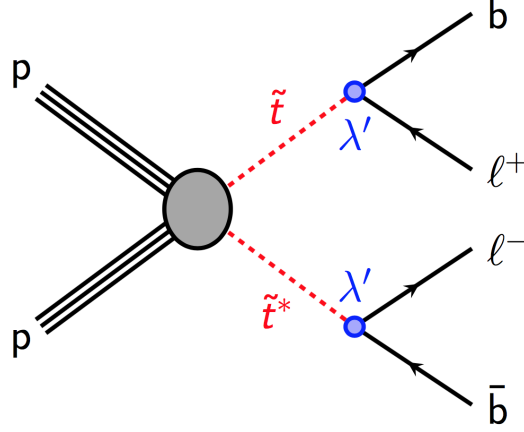
Figure 7.1: Benchmark signal model targeted by the analysis in Chapter 7, with a pair-produced stop decaying into b\text{-}\ell pairs through an RPV coupling.
