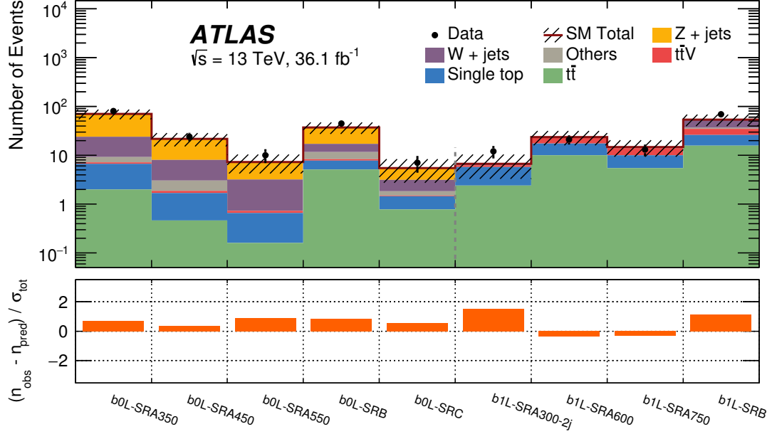
Figure 6.20: Results of the background only fits in the SRs of the analysis, using the background normalisation factors in Figure 6.18 [18]. The uncertainty band in the top panel includes all the variations presented in Section 5.3.4. The bottom panel shows the observed pulls in each SR, defined as the ratio of the difference between observed and predicted yields and the total uncertainty on the SM background, including the Poisson uncertainty.
