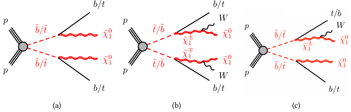
Figure 5.5: Pair-produced \tilde{t} decaying directly into a \tilde{\chi}_1^0 pair (a), a b\tilde{\chi}_1^+ pair (b) or a mixture of the two final states (c). The grey circles in the production vertices indicate generic effective couplings, which represent un-specified production modes of the particles. The figures also show how each diagram changes when replacing the \tilde{t} with the \tilde{b} .
