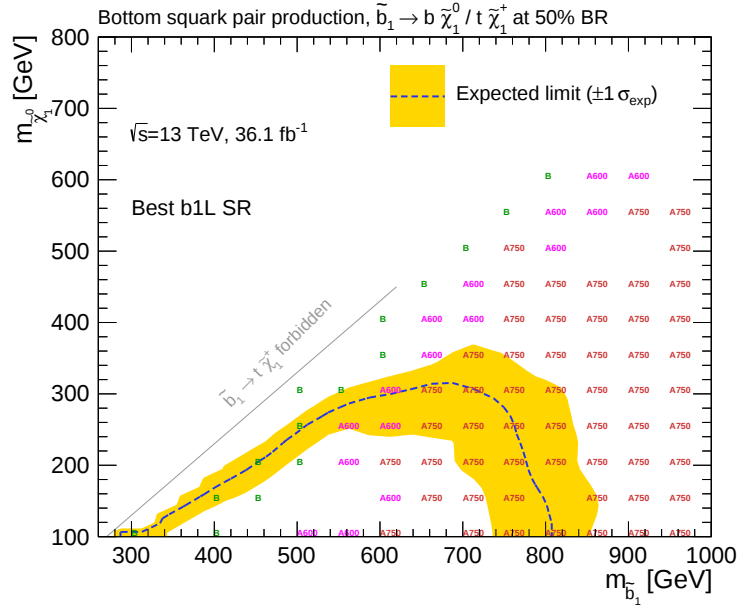
Figure 6.13: Expected exclusion limits of the one-lepton SRs on a tb + E_T^{\text{miss}} signal scenario in the m_{\tilde{b}_1}-m_{\tilde{\chi}_1^0} plane, obtained from the fit procedure described in Section 6.4. The SR with the best \text{CL}_s is indicated in the plot for every signal model considered. The b1L-SRA300-2j region is not appearing in the figure because it is less effective than the others in the signal grid under exam.
