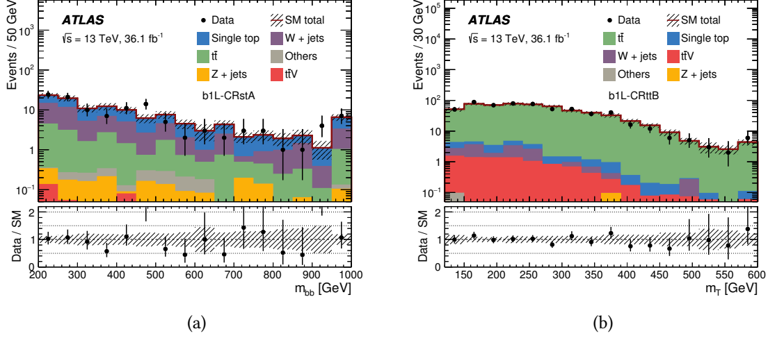
Figure 6.17: Kinematical distributions of key variables in b1L-CRs: m_{bb} in b1L-CRstA (a) [18] and m_T in b1L-CRttB (b) [18]. The MC samples are normalised using the results of the background fits, and good agreement is found between the data and the predictions. The uncertainty bands include the detector-related systematics described in Section 6.3.5, and the last bins of the distributions include overflow events.
