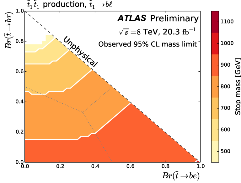
Figure 7.2: Observed limits on the mass of a pair produced \tilde{t} decaying into b\ell pairs in the Br(e) - Br(\tau) plane with Br(e) + Br(\mu) + Br(\tau) = 1 , obtained from a dedicated Run 1 ATLAS search [226].
