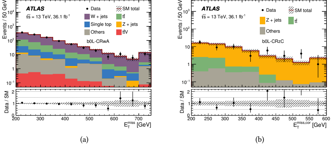
Figure 6.14: Kinematical distributions of key variables in b0L-CRs: E_T^{\text{miss}} in b0L-CRwA (a) [18] and E_T^{\text{miss,corr}} in b0L-CRzC (b) [18]. The MC samples are normalised using the results of the background fits, and good agreement is found between the data and the predictions. The uncertainty bands include the detector-related systematics described in Section 6.3.5, and the last bins of the distributions include overflow events.
