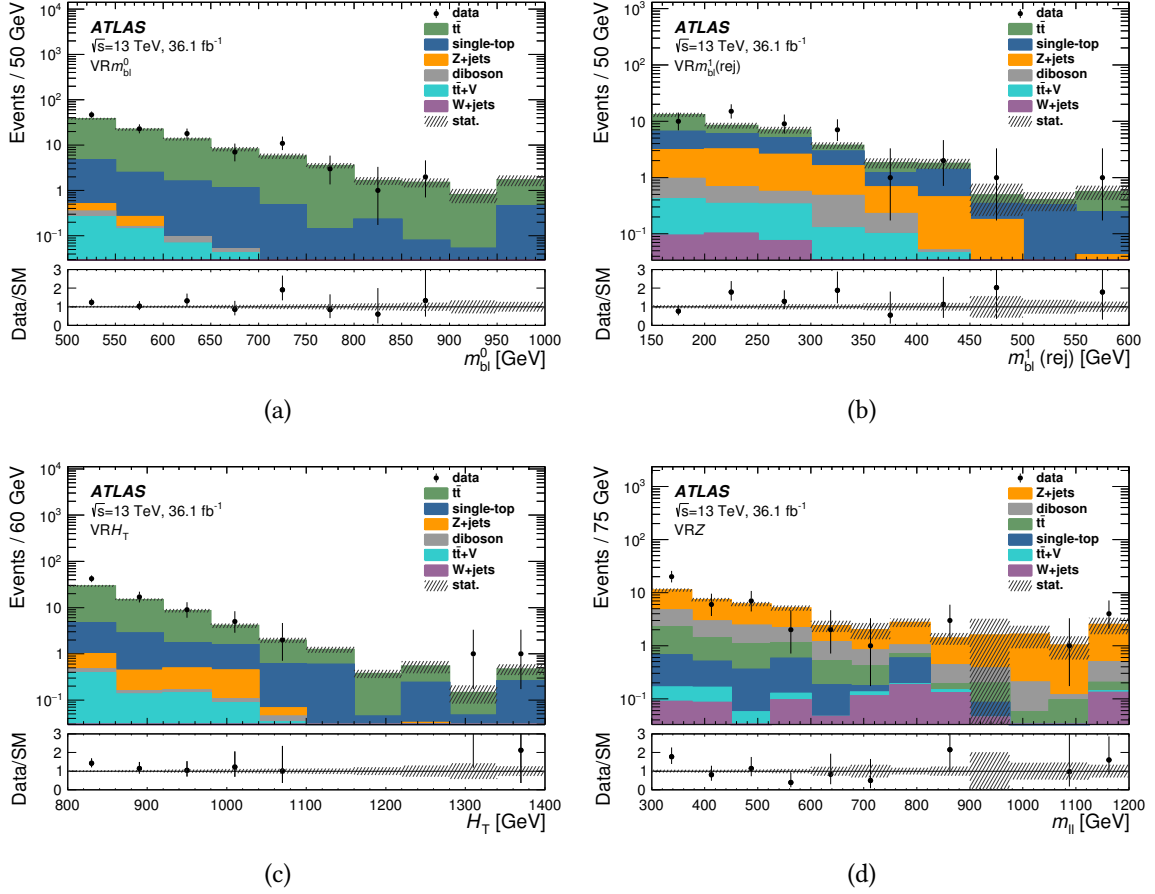
Figure 7.7: Kinematical distributions of m_{bl}^0 in VRm_{bl}^0 (a), m_{bl}^1(\text{rej}) in VRm_{bl}^1(\text{rej}) (b), H_T^{b\ell} in VRH_T^{b\ell} (c) and m_{\ell\ell} in VRZ (d) after the background only fit [19].
