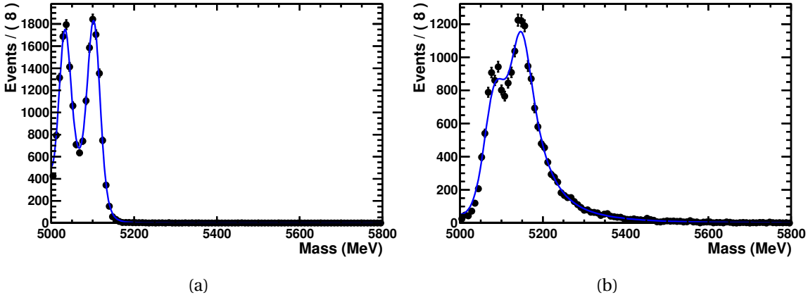
Figure 6.6: B^0 \rightarrow D^{*-} \pi^+ , D^{*-} \rightarrow D^- \pi^0 reconstructed B^0 mass shape (under the \pi^\pm mass hypothesis (a), under the K^\pm mass hypothesis (b) for the bachelor particle). The blue solid curve is the RooKeysPDF used to model them.
