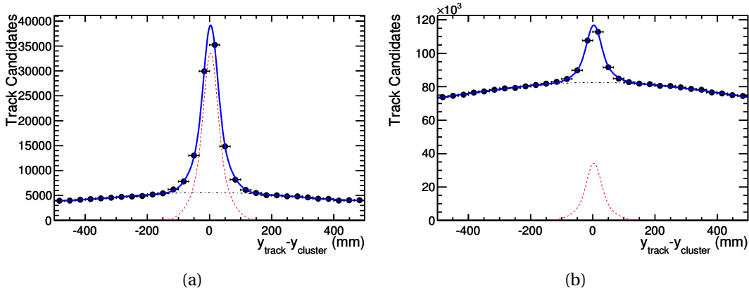
Figure 5.3: Distance in the y -axis between the calorimeter cluster and the trajectory ( \Delta y distribution) at the calorimeter for “found” tracks (a) and “all” tracks (b). The signal component, fitted with a double Gaussian, is drawn in red-dashed line, while the background component, fitted with a 4^{th} degree polynomial, is drawn in black-dashed-dot line.
