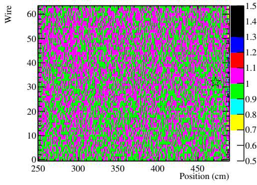
(a) Irrad. time 20 h
