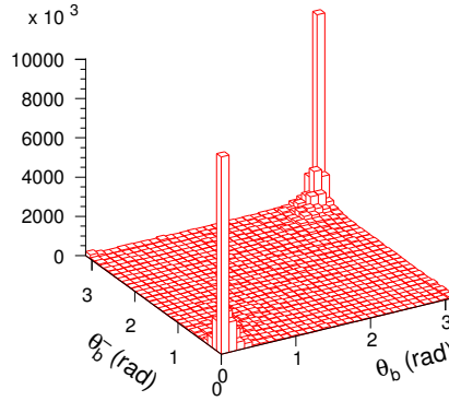
Figure 2.2: Polar angle distribution of b - and \bar{b} -hadrons produced in pp interaction as calculated by the PYTHIA event generator.
