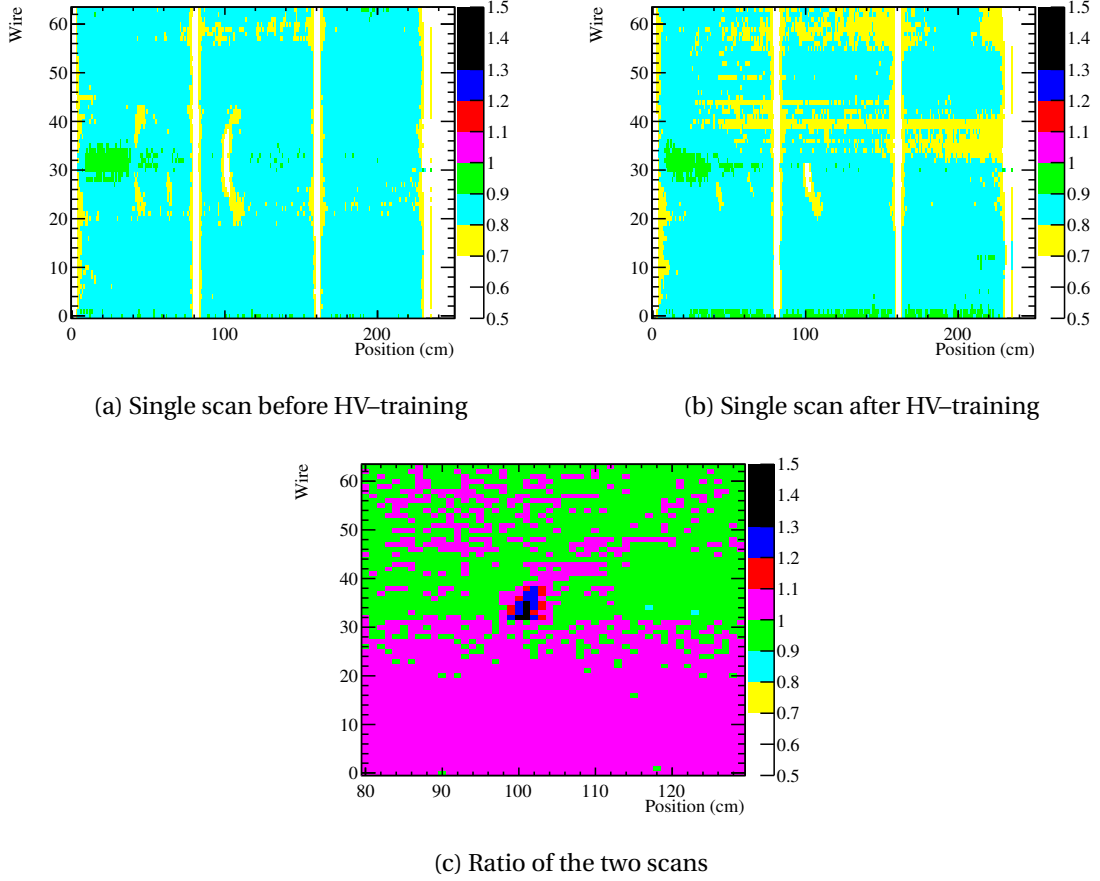
Figure 4.11: Results of an HV-training section applied to the upper half (wires 33-64) of the module (S1-122-125 on position T2L0Q1M8). (a) and (b): single scan maps before and after the HV training campaign. The color scale is in arbitrary units since no correction for the atmospheric conditions is applied. The “half-moon” shape of the typical gain loss is evident in (a). Note that the white regions around 80 and 160 cm in (a) and (b) are the wire-locators. (c): a recovery of the gain around position 105 cm. Note that the green/purple split between the two halves of the detector is not relevant and it is due to a temporary 7 behaviour seen in most cases after the HV training. No clear explanation of this effect can be provided.
