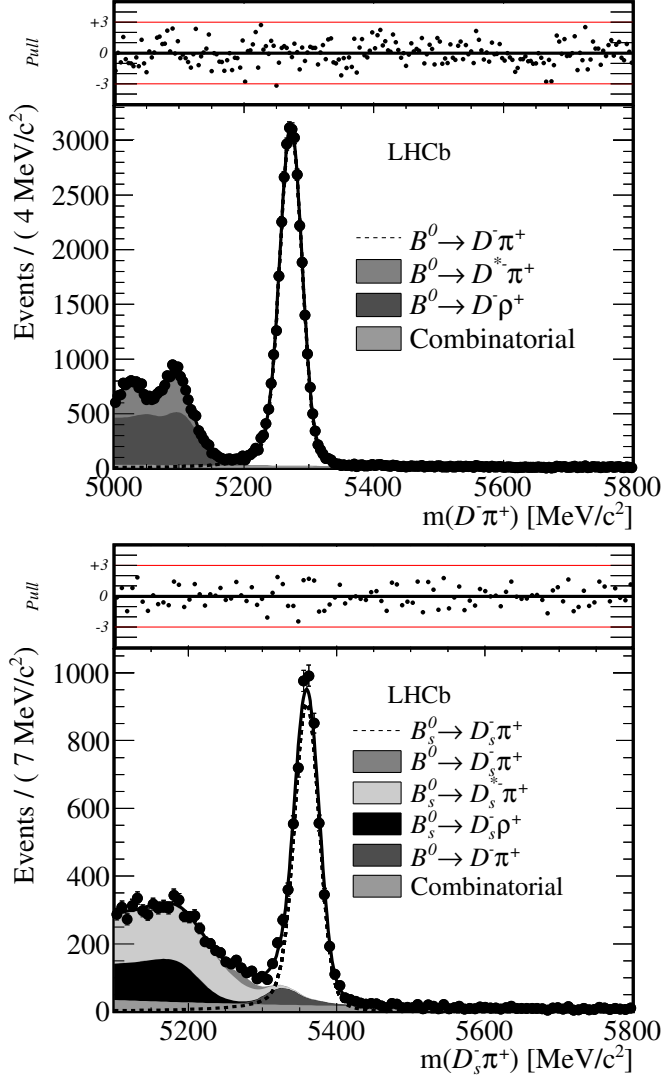
Figure 1: Mass distribution of the B^0 \rightarrow D^-\pi^+ candidates (top) and B_s^0 \rightarrow D_s^-\pi^+ candidates (bottom). The stacked background shapes follow the same top-to-bottom order in the legend and the plot. For illustration purposes the plot includes events from both magnet polarities, but they are fitted separately as described in the text.
