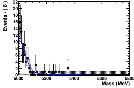
Figure 6.9: B_s^0 \rightarrow D_s^- \pi^+ \pi^+ \pi^- reconstructed B_s^0 mass shape under the \pi^\pm mass hypothesis where two pions are not considered. The blue solid curve is the RooKeysPDF used to model them.
