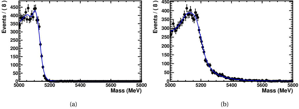
Figure 6.7: B^0 \rightarrow D^- \rho^+ , \rho^+ \rightarrow \pi^+ \pi^0 reconstructed B^0 mass shape (under the \pi^\pm mass hypothesis (a), under the K^\pm mass hypothesis (b) for the bachelor particle). The blue solid curve is the RooKeysPDF used to model them.
