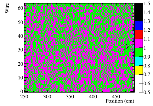
(b) Irrad. time 164 h
