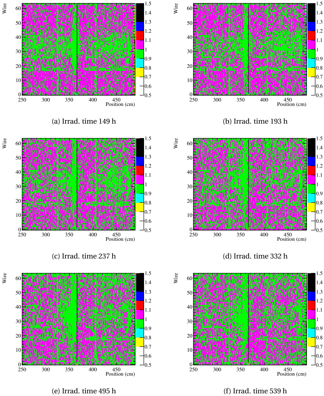
Figure 4.6: Time evolution of the source region due to the irradiation with a collimated source of 20mCi. The location of the source was at 366 cm (line), irradiating the full width of the module. The gas flowed from right to left. The colour code represents the relative detector gain.
