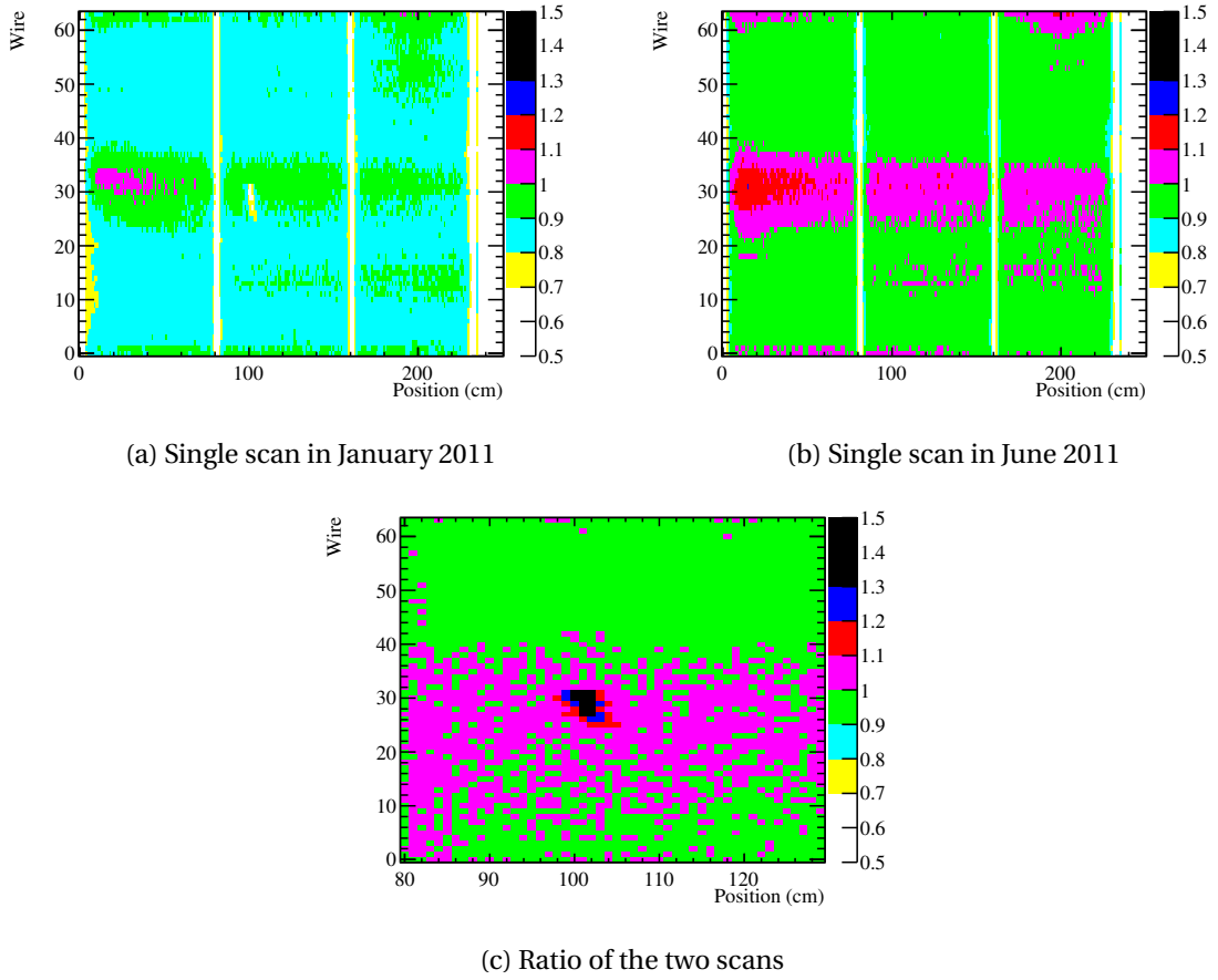
Figure 4.15: Results of the scan of module in position T2Q1L0M8 in January 2011 (a) and in June 2011 (b). From the ratio of the two single scans (c) a gain recovery placed around 105 cm is observed. This is probably due to the fact that beneficial radicals were produced during the running period and they removed previous deposits on the wire with a similar mechanism of the HV-training with the source. The color scale in the two single scan maps is in arbitrary units since no correction for the atmospheric condition is applied, while in the ratio of the two scans represents the relative gain. No gain variation along the detector is observed.
