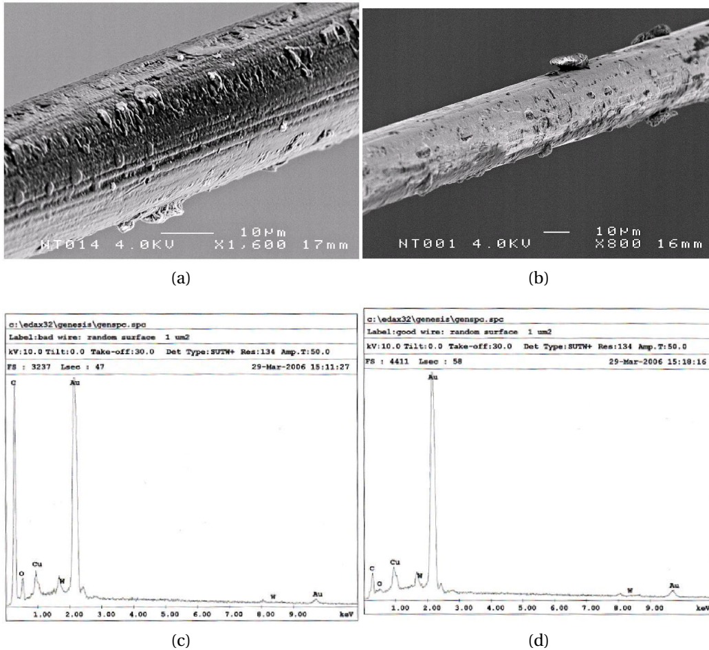
Figure 4.1: (a): a Scanning Electron Microscope (SEM) picture of an irradiated OT wire sample, (b): SEM picture of a not irradiated OT wire sample, (c): Energy Dispersion X-ray (EDX) spectra for an irradiated OT wire. A clear carbon peak is observed. (d): EDX spectra for a not irradiated OT wire sample. Note still the presence of a small carbon peak.
