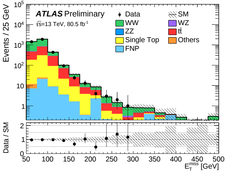
(a) E_T^{miss} in VR-WW-0J
