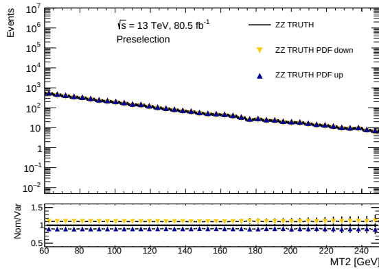
(c) ZZ process, preliminary selection
