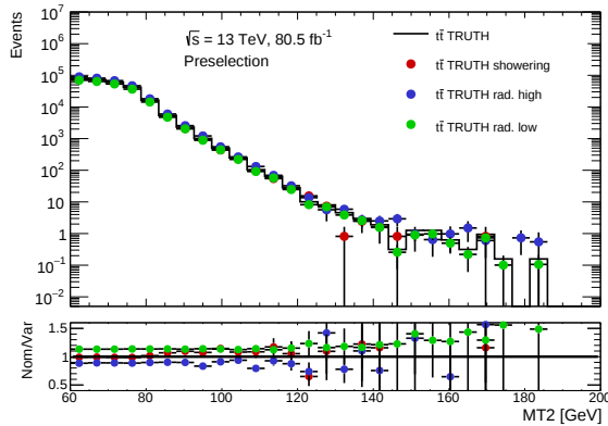
Figure 7.19: The m_{T2} distribution for the nominal t\bar{t} sample and the theoretical systematics variation, at the Truth level. The preliminary selection is considered.
