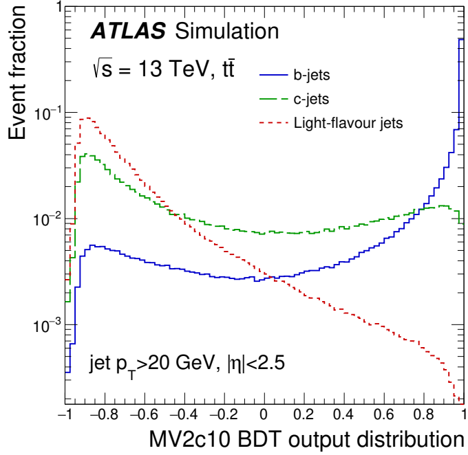
Figure 4.3: The MV2c10 output for b -jets, c -jets and light-flavor jets, considering simulated t\bar{t} Monte Carlo events [107].
