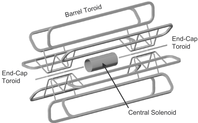
Figure 2.8: Schematic view of the four ATLAS magnets [8].
