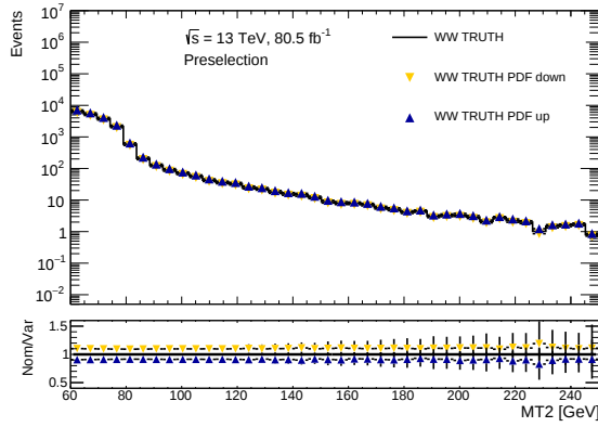
(a) WW process, preliminary selection
