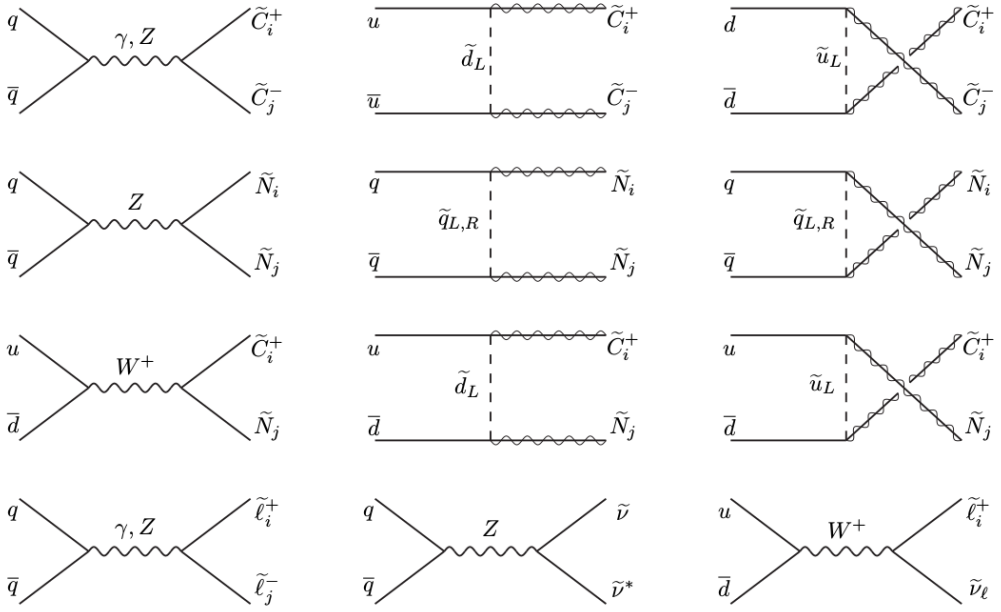
Figure 1.6: Feynman production diagrams for slepton, chargino and neutralino pairs. The t-channel production is supposed to be negligible, since squarks are assumed to be very heavy compared to sleptons, charginos and neutralinos. The s-channel mediated by photon, Z or W^\pm is the relevant production channel for this work [35].
