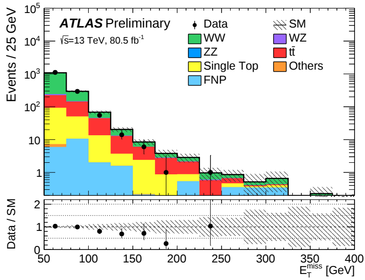
Figure 7.8: The E_T^{miss} distribution for the data and the estimated SM backgrounds in CR-WW, after performing the background-only likelihood fit. The uncertainty bands include all systematic and statistical contributions.
