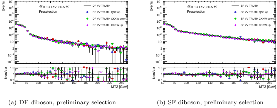
Figure 7.18: The m_{T2} distribution for the nominal Sherpa diboson samples and the theoretical systematics variation, for events with DF leptons (a) or SF leptons (b), at the Truth level. The preliminary selection is considered.
