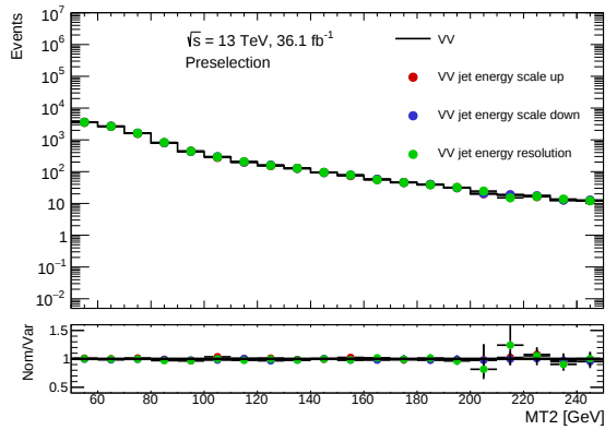
(c) VV SF, preliminary selection
