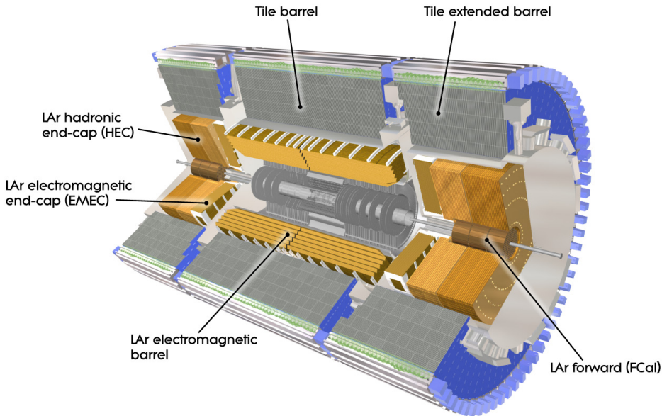
Figure 2.10: Illustration of ATLAS Calorimeters system [8].
