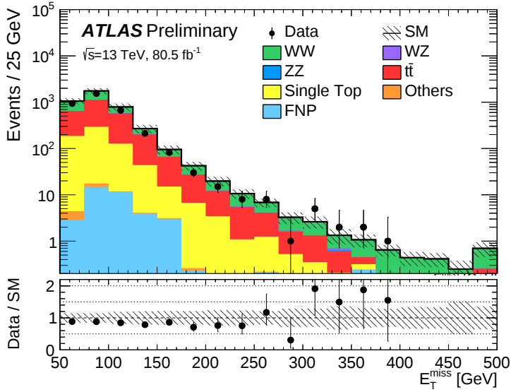
(b) E_T^{miss} in VR-WW-1J
