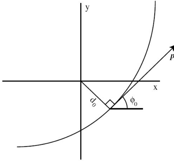
Figure 4.1: Track parameter definitions at the perigee. Taken from [15].
