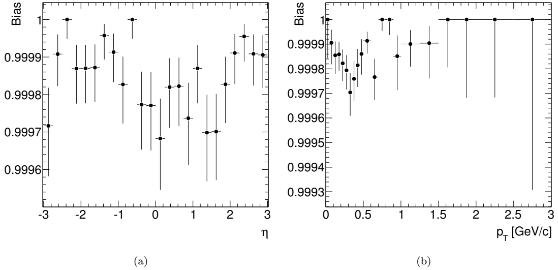
Figure 3.5: Bias of the MBTS_2 trigger as a function of \eta (a) and p_T (b) for the simulated inelastic event sample described in Appendix A. The \eta plot is integrated over p_T > 0.15 GeV/c and the p_T plot is integrated over |\eta| < 2.5 .
