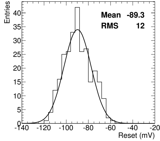
Figure C.3: Difference of voltage measured at PP1 and expected voltage at the SC-OLink for Opto_-Reset channels. Measurements at PP1 are made with the Service Test hardware. The expected voltage of 2.5 V is used here since no measurement is made by the SC-OLink for this channel. The distribution has been fit with a Gaussian function.
