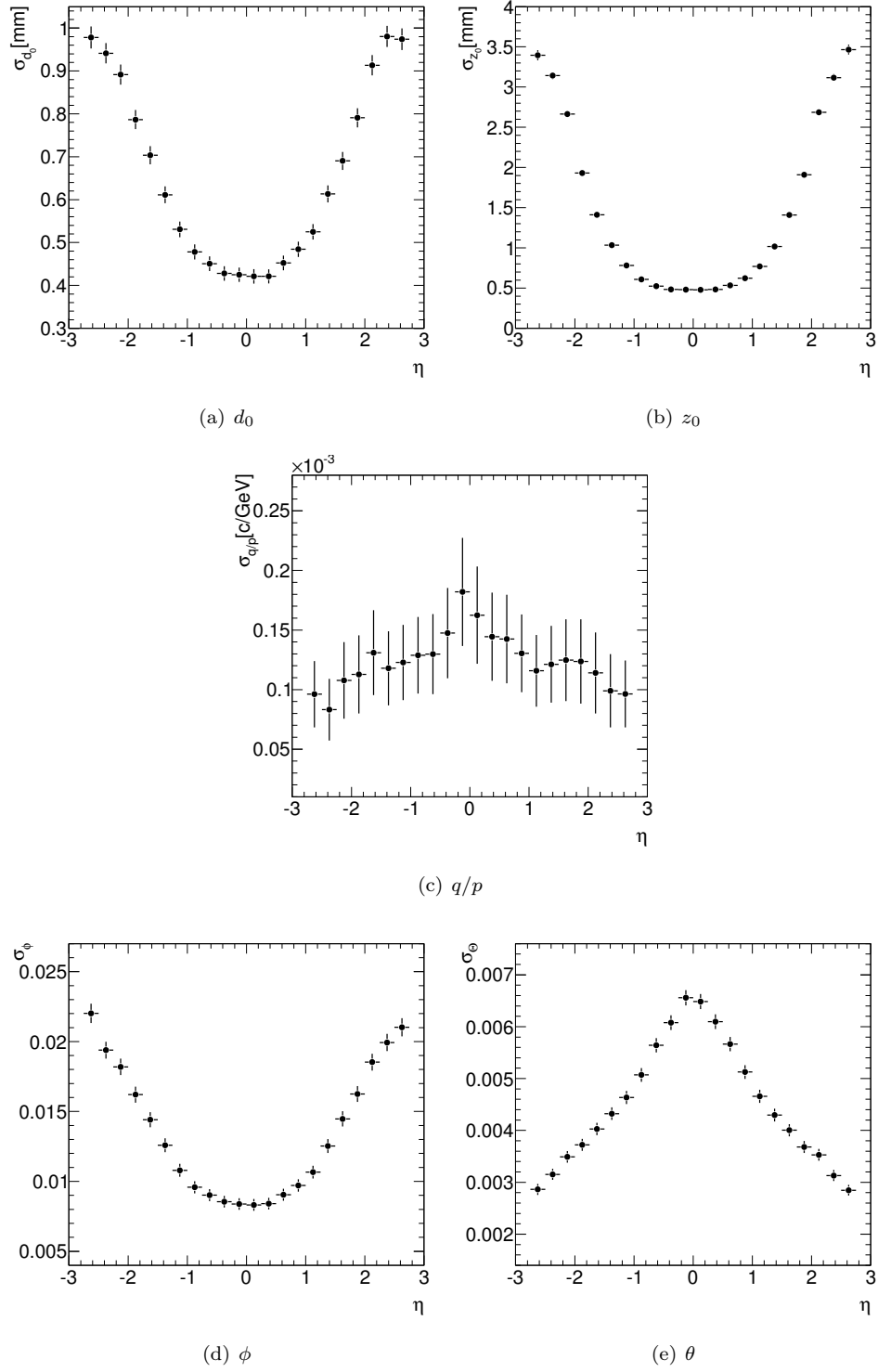
Figure 5.1: Resolutions of the track parameters versus \eta for the minimum bias event sample, integrated over p_T > 0.15 GeV/c. TRT stand-alone tracks have been excluded. Resolutions are calculated over a range which includes 99.7% of the data (corresponding to \pm 3\sigma ).
