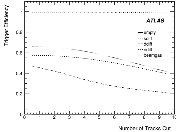
Figure 3.2: Trigger efficiency at the Event Filter versus the number of reconstructed tracks with z_0 < 200 mm, for various physics processes simulated at \sqrt{s} = 14 TeV satisfying the Level-2 spacepoint requirement. Taken from [3].
