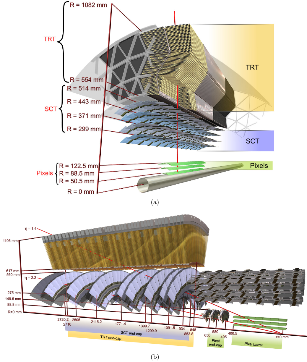
Figure 1.5: (a) Sensors and structural elements traversed by a charged track with p_T = 10 GeV/ c in the Inner Detector barrel ( \eta = 0.3 ). The track successively traverses the beam-pipe, the three barrel layers of the pixel detector, the four double layers of the barrel SCT and approximately 36 axial straws contained in the barrel TRT. Taken from [6]. (b) Sensors and structural elements traversed by two charged tracks with p_T = 10 GeV/ c in the Inner Detector end-cap ( \eta = 1.4 and \eta = 2.2 ). The end-cap track at \eta = 1.4 successively traverses the beam-pipe, the three barrel layers of the pixel detector, four of the double-layered SCT end-cap disks and approximately 40 straws contained in the TRT end-cap wheels. In contrast, the track at \eta = 2.2 traverses only the first of the barrel pixel layers, two end-cap pixel disks and the last four disks of the end-cap SCT. The coverage of the end-cap TRT does not extend beyond |\eta| = 2 . Taken from [6].
