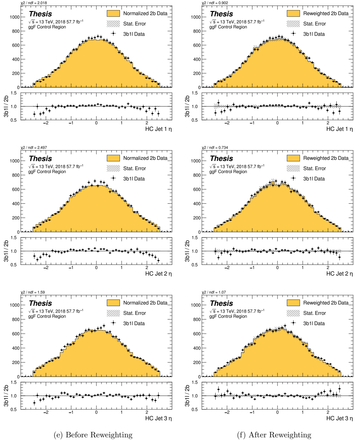
Figure 8.23: Non-resonant Search (3b1l) : Distributions of \eta of the 1st, 2nd, and 3rd leading Higgs Candidate jets before (left) and after (right) CR derived reweighting for the 2018 3b1l Control Region.
