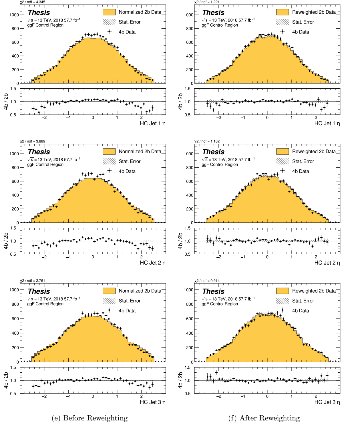
Figure 8.14: Non-resonant Search (4b): Distributions of \eta of the 1st, 2nd, and 3rd leading Higgs Candidate jets before (left) and after (right) CR derived reweighting for the 2018 4b Control Region.
