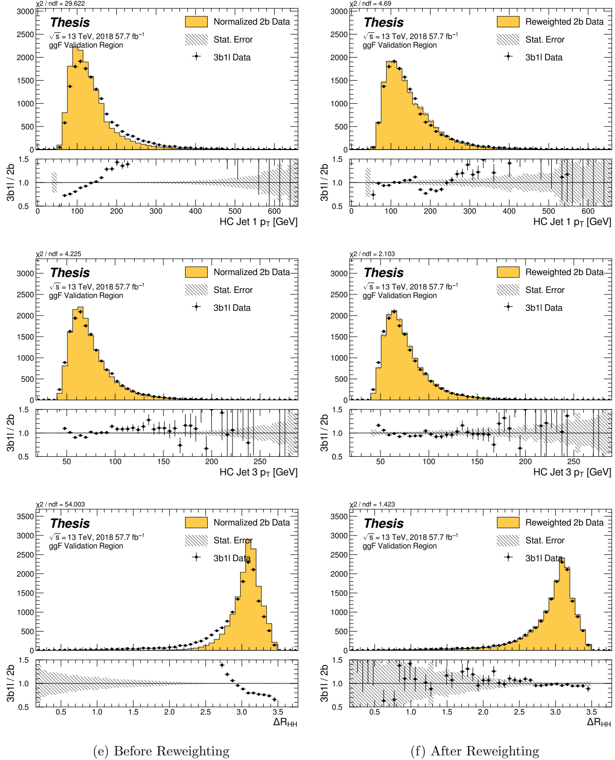
Figure C.22: Non-resonant Search (3b1l) : Distributions of p_T of the 1st and 3rd leading Higgs Candidate jets and \Delta R between Higgs candidates before (left) and after (right) CR derived reweighting for the 2018 3b1l Validation Region.
