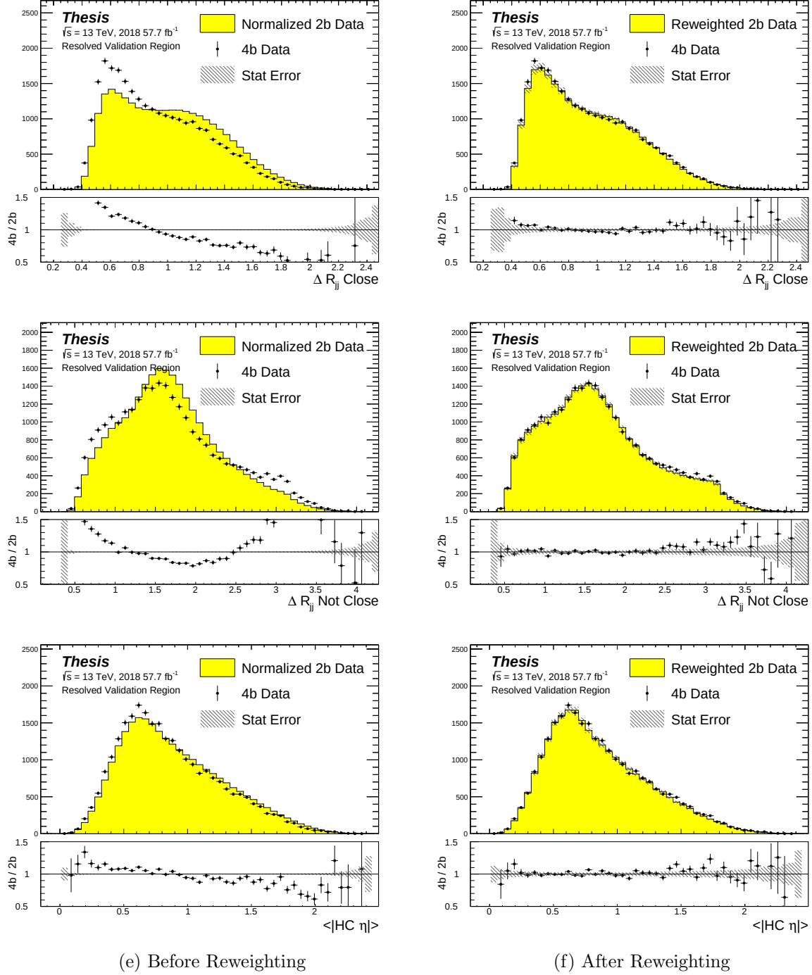
Figure C.1: Resonant Search: Distributions of \Delta R between the closest Higgs Candidate jets, \Delta R between the other two, and average absolute value of HC jet \eta before (left) and after (right) CR derived reweighting for the 2018 Validation Region.
