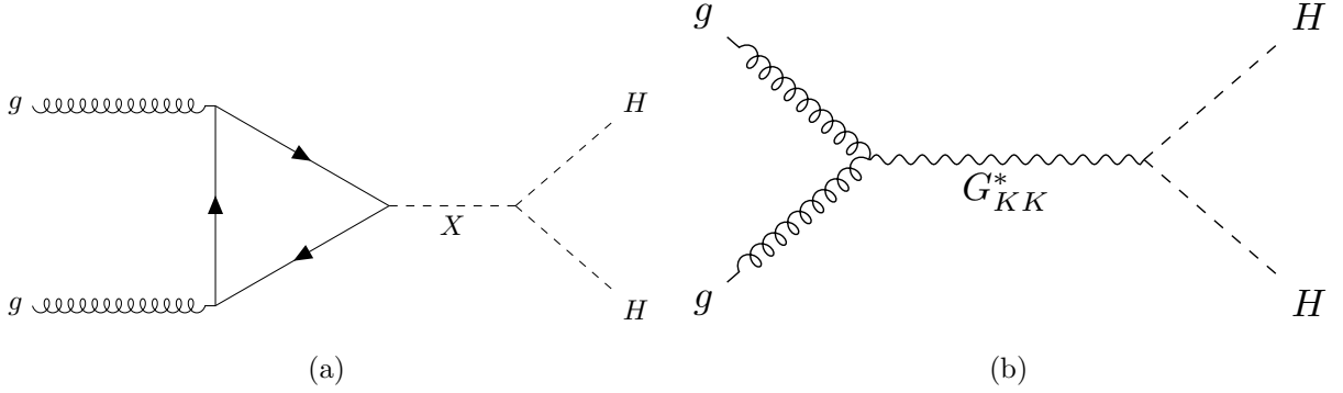
Figure 2.1: Representative diagrams for the gluon-gluon fusion production of spin-0 ( X ) and spin-2 ( G_{KK}^* ) resonances which decay to two Standard Model Higgs bosons. The spin-0 resonance considered for this thesis is a generic narrow width resonance which may be interpreted in the context of two Higgs doublet models [23], whereas the spin-2 resonance is considered as a Kaluza-Klein graviton within the bulk Randall-Sundrum (RS) model [24, 25].
