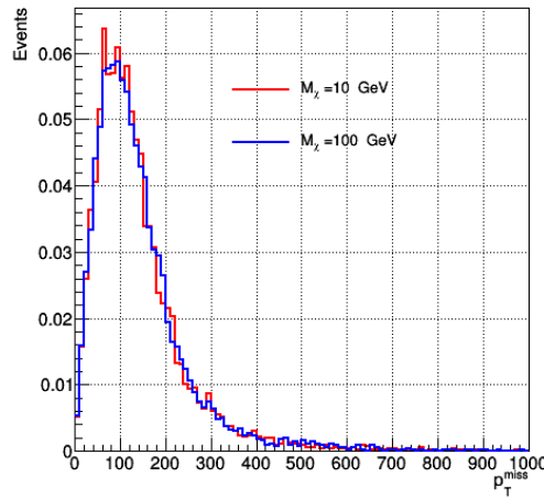
Figure 5.5: p_T^{\text{miss}} distributions for signal samples with varying the mass of the DM particle.
