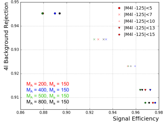
Figure 6.4: Signal efficiency vrs. background rejection for applying different cuts on the 4 leptons invariant mass.
