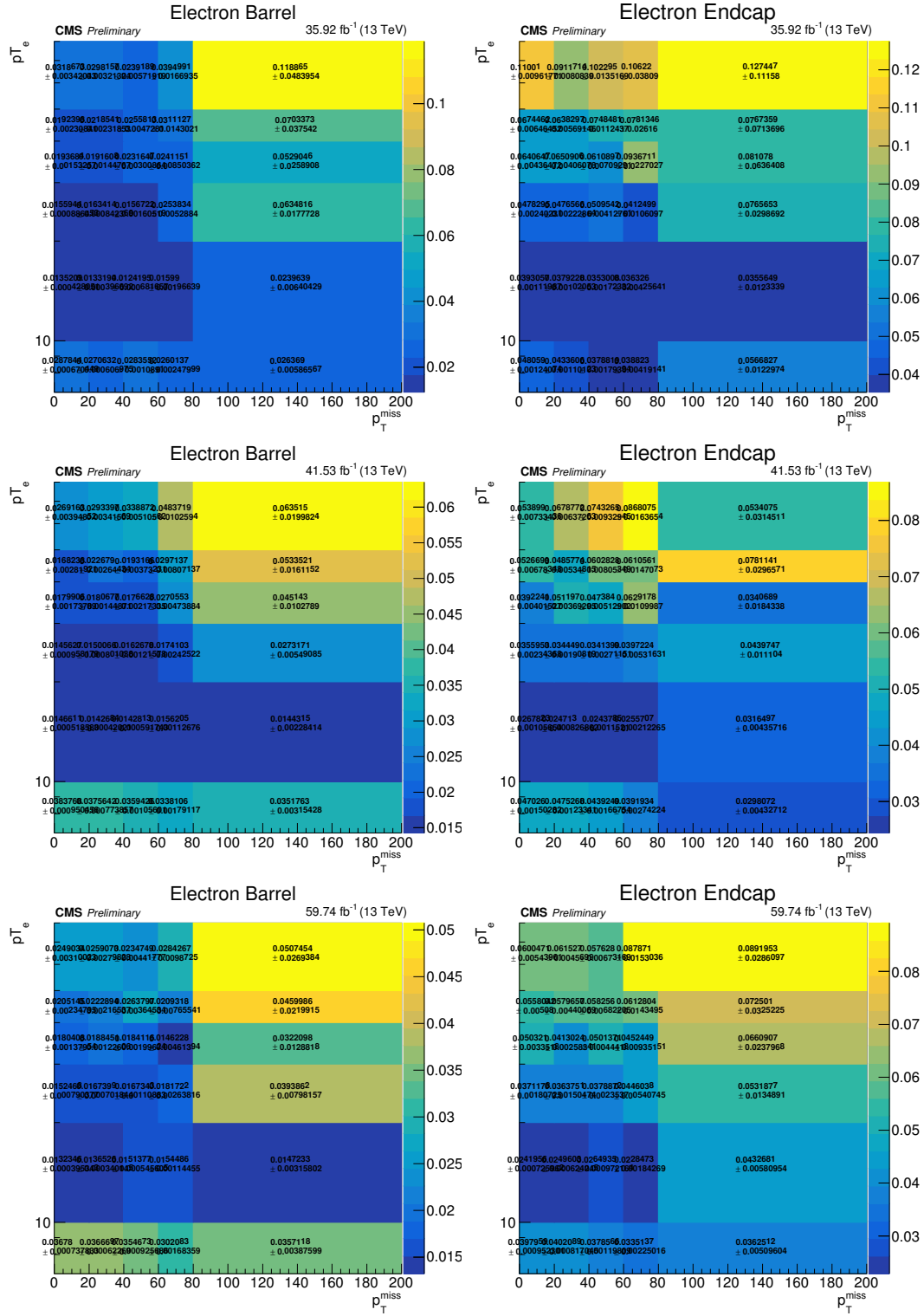
Figure 6.18: Electron fake rate measured as a function of electron's p_T^l and the p_T^{\text{miss}} in barrel (left) and endcap (right) regions for 2016 (top), 2017 (middle) and 2018 (bottom) datasets.
