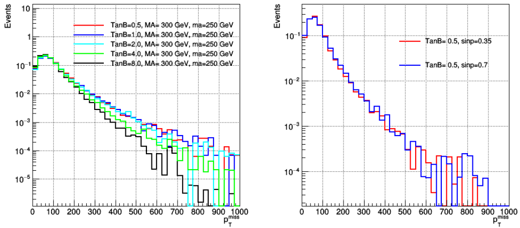
Figure 5.4: p_T^{miss} distributions for signal samples with varying the \tan\beta value (left) and the \sin\theta value (right).
