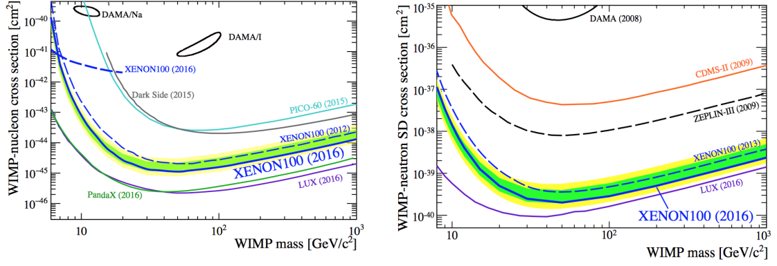
Figure 1.9: Shows cross section limits as a function of the DM mass spin-independent (left) and spin dependent (right) interactions for various experiments [6].
