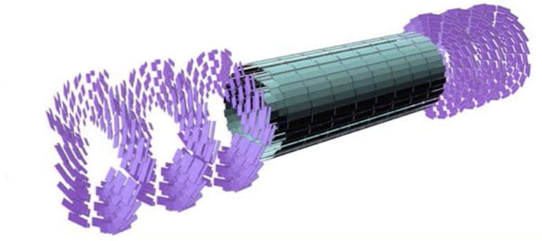
Figure 2.11: View of the CMS silicon pixel sub-detector geometry. In the middle there are three layers of the barrel pixels, and on either end of the barrel are two end-cap disks [17].
