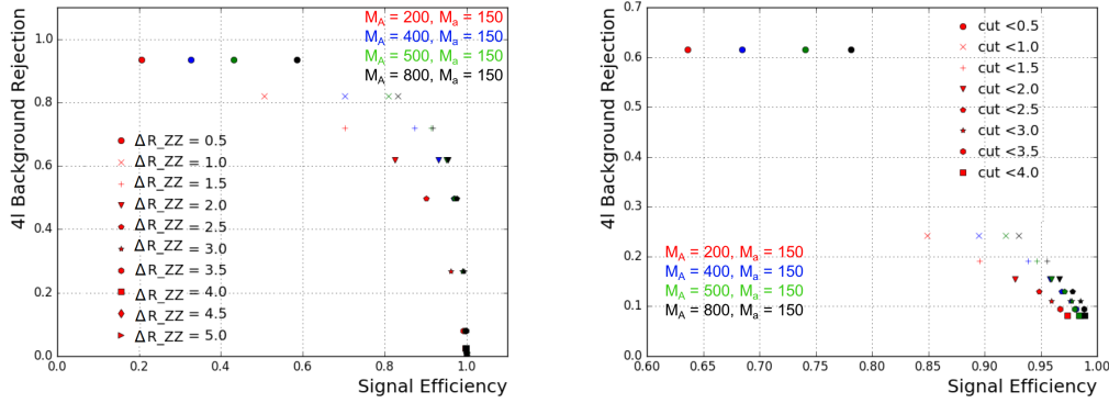
Figure 6.10: Signal efficiency vrs. background rejection for applying different cuts on the \Delta R between the two Z 's coming from the Higgs decay (left) and cuts on |\frac{p_T^{\text{miss}} - p_T^{4l}}{p_T^{4l}}| quantity (right).
