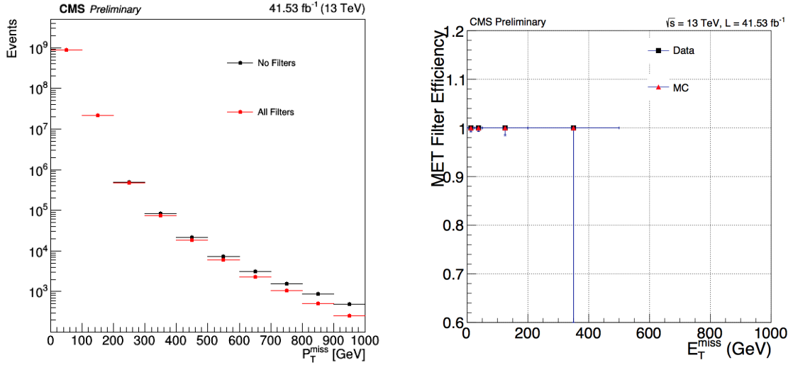
Figure 5.22: Shows the MET distribution before and after applying the MET filters (left), MET filters efficiency as a function of MET distribution after reconstruction of Higgs boson from four charged leptons (right) using dataset recorded in 2017.
