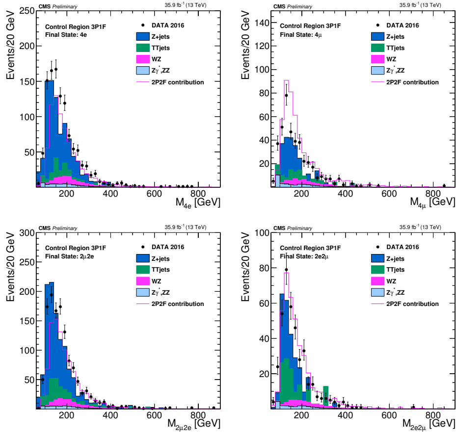
Figure 6.21: Invariant mass distribution of the events populated in the 3P+1F control sample in the 2016 dataset for 4e (top left), 4μ (top right), 2μ2e (bottom left) and 2e2μ (bottom right).
