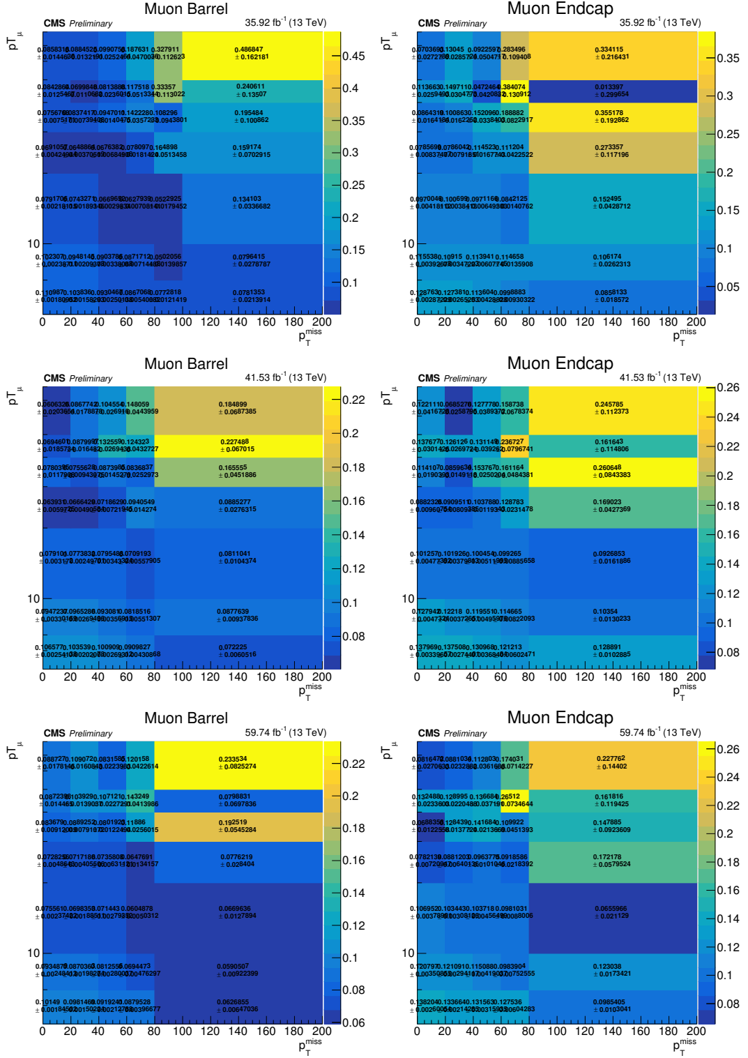
Figure 6.19: Muon fake rate measured as a function of muon's p_T^l and the p_T^{\text{miss}} in barrel (left) and endcap (right) regions for 2016 (top), 2017 (middle) and 2018 (bottom) datasets.
