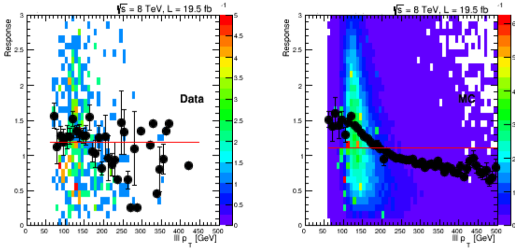
FIGURE 6.15: \mu\mu + e channel. Calibrated response for about 25% for both of data and MC.
