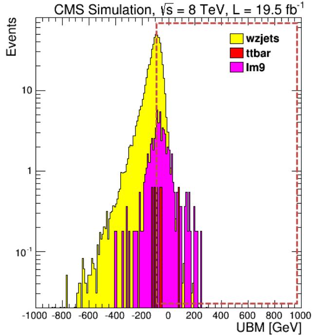
FIGURE 6.3: UBM distribution with \mu\mu + e in WZ+jets, t\bar{t} and SUSY MC simulation, scaled to 19.5 \text{ fb}^{-1} . The asymmetric distribution shows the SM dominant regions on left side and the signal dominant region on right side.
