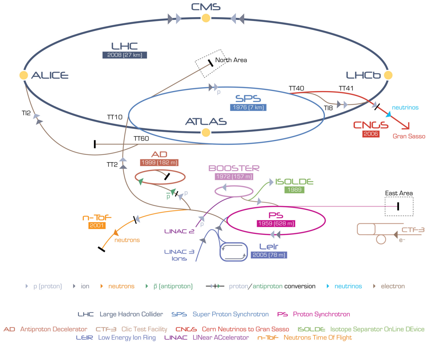
Figure 3.1: Layout of accelerators and detectors at CERN [16].
