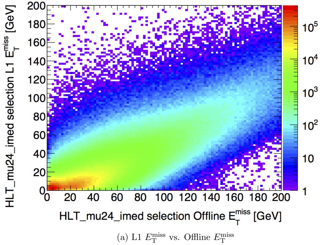
Figure 6.6: Correlations with L1 E_T^{\text{miss}} in events passing the HLT_mu24_imedium trigger.
