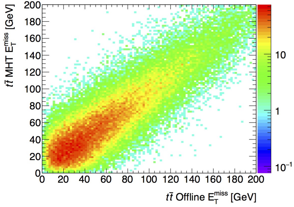
(c) H_T^{\text{miss}}
