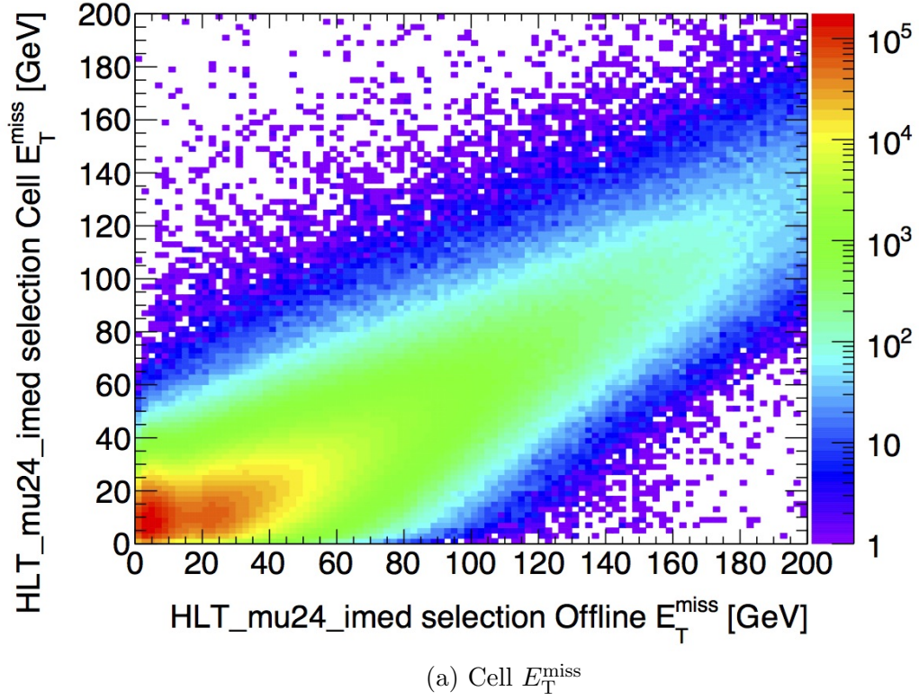
Figure 6.5: Correlations between trigger E_T^{\text{miss}} and offline E_T^{\text{miss}} in events passing the HLT_mu24_imedium trigger.
