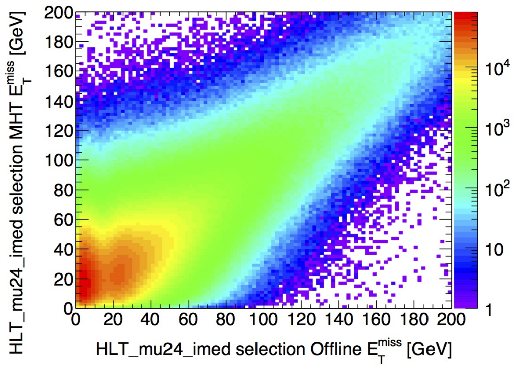
(e) H_T^{\text{miss}}
