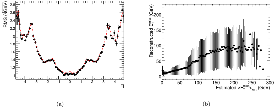
FIGURE 3.2: (a) \lambda(E)_{RMS} versus \eta_j for fully simulated QCD jets in the kinematic range 35\text{GeV} < p_T < 1120\text{GeV} . (b) Correlation between estimated \langle \cancel{E}_T \rangle and reconstructed \cancel{E}_T .
