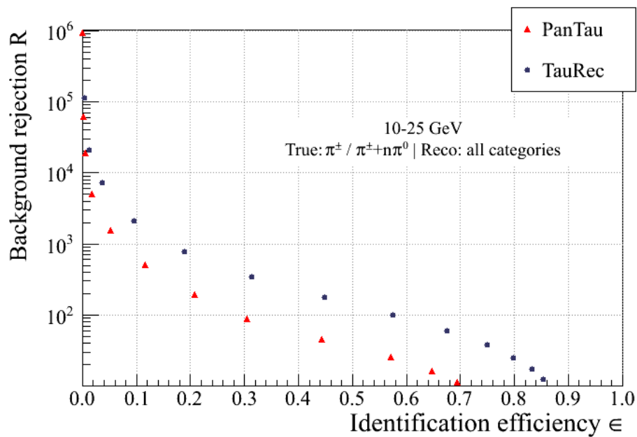
(a) 10-25 GeV
