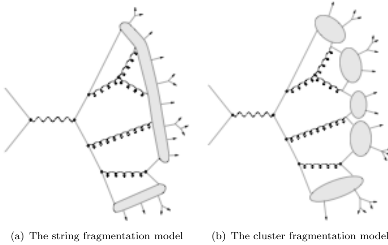
FIGURE 1.6: Schematic representation of hadronization models [21].
