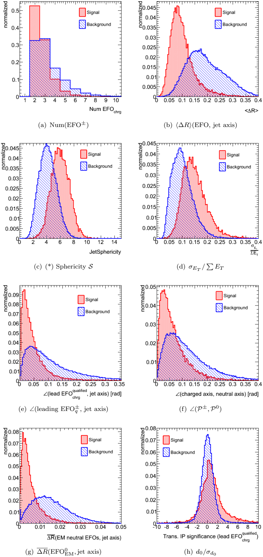
FIGURE 2.33: Feature distributions: 2-prong+neutral, 10 \text{ GeV} < p_T^{\text{seed}} < 25 \text{ GeV} , ( |\eta^{\text{seed}}| < 2.0 ). Distributions marked with an (*) have been transformed with an inverse sigmoid function.
