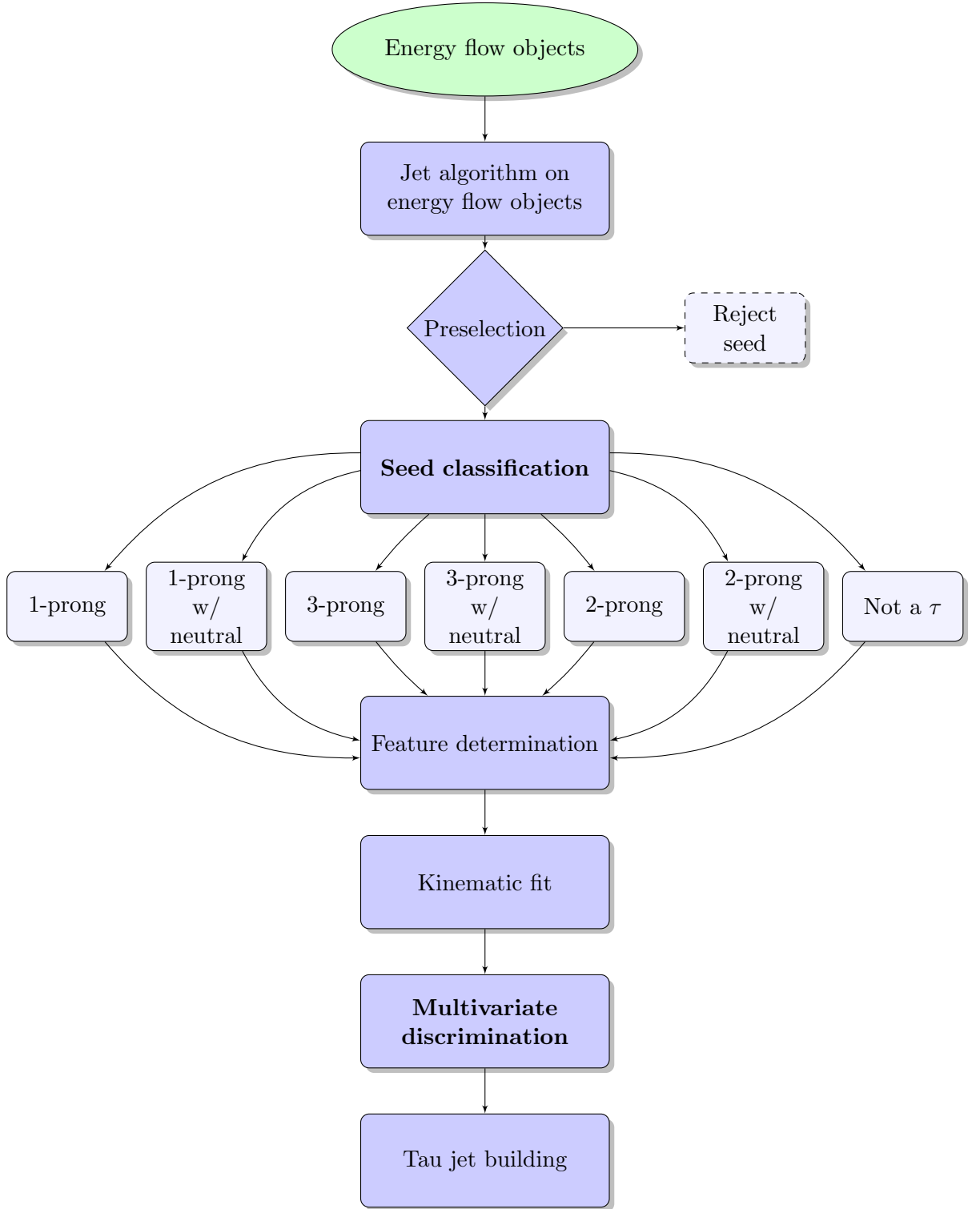
FIGURE 2.11: Data flow in PanTau: EFOs form the raw input to the algorithm. These are collected by a jet algorithm to form \tau -seeds. The seeds are subsequently classified according to content, if found to satisfy a basic preselection. (Seeds classified as 2-prong or 2-prong w/neutral have two \text{EFO}_q^\pm .) After classification, properties of the seeds are derived from the constituent objects and fed into a multivariate discriminant to facilitate the separation of QCD-induced fakes.
