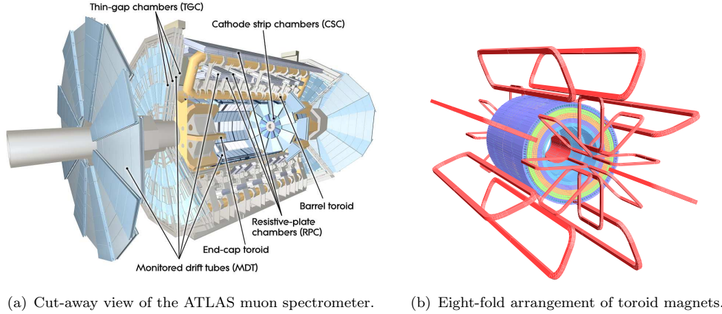
FIGURE 1.16: The ATLAS muon spectrometer [37].
