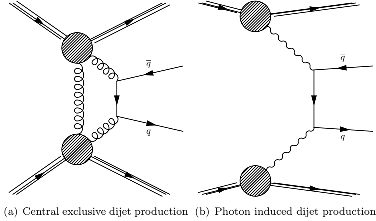
FIGURE 4.12: Diagram for exclusive jet production at the LHC.
