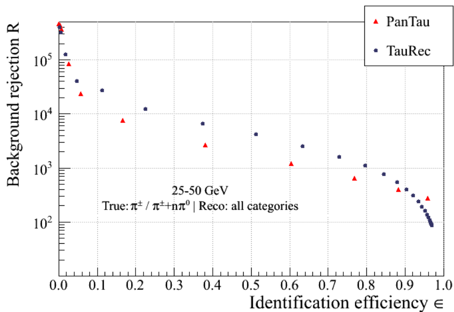
(b) 25-50 GeV
