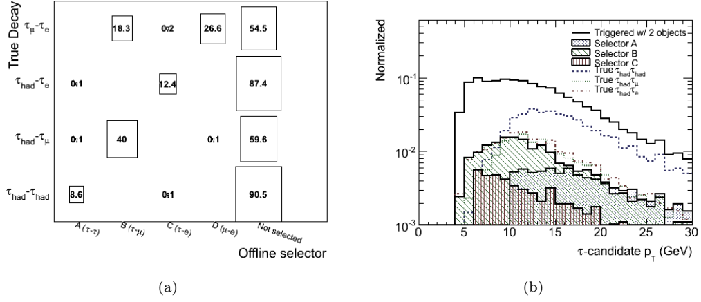
FIGURE 4.14: (a) The fraction of true decays satisfying p_T^{vis}(\tau_{\text{had}}) > 10 GeV and/or p_T^{vis}(\tau_{\text{lep}}) > 4 GeV, selected by each offline selector after online trigger selection. (b) Transverse momentum spectrum of \tau -candidates in the subset of the triggered signal with exactly two reconstructed objects along with the subsets selected by Selectors A-C. The subsets corresponding to true p_T(\tau_{\text{had}}) > 10 GeV and p_T(\tau_{\text{lep}}) > 4 GeV are also shown for \gamma\gamma \rightarrow \tau_{\text{had}}\tau_{\text{had}} , \gamma\gamma \rightarrow \tau_{\text{had}}\tau_\mu and \gamma\gamma \rightarrow \tau_{\text{had}}\tau_e decays. Selector B is seen to be the only selector with a good efficiency with respect to the target process across the full spectrum.
