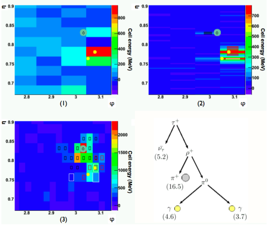
FIGURE 2.7: Topological clustering in the first three layers of the electromagnetic calorimeters: (1) presampler, (2) \eta -strip layer and (3) middle layer (ref. Figure 1.15(a)). The true \pi^\pm is marked as grey dot, the two photons emerging from the decay \pi^0 \rightarrow \gamma\gamma by two yellow dots. The track associated with the \pi^\pm is marked by a diamond. The cells forming part of a topocluster are marked by coloured rectangles. A separation of the \pi^\pm shower (black cluster) from the \pi^0 shower in (red cluster) is achieved, despite a small spatial separation. In the finely segmented \eta -strip layer, the individual photons are resolved.
