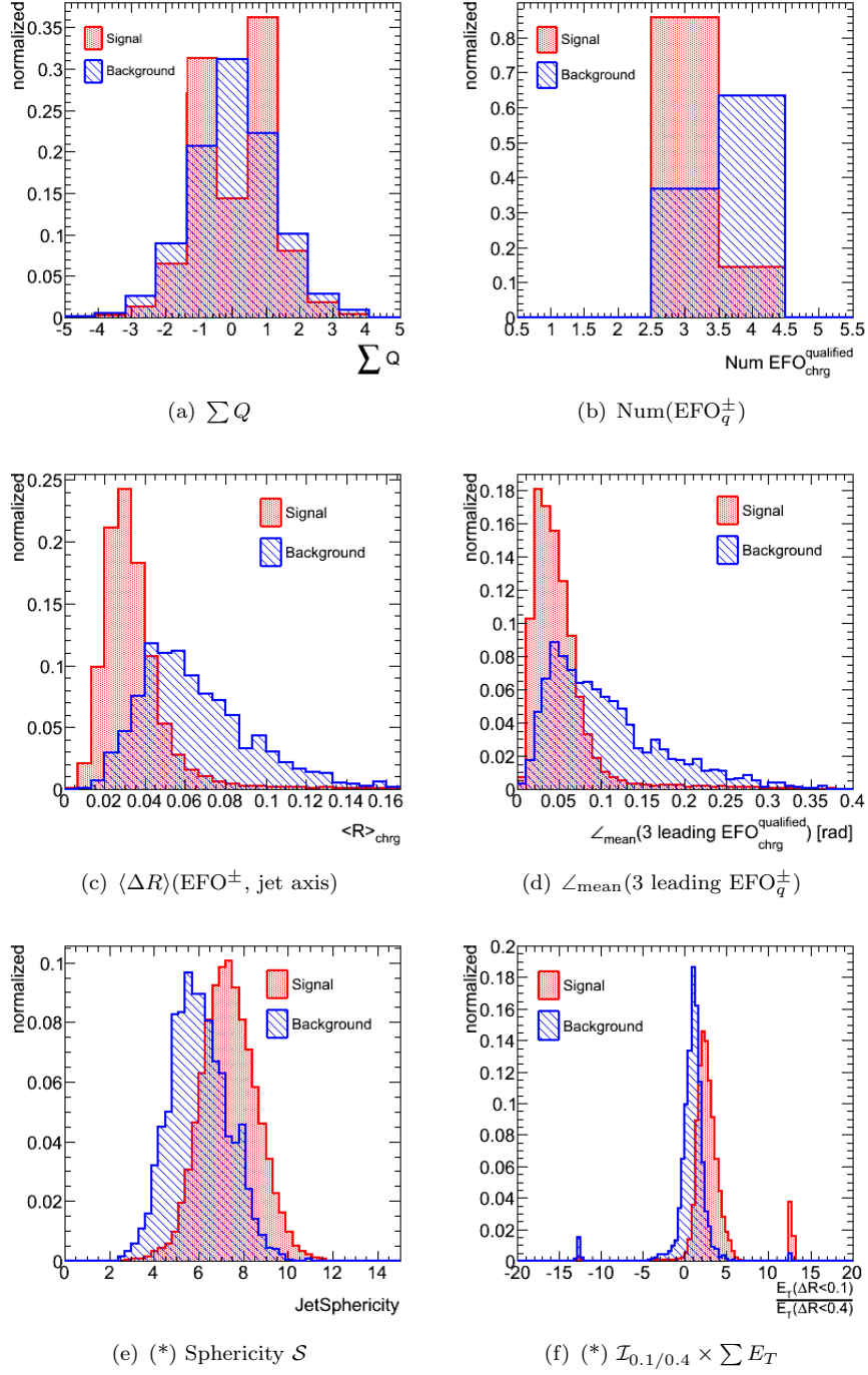
FIGURE 2.29: Feature distributions: 3-prong, 25 \text{ GeV} < p_T^{\text{seed}} < 50 \text{ GeV} , (|\eta^{\text{seed}}| < 2.0) . Distributions marked with an (*) have been transformed with an inverse sigmoid function.
