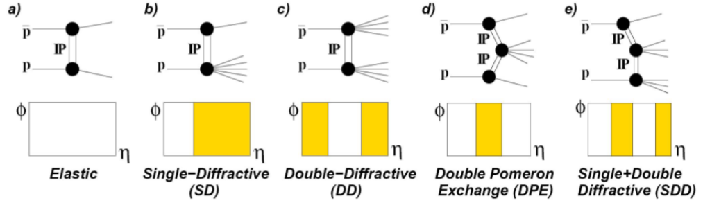
FIGURE 1.10: Various soft elastic and inelastic scattering processes, with corresponding event topologies in \eta - \phi space, whereby coloured regions indicate particle activity and empty regions rapidity gaps [34].
