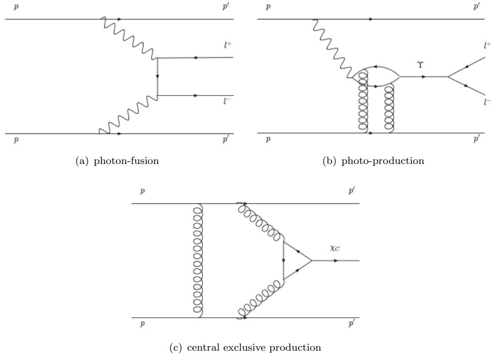
FIGURE 4.7: Diagrams of various exclusive processes with lepton final states (to which the MV-trigger items are expected to retain sensitivity).
