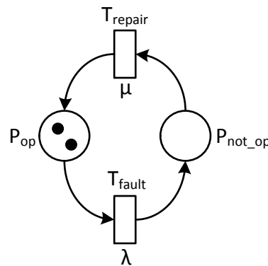
Figure 16 Petri net for reliability modeling
