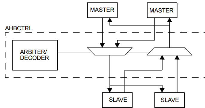
Figure 21 AMBA AHB controller functional block diagram [103]
