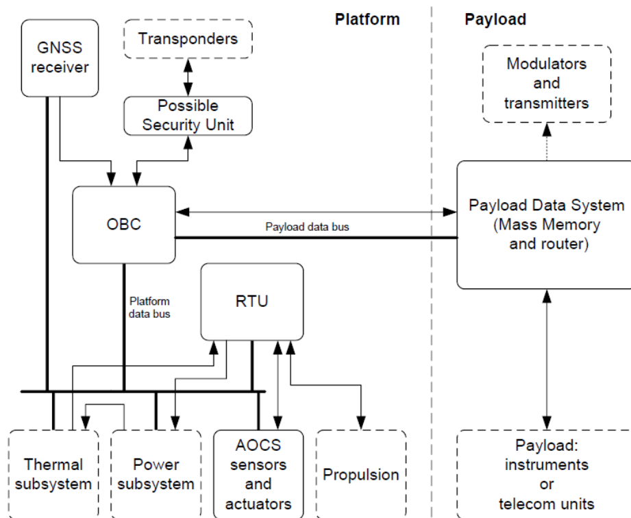
Figure 6 Typical modern hi-end satellite avionics architecture [10]
