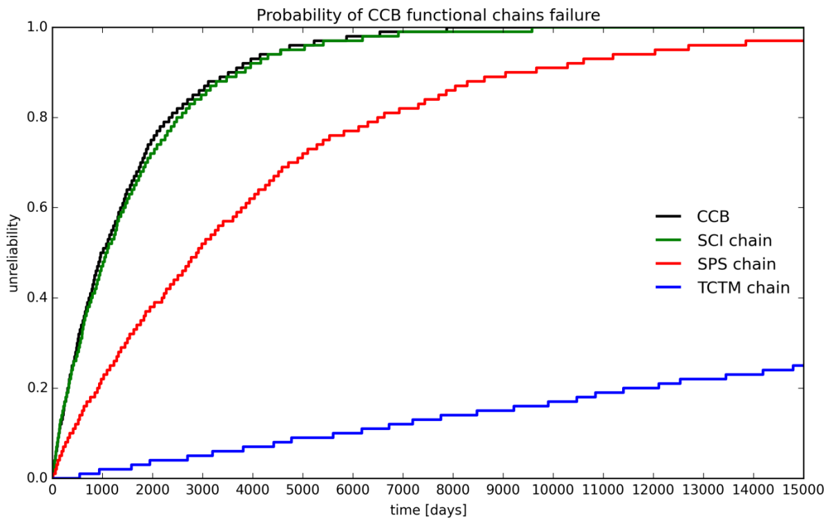
Figure 50 Petri Nets simulation result for CCB DPU chains
