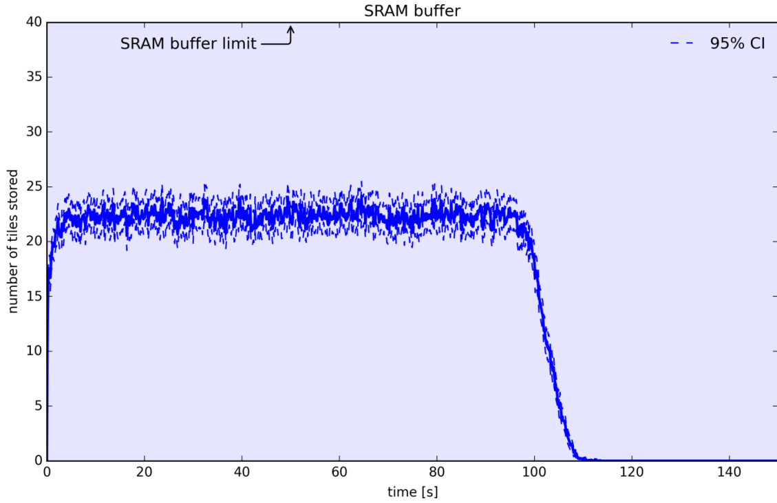
Figure 43 Simulated tiles pile-up in SRAM (N=10000, T8=1.00E-01, T9=1.00E-01, AMBA_blocking_ratio=50%, compression-off configuration)
