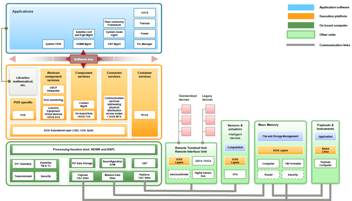
Figure 3 SAVOIR avionic architecture [10]
