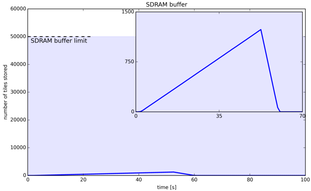
Figure 39 Simulated tiles pile-up in SDRAM (N=10000, T_8=1.00E-04 , T_9=1.11E-05 , AMBA_blocking_ratio=10%, compression-off configuration)
