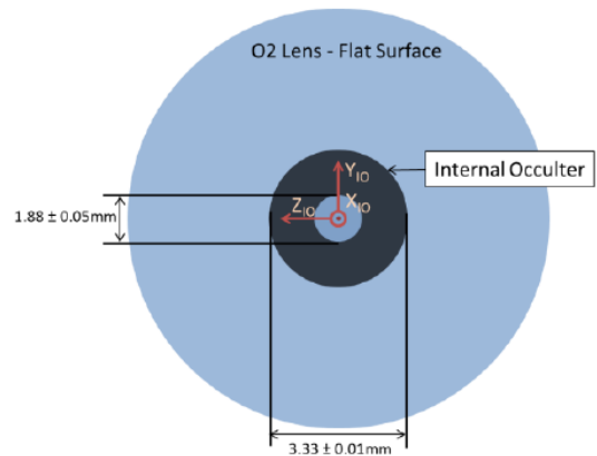
Figure 59 IO design (typical dimensions)
