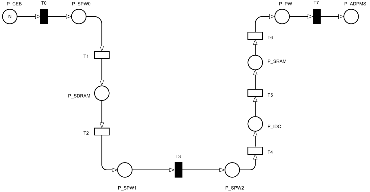
Figure 32 DPU pipeline model expressed as Petri net.
