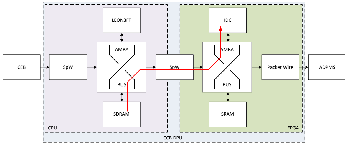
Figure 24 System data transfer: SDRAM - SpaceWire - IDC
