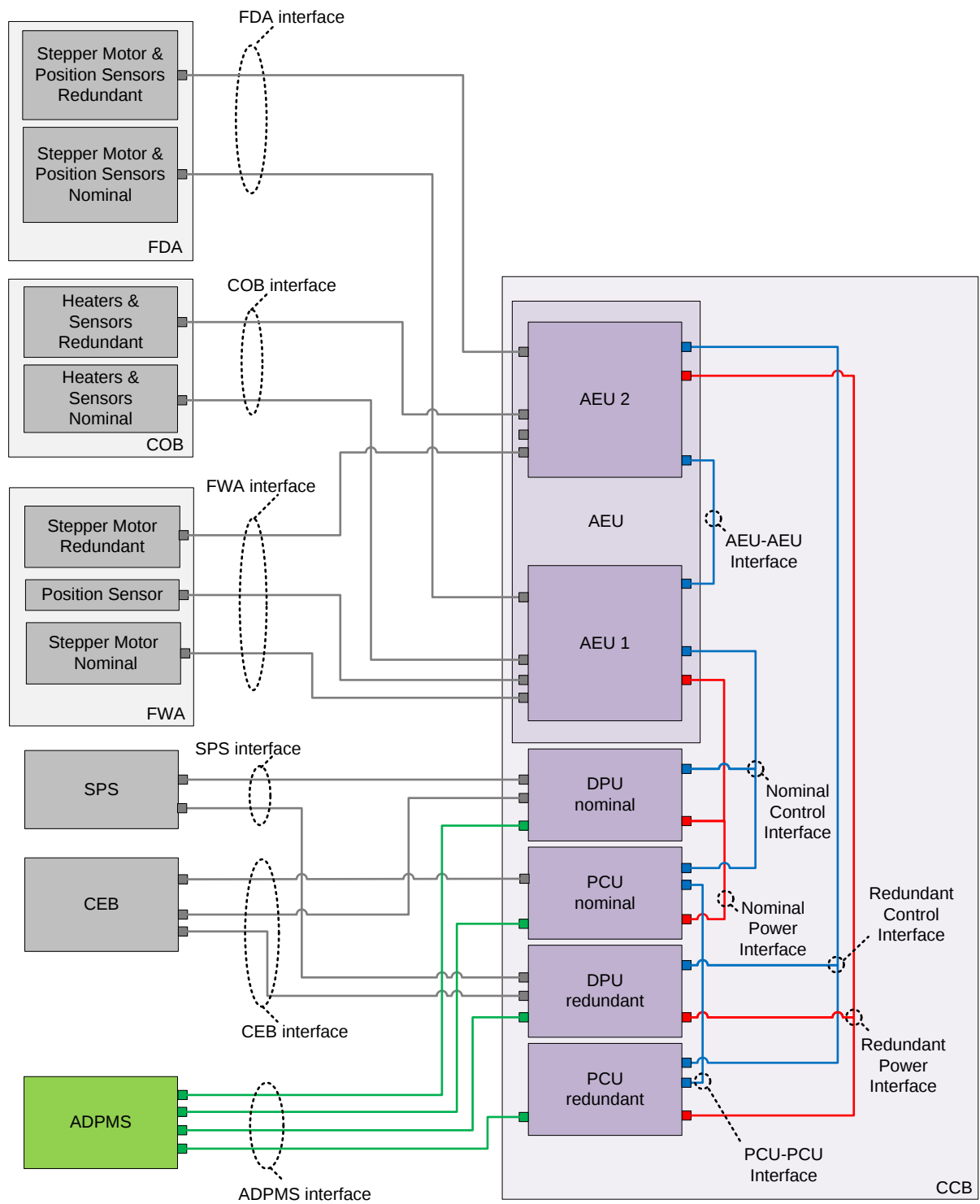
Figure 19 CCB architecture
