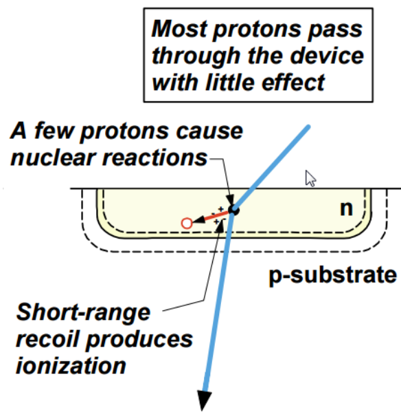
Figure 9 Indirect semiconductor ionization [39]
