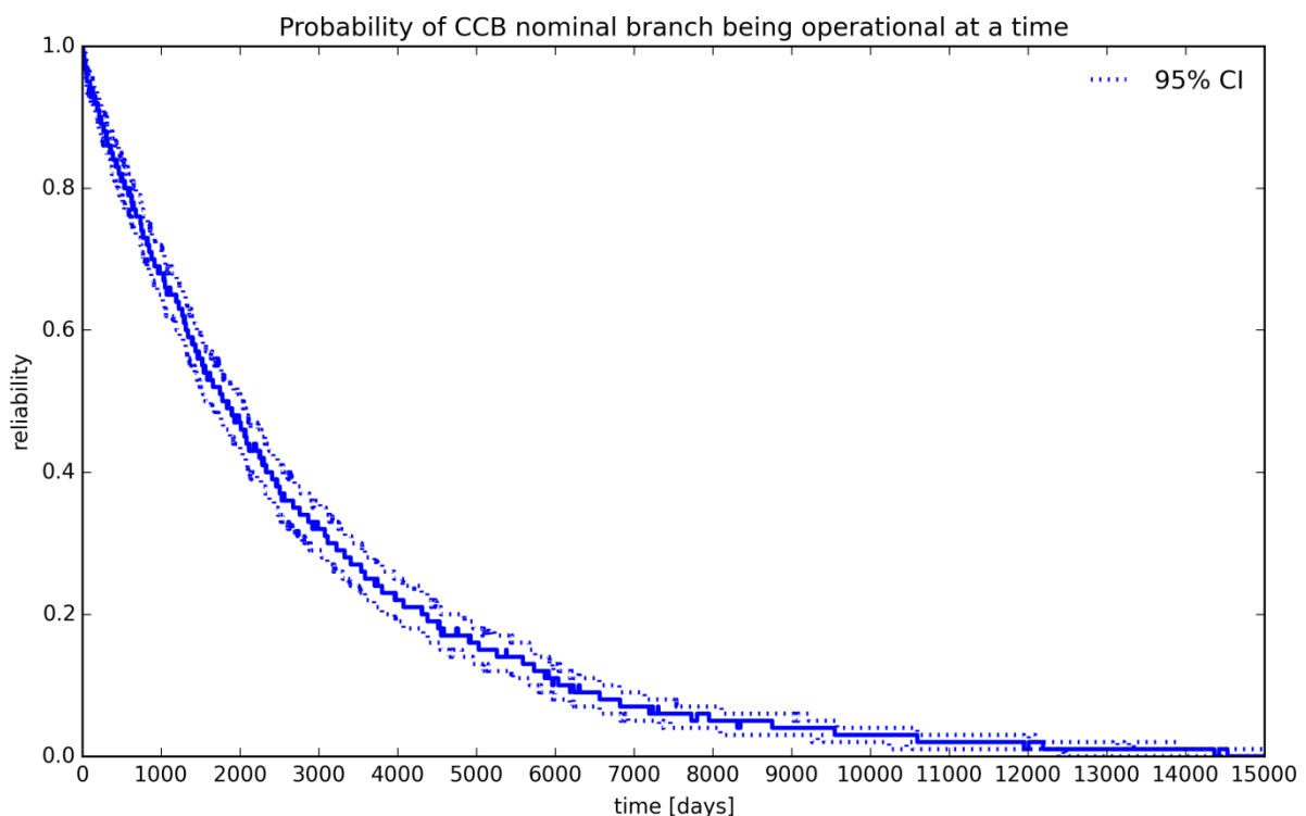
Figure 52 Petri Net simulation of CCB nominal branch reliability
