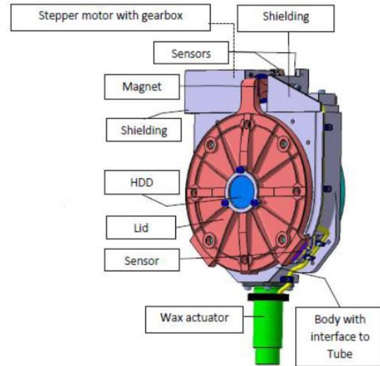
Figure 64 Front Door Assembly (FDA)
