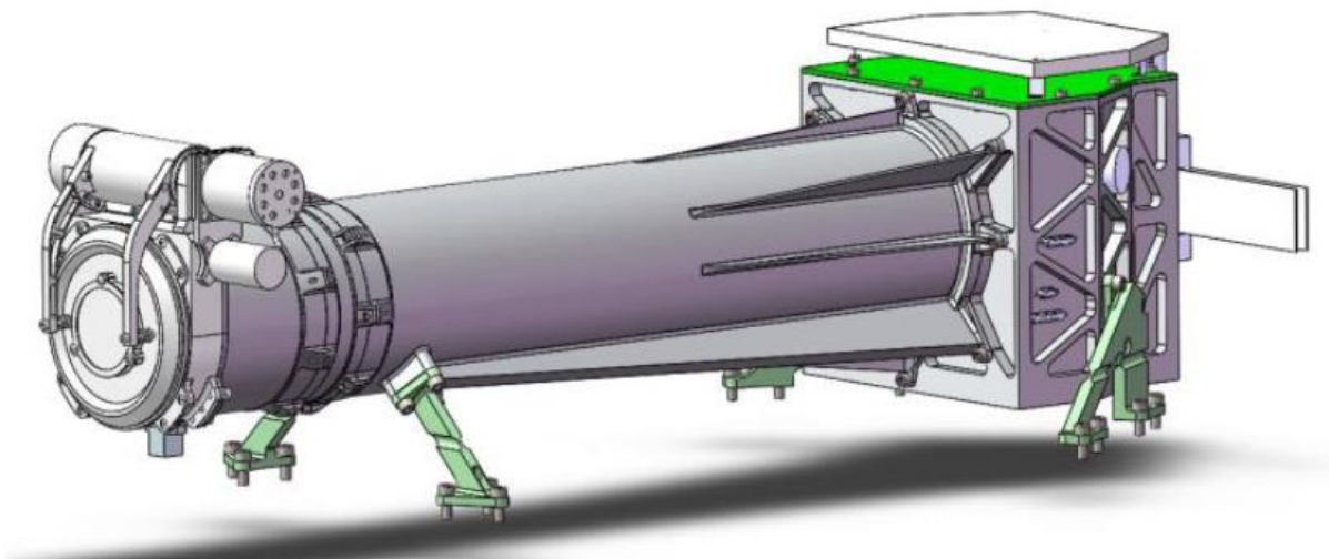
Figure 62 Coronagraph COB overview.
