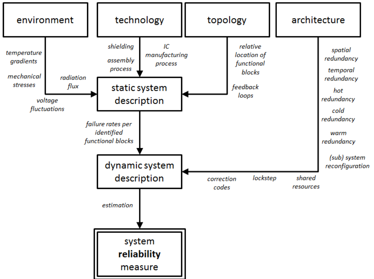
Figure 28 Generic system reliability modeling methodology
