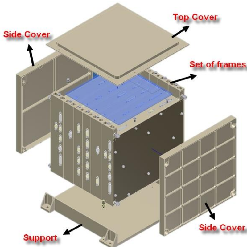
Figure 69 Coronagraph Control Box (CCB) housing
