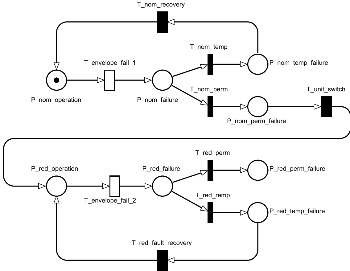
Figure 51 Petri Net modeling CCB DPU redundancy
