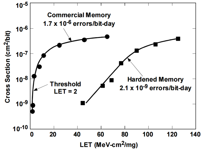
Figure 10 Example commercial and radiation-hardened device cross-sections [39].
