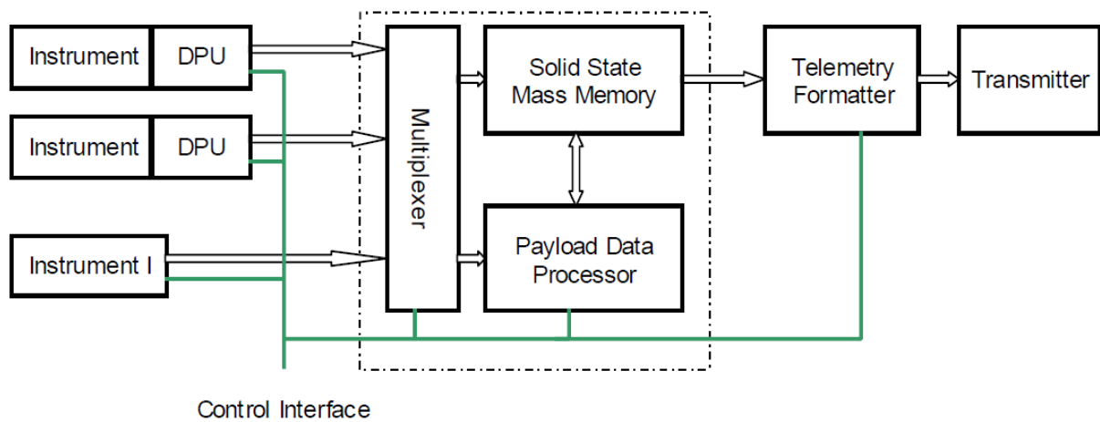
Figure 4 Multi-pipeline architecture scientific class avionics [11]
