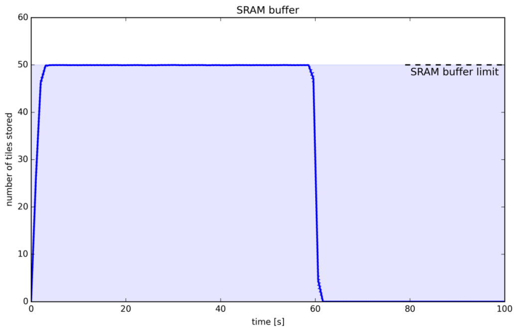
Figure 40 Simulated tiles pile-up in SRAM (N=10000, T_8=1.00E-04 , T_9=1.11E-05 , AMBA_blocking_ratio=10%, compression-off configuration)
