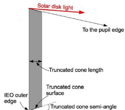
Figure 65 EO geometry
