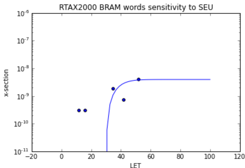
Figure 74 RTAX2000 BRAM 8bit EDAC word SEU cross-section [120]
