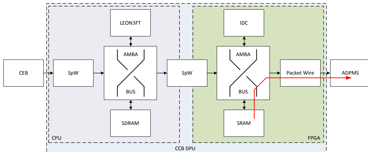
Figure 25 System data transfer: SRAM - PacketWire -ADPMS
