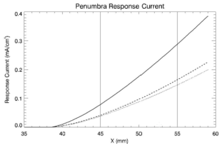
Figure 67 SPS response current in the penumbra on the entrance pupil plane as a function of the distance from the telescope optical axis.
