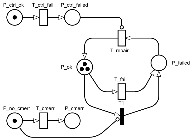
Figure 18 Complex Petri Net example (GSPN)
