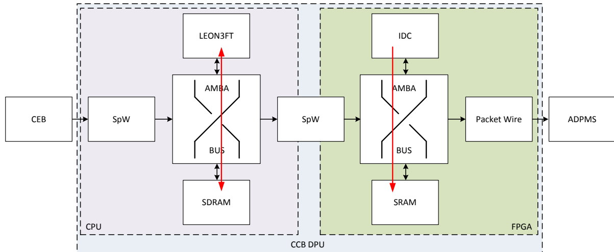
Figure 23 System data transfer: tile processing and IDC - SRAM
