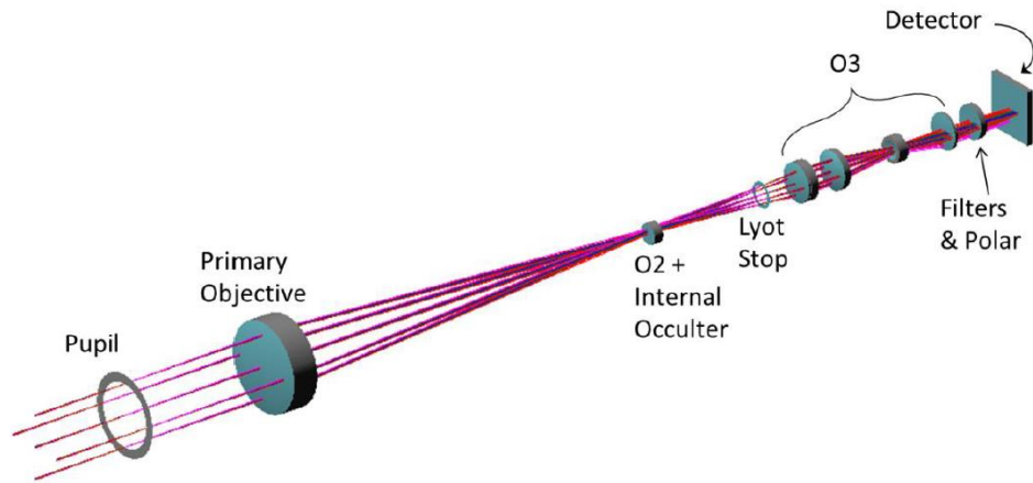
Figure 57 Coronagraph System Lens Objectives
