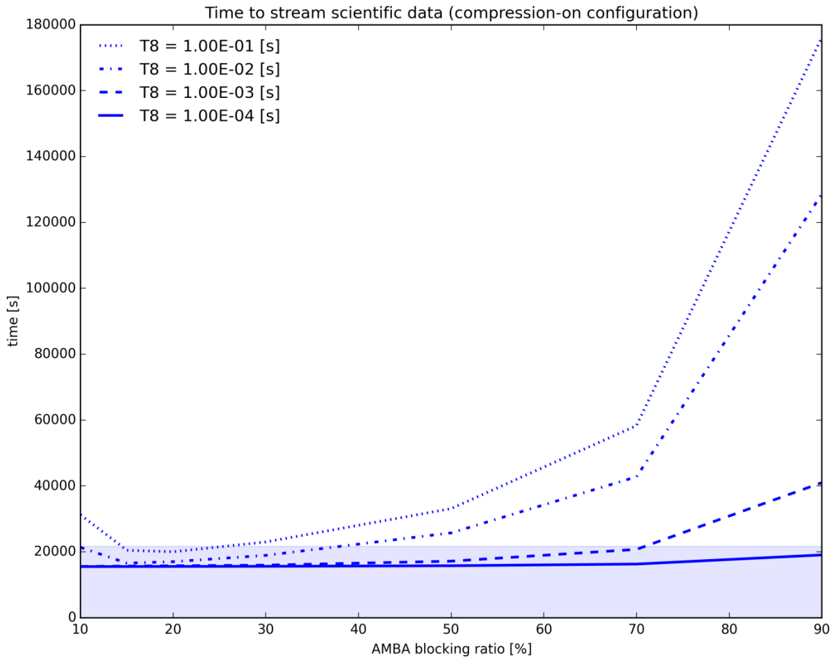
Figure 35 Simulated time to send all tiles of CME-watch observation program for final model, compression-on
