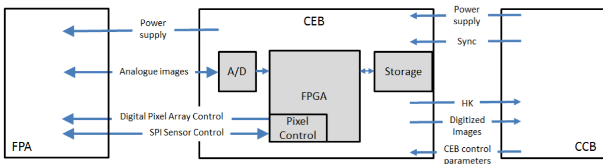
Figure 61 CEB functional diagram
