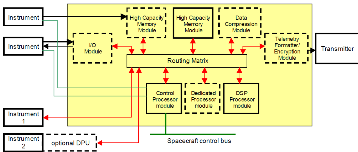
Figure 5 Reconfigurable architecture scientific class avionics [11]
