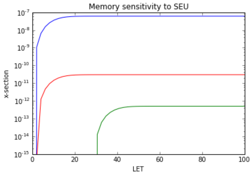
Figure 75 Memories bit SEU cross-sections
