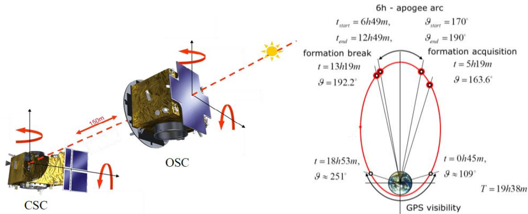
Figure 55 PROBA-3 formation flying overview and orbit
