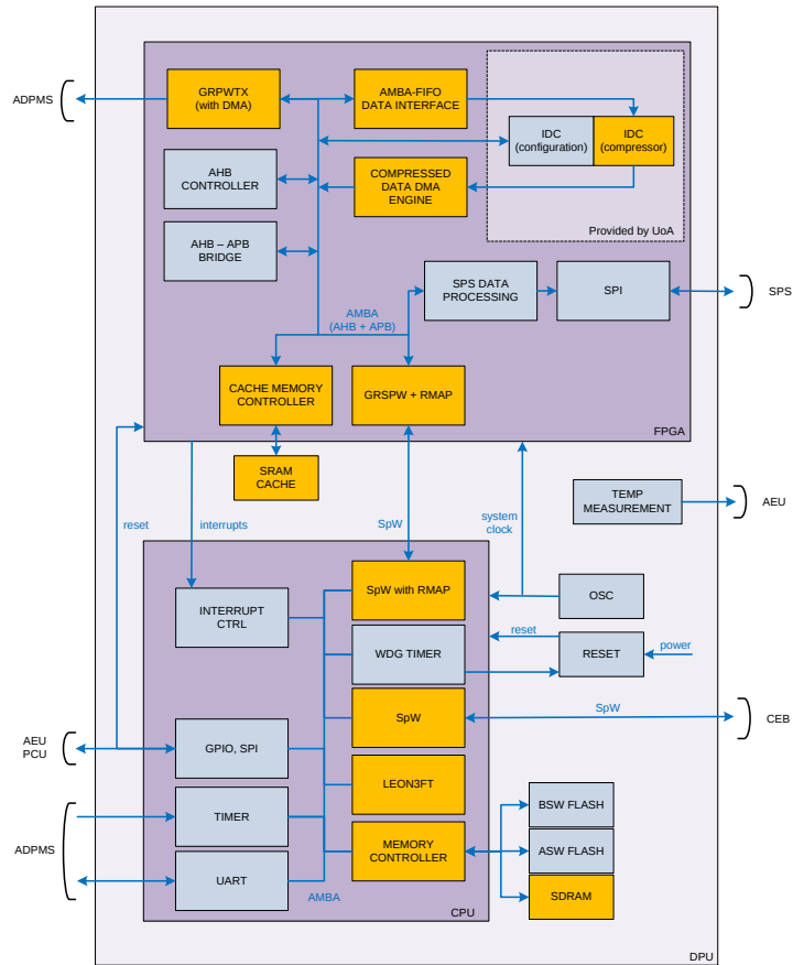
Figure 46 Science data chain
