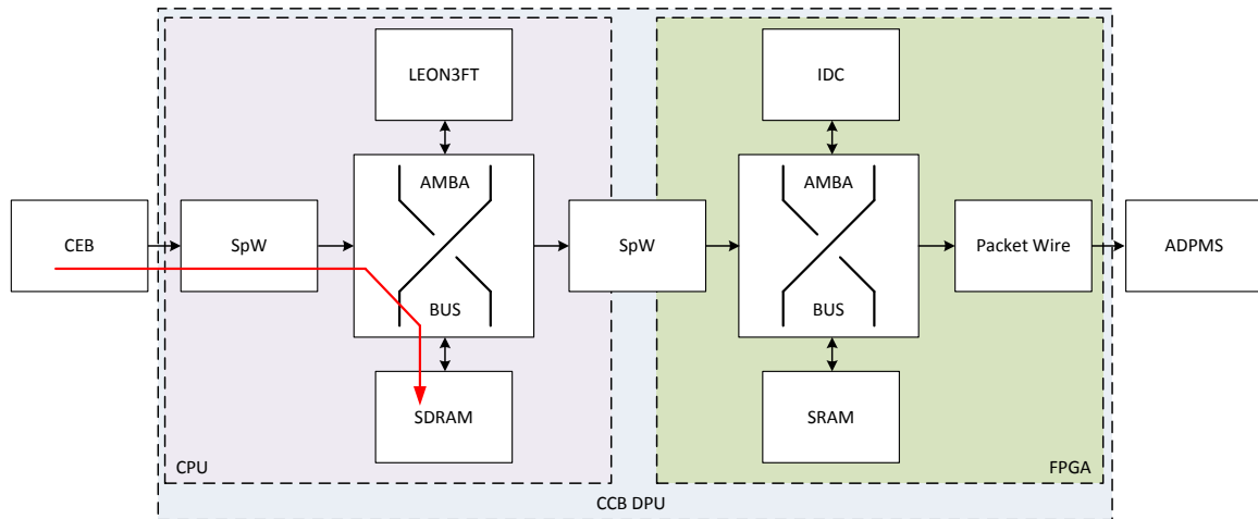
Figure 22 System data transfer: CEB - SpaceWire - SDRAM
