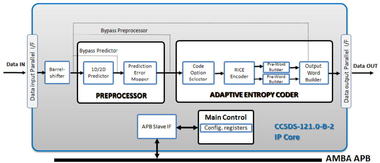
Figure 70 Image data compression IP core block diagram.
