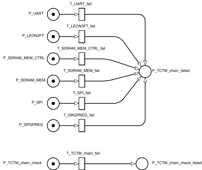
Figure 47 Petri Net modeling TCTM functional chain
