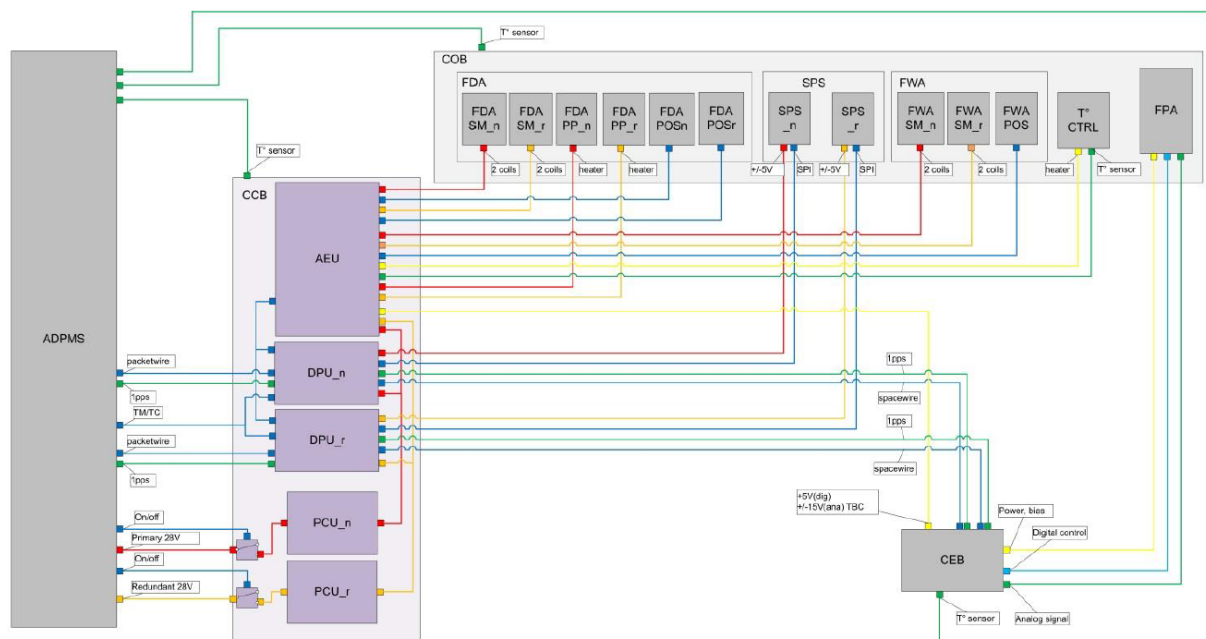
Figure 68 ASPIICS electrical architecture.
