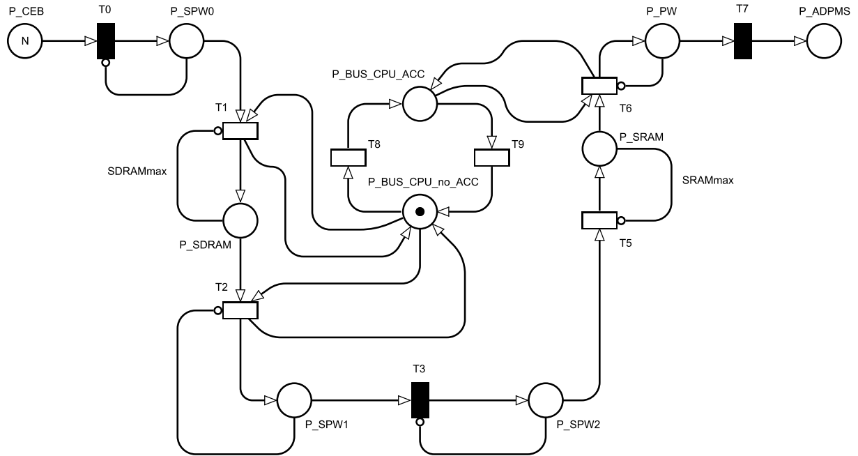
Figure 36 DPU dynamic model with CPU flow control - compression off
