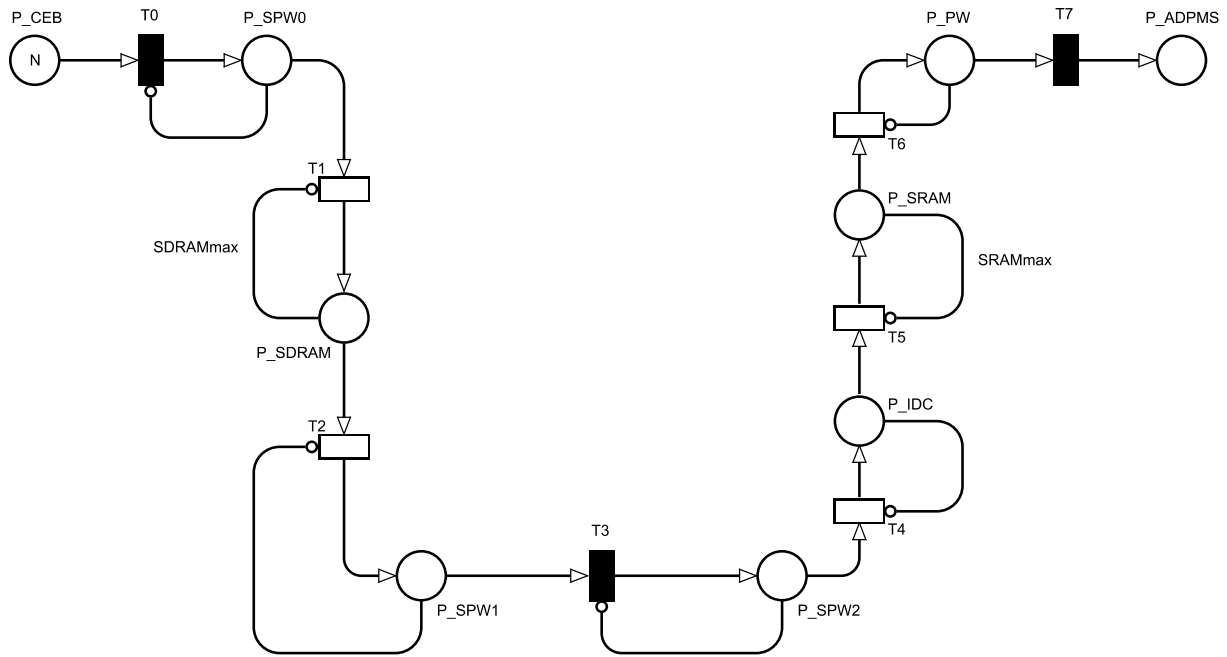
Figure 33 DPU dynamic model – added buffer limits.
