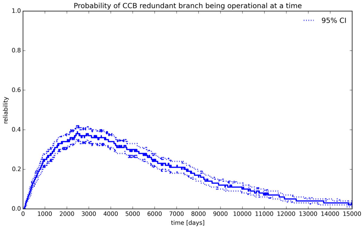
Figure 53 Petri Net simulation of CCB redundant branch reliability
