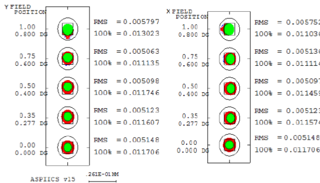
Figure 58 Image spot diagrams at focal plane.
