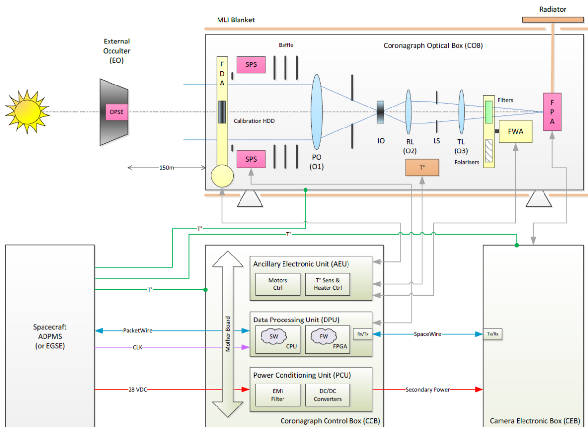
Figure 56 Coronagraph system functional block diagram
