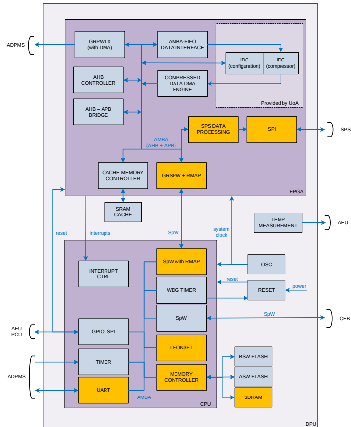
Figure 45 SPS data chain
