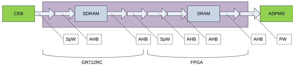
Figure 30 DPU pipeline model - compression on
