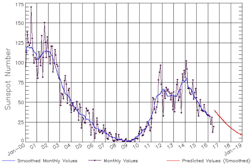
Figure 26 Sunspot number progression [107]
