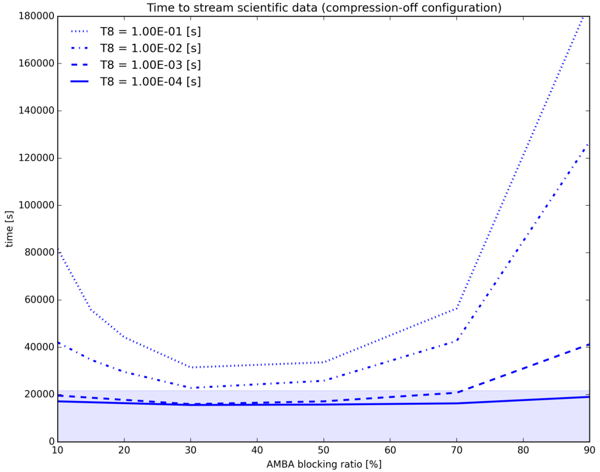
Figure 37 Simulated time to send all tiles of CME-watch observation program, compression-off
