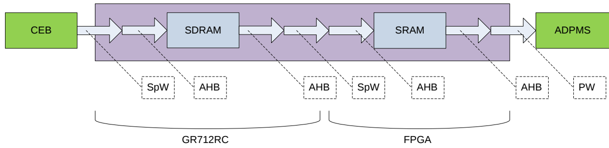
Figure 31 DPU pipeline model - compression off
