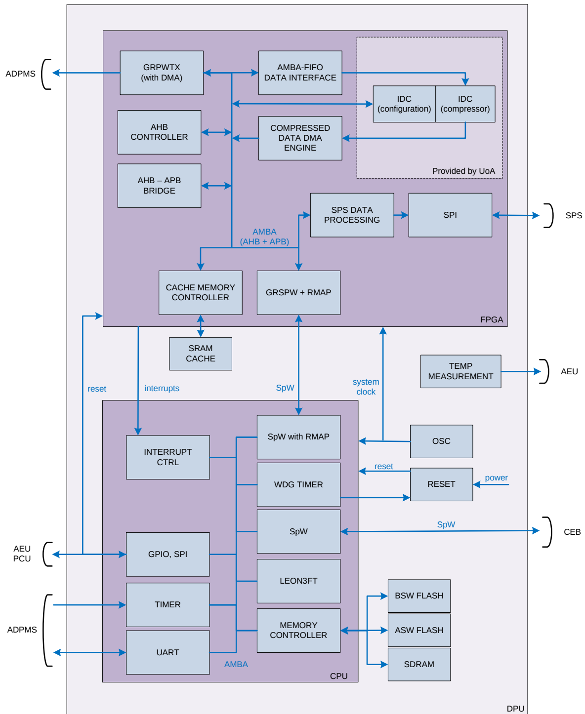
Figure 20 DPU architecture
