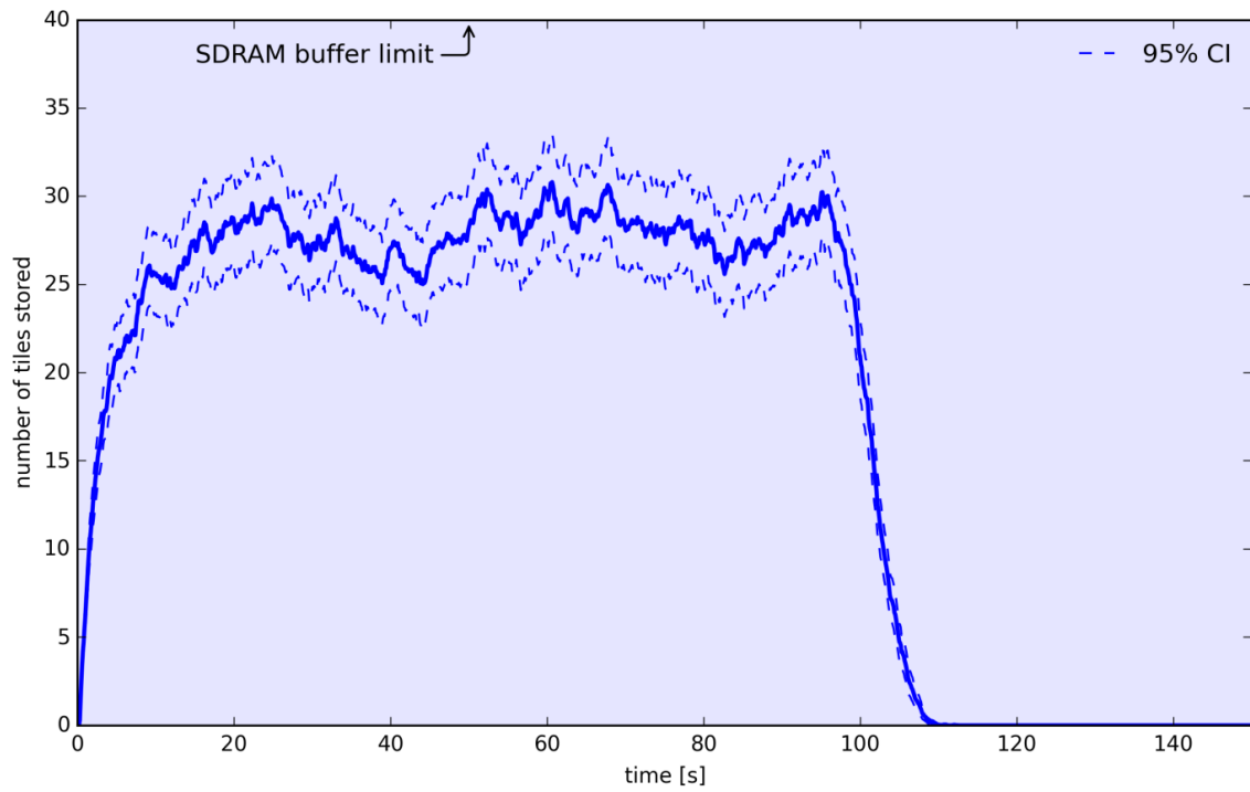
Figure 42 Simulated tiles pile-up in SDRAM ( N=10000 , T8=1.00E-01 , T9=1.00E-01 , AMBA_blocking_ratio=50%, compression-off configuration)
