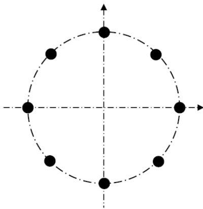
Figure 66 SPS photodiode arrangement around entrance pupil.
