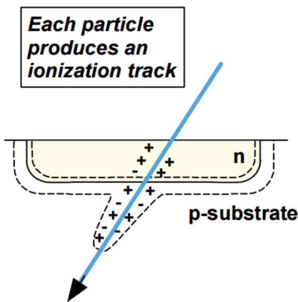
Figure 8 Direct semiconductor ionization [39]
