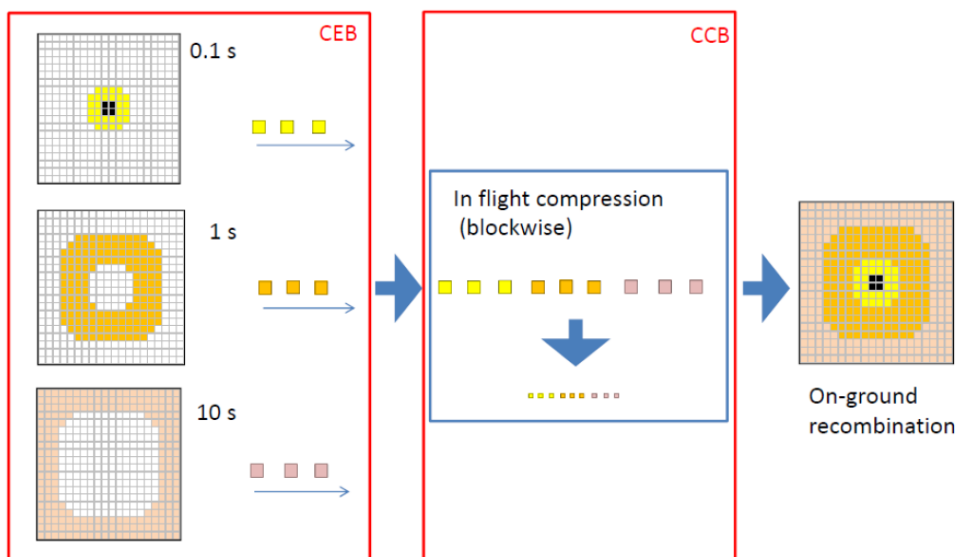
Figure 60 Image data handling principle
