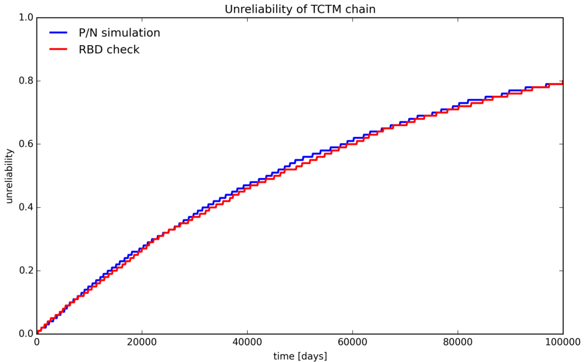
Figure 48 Petri Nets simulation result for TCTM chain
