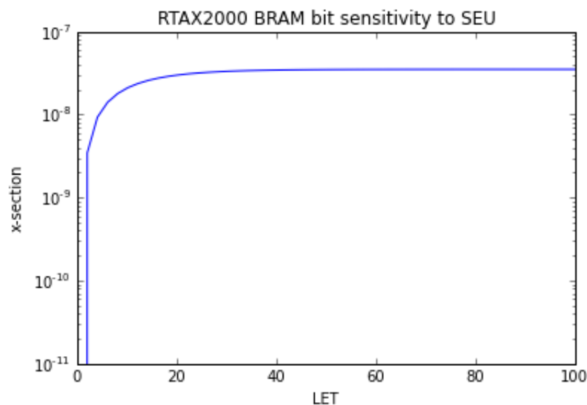
Figure 73 RTAX2000 BRAM bit upset cross-sections
