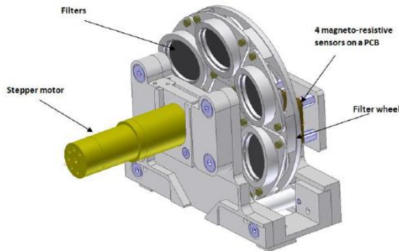
Figure 63 Filter Wheel Assembly (FWA)
