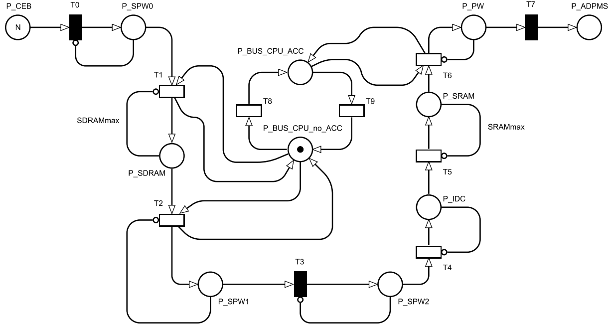
Figure 34 DPU dynamic model with CPU flow control - compression on
