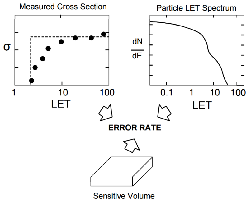
Figure 11 Error (upset) rate calculation [39]
