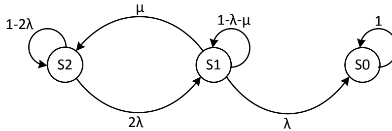
Figure 15 Markov process (chain) example
