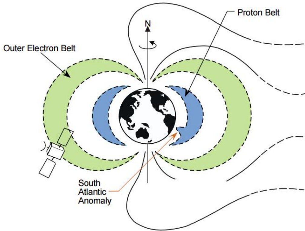
Figure 7 Earth's radiation belts and South Atlantic Anomaly [39]
