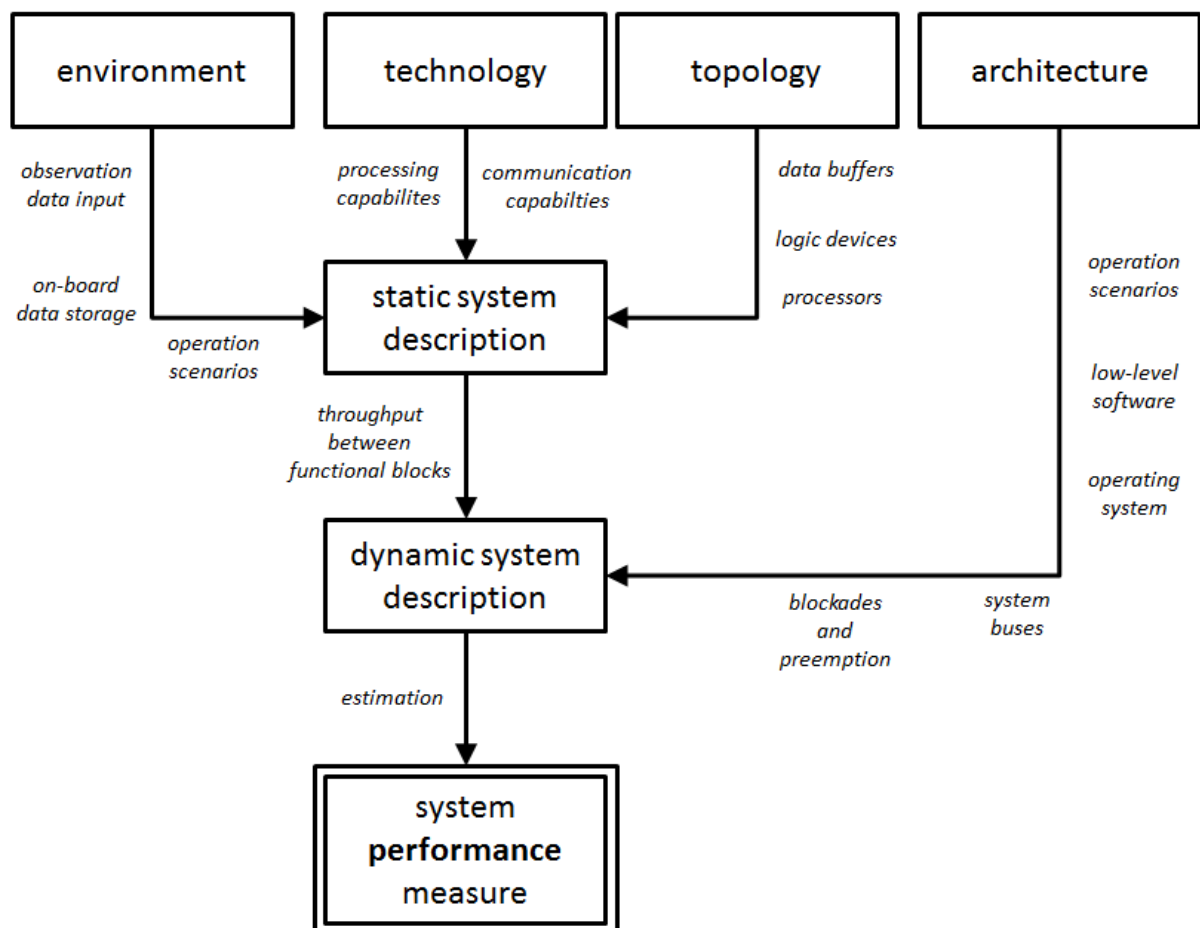
Figure 29 Generic system performance modeling methodology
