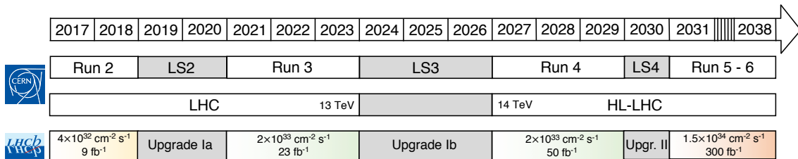
Figure 1.2: Timeline of the LHC and LHCb experiment. The detector Upgrade Ia is currently ongoing, and will be consolidated during Upgrade Ib. Although the HL-LHC will start operation in 2027, the luminosity in the LHCb experiment will not be increased until LHC Run 5.
