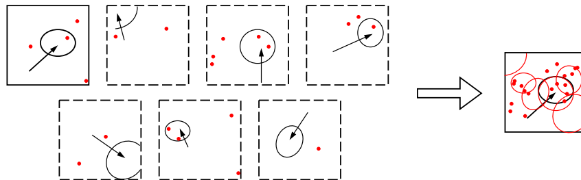
Figure 3.8: In order to estimate the effect of pile-up in the Upgrade Ia framework, six events (dashed frames) are superimposed as background (marked in red) onto the event of interest (solid frame).
