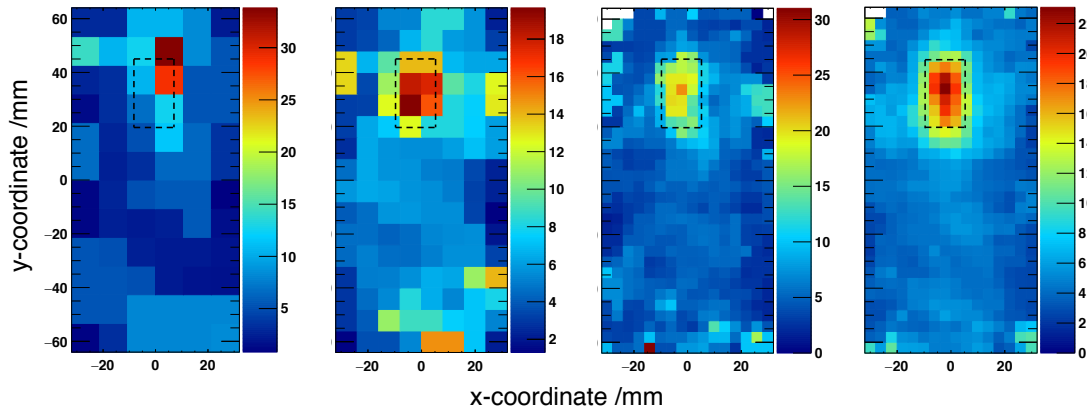
Figure 5.15: ASR images of a lead sample. From left to right: 100, 1000, 5000 and 25000 muons from experiment. The volume element size is increased at low statistics, in order to keep a sufficient number of muons in each element. The colour scales are chosen to present the best contrast.
