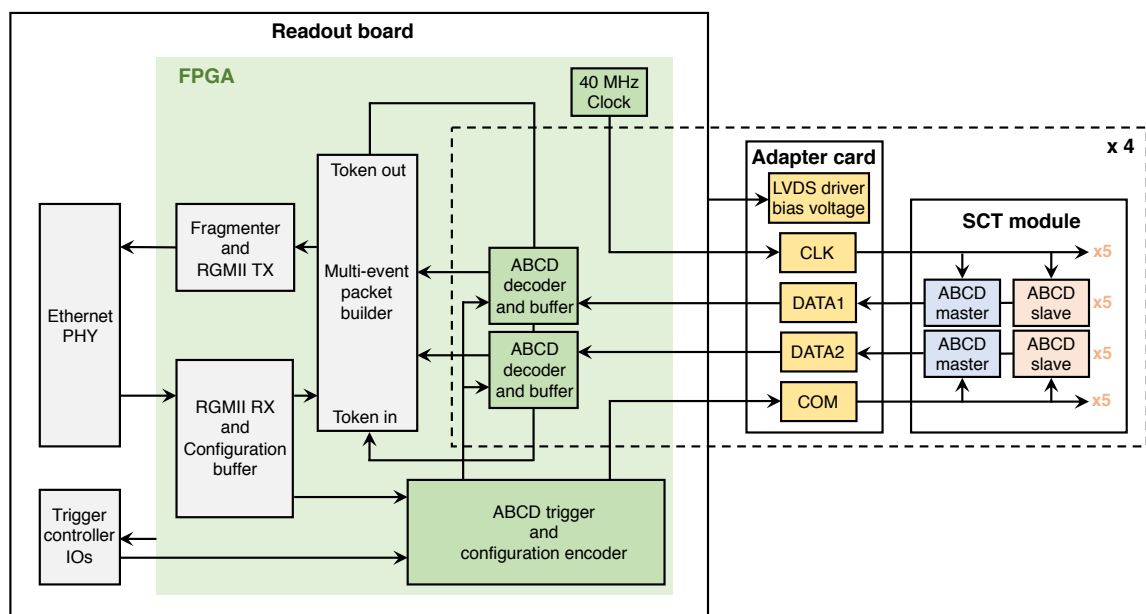
Figure 4.11: FPGA logic diagram for the configuration and readout of SCT modules. The ABCD trigger and configuration encoder and ABCD decoder and buffer logic was adapted to the SCT modules, while the Ethernet interface shaded in grey has not been modified for these studies.
