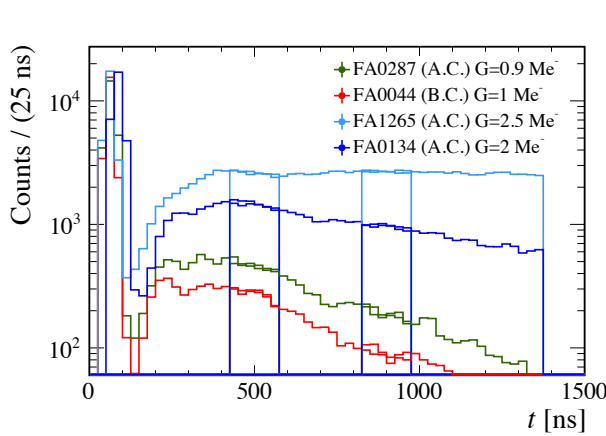
Figure 2.24: The number of hits per 25 ns over a time period of 1.4 \mu\text{s} , for four different MAPMTs. The signal at 100 ns is followed by a tail of SIN hits with different time constants. Source: [83].
