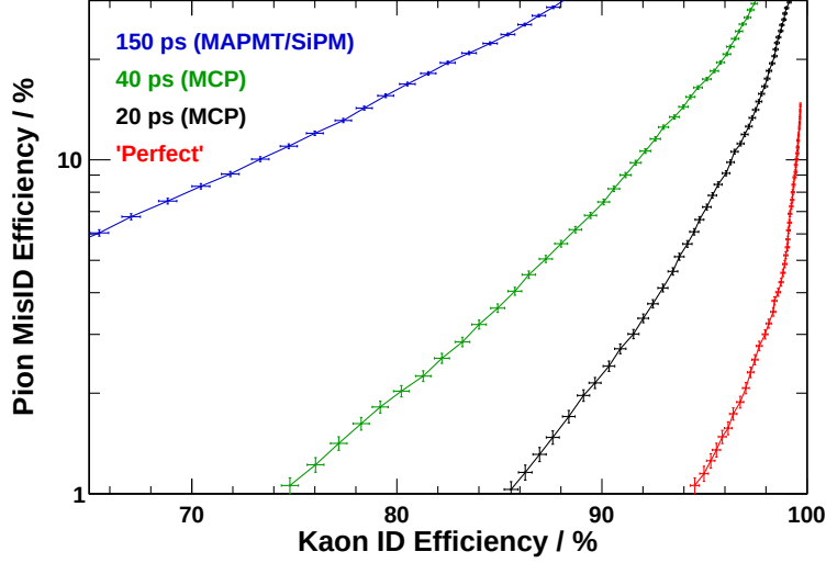
Figure 3.32: Particle ID curves for different sensor time resolutions, each with a 3\sigma_{sensor} time gate and in the presence of pile-up. The curves demonstrate the improvement from time resolution only. A resolution of approximately 150 ps is expected for the MAPMT and SiPM, while 20 to 40 ps can be achieved by MCP detectors.
