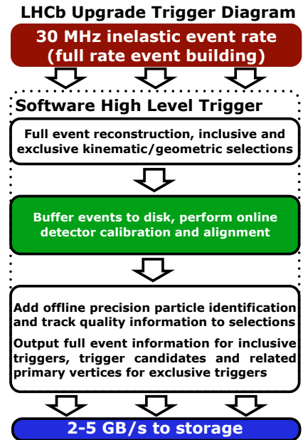
Figure 1.21: The high-level trigger reduces the data rate from the event builder to storage and performs run-by-run calibration. Source: [65].
