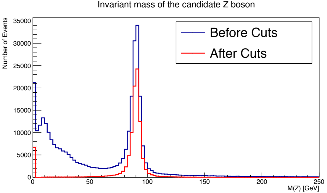
Figure 6.3: Invariant mass of the four-vector addition of the first- and second-highest p_T electrons in a MC sample of gg \rightarrow ZZ . The blue line shows the invariant mass of the electrons before any of the selection criteria have been applied, and the red line shows the invariant mass of the electrons in the sample after all selections are applied.
