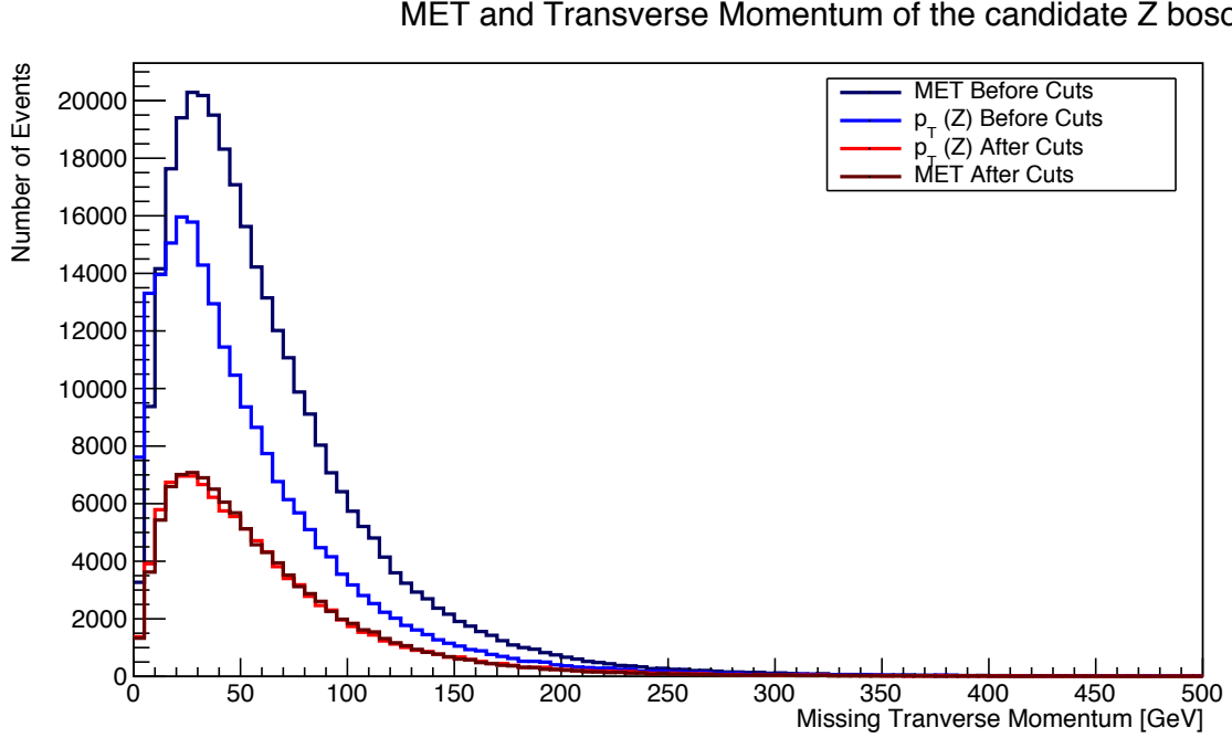
Figure 6.8: Comparison of the \mu\mu p_T ( Z \rightarrow \mu^+\mu^- ) and the missing transverse momentum in a MC sample of gg \rightarrow ZZ , after all of the object selection cuts have been performed, and keeping events with two selected muons. The red ( p_T ( Z \rightarrow \mu^+\mu^- )) and dark red ( E_T^{\text{miss}} ) distributions show very good agreement after keeping events with two selected muons.
