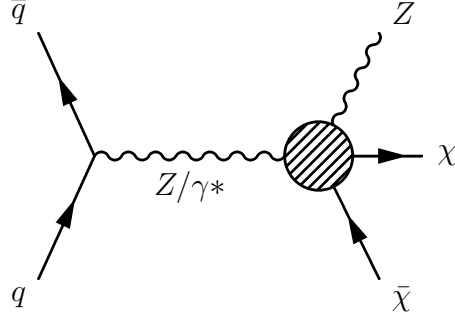
Figure 3.12: Diagram for contact interaction effective field theory.
