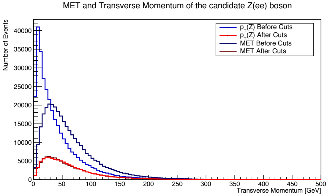
Figure 6.4: Comparison of the p_T ( Z \rightarrow e^+e^- ) and the missing transverse momentum in a MC sample of gg \rightarrow ZZ after all of the object selection cuts have been performed, and keeping events with two selected electrons. The red ( p_T ( Z \rightarrow e^+e^- )) and dark red ( E_T^{\text{miss}} ) distributions show very good agreement after keeping events with two selected electrons.
