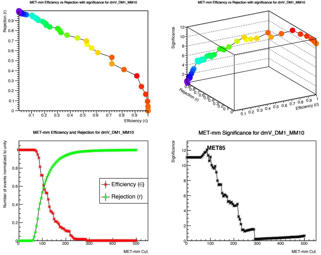
Figure 6.10: Optimization example of the missing energy. The significance as a function of the cut value can be seen in the lower right plot. The lower left plot shows the efficiency and rejection curves as a function of cut values. The top left plot shows the efficiency as a function of rejection, where the colour indicates the value of the significance at each point, that corresponds to the values in the top right plot. Finally, the top right plot shows the same as the top left, but as a three-dimensional plot with the significance on the third axis (with coloured values).
