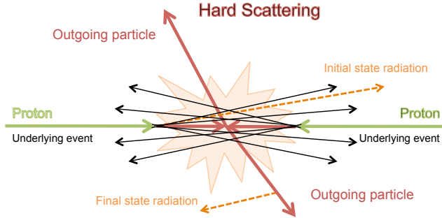
Figure 3.8: Proton-proton collision schematic (based on figure in [50]).
