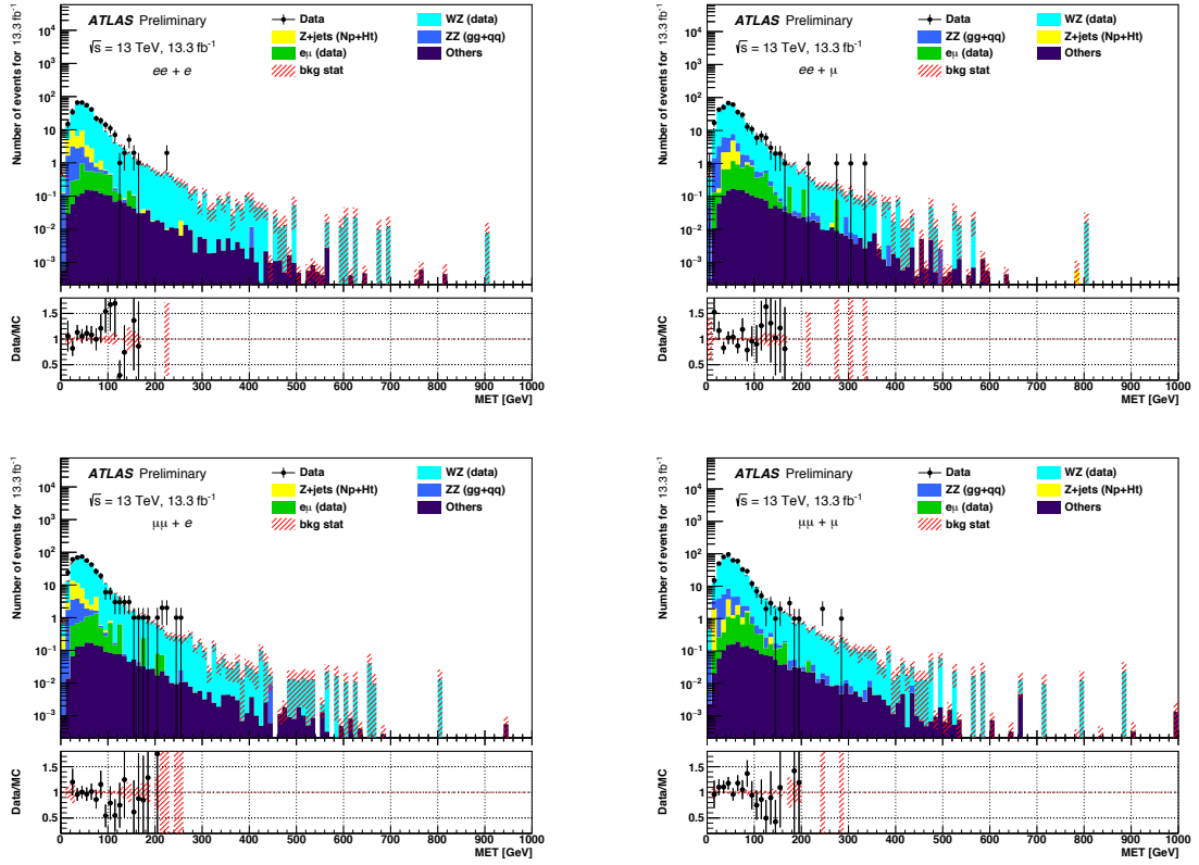
Figure 7.4: E_T^{\text{miss}} distributions after the m_T(W) cut for data and MC in (a) the ee + e channel, (b) ee + \mu channel, (c) \mu\mu + e channel and (d) \mu\mu + \mu channel in events with one additional electron or muon with respect to the lepton pair whose invariant mass is consistent with the Z boson mass. MC samples are normalized to their cross section values as given in Chapter 5 and re-scaled to the data integrated luminosity reported in the figure. The bottom plots show the ratio of the data and MC.
