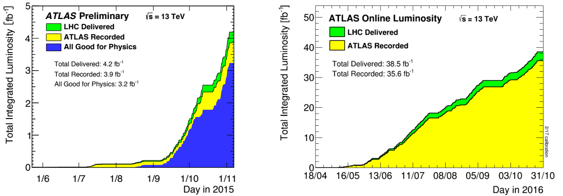
Figure 5.2: Integrated luminosity by day for 2015 (left) and 2016 (right).
