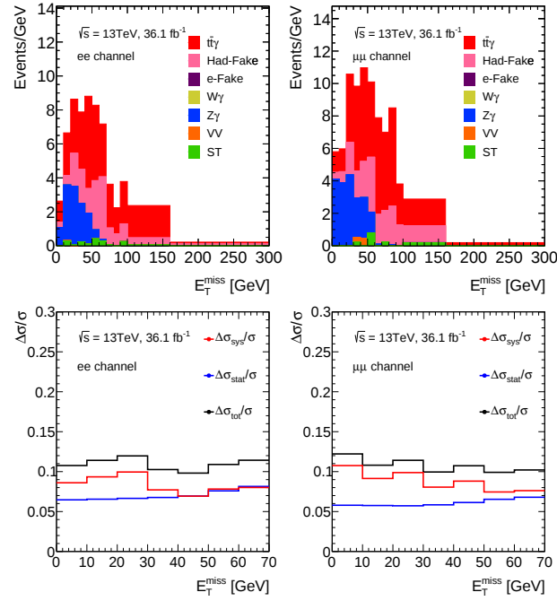
Figure 6.4: Distributions of the missing transverse momentum (top). The uncertainty on the expected cross section as a function of this variable (bottom), in the ee (left) and \mu\mu (right) channels. The systematic uncertainty is shown in red, the statistical uncertainty in blue and the total uncertainty in black. Had-Fake refers to the hadronic-fake background, VV to the diboson background and ST to the single-top background.
