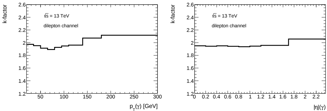
Figure 6.3: The k-factor distribution as a function of the photon p_T (left) and the photon |\eta| (right), estimated using particle-level objects at LO in the dilepton channel.
