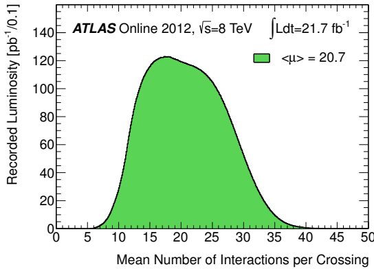
Figure 4.3: The average number of interactions per bunch crossing during proton–proton collisions at \sqrt{s} = 8 TeV (left) [80], and \sqrt{s} = 13 TeV for the 2015 and 2016 runs (right) [82], at the ATLAS detector.
