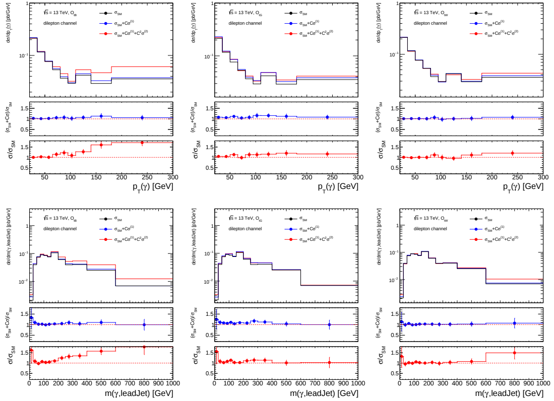
Figure 7.1: The effect of the EFT operators O_{IB} (left) O_{IG} (middle), and O_{IW} (right) on the t\bar{t}\gamma dilepton fiducial cross section as a function of the photon p_T (top) and invariant mass of the photon and the hardest jet (bottom), for values of C_{IB} = \pm 5 , C_{IG} = \pm 0.3 and C_{IW} = \pm 2 . The SM differential cross section is shown in black, the effect of the interference term in blue, the effect of both, interference and quadratic terms in red.
