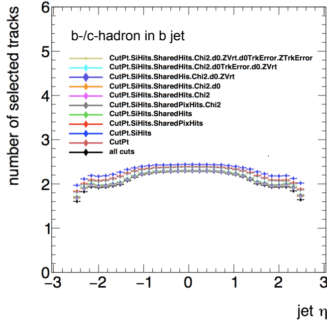
Figure A.2: The basic track selection requirements as a function \eta for b -jets. The selections are applied to tracks coming from b - c -hadron decay. The applied values described in Table A.1 are used incrementally, starting with the p_T requirement (brown), and adding the silicon hits (dark blue), shared pixel hits (red), shared hits (green), \chi^2 (gray, pink), d_0 (orange), z_0 (purple), d_0 track error (light blue), z_0 track error (dark green) requirement and all basic requirements in Table A.1 (black).
