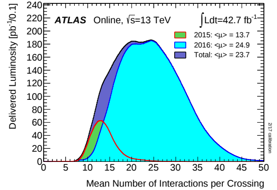
Figure 4.3: The average number of interactions per bunch crossing during proton–proton collisions at \sqrt{s} = 8 TeV (left) [80], and \sqrt{s} = 13 TeV for the 2015 and 2016 runs (right) [82], at the ATLAS detector.
