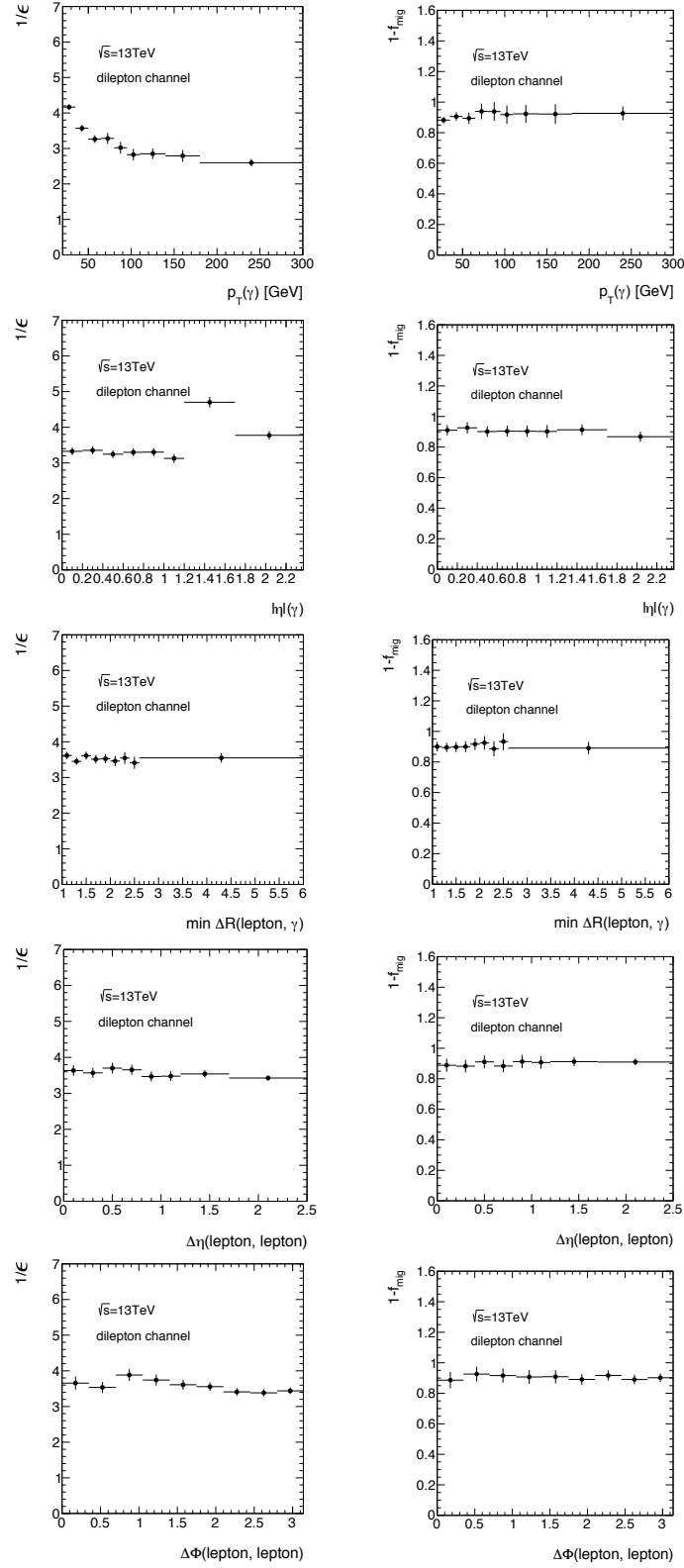
Figure 6.15: The inverse of signal efficiency 1/\epsilon (left) and the fraction of non-outside migration ( 1 - f_{\text{mig}} ) (right) as a function of the photon p_T (first row), the photon |\eta| (second row), the minimum \Delta R(\ell, \gamma) (third row), the \Delta\eta(\ell, \ell) (fourth row) and the \Delta\phi(\ell, \ell) (fifth row), in the dilepton channel.
