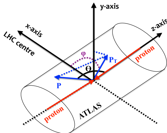
Figure 3.4: The right-handed coordinate system of the ATLAS detector.
