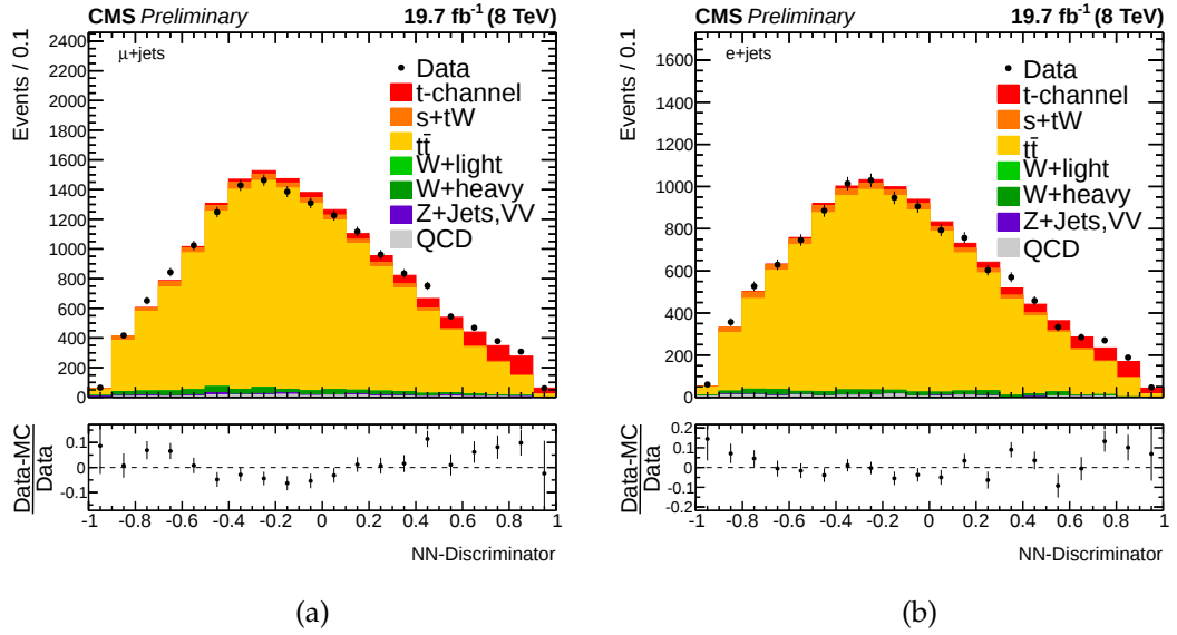
Figure 6.11.: Neural network discriminator in the tt control region (3j2t) for the muon (a) and electron (b) channel.
