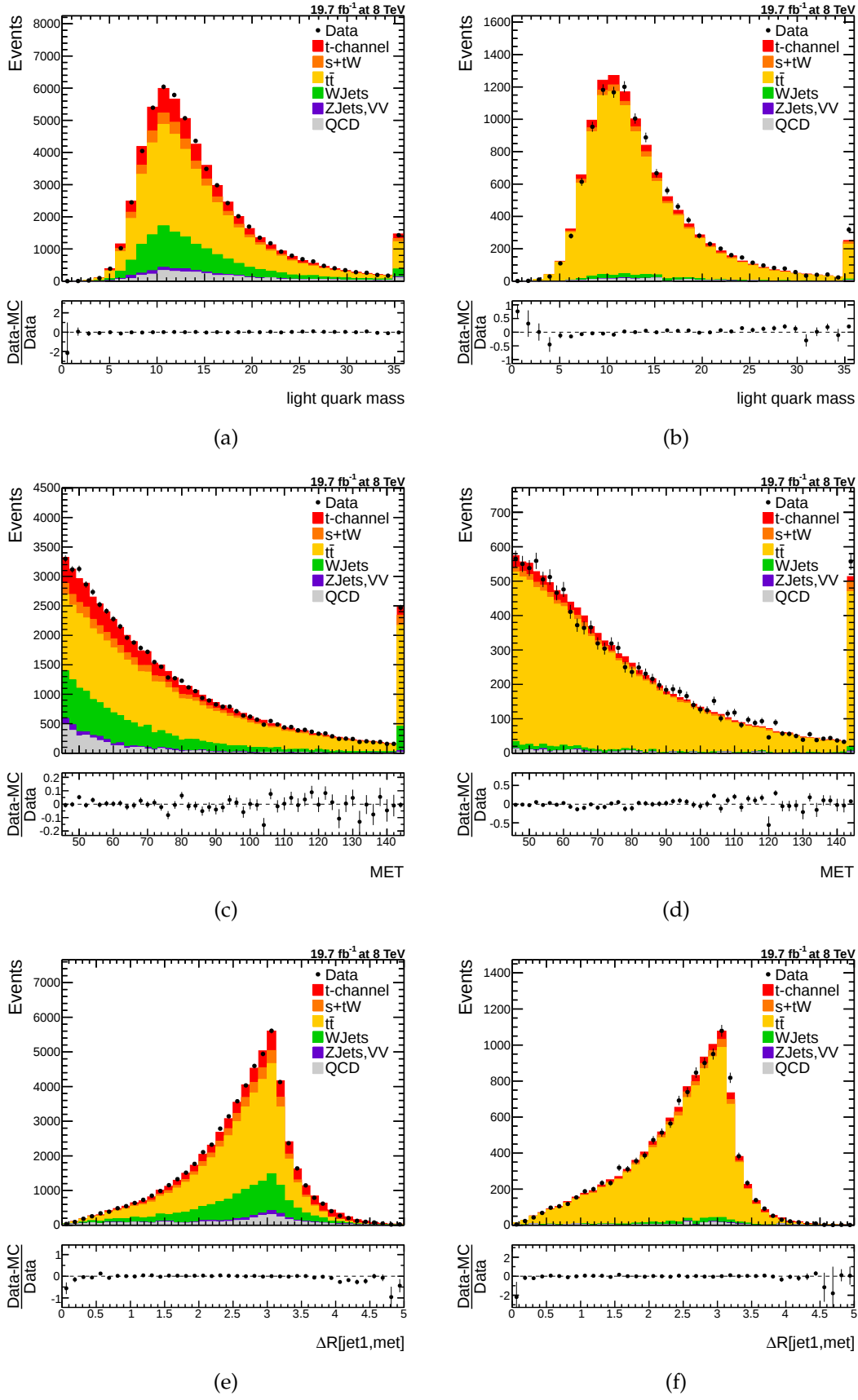
Figure C.11.: Electron channel input variables. m_{lq} , \cancel{E}_T and \Delta R(jet1, \cancel{E}_T) .
