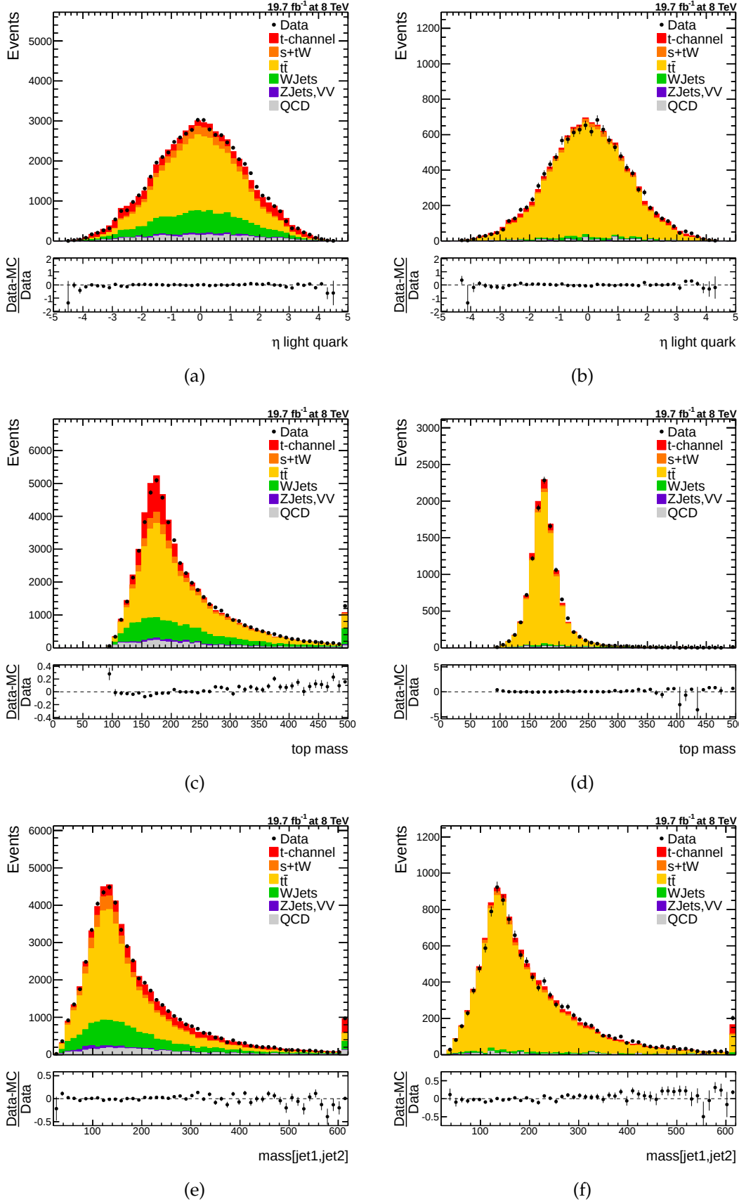
Figure C.7.: Electron channel input variables. \eta_{lq} , m_{\ell vb} and m_{jet1, jet2} .
