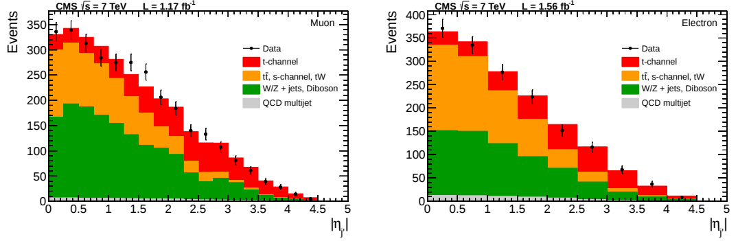
Figure 2.1.: Pseudorapidity of the light quark jet \eta_{lj} in the 7 TeV measurement. Result of a simultaneous fit to the pseudorapidity of the light quark jet \eta_{lj} in the muon (left) and electron (right) decay channels.
