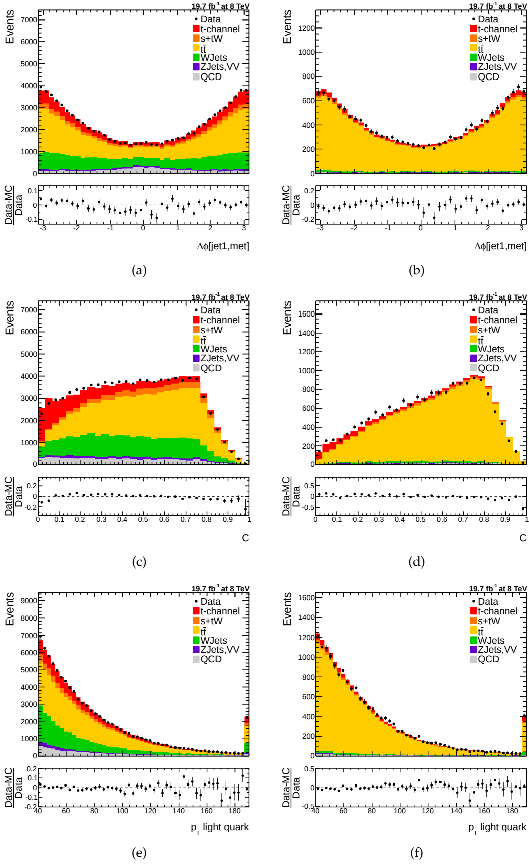
Figure C.4.: Muon channel input variables. \Delta\phi(\text{jet1}, \cancel{E}_T) , C and p_{T, \text{lq}} .
