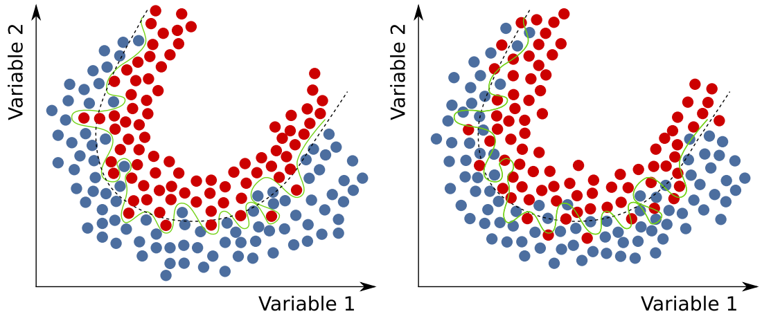
Figure 6.3.: Visualization of overtraining. Two-dimensional representation of signal (red) and background (blue) events. The dashed line represents the optimal decision boundary for both the training and validation data. The green line shows the overtrained decision boundary. The diagram on the left shows an overtrained network on the training data. If this network is applied on the validation sample (right), background events within the green line would be wrongly classified as signal [168].
