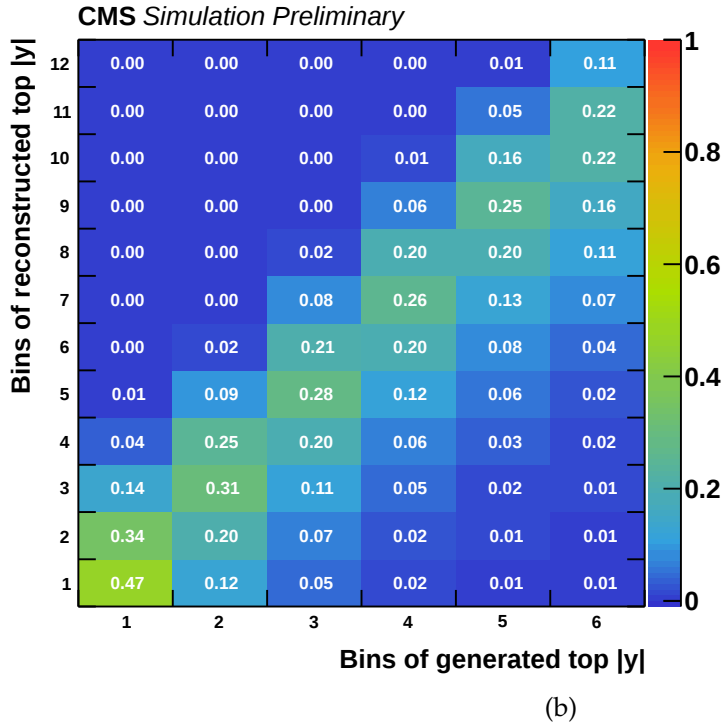
Figure 7.4.: Migration matrices for top quark p_T and |y| . Each migration matrix gives the probability of an event with a certain true top quark p_T to show up in one of the bins of the reconstructed top quark p_T (a), same for |y| (b).
