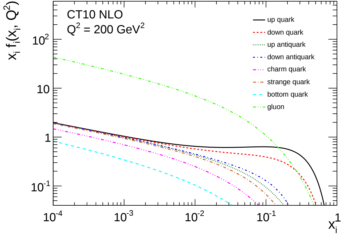
Figure 1.4.: CT10 [30] parton distribution functions for u, \bar{u}, d, \bar{d}, c, s, b quarks and gluons at NLO. The energy scale was set to Q^2 = 200 \text{ GeV}^2 .
