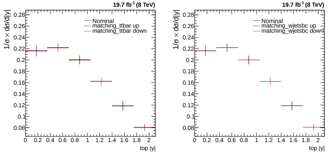
Figure 7.14.: Effect on the shape of the unfolded top-quark rapidity spectrum due to variations in the matching threshold of (a) t\bar{t} and (b) W+\text{jets} simulated events.
