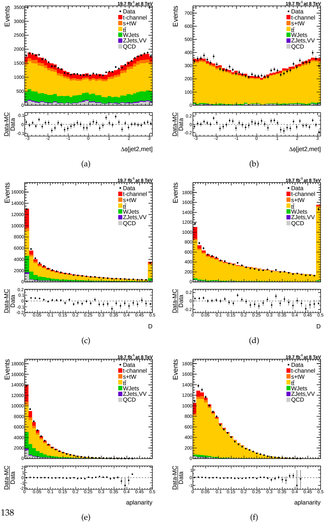
Figure C.12.: Electron channel input variables. \Delta\phi(\text{jet2}, \cancel{E}_T) , D and A .
