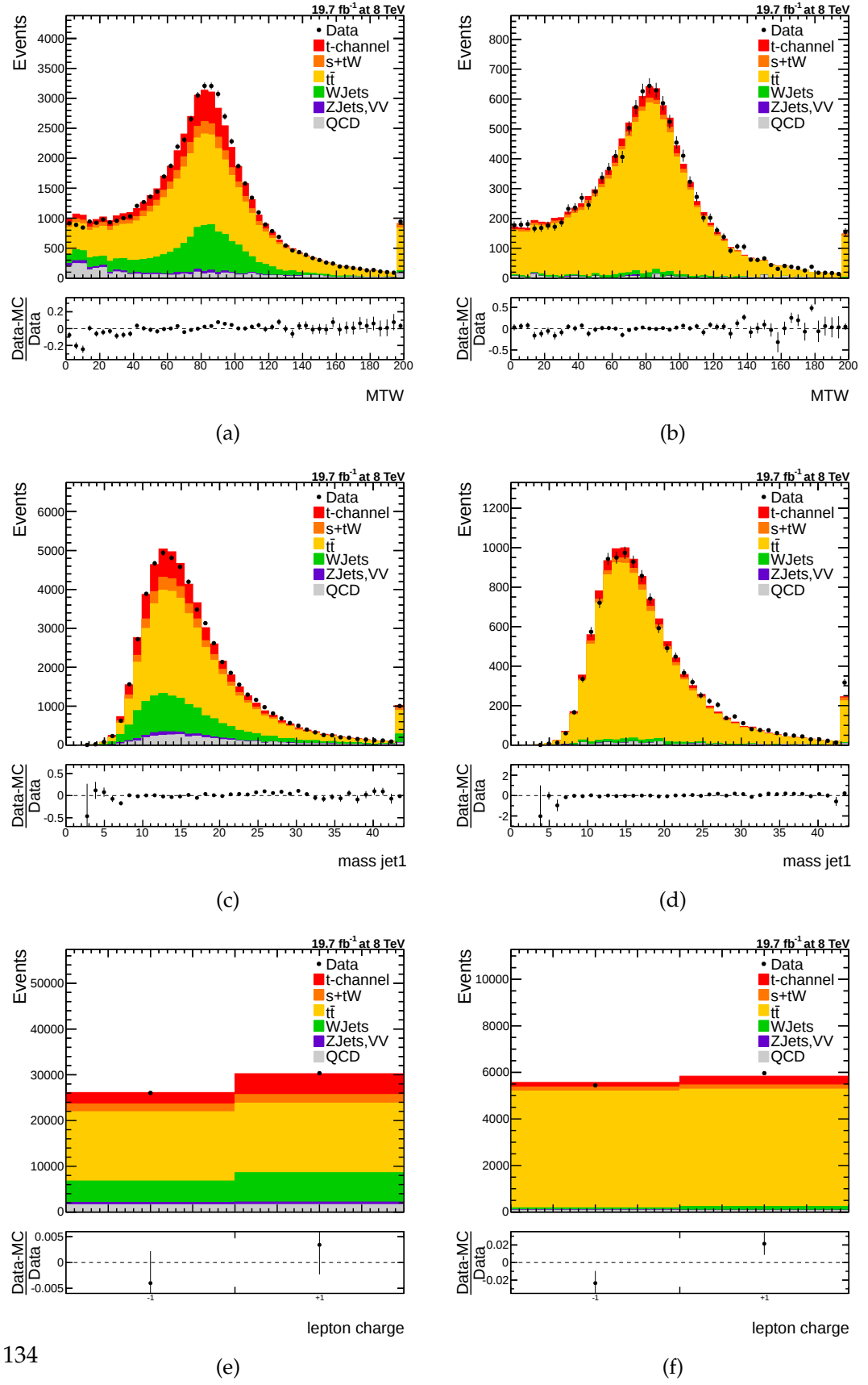
Figure C.8.: Electron channel input variables. m_{T,W} , m_{jet1} and Q_\ell .
