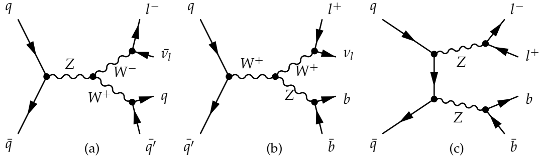
Figure 5.2.: Diboson production in the WW (a), WZ (b) and ZZ (c) production modes.
