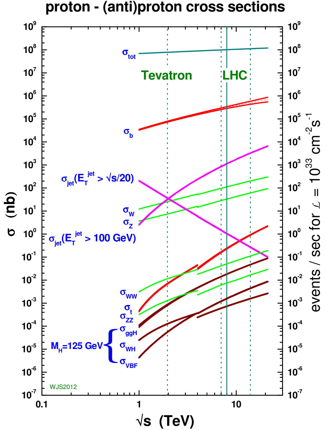
Figure 1.3.: Standard model cross sections as a function of collider energy [26].
