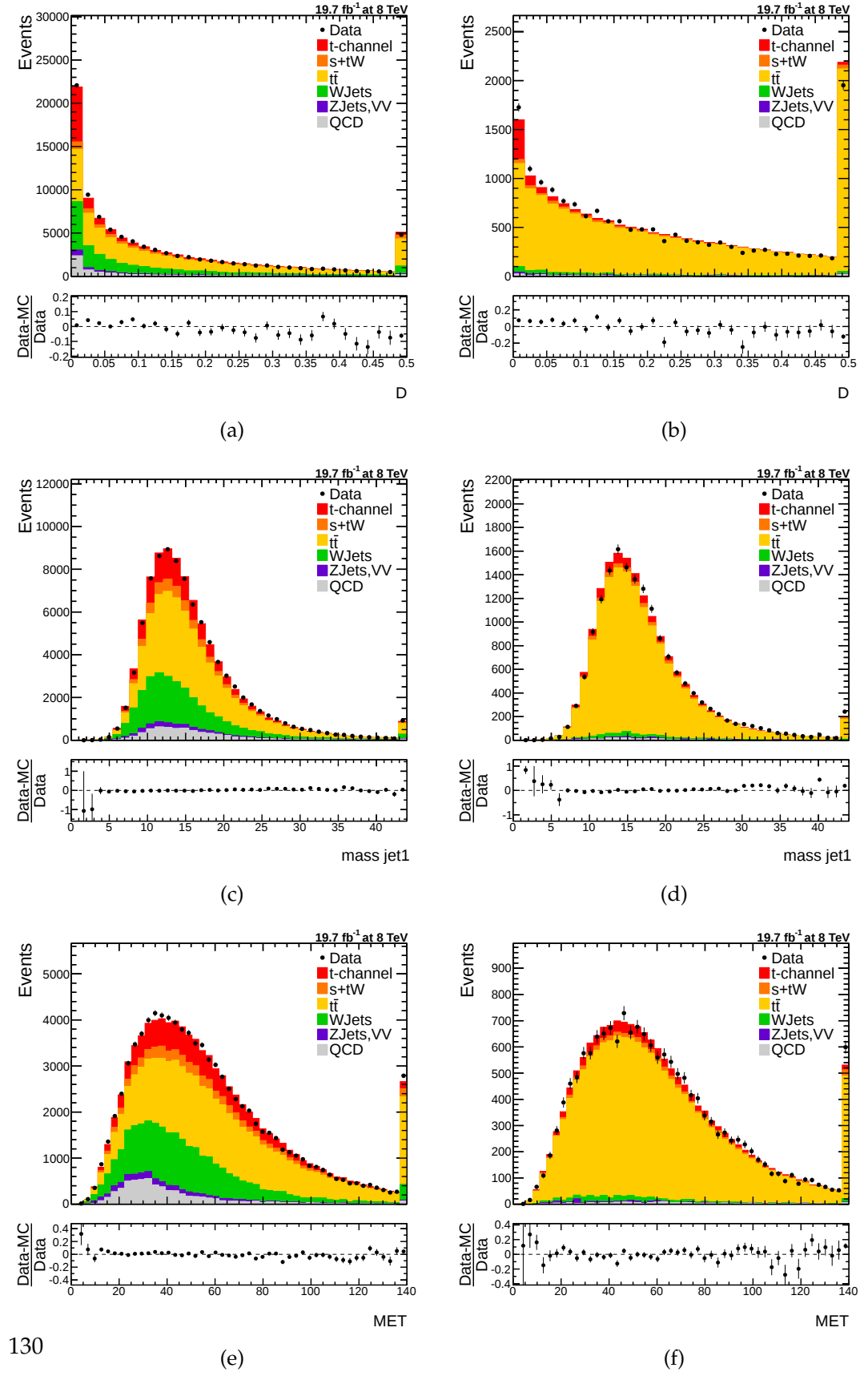
Figure C.5.: Muon channel input variables. D , m_{\text{jet1}} and \cancel{E}_T .
