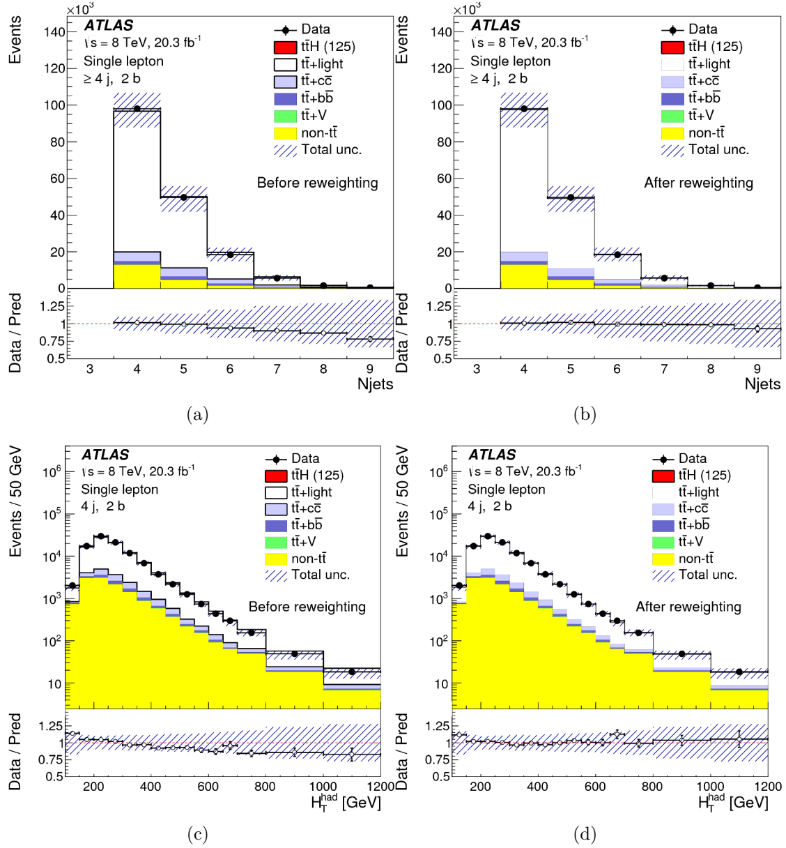
Figure 6.2: Effect of the reweighting of the t\bar{t} system p_T and of the top quark p_T in POWHEG + PYTHIA t\bar{t} sample. Plots on the left are before the reweighting, the one on the right are after. Top row shows the jet multiplicity distribution, bottom row shows H_T^{\text{had}} distribution. Plots are made with the t\bar{t}H ( H \rightarrow b\bar{b} ) semi-leptonic decay channel [11].
