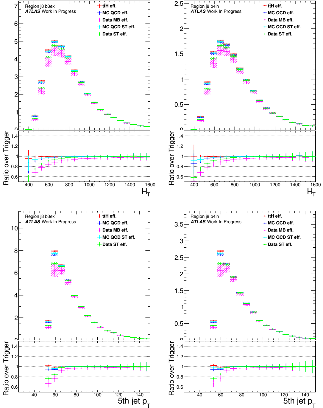
Figure 4.12: Distributions of predicted H_T and 5 th leading jet p_T in fully hadronic t\bar{t}H MC events passing the offline selection. Different predictions are derived applying event weights using efficiencies estimated from t\bar{t}H sample (red points), PYTHIA MC di-jet (blue points) and random triggered data (purple points), using EF_j110_a4tchad for PYTHIA MC di-jet (cyan points) and data (green points). Bottom panel shows the ratio between the prediction and the requirement of EF_5j55_a4tchad_L2FS trigger. Plots correspond to \geq 8 jet multiplicity bin and exactly 3, left, and \geq 4 , right, b -tagged jet multiplicity bins. The systematic undershooting of the prediction made with efficiency from data seen in Figure 4.9 has been corrected.
