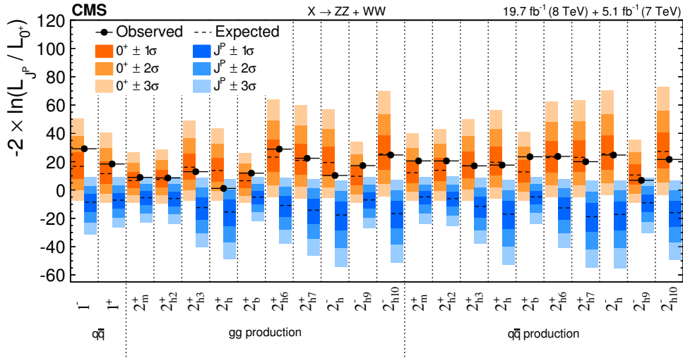
Figure 1.7: Distributions of the test statistic q = -2\ln(\mathcal{L}_{JP}/\mathcal{L}_{0+}) for the different models tested against the SM Higgs boson hypothesis. The expected median and 1,2,3 \sigma CL regions for the tested J^P models (blue bands) and for the SM Higgs boson hypothesis (red bands) are shown. The observed q values are indicated by the black dots [52].
