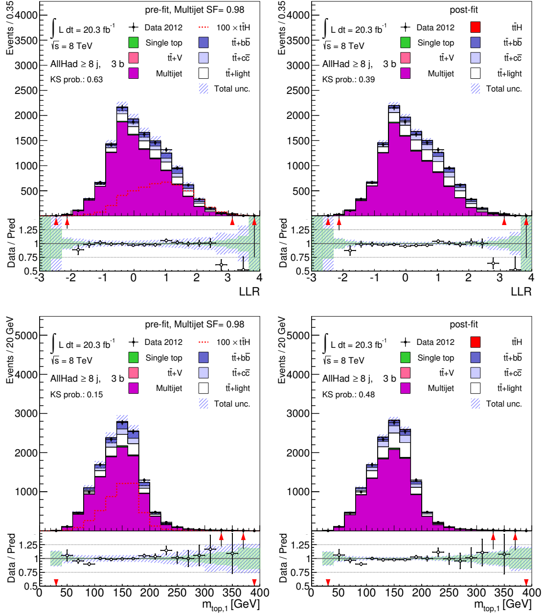
Figure 6.65: Comparison between data and predictions for the LLR (top) and for the m_{top,1} (bottom) in the (\geq 8j, 3b) region; Left : background predictions before performing the fit to data. The uncertainty band contains the full statistical and systematical uncertainties. The signal contribution is not included in the stack plot. Right : signal and background predictions corrected with the result of the fit to data. The uncertainty band contains statistical and systematical uncertainties and takes into account the correlations among the nuisance parameters induced by the fit. Signal contribution is included in the stack plot.
