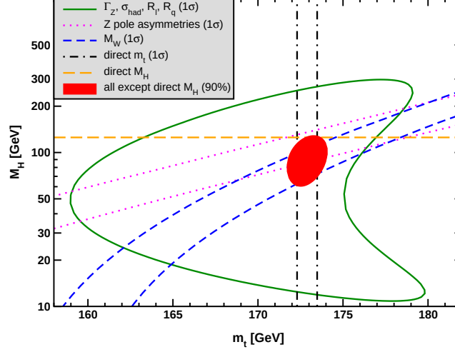
Figure 2.4: Global \chi^2 fit result shown for the Higgs boson mass M_H as a function of the top quark mass m_t including all electroweak data except the direct Higgs boson measurement at the LHC, which is displayed in the yellow dashed line for completeness[19]. The red contour represents the 90% CL region ( \Delta\chi^2 = 4.605 ) allowed by all data. The one-standard-deviation uncertainties of several inputs are also shown: the dashed lines delimit the 68% uncertainty bounds, whereas the filled lines the 39.35% uncertainty bounds.
