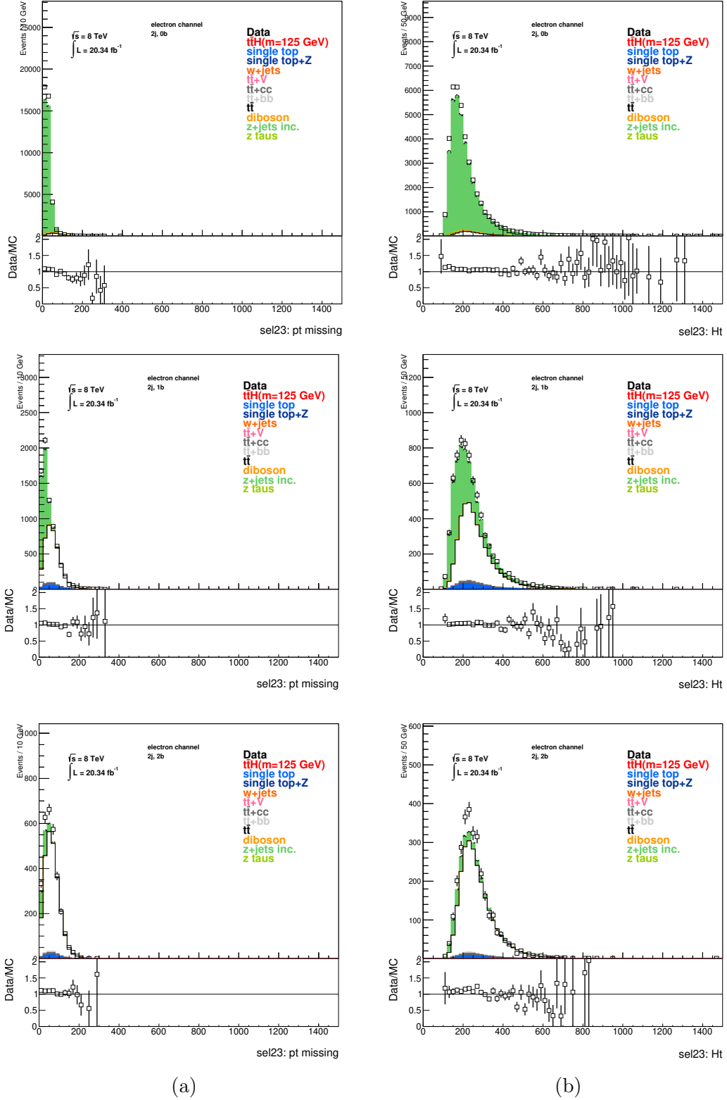
Figure 6.17: Missing transverse momentum (a) and H_T (b) in the two jet region of the di-electron channel after the full Z+jets data driven correction. The error bars associated to the data points include only the statistical uncertainties on the measurement.
