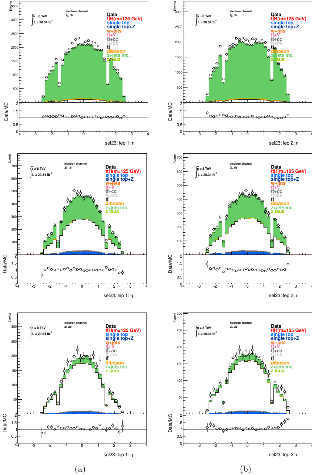
Figure 6.14: Pseudorapidity, \eta , of the leading (a) and subleading (b) lepton in the two jet region of the dielectron channel after the full Z +jets data driven correction. The error bars associated to the data points include only the statistical uncertainties on the measurement.
