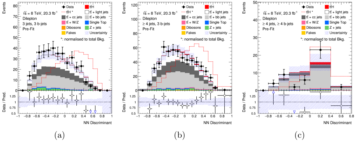
Figure 7.8: NN output discriminants in data and MC simulation for the different regions: (a) for (3j, 3b); (b) for ( \geq 4j , 3b) and (c) for ( \geq 4j , \geq 4b ). The uncertainty bands include both MC statistical uncertainty and systematic uncertainties before the fit procedure. The red dashed line shows the t\bar{t}H signal normalised to the background yield.
