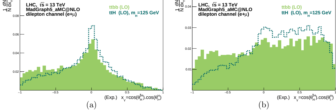
Figure 8.3: Double angular product distributions after the event selection and full kinematic reconstruction. The distributions represent the product of the cosine of \theta_H^{\ell^+} and the cosine of \theta_H^{\ell^-} (a) or \theta_H^{\ell^-} (b).
