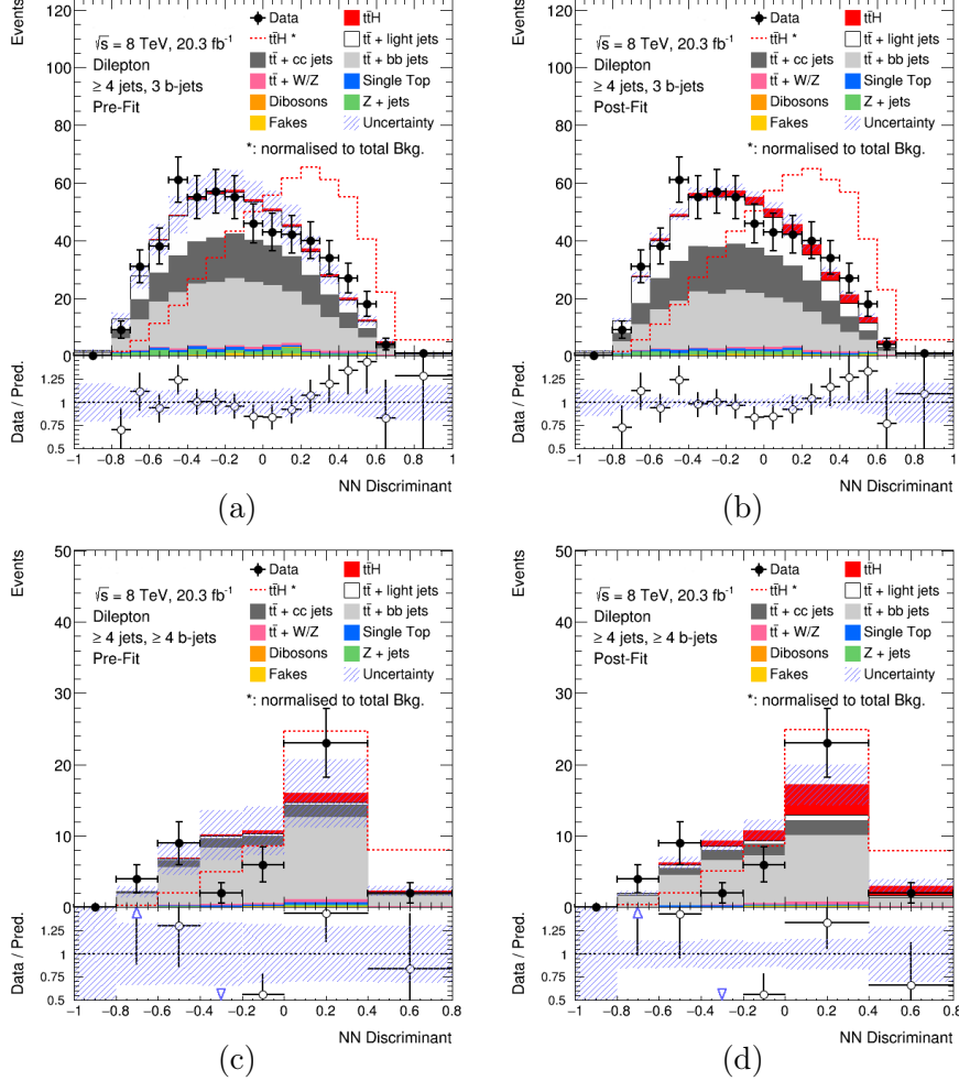
Figure 7.10: Comparison between data and prediction for the NN discriminant distributions on the signal-rich regions before (left) and after (right) the combined fit: (a) and (b) for (\geq 4j, 3b) ; and (c) and (d) for (\geq 4j, 4b) . The t\bar{t}H signal yield is shown normalised to the fitted \mu (solid red histogram) and normalised to the total background prediction (hashed red line). The hashed area represents the uncertainty on the background and the first (last) bin in all figures contains the underflow (overflow).
