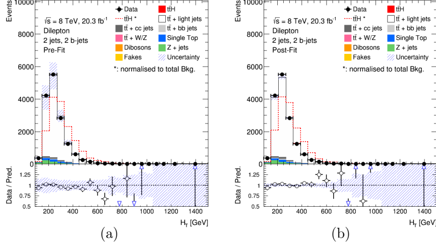
Figure 7.11: Comparison between data and prediction for the validation region (2j, 2b) before (a) and after (b) the statistical fit. The ttH signal yield is shown normalised to the fitted \mu (solid red histogram) and normalised to the total background prediction (hashed red line). The hashed area represents the uncertainty on the background and the first (last) bin in all figures contains the underflow (overflow).
