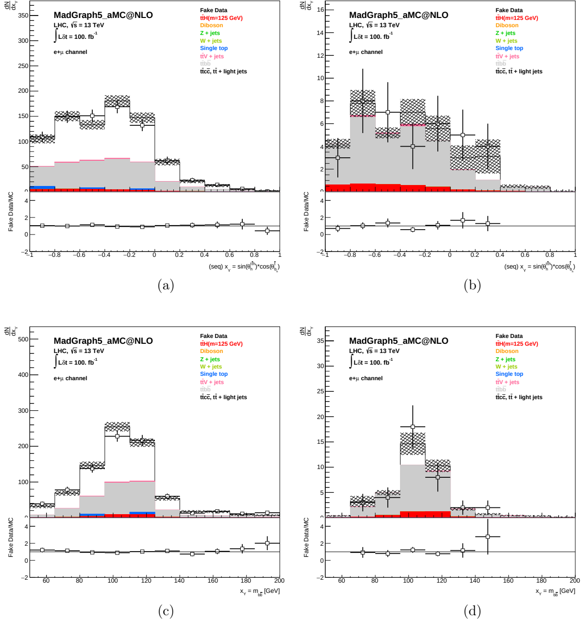
Figure 8.12: Distributions of x_Y = \sin(\theta_{H^{\pm}}^{t\bar{t}}) \cos(\theta_{bH^{\pm}}^{\bar{t}}) (top) and m_{b\bar{b}} (bottom) after the final selection at 13 TeV for 100 \text{ fb}^{-1} . The distributions on the left (right) correspond to events with at least three (four) jets from the hadronisation of b -quarks [4].
