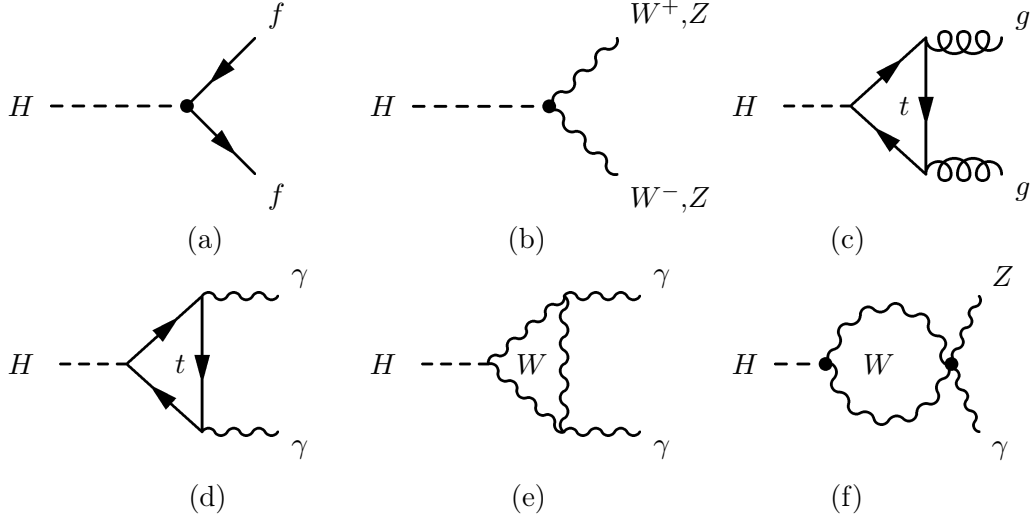
Figure 2.12: Lowest order Feynman diagrams of the SM Higgs boson decay: (a) H \rightarrow f\bar{f} ; (b) H \rightarrow W^+W^- or H \rightarrow ZZ ; (c) H \rightarrow gg ; (d) and (e) H \rightarrow \gamma\gamma via a top quark or W boson virtual loop, respectively; (f) H \rightarrow \gamma Z via a W boson virtual loop.
