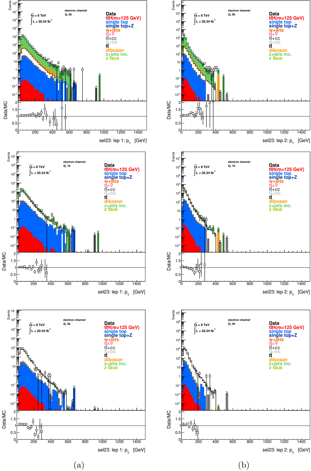
Figure 6.13: Transverse momentum of the leading (a) and subleading (b) lepton in the two jet region of the dielectron channel after the full Z+jets data driven correction. The error bars associated to the data points include only the statistical uncertainties on the measurement.
