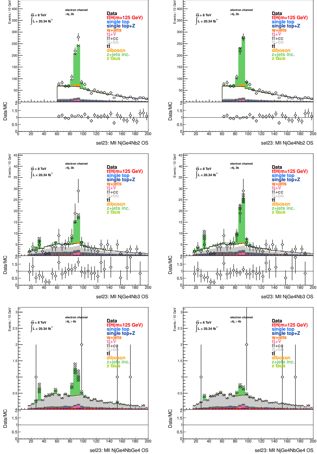
Figure 6.5: Dilepton mass distribution before (on the left) and after (right) the renormalisation of the Z +jets population, for at least four jets and the relevant b -tagged jet multiplicity bins of the dielectron channel. The error bars associated to the data points include only the statistical uncertainties on the measurement.
