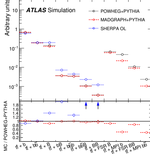
Figure 7.3: POWHEG+PYTHIA, SHERPA+OPENLOOPS and MADGRAPH+PYTHIA comparisons of the t\bar{t} + b\bar{b} jets production.
