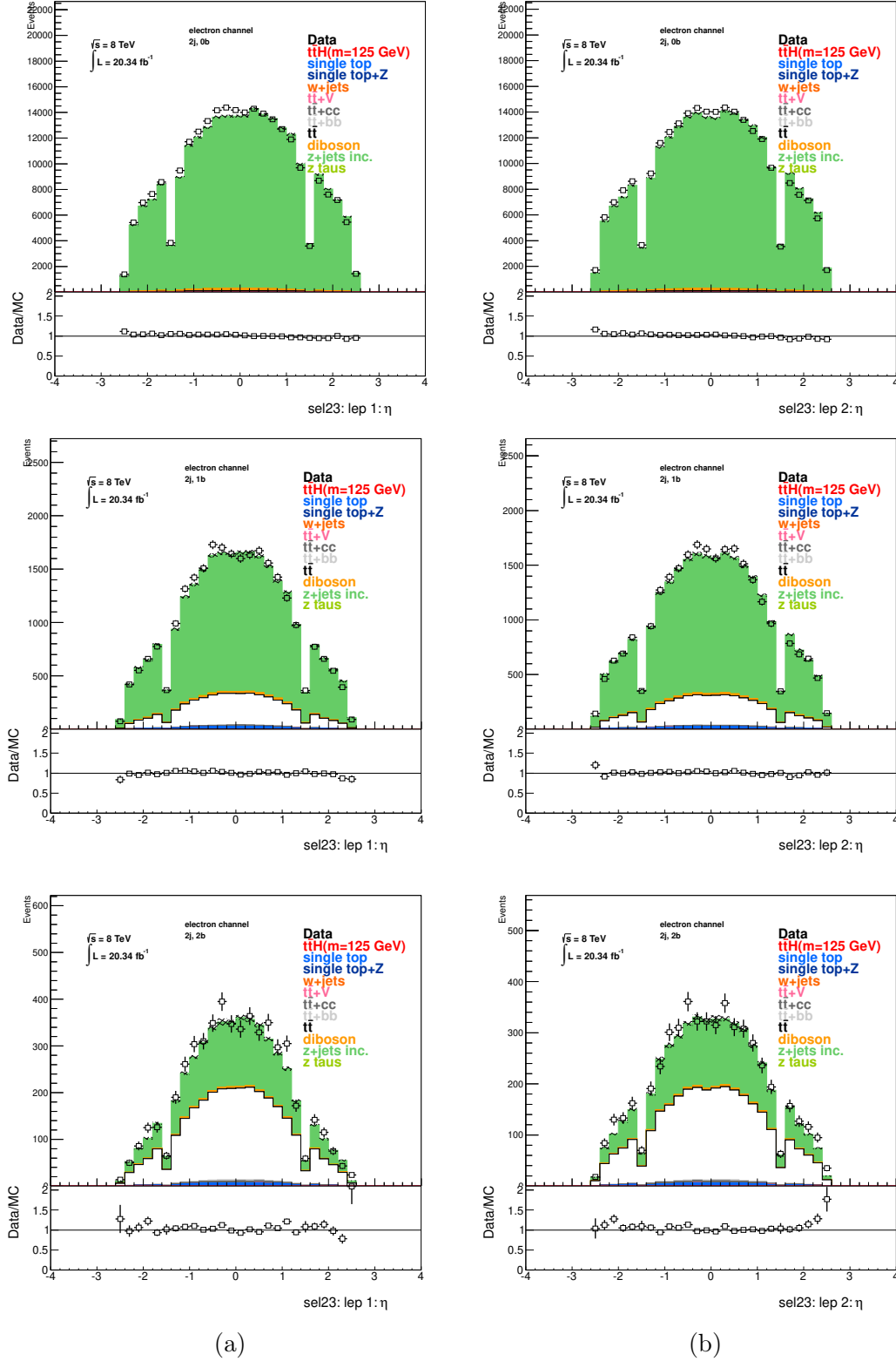
Figure 6.7: Pseudorapidity, \eta , of the leading (a) and subleading (b) lepton in the two jet region of the dielectron channel after the Z+jets data driven cross-section correction. The error bars associated to the data points include only the statistical uncertainties on the measurement.
