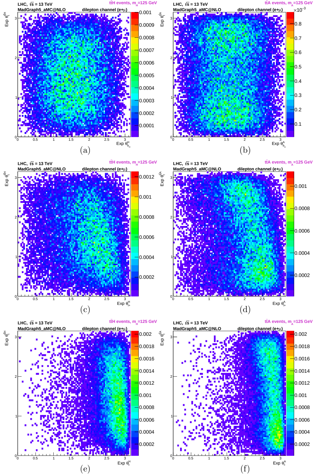
Figure 8.8: In the same disposition of Figure 8.7, but now after all selection cuts and full kinematic reconstruction, two dimensional distribution of \theta_t^{t\bar{t}h} versus \theta_V^h for (a) and (d) Y = b_h , (b) and (e) Y = \ell+_t , (c) and (f) Y = \ell-_t , where h represents the SM Higgs boson H in left distributions, and the pseudoscalar A in the right ones [4].
