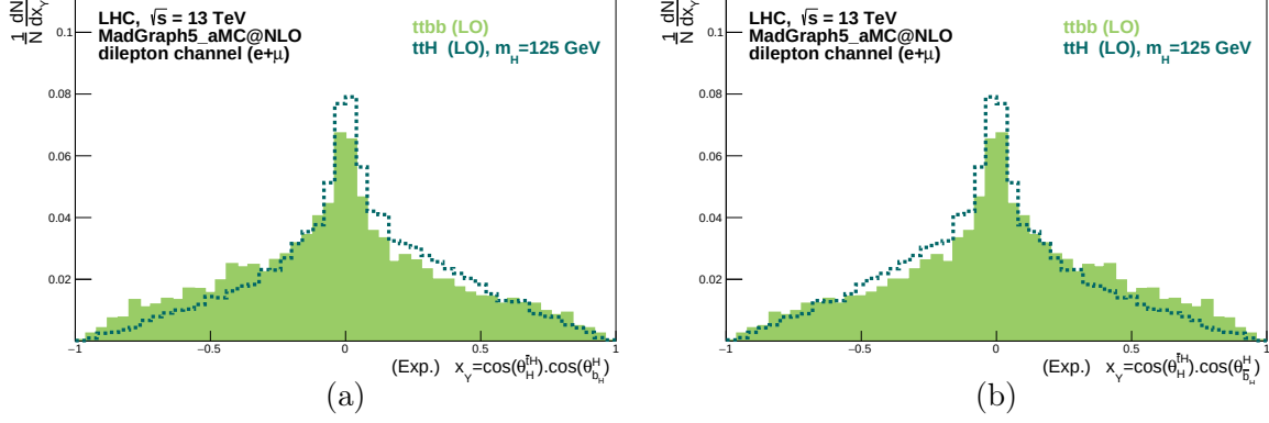
Figure 8.5: Angular distributions (a) \cos(\theta_H^{tH}) \times \cos(\theta_{bH}^H) and (b) \cos(\theta_H^{tH}) \times \cos(\theta_{bH}^H) after event selection and full kinematic reconstruction. \theta_H^{tH} is the angle between the direction of the momentum of the H boson (in the \bar{t}H centre-of-mass frame) with respect to the direction of the momentum of the \bar{t}H system (in the t\bar{t}H centre-of-mass frame), while \theta_{bH}^H ( \theta_{\bar{b}H}^H ) is the angle between the direction of the momentum of the b ( \bar{b} ) jet coming from the Higgs boson (in the H centre-of-mass system) and the direction of the H boson momentum (in the \bar{t}H centre-of-mass frame).
