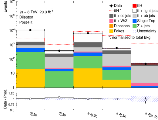
Figure 7.12: Post-fit summary of the MC prediction to data comparison after in all analysis regions. The signal is shown in red, both normalised to the SM prediction (filled red area stacked on the background) and normalised to the total number of background events (dashed red line). The total uncertainty on the yields is represented by the hashed area.
