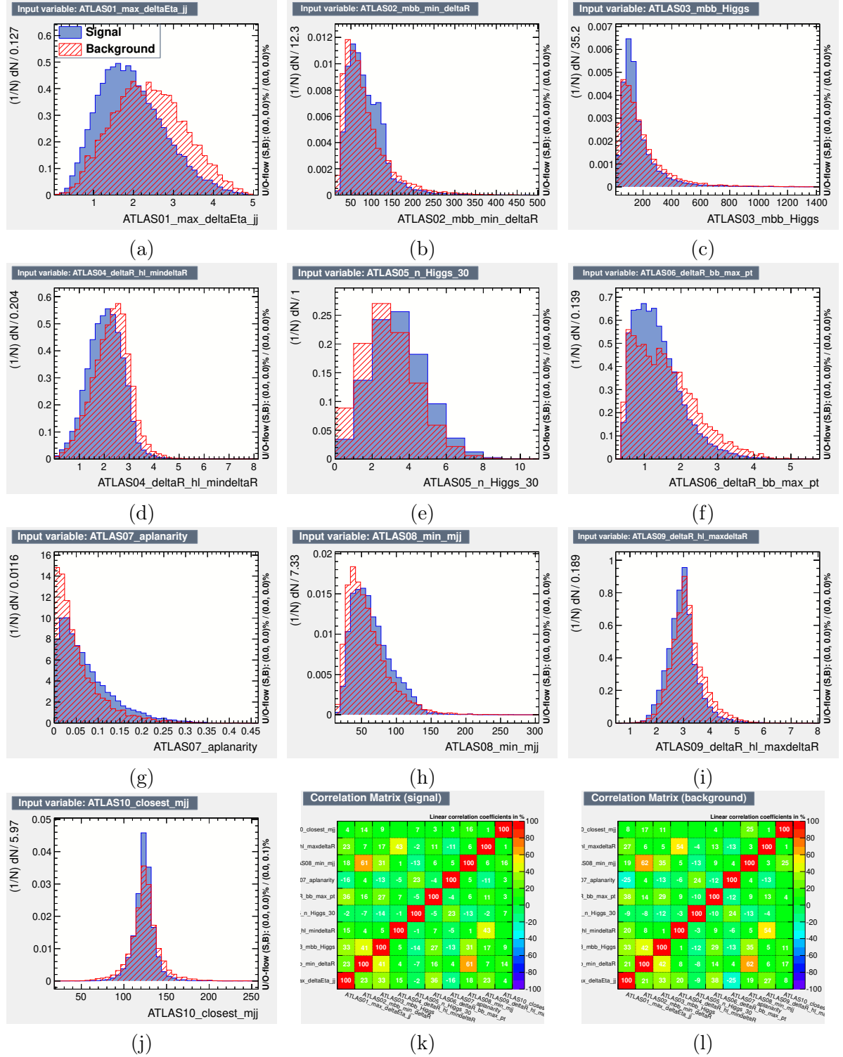
Figure 7.6: Normalised distributions of the NN highest-ranked input variables in the (\geq 4j, \geq 4b) region: (a) \Delta\eta_{jj}^{\max}\Delta\eta ; (b) m_{bb}^{\min}\Delta R ; (c) m_{bb} ; (d) \Delta R_{hl}^{\min}\Delta R ; (e) N_{30}^{\text{Higgs}} ; (f) \Delta R_{bb}^{\max p_T} ; (g) A_{\text{plan}_{\text{jet}}} ; (h) m_{jj}^{\min m} ; (i) \Delta R_{hl}^{\max}\Delta R ; and (j) m_{jj}^{\text{closest}} . The correlation among the variables are also shown, (k) for the signal and (l) for the background events.
