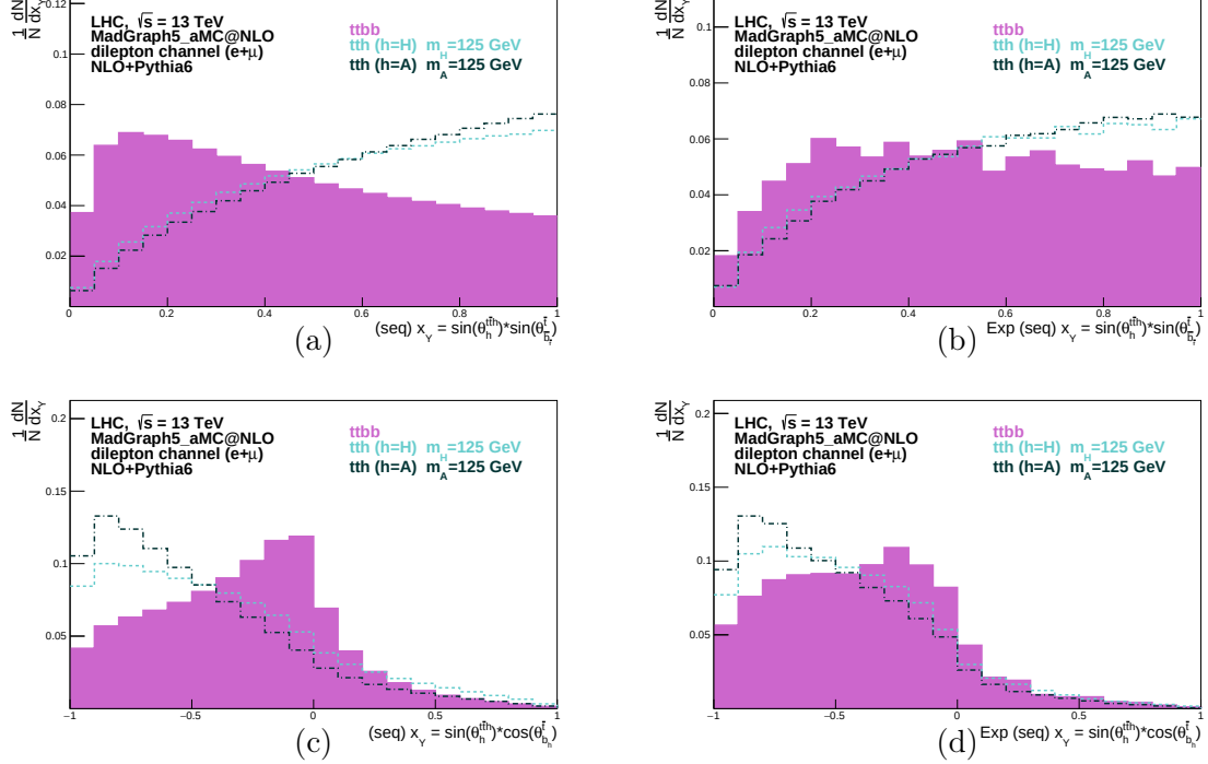
Figure 8.9: Distributions of x_Y = \sin(\theta_h^{t\bar{t}h}) \sin(\theta_{b\bar{t}}^f) (top) and x_Y = \sin(\theta_h^{t\bar{t}h}) \cos(\theta_{b\bar{t}}^f) (bottom). The distributions at parton level ((a) and (c)) and after selection cuts, full kinematic reconstruction and extra b -tag multiplicity and m_{\ell\ell} requirements ((b) and (d)), are shown. The dashed line represents the t\bar{t}h SM model signal (where h represents H , the SM Higgs boson with CP = +1 ) and the dashed-dotted line corresponds to the pure pseudoscalar distribution t\bar{t}h (where h represents A , the pseudoscalar boson with CP = -1 ). Here, the laboratory four-momentum of b quarks is boosted sequentially to the Higgs centre of mass system [4]
