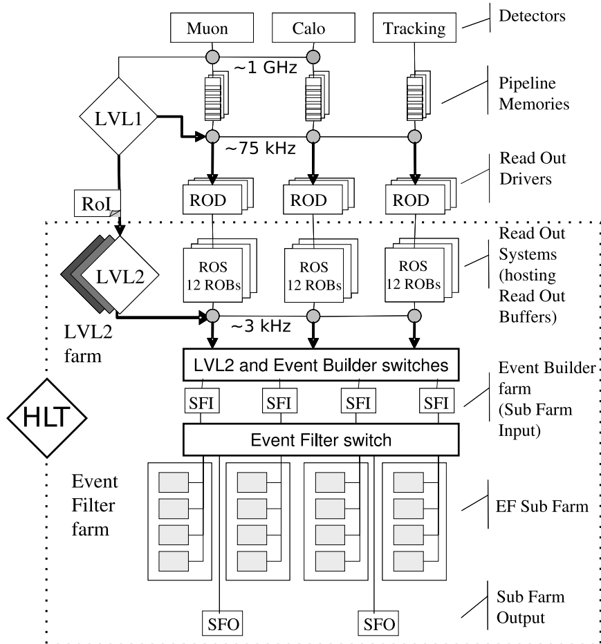
Figure 3.12: Block Diagram of the Trigger and DAQ system [187].
