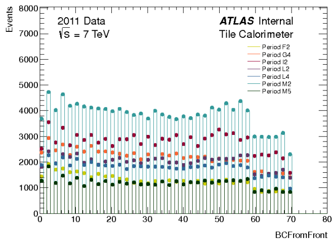
Figure 4.18: Distribution of the bunch crossing IDs for several periods of \sqrt{s} = 7 TeV data. The dots represent the data, one run from each period F2, G4, I2, L2, L4, M2 and M5 according to the colours in the legend [2].
