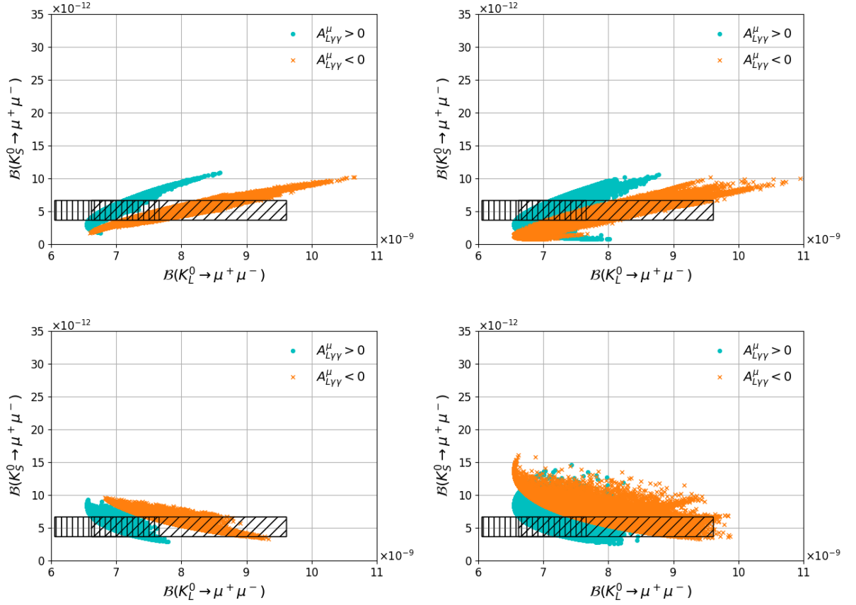
Figure 5.5: Scenario B, motivated by Higgsino Dark Matter with universal gaugino masses: \mathcal{B}(K_S^0 \rightarrow \mu^+\mu^-) vs \mathcal{B}(K_L^0 \rightarrow \mu^+\mu^-) for (\delta_d^{LL})_{12} \neq 0 and (M_3 \cdot \mu) > 0 (upper left), (\delta_d^{LL})_{12} \neq 0 and (M_3 \cdot \mu) < 0 (upper right), (\delta_d^{RR})_{12} \neq 0 and (M_3 \cdot \mu) > 0 (lower left), and (\delta_d^{RR})_{12} \neq 0 and (M_3 \cdot \mu) < 0 (lower right). The cyan dots correspond to A_{L\gamma\gamma}^\mu > 0 and the orange crosses to A_{L\gamma\gamma}^\mu < 0 . The vertically hatched area corresponds to the SM prediction for A_{L\gamma\gamma}^\mu > 0 and the inclined hatched area corresponds to the SM prediction for A_{L\gamma\gamma}^\mu < 0 .
