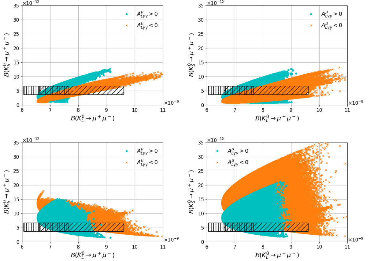
Figure 5.3: Scenario A: \mathcal{B}(K_S^0 \rightarrow \mu^+\mu^-) vs \mathcal{B}(K_L^0 \rightarrow \mu^+\mu^-) for (\delta_d^{LL})_{12} \neq 0 and (M_3 \cdot \mu) > 0 (upper left), (\delta_d^{LL})_{12} \neq 0 and (M_3 \cdot \mu) < 0 (upper right), (\delta_d^{RR})_{12} \neq 0 and (M_3 \cdot \mu) > 0 (lower left), and (\delta_d^{RR})_{12} \neq 0 and (M_3 \cdot \mu) < 0 (lower right). The cyan dots correspond to A_{L\gamma\gamma}^\mu > 0 and the orange crosses to A_{L\gamma\gamma}^\mu < 0 . The vertically hatched area corresponds to the SM prediction for A_{L\gamma\gamma}^\mu > 0 and the inclined hatched area corresponds to the SM prediction for A_{L\gamma\gamma}^\mu < 0 .
