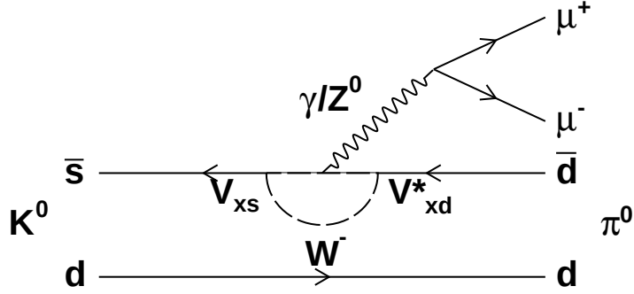
Figure 5.13: Feynman diagram of the process K^0 \rightarrow \pi^0 \mu^+ \mu^- .
