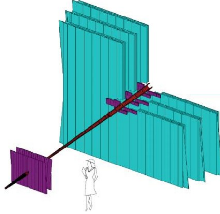
Figure 4.7: Arrangement of OT straw-tube modules in layer and stations. Figure taken from Ref. [74].
