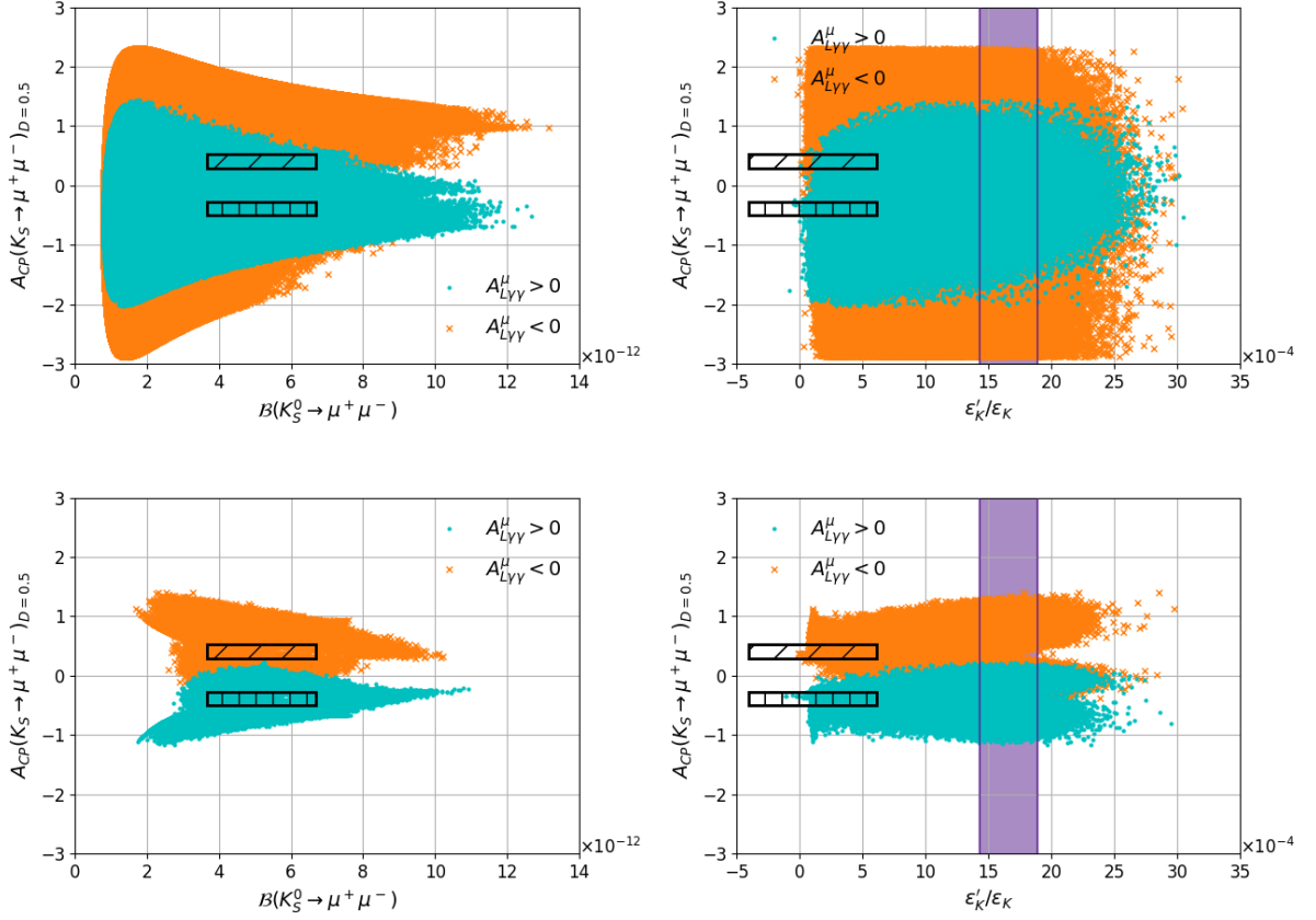
Figure 5.10: A_{CP} vs \mathcal{B}(K_S^0 \rightarrow \mu^+ \mu^-) (left) and vs \varepsilon'_K/\varepsilon_K (right). The top panels correspond to Scenario A, (\delta_d^{LL})_{12} \neq 0 and (M_3 \cdot \mu) < 0 . The bottom panels correspond to Scenario B, (\delta_d^{LL})_{12} \neq 0 and (M_3 \cdot \mu) > 0 . The plots are done for D = -D' = 0.5 . The cyan dots correspond to A_{L\gamma\gamma}^\mu > 0 and the orange crosses to A_{L\gamma\gamma}^\mu < 0 . The deep purple bands correspond to the experimental value of \varepsilon'_K/\varepsilon_K , the vertically hatched areas correspond to the SM prediction for A_{L\gamma\gamma}^\mu > 0 and the inclined hatched areas to the SM prediction for A_{L\gamma\gamma}^\mu < 0 .
