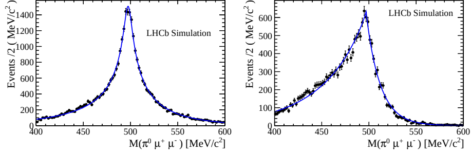
Figure 5.28: Signal fit using the Hypathia function for FULL (left) and PARTIAL (right) categories.
