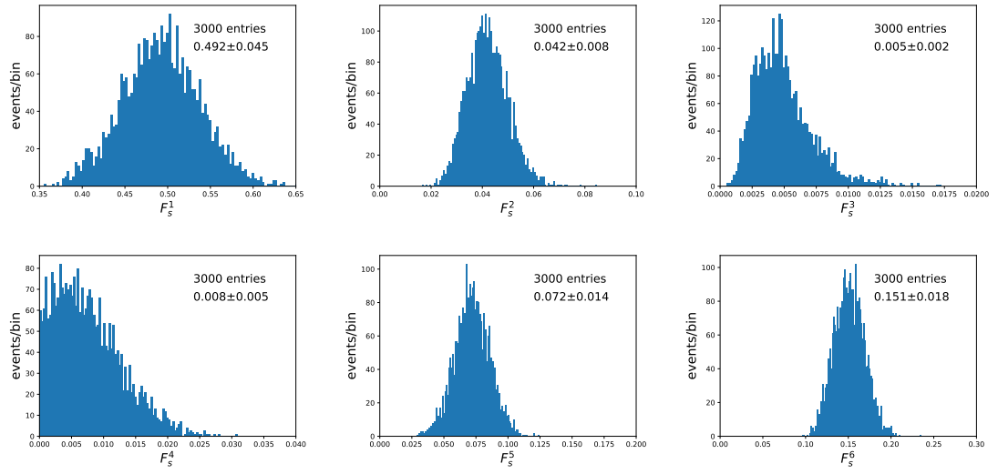
Figure D.4: Distributions of the fit parameters using bootstrapping (data).
