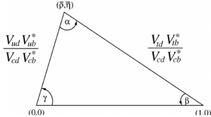
Figure 3.1: Unitarity Triangle, using the Wolfenstein parametrization [59]. Figure taken from Ref. [60].
