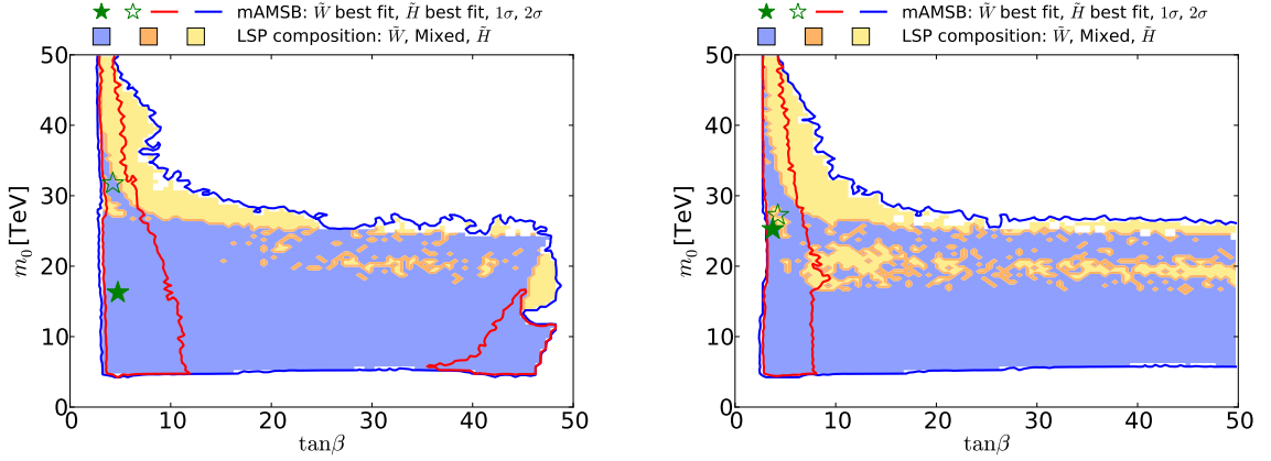
Figure 7.14: The (\tan\beta, m_0) planes for \mu > 0 (left panel) and for \mu < 0 (right panel), assuming that the \tilde{\chi}_1^0 provides all the CDM density. The colouring convention for the shadings and contours is the same as in Figure 7.13, and the best-fit points for the two signs of \mu are again indicated by green stars.
