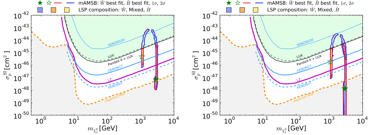
Figure 7.22: The (m_{\tilde{\chi}_1^0}, \sigma_p^{SI}) planes in the mAMSB for \mu > 0 (left) and \mu < 0 (right) in the case when the LSP accounts for the whole DM density. The red and blue solid lines are the 1 and 2 CL contours, and the solid purple and blue lines show the projected 95% exclusion sensitivities of the LUX-Zeplin (LZ) [319] and XENON1T/nT experiments [318], respectively. The green line and shaded region show the combined limit from the LUX and PandaX experiments [302, 303], and the dashed orange line shows the astrophysical neutrino ‘floor’ [305], below which astrophysical neutrino backgrounds dominate (grey region). The blue, orange and yellow shadings are the same as in Figure 7.13.
