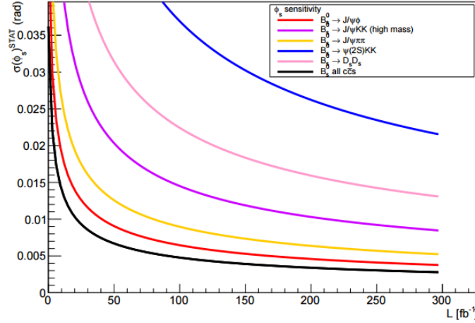
Figure 6.14: Expected sensitivity for \phi_s as a function of the luminosity. The current central value is \phi_s^{c\bar{c}s} = -0.021 \pm 0.031 [245], and the SM prediction: -2\beta_s = -0.0364 \pm 0.0016 \text{ rad} [222].
