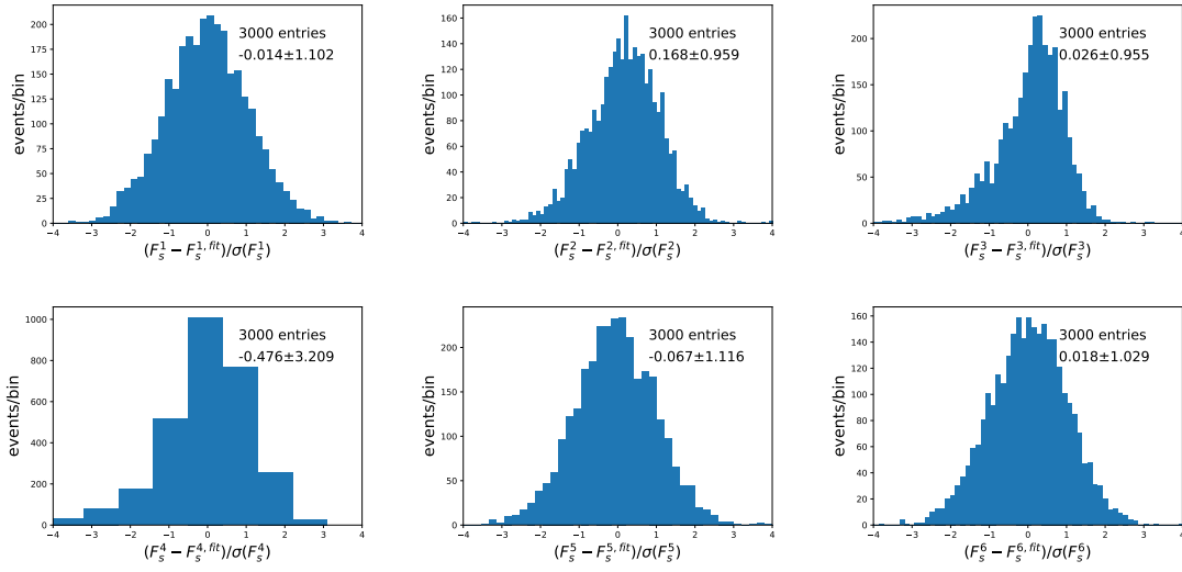
Figure D.6: Pull distributions of the fit parameters using bootstrapping (data). Pulls are computed relative to data central values.
