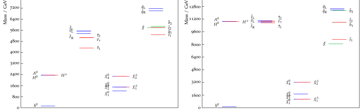
Figure 7.12: The spectra of Higgs bosons and sparticles at the best-fit points in the CMSSM for \mu < 0 (left) and \mu > 0 (right). These plots were made using PySLHA [270].
