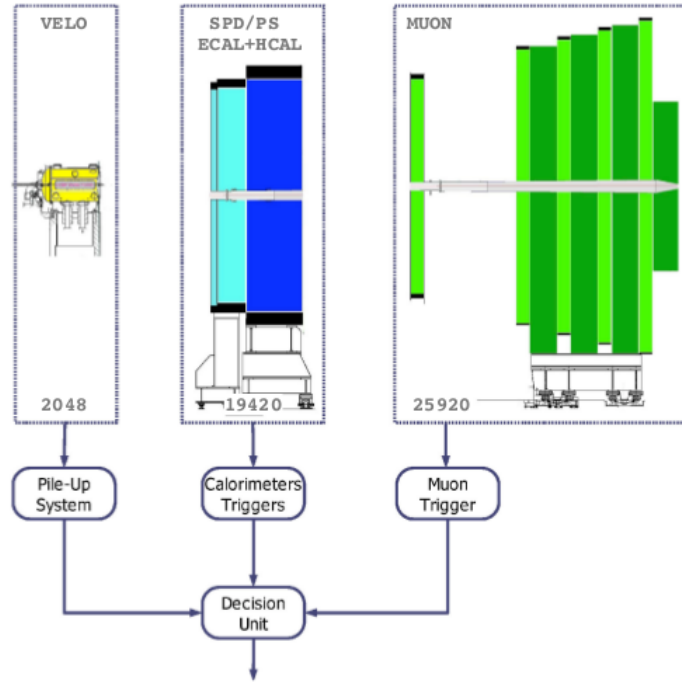
Figure 4.15: Overview of the L0. Figure taken from Ref. [74].
