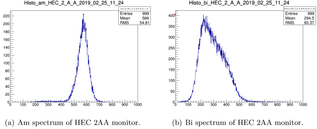
Figure 12.6: Am (left) and Bi (right) spectra for HEC 2AA LAr purity monitor. HV module for Bi source of HEC 1AA monitor is switched off. So, Bi HV module of HEC 1AA monitor impacts Bi spectrum of HEC 2AA monitor.
