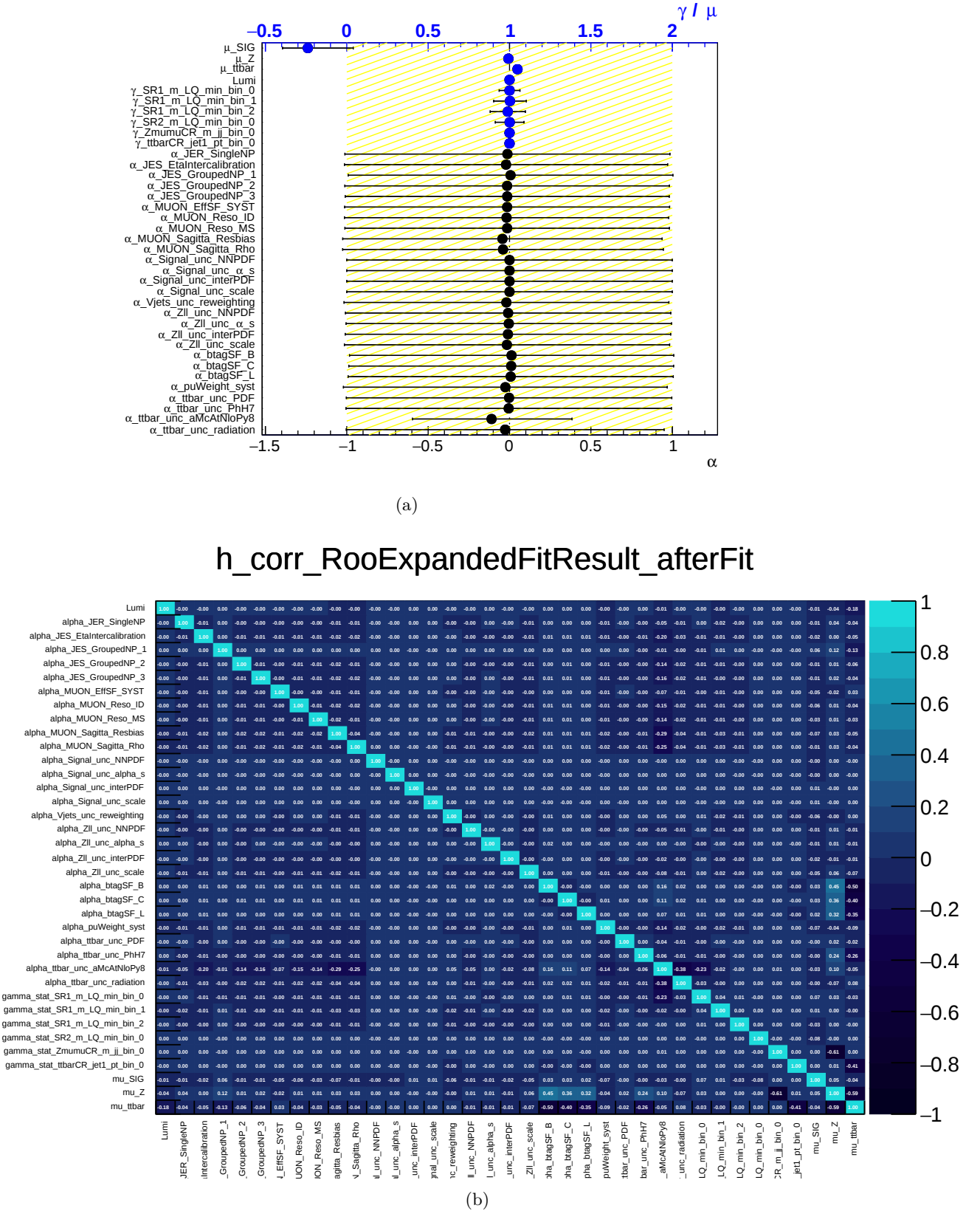
Figure 8.3: Fit diagnostics for the example of an LQ mass hypothesis of 1.4 TeV in muon channel. (a): fit parameters, (b): correlation matrix.
