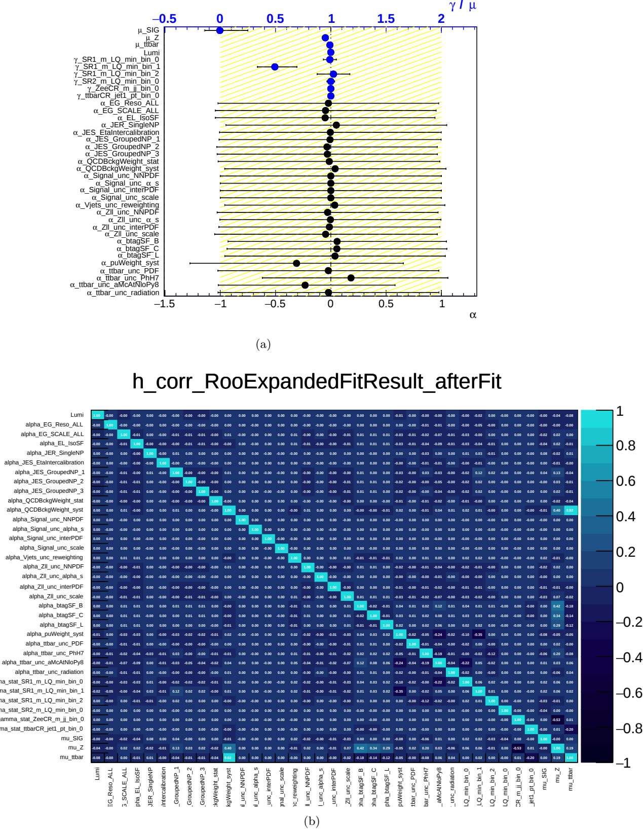
Figure 8.2: Fit diagnostics for the example of an LQ mass hypothesis of 1.4 TeV in electron channel. (a): fit parameters, (b): correlation matrix.
