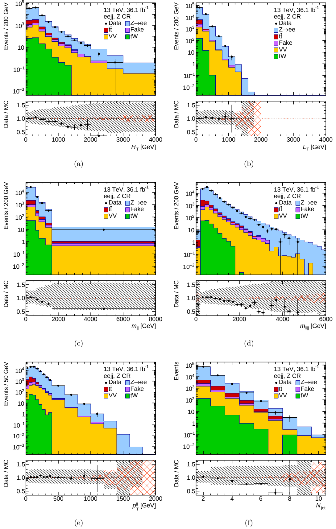
Figure 7.9: Kinematic distributions of H_T , L_T , m_{jj} , m_{ljj} , p_T^{ll} and N_{jet} (see Table 7.2 for the variable descriptions) in the Z CR for the electron channel. The gray band displays the total systematic uncertainty. The hatched orange band shows the statistical uncertainty in the simulation.
