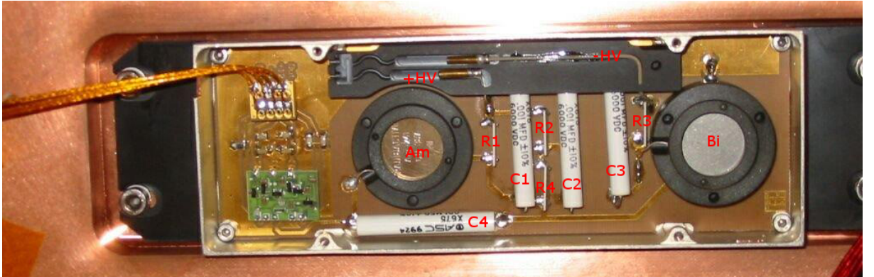
Figure 11.14: The standard configuration of the basic monitor as it is used in ATLAS detector (here just before complete construction) [240]. The red description of the components is based on the convention given in Figure 11.11.
