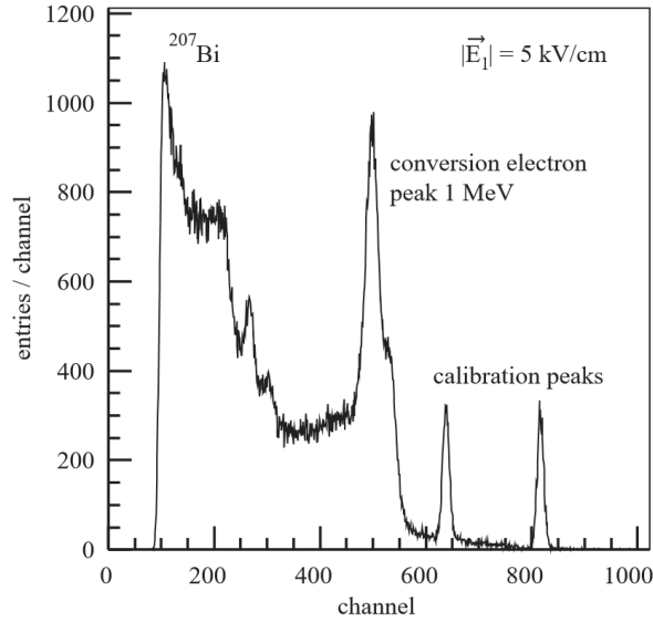
Figure 11.9: Signal spectrum of the ^{207}\text{Bi} -cell recorded with the CERN testbeam setup ( p \approx 0.3\text{ ppmO}_2 ). The two conversion electron lines at 1047 keV and 976 keV are not resolved separately and form the largest peak. The \gamma -line at 1064 keV is strongly suppressed. The background on the left from it consists of the Compton continuum with the Compton-edge at 858 keV and the contributions to the \gamma -line at 569 keV. Calibration peaks are used to monitor the stability of the electronics chain [234].
