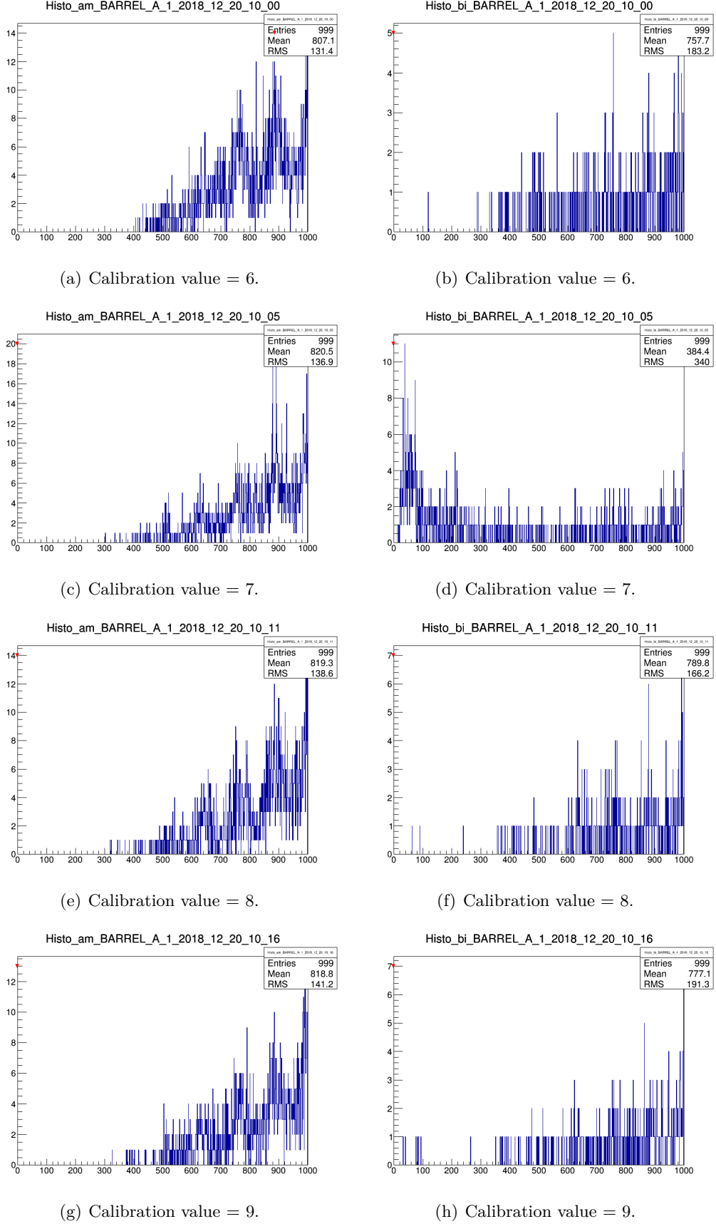
Figure D.2: Am (left) and Bi (right) spectra for Barrel A1 LAr purity monitor. The calibration value is set to 6, 7, 8, 9 from the first row to the last, and HV is off.
