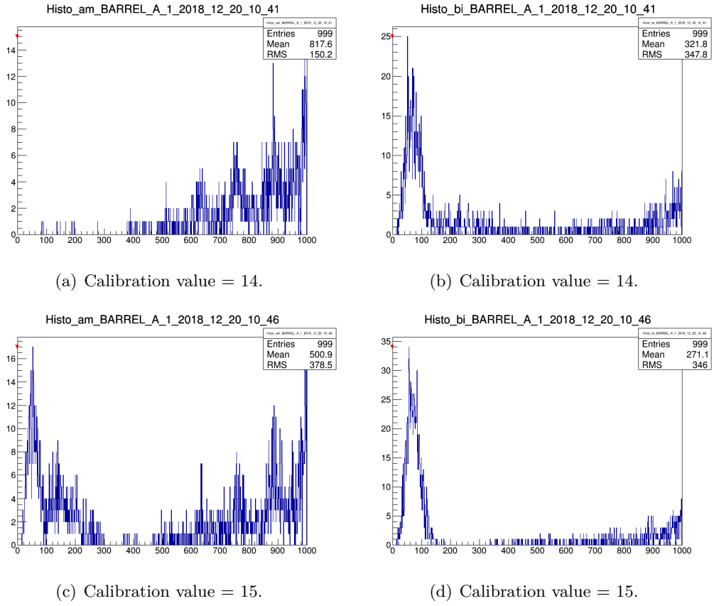
Figure D.4: Am (left) and Bi (right) spectra for Barrel A1 LAr purity monitor. The calibration value is setted to 14 (top) and 15 (bottom), and HV is off.
