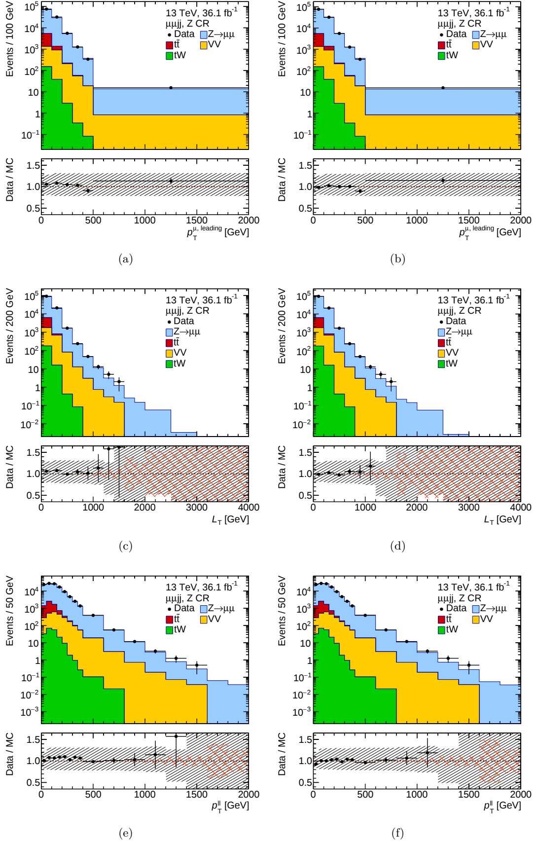
Figure 7.19: Distributions of p_T^{\mu, \text{leading}} , L_T and p_T^{\text{ll}} in the Z CR for the muon channel before (left) and after (right) reweighting in m_{jj} . The gray band displays the total systematic uncertainty. The hatched orange band shows the statistical uncertainty in the simulation.
