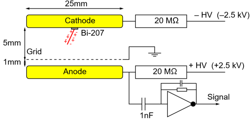
Figure 11.8: Schematic view of the ^{207}\text{Bi} -cell. Conversion electrons of \approx 1\text{ MeV} ionize the LAr along their \approx 3\text{ mm} long tracks in front of the cathode. Only electrons drifting between the grid and the anode are taken into account for the signal [234].
