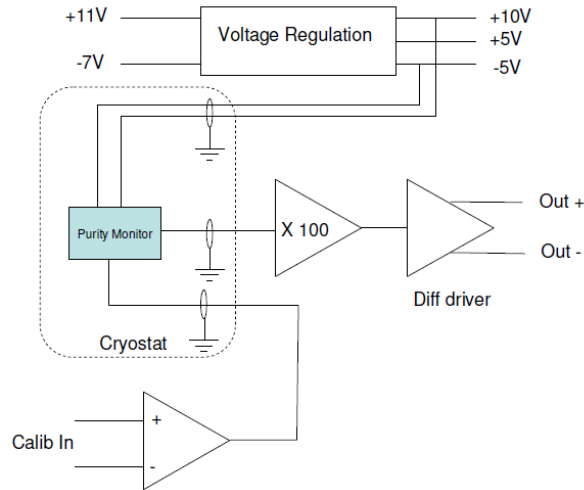
Figure 11.15: Block diagram of the functionality of the FEB [242].
