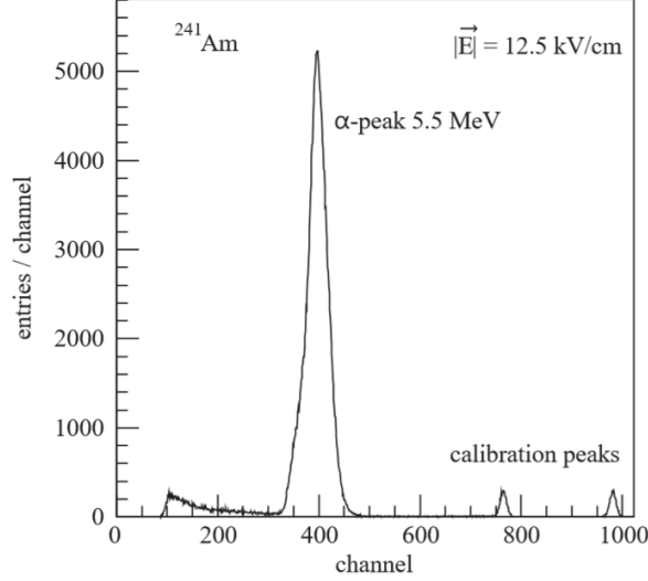
Figure 11.6: Signal spectrum of the ^{241}\text{Am} -cell recorded with the CERN testbeam setup ( p \approx 0.3 \text{ ppmO}_2 ). Calibration peaks are used to monitor the stability of the electronics chain [234].
