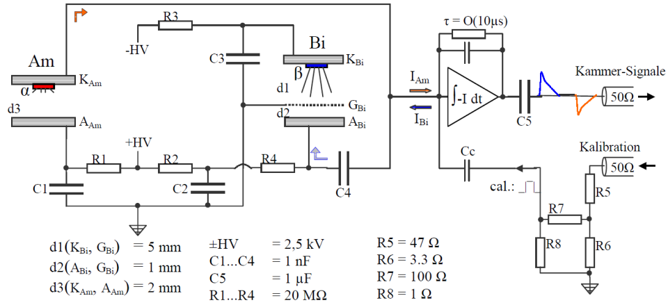
Figure 11.11: Schematic presentation of the basic monitor [239].
