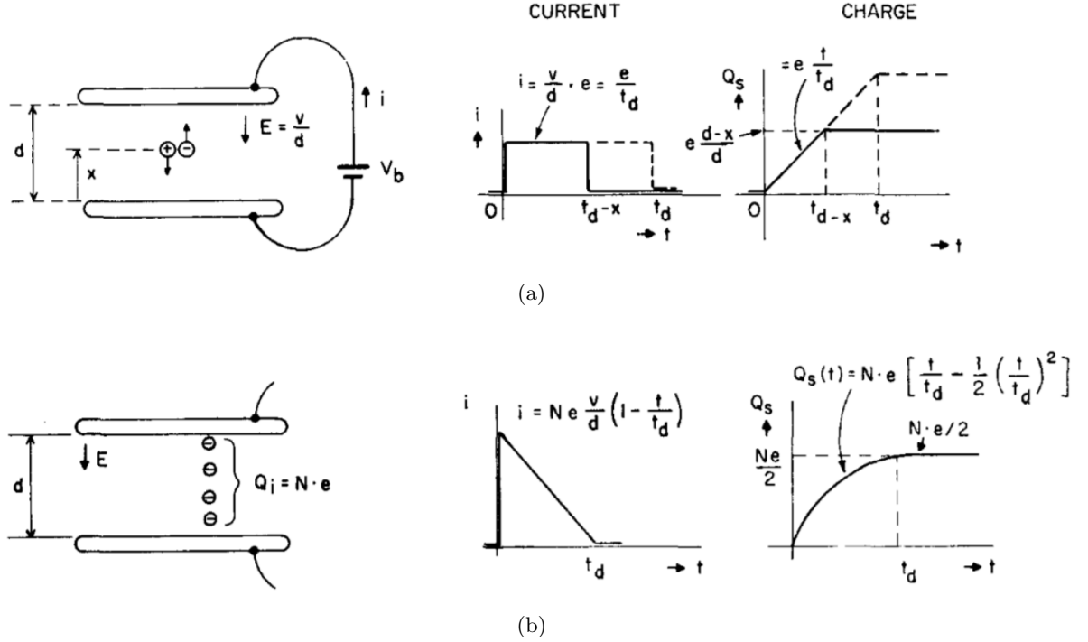
Figure 11.1: Charge collection in LAr chamber, (a) single ion pair (solid lines), and for ions formed at the negatively biased plate (dashed lines); (b) uniform ionization [230].
