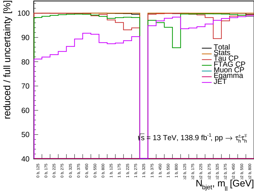
Figure 3.6: Ratio between the uncertainties before and after pruning on the MC m_{\ell\ell} \mathcal{T}_{\text{had}} \mathcal{T}_{\text{had}} distribution after the unfolding. For the before and after pruning distributions, including the e\mu region, see Figure D.2 in Appendix D.1. The gap at 1 b, 325 GeV is due to having empty bins.
