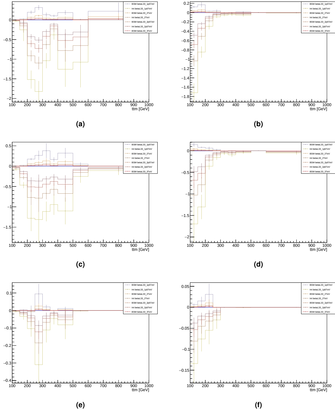
Figure 3.8: Signal events of the high mass opposite sign \tau_{\text{had}} \tau_{\text{had}} (left side plots) and e\mu (right side plots) regions for the m_{\text{H}}^{\text{total}} variable for the different masses 1.5 TeV to 3 TeV. The \hat{s}_{\text{min}}^{1/2} and m_{\ell\ell} variable can be found in the Appendix D.4. Visible are the above mentioned problematic negative bins for the maximum likelihood fit.
