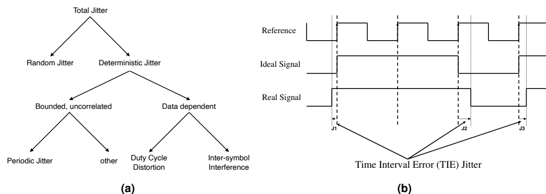
Figure 5.4: (a) shows the hierarchy of the different jitter categories and (b) the standard definition of jitter on a digital signal, also referred to as TIE or total jitter. A reference signal is provided or generated (usually a clock) and the real signal is compared to the 0-to-1 or 1-to-0 transitions of the reference signal. Figures taken from [197, 198].
