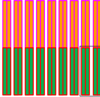
Figure 4.15: Sketch of the EC L4 rings. The black border marks the four SP chains of ring 8 and 9 used in the example.
