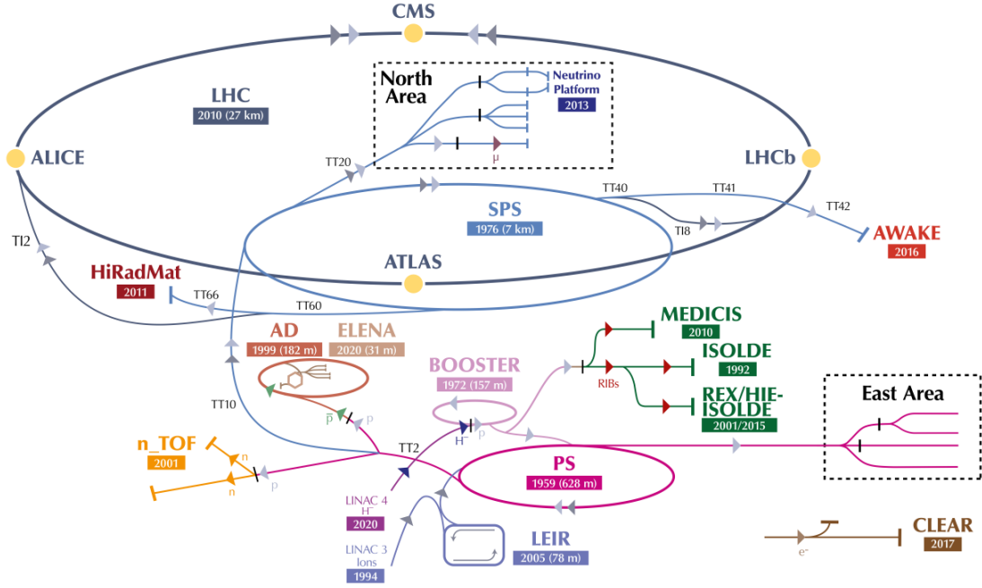
Figure 2.2: The CERN accelerator complex. Visible are the LHC and its main pre-accelerators plus many different, smaller experiments that profit from the several accelerators. Figure (adjusted) taken from [54].
