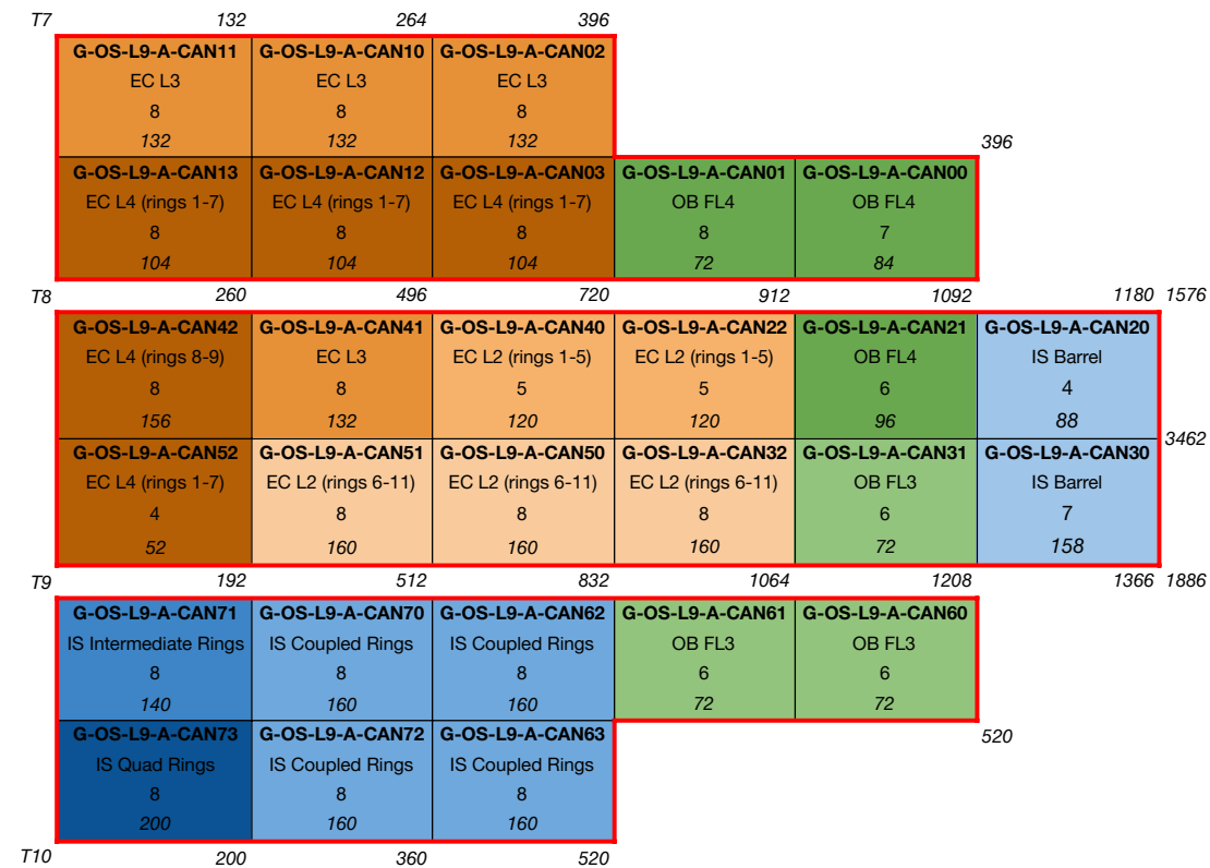
Figure 4.16: Optobox distribution in the A side sector 9 Optopanel (DFT a4-5). Each box represents an Optobox, its background colour is to distinguish the different layers. The Optobox ID is bold and the layer name is given below. The first number in each box is the amount of Optoboards and the italic number the amount of Twinax cables ending at that Optobox. The thicker, coloured border indicates the source of powering cavern – in this sector all the same from USA15.
