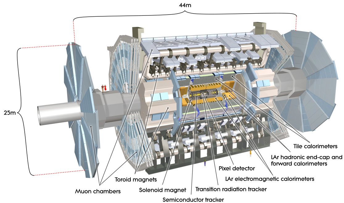
Figure 2.5: Rendering of the complete, current ATLAS detector and its main sub-detectors. Figure taken from [65].
