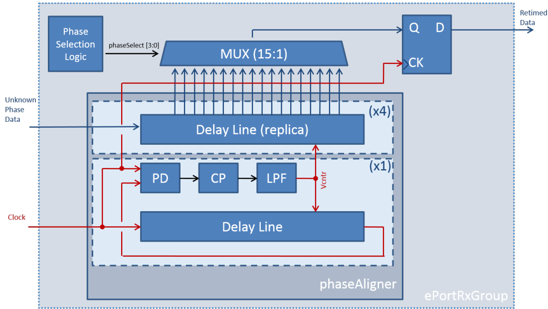
Figure 5.12: The eLink phase aligner. It consists mainly of the DLL (lower light blue background rectangle) and four delay lines (upper light blue background). The Phase Selection Logic sets the phase EPRX[G]OChnCntr[7:4] with the Multiplexer (MUX) and together with the IpGBT outputs the retimed data. Figure taken from [183].
