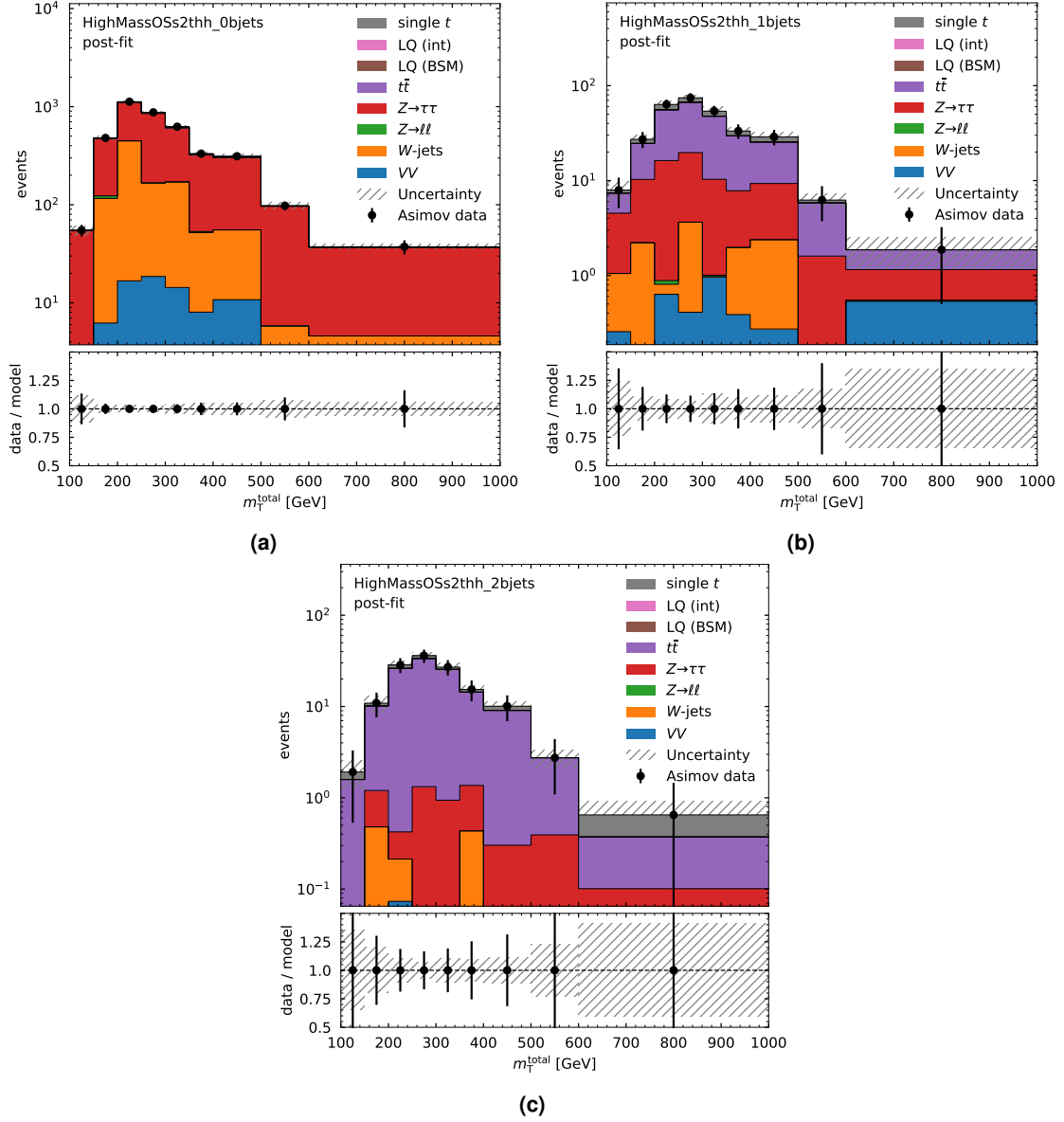
Figure D.8: Post-fit distributions of the di-lepton m_T^{\text{total}} in high-mass, opposite-sign \tau_{\text{had}}\tau_{\text{had}} region for the \beta_L^{b\tau} = 1 , m_{LQ} = 2 \text{ TeV} fit. Distributions are shown (a) in the 0, (b) 1, and (c) 2+ b -jet multiplicity regions after the fit is performed. Uncertainties include the process modelling and cross section uncertainties described in Section 3.4.
