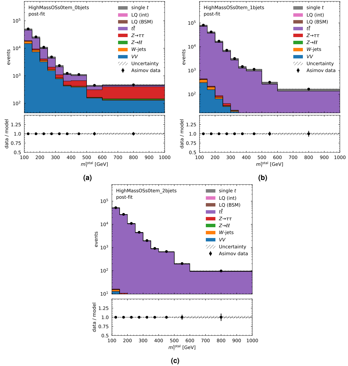
Figure D.9: Post-fit distributions of the di-lepton m_l^{\text{total}} in high-mass, opposite-sign e\mu region for the \beta_L^{b\tau} = 1 , m_{LQ} = 2 TeV fit. Distributions are shown (a) in the 0, (b) 1, and (c) 2+ b -jet multiplicity regions after the fit is performed. Uncertainties include the process modelling and cross section uncertainties described in Section 3.4.
