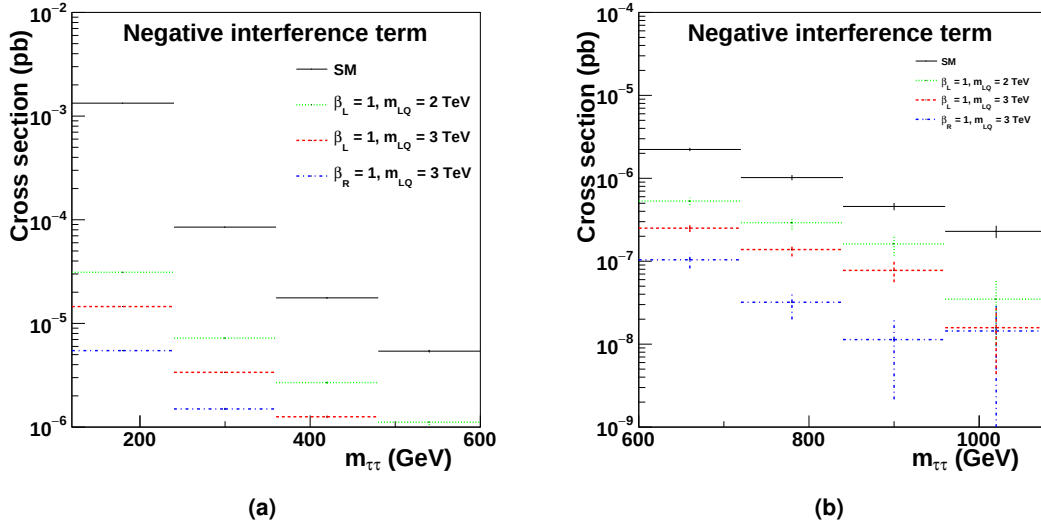
Figure 3.2: Predicted particle-level cross sections for Drell-Yan di- \tau production for the SM as well the expected interference for several leptoquark scenarios. In all cases above, the predicted correction from interference reduces the total cross section, so its absolute value is reported. The differential m_{\tau\tau} distribution is shown in the 1- b -jet region for: (a) 100 < m_{\tau\tau}/\text{GeV} < 600 , and (b) 600 < m_{\tau\tau}/\text{GeV} < 1000 . Note: these are differential cross sections ( \frac{d\sigma}{dm_{\tau\tau}} [pb / GeV]) despite the y-axis label.
