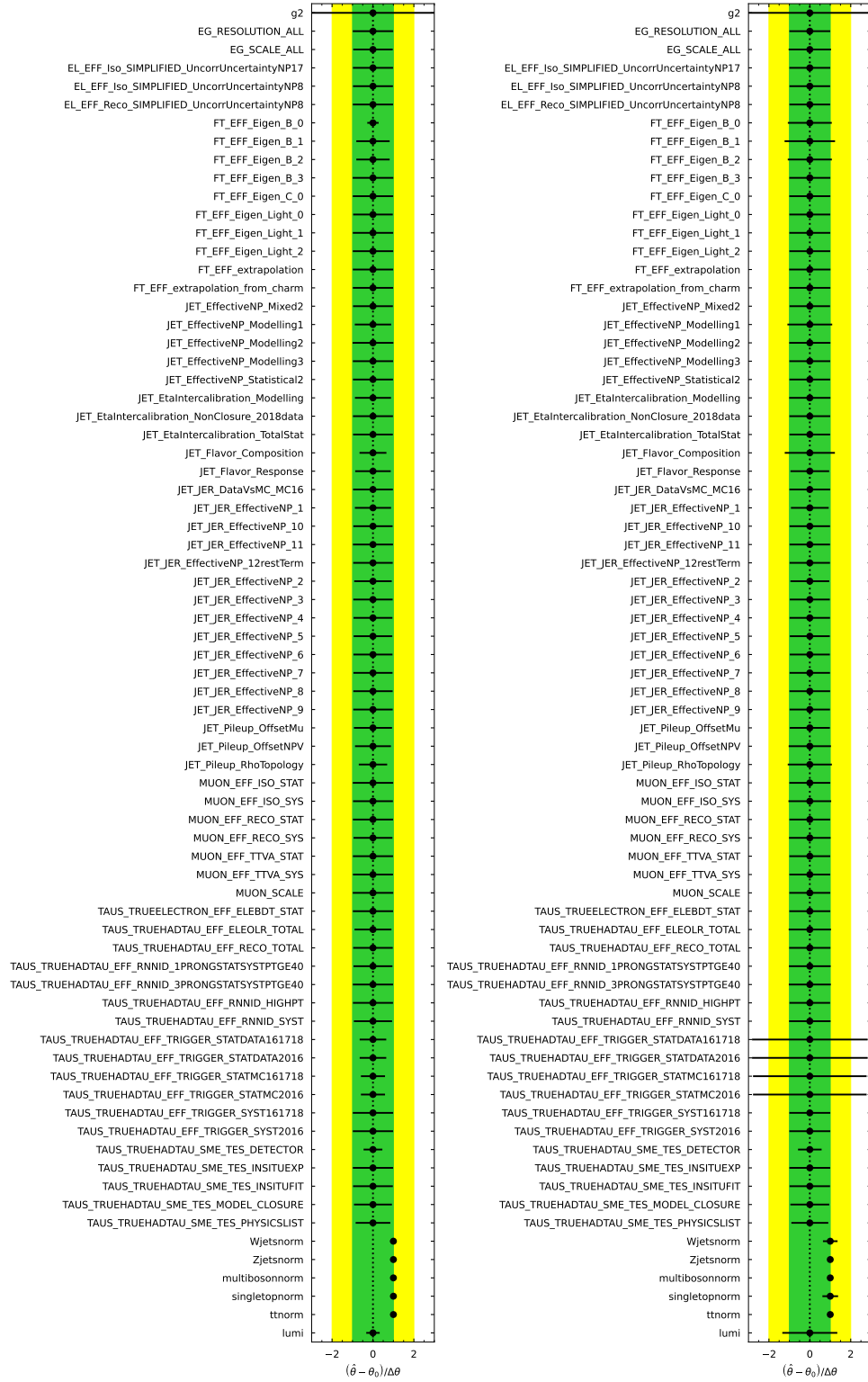
Figure D.14: Pull plots of the \hat{s}_{\min}^{1/2} variable.
