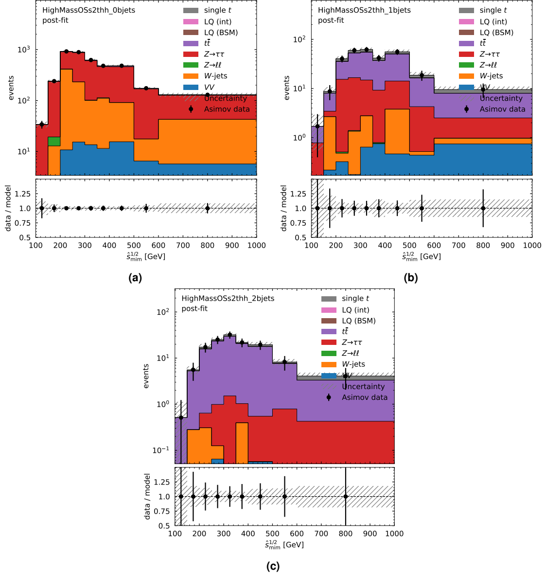
Figure D.10: Post-fit distributions of the di-lepton \hat{s}_{\text{mim}}^{1/2} in high-mass, opposite-sign \tau_{\text{had}}\tau_{\text{had}} region for the \beta_L^{b\tau} = 1 , m_{\text{LQ}} = 2 TeV fit. Distributions are shown (a) in the 0, (b) 1, and (c) 2 b -jet multiplicity regions after the fit is performed. Uncertainties include the process modelling and cross section uncertainties described in Section 3.4.
