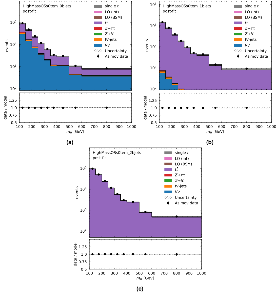
Figure 3.14: Post-fit distributions of the di-lepton m_{\ell\ell} in high-mass, opposite-sign e\mu region for the \beta_L^{b\tau} = 1 , m_{LQ} = 1.5 TeV fit. Distributions are shown (a) in the 0, (b) 1, and (c) 2 b -jet multiplicity regions after the fit is performed. Uncertainties include the process modelling and cross section uncertainties described in Section 3.4.
