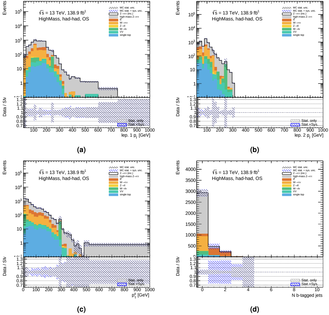
Figure 3.7: Distributions of MC simulation for a number of kinematic quantities in the high-mass, opposite-sign, \tau_{\text{had}}\tau_{\text{had}} region: (a) the leading \tau_{\text{had}} p_T^{\text{vis}} , (b) the subleading \tau_{\text{had}} p_T^{\text{vis}} , (c) the p_T^{\text{vis}} of the \tau_{\text{had}}\tau_{\text{had}} system, and (d) the b -jet multiplicity.
