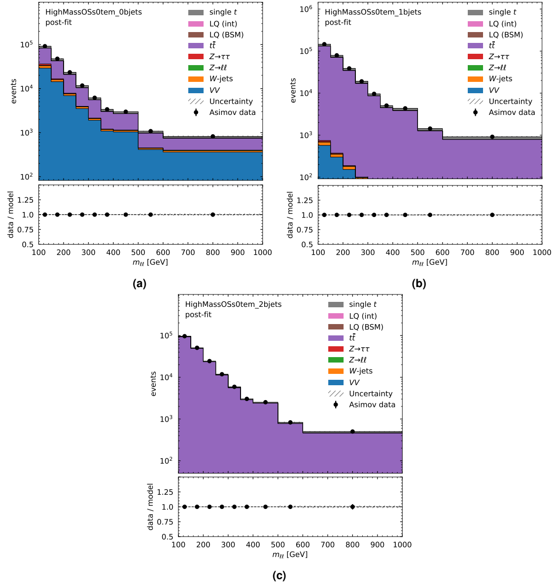
Figure D.13: Post-fit distributions of the di-lepton m_{\ell\ell} in high-mass, opposite-sign e\mu region for the \beta_L^{b\tau} = 1 , m_{LQ} = 2\text{ TeV} fit. Distributions are shown (a) in the 0, (b) 1, and (c) 2 b -jet multiplicity regions after the fit is performed. Uncertainties include the process modelling and cross section uncertainties described in Section 3.4.
