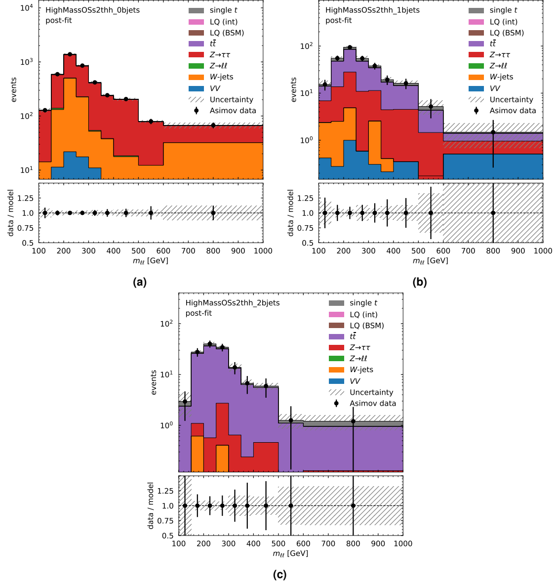
Figure 3.13: Post-fit distributions of the di-lepton m_{\ell\ell} in high-mass, opposite-sign \tau_{\text{had}}\tau_{\text{had}} region for the \beta_L^{b\tau} = 1 , m_{\text{LQ}} = 1.5 \text{ TeV} fit. Distributions are shown (a) in the 0, (b) 1, and (c) 2 b -jet multiplicity regions after the fit is performed. Uncertainties include the process modelling and cross section uncertainties described in Section 3.4.
