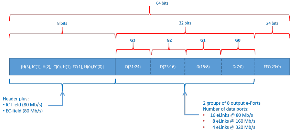
Figure 5.8: The lpGBT downlink frame before interleaving, i.e. rearranging the code for error corrections at the transmitter or after it has been de-interleaved at the receiver. The uplink frame is very similar to this one, differing only in bit lengths. Figure taken from [183].
