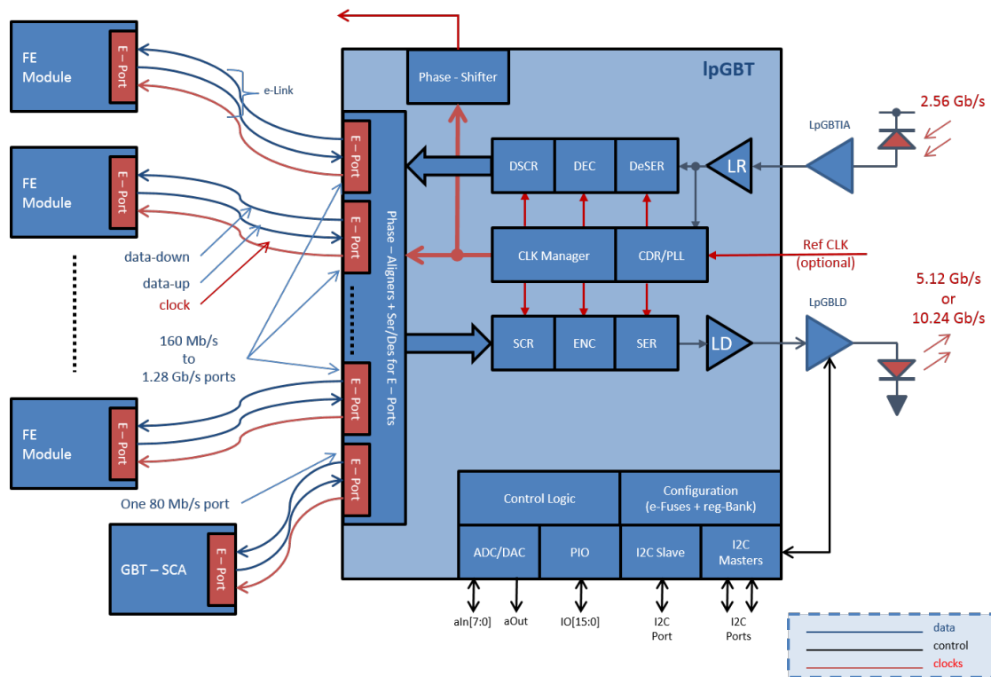
Figure 5.7: Overview of the lpGBT architecture. The downlink is defined as going from right to left, whereas the uplink goes from the FE modules on the left to the right. Note that in the case of the ITk Pixel data transmission chain, no specific clock lines are used between the FE modules and the ePorts. The clock is embedded in the electrical downlink (here “data-down”). Figure taken from [183].
