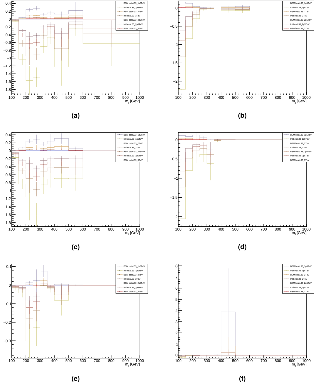
Figure D.7: Signal events of the high mass opposite sign \tau_{\text{had}} \tau_{\text{had}} (left side plots) and e\mu (right side plots) regions for the m_{\tau}^{\text{total}} variable.
