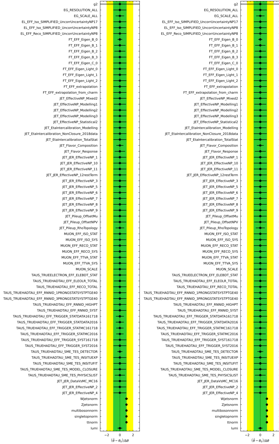
Figure D.16: Pull plots of the m_{\ell\ell} variable.
