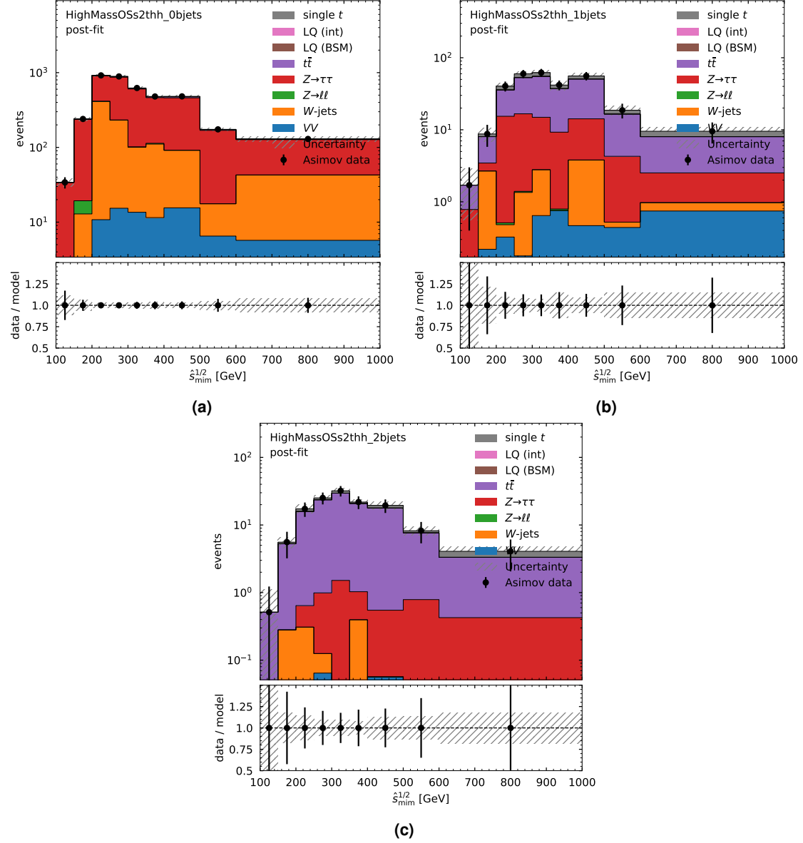
Figure 3.11: Post-fit distributions of the di-lepton \hat{s}_{\text{mim}}^{1/2} in high-mass, opposite-sign \tau_{\text{had}}\tau_{\text{had}} region for the \beta_L^{b\tau} = 1 , m_{\text{LQ}} = 1.5 TeV fit. Distributions are shown (a) in the 0, (b) 1, and (c) 2 b -jet multiplicity regions after the fit is performed. Uncertainties include the process modelling and cross section uncertainties described in Section 3.4.
