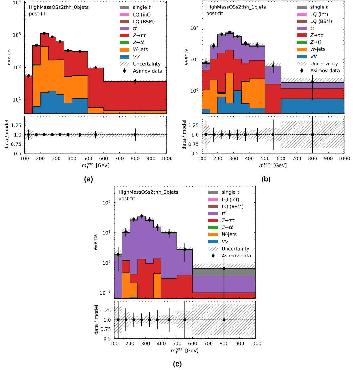
Figure 3.9: Post-fit distributions of the di-lepton m_T^{\text{total}} in high-mass, opposite-sign \tau_{\text{had}}\tau_{\text{had}} region for the \beta_L^{b\tau} = 1 , m_{LQ} = 1.5 \text{ TeV} fit. Distributions are shown (a) in the 0, (b) 1, and (c) 2+ b -jet multiplicity regions after the fit is performed. Uncertainties include the process modelling and cross section uncertainties described in Section 3.4.
