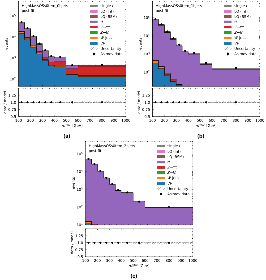
Figure 3.10: Post-fit distributions of the di-lepton m_l^{\text{total}} in high-mass, opposite-sign e\mu region for the \beta_L^{b\tau} = 1 , m_{LQ} = 1.5 TeV fit. Distributions are shown (a) in the 0, (b) 1, and (c) 2+ b -jet multiplicity regions after the fit is performed. Uncertainties include the process modelling and cross section uncertainties described in Section 3.4.
