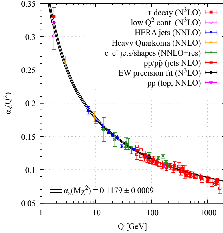
Figure 1.2: Summary of measurements of \alpha_s as a function of the energy scale Q . The respective degree of QCD perturbation theory used in the extraction of \alpha_s is indicated in brackets (Next-to-leading Order (NLO), Next-to-next-to-leading Order (NNLO), NNLO matched to a resummed calculation (NNLO+res.), Next-to-NNLO ( N^3 LO)). Figure taken from [37].
