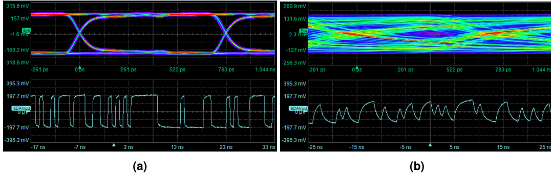
Figure 5.1: Example of a signal with 1.28 Gb/s data rate captured by an oscilloscope by taking the difference of the positive and negative amplitudes of the differential signals. The lower waveforms show a 50 ns time range of the signal voltage while the upper graphs show the eye-diagram of many signal transitions. For reference, the logical signal transmitted between -7 ns and 3 ns is 13'b1001100101010 . (a) shows the output close after the generation of the signal while (b) shows the signal after about 6 m of Twinax. Note that the time of acquisition for (a) and (b) was taken at different positions and the bit sequence does not match.
