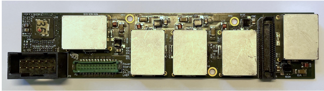
Figure 4.6: Photograph of the Powerboard. Visible are the five shields of the bPOL12V with their coils and ASICs underneath it. The green connector is for the power input coming from the detector services, while the black vertical connector mates with the Connectorboard of the Optobox. The MOPS can be seen in the upper left corner with its connector just below.
