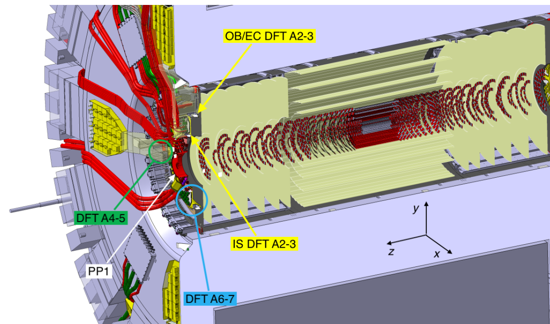
Figure 4.13: Computer generated drawing of a cut-in-half ITk. Visible are the ITk Pixel Detector's individual modules and the ITk Strips (light yellow) surrounding them. Three out of four Optopanel (in yellow) are shown with power lines (in red) for the ITk Pixel Detector coming from high r to PP1. Three DFTs are visible with the DFT A2-3 with more detail on the exact IS and OB/EC feedthrough, the fourth DFT A1-8 is cut away in this rendering. Drawing provided by Martin Janda.
