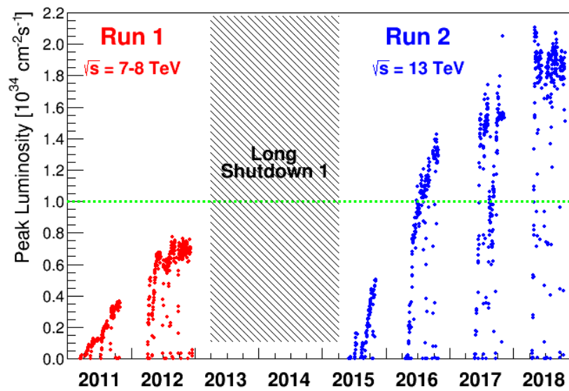
Figure 2.1: The peak luminosities of Run 1 and Run 2 delivered by the LHC up until 2018. The green horizontal line indicates the LHC's design luminosity. Note that this was before the installation of LINAC 4. Figure taken from [52].
