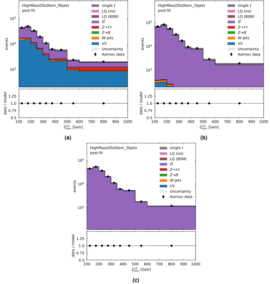
Figure 3.12: Post-fit distributions of the di-lepton s_{\min}^{1/2} in high-mass, opposite-sign e\mu region for the \beta_L^{b\tau} = 1 , m_{LQ} = 1.5 TeV fit. Distributions are shown (a) in the 0, (b) 1, and (c) 2 b -jet multiplicity regions after the fit is performed. Uncertainties include the process modelling and cross section uncertainties described in Section 3.4.
