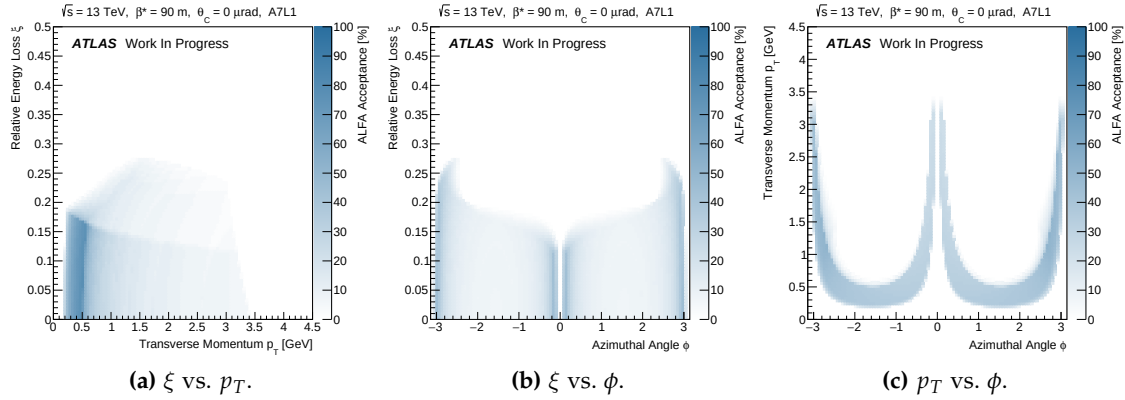
Figure 8.17: Two-dimensional projections of the ALFA acceptance plots for \theta_c = 0 \mu\text{rad} .
