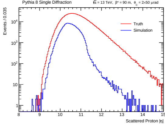
Figure 8.39: |\eta| distribution for truth level and after all smearing, acceptance, and cuts in the simulation framework.
