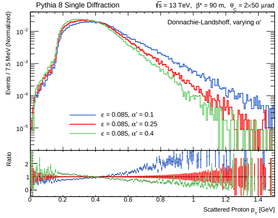
(b) DL – varying \alpha' , keeping \epsilon constant.
