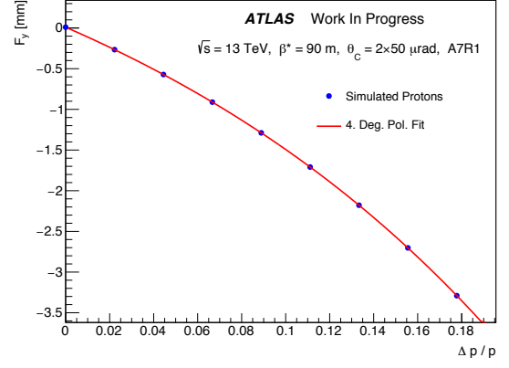
Figure 8.6: The function F_y as a function of \Delta p/p . Fitted with a fourth degree polynomial.
