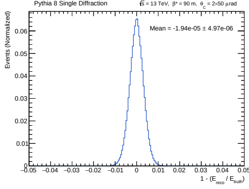
Figure 8.21: The resolution of the reconstructed E from ALFAReco.
