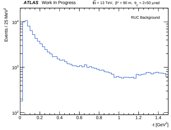
Figure 10.35: Distribution of the reconstructed t for the beam background particles in unpaired bunches.
