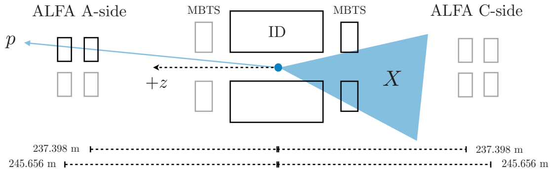
Figure 10.8: Simplified illustration of the signal diffractive event selection using ALFA and ATLAS.
