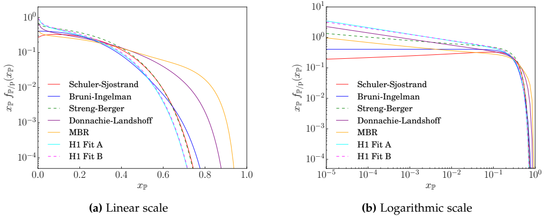
Figure 4.12: The seven different Pomeron flux parameterizations implemented in PYTHIA 8 on linear (a) and logarithmic (b) scale. Figures from [37].
