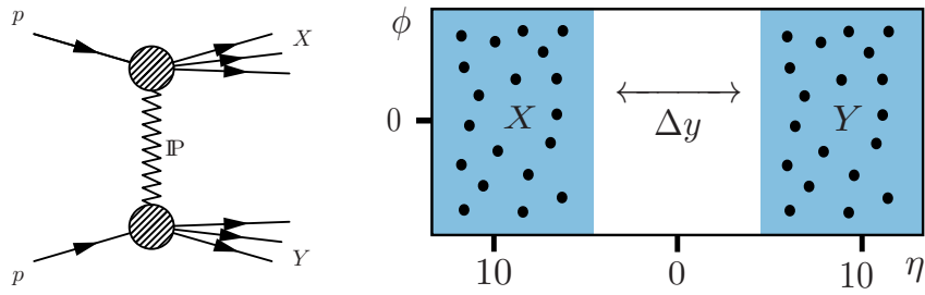
(c) Double diffraction (DD)
