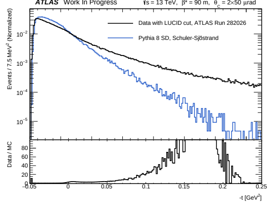
Figure 10.47: Distribution of the reconstructed t for data with the LUCID cut compared to simulated events.
