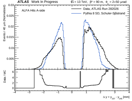
Figure 10.19: Difference in the proton hit y -coordinate between the near and far ALFA station, \Delta y = y_{237} - y_{245} , on the A-side.
