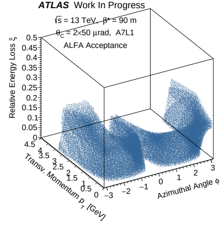
(b) ALFA acceptance.
