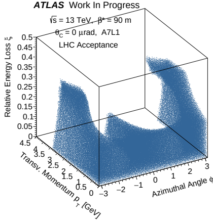
(a) LHC acceptance.
