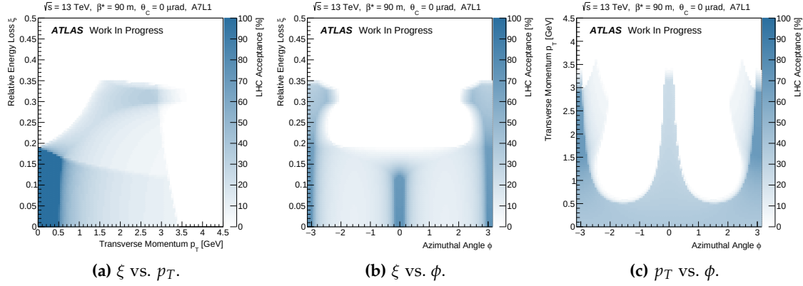
Figure 8.16: Two-dimensional projections of the LHC acceptance plots for \theta_c = 0 \mu\text{rad} .
