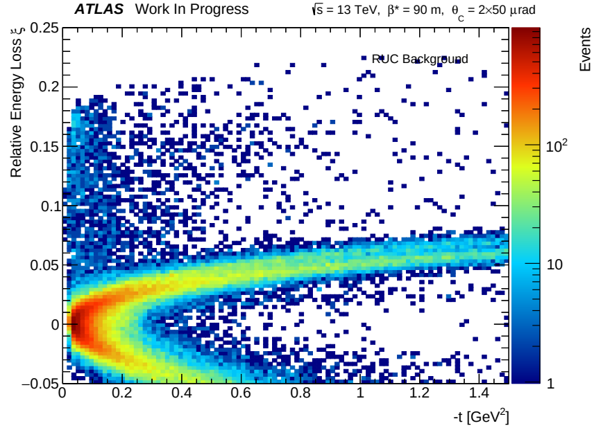
Figure 10.36: Correlation of the reconstructed \xi and t for the beam background particles in unpaired bunches.
