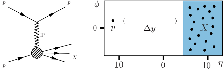
(b) Single diffraction (SD)
