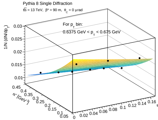
Figure 9.26: The distribution dN/dp_T as a function of the model parameters \varepsilon and \alpha' for the nine samples (markers) plotted along with the fitted expectation function (surface).
