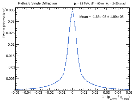
Figure 8.25: The resolution of the reconstructed p_y from ALFAReco.
