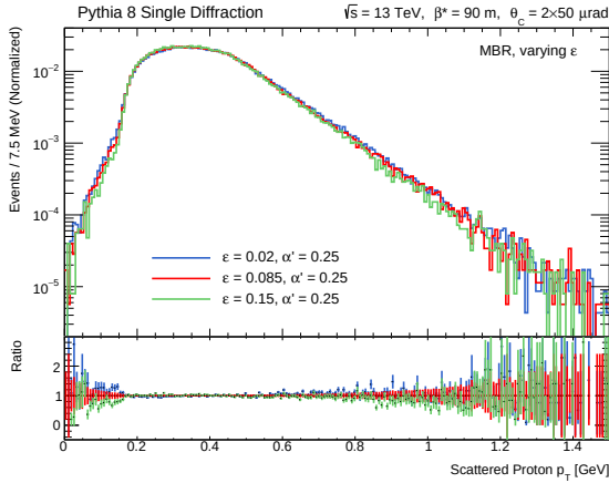
(c) MBR – varying \epsilon , keeping \alpha' constant.
