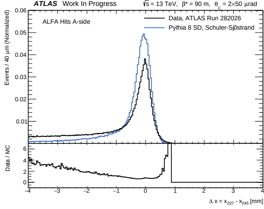
Figure 10.18: Difference in the proton hit x -coordinate between the near and far ALFA station, \Delta x = x_{237} - x_{245} , on the A-side.
