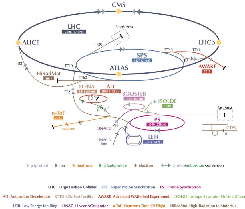
Figure 5.1: Overview of the CERN accelerator complex. Image from [OPEN-PH0-ACCEL-2016-001-2], © 2017 CERN.
