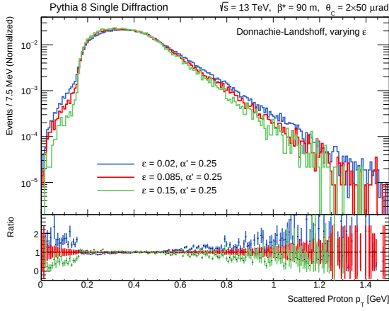
(a) DL – varying \epsilon , keeping \alpha' constant.
