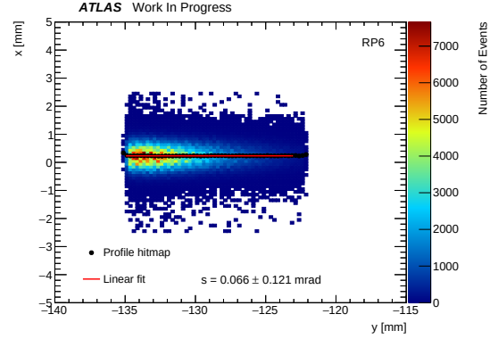
Figure 10.2: Linear fit to a profile histogram of the track pattern in the x - y -plane for RP6 (B7R1U) to determine the rotation angle around the beam axis. The track coordinates are in the detector coordinate system.
