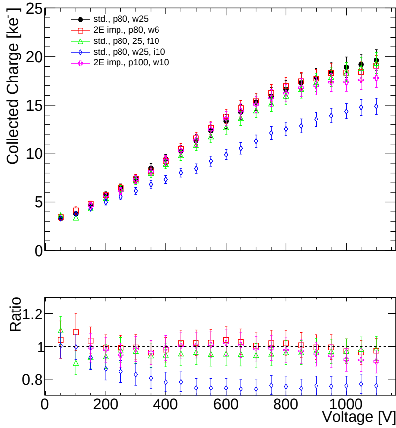
FIGURE 9.16: The collected charge (top) and the ratio compared to the standard (bottom) as a function of the bias voltage for detectors irradiated with protons to 1 \times 10^{15} \text{ n}_{eq} .
