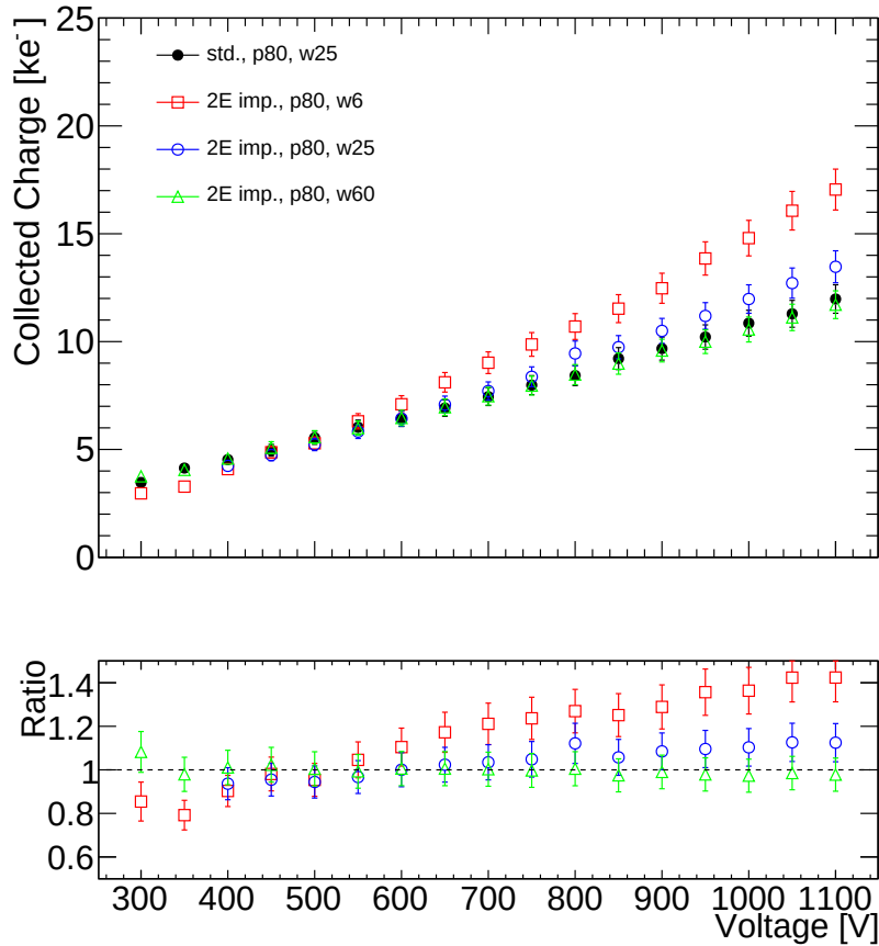
FIGURE 9.18: The collected charge (top) and the ratio compared to the standard (bottom) as a function of the bias voltage for 2E imp. sensors irradiated with neutrons to 5 \times 10^{15} \text{ n}_{eq} .
