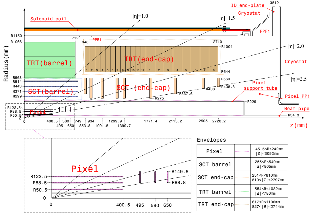
FIGURE 5.4: A schematic of a quarter-section of the ATLAS inner detector showing the arrangement of pixel layers [82].
