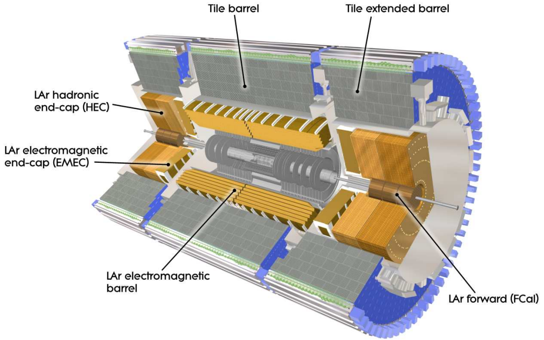
FIGURE 5.5: A cut-away of the calorimeter system within the ATLAS detector [82].
