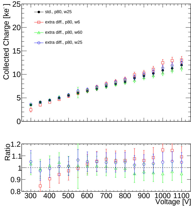
FIGURE 9.19: The collected charge (top) and the ratio compared to the standard (bottom) as a function of the bias voltage for extra diff. sensors irradiated with neutrons to 5 \times 10^{15} \text{ n}_{eq} .
