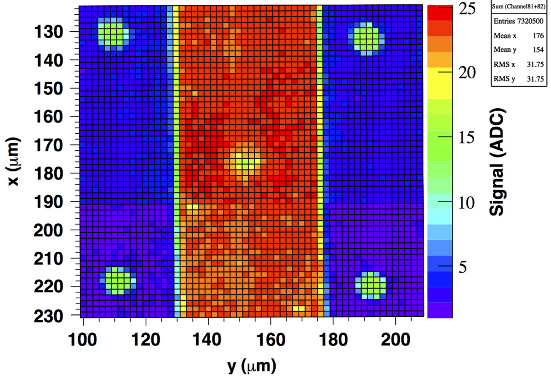
FIGURE 9.9: Laser scan performed on DC coupled strip sensor over an area of \sim 100 \times 100 \mu\text{m}^2 at a bias voltage of 30 V.
