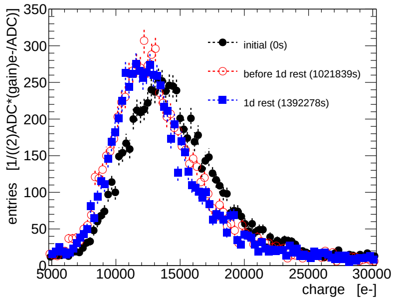
FIGURE 9.28: The signal spectra of the sensor shown in figure 9.27 before the drop (black), after the initial drop before the day of rest (red) and after the day of rest (blue).
