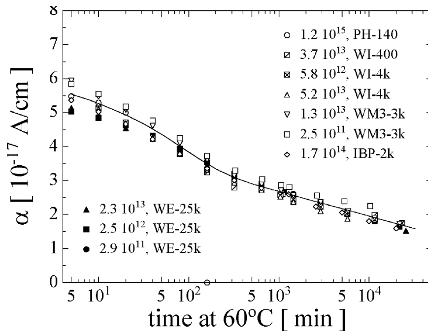
FIGURE 4.17: The damage constant \alpha as a function of time taken at 60° C. Different data points are measurements on different sensors, showing a universal dependence on annealing [67].
