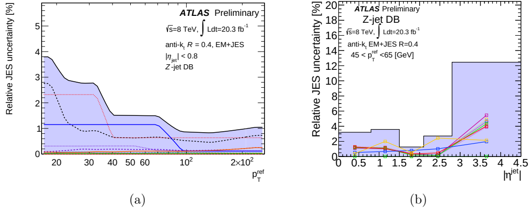
FIGURE 5.15: The relative JES uncertainty for anti- k_T jets with R = 0.4 using Z + jets events as a function of (a) jet p_T and (b) jet \eta [103].
