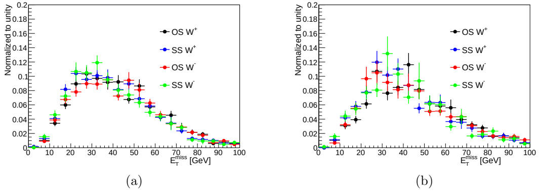
FIGURE 6.7: The W +light-jets template for the (a) 1-jet and (b) 2-jet bin
