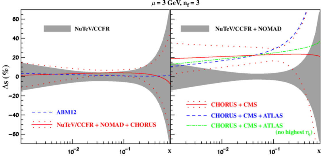
FIGURE 6.1: Relative strange quark PDF uncertainties including data from different experiments [115]. The left plot includes NuTeV/CCFR data in comparison with the one including also the NOMAD [116] and CHORUS [117] data. The right plot includes data from CMS and ATLAS
