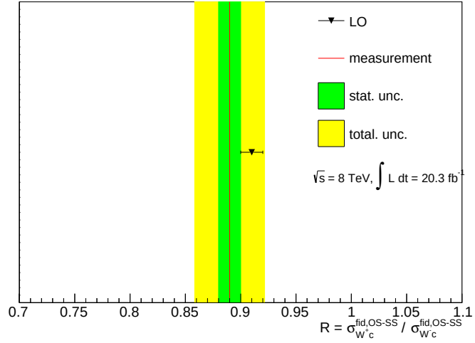
FIGURE 7.17: Measurement of the \sigma_{W^+\bar{c}}^{fid,OS-SS} / \sigma_{W^-c}^{fid,OS-SS} cross section ratio in the 1-jet inclusive sample compared to the LO ALPGEN+PYTHIA prediction.
