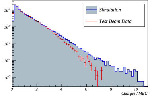
(b) Hit Charge Spectrum
