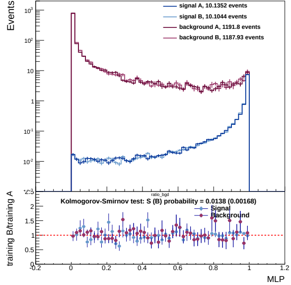
Figure 9.10: The comparison of the NN response MLP evaluated on the corresponding testing samples for the trainings A and B.
