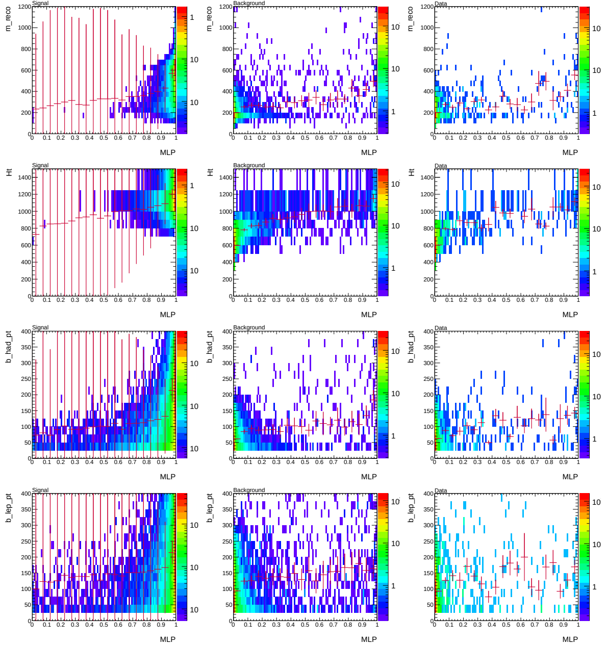
Figure C.42: Scatter plots of the M_{\text{reco}} , H_{\text{T}} , p_{\text{T}}^{\text{bhad}} and p_{\text{T}}^{\text{blep}} variables versus the NN response (MLP) arranged in this order from the top to the bottom of the figure. The plots are presented for the signal (left), the background (middle) and the data (right) samples after the W_{\text{had}} -Selection.
