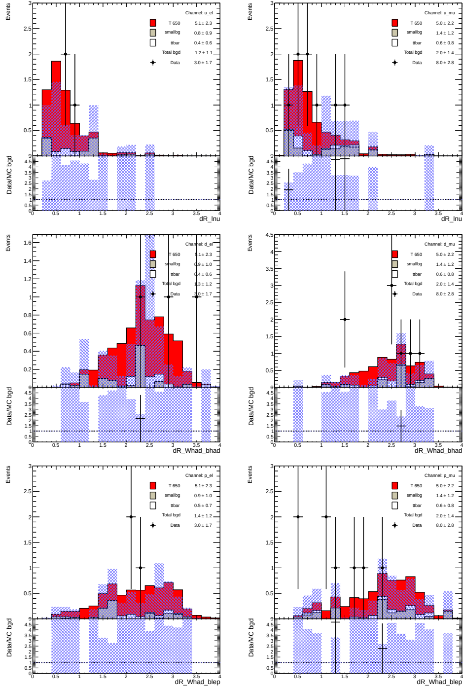
Figure C.37: Data/MC comparison of the NN input variables after the NN Selection for the e -Channel (left) and \mu -Channel (right) separately: \Delta R^{l\nu} (top), \Delta R^{W_{\text{had}}b_{\text{had}}} (middle), \Delta R^{W_{\text{had}}b_{\text{lep}}} (bottom). The blue shaded area represents the 1\sigma systematic error bands on the expected event yields.
