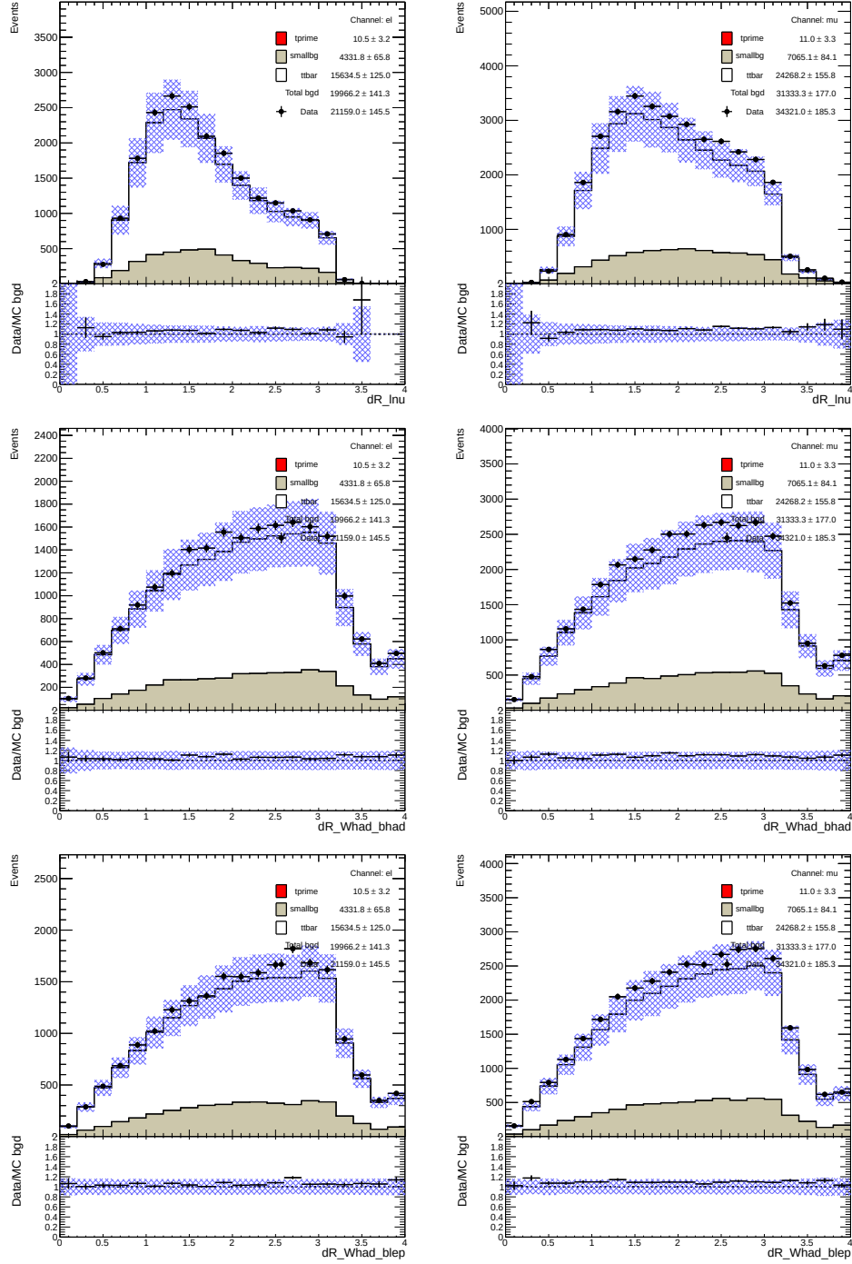
Figure C.10: Data/MC comparison of the NN input variables in the Control Region Pre-selection, \geq 4 jets, \geq 1 b -tags, M_{\text{reco}} < 350 GeV for the e -Channel (left) and \mu -Channel (right) separately: \Delta R^{l\nu} (top), \Delta R^{W_{\text{had}}b_{\text{had}}} (middle), \Delta R^{W_{\text{had}}b_{\text{lep}}} (bottom). The blue shaded area represents the 1\sigma systematic error bands on the expected event yields.
