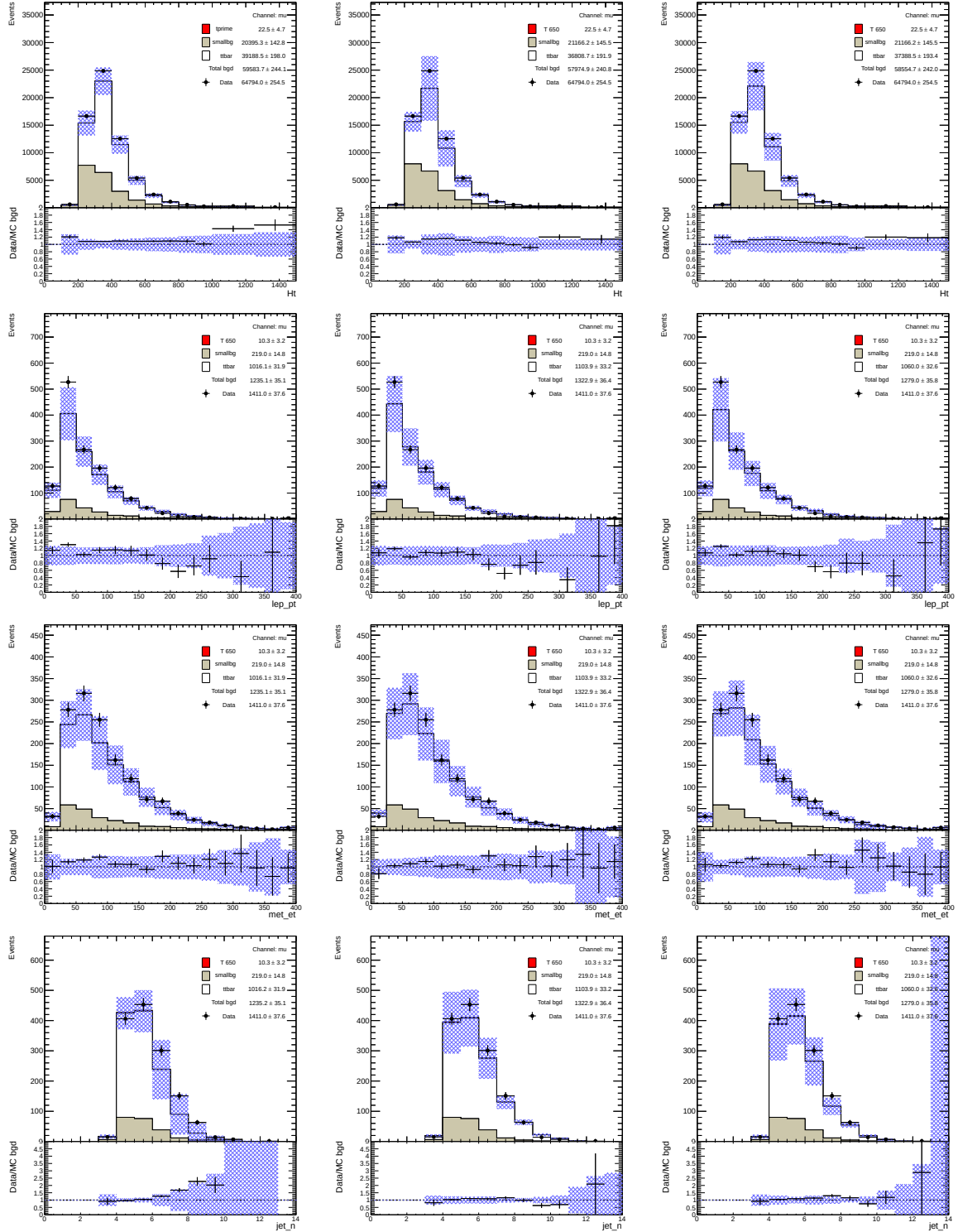
Figure C.40: Data/MC comparison of the H_T variable, p_T of the lepton, missing transverse energy and jet multiplicity after the W_{had} -selection for three samples generated using different generators: MC@NLO (left column), Powheg-Pythia (middle column), Powheg-Jimmy (right column). The blue shaded area represents the 1\sigma systematic error bands on the expected event yields.
