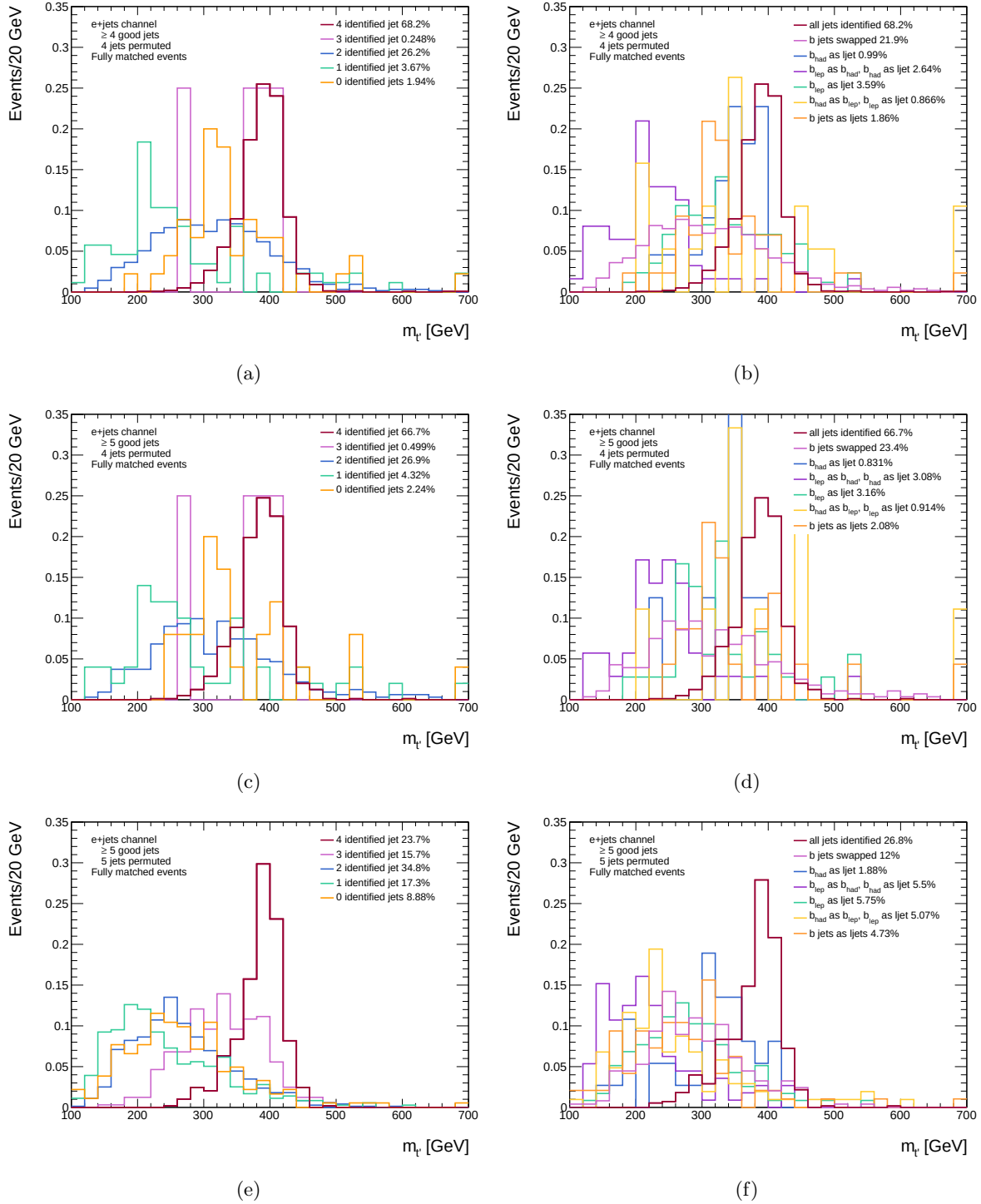
Figure 8.5: Shapes of the various components of the fitted t' mass distribution of the fully matched events decomposed according to: the number of identified jets ((a), (c), and (e)) and nature of the mis-identification ((b), (d), and (f)). All histograms are normalised to unity. The distributions are shown for the samples with \geq 4 ((a), (b)) and \geq 5 ((c) – (f)) reconstructed jets in the event in the e+\text{jets} channel. The distributions have been produced by fitting four ((a) – (d)) or five ((e), (f)) leading jets in the nominal t' sample with m_{t'} = 400 GeV.
