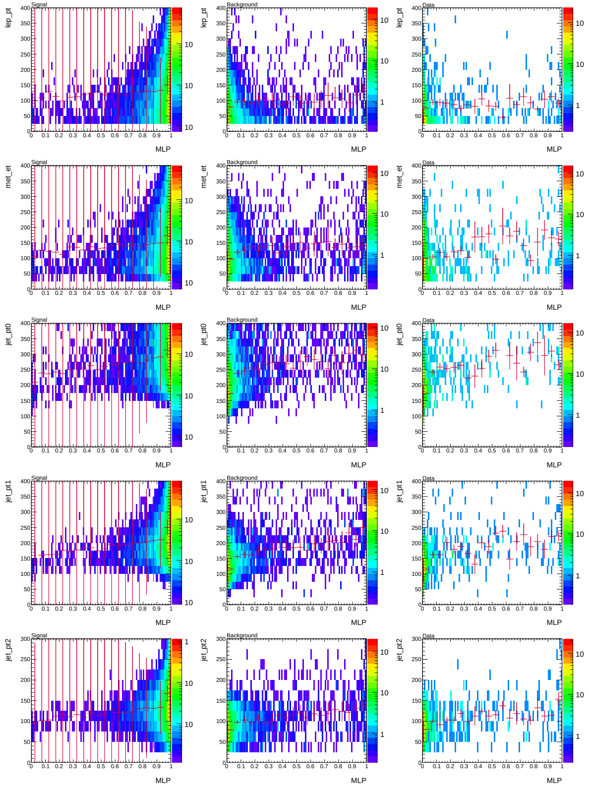
Figure C.44: Scatter plots of the p_T of the lepton, E_T^{\text{miss}} , as well as the p_T of three hardest jets versus the NN response (MLP) arranged in this order from the top to the bottom of the figure. The plots are presented for the signal (left), the background (middle) and the data (right) samples after the W_{\text{had}} -Selection.
