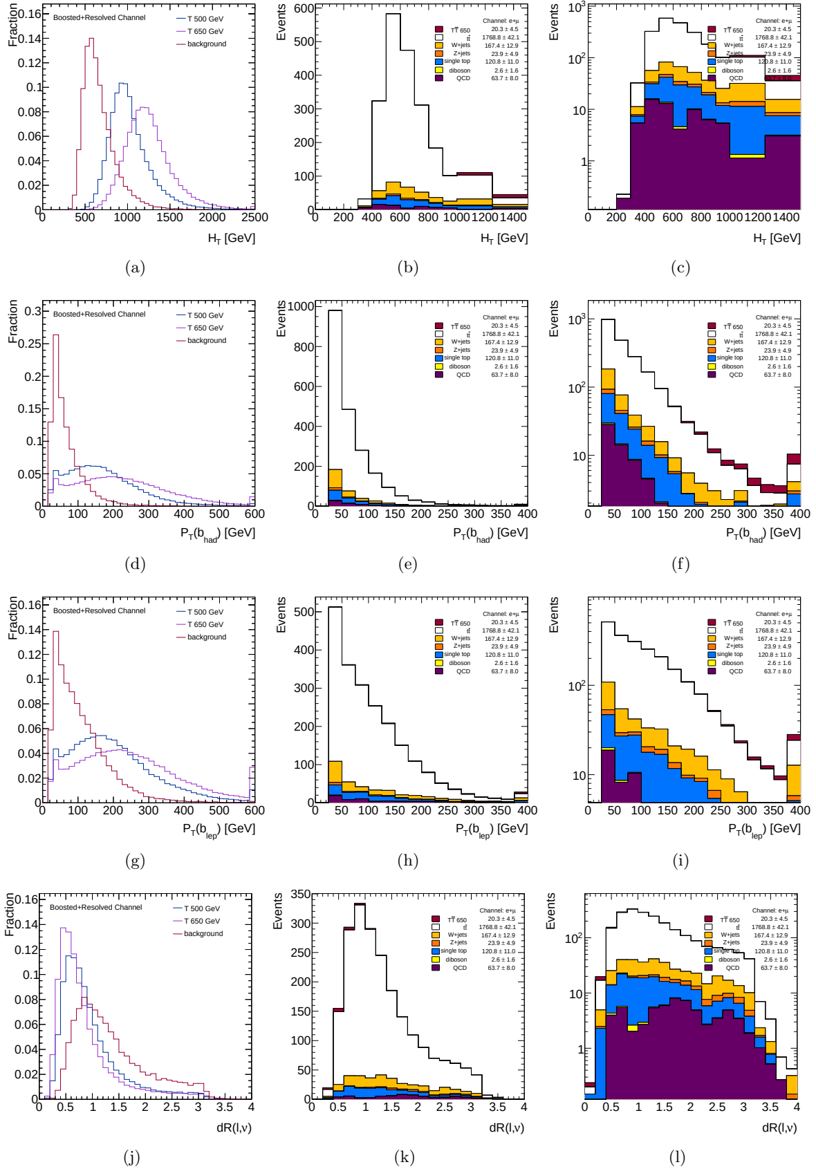
Figure 9.3: Discriminating variables for the signal events passing the W_{had} -selection with T mass of 500 GeV and 650 GeV and the combined MC background. The figures contain events passing either the BOOSTED or the RESOLVED selection. Distributions normalised to unity ((a), (d), (g) and (j)), and the absolute expected distributions normalised to an integrated luminosity of 4.7 \text{ fb}^{-1} assuming the production cross-section in linear ((b), (e), (h), and (k)) and logarithmic ((c), (f), (i), and (l)) scales.
