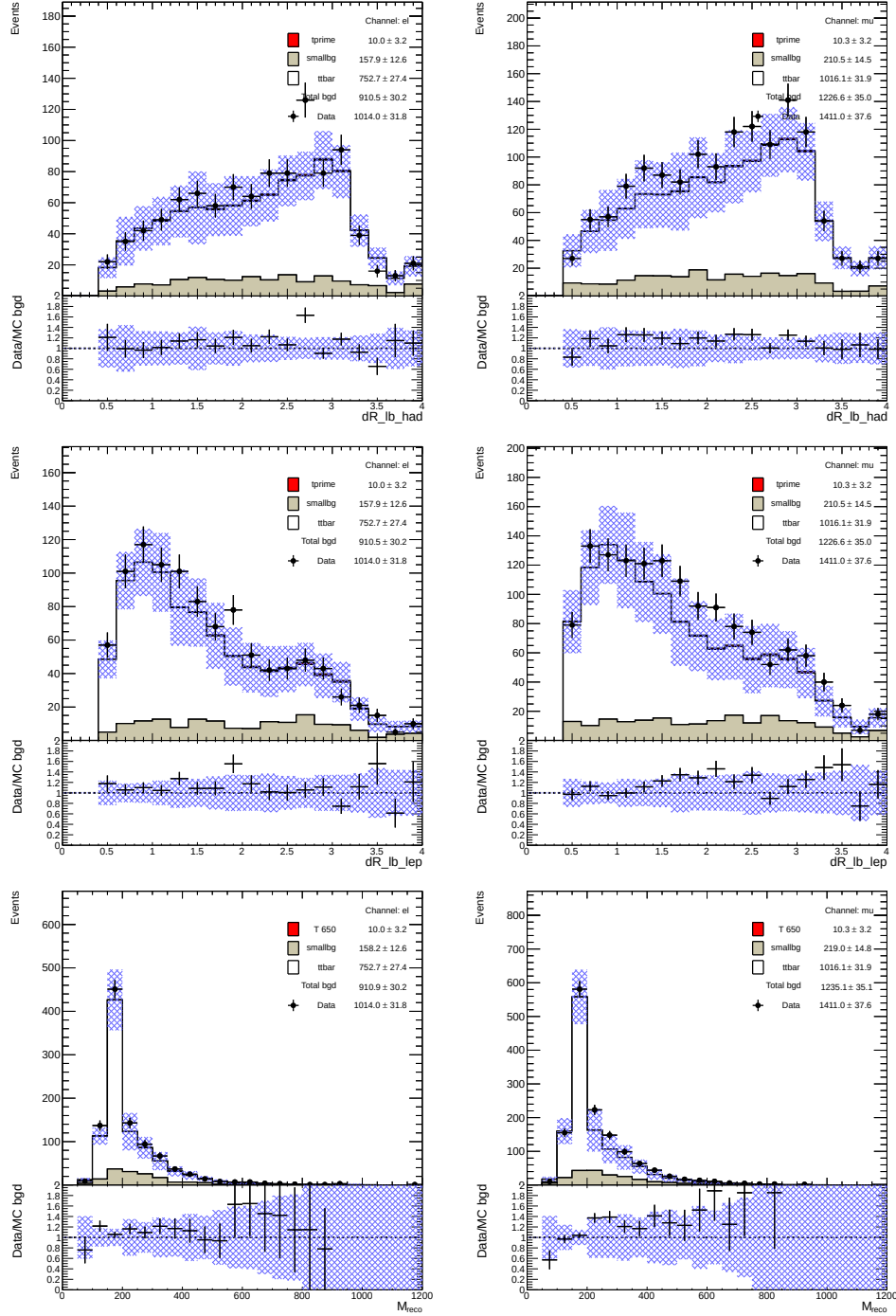
Figure C.32: Data/MC comparison of the NN input variables after W_{\text{had}} -Selection for the e -Channel (left) and \mu -Channel (right) separately: \Delta R^{l_{\text{had}}} (top), \Delta R^{l_{\text{lep}}} (middle), M_{\text{reco}} (bottom). The blue shaded area represents the 1\sigma systematic error bands on the expected event yields.
