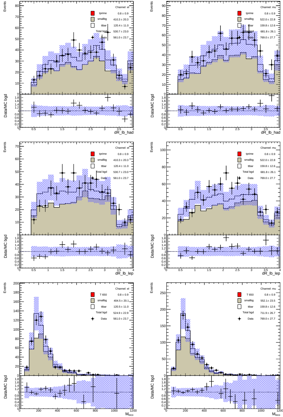
Figure C.20: Data/MC comparison of the NN input variables in the Control Region W_{had} -Selection, = 0 b -tags for the e -Channel (left) and \mu -Channel (right) separately: \Delta R^{lb}_{had} (top), \Delta R^{lb}_{lep} (middle), M_{reco} (bottom). The blue shaded area represents the 1\sigma systematic error bands on the expected event yields.
