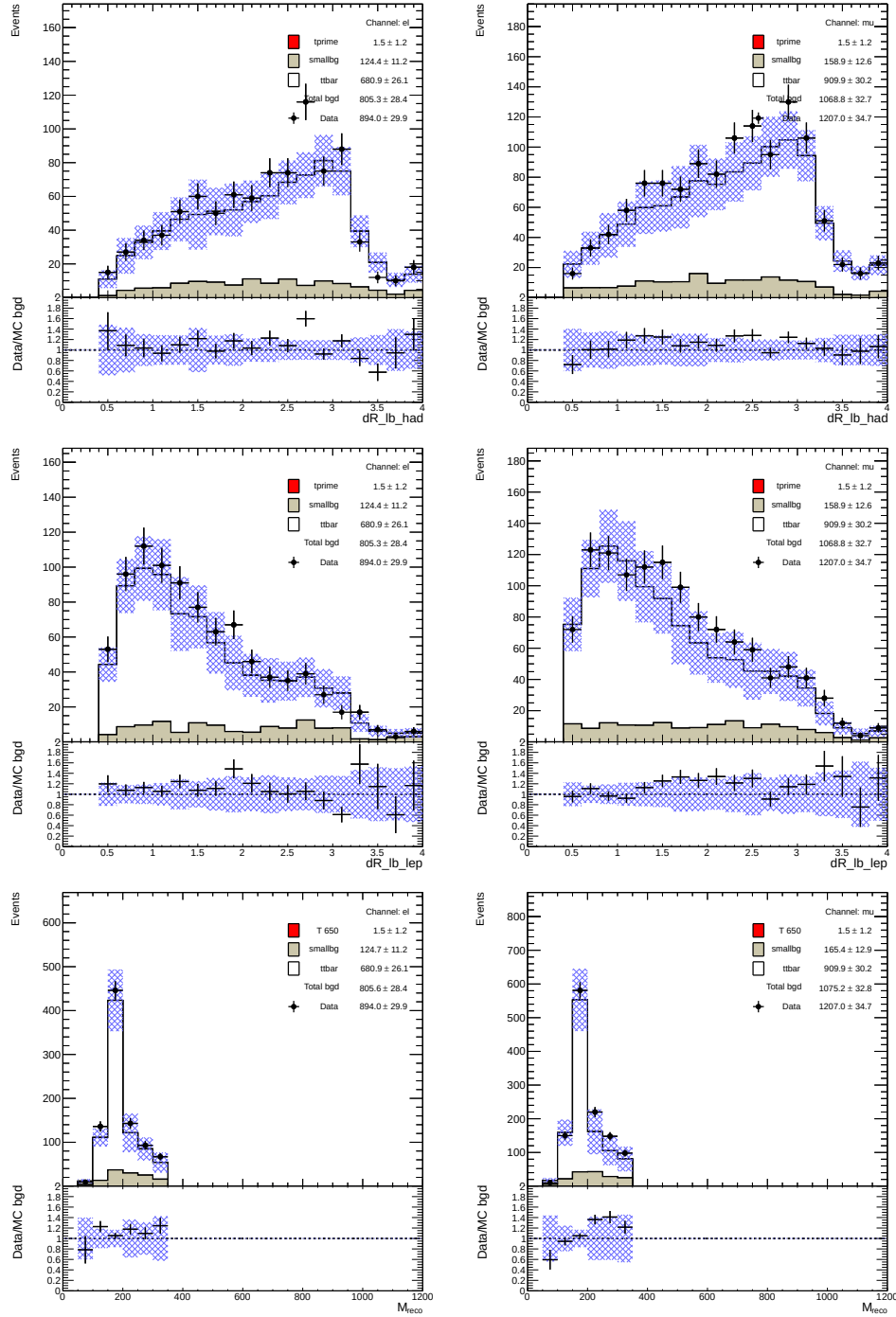
Figure C.23: Data/MC comparison of the NN input variables in the Control Region W_{\text{had}} -Selection, \geq 4 jets, \geq 1 b -tags, M_{\text{reco}} < 350 GeV for the e -Channel (left) and \mu -Channel (right) separately: \Delta R^{lb}_{\text{had}} (top), \Delta R^{lb}_{\text{lep}} (middle), M_{\text{reco}} (bottom). The blue shaded area represents the 1\sigma systematic error bands on the expected event yields.
