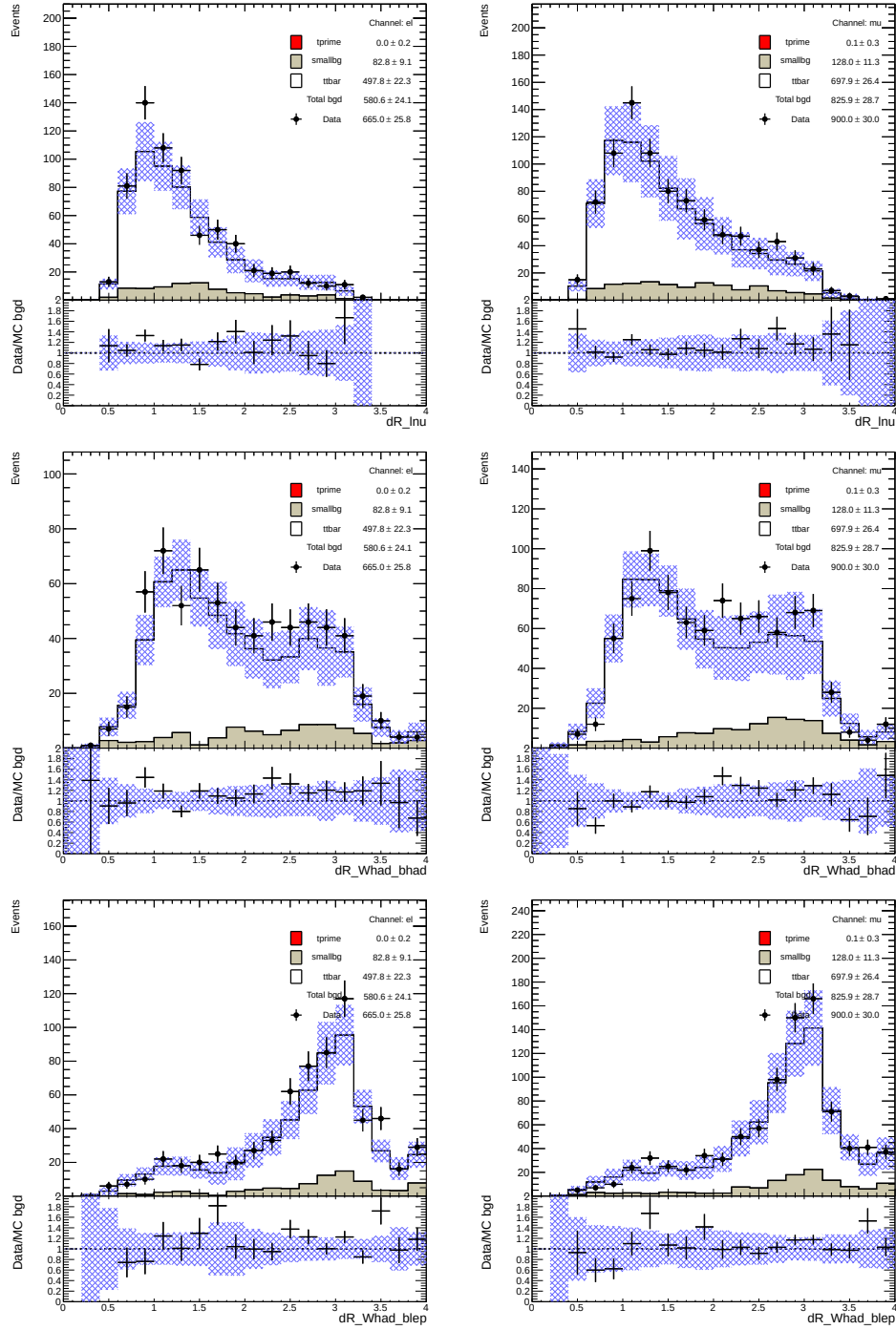
Figure C.25: Data/MC comparison of the NN input variables in the Control Region W_{had} -Selection, \geq 4 jets, \geq 1 b -tags, H_T < 700 GeV for the e -Channel (left) and \mu -Channel (right) separately: \Delta R^{l\nu} (top), \Delta R^{W_{had}b_{had}} (middle), \Delta R^{W_{had}b_{lep}} (bottom). The blue shaded area represents the 1\sigma systematic error bands on the expected event yields.
