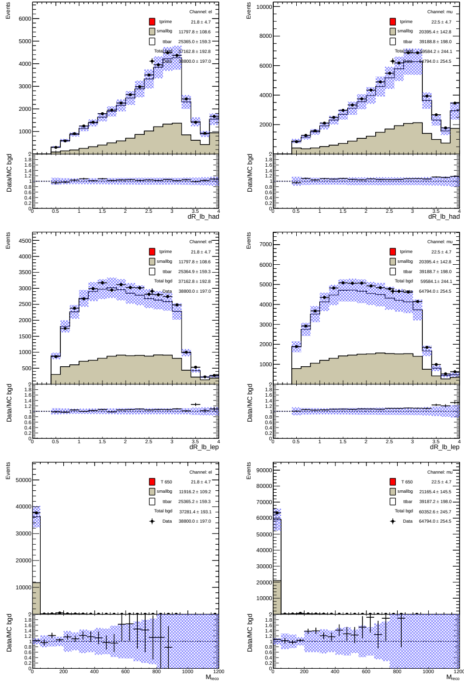
Figure C.17: Data/MC comparison of the NN input variables after Pre-selection for the e -Channel (left) and \mu -Channel (right) separately: \Delta R^{lb_{had}} (top), \Delta R^{lb_{lep}} (middle), M_{reco} (bottom). The blue shaded area represents the 1\sigma systematic error bands on the expected event yields.
