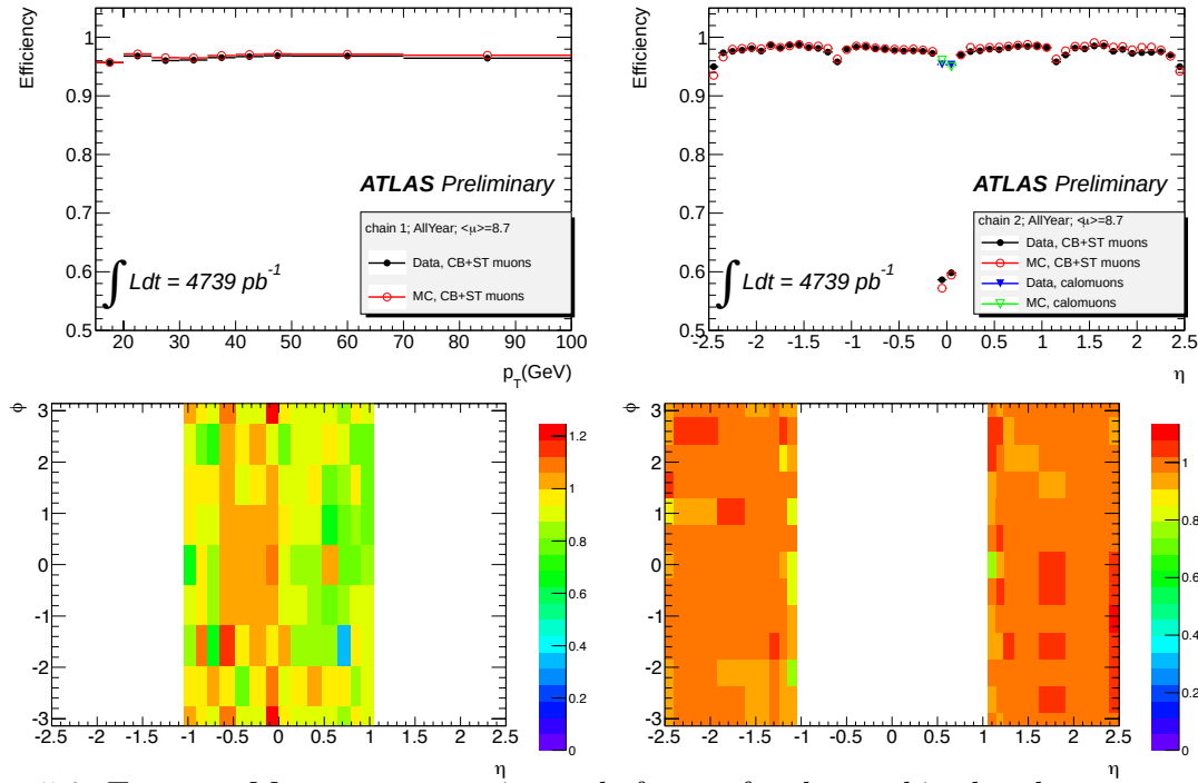
Figure 5.6: Top row: Muon reconstruction scale factors for the combined and segment tagged muons for the produced from the Z \rightarrow \mu\mu events collected in the period B-M of the 2011 data taking campaign [155]. Bottom row: Muon trigger scale factors for the barrel (left) and the endcaps (right) regions corresponding to the mu18 trigger derived from the Z data samples using the T&P method. The SFs plotted in bins of \eta and \phi are shown for L-M (bottom) [142].
