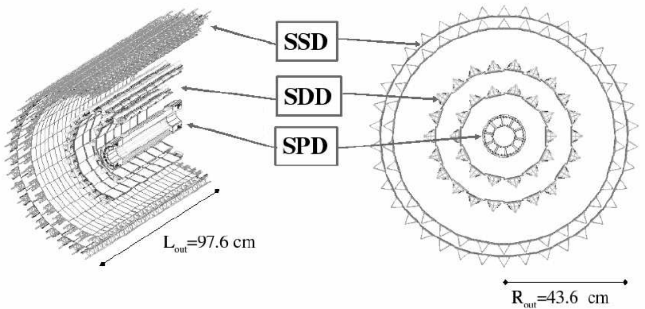
Figure 3-3: (Color online) Inner Tracking System (ITS) :The two innermost layers of Silicon Pixel Detector (SPD), the two intermediate layers of Silicon Drift Detector (SDD), and two outermost layers of Silicon Strip Detector (SSD) [5].
