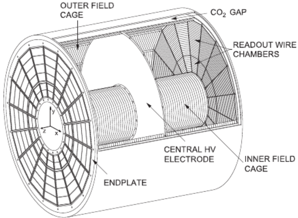
Figure 3-4: (Color online) A 3D view of the TPC. At the centre of the TPC drift volume, there is the high voltage electrode. There are total 18 sectors and 36 readouts at endplates on each end [11].
