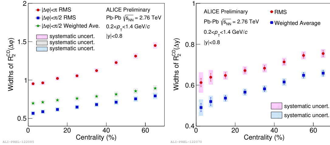
Figure 4-9: (Color online) [ALICE preliminary] The Centrality dependence of width in \Delta\varphi (left plot) and \Delta y (right plot) for Pb+Pb collisions at \sqrt{s_{NN}} = 2.76 TeV. The transverse momentum used in this plot is within the range 0.2 < p_T < 1.4 GeV/c. 0-5% centrality is taken as most central collision and 60-70% centrality is taken as most peripheral collision.
