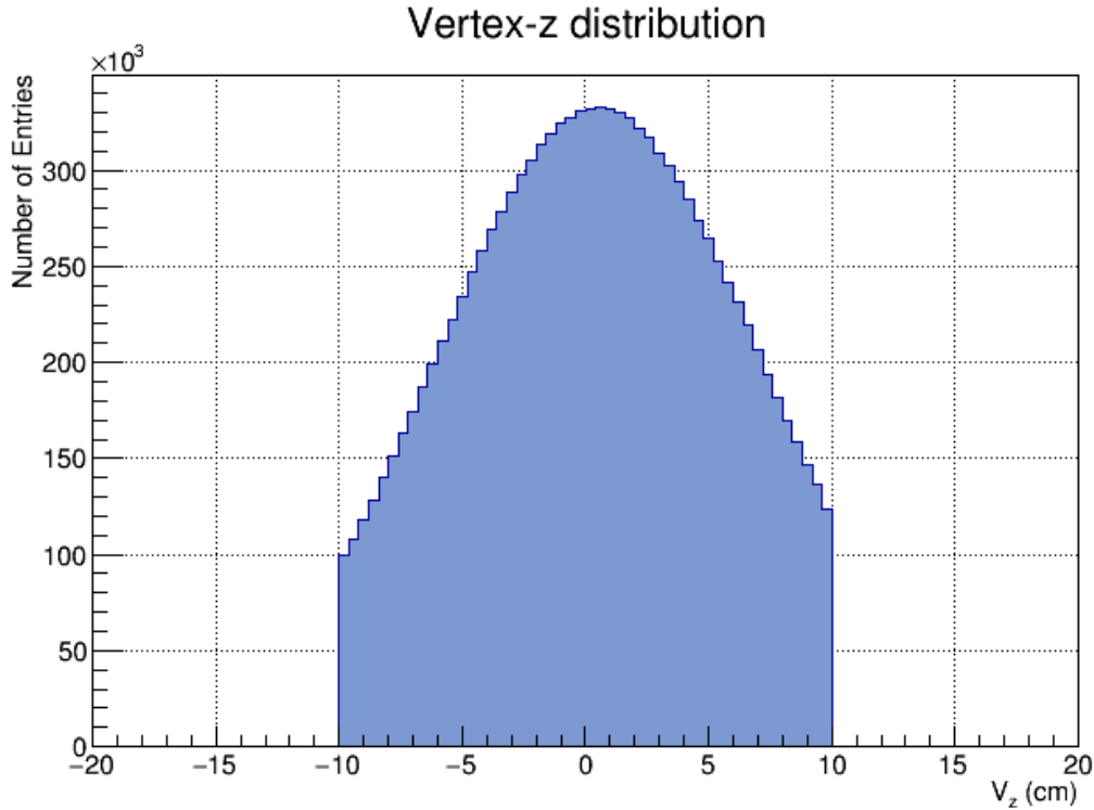
Figure 4-1: (Color online) Vertex-z distribution of Pb+Pb collisions at \sqrt{s_{NN}} = 2.76 TeV.
