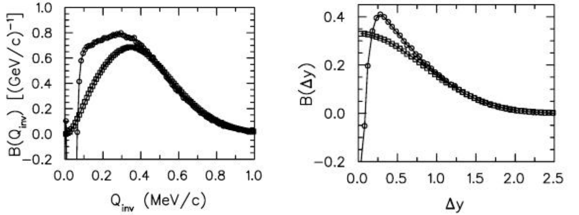
Figure 2-4: (Color online) Pion balance function with (circles) and without (squares) distortion (it is coming from interpair interaction) from blast-wave model are shown in left plot. Blast-wave model has a breakup temperature 120 MeV, a maximum transverse velocity of 0.7c and spread \sigma_\eta = 0 . The balance function without distortion was scaled by 70% to account for balancing pairs by other species. These balance functions are filtered by STAR acceptance. Balance function as a function of relative rapidity ( \Delta y ) with and without distortion are shown in right plot. There is a less distortion effect in \Delta y . [10]
