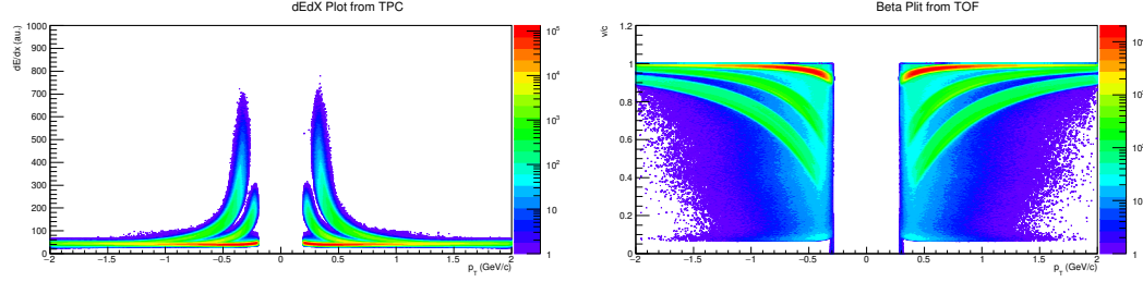
Figure 4-3: (Color online) dE/dx (left) and Beta (right) plot from TPC and TOF detector respectively for pion, kaon and proton at Pb+Pb collisions with \sqrt{s_{NN}} = 2.76 TeV.
