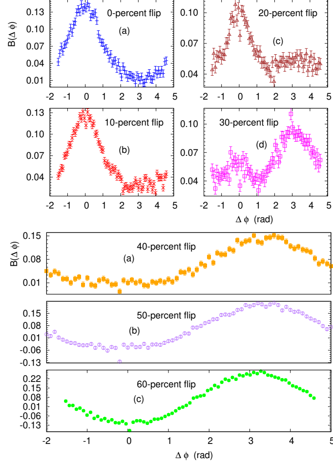
Figure 5-4: (Color online) BF for Au+Au minimum bias at \sqrt{s_{NN}} = 200 GeV with different flipping fractions from 0 to 60 %
