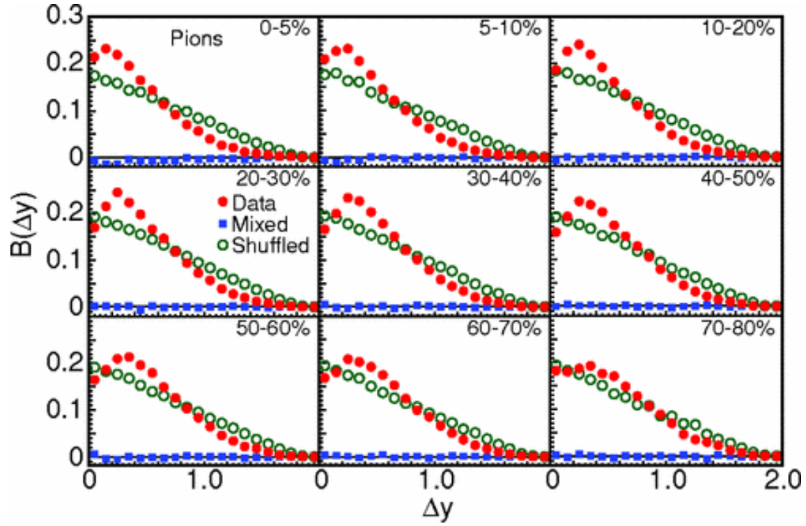
Figure 2-10: (Color online) The balance function distribution as a function of \Delta y for identified charged pions produced in Au+Au collisions at \sqrt{s_{NN}} = 200 GeV. Pion balance function get narrower in central collisions with respect to peripheral collisions [21].
