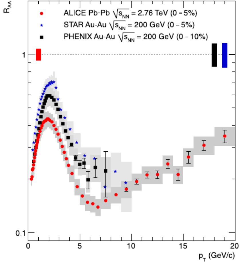
Figure 1-11: (Color online) Comparison of nuclear modification factor in central Pb+Pb collisions at LHC to measurements at STAR and PHENIX at \sqrt{s_{NN}} = 200 GeV. The statistical and systematic errors are shown by error bars and boxes respectively. The vertical bars around R_{AA} = 1 represents p_T independent scaling errors on R_{AA} [60].
