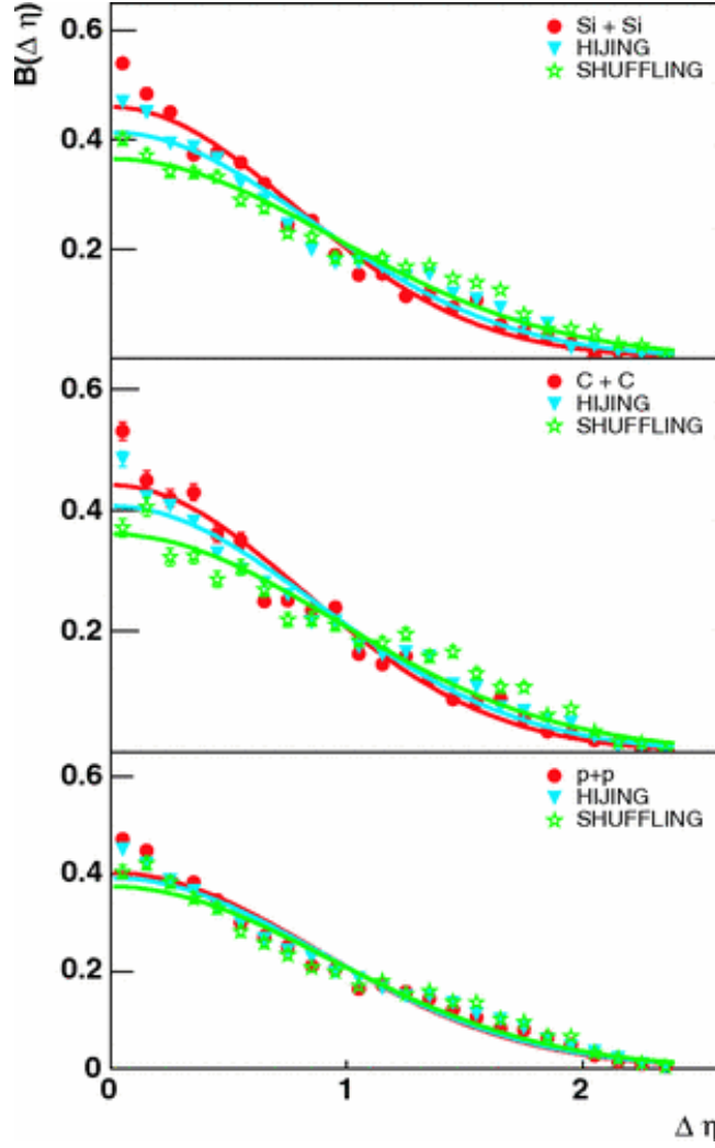
Figure 2-8: (Color online) Balance function distribution as a function of \Delta\eta for Si+Si, C+C and p+p collisions with real, shuffled and HIJING events are shown. The BF from HIJING event generator is independent of centrality and system size of nuclei. The distribution is wider than BF from real data. It is also observed that BF distribution is more narrower for Si+Si collisions than C+C and pp collisions [20].
