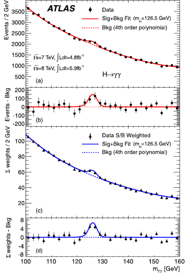
Figure 1-1: (Color online) Distribution of invariant mass spectrum of diphoton from pp collisions at \sqrt{s} = 7 TeV and 8 TeV respectively. Background of diphoton reconstruction is eliminated from signal by fitting fourth-order Bernstein polynomial. Here H \rightarrow \gamma\gamma decay channel is considered. It is observed from lower panel that Higgs boson has mass around 126.5 GeV [3].
