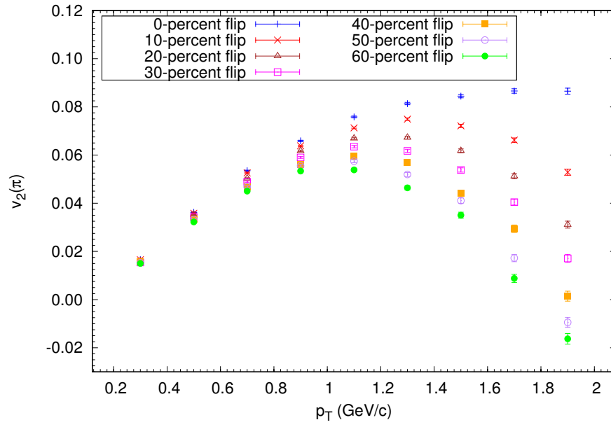
Figure 0-7: Elliptic flow of pions for different flipping fractions and no flip
