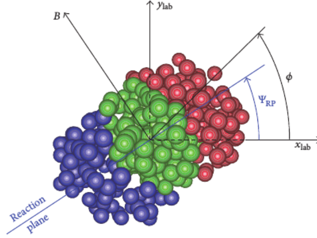
Figure 1-7: (Color online) A picture of transverse plane for a collision . (the left one emerging from and the right one going into the page) [37].
