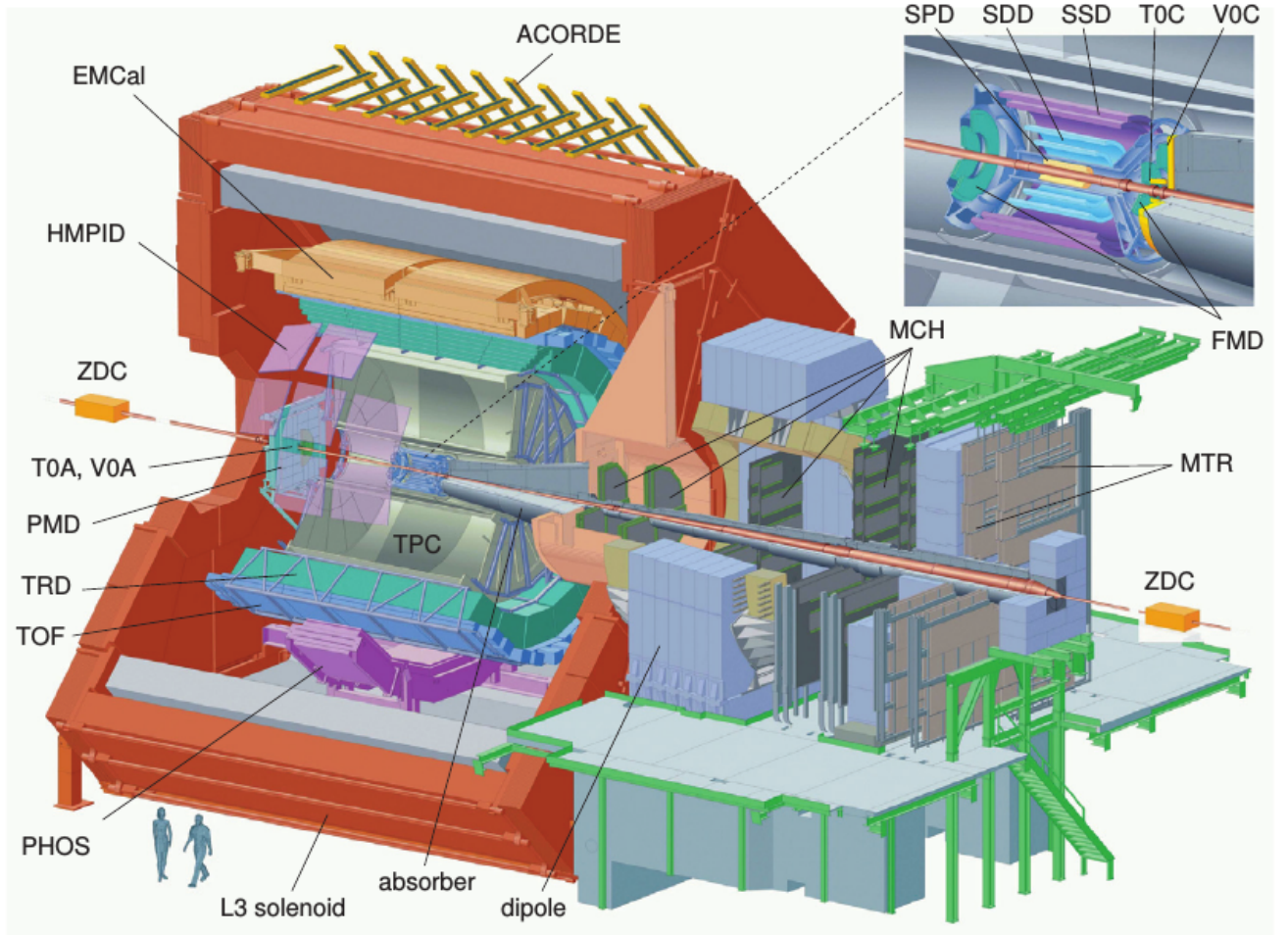
Figure 3-2: (Color online) layout of the ALICE experiment [8].
