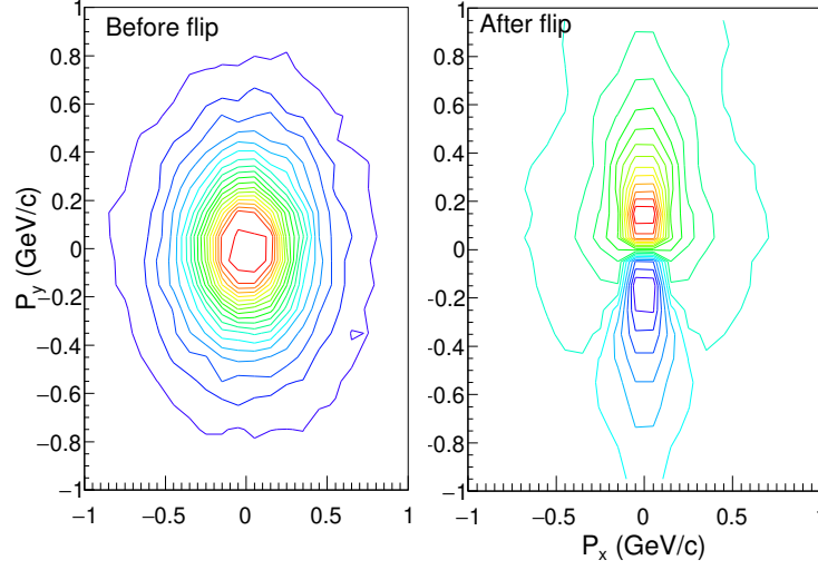
Figure 5-3: (Color online) Net electric charge distributions on the transverse plane before and after flipping with a 20% flipping fraction.
