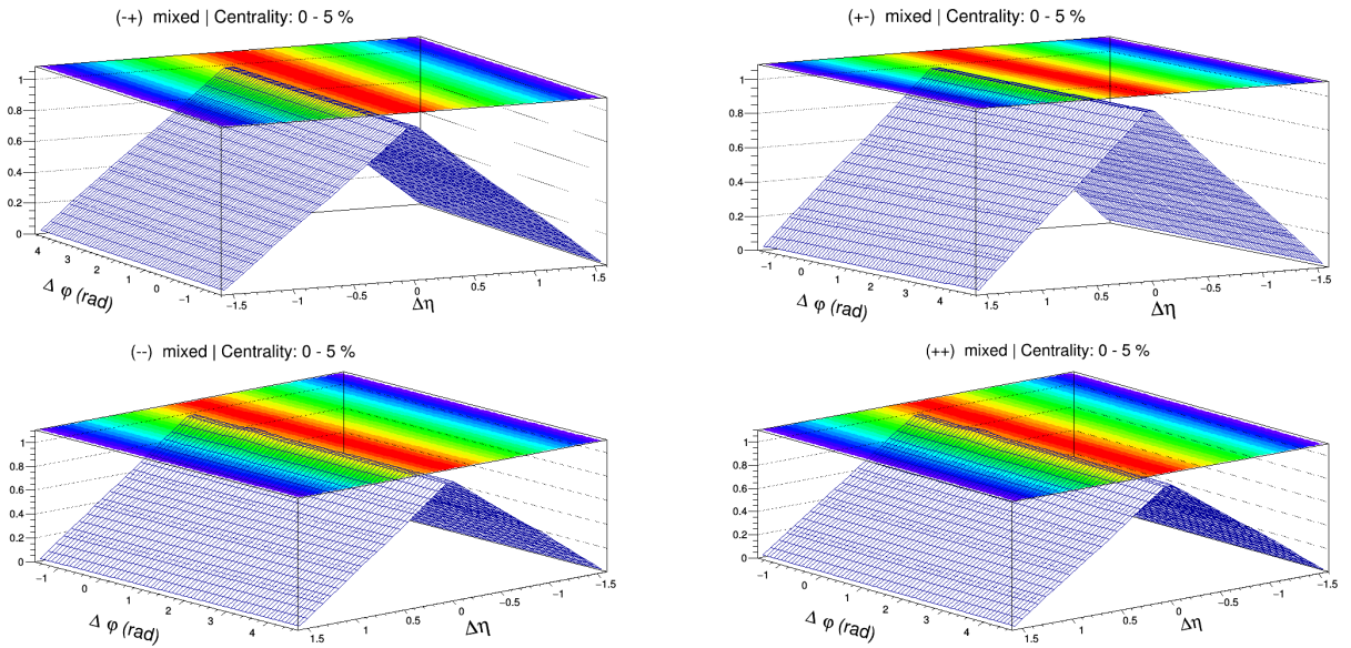
Figure 4-6: (Color online) Two particle correlation for unlike sign (upper) and like sign pairs (lower) in \Delta\eta - \Delta\varphi space using particles from mixed events for 0-5%
