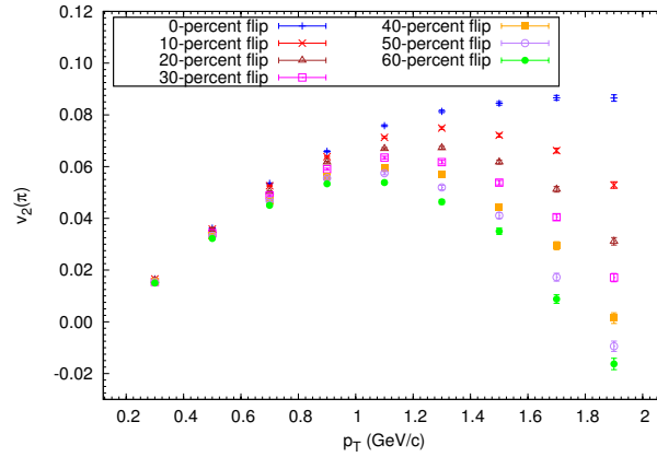
Figure 5-7: (Color online) Elliptic flow of pions for different flipping fractions and no flip
