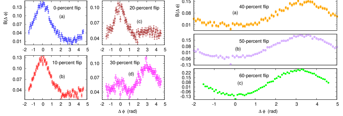
Figure 0-6: BF for Au+Au minimum bias at \sqrt{s_{NN}} = 200 GeV with different flipping fractions from 0 to 60 %
