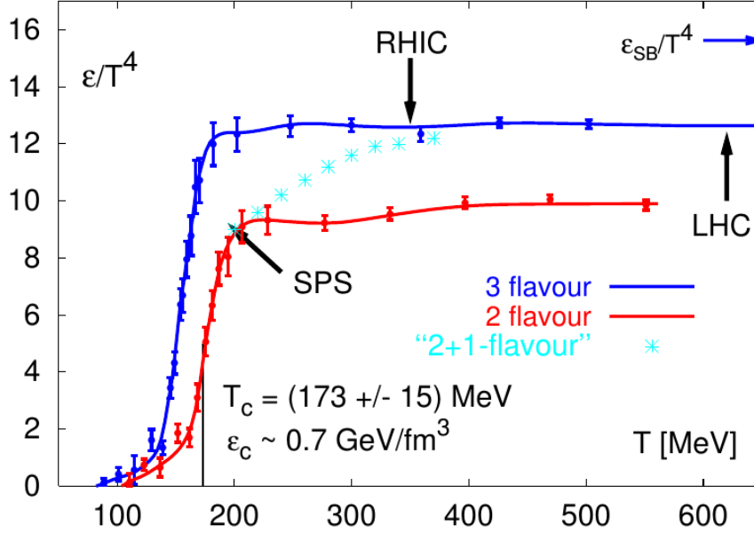
Figure 1-3: (Color online) The energy density of QCD as a function of temperature. The lattice calculations are performed for two massless quarks, three massless quarks and two massless quark plus one with its actual real mass. It is observed that there is a transition at temperature at 173 MeV and at energy density 0.7 GeV/fm 3 [25].
