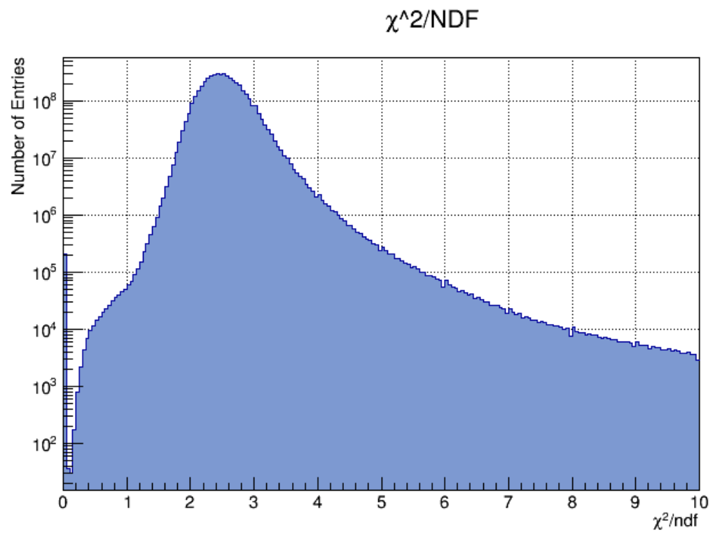
Figure 4-2: (Color online) Distribution of \chi^2/\text{NDF} for TPC cluster.
