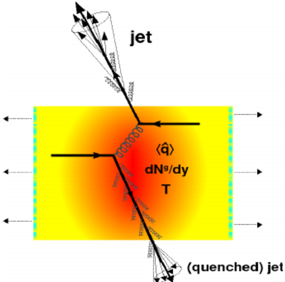
Figure 1-10: (Color online) A hard scattering between two quarks. One quark goes out to vacuum by radiating a few gluons and finally hadronise. Other quark goes through the dense QGP medium. This quark loses energy due to medium-induced gluonstrahlung and finally it fragments into a quenched jet [52].
