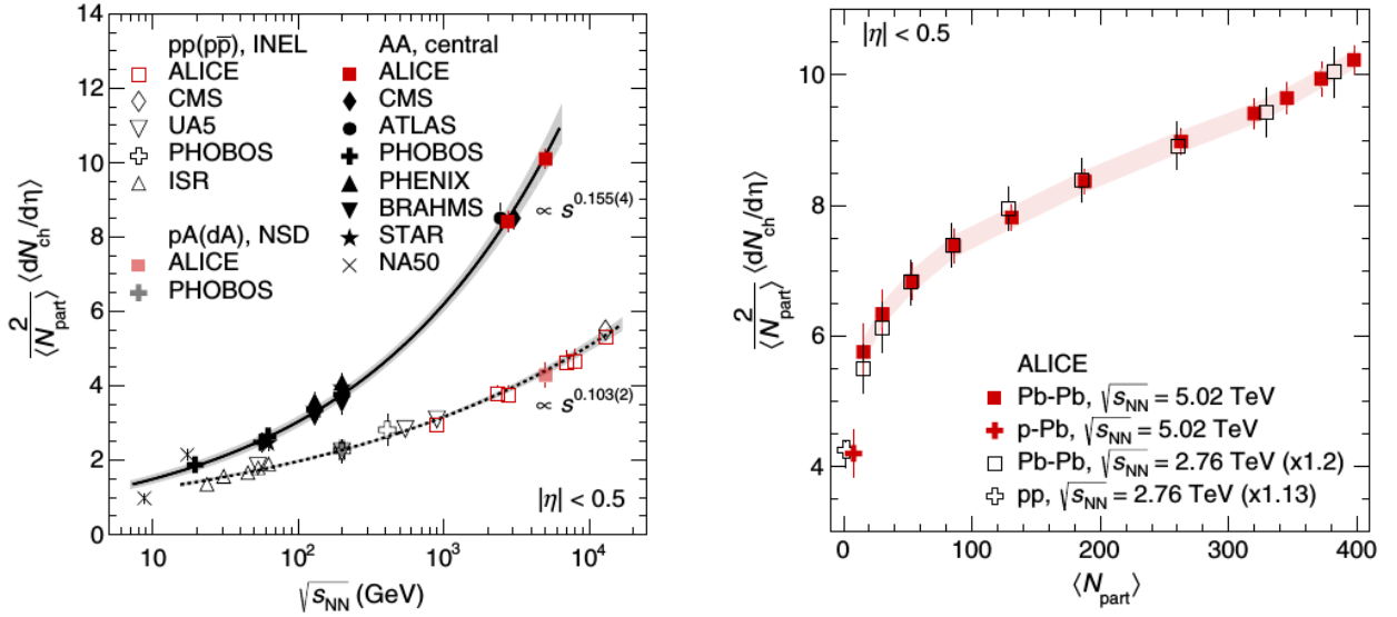
Figure 1-6: (Color online) Values of (\frac{2}{\langle N_{part} \rangle} \langle dN_{ch}/d\eta \rangle) as a function of \sqrt{s_{NN}} (left panel) and \langle N_{part} \rangle (right panel) for pp, Pb+Pb and Au+Au collisions are shown [31].
