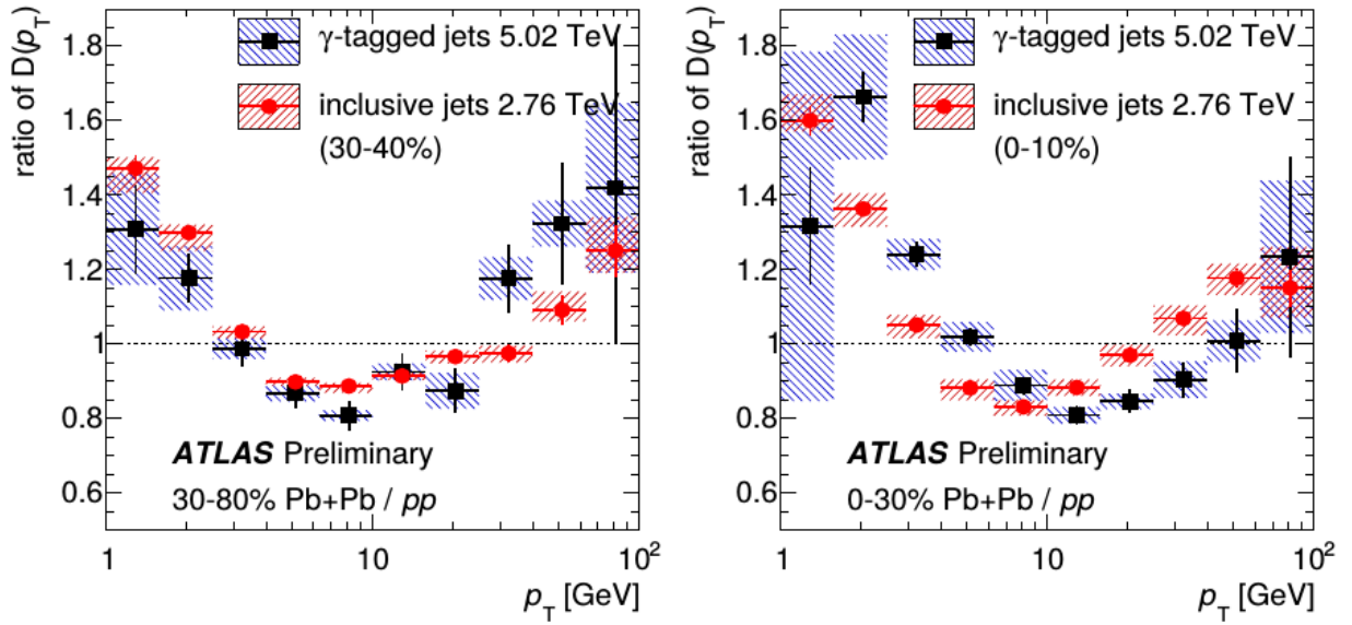
Figure 1-12: (Color online) Ratio of fragmentation function for jets which are azimuthally balanced with high- p_T photon for two centrality 30-80% (left plot) and 0-30% (right plot). Black points are for results with photon-tagged jets and red points show results for inclusive jets [61].
