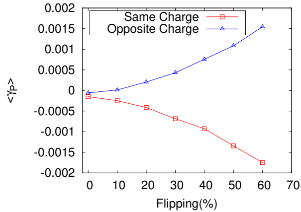
Figure 5-6: (Color online) \langle \gamma_P \rangle with different flipping fractions
