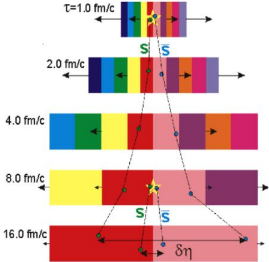
Figure 2-1: (Color online) Balancing partners produced at 1 fm/c and 8 fm/c respectively. Separation is larger in early produced pair than late produced pair [2].
