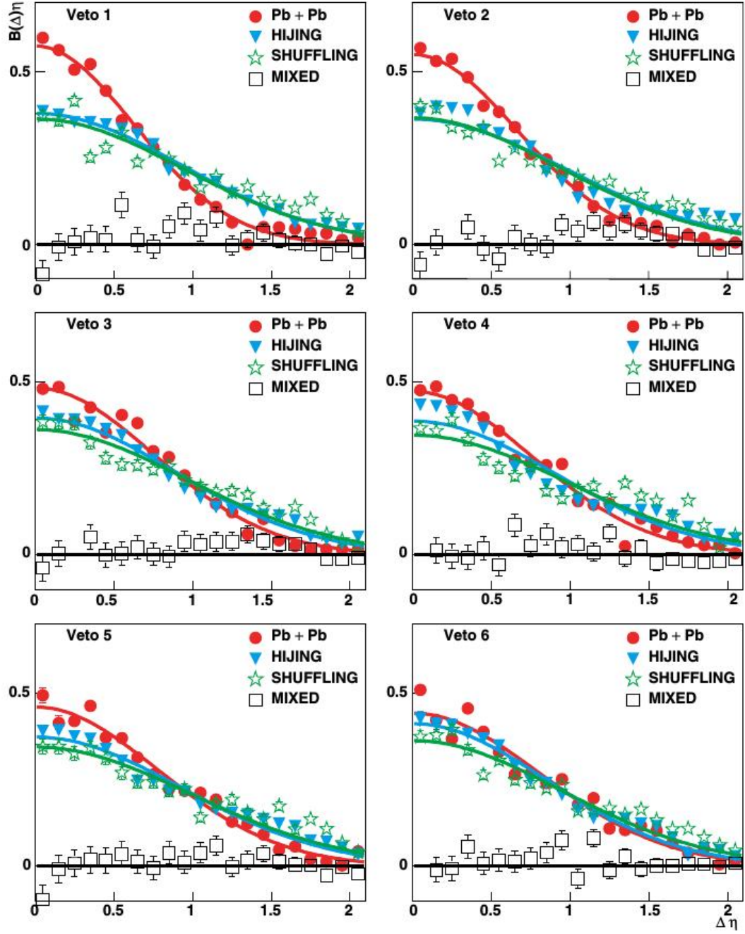
Figure 2-9: (Color online) The balance function distribution of Pb+Pb collisions with different centrality are shown. Real data points are shown with darkened circle and marker [20].
