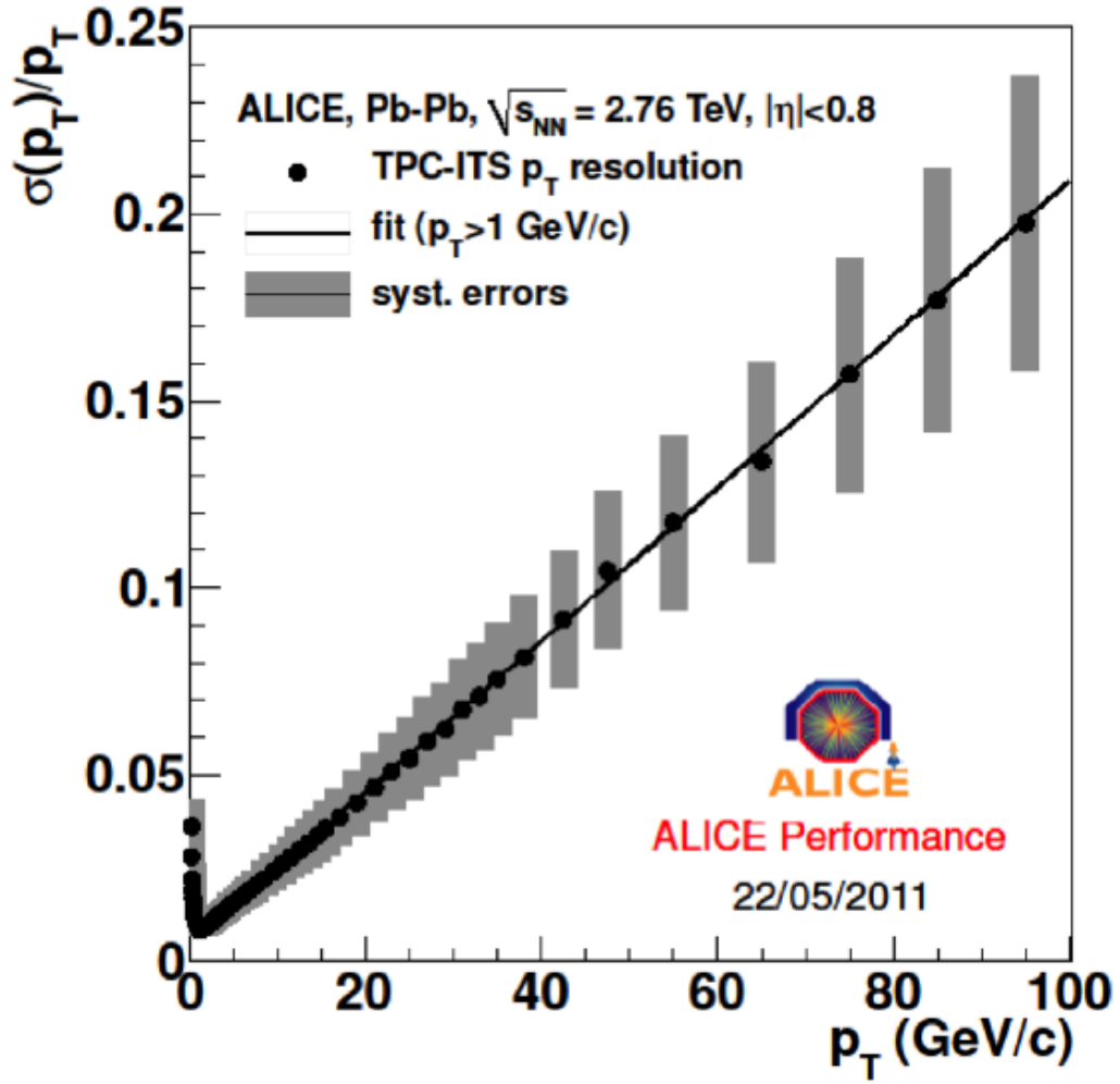
Figure 3-5: (Color online) ITS-TPC p_T resolution in Pb+Pb collisions at \sqrt{s_{NN}} = 2.76 TeV [8].
