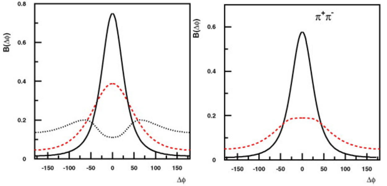
Figure 2-3: (Color online) Left plot: Pion's balance function for two different freeze-out conditions: T_f = 165 MeV , average transverse velocity \langle\beta\rangle = 0.5 and T_f = 90 MeV , \langle\beta\rangle = 0.6 . Dashed line is for nonresonant pions and dotted line is for pions from decay of \rho_0 resonance at T_f=165 MeV and \langle\beta\rangle = 0.5 . Solid line is for nonresonant pions at T_f = 90 MeV and \langle\beta\rangle = 0.6 . Right plot: The correlation between the pions is given by a weighed [6] sum of the two mechanisms i.e non-resonant pions and decay products of resonances for T_f = 165 MeV (dashed line) and by nonresonant pion pairs for the freeze-out at 90 MeV (solid line) [7].
