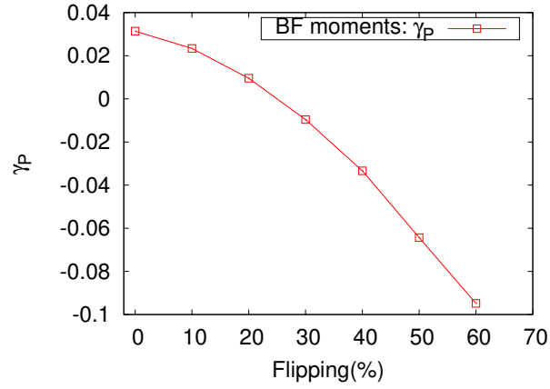
Figure 5-5: (Color online) \gamma -correlator in the form of BF's moment with different flipping fractions
