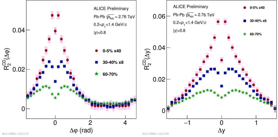
Figure 4-8: (Color online) Projected Balance function distributions of pion for Pb+Pb collisions at \sqrt{s_{NN}} = 2.76 TeV in \Delta y and \Delta\varphi for three centrality classes 0-5%, 30-40% and 60-70%.
