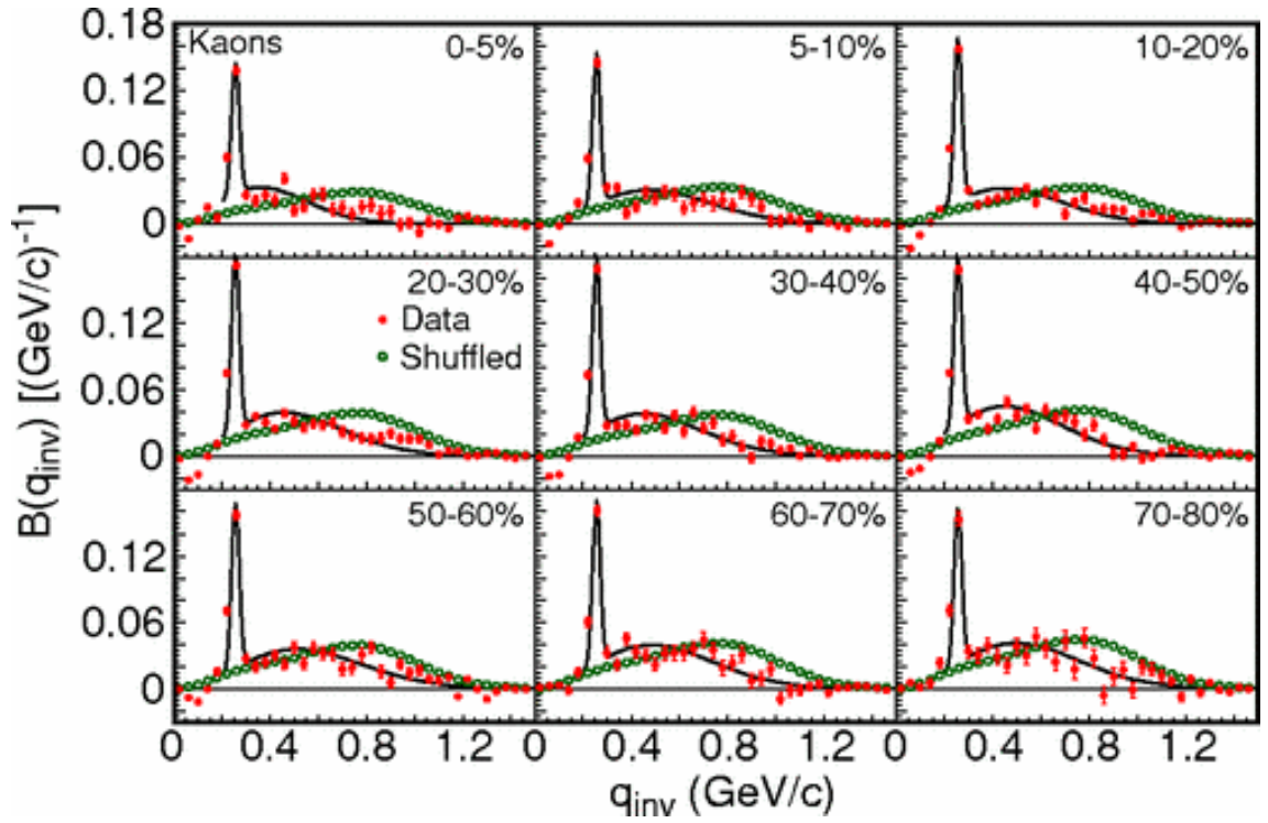
Figure 2-13: (Color online) The balance function distribution as a function of q_{inv} for identified charged kaons produced in Au+Au collisions at \sqrt{s_{NN}} = 200 GeV in nine centrality bins. Contribution from a thermal distribution and \varphi decay is represented by curves [21].
