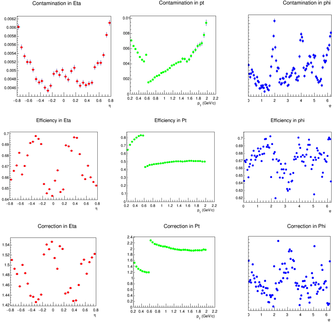
Figure 4-5: (Color online) distributions of Contamination , Efficiency and Correction for Pion in \eta , p_T and \phi at Pb+Pb collisions with \sqrt{S_{NN}} = 2.76 TeV energy.
