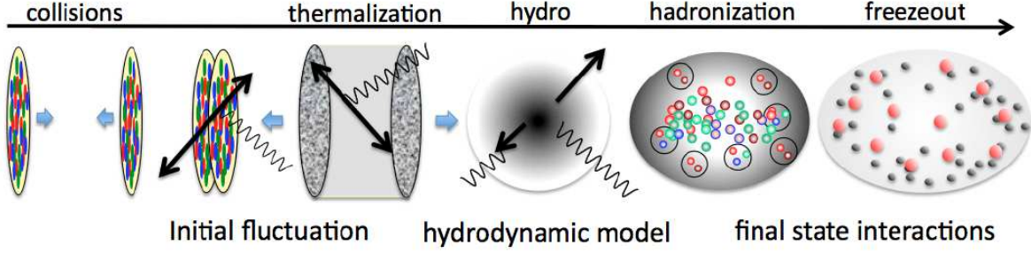
Figure 1-5: (Color online) Schematic view of the evolution of heavy ion collisions [30].
