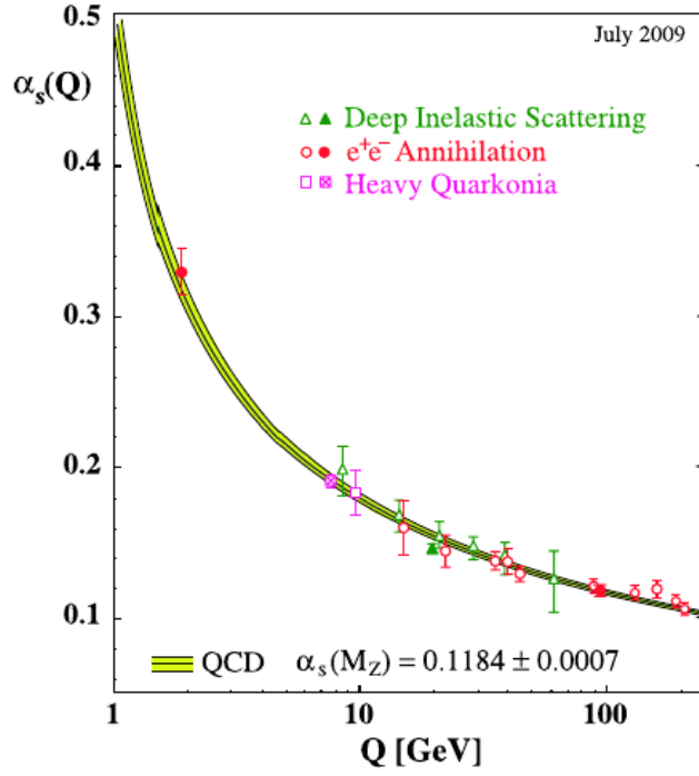
Figure 1-2: (Color online) Summary of measurements of \alpha_s as a function of momentum transfer Q . Results from N3LO QCD are shown by full symbols. Open circles are from NNLO QCD theory and Open triangles/squares are from NLO QCD theory [15].
