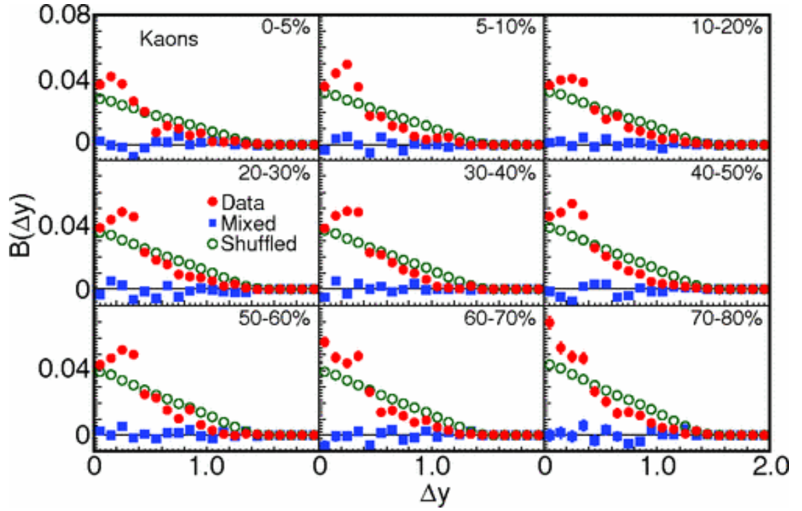
Figure 2-11: (Color online) The balance function distribution as a function of \Delta y for identified charged kaons produced in Au+Au collisions at \sqrt{s_{NN}} = 200 GeV. There is a very little dependence on centrality in kaon balance function distribution [21].
