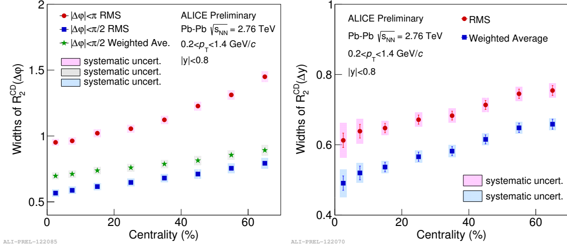
Figure 0-4: The width of the balance function for pions in terms of \langle\Delta y\rangle and \langle\Delta\phi\rangle as a function of centrality. Error bars shown are systematic. The width in \Delta\phi is shown for different ranges in \Delta\phi when projecting.
