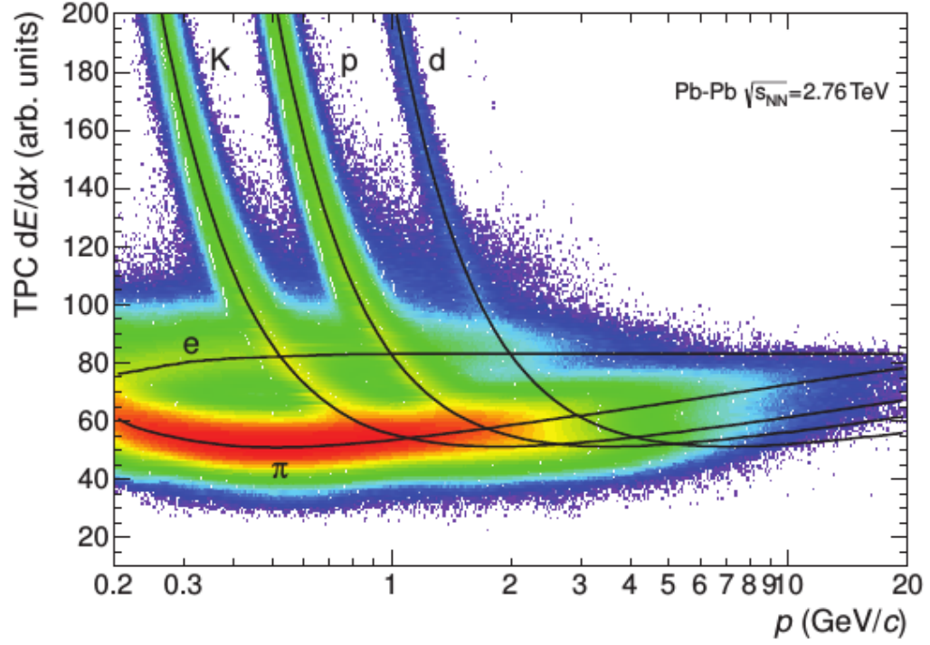
Figure 3-6: (Color online) Left: Specific energy loss ( dE/dx ) in the TPC vs. particle momentum in Pb-Pb collisions at \sqrt{s_{NN}} = 2.76 TeV. The lines show the parametrisation of the expected mean energy loss. There are no separation between pion, kaon and proton at large momentum. [8].
