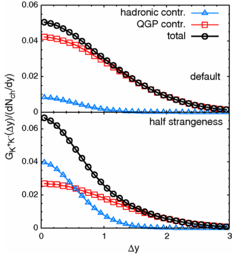
Figure 2-6: (Color online) The contribution from hadronisation in balance function of K^+K^- is small. It is shown in the upper panel. If there is half strangeness in the QGP, hadronisation contribution would be larger and balance function distribution is narrow. [17]
