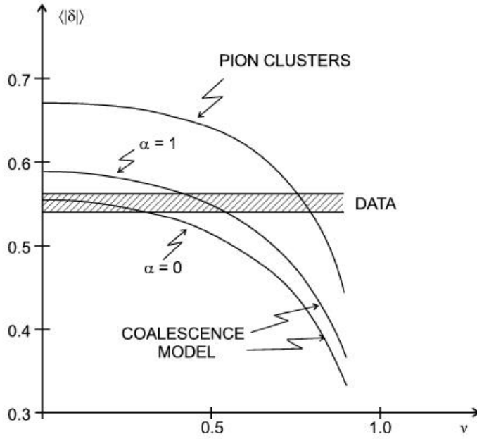
Figure 2-5: (Color online) The width of the balance function i.e. \langle |\delta| \rangle is plotted versus transverse velocity v . The width of balance function decreases when transverse velocity of clusters increase. The quantitative agreement with data is gained when transverse velocity of clusters is nearly 0.8c . [13]
