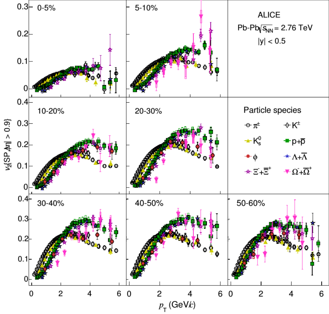
Figure 1-8: (Color online) The p_T differential v_2 for identified different particle species for different centrality collisions of Pb+Pb at \sqrt{s_{NN}} = 2.76 TeV [40].
