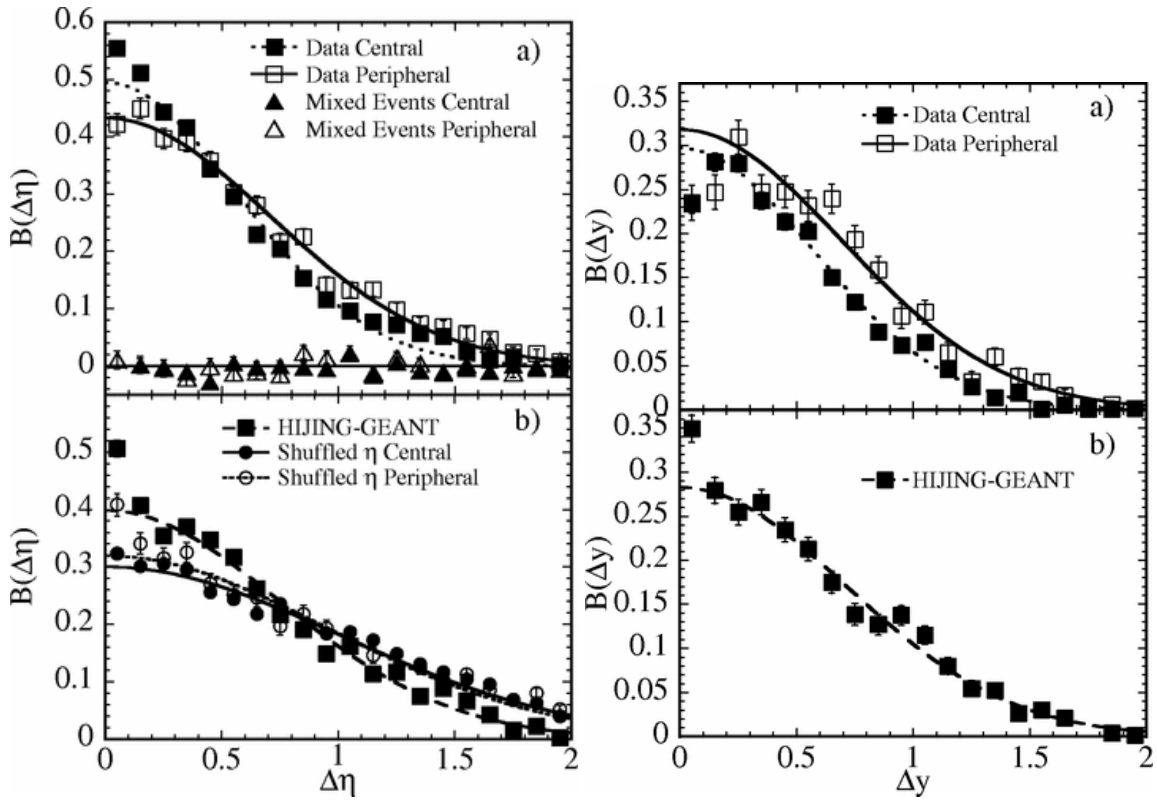
Figure 2-7: (Color online) The balance function distribution of all charged particles and identified pions for central and peripheral collisions between two Au nuclei at \sqrt{s_{NN}} = 130 GeV are shown in left and right plot respectively [18].
