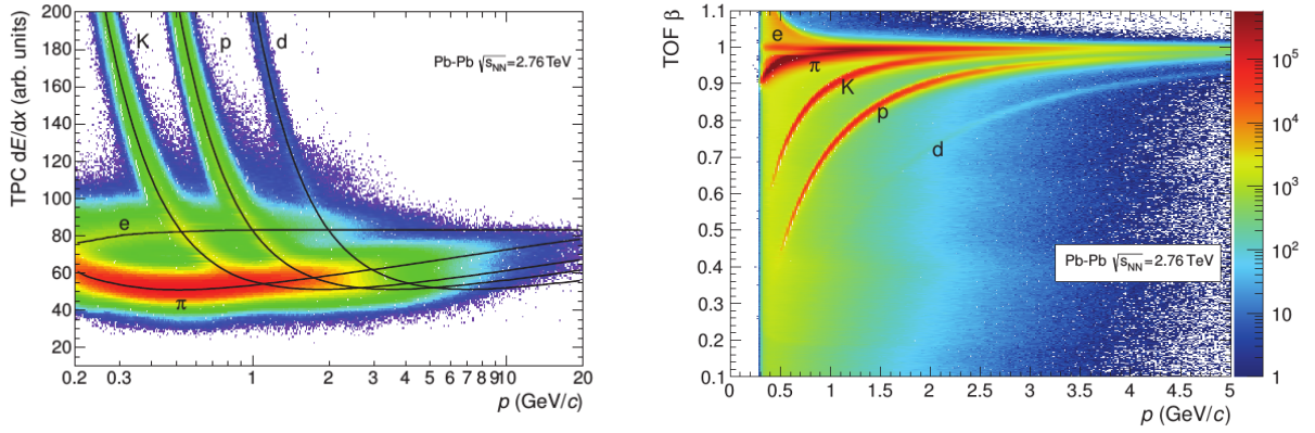
Figure 0-2: Left: Specific energy loss (dE/dx) in the TPC vs. particle momentum in Pb-Pb collisions at \sqrt{s_{NN}} = 2.76 TeV. The lines show the parametrisation of the expected mean energy loss. Right: Distribution of \beta as measured by the TOF detector as a function of momentum for particles reaching the TOF in Pb-Pb interactions. Figures are taken from [14].
