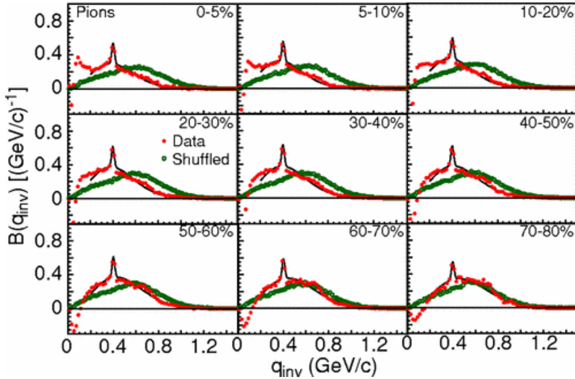
Figure 2-12: (Color online) The balance function distribution as a function of q_{inv} for identified charged pions produced in Au+Au collisions at \sqrt{s_{NN}} = 200 GeV in nine centrality bins. Contribution from a thermal distribution and K_S^0 decay is represented by curves [21].
