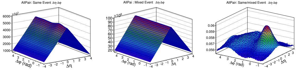
Figure 0-1: \Delta\eta-\Delta\varphi plot of same event (left) , mixed event (middle) and correlation i.e same/mixed (right)
