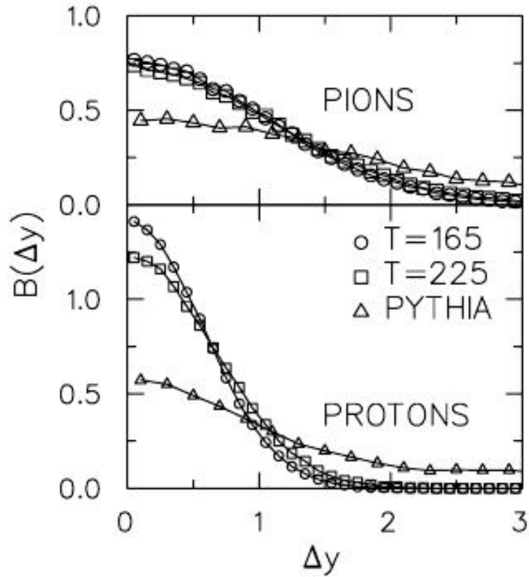
Figure 2-2: (Color online) Balance function of pions and proton for two temperature 225 and 165 MeV. Heavier particles with lower temperature are strongly correlated in rapidity. Balance function distribution of pions and protons are compared with PYTHIA simulation result. Balance function from PYTHIA has wider distribution with respect to thermally generated balance function [1].
