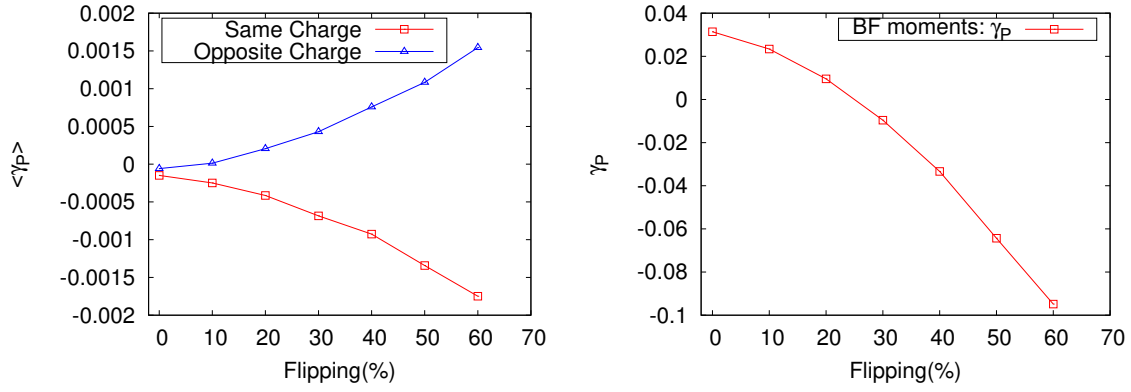
Figure 0-5: \langle \gamma_P \rangle with different flipping fractions (left plot) ; \gamma -correlator in the form of BF's moment with different flipping fractions (right plot)
