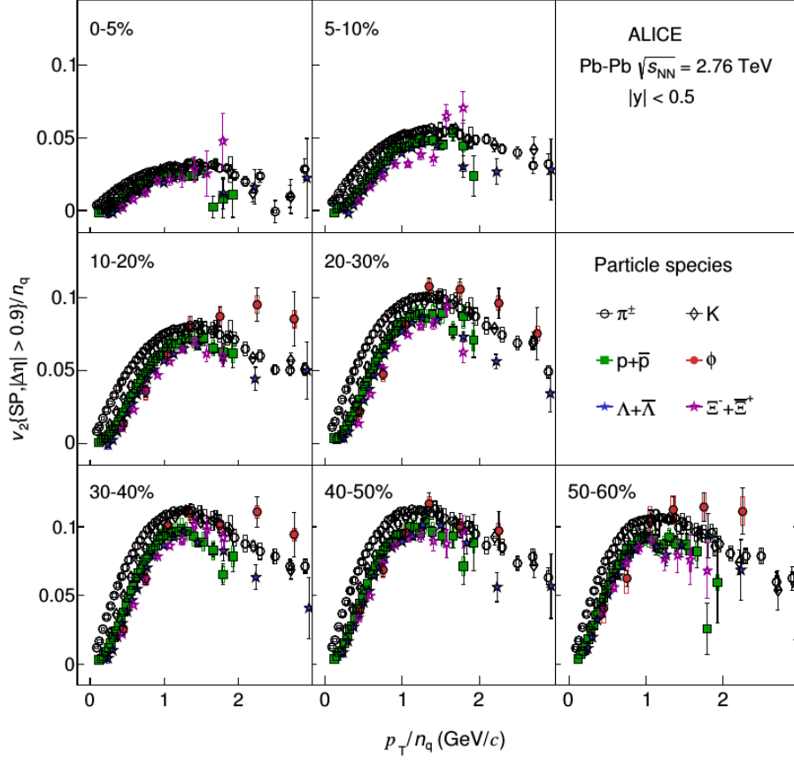
Figure 1-9: (Color online) v_2/n_q plotted as a function of p_T/n_q for \pi^\pm , K , p+\bar{p} , \phi , \Lambda+\bar{\Lambda} and \Xi^-+\Xi^+ for Pb+Pb collisions at \sqrt{s_{NN}} = 2.76 TeV [40].
