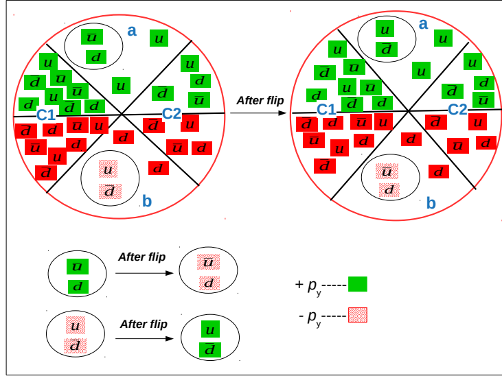
Figure 5-2: (Color online) Charge Separation mechanism shown schematically
