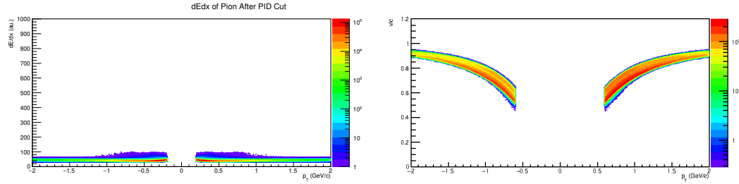
Figure 4-4: (Color online) dE/dx (left) and Beta (right) plot from TPC and TOF detector respectively for pion at Pb+Pb collisions with \sqrt{s_{NN}} = 2.76 TeV after n\sigma < 3 cut.
