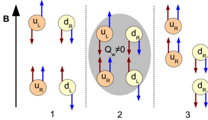
Figure 5-1: Illustrative description of chiral magnetic effect in the presence of large magnetic field. The red arrows and blue arrows represent momentum and spin of quarks respectively as shown in left panel. Up and down quarks have lowest Landau level in the presence of a large magnetic field. Initially there are equal number of right handed and left handed quarks. Now these quarks interact with a gauge field configuration with non-zero negative Q_w and a left handed up or down quark converts to right handed up or down quark by reversing the momentum direction as shown in middle panel. Because of this, there is a motion of right handed up quarks in upward direction and right handed down quarks in downward direction as shown in right panel. A charge difference of Q = 2e will be created between two sides of a plane perpendicular to the magnetic field [8].
